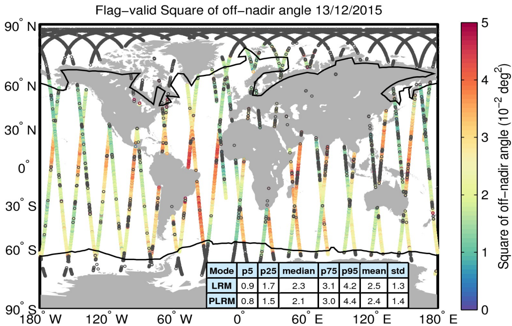
Figure 37. Geographical distribution of flag-valid mispointing data over oceans and lakes for 13/12/2015. The statistical values shown in the table refer to the mispointing in 10^{-2} deg 2 and are calculated separately for LRM and PLRM regions. Measurements taken over polar polygons have been excluded from the computation of the statistical values. The black lines mark the outer limit of the Arctic and Antarctic polar polygons. Gray circles denote negative values.
