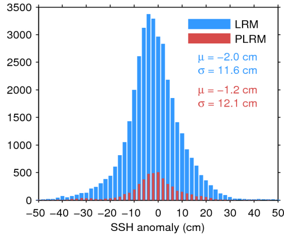
Figure 11. Histogram of science-valid SSH anomaly over oceans and lakes for LRM (blue) and PLRM (red) for 13/12/2015. The mean ( \mu ) and standard deviation ( \sigma ) are also shown. Note that values outside [-50\ 50] cm are excluded from the histogram for the sake of readability but not from the computation of \mu and \sigma .
