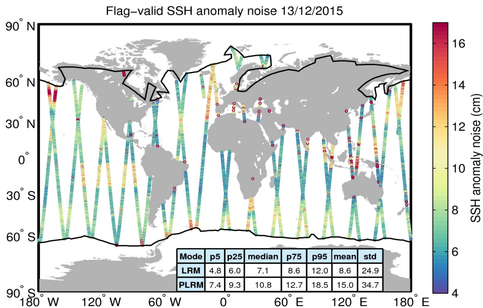
Figure 8. Geographical distribution of flag-valid 20-Hz SSH anomaly measurement noise over oceans and lakes for 13/12/2015. The statistical values shown in the table refer to the SSH anomaly noise and are calculated separately for LRM and PLRM regions. Measurements taken over polar polygons have been excluded from the computation of the statistical values. The black lines mark the outer limit of the Arctic and Antarctic polar polygons.
