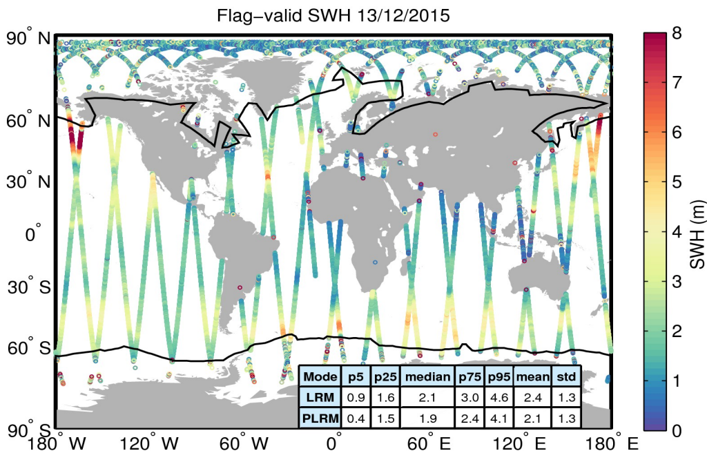
Figure 15. Geographical distribution of flag-valid SWH data over oceans and lakes for 13/12/2015. The statistical values shown in the table refer to the SWH in m and are calculated separately for LRM and PLRM regions. Measurements taken over polar polygons have been excluded from the computation of the statistical values. The black lines mark the outer limit of the Arctic and Antarctic polar polygons.
