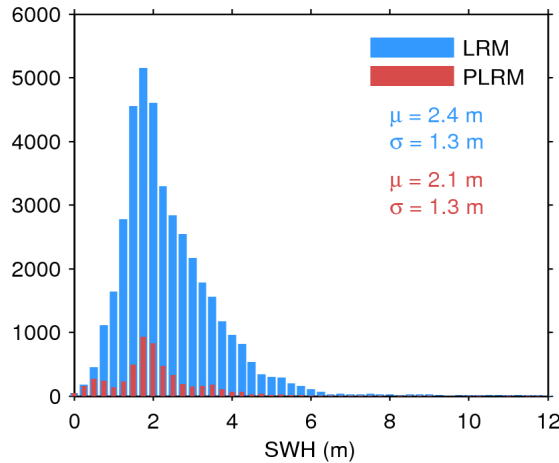
Figure 17. Histogram of flag-valid SWH over oceans and lakes for LRM (blue) and PLRM (red) for 13/12/2015. The mean ( \mu ) and standard deviation ( \sigma ) are also shown. Note that values larger than 12 m are excluded from the histogram for the sake of readability but not from the computation of \mu and \sigma .
