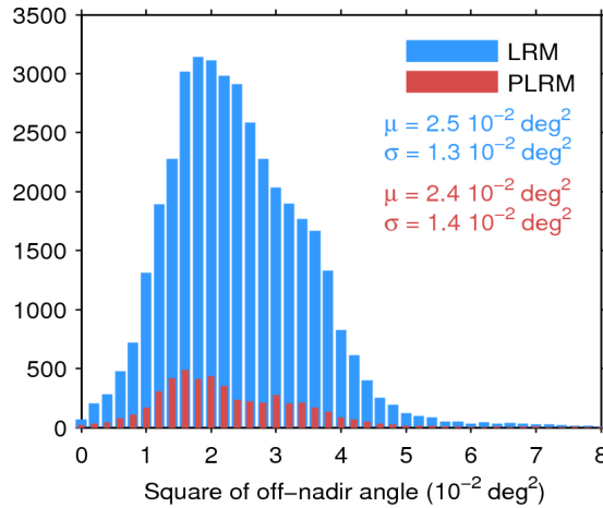
Figure 39. Histogram of flag-valid mispointing over oceans and lakes for LRM (blue) and PLRM (red) for 13/12/2015. Only positive values have been considered. The mean ( \mu ) and standard deviation ( \sigma ) are also shown. Note that values larger than 8 \cdot 10^{-2} \text{ deg}^2 are excluded from the histogram for the sake of readability but not from the computation of \mu and \sigma .
