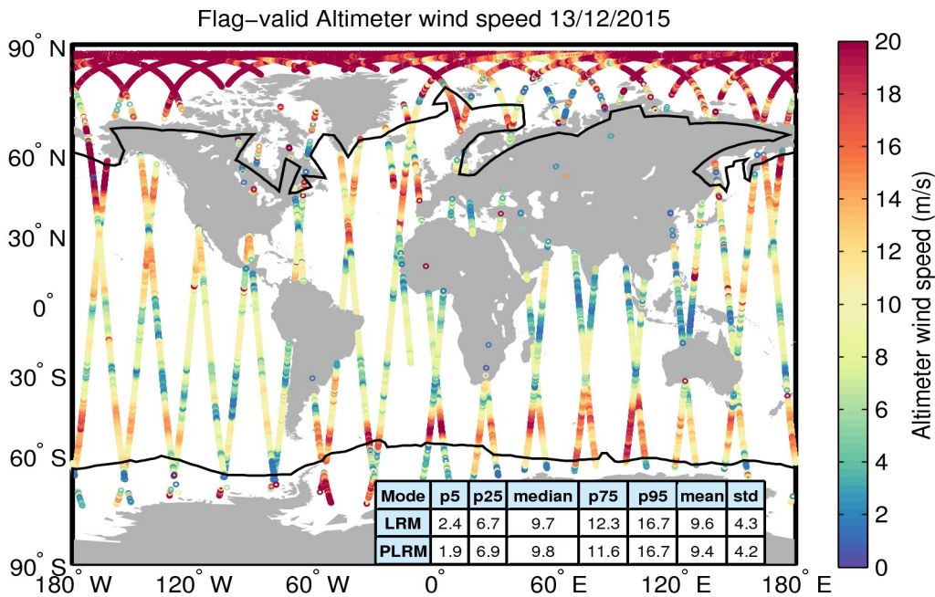
Figure 31. Geographical distribution of flag-valid wind data over oceans and lakes for 13/12/2015. The statistical values shown in the table refer to the wind in m/s and are calculated separately for LRM and PLRM regions. Measurements taken over polar polygons have been excluded from the computation of the statistical values. The black lines mark the outer limit of the Arctic and Antarctic polar polygons.
