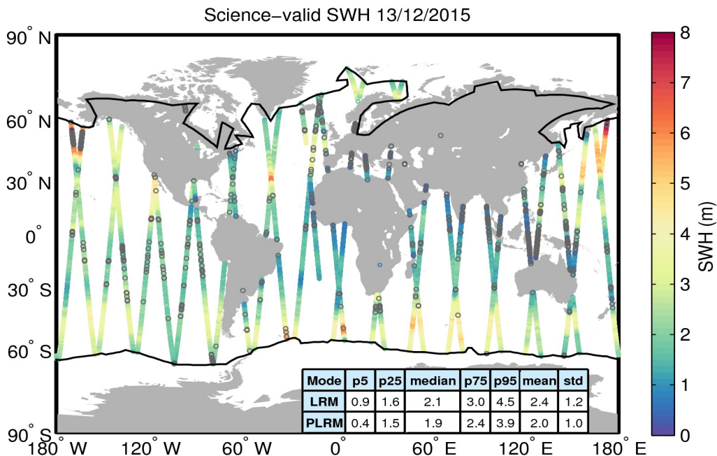
Figure 19. Geographical distribution of science-valid SWH data over oceans and lakes for 13/12/2015. The statistical values shown in the table refer to the SWH in m and are calculated separately for LRM and PLRM regions. The black lines mark the outer limit of the Arctic and Antarctic polar polygons. Gray circles denote records that have been rejected based on the editing criteria described in Table 3.
