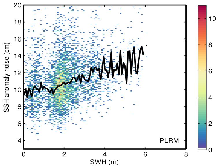
Figure 9. 2D histogram showing flag-valid SSH anomaly noise as a function of SWH for LRM (top) and PLRM (bottom) for 13/12/2015. The black line denotes the median SSH anomaly noise as a function of SWH.
