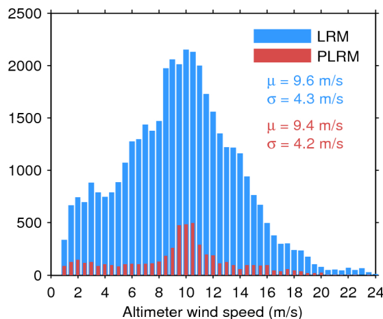
Figure 35. Histogram of science-valid wind over oceans and lakes for LRM (blue) and PLRM (red) for 13/12/2015. The mean ( \mu ) and standard deviation ( \sigma ) are also shown. Note that values larger than 24 m/s are excluded from the histogram for the sake of readability but not from the computation of \mu and \sigma .
