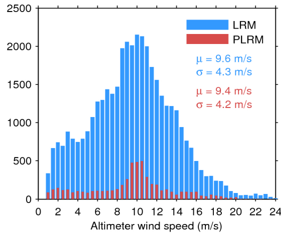
Figure 33. Histogram of flag-valid wind over oceans and lakes for LRM (blue) and PLRM (red) for 13/12/2015. The mean ( \mu ) and standard deviation ( \sigma ) are also shown. Note that values larger than 24 m/s are excluded from the histogram for the sake of readability but not from the computation of \mu and \sigma .
