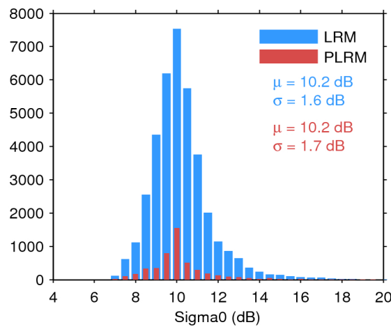
Figure 28. Histogram of science-valid sigma0 over oceans and lakes for LRM (blue) and PLRM (red) for 13/12/2015. The mean ( \mu ) and standard deviation ( \sigma ) are also shown. Note that values outside [4 20] dB are excluded from the histogram for the sake of readability but not from the computation of \mu and \sigma .
