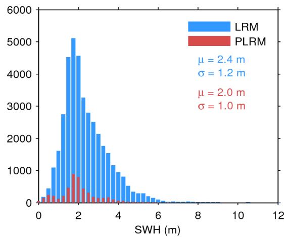
Figure 20. Histogram of science-valid SWH over oceans and lakes for LRM (blue) and PLRM (red) for 13/12/2015. The mean ( \mu ) and standard deviation ( \sigma ) are also shown. Note that values larger than 12 m are excluded from the histogram for the sake of readability but not from the computation of \mu and \sigma .
