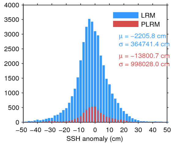
Figure 7. Histogram of flag-valid SSH anomaly over oceans and lakes for LRM (blue) and PLRM (red) for 13/12/2015. The mean ( \mu ) and standard deviation ( \sigma ) are also shown. Note that values outside [-50 50] cm are excluded from the histogram for the sake of readability but not from the computation of \mu and \sigma .
