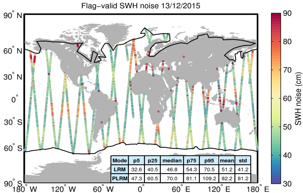
Figure 18. Geographical distribution of flag-valid 20-Hz SWH measurement noise over oceans and lakes for 13/12/2015. The statistical values shown in the table refer to the SWH noise and are calculated separately for LRM and PLRM regions. Measurements taken over polar polygons have been excluded from the computation of the statistical values. The black lines mark the outer limit of the Arctic and Antarctic polar polygons.
