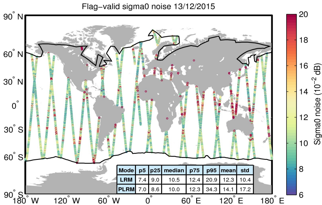
Figure 26. Geographical distribution of flag-valid 20-Hz sigma0 measurement noise over oceans and lakes for 13/12/2015. The statistical values shown in the table refer to the sigma0 noise and are calculated separately for LRM and PLRM regions. Measurements taken over polar polygons have been excluded from the computation of the statistical values. The black lines mark the outer limit of the Arctic and Antarctic polar polygons.
