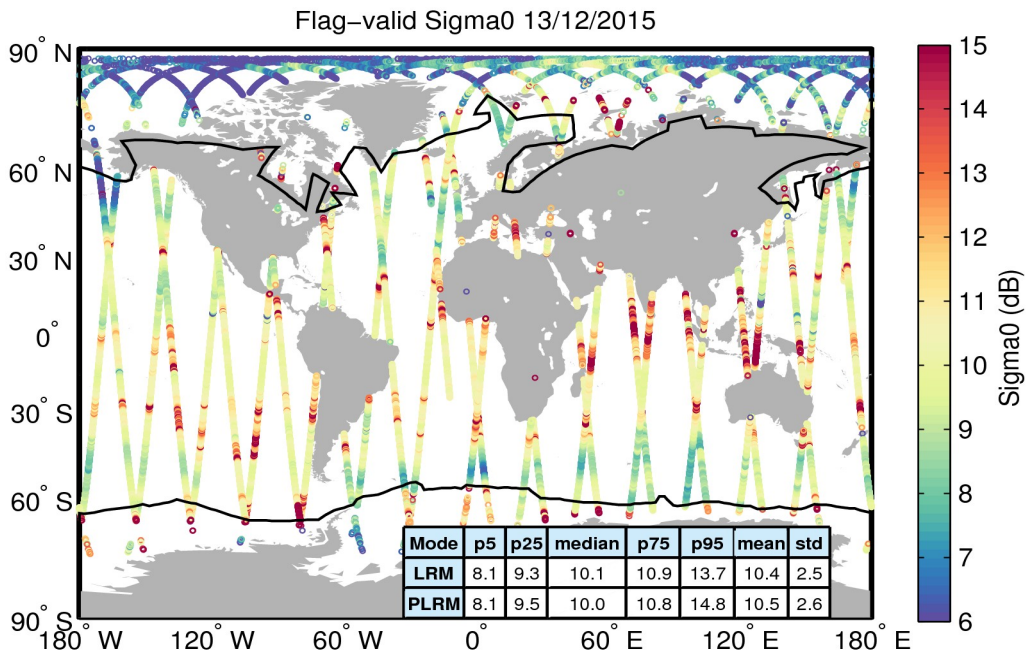
Figure 23. Geographical distribution of flag-valid sigma0 data over oceans and lakes for 13/12/2015. The statistical values shown in the table refer to the sigma0 in dB and are calculated separately for LRM and PLRM regions. Measurements taken over polar polygons have been excluded from the computation of the statistical values. The black lines mark the outer limit of the Arctic and Antarctic polar polygons.
