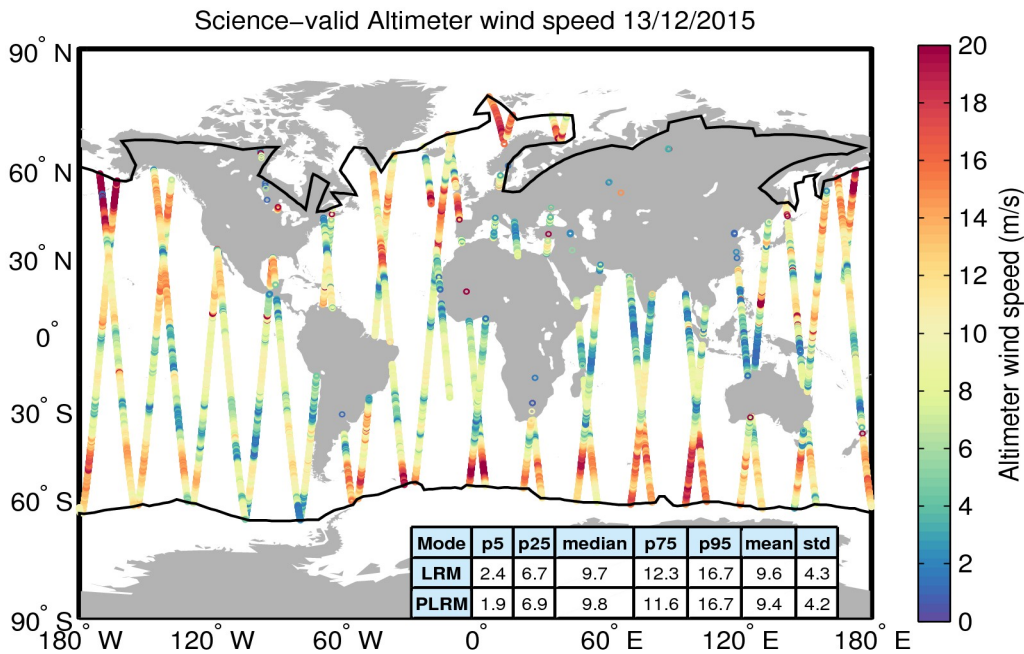
Figure 34. Geographical distribution of science-valid wind data over oceans and lakes for 13/12/2015. The statistical values shown in the table refer to the wind in m/s and are calculated separately for LRM and PLRM regions. The black lines mark the outer limit of the Arctic and Antarctic polar polygons. Gray circles denote records that have been rejected based on the editing criteria described in Table 5.
