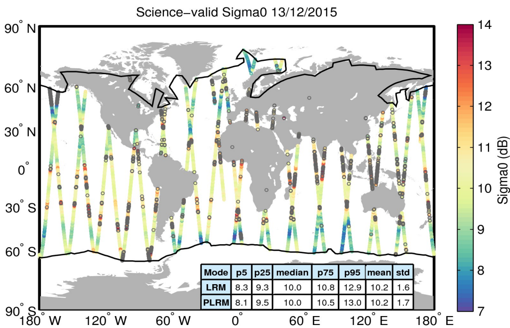
Figure 27. Geographical distribution of science-valid sigma0 data over oceans and lakes for 13/12/2015. The statistical values shown in the table refer to the sigma0 in dB and are calculated separately for LRM and PLRM regions. The black lines mark the outer limit of the Arctic and Antarctic polar polygons. Gray circles denote records that have been rejected based on the editing criteria described in Table 4.
