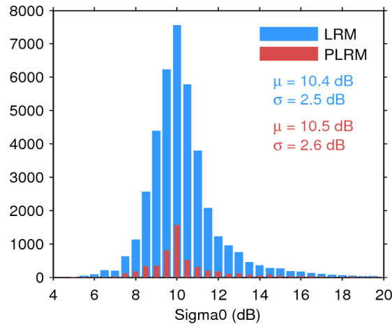
Figure 25. Histogram of flag-valid sigma0 over oceans and lakes for LRM (blue) and PLRM (red) for 13/12/2015. The mean ( \mu ) and standard deviation ( \sigma ) are also shown. Note that values outside [4 20] dB are excluded from the histogram for the sake of readability but not from the computation of \mu and \sigma .
