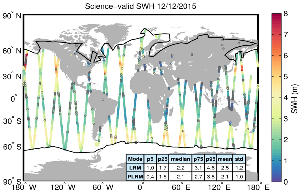
Figure 19. Geographical distribution of science-valid SWH data over oceans and lakes for 12/12/2015. The statistical values shown in the table refer to the SWH in m and are calculated separately for LRM and PLRM regions. The black lines mark the outer limit of the Arctic and Antarctic polar polygons. Gray circles denote records that have been rejected based on the editing criteria described in Table 3.
