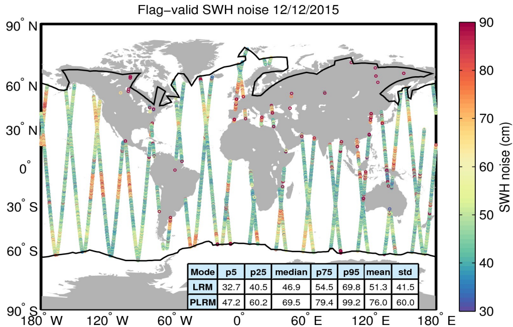
Figure 18. Geographical distribution of flag-valid 20-Hz SWH measurement noise over oceans and lakes for 12/12/2015. The statistical values shown in the table refer to the SWH noise and are calculated separately for LRM and PLRM regions. Measurements taken over polar polygons have been excluded from the computation of the statistical values. The black lines mark the outer limit of the Arctic and Antarctic polar polygons.
