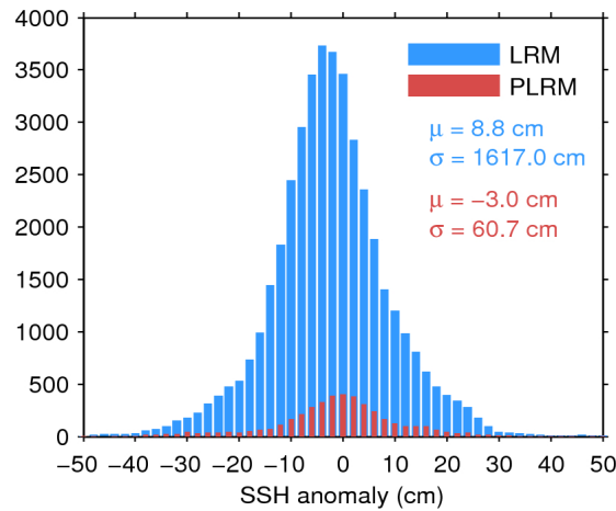
Figure 7. Histogram of flag-valid SSH anomaly over oceans and lakes for LRM (blue) and PLRM (red) for 12/12/2015. The mean ( \mu ) and standard deviation ( \sigma ) are also shown. Note that values outside [-50\ 50] cm are excluded from the histogram for the sake of readability but not from the computation of \mu and \sigma .
