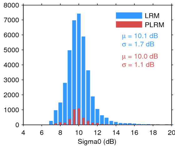
Figure 28. Histogram of science-valid sigma0 over oceans and lakes for LRM (blue) and PLRM (red) for 12/12/2015. The mean ( \mu ) and standard deviation ( \sigma ) are also shown. Note that values outside [4 20] dB are excluded from the histogram for the sake of readability but not from the computation of \mu and \sigma .
