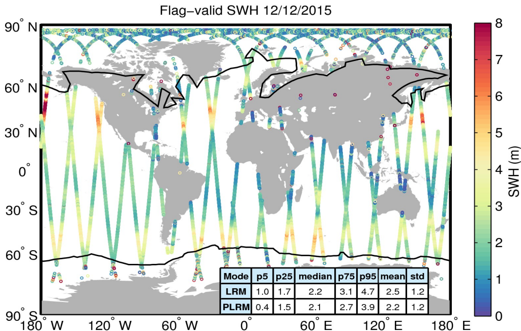
Figure 15. Geographical distribution of flag-valid SWH data over oceans and lakes for 12/12/2015. The statistical values shown in the table refer to the SWH in m and are calculated separately for LRM and PLRM regions. Measurements taken over polar polygons have been excluded from the computation of the statistical values. The black lines mark the outer limit of the Arctic and Antarctic polar polygons.
