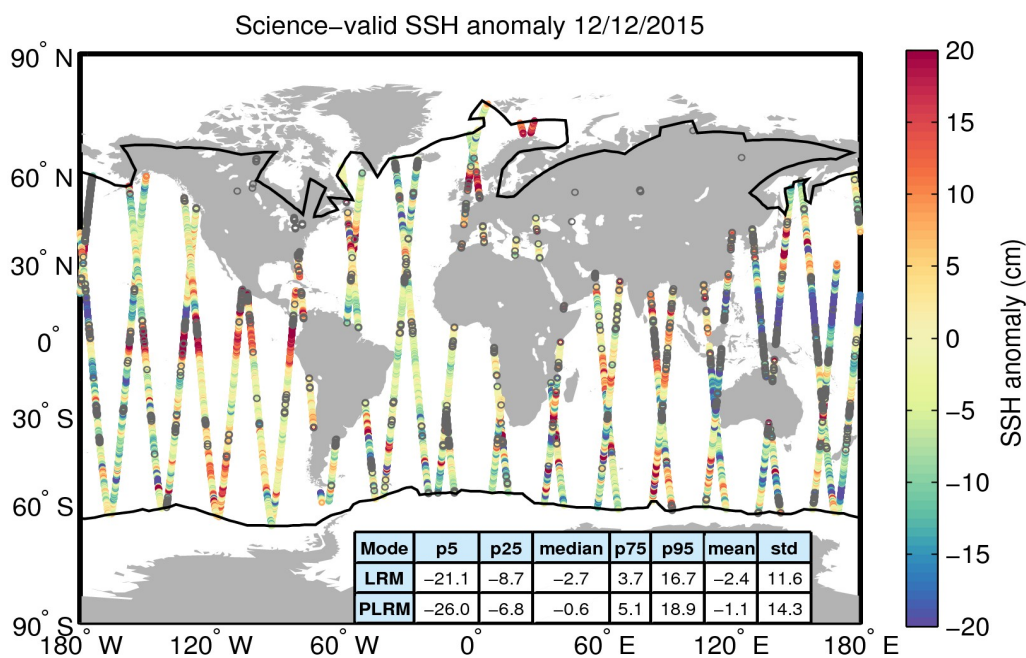
Figure 10. Geographical distribution of science-valid SSH anomaly data over oceans and lakes for 12/12/2015. The statistical values shown in the table refer to the SSH anomaly in cm and are calculated separately for LRM and PLRM regions. The black lines mark the outer limit of the Arctic and Antarctic polar polygons. Gray circles denote records that have been rejected based on the editing criteria described in Table 2.
