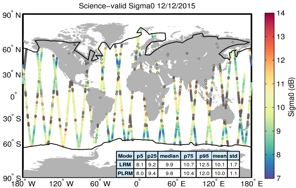
Figure 27. Geographical distribution of science-valid sigma0 data over oceans and lakes for 12/12/2015. The statistical values shown in the table refer to the sigma0 in dB and are calculated separately for LRM and PLRM regions. The black lines mark the outer limit of the Arctic and Antarctic polar polygons. Gray circles denote records that have been rejected based on the editing criteria described in Table 4.
