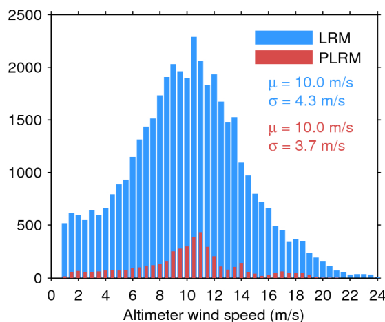
Figure 35. Histogram of science-valid wind over oceans and lakes for LRM (blue) and PLRM (red) for 12/12/2015. The mean ( \mu ) and standard deviation ( \sigma ) are also shown. Note that values larger than 24 m/s are excluded from the histogram for the sake of readability but not from the computation of \mu and \sigma .
