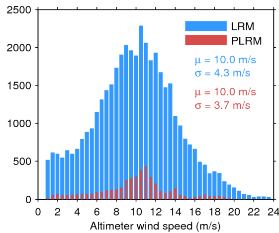
Figure 33. Histogram of flag-valid wind over oceans and lakes for LRM (blue) and PLRM (red) for 12/12/2015. The mean ( \mu ) and standard deviation ( \sigma ) are also shown. Note that values larger than 24 m/s are excluded from the histogram for the sake of readability but not from the computation of \mu and \sigma .
