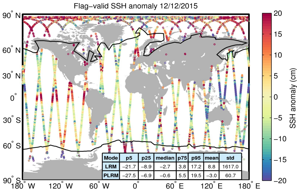
Figure 5. Geographical distribution of flag-valid 1-Hz SSH anomaly data over oceans and lakes for 12/12/2015. The statistical values shown in the table refer to the SSH anomaly in cm and are calculated separately for LRM and PLRM regions. Measurements taken over polar polygons have been excluded from the computation of the statistical values. The black lines mark the outer limit of the Arctic and Antarctic polar polygons.
