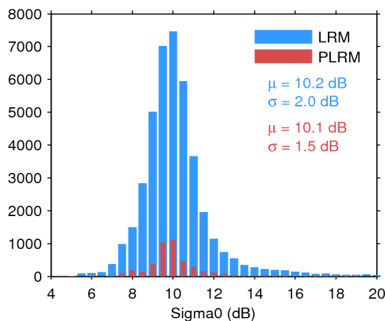
Figure 25. Histogram of flag-valid sigma0 over oceans and lakes for LRM (blue) and PLRM (red) for 12/12/2015. The mean ( \mu ) and standard deviation ( \sigma ) are also shown. Note that values outside [4 20] dB are excluded from the histogram for the sake of readability but not from the computation of \mu and \sigma .
