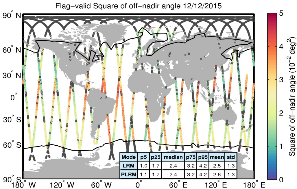
Figure 37. Geographical distribution of flag-valid mispointing data over oceans and lakes for 12/12/2015. The statistical values shown in the table refer to the mispointing in 10^{-2} deg 2 and are calculated separately for LRM and PLRM regions. Measurements taken over polar polygons have been excluded from the computation of the statistical values. The black lines mark the outer limit of the Arctic and Antarctic polar polygons. Gray circles denote negative values.
