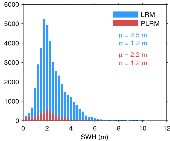
Figure 17. Histogram of flag-valid SWH over oceans and lakes for LRM (blue) and PLRM (red) for 12/12/2015. The mean ( \mu ) and standard deviation ( \sigma ) are also shown. Note that values larger than 12 m are excluded from the histogram for the sake of readability but not from the computation of \mu and \sigma .
