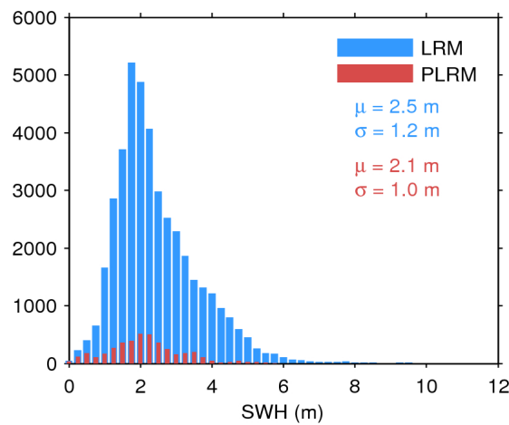
Figure 20. Histogram of science-valid SWH over oceans and lakes for LRM (blue) and PLRM (red) for 12/12/2015. The mean ( \mu ) and standard deviation ( \sigma ) are also shown. Note that values larger than 12 m are excluded from the histogram for the sake of readability but not from the computation of \mu and \sigma .
