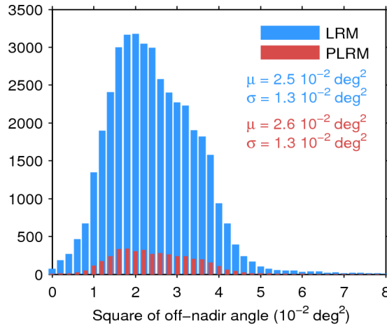
Figure 39. Histogram of flag-valid mispointing over oceans and lakes for LRM (blue) and PLRM (red) for 12/12/2015. Only positive values have been considered. The mean ( \mu ) and standard deviation ( \sigma ) are also shown. Note that values larger than 8 \cdot 10^{-2} \text{ deg}^2 are excluded from the histogram for the sake of readability but not from the computation of \mu and \sigma .
