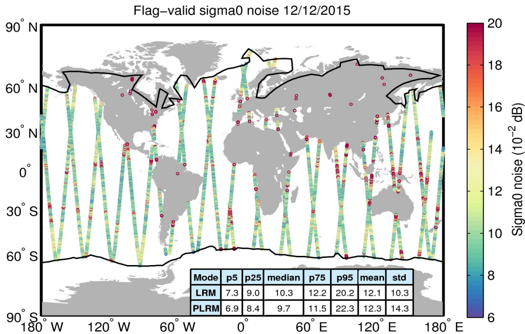
Figure 26. Geographical distribution of flag-valid 20-Hz sigma0 measurement noise over oceans and lakes for 12/12/2015. The statistical values shown in the table refer to the sigma0 noise and are calculated separately for LRM and PLRM regions. Measurements taken over polar polygons have been excluded from the computation of the statistical values. The black lines mark the outer limit of the Arctic and Antarctic polar polygons.
