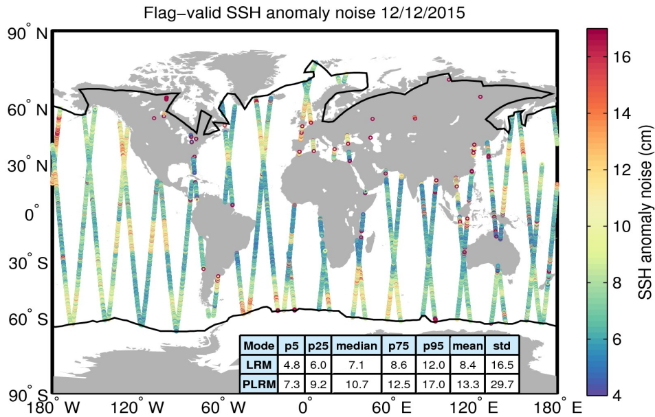
Figure 8. Geographical distribution of flag-valid 20-Hz SSH anomaly measurement noise over oceans and lakes for 12/12/2015. The statistical values shown in the table refer to the SSH anomaly noise and are calculated separately for LRM and PLRM regions. Measurements taken over polar polygons have been excluded from the computation of the statistical values. The black lines mark the outer limit of the Arctic and Antarctic polar polygons.
