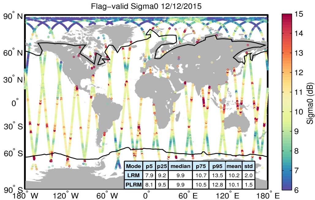
Figure 23. Geographical distribution of flag-valid sigma0 data over oceans and lakes for 12/12/2015. The statistical values shown in the table refer to the sigma0 in dB and are calculated separately for LRM and PLRM regions. Measurements taken over polar polygons have been excluded from the computation of the statistical values. The black lines mark the outer limit of the Arctic and Antarctic polar polygons.
