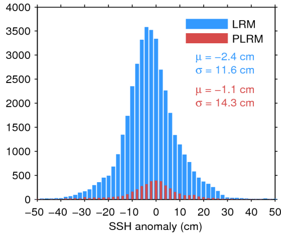
Figure 11. Histogram of science-valid SSH anomaly over oceans and lakes for LRM (blue) and PLRM (red) for 12/12/2015. The mean ( \mu ) and standard deviation ( \sigma ) are also shown. Note that values outside [-50 50] cm are excluded from the histogram for the sake of readability but not from the computation of \mu and \sigma .
