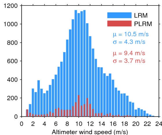
Figure 35. Histogram of science-valid wind over oceans and lakes for LRM (blue) and PLRM (red) for 08/12/2015. The mean ( \mu ) and standard deviation ( \sigma ) are also shown. Note that values larger than 24 m/s are excluded from the histogram for the sake of readability but not from the computation of \mu and \sigma .
