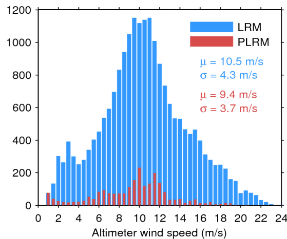
Figure 33. Histogram of flag-valid wind over oceans and lakes for LRM (blue) and PLRM (red) for 08/12/2015. The mean ( \mu ) and standard deviation ( \sigma ) are also shown. Note that values larger than 24 m/s are excluded from the histogram for the sake of readability but not from the computation of \mu and \sigma .
