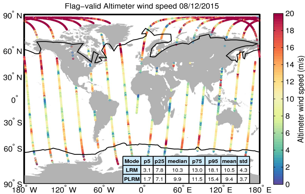
Figure 31. Geographical distribution of flag-valid wind data over oceans and lakes for 08/12/2015. The statistical values shown in the table refer to the wind in m/s and are calculated separately for LRM and PLRM regions. Measurements taken over polar polygons have been excluded from the computation of the statistical values. The black lines mark the outer limit of the Arctic and Antarctic polar polygons.
