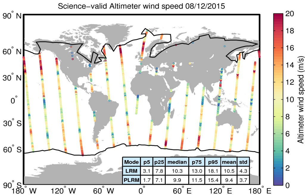
Figure 34. Geographical distribution of science-valid wind data over oceans and lakes for 08/12/2015. The statistical values shown in the table refer to the wind in m/s and are calculated separately for LRM and PLRM regions. The black lines mark the outer limit of the Arctic and Antarctic polar polygons. Gray circles denote records that have been rejected based on the editing criteria described in Table 5.
