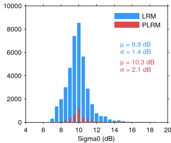
Figure 28. Histogram of science-valid sigma0 over oceans and lakes for LRM (blue) and PLRM (red) for 08/12/2015. The mean ( \mu ) and standard deviation ( \sigma ) are also shown. Note that values outside [4 20] dB are excluded from the histogram for the sake of readability but not from the computation of \mu and \sigma .
