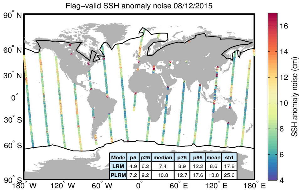
Figure 8. Geographical distribution of flag-valid 20-Hz SSH anomaly measurement noise over oceans and lakes for 08/12/2015. The statistical values shown in the table refer to the SSH anomaly noise and are calculated separately for LRM and PLRM regions. Measurements taken over polar polygons have been excluded from the computation of the statistical values. The black lines mark the outer limit of the Arctic and Antarctic polar polygons.
