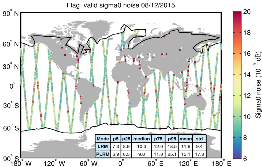
Figure 26. Geographical distribution of flag-valid 20-Hz sigma0 measurement noise over oceans and lakes for 08/12/2015. The statistical values shown in the table refer to the sigma0 noise and are calculated separately for LRM and PLRM regions. Measurements taken over polar polygons have been excluded from the computation of the statistical values. The black lines mark the outer limit of the Arctic and Antarctic polar polygons.
