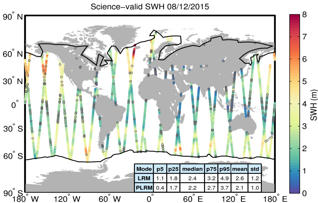
Figure 19. Geographical distribution of science-valid SWH data over oceans and lakes for 08/12/2015. The statistical values shown in the table refer to the SWH in m and are calculated separately for LRM and PLRM regions. The black lines mark the outer limit of the Arctic and Antarctic polar polygons. Gray circles denote records that have been rejected based on the editing criteria described in Table 3.
