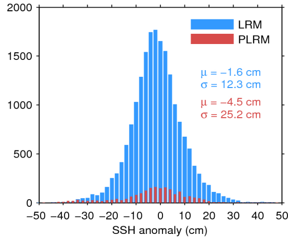
Figure 11. Histogram of science-valid SSH anomaly over oceans and lakes for LRM (blue) and PLRM (red) for 08/12/2015. The mean ( \mu ) and standard deviation ( \sigma ) are also shown. Note that values outside [-50\ 50] cm are excluded from the histogram for the sake of readability but not from the computation of \mu and \sigma .
