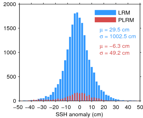
Figure 7. Histogram of flag-valid SSH anomaly over oceans and lakes for LRM (blue) and PLRM (red) for 08/12/2015. The mean ( \mu ) and standard deviation ( \sigma ) are also shown. Note that values outside [-50 50] cm are excluded from the histogram for the sake of readability but not from the computation of \mu and \sigma .
