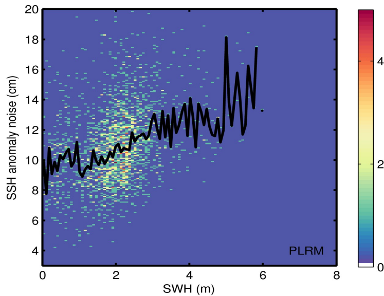
Figure 9. 2D histogram showing flag-valid SSH anomaly noise as a function of SWH for LRM (top) and PLRM (bottom) for 08/12/2015. The black line denotes the median SSH anomaly noise as a function of SWH.
