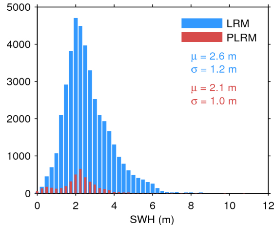
Figure 17. Histogram of flag-valid SWH over oceans and lakes for LRM (blue) and PLRM (red) for 08/12/2015. The mean ( \mu ) and standard deviation ( \sigma ) are also shown. Note that values larger than 12 m are excluded from the histogram for the sake of readability but not from the computation of \mu and \sigma .
