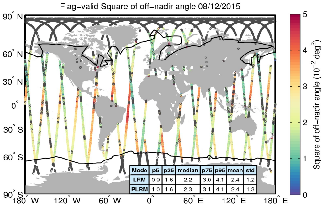
Figure 37. Geographical distribution of flag-valid mispointing data over oceans and lakes for 08/12/2015. The statistical values shown in the table refer to the mispointing in 10^{-2} deg 2 and are calculated separately for LRM and PLRM regions. Measurements taken over polar polygons have been excluded from the computation of the statistical values. The black lines mark the outer limit of the Arctic and Antarctic polar polygons. Gray circles denote negative values.
