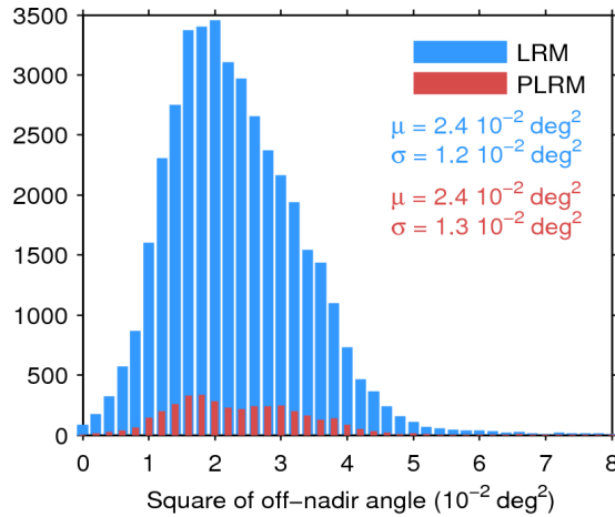
Figure 39. Histogram of flag-valid mispointing over oceans and lakes for LRM (blue) and PLRM (red) for 08/12/2015. Only positive values have been considered. The mean ( \mu ) and standard deviation ( \sigma ) are also shown. Note that values larger than 8 \cdot 10^{-2} \text{ deg}^2 are excluded from the histogram for the sake of readability but not from the computation of \mu and \sigma .
