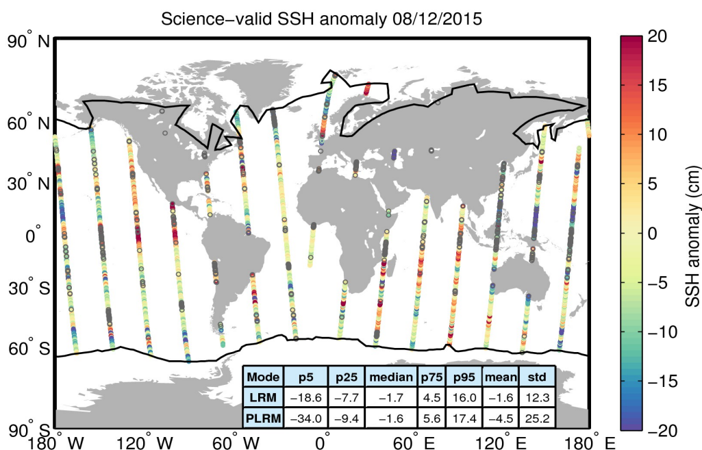
Figure 10. Geographical distribution of science-valid SSH anomaly data over oceans and lakes for 08/12/2015. The statistical values shown in the table refer to the SSH anomaly in cm and are calculated separately for LRM and PLRM regions. The black lines mark the outer limit of the Arctic and Antarctic polar polygons. Gray circles denote records that have been rejected based on the editing criteria described in Table 2.
