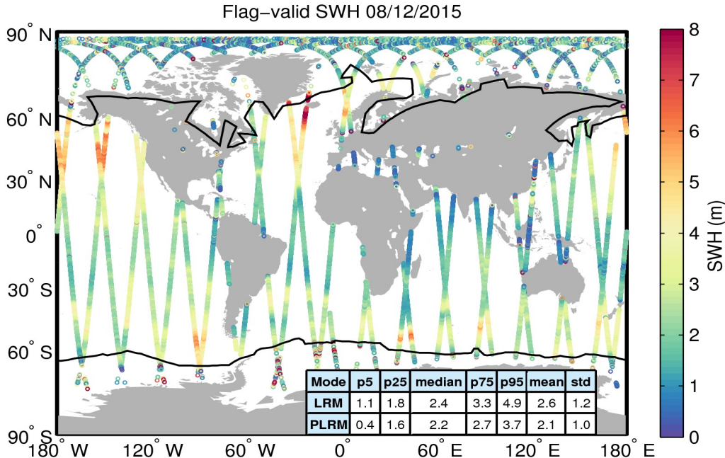
Figure 15. Geographical distribution of flag-valid SWH data over oceans and lakes for 08/12/2015. The statistical values shown in the table refer to the SWH in m and are calculated separately for LRM and PLRM regions. Measurements taken over polar polygons have been excluded from the computation of the statistical values. The black lines mark the outer limit of the Arctic and Antarctic polar polygons.
