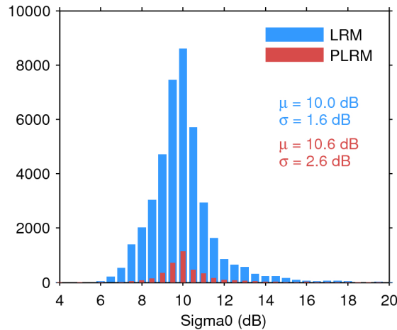
Figure 25. Histogram of flag-valid sigma0 over oceans and lakes for LRM (blue) and PLRM (red) for 08/12/2015. The mean ( \mu ) and standard deviation ( \sigma ) are also shown. Note that values outside [4 20] dB are excluded from the histogram for the sake of readability but not from the computation of \mu and \sigma .
