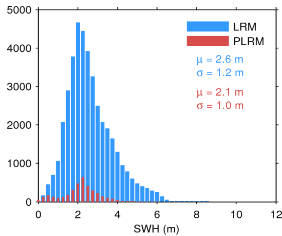
Figure 20. Histogram of science-valid SWH over oceans and lakes for LRM (blue) and PLRM (red) for 08/12/2015. The mean ( \mu ) and standard deviation ( \sigma ) are also shown. Note that values larger than 12 m are excluded from the histogram for the sake of readability but not from the computation of \mu and \sigma .
