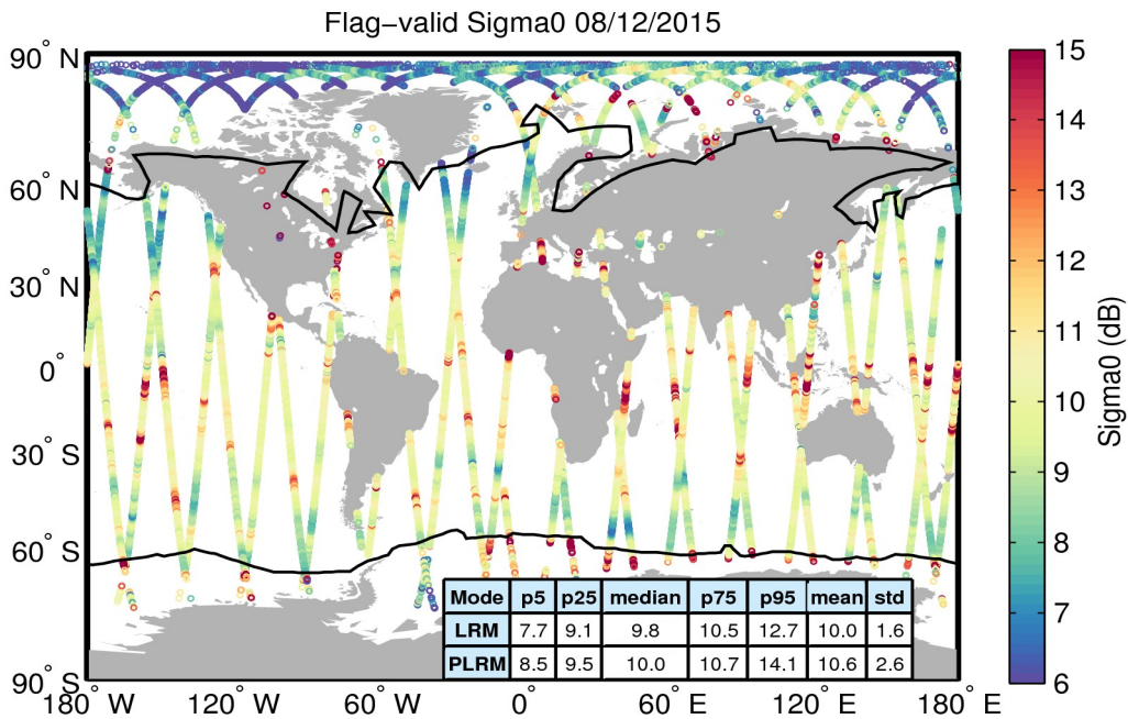
Figure 23. Geographical distribution of flag-valid sigma0 data over oceans and lakes for 08/12/2015. The statistical values shown in the table refer to the sigma0 in dB and are calculated separately for LRM and PLRM regions. Measurements taken over polar polygons have been excluded from the computation of the statistical values. The black lines mark the outer limit of the Arctic and Antarctic polar polygons.
