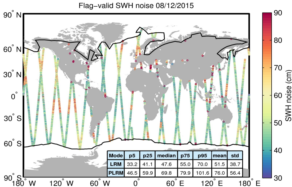
Figure 18. Geographical distribution of flag-valid 20-Hz SWH measurement noise over oceans and lakes for 08/12/2015. The statistical values shown in the table refer to the SWH noise and are calculated separately for LRM and PLRM regions. Measurements taken over polar polygons have been excluded from the computation of the statistical values. The black lines mark the outer limit of the Arctic and Antarctic polar polygons.
