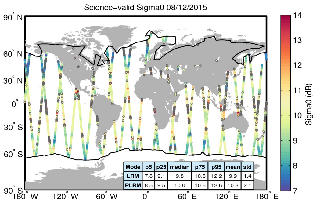
Figure 27. Geographical distribution of science-valid sigma0 data over oceans and lakes for 08/12/2015. The statistical values shown in the table refer to the sigma0 in dB and are calculated separately for LRM and PLRM regions. The black lines mark the outer limit of the Arctic and Antarctic polar polygons. Gray circles denote records that have been rejected based on the editing criteria described in Table 4.
