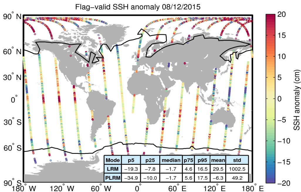
Figure 5. Geographical distribution of flag-valid 1-Hz SSH anomaly data over oceans and lakes for 08/12/2015. The statistical values shown in the table refer to the SSH anomaly in cm and are calculated separately for LRM and PLRM regions. Measurements taken over polar polygons have been excluded from the computation of the statistical values. The black lines mark the outer limit of the Arctic and Antarctic polar polygons.
