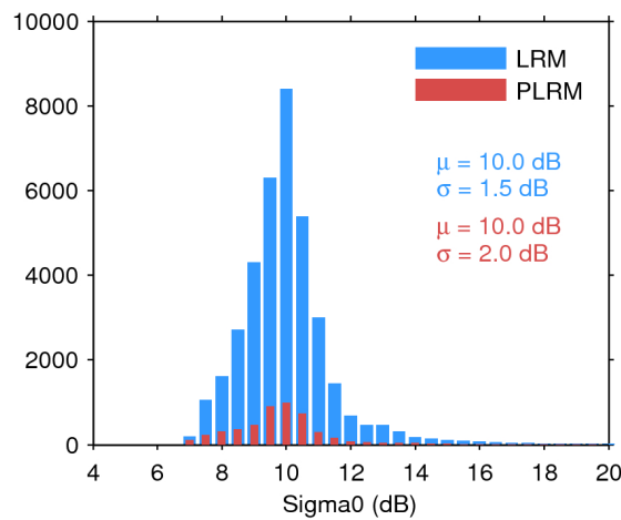
Figure 28. Histogram of science-valid sigma0 over oceans and lakes for LRM (blue) and PLRM (red) for 07/12/2015. The mean ( \mu ) and standard deviation ( \sigma ) are also shown. Note that values outside [4 20] dB are excluded from the histogram for the sake of readability but not from the computation of \mu and \sigma .
