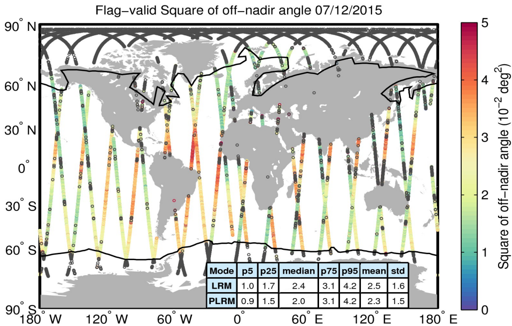
Figure 37. Geographical distribution of flag-valid mispointing data over oceans and lakes for 07/12/2015. The statistical values shown in the table refer to the mispointing in 10^{-2} deg 2 and are calculated separately for LRM and PLRM regions. Measurements taken over polar polygons have been excluded from the computation of the statistical values. The black lines mark the outer limit of the Arctic and Antarctic polar polygons. Gray circles denote negative values.
