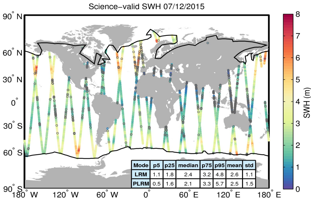
Figure 19. Geographical distribution of science-valid SWH data over oceans and lakes for 07/12/2015. The statistical values shown in the table refer to the SWH in m and are calculated separately for LRM and PLRM regions. The black lines mark the outer limit of the Arctic and Antarctic polar polygons. Gray circles denote records that have been rejected based on the editing criteria described in Table 3.
