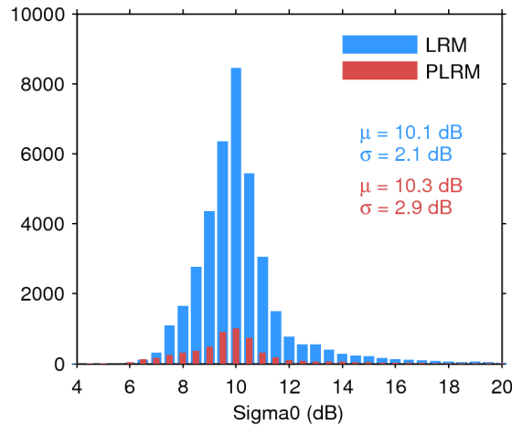
Figure 25. Histogram of flag-valid sigma0 over oceans and lakes for LRM (blue) and PLRM (red) for 07/12/2015. The mean ( \mu ) and standard deviation ( \sigma ) are also shown. Note that values outside [4 20] dB are excluded from the histogram for the sake of readability but not from the computation of \mu and \sigma .
