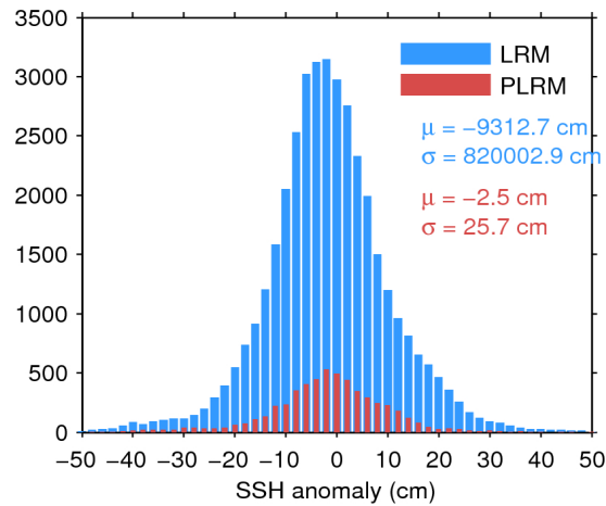
Figure 7. Histogram of flag-valid SSH anomaly over oceans and lakes for LRM (blue) and PLRM (red) for 07/12/2015. The mean ( \mu ) and standard deviation ( \sigma ) are also shown. Note that values outside [-50 50] cm are excluded from the histogram for the sake of readability but not from the computation of \mu and \sigma .
