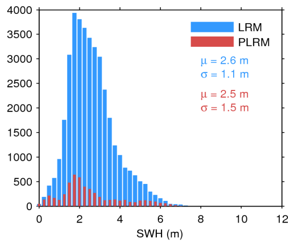
Figure 20. Histogram of science-valid SWH over oceans and lakes for LRM (blue) and PLRM (red) for 07/12/2015. The mean ( \mu ) and standard deviation ( \sigma ) are also shown. Note that values larger than 12 m are excluded from the histogram for the sake of readability but not from the computation of \mu and \sigma .
