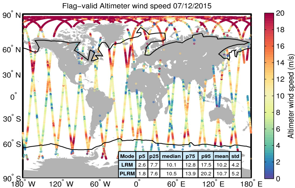
Figure 31. Geographical distribution of flag-valid wind data over oceans and lakes for 07/12/2015. The statistical values shown in the table refer to the wind in m/s and are calculated separately for LRM and PLRM regions. Measurements taken over polar polygons have been excluded from the computation of the statistical values. The black lines mark the outer limit of the Arctic and Antarctic polar polygons.
