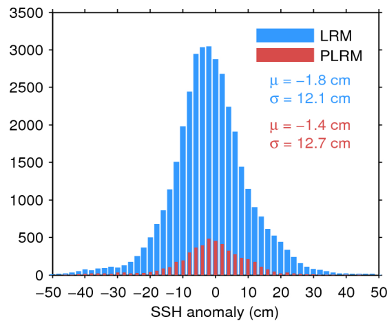
Figure 11. Histogram of science-valid SSH anomaly over oceans and lakes for LRM (blue) and PLRM (red) for 07/12/2015. The mean ( \mu ) and standard deviation ( \sigma ) are also shown. Note that values outside [-50 50] cm are excluded from the histogram for the sake of readability but not from the computation of \mu and \sigma .
