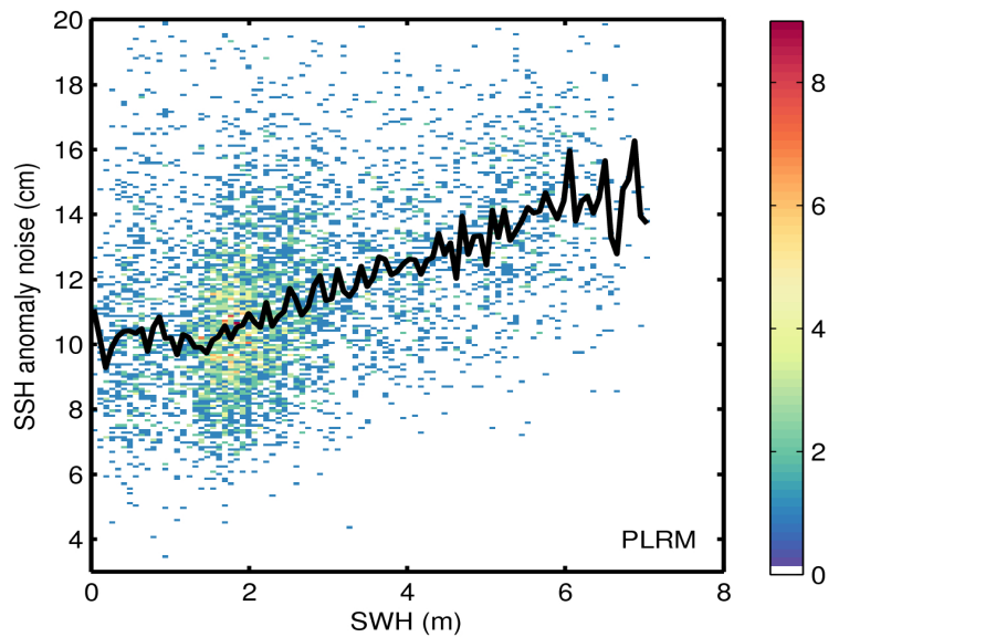
Figure 9. 2D histogram showing flag-valid SSH anomaly noise as a function of SWH for LRM (top) and PLRM (bottom) for 07/12/2015. The black line denotes the median SSH anomaly noise as a function of SWH.
