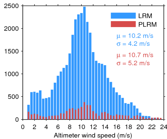
Figure 33. Histogram of flag-valid wind over oceans and lakes for LRM (blue) and PLRM (red) for 07/12/2015. The mean ( \mu ) and standard deviation ( \sigma ) are also shown. Note that values larger than 24 m/s are excluded from the histogram for the sake of readability but not from the computation of \mu and \sigma .
