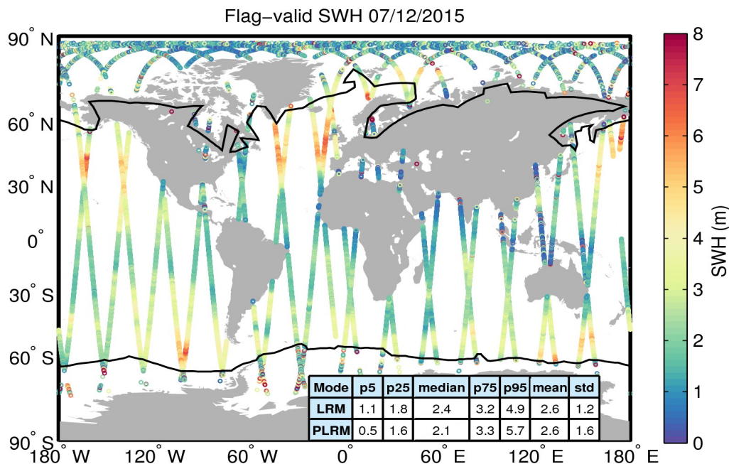
Figure 15. Geographical distribution of flag-valid SWH data over oceans and lakes for 07/12/2015. The statistical values shown in the table refer to the SWH in m and are calculated separately for LRM and PLRM regions. Measurements taken over polar polygons have been excluded from the computation of the statistical values. The black lines mark the outer limit of the Arctic and Antarctic polar polygons.
