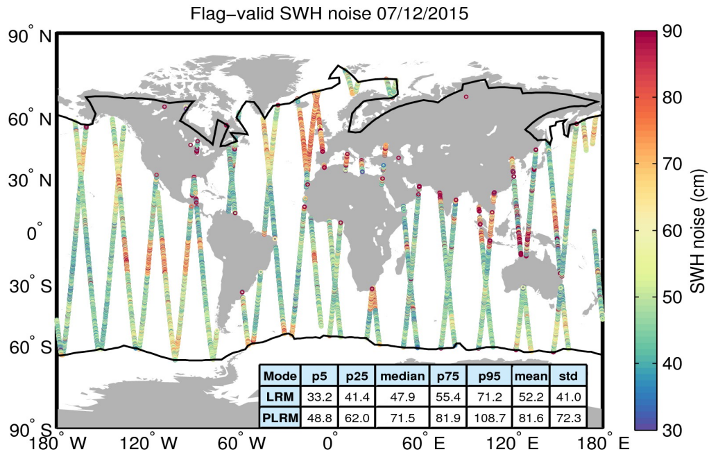
Figure 18. Geographical distribution of flag-valid 20-Hz SWH measurement noise over oceans and lakes for 07/12/2015. The statistical values shown in the table refer to the SWH noise and are calculated separately for LRM and PLRM regions. Measurements taken over polar polygons have been excluded from the computation of the statistical values. The black lines mark the outer limit of the Arctic and Antarctic polar polygons.
