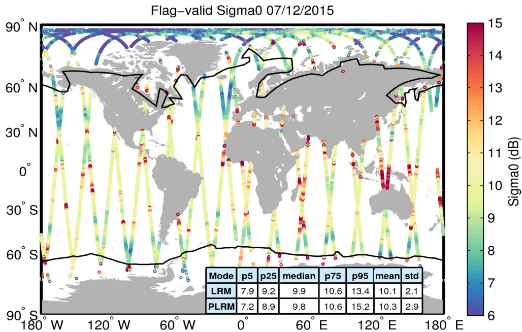
Figure 23. Geographical distribution of flag-valid sigma0 data over oceans and lakes for 07/12/2015. The statistical values shown in the table refer to the sigma0 in dB and are calculated separately for LRM and PLRM regions. Measurements taken over polar polygons have been excluded from the computation of the statistical values. The black lines mark the outer limit of the Arctic and Antarctic polar polygons.
