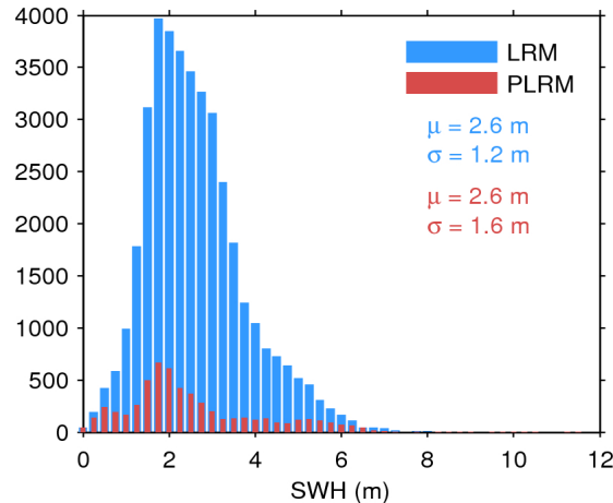
Figure 17. Histogram of flag-valid SWH over oceans and lakes for LRM (blue) and PLRM (red) for 07/12/2015. The mean ( \mu ) and standard deviation ( \sigma ) are also shown. Note that values larger than 12 m are excluded from the histogram for the sake of readability but not from the computation of \mu and \sigma .
