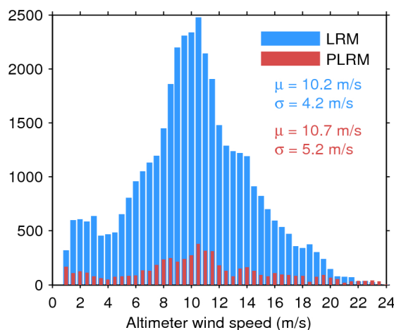
Figure 35. Histogram of science-valid wind over oceans and lakes for LRM (blue) and PLRM (red) for 07/12/2015. The mean ( \mu ) and standard deviation ( \sigma ) are also shown. Note that values larger than 24 m/s are excluded from the histogram for the sake of readability but not from the computation of \mu and \sigma .
