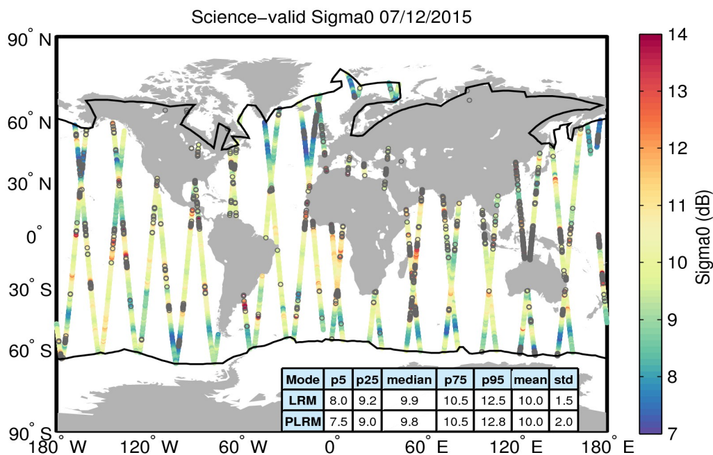
Figure 27. Geographical distribution of science-valid sigma0 data over oceans and lakes for 07/12/2015. The statistical values shown in the table refer to the sigma0 in dB and are calculated separately for LRM and PLRM regions. The black lines mark the outer limit of the Arctic and Antarctic polar polygons. Gray circles denote records that have been rejected based on the editing criteria described in Table 4.
