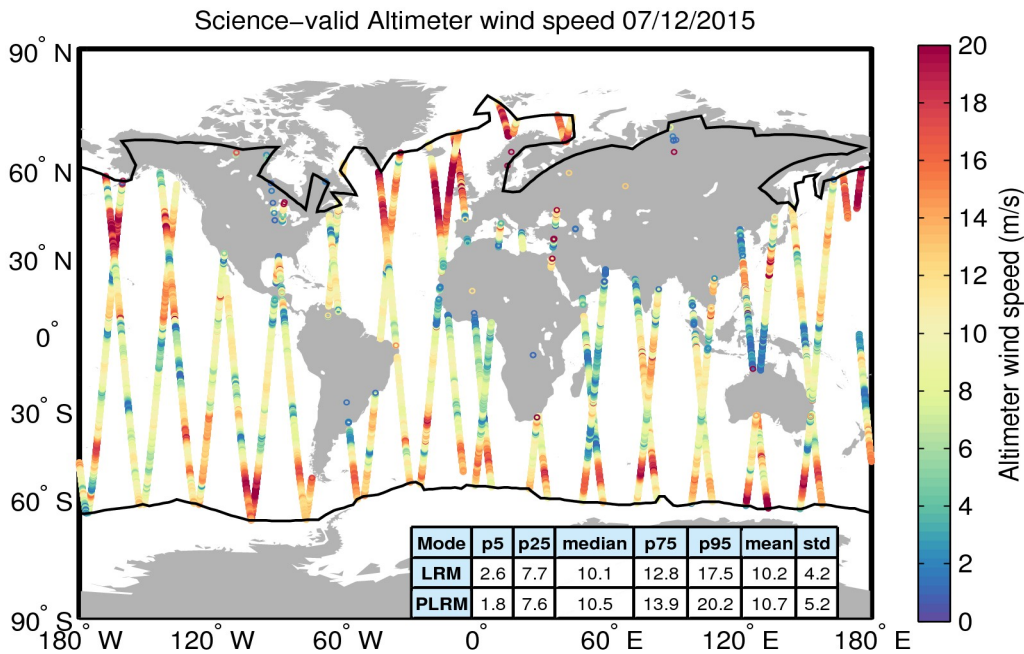
Figure 34. Geographical distribution of science-valid wind data over oceans and lakes for 07/12/2015. The statistical values shown in the table refer to the wind in m/s and are calculated separately for LRM and PLRM regions. The black lines mark the outer limit of the Arctic and Antarctic polar polygons. Gray circles denote records that have been rejected based on the editing criteria described in Table 5.
