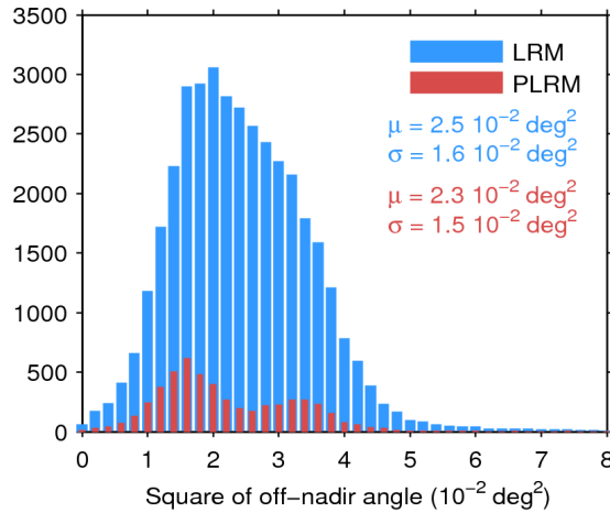
Figure 39. Histogram of flag-valid mispointing over oceans and lakes for LRM (blue) and PLRM (red) for 07/12/2015. Only positive values have been considered. The mean ( \mu ) and standard deviation ( \sigma ) are also shown. Note that values larger than 8 \cdot 10^{-2} \text{ deg}^2 are excluded from the histogram for the sake of readability but not from the computation of \mu and \sigma .
