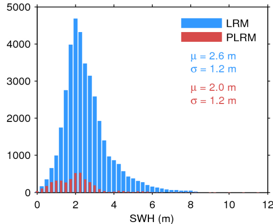
Figure 17. Histogram of flag-valid SWH over oceans and lakes for LRM (blue) and PLRM (red) for 30/11/2015. The mean ( \mu ) and standard deviation ( \sigma ) are also shown. Note that values larger than 12 m are excluded from the histogram for the sake of readability but not from the computation of \mu and \sigma .
