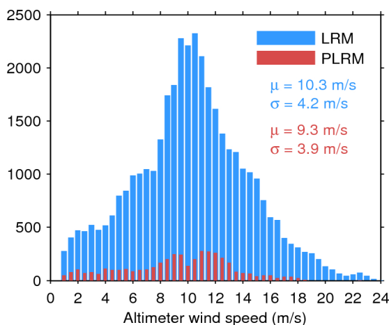
Figure 33. Histogram of flag-valid wind over oceans and lakes for LRM (blue) and PLRM (red) for 30/11/2015. The mean ( \mu ) and standard deviation ( \sigma ) are also shown. Note that values larger than 24 m/s are excluded from the histogram for the sake of readability but not from the computation of \mu and \sigma .
