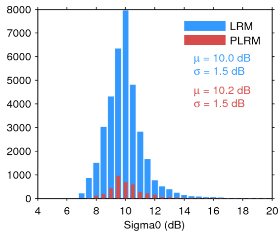
Figure 28. Histogram of science-valid sigma0 over oceans and lakes for LRM (blue) and PLRM (red) for 30/11/2015. The mean ( \mu ) and standard deviation ( \sigma ) are also shown. Note that values outside [4 20] dB are excluded from the histogram for the sake of readability but not from the computation of \mu and \sigma .
