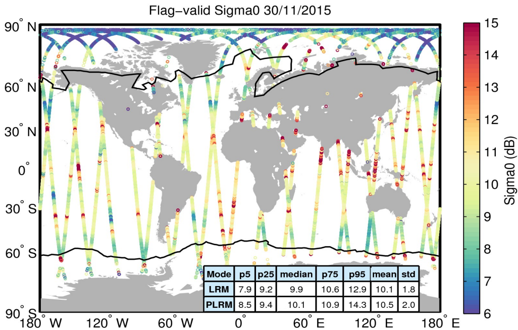
Figure 23. Geographical distribution of flag-valid sigma0 data over oceans and lakes for 30/11/2015. The statistical values shown in the table refer to the sigma0 in dB and are calculated separately for LRM and PLRM regions. Measurements taken over polar polygons have been excluded from the computation of the statistical values. The black lines mark the outer limit of the Arctic and Antarctic polar polygons.
