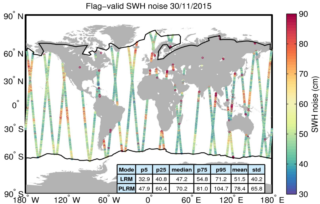
Figure 18. Geographical distribution of flag-valid 20-Hz SWH measurement noise over oceans and lakes for 30/11/2015. The statistical values shown in the table refer to the SWH noise and are calculated separately for LRM and PLRM regions. Measurements taken over polar polygons have been excluded from the computation of the statistical values. The black lines mark the outer limit of the Arctic and Antarctic polar polygons.
