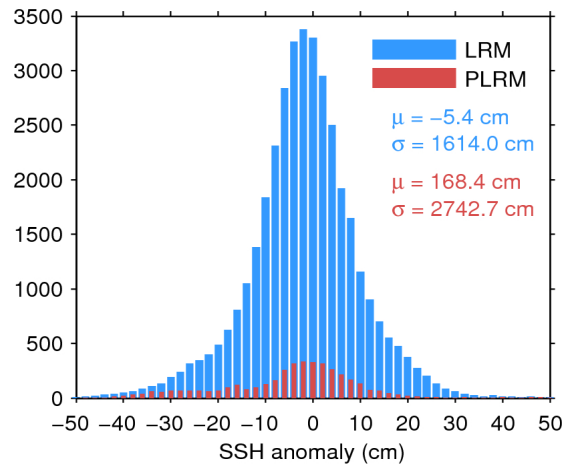
Figure 7. Histogram of flag-valid SSH anomaly over oceans and lakes for LRM (blue) and PLRM (red) for 30/11/2015. The mean ( \mu ) and standard deviation ( \sigma ) are also shown. Note that values outside [-50 50] cm are excluded from the histogram for the sake of readability but not from the computation of \mu and \sigma .
