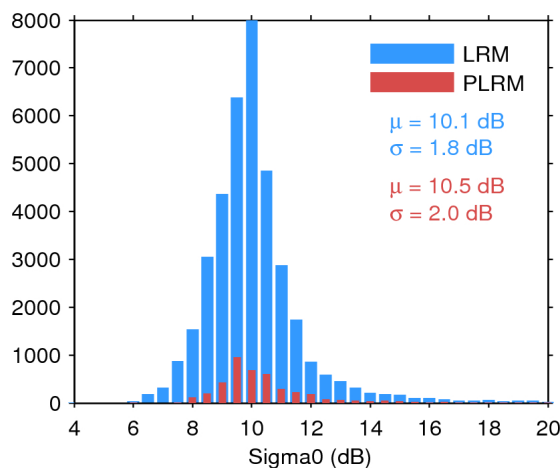
Figure 25. Histogram of flag-valid sigma0 over oceans and lakes for LRM (blue) and PLRM (red) for 30/11/2015. The mean ( \mu ) and standard deviation ( \sigma ) are also shown. Note that values outside [4 20] dB are excluded from the histogram for the sake of readability but not from the computation of \mu and \sigma .
