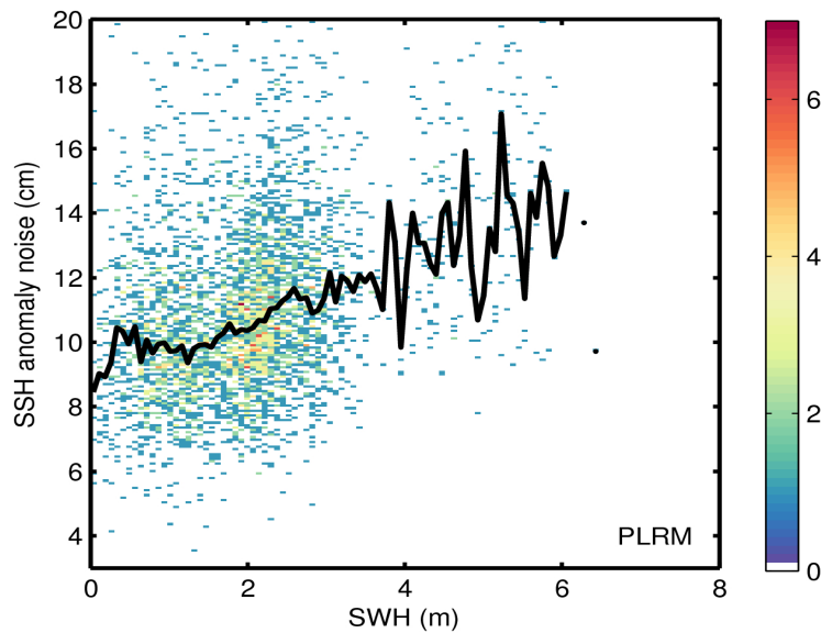
Figure 9. 2D histogram showing flag-valid SSH anomaly noise as a function of SWH for LRM (top) and PLRM (bottom) for 30/11/2015. The black line denotes the median SSH anomaly noise as a function of SWH.
