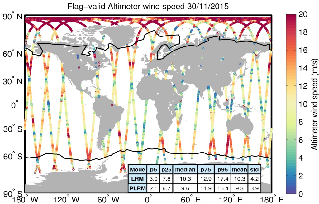
Figure 31. Geographical distribution of flag-valid wind data over oceans and lakes for 30/11/2015. The statistical values shown in the table refer to the wind in m/s and are calculated separately for LRM and PLRM regions. Measurements taken over polar polygons have been excluded from the computation of the statistical values. The black lines mark the outer limit of the Arctic and Antarctic polar polygons.
