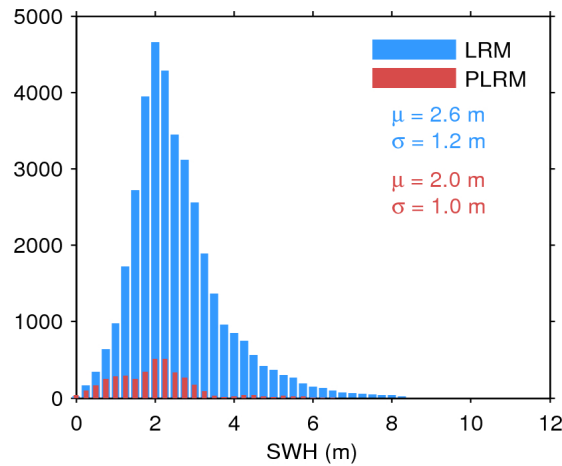
Figure 20. Histogram of science-valid SWH over oceans and lakes for LRM (blue) and PLRM (red) for 30/11/2015. The mean ( \mu ) and standard deviation ( \sigma ) are also shown. Note that values larger than 12 m are excluded from the histogram for the sake of readability but not from the computation of \mu and \sigma .
