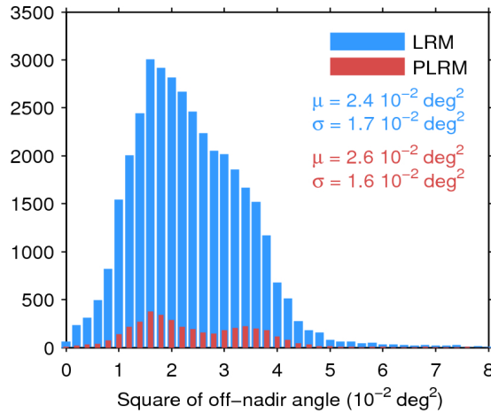
Figure 39. Histogram of flag-valid mispointing over oceans and lakes for LRM (blue) and PLRM (red) for 30/11/2015. Only positive values have been considered. The mean ( \mu ) and standard deviation ( \sigma ) are also shown. Note that values larger than 8 \cdot 10^{-2} \text{ deg}^2 are excluded from the histogram for the sake of readability but not from the computation of \mu and \sigma .
