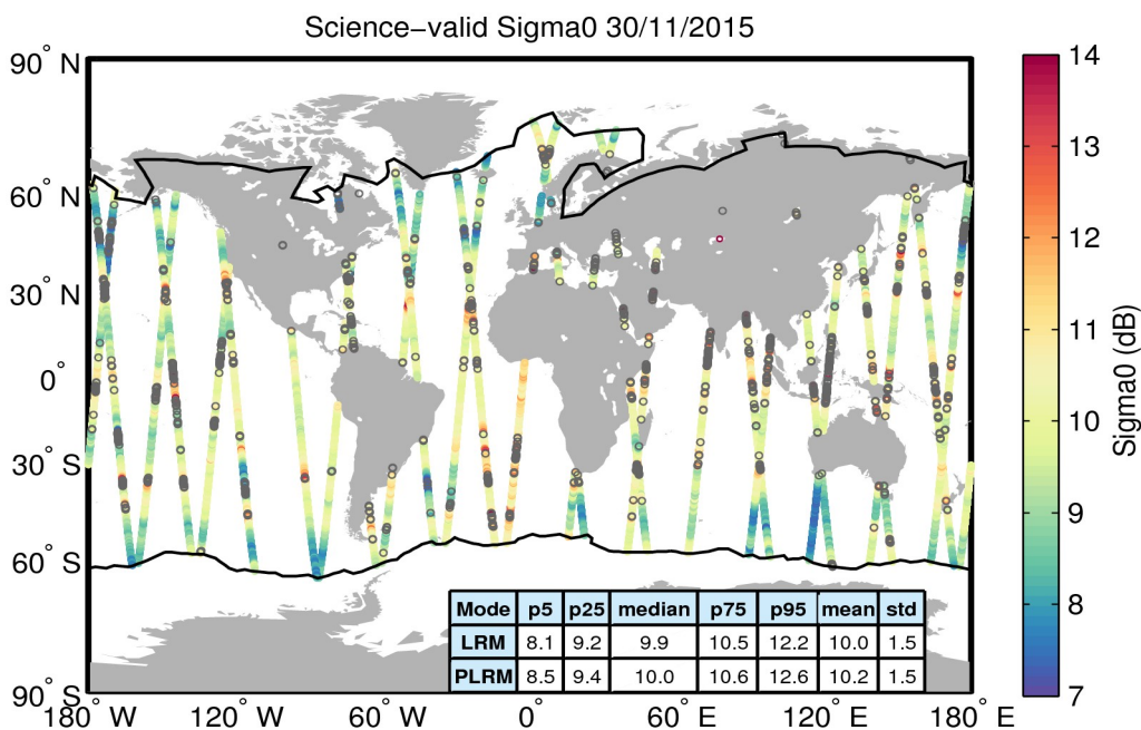
Figure 27. Geographical distribution of science-valid sigma0 data over oceans and lakes for 30/11/2015. The statistical values shown in the table refer to the sigma0 in dB and are calculated separately for LRM and PLRM regions. The black lines mark the outer limit of the Arctic and Antarctic polar polygons. Gray circles denote records that have been rejected based on the editing criteria described in Table 4.
