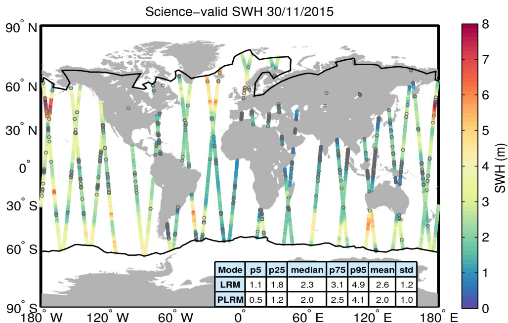
Figure 19. Geographical distribution of science-valid SWH data over oceans and lakes for 30/11/2015. The statistical values shown in the table refer to the SWH in m and are calculated separately for LRM and PLRM regions. The black lines mark the outer limit of the Arctic and Antarctic polar polygons. Gray circles denote records that have been rejected based on the editing criteria described in Table 3.
