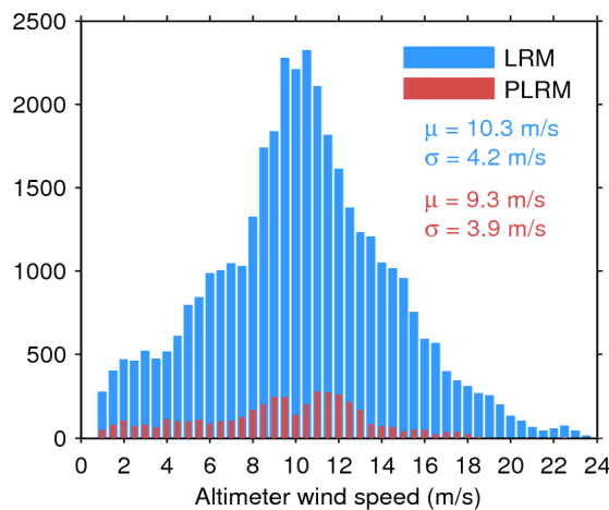
Figure 35. Histogram of science-valid wind over oceans and lakes for LRM (blue) and PLRM (red) for 30/11/2015. The mean ( \mu ) and standard deviation ( \sigma ) are also shown. Note that values larger than 24 m/s are excluded from the histogram for the sake of readability but not from the computation of \mu and \sigma .
