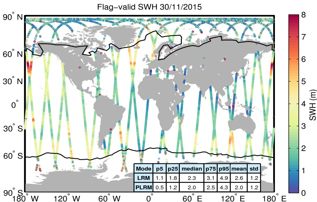
Figure 15. Geographical distribution of flag-valid SWH data over oceans and lakes for 30/11/2015. The statistical values shown in the table refer to the SWH in m and are calculated separately for LRM and PLRM regions. Measurements taken over polar polygons have been excluded from the computation of the statistical values. The black lines mark the outer limit of the Arctic and Antarctic polar polygons.
