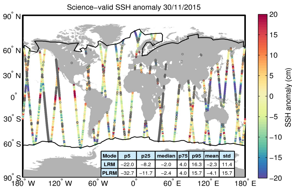
Figure 10. Geographical distribution of science-valid SSH anomaly data over oceans and lakes for 30/11/2015. The statistical values shown in the table refer to the SSH anomaly in cm and are calculated separately for LRM and PLRM regions. The black lines mark the outer limit of the Arctic and Antarctic polar polygons. Gray circles denote records that have been rejected based on the editing criteria described in Table 2.
