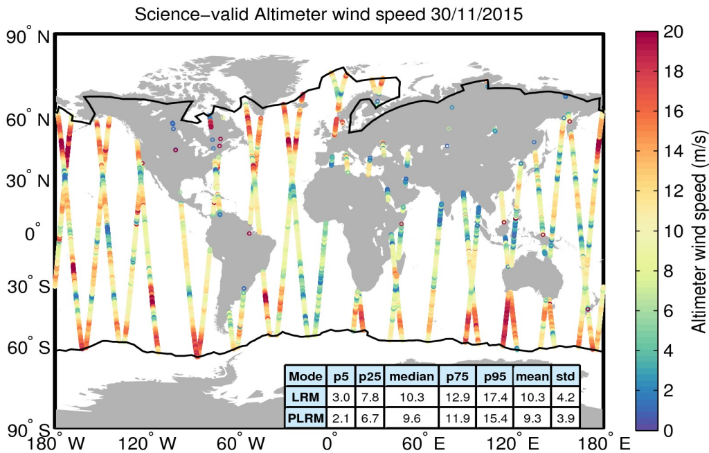
Figure 34. Geographical distribution of science-valid wind data over oceans and lakes for 30/11/2015. The statistical values shown in the table refer to the wind in m/s and are calculated separately for LRM and PLRM regions. The black lines mark the outer limit of the Arctic and Antarctic polar polygons. Gray circles denote records that have been rejected based on the editing criteria described in Table 5.
