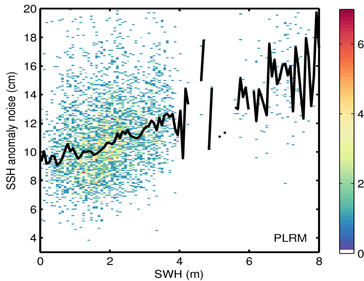
Figure 9. 2D histogram showing flag-valid SSH anomaly noise as a function of SWH for LRM (top) and PLRM (bottom) for 28/11/2015. The black line denotes the median SSH anomaly noise as a function of SWH.
