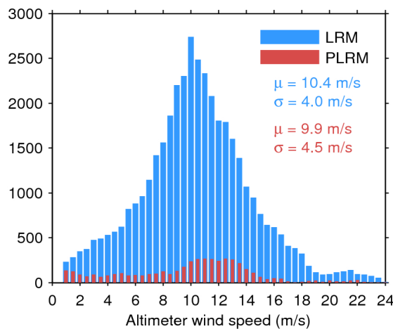
Figure 35. Histogram of science-valid wind over oceans and lakes for LRM (blue) and PLRM (red) for 28/11/2015. The mean ( \mu ) and standard deviation ( \sigma ) are also shown. Note that values larger than 24 m/s are excluded from the histogram for the sake of readability but not from the computation of \mu and \sigma .
