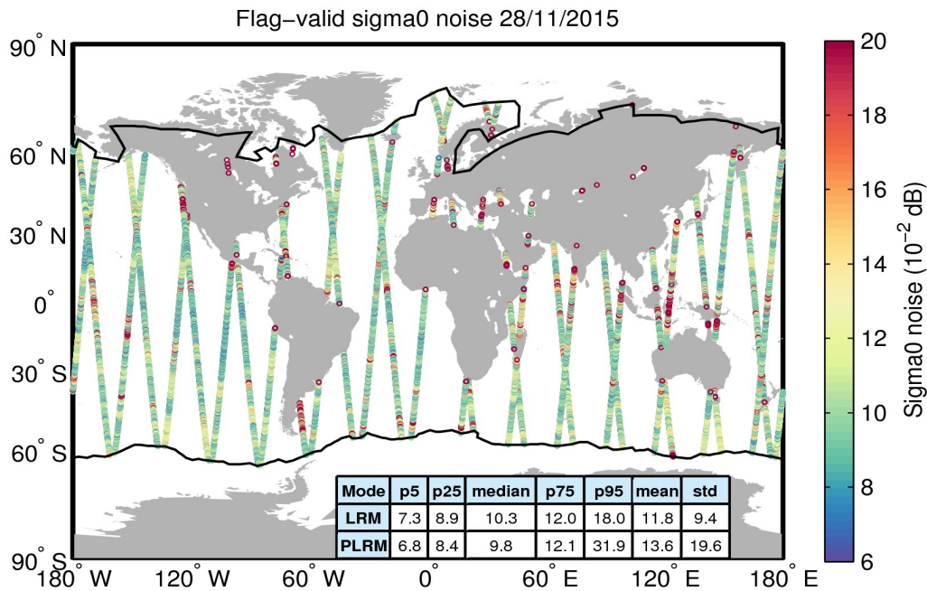
Figure 26. Geographical distribution of flag-valid 20-Hz sigma0 measurement noise over oceans and lakes for 28/11/2015. The statistical values shown in the table refer to the sigma0 noise and are calculated separately for LRM and PLRM regions. Measurements taken over polar polygons have been excluded from the computation of the statistical values. The black lines mark the outer limit of the Arctic and Antarctic polar polygons.
