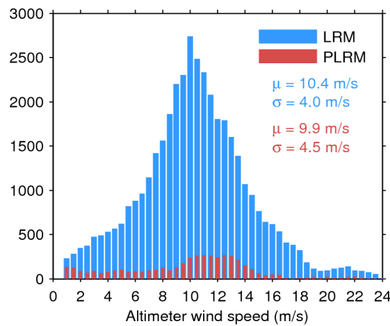
Figure 33. Histogram of flag-valid wind over oceans and lakes for LRM (blue) and PLRM (red) for 28/11/2015. The mean ( \mu ) and standard deviation ( \sigma ) are also shown. Note that values larger than 24 m/s are excluded from the histogram for the sake of readability but not from the computation of \mu and \sigma .
