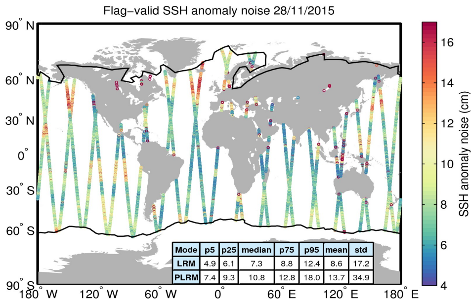
Figure 8. Geographical distribution of flag-valid 20-Hz SSH anomaly measurement noise over oceans and lakes for 28/11/2015. The statistical values shown in the table refer to the SSH anomaly noise and are calculated separately for LRM and PLRM regions. Measurements taken over polar polygons have been excluded from the computation of the statistical values. The black lines mark the outer limit of the Arctic and Antarctic polar polygons.
