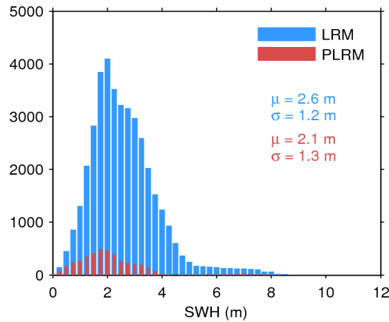
Figure 20. Histogram of science-valid SWH over oceans and lakes for LRM (blue) and PLRM (red) for 28/11/2015. The mean ( \mu ) and standard deviation ( \sigma ) are also shown. Note that values larger than 12 m are excluded from the histogram for the sake of readability but not from the computation of \mu and \sigma .
