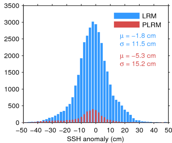
Figure 11. Histogram of science-valid SSH anomaly over oceans and lakes for LRM (blue) and PLRM (red) for 28/11/2015. The mean ( \mu ) and standard deviation ( \sigma ) are also shown. Note that values outside [-50 50] cm are excluded from the histogram for the sake of readability but not from the computation of \mu and \sigma .
