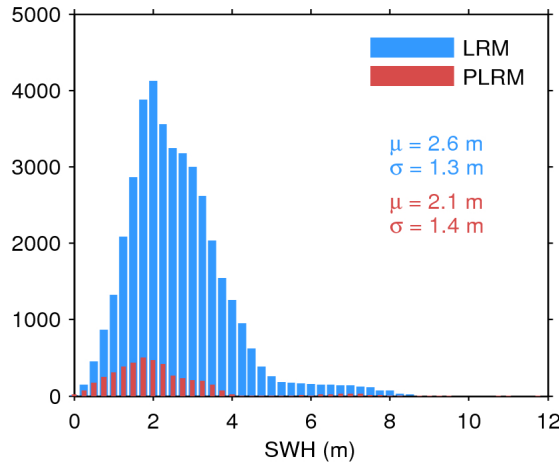
Figure 17. Histogram of flag-valid SWH over oceans and lakes for LRM (blue) and PLRM (red) for 28/11/2015. The mean ( \mu ) and standard deviation ( \sigma ) are also shown. Note that values larger than 12 m are excluded from the histogram for the sake of readability but not from the computation of \mu and \sigma .
