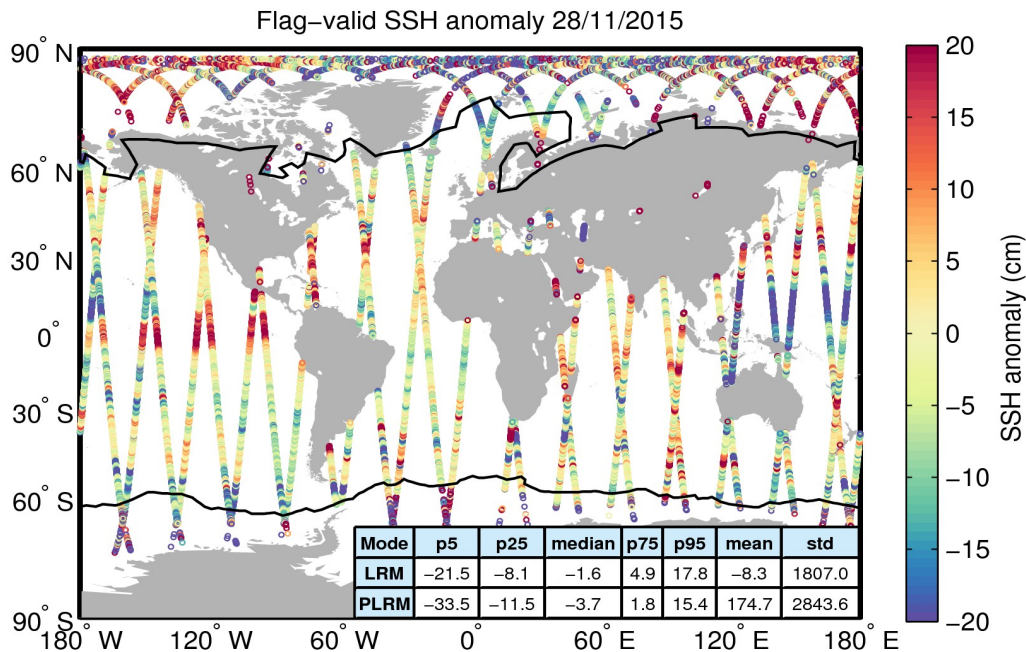
Figure 5. Geographical distribution of flag-valid 1-Hz SSH anomaly data over oceans and lakes for 28/11/2015. The statistical values shown in the table refer to the SSH anomaly in cm and are calculated separately for LRM and PLRM regions. Measurements taken over polar polygons have been excluded from the computation of the statistical values. The black lines mark the outer limit of the Arctic and Antarctic polar polygons.
