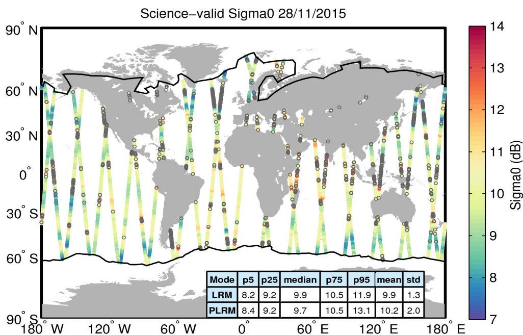
Figure 27. Geographical distribution of science-valid sigma0 data over oceans and lakes for 28/11/2015. The statistical values shown in the table refer to the sigma0 in dB and are calculated separately for LRM and PLRM regions. The black lines mark the outer limit of the Arctic and Antarctic polar polygons. Gray circles denote records that have been rejected based on the editing criteria described in Table 4.
