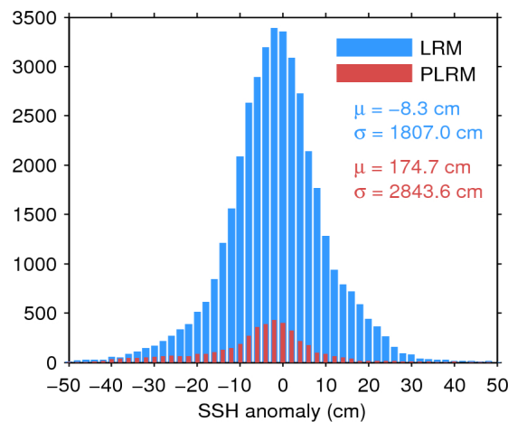
Figure 7. Histogram of flag-valid SSH anomaly over oceans and lakes for LRM (blue) and PLRM (red) for 28/11/2015. The mean ( \mu ) and standard deviation ( \sigma ) are also shown. Note that values outside [-50\ 50] cm are excluded from the histogram for the sake of readability but not from the computation of \mu and \sigma .
