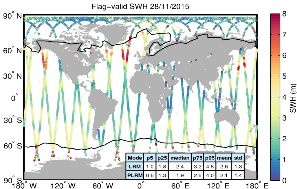
Figure 15. Geographical distribution of flag-valid SWH data over oceans and lakes for 28/11/2015. The statistical values shown in the table refer to the SWH in m and are calculated separately for LRM and PLRM regions. Measurements taken over polar polygons have been excluded from the computation of the statistical values. The black lines mark the outer limit of the Arctic and Antarctic polar polygons.
