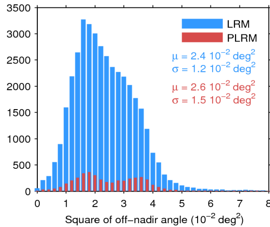
Figure 39. Histogram of flag-valid mispointing over oceans and lakes for LRM (blue) and PLRM (red) for 28/11/2015. Only positive values have been considered. The mean ( \mu ) and standard deviation ( \sigma ) are also shown. Note that values larger than 8 \cdot 10^{-2} \text{ deg}^2 are excluded from the histogram for the sake of readability but not from the computation of \mu and \sigma .
