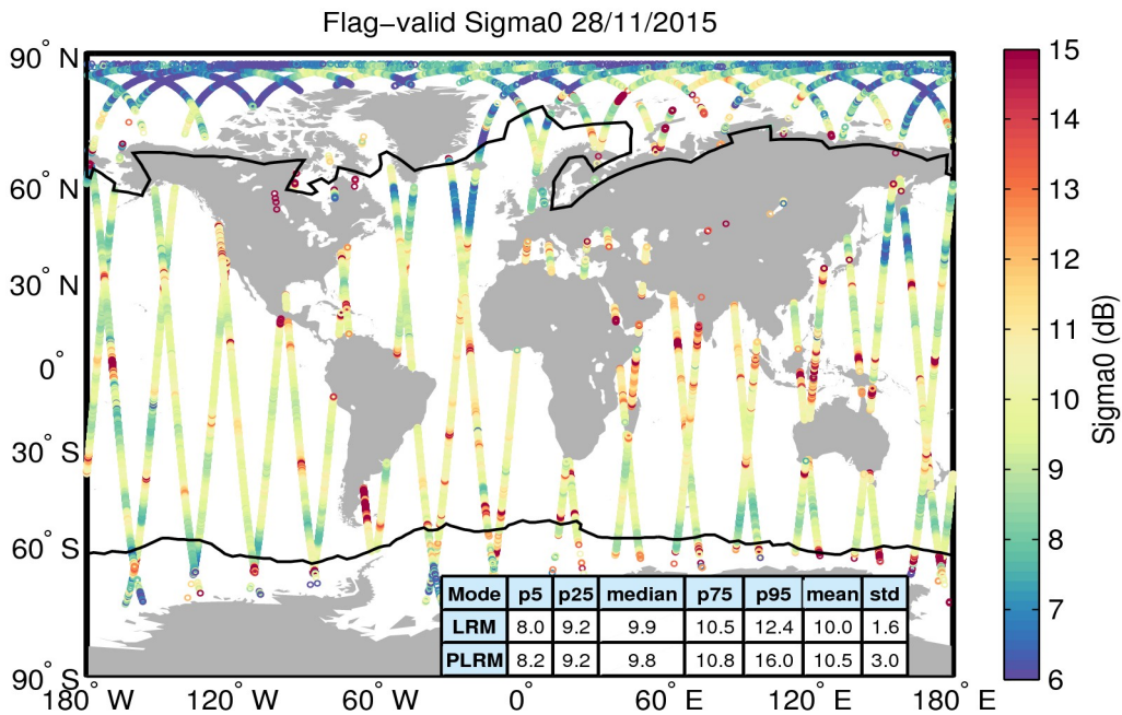
Figure 23. Geographical distribution of flag-valid sigma0 data over oceans and lakes for 28/11/2015. The statistical values shown in the table refer to the sigma0 in dB and are calculated separately for LRM and PLRM regions. Measurements taken over polar polygons have been excluded from the computation of the statistical values. The black lines mark the outer limit of the Arctic and Antarctic polar polygons.
