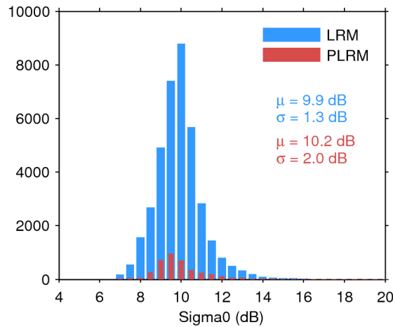
Figure 28. Histogram of science-valid sigma0 over oceans and lakes for LRM (blue) and PLRM (red) for 28/11/2015. The mean ( \mu ) and standard deviation ( \sigma ) are also shown. Note that values outside [4 20] dB are excluded from the histogram for the sake of readability but not from the computation of \mu and \sigma .
