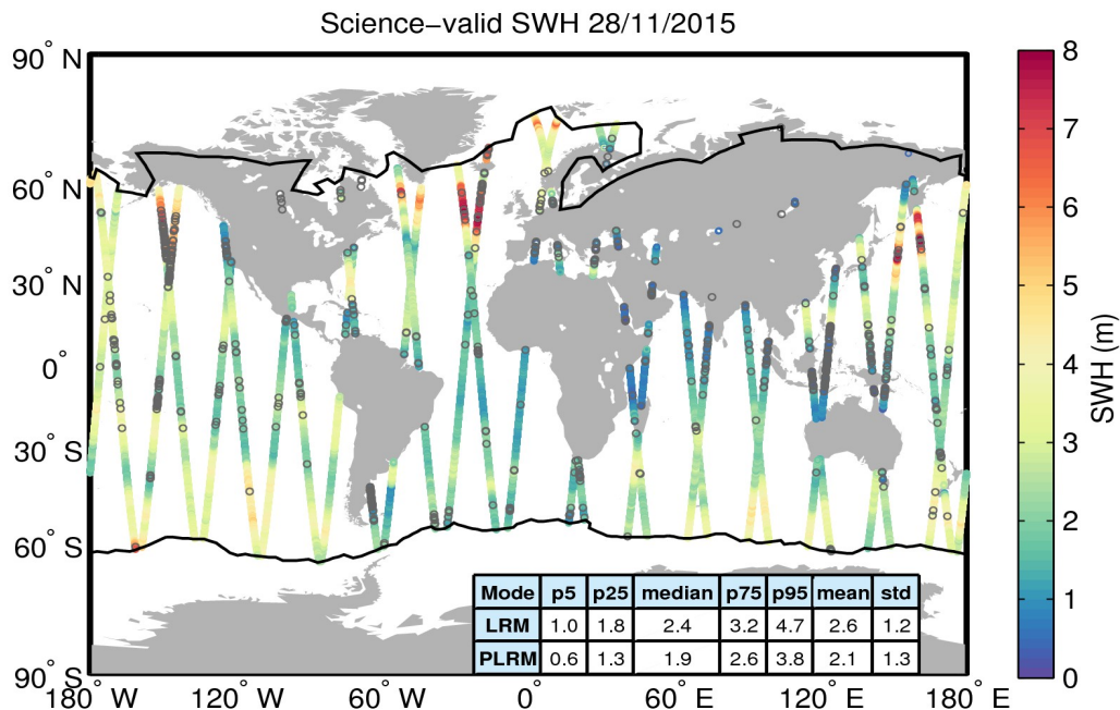
Figure 19. Geographical distribution of science-valid SWH data over oceans and lakes for 28/11/2015. The statistical values shown in the table refer to the SWH in m and are calculated separately for LRM and PLRM regions. The black lines mark the outer limit of the Arctic and Antarctic polar polygons. Gray circles denote records that have been rejected based on the editing criteria described in Table 3.
