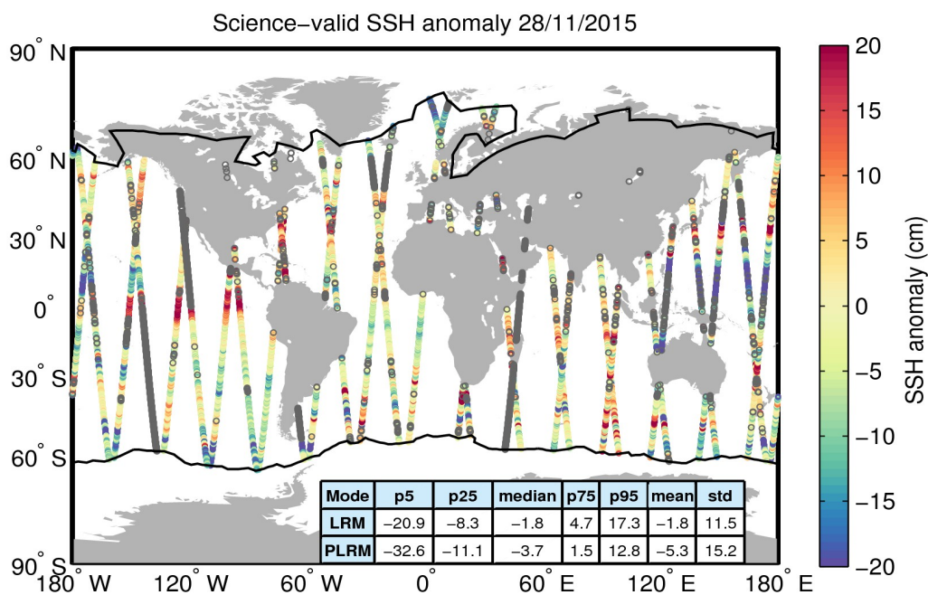
Figure 10. Geographical distribution of science-valid SSH anomaly data over oceans and lakes for 28/11/2015. The statistical values shown in the table refer to the SSH anomaly in cm and are calculated separately for LRM and PLRM regions. The black lines mark the outer limit of the Arctic and Antarctic polar polygons. Gray circles denote records that have been rejected based on the editing criteria described in Table 2.
