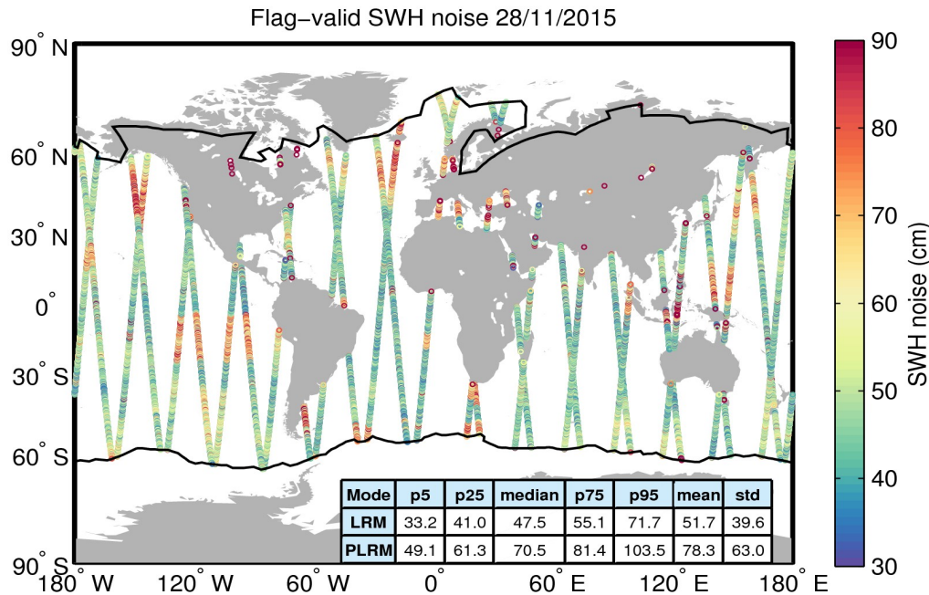
Figure 18. Geographical distribution of flag-valid 20-Hz SWH measurement noise over oceans and lakes for 28/11/2015. The statistical values shown in the table refer to the SWH noise and are calculated separately for LRM and PLRM regions. Measurements taken over polar polygons have been excluded from the computation of the statistical values. The black lines mark the outer limit of the Arctic and Antarctic polar polygons.
