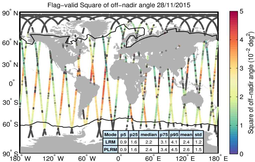
Figure 37. Geographical distribution of flag-valid mispointing data over oceans and lakes for 28/11/2015. The statistical values shown in the table refer to the mispointing in 10^{-2} \text{ deg}^2 and are calculated separately for LRM and PLRM regions. Measurements taken over polar polygons have been excluded from the computation of the statistical values. The black lines mark the outer limit of the Arctic and Antarctic polar polygons. Gray circles denote negative values.
