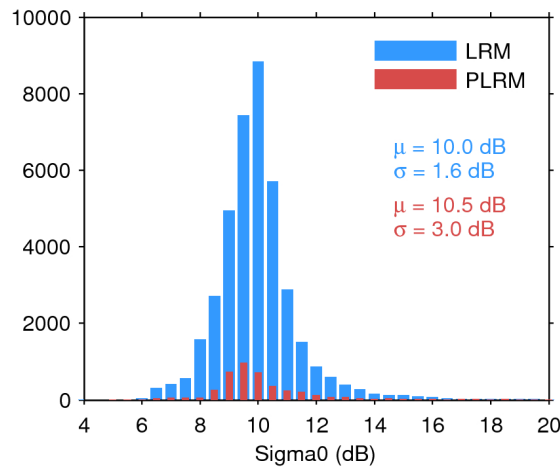
Figure 25. Histogram of flag-valid sigma0 over oceans and lakes for LRM (blue) and PLRM (red) for 28/11/2015. The mean ( \mu ) and standard deviation ( \sigma ) are also shown. Note that values outside [4 20] dB are excluded from the histogram for the sake of readability but not from the computation of \mu and \sigma .
