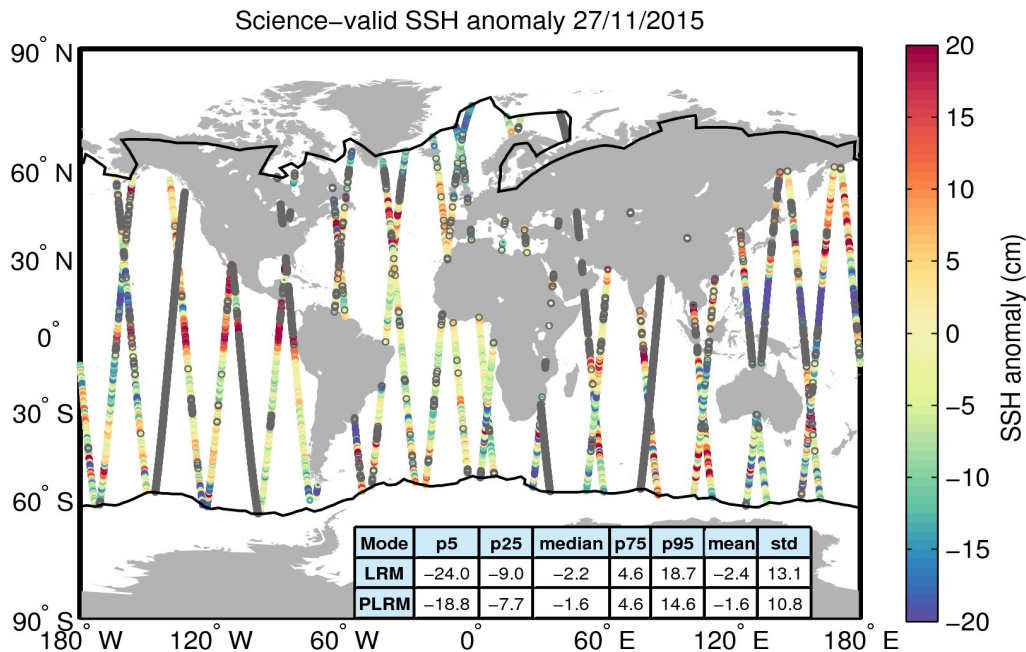
Figure 10. Geographical distribution of science-valid SSH anomaly data over oceans and lakes for 27/11/2015. The statistical values shown in the table refer to the SSH anomaly in cm and are calculated separately for LRM and PLRM regions. The black lines mark the outer limit of the Arctic and Antarctic polar polygons. Gray circles denote records that have been rejected based on the editing criteria described in Table 2.
