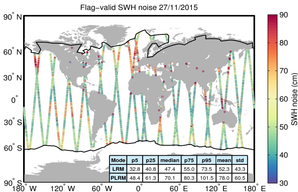
Figure 18. Geographical distribution of flag-valid 20-Hz SWH measurement noise over oceans and lakes for 27/11/2015. The statistical values shown in the table refer to the SWH noise and are calculated separately for LRM and PLRM regions. Measurements taken over polar polygons have been excluded from the computation of the statistical values. The black lines mark the outer limit of the Arctic and Antarctic polar polygons.
