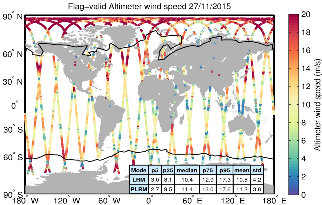
Figure 31. Geographical distribution of flag-valid wind data over oceans and lakes for 27/11/2015. The statistical values shown in the table refer to the wind in m/s and are calculated separately for LRM and PLRM regions. Measurements taken over polar polygons have been excluded from the computation of the statistical values. The black lines mark the outer limit of the Arctic and Antarctic polar polygons.
