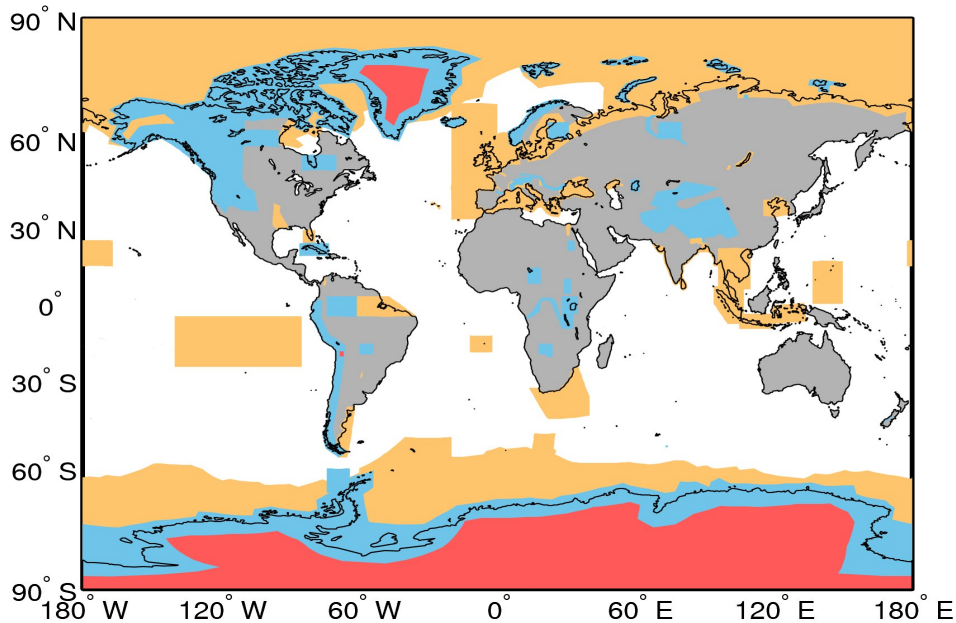
Figure A1. Extent of the regions defining the geographical mode mask for 27/11/2015. The regions where SAR, and SARIn are operated are denoted by the orange and blue polygons, respectively. LRM is operated over areas of the continental ice sheets (red polygons) and over oceans and land not covered by other modes.
