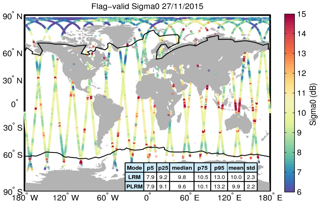
Figure 23. Geographical distribution of flag-valid sigma0 data over oceans and lakes for 27/11/2015. The statistical values shown in the table refer to the sigma0 in dB and are calculated separately for LRM and PLRM regions. Measurements taken over polar polygons have been excluded from the computation of the statistical values. The black lines mark the outer limit of the Arctic and Antarctic polar polygons.
