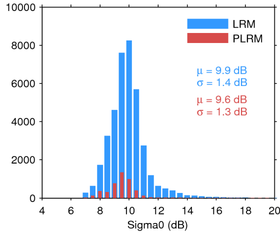
Figure 28. Histogram of science-valid sigma0 over oceans and lakes for LRM (blue) and PLRM (red) for 27/11/2015. The mean ( \mu ) and standard deviation ( \sigma ) are also shown. Note that values outside [4 20] dB are excluded from the histogram for the sake of readability but not from the computation of \mu and \sigma .
