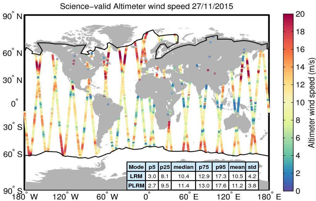
Figure 34. Geographical distribution of science-valid wind data over oceans and lakes for 27/11/2015. The statistical values shown in the table refer to the wind in m/s and are calculated separately for LRM and PLRM regions. The black lines mark the outer limit of the Arctic and Antarctic polar polygons. Gray circles denote records that have been rejected based on the editing criteria described in Table 5.
