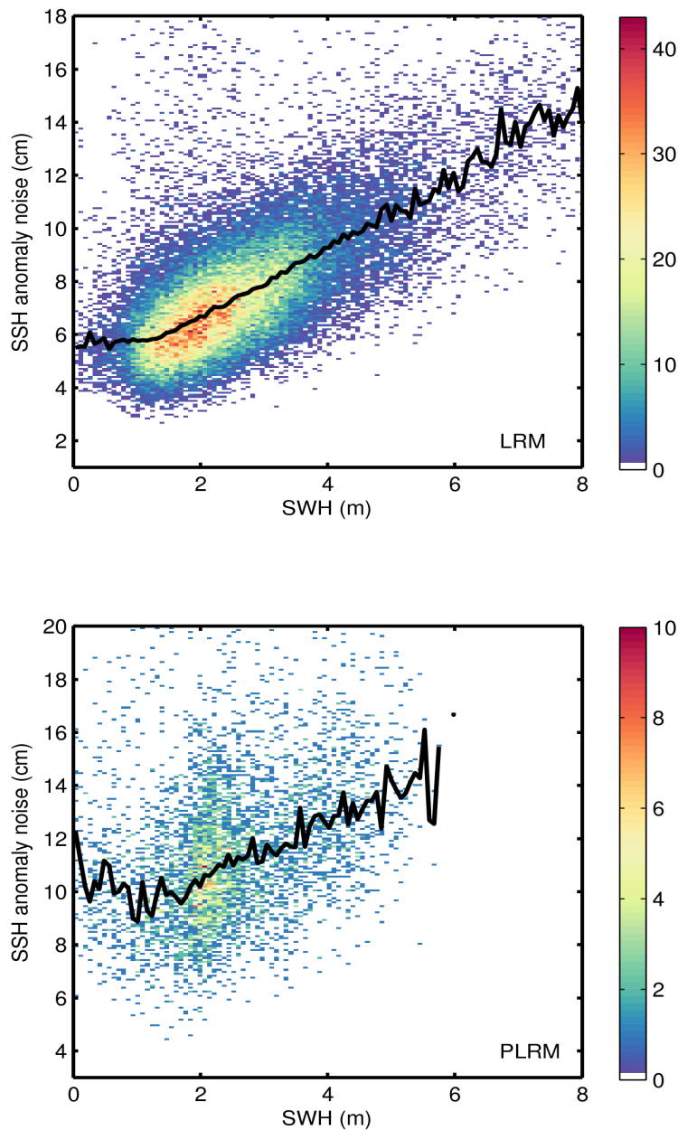
Figure 9. 2D histogram showing flag-valid SSH anomaly noise as a function of SWH for LRM (top) and PLRM (bottom) for 27/11/2015. The black line denotes the median SSH anomaly noise as a function of SWH.
