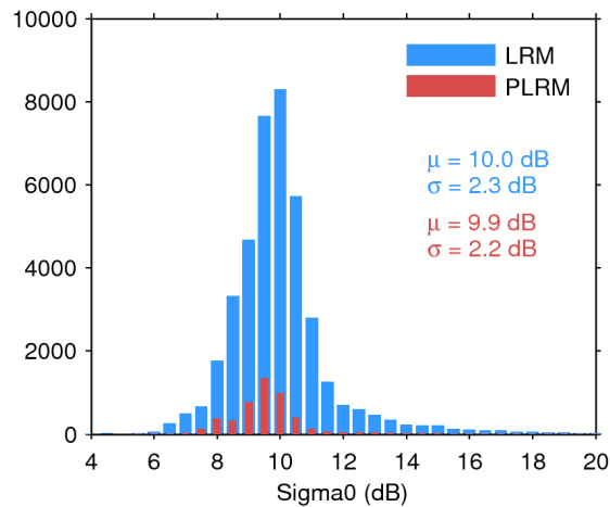
Figure 25. Histogram of flag-valid sigma0 over oceans and lakes for LRM (blue) and PLRM (red) for 27/11/2015. The mean ( \mu ) and standard deviation ( \sigma ) are also shown. Note that values outside [4 20] dB are excluded from the histogram for the sake of readability but not from the computation of \mu and \sigma .
