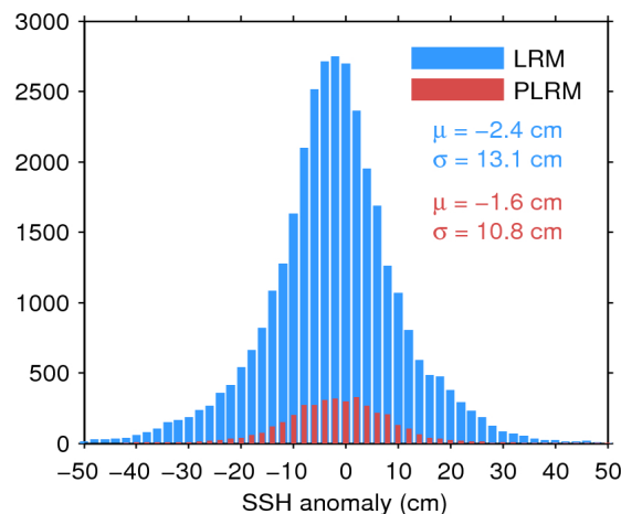
Figure 11. Histogram of science-valid SSH anomaly over oceans and lakes for LRM (blue) and PLRM (red) for 27/11/2015. The mean ( \mu ) and standard deviation ( \sigma ) are also shown. Note that values outside [-50 50] cm are excluded from the histogram for the sake of readability but not from the computation of \mu and \sigma .
