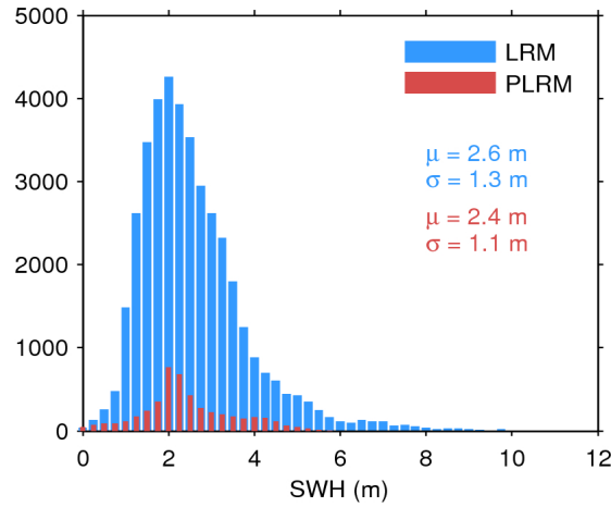
Figure 20. Histogram of science-valid SWH over oceans and lakes for LRM (blue) and PLRM (red) for 27/11/2015. The mean ( \mu ) and standard deviation ( \sigma ) are also shown. Note that values larger than 12 m are excluded from the histogram for the sake of readability but not from the computation of \mu and \sigma .
