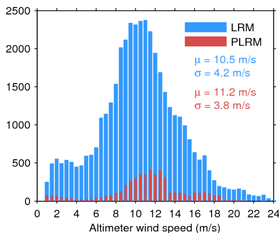
Figure 35. Histogram of science-valid wind over oceans and lakes for LRM (blue) and PLRM (red) for 27/11/2015. The mean ( \mu ) and standard deviation ( \sigma ) are also shown. Note that values larger than 24 m/s are excluded from the histogram for the sake of readability but not from the computation of \mu and \sigma .
