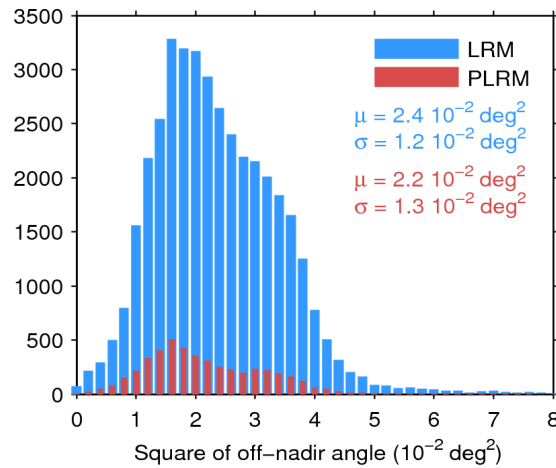
Figure 39. Histogram of flag-valid mispointing over oceans and lakes for LRM (blue) and PLRM (red) for 27/11/2015. Only positive values have been considered. The mean ( \mu ) and standard deviation ( \sigma ) are also shown. Note that values larger than 8 \cdot 10^{-2} \text{ deg}^2 are excluded from the histogram for the sake of readability but not from the computation of \mu and \sigma .
