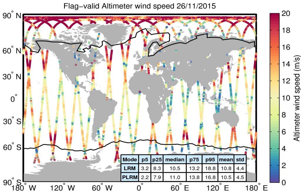
Figure 31. Geographical distribution of flag-valid wind data over oceans and lakes for 26/11/2015. The statistical values shown in the table refer to the wind in m/s and are calculated separately for LRM and PLRM regions. Measurements taken over polar polygons have been excluded from the computation of the statistical values. The black lines mark the outer limit of the Arctic and Antarctic polar polygons.
