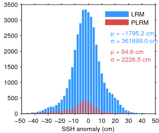
Figure 7. Histogram of flag-valid SSH anomaly over oceans and lakes for LRM (blue) and PLRM (red) for 26/11/2015. The mean ( \mu ) and standard deviation ( \sigma ) are also shown. Note that values outside [-50\ 50] cm are excluded from the histogram for the sake of readability but not from the computation of \mu and \sigma .
