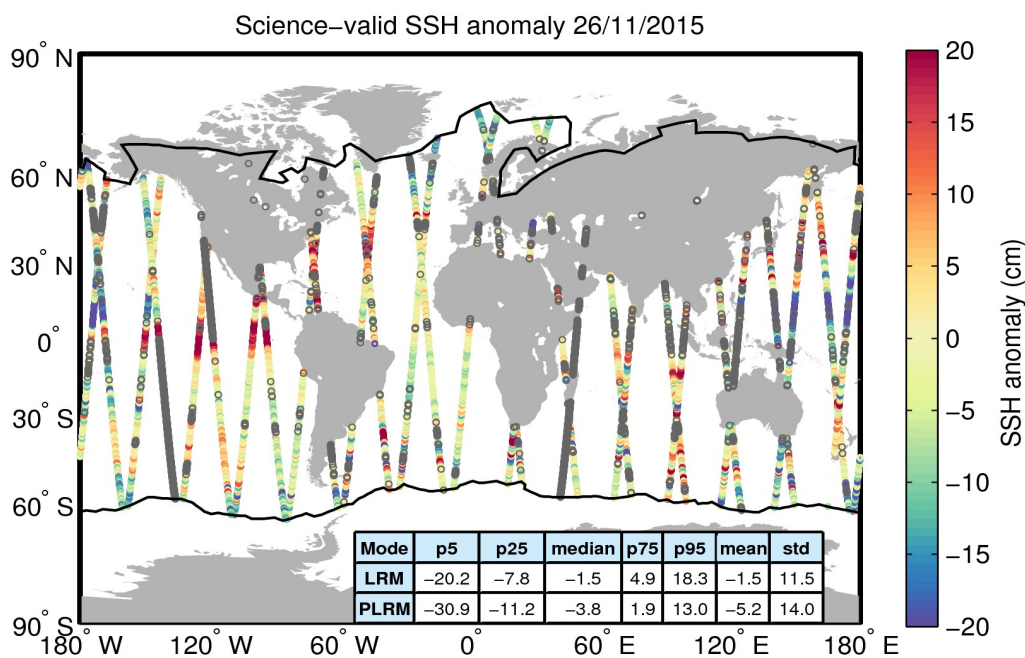
Figure 10. Geographical distribution of science-valid SSH anomaly data over oceans and lakes for 26/11/2015. The statistical values shown in the table refer to the SSH anomaly in cm and are calculated separately for LRM and PLRM regions. The black lines mark the outer limit of the Arctic and Antarctic polar polygons. Gray circles denote records that have been rejected based on the editing criteria described in Table 2.
