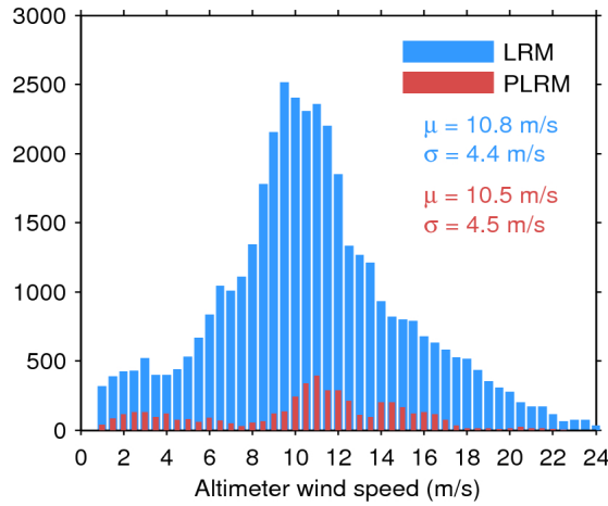
Figure 33. Histogram of flag-valid wind over oceans and lakes for LRM (blue) and PLRM (red) for 26/11/2015. The mean ( \mu ) and standard deviation ( \sigma ) are also shown. Note that values larger than 24 m/s are excluded from the histogram for the sake of readability but not from the computation of \mu and \sigma .
