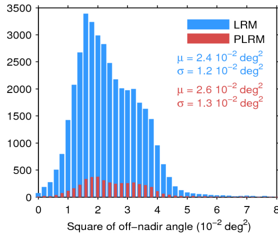
Figure 39. Histogram of flag-valid mispointing over oceans and lakes for LRM (blue) and PLRM (red) for 26/11/2015. Only positive values have been considered. The mean ( \mu ) and standard deviation ( \sigma ) are also shown. Note that values larger than 8 \cdot 10^{-2} \text{ deg}^2 are excluded from the histogram for the sake of readability but not from the computation of \mu and \sigma .
