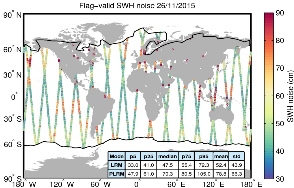
Figure 18. Geographical distribution of flag-valid 20-Hz SWH measurement noise over oceans and lakes for 26/11/2015. The statistical values shown in the table refer to the SWH noise and are calculated separately for LRM and PLRM regions. Measurements taken over polar polygons have been excluded from the computation of the statistical values. The black lines mark the outer limit of the Arctic and Antarctic polar polygons.
