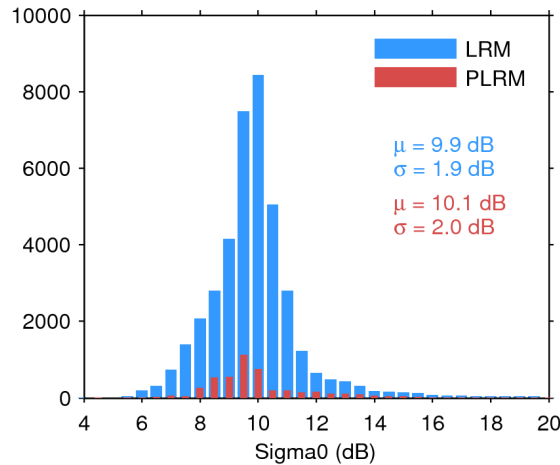
Figure 25. Histogram of flag-valid sigma0 over oceans and lakes for LRM (blue) and PLRM (red) for 26/11/2015. The mean ( \mu ) and standard deviation ( \sigma ) are also shown. Note that values outside [4 20] dB are excluded from the histogram for the sake of readability but not from the computation of \mu and \sigma .
