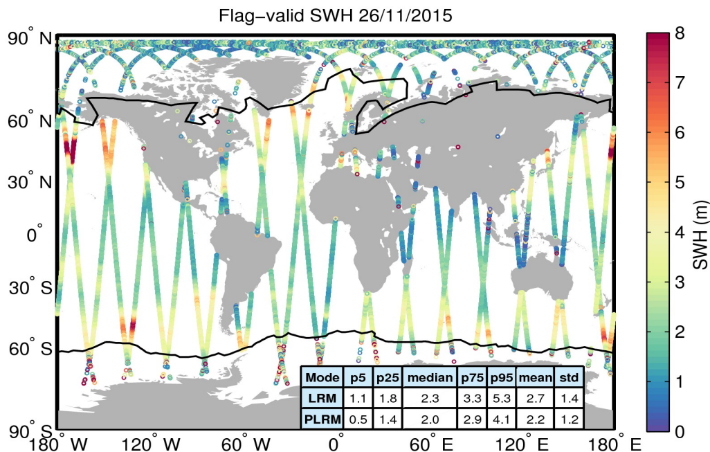
Figure 15. Geographical distribution of flag-valid SWH data over oceans and lakes for 26/11/2015. The statistical values shown in the table refer to the SWH in m and are calculated separately for LRM and PLRM regions. Measurements taken over polar polygons have been excluded from the computation of the statistical values. The black lines mark the outer limit of the Arctic and Antarctic polar polygons.
