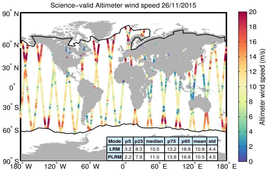
Figure 34. Geographical distribution of science-valid wind data over oceans and lakes for 26/11/2015. The statistical values shown in the table refer to the wind in m/s and are calculated separately for LRM and PLRM regions. The black lines mark the outer limit of the Arctic and Antarctic polar polygons. Gray circles denote records that have been rejected based on the editing criteria described in Table 5.
