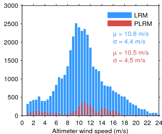
Figure 35. Histogram of science-valid wind over oceans and lakes for LRM (blue) and PLRM (red) for 26/11/2015. The mean ( \mu ) and standard deviation ( \sigma ) are also shown. Note that values larger than 24 m/s are excluded from the histogram for the sake of readability but not from the computation of \mu and \sigma .
