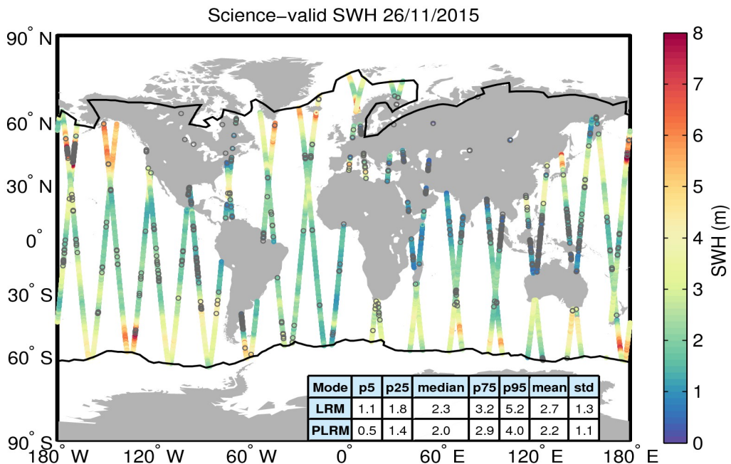
Figure 19. Geographical distribution of science-valid SWH data over oceans and lakes for 26/11/2015. The statistical values shown in the table refer to the SWH in m and are calculated separately for LRM and PLRM regions. The black lines mark the outer limit of the Arctic and Antarctic polar polygons. Gray circles denote records that have been rejected based on the editing criteria described in Table 3.
