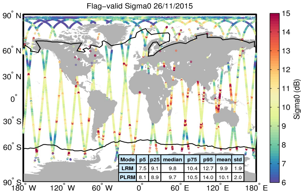
Figure 23. Geographical distribution of flag-valid sigma0 data over oceans and lakes for 26/11/2015. The statistical values shown in the table refer to the sigma0 in dB and are calculated separately for LRM and PLRM regions. Measurements taken over polar polygons have been excluded from the computation of the statistical values. The black lines mark the outer limit of the Arctic and Antarctic polar polygons.
