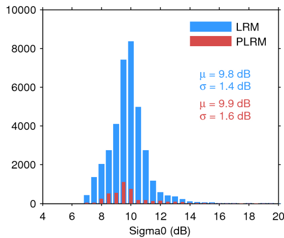
Figure 28. Histogram of science-valid sigma0 over oceans and lakes for LRM (blue) and PLRM (red) for 26/11/2015. The mean ( \mu ) and standard deviation ( \sigma ) are also shown. Note that values outside [4 20] dB are excluded from the histogram for the sake of readability but not from the computation of \mu and \sigma .
