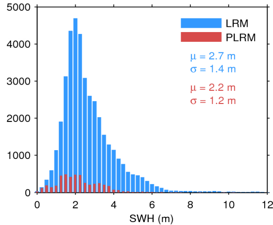
Figure 17. Histogram of flag-valid SWH over oceans and lakes for LRM (blue) and PLRM (red) for 26/11/2015. The mean ( \mu ) and standard deviation ( \sigma ) are also shown. Note that values larger than 12 m are excluded from the histogram for the sake of readability but not from the computation of \mu and \sigma .
