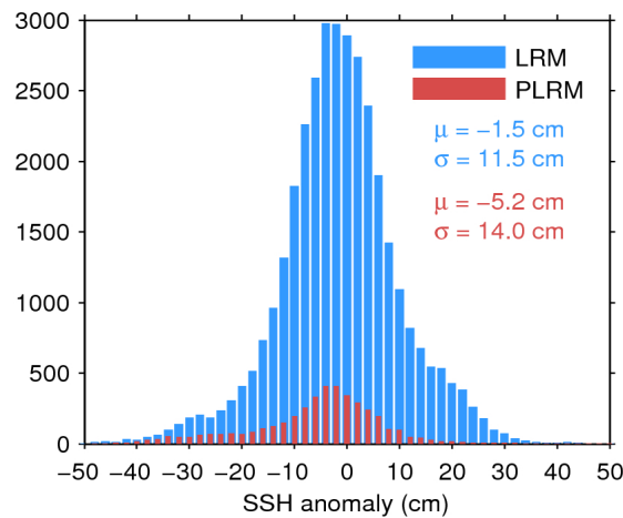
Figure 11. Histogram of science-valid SSH anomaly over oceans and lakes for LRM (blue) and PLRM (red) for 26/11/2015. The mean ( \mu ) and standard deviation ( \sigma ) are also shown. Note that values outside [-50 50] cm are excluded from the histogram for the sake of readability but not from the computation of \mu and \sigma .
