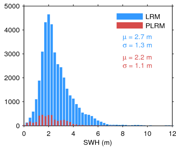
Figure 20. Histogram of science-valid SWH over oceans and lakes for LRM (blue) and PLRM (red) for 26/11/2015. The mean ( \mu ) and standard deviation ( \sigma ) are also shown. Note that values larger than 12 m are excluded from the histogram for the sake of readability but not from the computation of \mu and \sigma .
