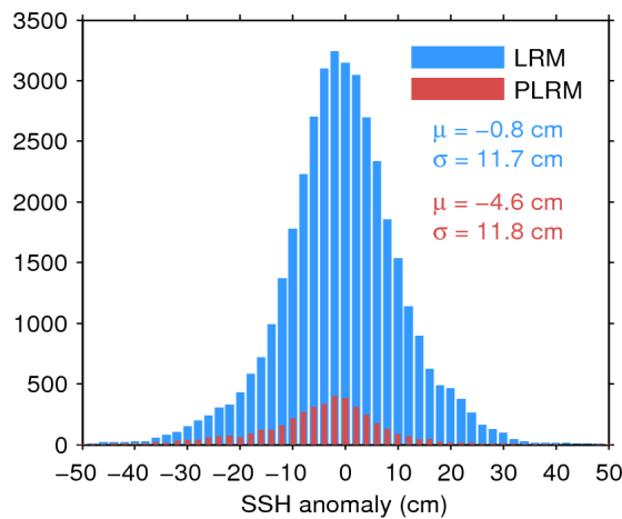
Figure 11. Histogram of science-valid SSH anomaly over oceans and lakes for LRM (blue) and PLRM (red) for 24/11/2015. The mean ( \mu ) and standard deviation ( \sigma ) are also shown. Note that values outside [-50\ 50] cm are excluded from the histogram for the sake of readability but not from the computation of \mu and \sigma .
