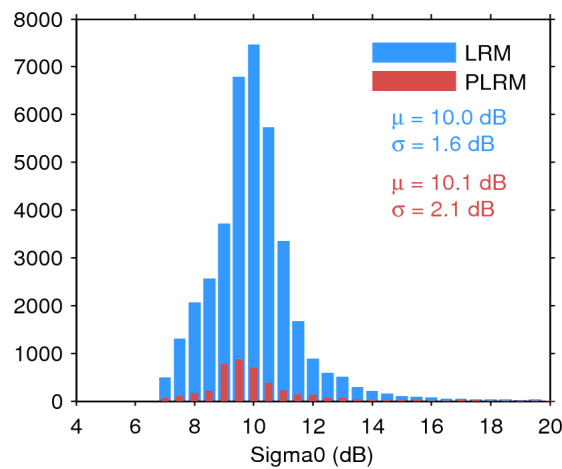
Figure 28. Histogram of science-valid sigma0 over oceans and lakes for LRM (blue) and PLRM (red) for 24/11/2015. The mean ( \mu ) and standard deviation ( \sigma ) are also shown. Note that values outside [4 20] dB are excluded from the histogram for the sake of readability but not from the computation of \mu and \sigma .
