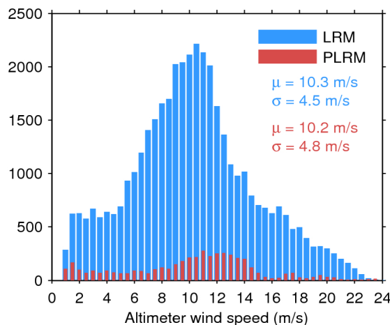
Figure 35. Histogram of science-valid wind over oceans and lakes for LRM (blue) and PLRM (red) for 24/11/2015. The mean ( \mu ) and standard deviation ( \sigma ) are also shown. Note that values larger than 24 m/s are excluded from the histogram for the sake of readability but not from the computation of \mu and \sigma .
