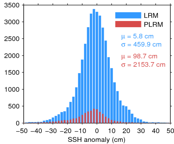
Figure 7. Histogram of flag-valid SSH anomaly over oceans and lakes for LRM (blue) and PLRM (red) for 24/11/2015. The mean ( \mu ) and standard deviation ( \sigma ) are also shown. Note that values outside [-50 50] cm are excluded from the histogram for the sake of readability but not from the computation of \mu and \sigma .
