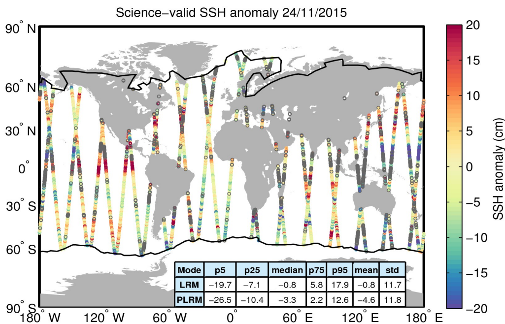
Figure 10. Geographical distribution of science-valid SSH anomaly data over oceans and lakes for 24/11/2015. The statistical values shown in the table refer to the SSH anomaly in cm and are calculated separately for LRM and PLRM regions. The black lines mark the outer limit of the Arctic and Antarctic polar polygons. Gray circles denote records that have been rejected based on the editing criteria described in Table 2.
