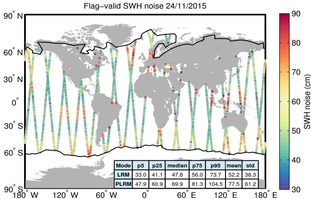
Figure 18. Geographical distribution of flag-valid 20-Hz SWH measurement noise over oceans and lakes for 24/11/2015. The statistical values shown in the table refer to the SWH noise and are calculated separately for LRM and PLRM regions. Measurements taken over polar polygons have been excluded from the computation of the statistical values. The black lines mark the outer limit of the Arctic and Antarctic polar polygons.
