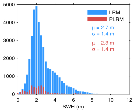
Figure 20. Histogram of science-valid SWH over oceans and lakes for LRM (blue) and PLRM (red) for 24/11/2015. The mean ( \mu ) and standard deviation ( \sigma ) are also shown. Note that values larger than 12 m are excluded from the histogram for the sake of readability but not from the computation of \mu and \sigma .
