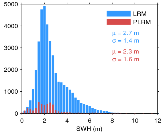
Figure 17. Histogram of flag-valid SWH over oceans and lakes for LRM (blue) and PLRM (red) for 24/11/2015. The mean ( \mu ) and standard deviation ( \sigma ) are also shown. Note that values larger than 12 m are excluded from the histogram for the sake of readability but not from the computation of \mu and \sigma .
