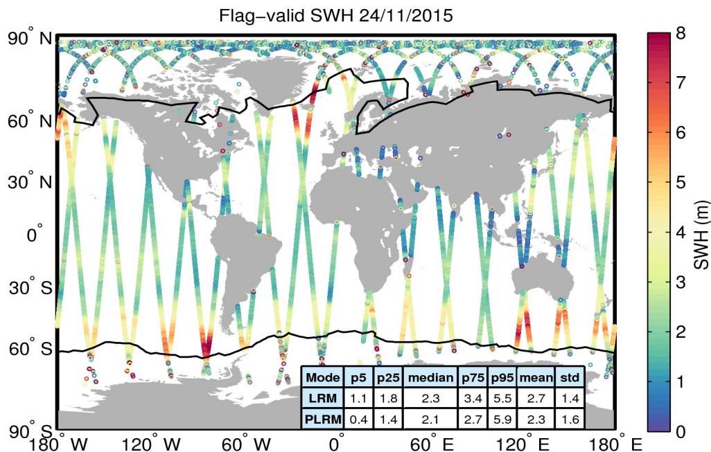
Figure 15. Geographical distribution of flag-valid SWH data over oceans and lakes for 24/11/2015. The statistical values shown in the table refer to the SWH in m and are calculated separately for LRM and PLRM regions. Measurements taken over polar polygons have been excluded from the computation of the statistical values. The black lines mark the outer limit of the Arctic and Antarctic polar polygons.
