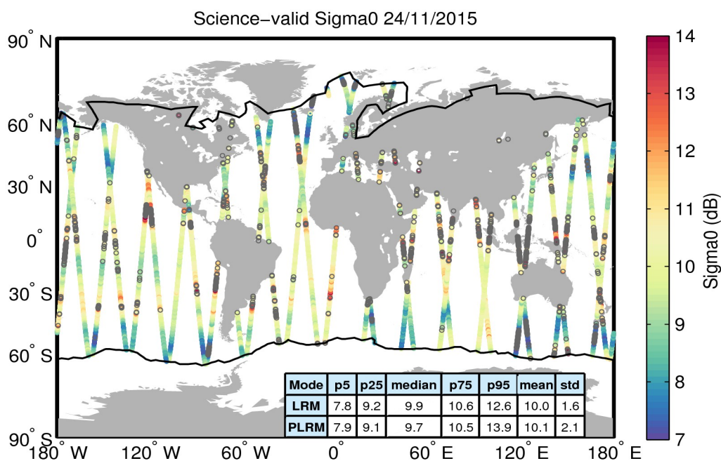
Figure 27. Geographical distribution of science-valid sigma0 data over oceans and lakes for 24/11/2015. The statistical values shown in the table refer to the sigma0 in dB and are calculated separately for LRM and PLRM regions. The black lines mark the outer limit of the Arctic and Antarctic polar polygons. Gray circles denote records that have been rejected based on the editing criteria described in Table 4.
