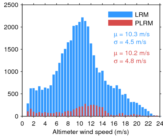
Figure 33. Histogram of flag-valid wind over oceans and lakes for LRM (blue) and PLRM (red) for 24/11/2015. The mean ( \mu ) and standard deviation ( \sigma ) are also shown. Note that values larger than 24 m/s are excluded from the histogram for the sake of readability but not from the computation of \mu and \sigma .
