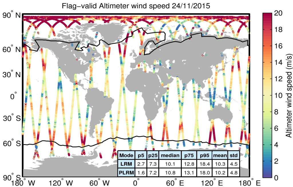
Figure 31. Geographical distribution of flag-valid wind data over oceans and lakes for 24/11/2015. The statistical values shown in the table refer to the wind in m/s and are calculated separately for LRM and PLRM regions. Measurements taken over polar polygons have been excluded from the computation of the statistical values. The black lines mark the outer limit of the Arctic and Antarctic polar polygons.
