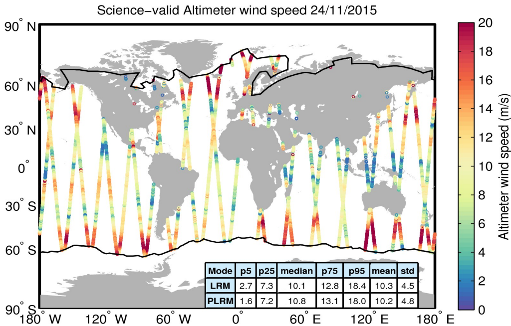
Figure 34. Geographical distribution of science-valid wind data over oceans and lakes for 24/11/2015. The statistical values shown in the table refer to the wind in m/s and are calculated separately for LRM and PLRM regions. The black lines mark the outer limit of the Arctic and Antarctic polar polygons. Gray circles denote records that have been rejected based on the editing criteria described in Table 5.
