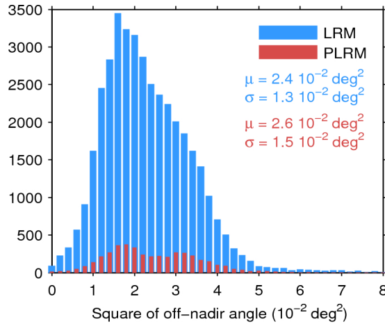
Figure 39. Histogram of flag-valid mispointing over oceans and lakes for LRM (blue) and PLRM (red) for 24/11/2015. Only positive values have been considered. The mean ( \mu ) and standard deviation ( \sigma ) are also shown. Note that values larger than 8 \cdot 10^{-2} \text{ deg}^2 are excluded from the histogram for the sake of readability but not from the computation of \mu and \sigma .
