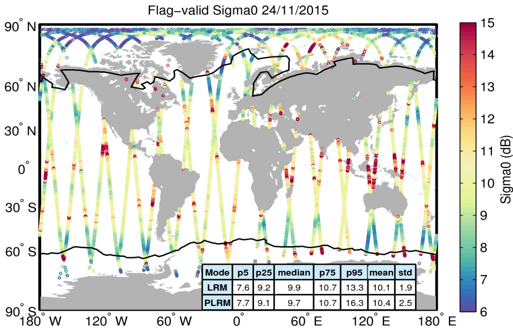
Figure 23. Geographical distribution of flag-valid sigma0 data over oceans and lakes for 24/11/2015. The statistical values shown in the table refer to the sigma0 in dB and are calculated separately for LRM and PLRM regions. Measurements taken over polar polygons have been excluded from the computation of the statistical values. The black lines mark the outer limit of the Arctic and Antarctic polar polygons.
