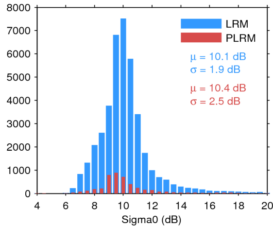
Figure 25. Histogram of flag-valid sigma0 over oceans and lakes for LRM (blue) and PLRM (red) for 24/11/2015. The mean ( \mu ) and standard deviation ( \sigma ) are also shown. Note that values outside [4 20] dB are excluded from the histogram for the sake of readability but not from the computation of \mu and \sigma .
