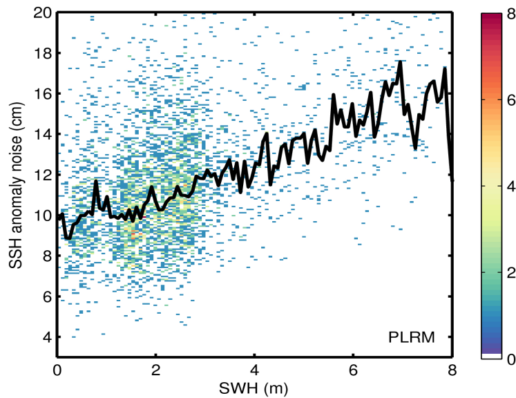
Figure 9. 2D histogram showing flag-valid SSH anomaly noise as a function of SWH for LRM (top) and PLRM (bottom) for 24/11/2015. The black line denotes the median SSH anomaly noise as a function of SWH.
