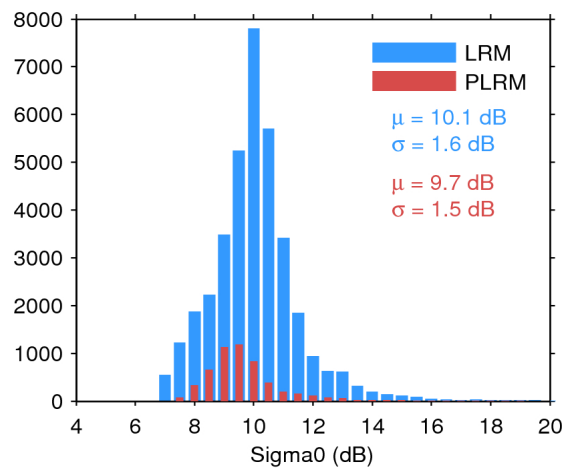
Figure 28. Histogram of science-valid sigma0 over oceans and lakes for LRM (blue) and PLRM (red) for 23/11/2015. The mean ( \mu ) and standard deviation ( \sigma ) are also shown. Note that values outside [4 20] dB are excluded from the histogram for the sake of readability but not from the computation of \mu and \sigma .
