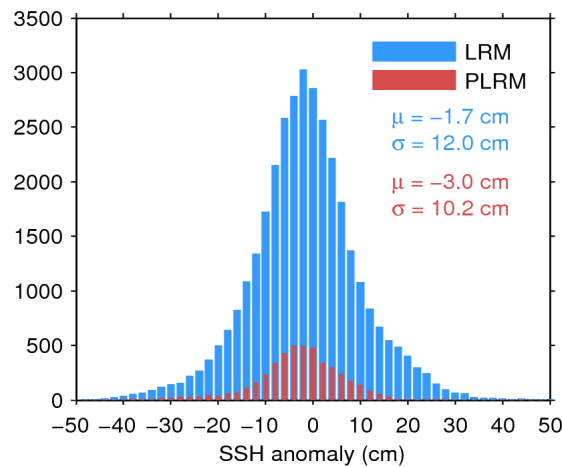
Figure 11. Histogram of science-valid SSH anomaly over oceans and lakes for LRM (blue) and PLRM (red) for 23/11/2015. The mean ( \mu ) and standard deviation ( \sigma ) are also shown. Note that values outside [-50 50] cm are excluded from the histogram for the sake of readability but not from the computation of \mu and \sigma .
