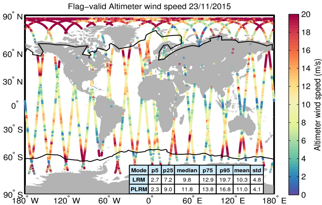
Figure 31. Geographical distribution of flag-valid wind data over oceans and lakes for 23/11/2015. The statistical values shown in the table refer to the wind in m/s and are calculated separately for LRM and PLRM regions. Measurements taken over polar polygons have been excluded from the computation of the statistical values. The black lines mark the outer limit of the Arctic and Antarctic polar polygons.
