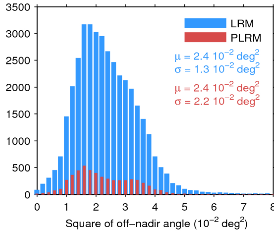
Figure 39. Histogram of flag-valid mispointing over oceans and lakes for LRM (blue) and PLRM (red) for 23/11/2015. Only positive values have been considered. The mean ( \mu ) and standard deviation ( \sigma ) are also shown. Note that values larger than 8 \cdot 10^{-2} \text{ deg}^2 are excluded from the histogram for the sake of readability but not from the computation of \mu and \sigma .
