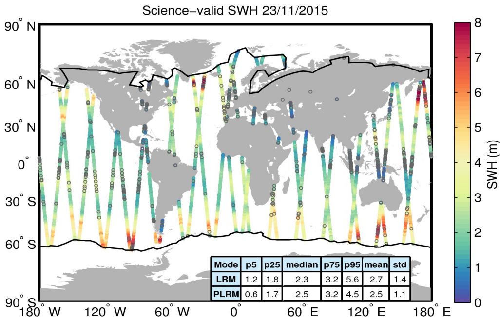
Figure 19. Geographical distribution of science-valid SWH data over oceans and lakes for 23/11/2015. The statistical values shown in the table refer to the SWH in m and are calculated separately for LRM and PLRM regions. The black lines mark the outer limit of the Arctic and Antarctic polar polygons. Gray circles denote records that have been rejected based on the editing criteria described in Table 3.
