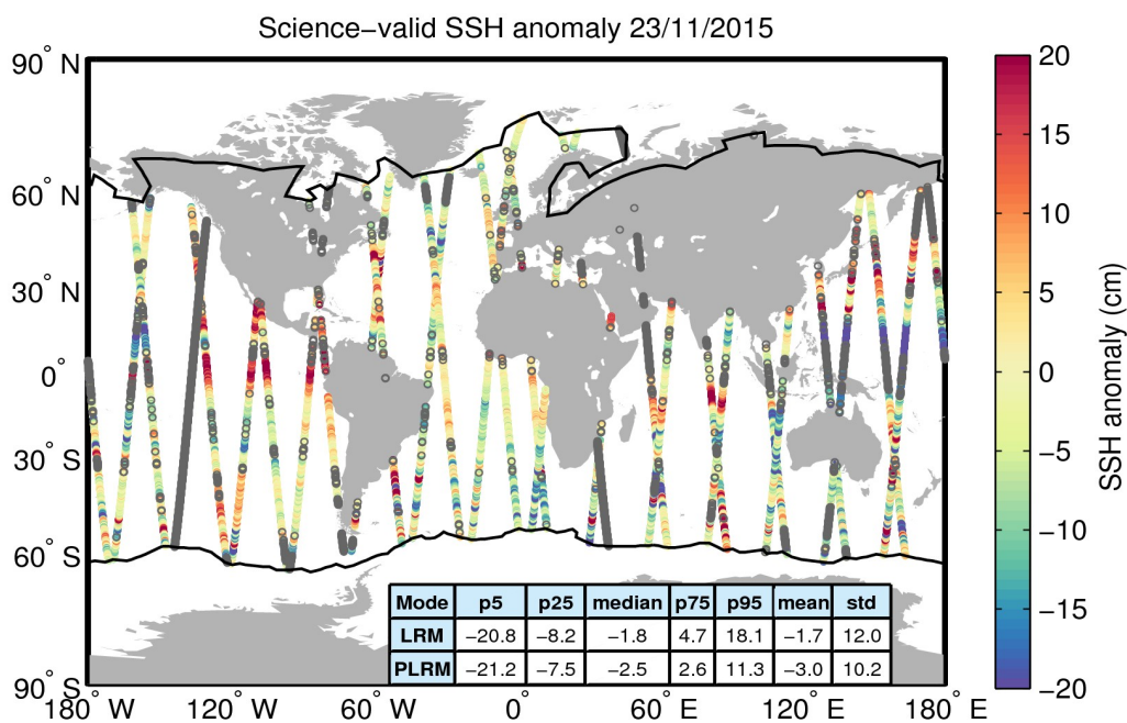
Figure 10. Geographical distribution of science-valid SSH anomaly data over oceans and lakes for 23/11/2015. The statistical values shown in the table refer to the SSH anomaly in cm and are calculated separately for LRM and PLRM regions. The black lines mark the outer limit of the Arctic and Antarctic polar polygons. Gray circles denote records that have been rejected based on the editing criteria described in Table 2.
