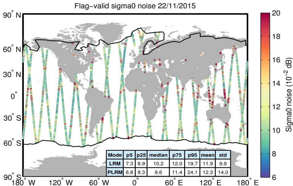
Figure 26. Geographical distribution of flag-valid 20-Hz sigma0 measurement noise over oceans and lakes for 22/11/2015. The statistical values shown in the table refer to the sigma0 noise and are calculated separately for LRM and PLRM regions. Measurements taken over polar polygons have been excluded from the computation of the statistical values. The black lines mark the outer limit of the Arctic and Antarctic polar polygons.
