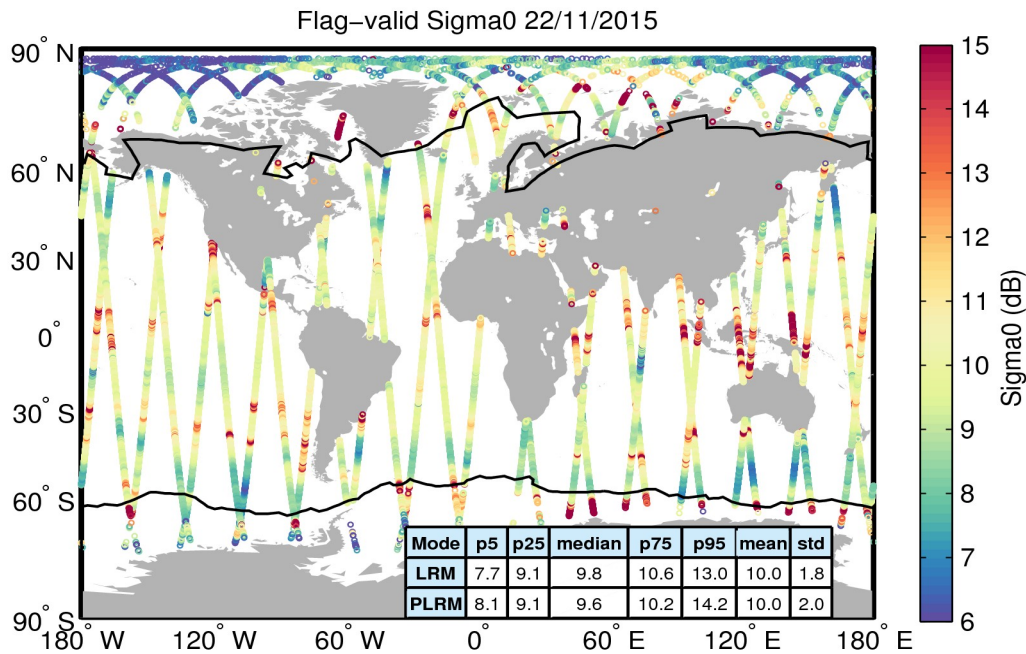
Figure 23. Geographical distribution of flag-valid sigma0 data over oceans and lakes for 22/11/2015. The statistical values shown in the table refer to the sigma0 in dB and are calculated separately for LRM and PLRM regions. Measurements taken over polar polygons have been excluded from the computation of the statistical values. The black lines mark the outer limit of the Arctic and Antarctic polar polygons.
