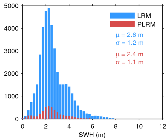
Figure 20. Histogram of science-valid SWH over oceans and lakes for LRM (blue) and PLRM (red) for 22/11/2015. The mean ( \mu ) and standard deviation ( \sigma ) are also shown. Note that values larger than 12 m are excluded from the histogram for the sake of readability but not from the computation of \mu and \sigma .
