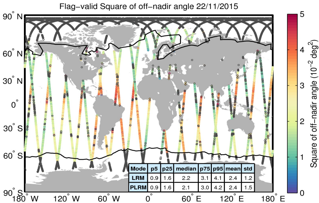
Figure 37. Geographical distribution of flag-valid mispointing data over oceans and lakes for 22/11/2015. The statistical values shown in the table refer to the mispointing in 10^{-2} deg 2 and are calculated separately for LRM and PLRM regions. Measurements taken over polar polygons have been excluded from the computation of the statistical values. The black lines mark the outer limit of the Arctic and Antarctic polar polygons. Gray circles denote negative values.
