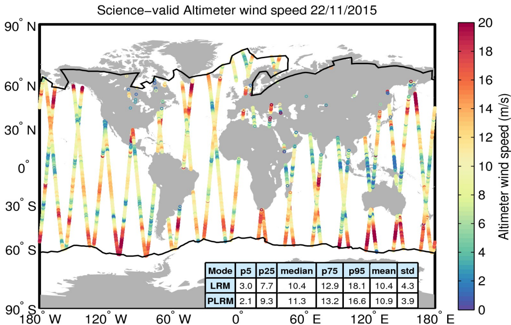
Figure 34. Geographical distribution of science-valid wind data over oceans and lakes for 22/11/2015. The statistical values shown in the table refer to the wind in m/s and are calculated separately for LRM and PLRM regions. The black lines mark the outer limit of the Arctic and Antarctic polar polygons. Gray circles denote records that have been rejected based on the editing criteria described in Table 5.
