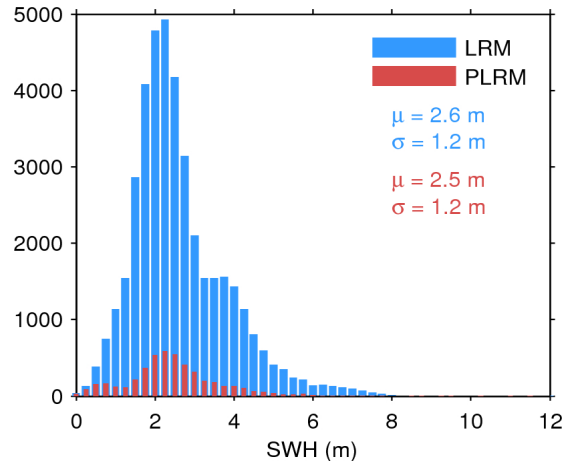
Figure 17. Histogram of flag-valid SWH over oceans and lakes for LRM (blue) and PLRM (red) for 22/11/2015. The mean ( \mu ) and standard deviation ( \sigma ) are also shown. Note that values larger than 12 m are excluded from the histogram for the sake of readability but not from the computation of \mu and \sigma .
