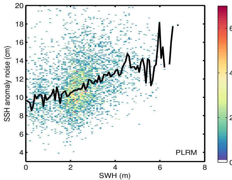
Figure 9. 2D histogram showing flag-valid SSH anomaly noise as a function of SWH for LRM (top) and PLRM (bottom) for 22/11/2015. The black line denotes the median SSH anomaly noise as a function of SWH.
