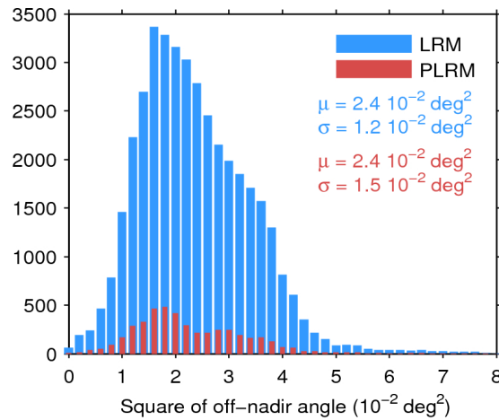
Figure 39. Histogram of flag-valid mispointing over oceans and lakes for LRM (blue) and PLRM (red) for 22/11/2015. Only positive values have been considered. The mean ( \mu ) and standard deviation ( \sigma ) are also shown. Note that values larger than 8 \cdot 10^{-2} \text{ deg}^2 are excluded from the histogram for the sake of readability but not from the computation of \mu and \sigma .
