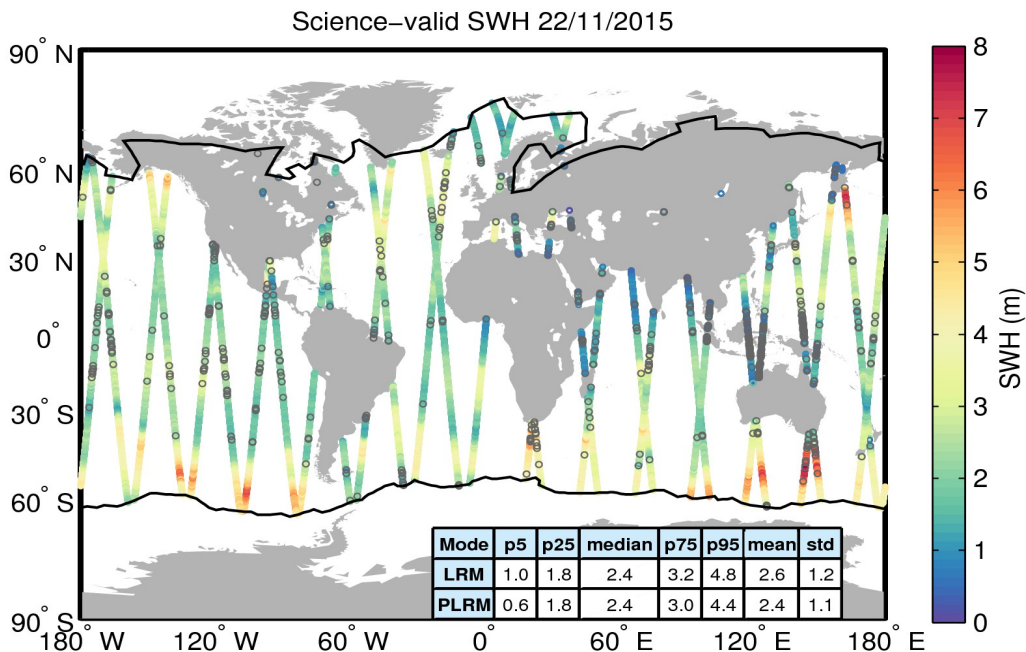
Figure 19. Geographical distribution of science-valid SWH data over oceans and lakes for 22/11/2015. The statistical values shown in the table refer to the SWH in m and are calculated separately for LRM and PLRM regions. The black lines mark the outer limit of the Arctic and Antarctic polar polygons. Gray circles denote records that have been rejected based on the editing criteria described in Table 3.
