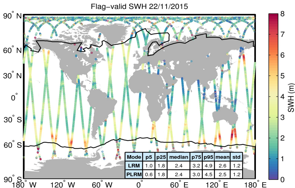
Figure 15. Geographical distribution of flag-valid SWH data over oceans and lakes for 22/11/2015. The statistical values shown in the table refer to the SWH in m and are calculated separately for LRM and PLRM regions. Measurements taken over polar polygons have been excluded from the computation of the statistical values. The black lines mark the outer limit of the Arctic and Antarctic polar polygons.
