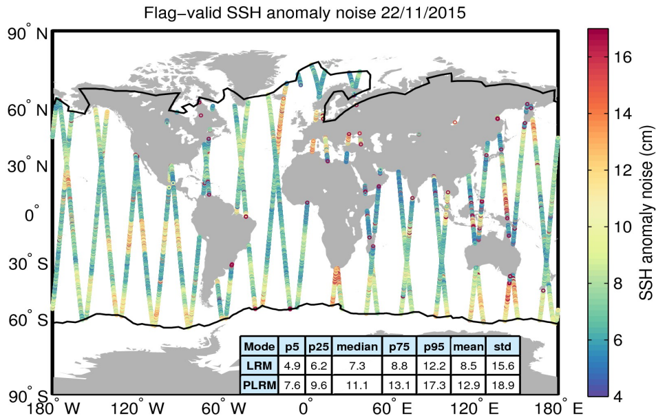
Figure 8. Geographical distribution of flag-valid 20-Hz SSH anomaly measurement noise over oceans and lakes for 22/11/2015. The statistical values shown in the table refer to the SSH anomaly noise and are calculated separately for LRM and PLRM regions. Measurements taken over polar polygons have been excluded from the computation of the statistical values. The black lines mark the outer limit of the Arctic and Antarctic polar polygons.
