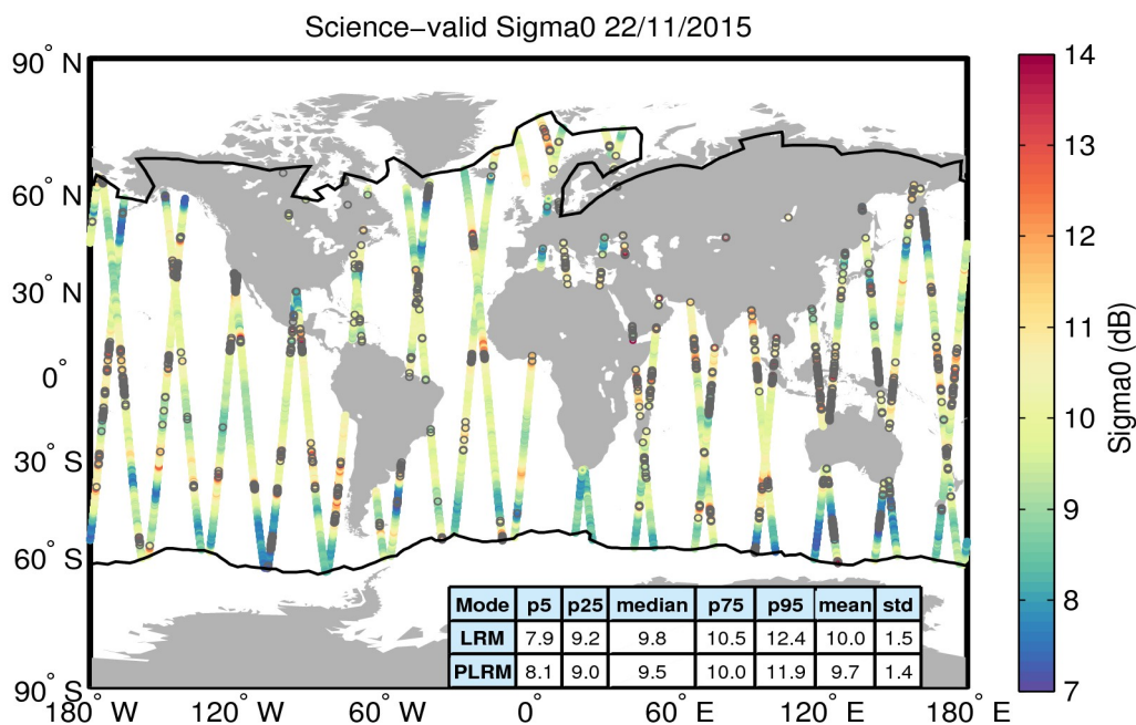
Figure 27. Geographical distribution of science-valid sigma0 data over oceans and lakes for 22/11/2015. The statistical values shown in the table refer to the sigma0 in dB and are calculated separately for LRM and PLRM regions. The black lines mark the outer limit of the Arctic and Antarctic polar polygons. Gray circles denote records that have been rejected based on the editing criteria described in Table 4.
