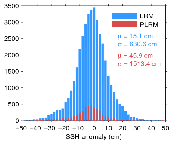
Figure 7. Histogram of flag-valid SSH anomaly over oceans and lakes for LRM (blue) and PLRM (red) for 22/11/2015. The mean ( \mu ) and standard deviation ( \sigma ) are also shown. Note that values outside [-50 50] cm are excluded from the histogram for the sake of readability but not from the computation of \mu and \sigma .
