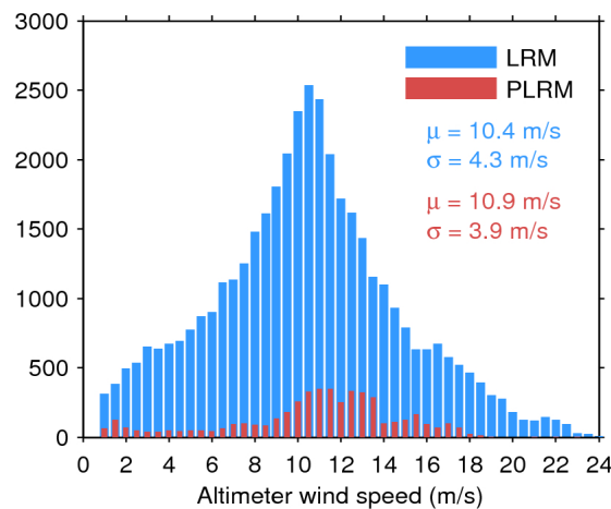
Figure 33. Histogram of flag-valid wind over oceans and lakes for LRM (blue) and PLRM (red) for 22/11/2015. The mean ( \mu ) and standard deviation ( \sigma ) are also shown. Note that values larger than 24 m/s are excluded from the histogram for the sake of readability but not from the computation of \mu and \sigma .
