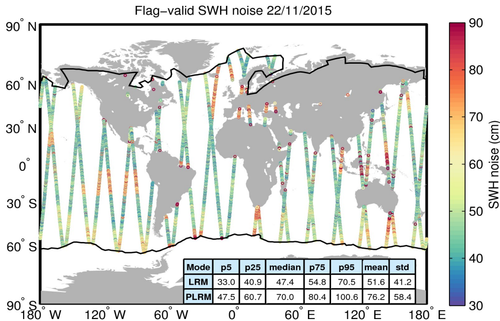
Figure 18. Geographical distribution of flag-valid 20-Hz SWH measurement noise over oceans and lakes for 22/11/2015. The statistical values shown in the table refer to the SWH noise and are calculated separately for LRM and PLRM regions. Measurements taken over polar polygons have been excluded from the computation of the statistical values. The black lines mark the outer limit of the Arctic and Antarctic polar polygons.
