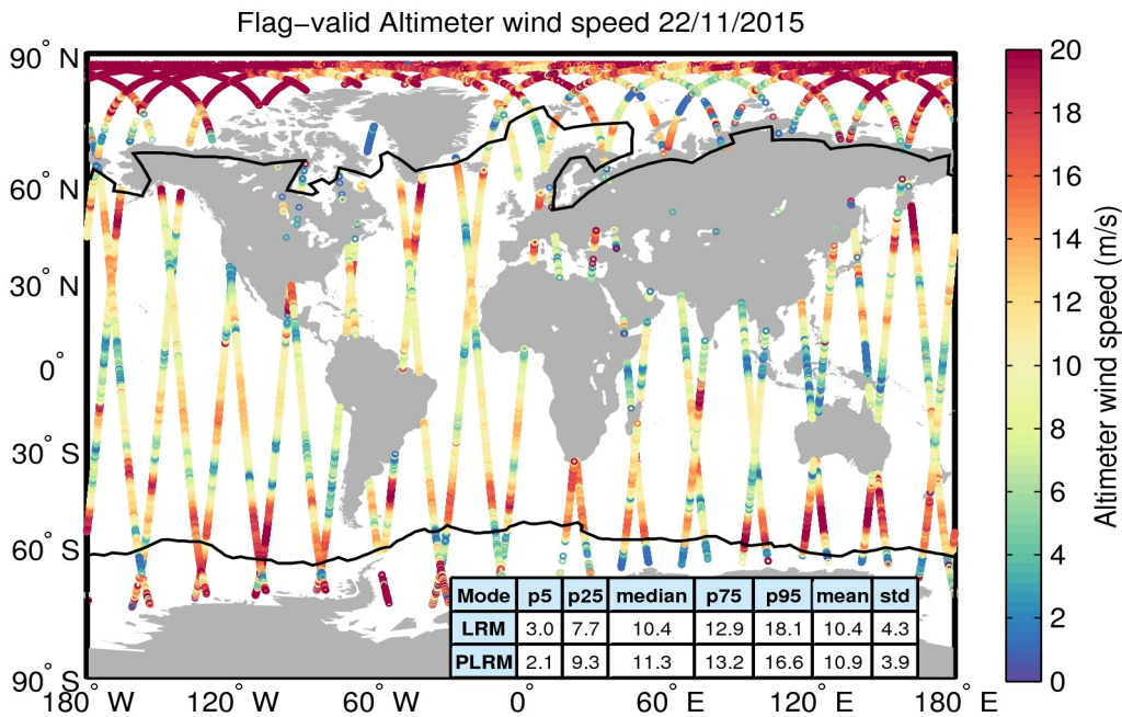
Figure 31. Geographical distribution of flag-valid wind data over oceans and lakes for 22/11/2015. The statistical values shown in the table refer to the wind in m/s and are calculated separately for LRM and PLRM regions. Measurements taken over polar polygons have been excluded from the computation of the statistical values. The black lines mark the outer limit of the Arctic and Antarctic polar polygons.
