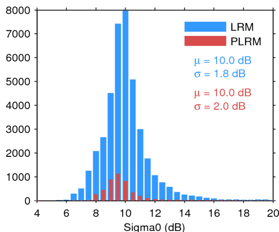
Figure 25. Histogram of flag-valid sigma0 over oceans and lakes for LRM (blue) and PLRM (red) for 22/11/2015. The mean ( \mu ) and standard deviation ( \sigma ) are also shown. Note that values outside [4 20] dB are excluded from the histogram for the sake of readability but not from the computation of \mu and \sigma .
