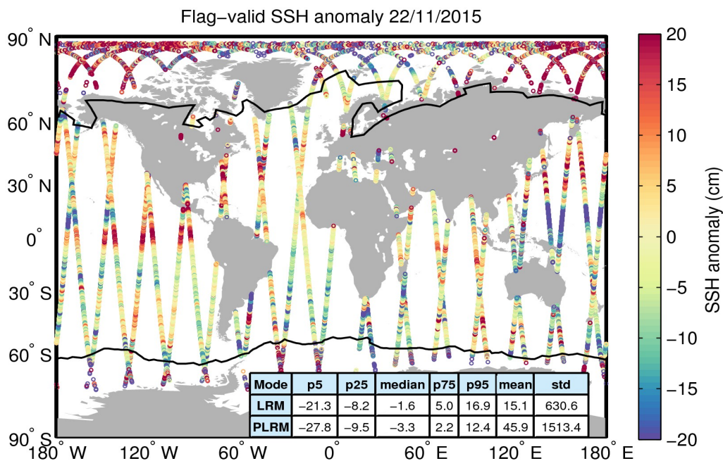
Figure 5. Geographical distribution of flag-valid 1-Hz SSH anomaly data over oceans and lakes for 22/11/2015. The statistical values shown in the table refer to the SSH anomaly in cm and are calculated separately for LRM and PLRM regions. Measurements taken over polar polygons have been excluded from the computation of the statistical values. The black lines mark the outer limit of the Arctic and Antarctic polar polygons.
