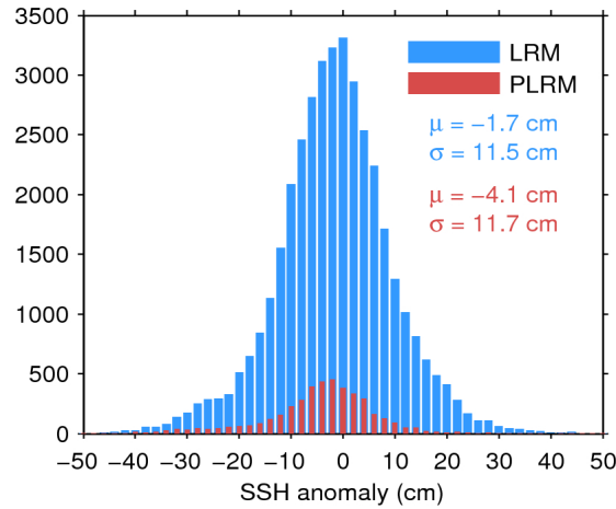
Figure 11. Histogram of science-valid SSH anomaly over oceans and lakes for LRM (blue) and PLRM (red) for 22/11/2015. The mean ( \mu ) and standard deviation ( \sigma ) are also shown. Note that values outside [-50 50] cm are excluded from the histogram for the sake of readability but not from the computation of \mu and \sigma .
