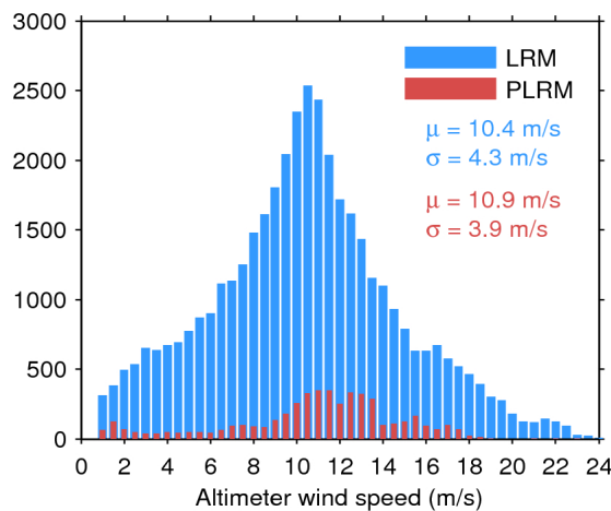
Figure 35. Histogram of science-valid wind over oceans and lakes for LRM (blue) and PLRM (red) for 22/11/2015. The mean ( \mu ) and standard deviation ( \sigma ) are also shown. Note that values larger than 24 m/s are excluded from the histogram for the sake of readability but not from the computation of \mu and \sigma .
