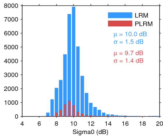
Figure 28. Histogram of science-valid sigma0 over oceans and lakes for LRM (blue) and PLRM (red) for 22/11/2015. The mean ( \mu ) and standard deviation ( \sigma ) are also shown. Note that values outside [4 20] dB are excluded from the histogram for the sake of readability but not from the computation of \mu and \sigma .
