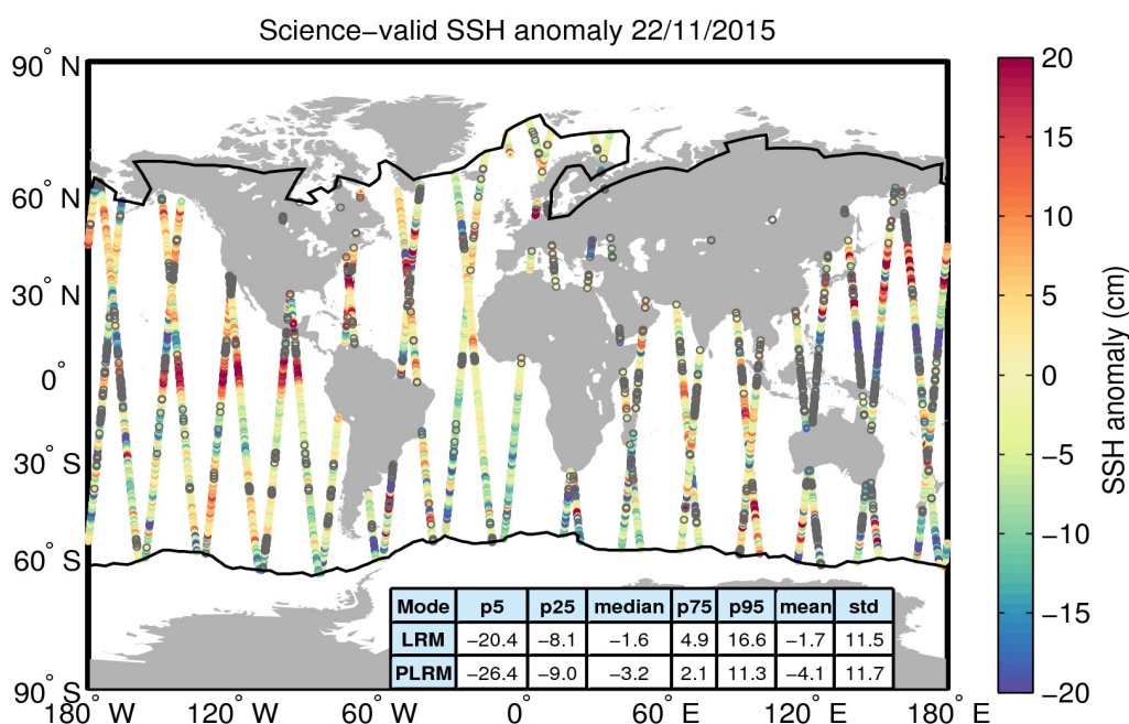
Figure 10. Geographical distribution of science-valid SSH anomaly data over oceans and lakes for 22/11/2015. The statistical values shown in the table refer to the SSH anomaly in cm and are calculated separately for LRM and PLRM regions. The black lines mark the outer limit of the Arctic and Antarctic polar polygons. Gray circles denote records that have been rejected based on the editing criteria described in Table 2.
