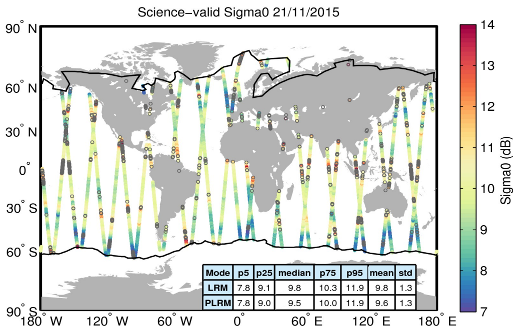
Figure 27. Geographical distribution of science-valid sigma0 data over oceans and lakes for 21/11/2015. The statistical values shown in the table refer to the sigma0 in dB and are calculated separately for LRM and PLRM regions. The black lines mark the outer limit of the Arctic and Antarctic polar polygons. Gray circles denote records that have been rejected based on the editing criteria described in Table 4.
