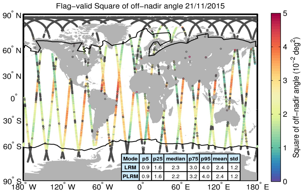
Figure 37. Geographical distribution of flag-valid mispointing data over oceans and lakes for 21/11/2015. The statistical values shown in the table refer to the mispointing in 10^{-2} deg 2 and are calculated separately for LRM and PLRM regions. Measurements taken over polar polygons have been excluded from the computation of the statistical values. The black lines mark the outer limit of the Arctic and Antarctic polar polygons. Gray circles denote negative values.
