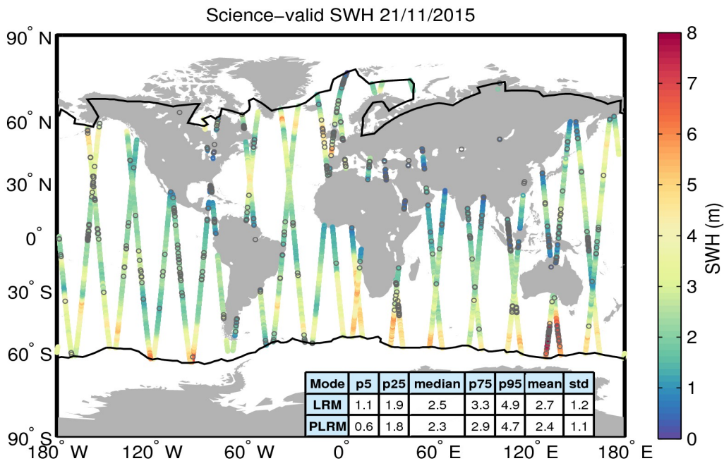
Figure 19. Geographical distribution of science-valid SWH data over oceans and lakes for 21/11/2015. The statistical values shown in the table refer to the SWH in m and are calculated separately for LRM and PLRM regions. The black lines mark the outer limit of the Arctic and Antarctic polar polygons. Gray circles denote records that have been rejected based on the editing criteria described in Table 3.
