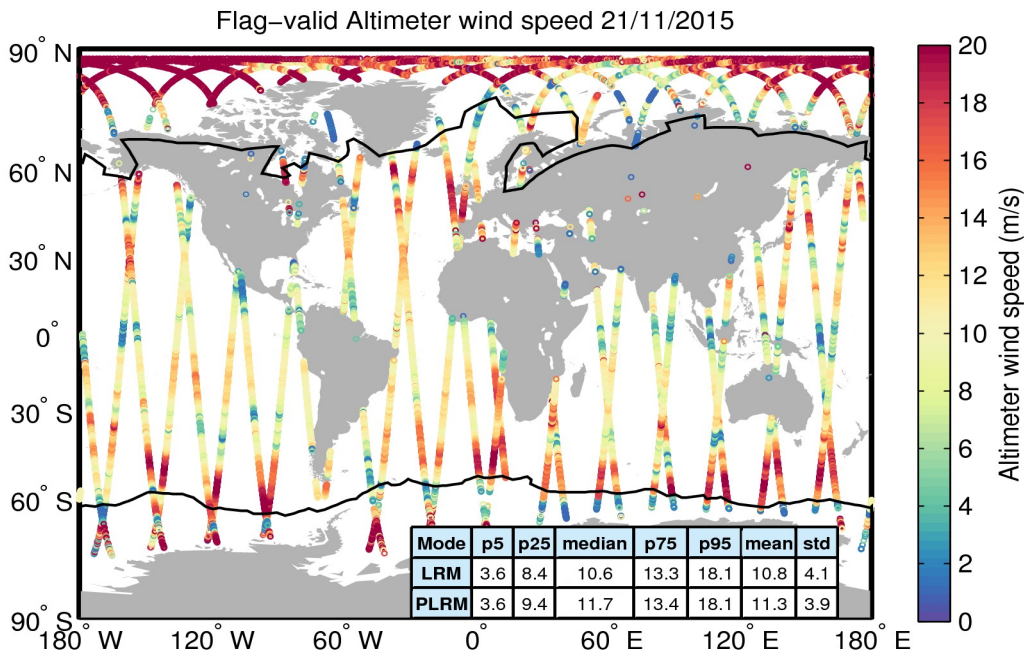
Figure 31. Geographical distribution of flag-valid wind data over oceans and lakes for 21/11/2015. The statistical values shown in the table refer to the wind in m/s and are calculated separately for LRM and PLRM regions. Measurements taken over polar polygons have been excluded from the computation of the statistical values. The black lines mark the outer limit of the Arctic and Antarctic polar polygons.
