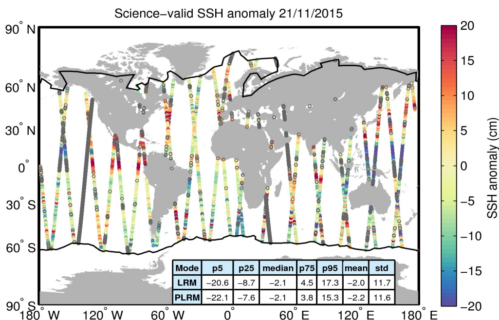
Figure 10. Geographical distribution of science-valid SSH anomaly data over oceans and lakes for 21/11/2015. The statistical values shown in the table refer to the SSH anomaly in cm and are calculated separately for LRM and PLRM regions. The black lines mark the outer limit of the Arctic and Antarctic polar polygons. Gray circles denote records that have been rejected based on the editing criteria described in Table 2.
