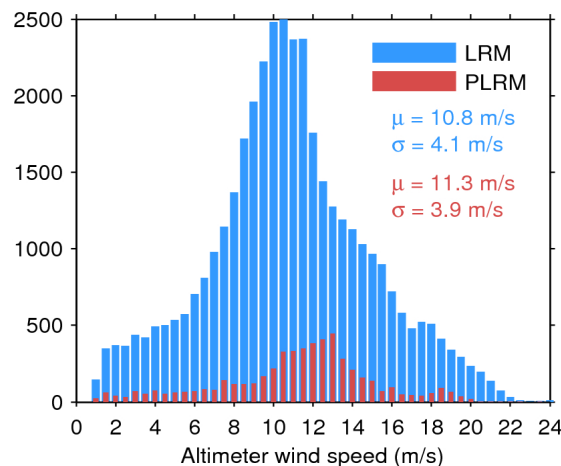
Figure 35. Histogram of science-valid wind over oceans and lakes for LRM (blue) and PLRM (red) for 21/11/2015. The mean ( \mu ) and standard deviation ( \sigma ) are also shown. Note that values larger than 24 m/s are excluded from the histogram for the sake of readability but not from the computation of \mu and \sigma .
