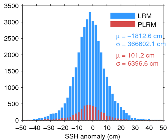
Figure 7. Histogram of flag-valid SSH anomaly over oceans and lakes for LRM (blue) and PLRM (red) for 21/11/2015. The mean ( \mu ) and standard deviation ( \sigma ) are also shown. Note that values outside [-50\ 50] cm are excluded from the histogram for the sake of readability but not from the computation of \mu and \sigma .
