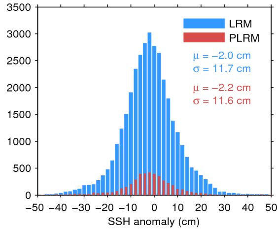
Figure 11. Histogram of science-valid SSH anomaly over oceans and lakes for LRM (blue) and PLRM (red) for 21/11/2015. The mean ( \mu ) and standard deviation ( \sigma ) are also shown. Note that values outside [-50\ 50] cm are excluded from the histogram for the sake of readability but not from the computation of \mu and \sigma .
