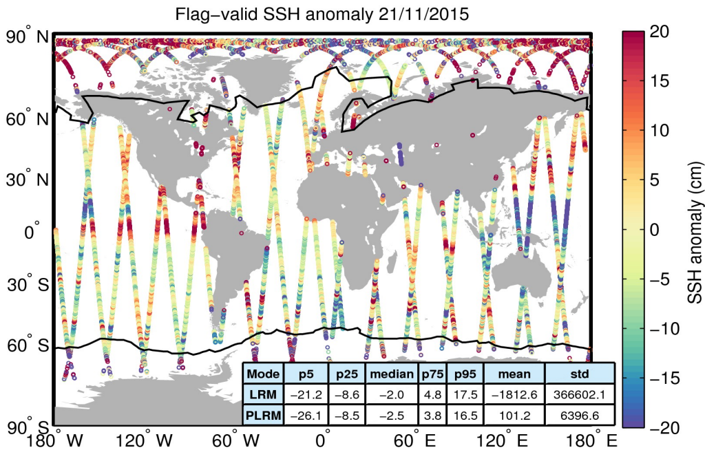
Figure 5. Geographical distribution of flag-valid 1-Hz SSH anomaly data over oceans and lakes for 21/11/2015. The statistical values shown in the table refer to the SSH anomaly in cm and are calculated separately for LRM and PLRM regions. Measurements taken over polar polygons have been excluded from the computation of the statistical values. The black lines mark the outer limit of the Arctic and Antarctic polar polygons.
