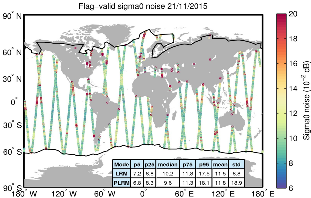
Figure 26. Geographical distribution of flag-valid 20-Hz sigma0 measurement noise over oceans and lakes for 21/11/2015. The statistical values shown in the table refer to the sigma0 noise and are calculated separately for LRM and PLRM regions. Measurements taken over polar polygons have been excluded from the computation of the statistical values. The black lines mark the outer limit of the Arctic and Antarctic polar polygons.
