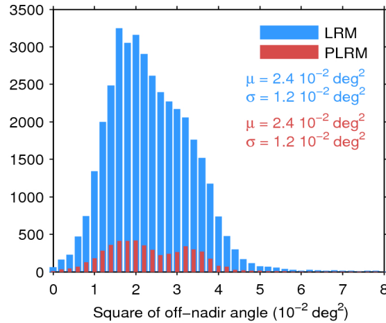
Figure 39. Histogram of flag-valid mispointing over oceans and lakes for LRM (blue) and PLRM (red) for 21/11/2015. Only positive values have been considered. The mean ( \mu ) and standard deviation ( \sigma ) are also shown. Note that values larger than 8 \cdot 10^{-2} \text{ deg}^2 are excluded from the histogram for the sake of readability but not from the computation of \mu and \sigma .
