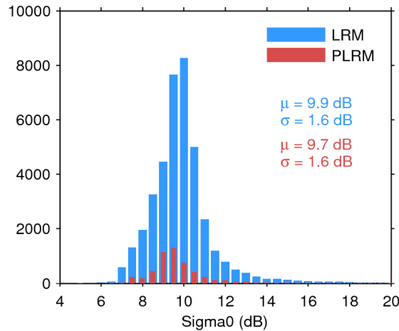
Figure 25. Histogram of flag-valid sigma0 over oceans and lakes for LRM (blue) and PLRM (red) for 21/11/2015. The mean ( \mu ) and standard deviation ( \sigma ) are also shown. Note that values outside [4 20] dB are excluded from the histogram for the sake of readability but not from the computation of \mu and \sigma .
