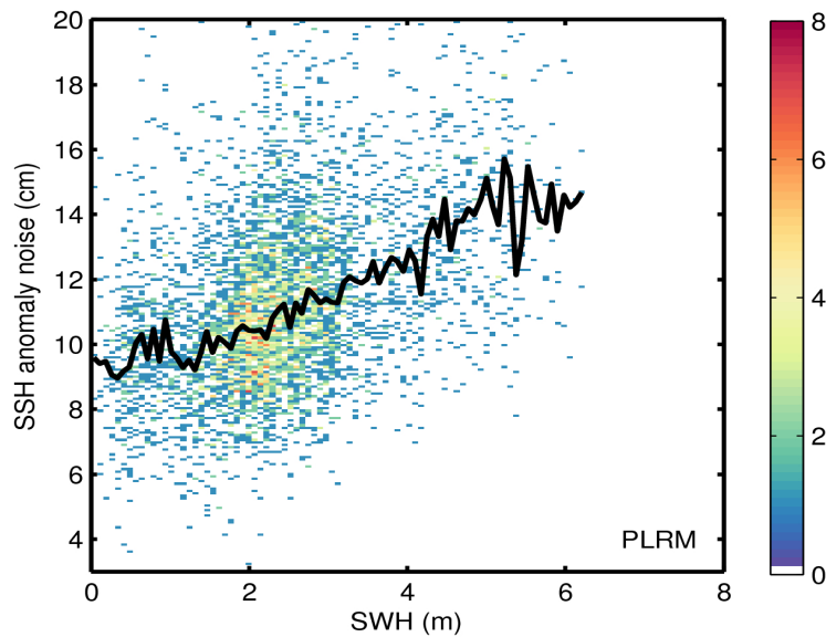
Figure 9. 2D histogram showing flag-valid SSH anomaly noise as a function of SWH for LRM (top) and PLRM (bottom) for 21/11/2015. The black line denotes the median SSH anomaly noise as a function of SWH.
