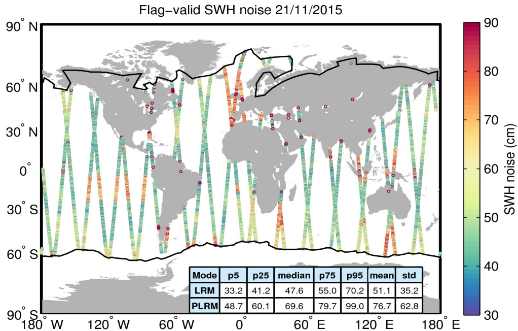
Figure 18. Geographical distribution of flag-valid 20-Hz SWH measurement noise over oceans and lakes for 21/11/2015. The statistical values shown in the table refer to the SWH noise and are calculated separately for LRM and PLRM regions. Measurements taken over polar polygons have been excluded from the computation of the statistical values. The black lines mark the outer limit of the Arctic and Antarctic polar polygons.
