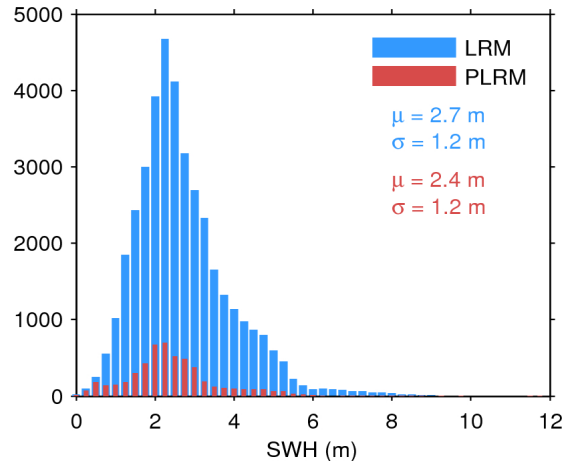
Figure 17. Histogram of flag-valid SWH over oceans and lakes for LRM (blue) and PLRM (red) for 21/11/2015. The mean ( \mu ) and standard deviation ( \sigma ) are also shown. Note that values larger than 12 m are excluded from the histogram for the sake of readability but not from the computation of \mu and \sigma .
