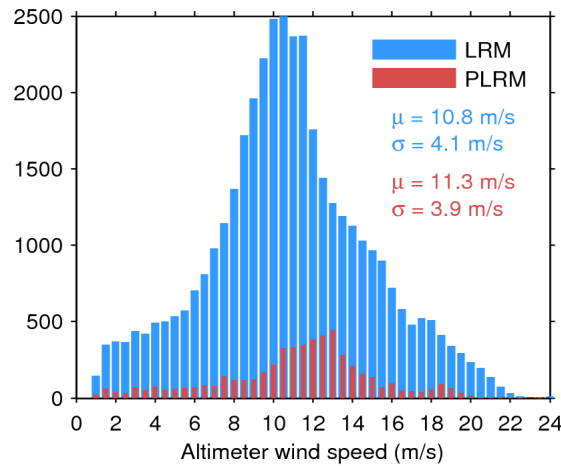
Figure 33. Histogram of flag-valid wind over oceans and lakes for LRM (blue) and PLRM (red) for 21/11/2015. The mean ( \mu ) and standard deviation ( \sigma ) are also shown. Note that values larger than 24 m/s are excluded from the histogram for the sake of readability but not from the computation of \mu and \sigma .
