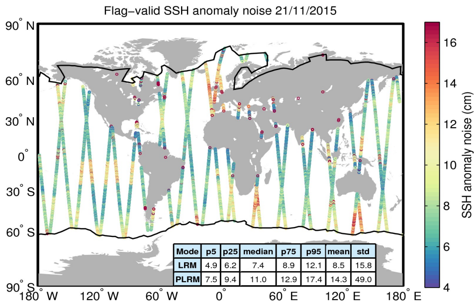
Figure 8. Geographical distribution of flag-valid 20-Hz SSH anomaly measurement noise over oceans and lakes for 21/11/2015. The statistical values shown in the table refer to the SSH anomaly noise and are calculated separately for LRM and PLRM regions. Measurements taken over polar polygons have been excluded from the computation of the statistical values. The black lines mark the outer limit of the Arctic and Antarctic polar polygons.
