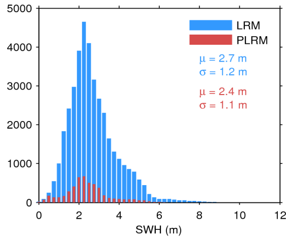
Figure 20. Histogram of science-valid SWH over oceans and lakes for LRM (blue) and PLRM (red) for 21/11/2015. The mean ( \mu ) and standard deviation ( \sigma ) are also shown. Note that values larger than 12 m are excluded from the histogram for the sake of readability but not from the computation of \mu and \sigma .
