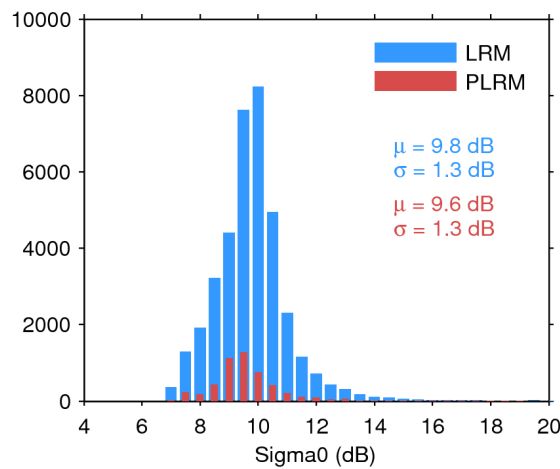
Figure 28. Histogram of science-valid sigma0 over oceans and lakes for LRM (blue) and PLRM (red) for 21/11/2015. The mean ( \mu ) and standard deviation ( \sigma ) are also shown. Note that values outside [4 20] dB are excluded from the histogram for the sake of readability but not from the computation of \mu and \sigma .
