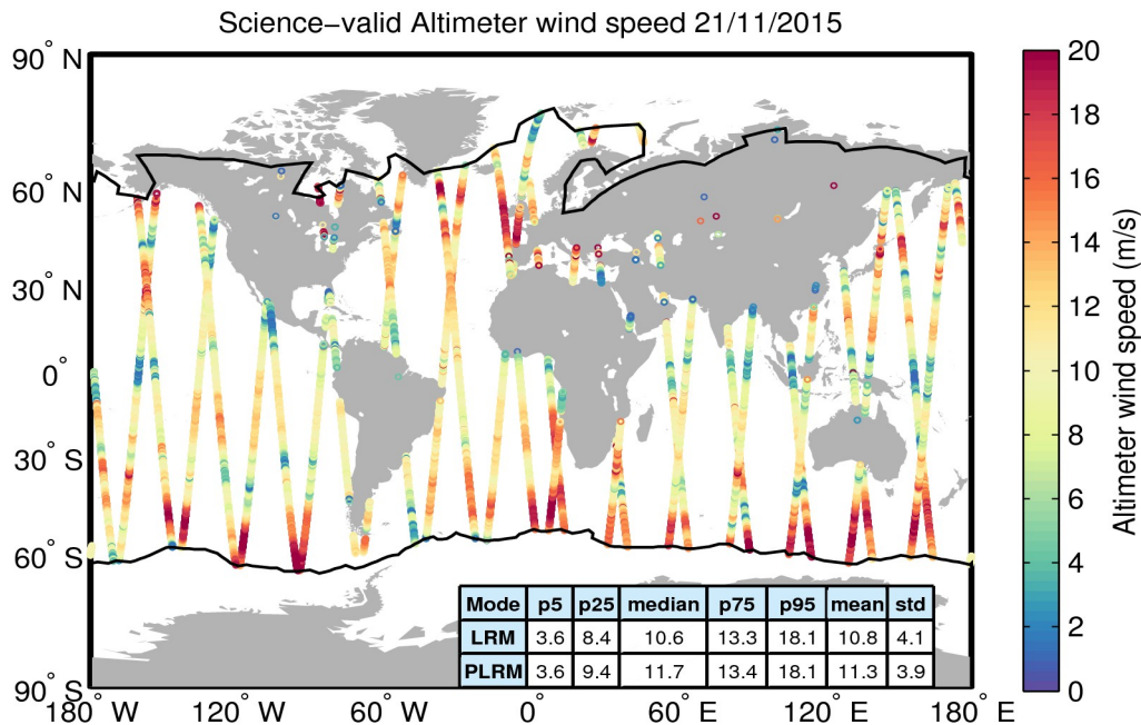
Figure 34. Geographical distribution of science-valid wind data over oceans and lakes for 21/11/2015. The statistical values shown in the table refer to the wind in m/s and are calculated separately for LRM and PLRM regions. The black lines mark the outer limit of the Arctic and Antarctic polar polygons. Gray circles denote records that have been rejected based on the editing criteria described in Table 5.
