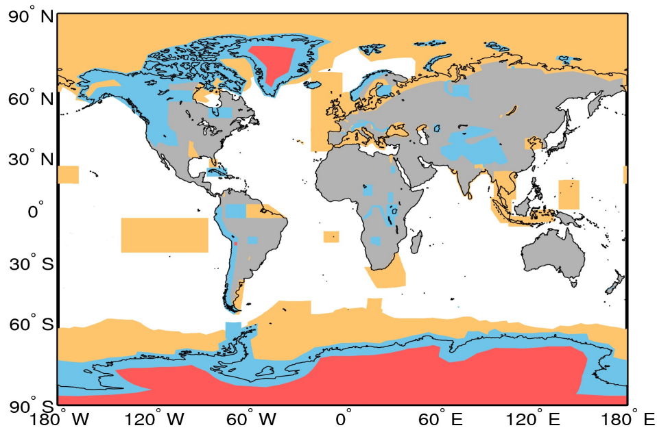
Figure A1. Extent of the regions defining the geographical mode mask for 21/11/2015. The regions where SAR, and SARIn are operated are denoted by the orange and blue polygons, respectively. LRM is operated over areas of the continental ice sheets (red polygons) and over oceans and land not covered by other modes.
