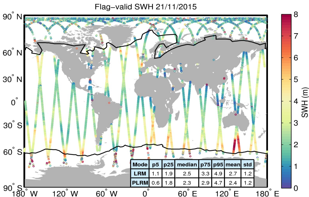
Figure 15. Geographical distribution of flag-valid SWH data over oceans and lakes for 21/11/2015. The statistical values shown in the table refer to the SWH in m and are calculated separately for LRM and PLRM regions. Measurements taken over polar polygons have been excluded from the computation of the statistical values. The black lines mark the outer limit of the Arctic and Antarctic polar polygons.
