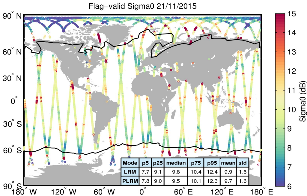
Figure 23. Geographical distribution of flag-valid sigma0 data over oceans and lakes for 21/11/2015. The statistical values shown in the table refer to the sigma0 in dB and are calculated separately for LRM and PLRM regions. Measurements taken over polar polygons have been excluded from the computation of the statistical values. The black lines mark the outer limit of the Arctic and Antarctic polar polygons.
