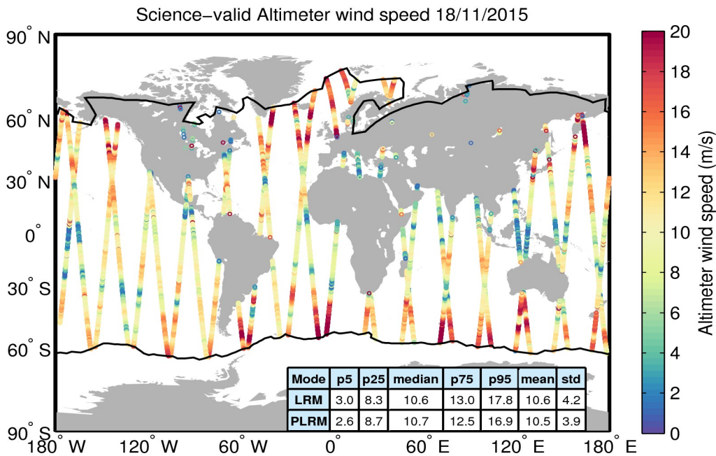
Figure 34. Geographical distribution of science-valid wind data over oceans and lakes for 18/11/2015. The statistical values shown in the table refer to the wind in m/s and are calculated separately for LRM and PLRM regions. The black lines mark the outer limit of the Arctic and Antarctic polar polygons. Gray circles denote records that have been rejected based on the editing criteria described in Table 5.
