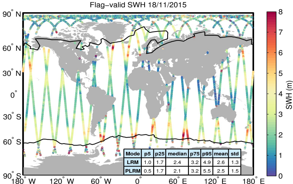
Figure 15. Geographical distribution of flag-valid SWH data over oceans and lakes for 18/11/2015. The statistical values shown in the table refer to the SWH in m and are calculated separately for LRM and PLRM regions. Measurements taken over polar polygons have been excluded from the computation of the statistical values. The black lines mark the outer limit of the Arctic and Antarctic polar polygons.
