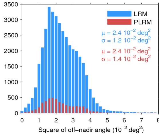
Figure 39. Histogram of flag-valid mispointing over oceans and lakes for LRM (blue) and PLRM (red) for 18/11/2015. Only positive values have been considered. The mean ( \mu ) and standard deviation ( \sigma ) are also shown. Note that values larger than 8 \cdot 10^{-2} \text{ deg}^2 are excluded from the histogram for the sake of readability but not from the computation of \mu and \sigma .
