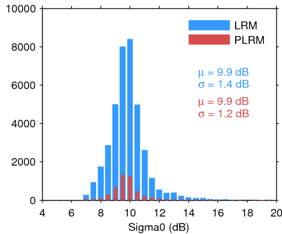
Figure 28. Histogram of science-valid sigma0 over oceans and lakes for LRM (blue) and PLRM (red) for 18/11/2015. The mean ( \mu ) and standard deviation ( \sigma ) are also shown. Note that values outside [4 20] dB are excluded from the histogram for the sake of readability but not from the computation of \mu and \sigma .
