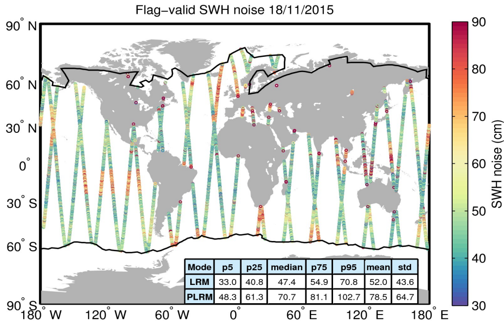
Figure 18. Geographical distribution of flag-valid 20-Hz SWH measurement noise over oceans and lakes for 18/11/2015. The statistical values shown in the table refer to the SWH noise and are calculated separately for LRM and PLRM regions. Measurements taken over polar polygons have been excluded from the computation of the statistical values. The black lines mark the outer limit of the Arctic and Antarctic polar polygons.
