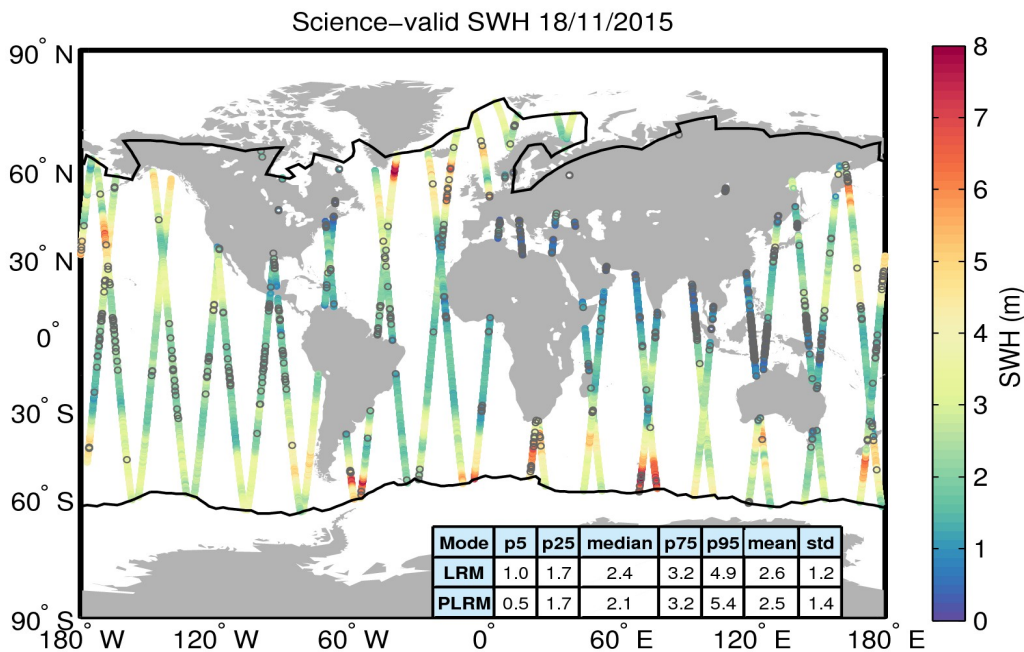
Figure 19. Geographical distribution of science-valid SWH data over oceans and lakes for 18/11/2015. The statistical values shown in the table refer to the SWH in m and are calculated separately for LRM and PLRM regions. The black lines mark the outer limit of the Arctic and Antarctic polar polygons. Gray circles denote records that have been rejected based on the editing criteria described in Table 3.
