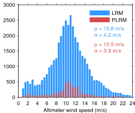
Figure 35. Histogram of science-valid wind over oceans and lakes for LRM (blue) and PLRM (red) for 18/11/2015. The mean ( \mu ) and standard deviation ( \sigma ) are also shown. Note that values larger than 24 m/s are excluded from the histogram for the sake of readability but not from the computation of \mu and \sigma .
