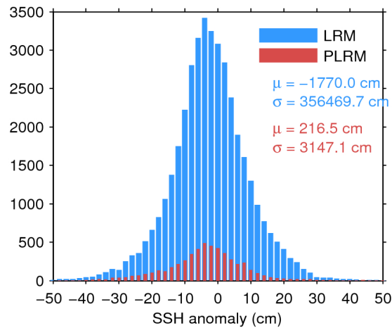
Figure 7. Histogram of flag-valid SSH anomaly over oceans and lakes for LRM (blue) and PLRM (red) for 18/11/2015. The mean ( \mu ) and standard deviation ( \sigma ) are also shown. Note that values outside [-50 50] cm are excluded from the histogram for the sake of readability but not from the computation of \mu and \sigma .
