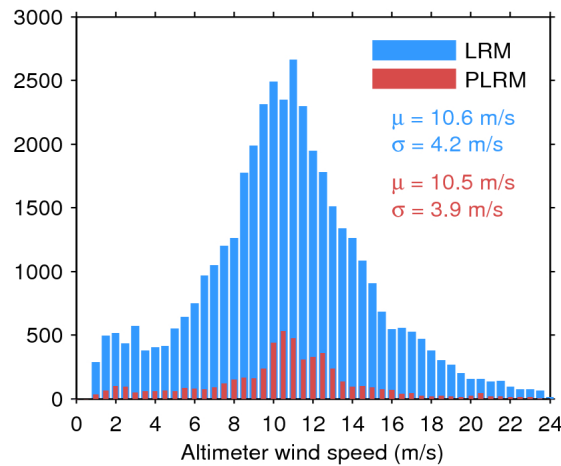
Figure 33. Histogram of flag-valid wind over oceans and lakes for LRM (blue) and PLRM (red) for 18/11/2015. The mean ( \mu ) and standard deviation ( \sigma ) are also shown. Note that values larger than 24 m/s are excluded from the histogram for the sake of readability but not from the computation of \mu and \sigma .
