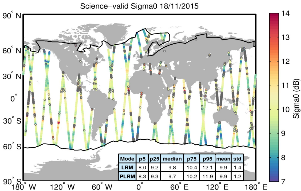
Figure 27. Geographical distribution of science-valid sigma0 data over oceans and lakes for 18/11/2015. The statistical values shown in the table refer to the sigma0 in dB and are calculated separately for LRM and PLRM regions. The black lines mark the outer limit of the Arctic and Antarctic polar polygons. Gray circles denote records that have been rejected based on the editing criteria described in Table 4.
