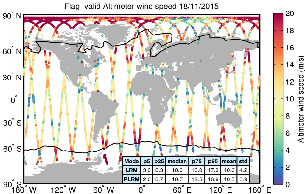
Figure 31. Geographical distribution of flag-valid wind data over oceans and lakes for 18/11/2015. The statistical values shown in the table refer to the wind in m/s and are calculated separately for LRM and PLRM regions. Measurements taken over polar polygons have been excluded from the computation of the statistical values. The black lines mark the outer limit of the Arctic and Antarctic polar polygons.
