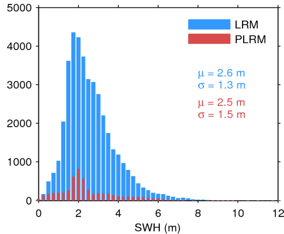
Figure 17. Histogram of flag-valid SWH over oceans and lakes for LRM (blue) and PLRM (red) for 18/11/2015. The mean ( \mu ) and standard deviation ( \sigma ) are also shown. Note that values larger than 12 m are excluded from the histogram for the sake of readability but not from the computation of \mu and \sigma .
