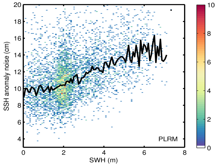
Figure 9. 2D histogram showing flag-valid SSH anomaly noise as a function of SWH for LRM (top) and PLRM (bottom) for 18/11/2015. The black line denotes the median SSH anomaly noise as a function of SWH.
