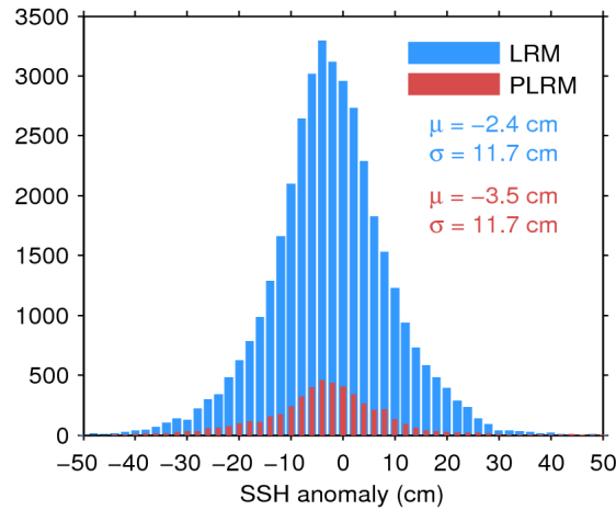
Figure 11. Histogram of science-valid SSH anomaly over oceans and lakes for LRM (blue) and PLRM (red) for 18/11/2015. The mean ( \mu ) and standard deviation ( \sigma ) are also shown. Note that values outside [-50\ 50] cm are excluded from the histogram for the sake of readability but not from the computation of \mu and \sigma .
