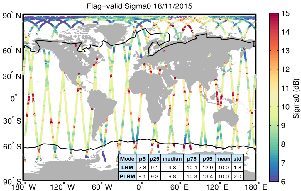
Figure 23. Geographical distribution of flag-valid sigma0 data over oceans and lakes for 18/11/2015. The statistical values shown in the table refer to the sigma0 in dB and are calculated separately for LRM and PLRM regions. Measurements taken over polar polygons have been excluded from the computation of the statistical values. The black lines mark the outer limit of the Arctic and Antarctic polar polygons.
