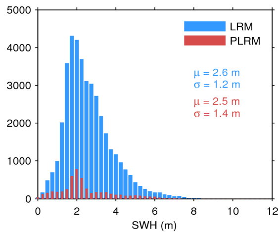
Figure 20. Histogram of science-valid SWH over oceans and lakes for LRM (blue) and PLRM (red) for 18/11/2015. The mean ( \mu ) and standard deviation ( \sigma ) are also shown. Note that values larger than 12 m are excluded from the histogram for the sake of readability but not from the computation of \mu and \sigma .
