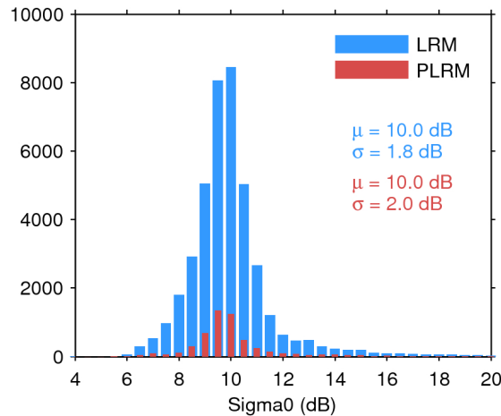
Figure 25. Histogram of flag-valid sigma0 over oceans and lakes for LRM (blue) and PLRM (red) for 18/11/2015. The mean ( \mu ) and standard deviation ( \sigma ) are also shown. Note that values outside [4 20] dB are excluded from the histogram for the sake of readability but not from the computation of \mu and \sigma .
