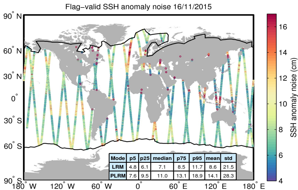
Figure 8. Geographical distribution of flag-valid 20-Hz SSH anomaly measurement noise over oceans and lakes for 16/11/2015. The statistical values shown in the table refer to the SSH anomaly noise and are calculated separately for LRM and PLRM regions. Measurements taken over polar polygons have been excluded from the computation of the statistical values. The black lines mark the outer limit of the Arctic and Antarctic polar polygons.
