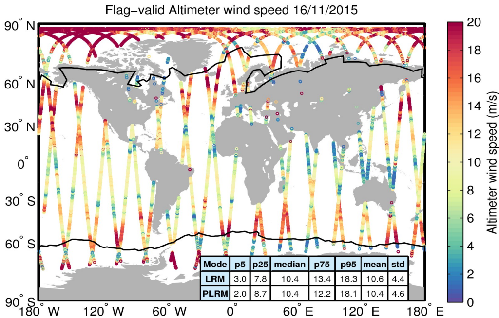
Figure 31. Geographical distribution of flag-valid wind data over oceans and lakes for 16/11/2015. The statistical values shown in the table refer to the wind in m/s and are calculated separately for LRM and PLRM regions. Measurements taken over polar polygons have been excluded from the computation of the statistical values. The black lines mark the outer limit of the Arctic and Antarctic polar polygons.
