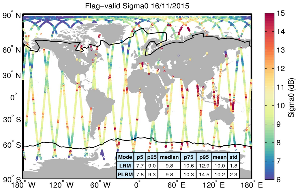
Figure 23. Geographical distribution of flag-valid sigma0 data over oceans and lakes for 16/11/2015. The statistical values shown in the table refer to the sigma0 in dB and are calculated separately for LRM and PLRM regions. Measurements taken over polar polygons have been excluded from the computation of the statistical values. The black lines mark the outer limit of the Arctic and Antarctic polar polygons.
