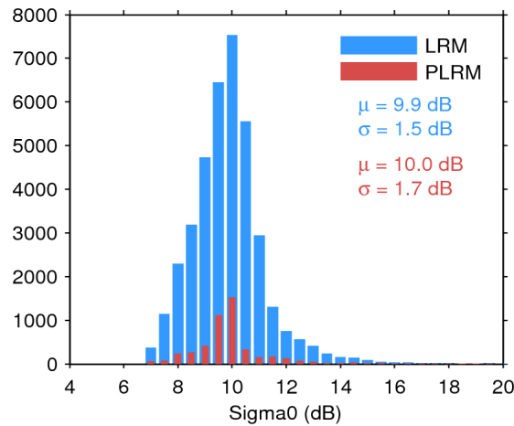
Figure 28. Histogram of science-valid sigma0 over oceans and lakes for LRM (blue) and PLRM (red) for 16/11/2015. The mean ( \mu ) and standard deviation ( \sigma ) are also shown. Note that values outside [4 20] dB are excluded from the histogram for the sake of readability but not from the computation of \mu and \sigma .
