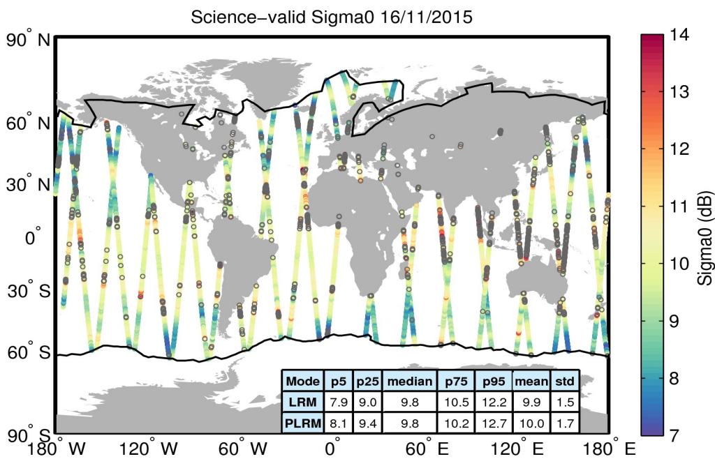
Figure 27. Geographical distribution of science-valid sigma0 data over oceans and lakes for 16/11/2015. The statistical values shown in the table refer to the sigma0 in dB and are calculated separately for LRM and PLRM regions. The black lines mark the outer limit of the Arctic and Antarctic polar polygons. Gray circles denote records that have been rejected based on the editing criteria described in Table 4.
