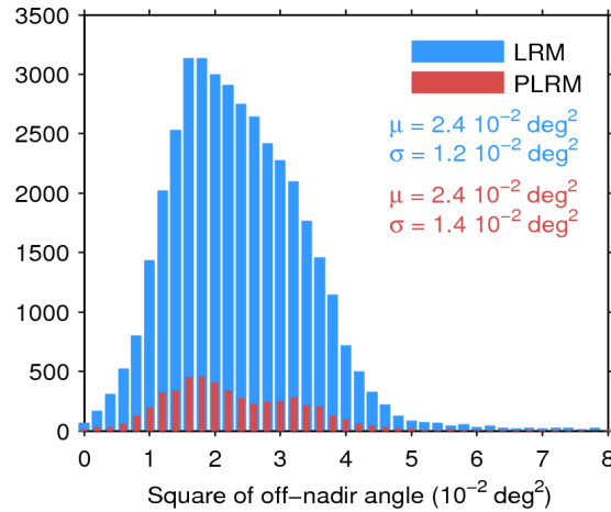
Figure 39. Histogram of flag-valid mispointing over oceans and lakes for LRM (blue) and PLRM (red) for 16/11/2015. Only positive values have been considered. The mean ( \mu ) and standard deviation ( \sigma ) are also shown. Note that values larger than 8 \cdot 10^{-2} \text{ deg}^2 are excluded from the histogram for the sake of readability but not from the computation of \mu and \sigma .
