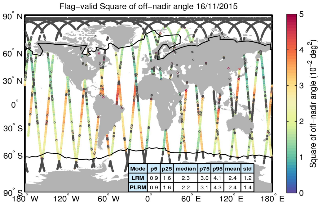
Figure 37. Geographical distribution of flag-valid mispointing data over oceans and lakes for 16/11/2015. The statistical values shown in the table refer to the mispointing in 10^{-2} \text{ deg}^2 and are calculated separately for LRM and PLRM regions. Measurements taken over polar polygons have been excluded from the computation of the statistical values. The black lines mark the outer limit of the Arctic and Antarctic polar polygons. Gray circles denote negative values.
