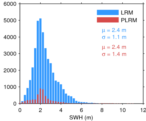
Figure 17. Histogram of flag-valid SWH over oceans and lakes for LRM (blue) and PLRM (red) for 16/11/2015. The mean ( \mu ) and standard deviation ( \sigma ) are also shown. Note that values larger than 12 m are excluded from the histogram for the sake of readability but not from the computation of \mu and \sigma .
