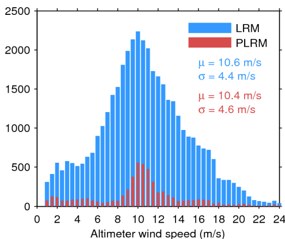
Figure 33. Histogram of flag-valid wind over oceans and lakes for LRM (blue) and PLRM (red) for 16/11/2015. The mean ( \mu ) and standard deviation ( \sigma ) are also shown. Note that values larger than 24 m/s are excluded from the histogram for the sake of readability but not from the computation of \mu and \sigma .
