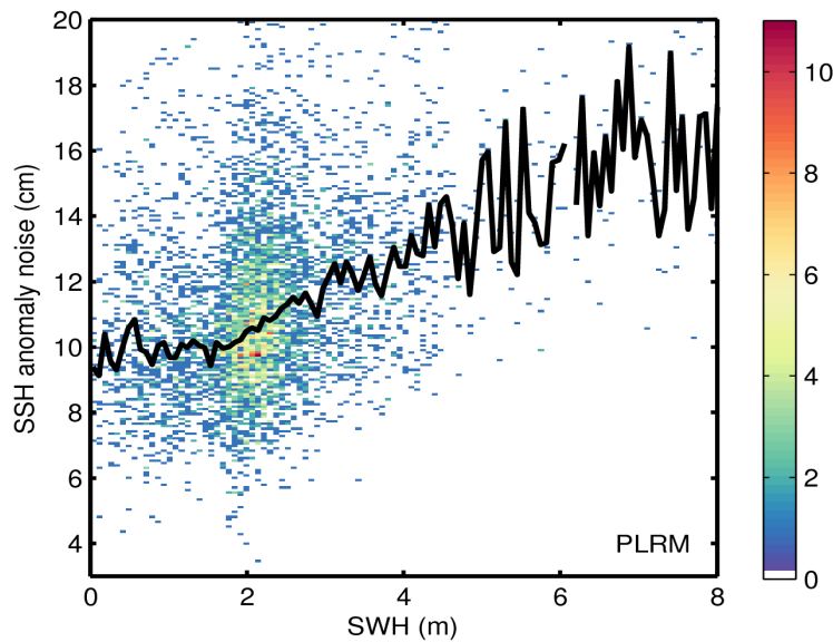
Figure 9. 2D histogram showing flag-valid SSH anomaly noise as a function of SWH for LRM (top) and PLRM (bottom) for 16/11/2015. The black line denotes the median SSH anomaly noise as a function of SWH.
