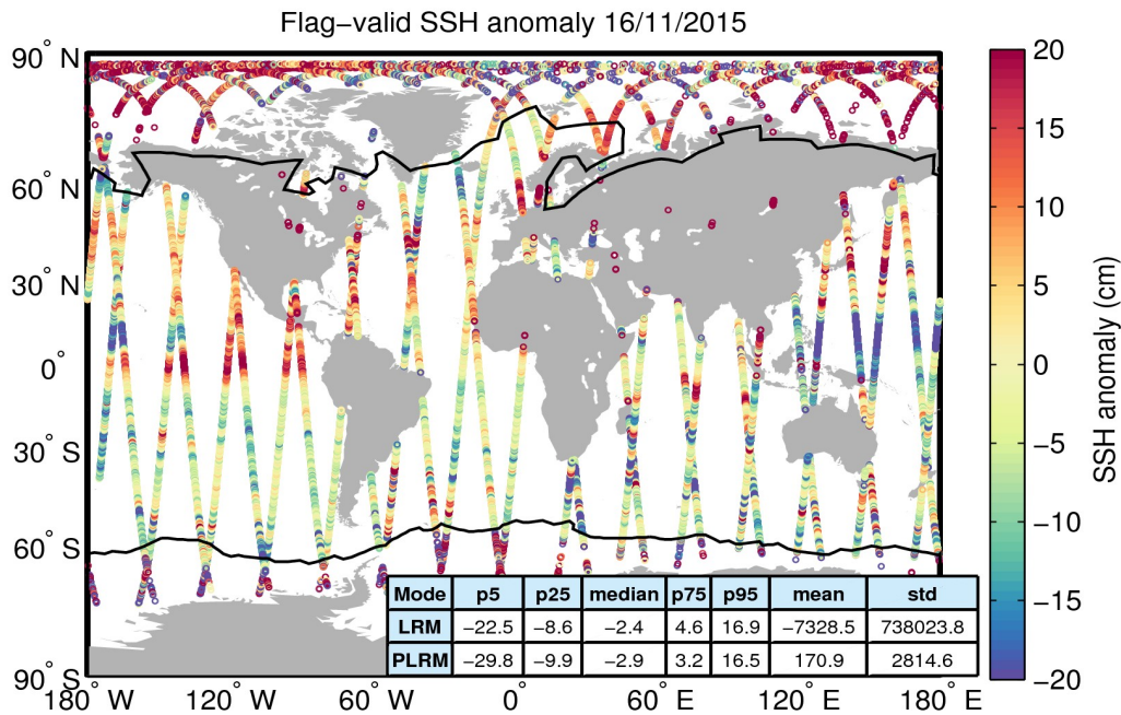
Figure 5. Geographical distribution of flag-valid 1-Hz SSH anomaly data over oceans and lakes for 16/11/2015. The statistical values shown in the table refer to the SSH anomaly in cm and are calculated separately for LRM and PLRM regions. Measurements taken over polar polygons have been excluded from the computation of the statistical values. The black lines mark the outer limit of the Arctic and Antarctic polar polygons.
