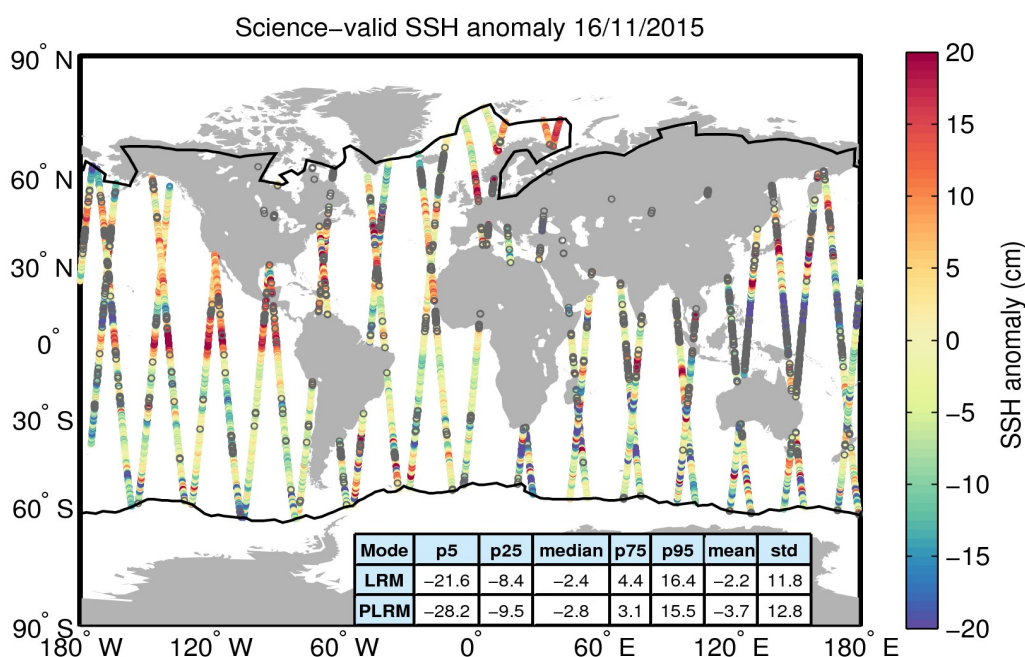
Figure 10. Geographical distribution of science-valid SSH anomaly data over oceans and lakes for 16/11/2015. The statistical values shown in the table refer to the SSH anomaly in cm and are calculated separately for LRM and PLRM regions. The black lines mark the outer limit of the Arctic and Antarctic polar polygons. Gray circles denote records that have been rejected based on the editing criteria described in Table 2.
