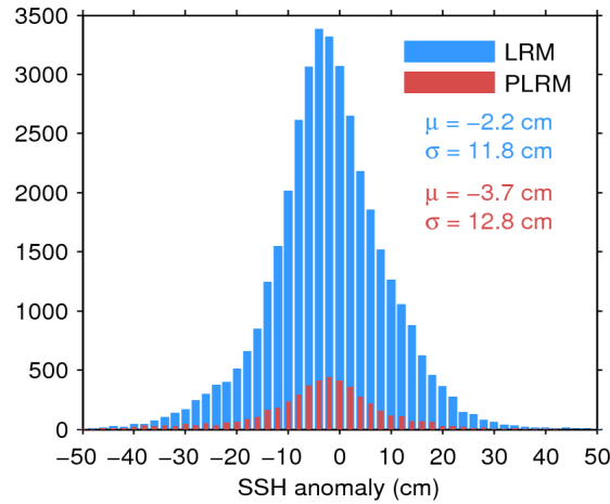
Figure 11. Histogram of science-valid SSH anomaly over oceans and lakes for LRM (blue) and PLRM (red) for 16/11/2015. The mean ( \mu ) and standard deviation ( \sigma ) are also shown. Note that values outside [-50\ 50] cm are excluded from the histogram for the sake of readability but not from the computation of \mu and \sigma .
