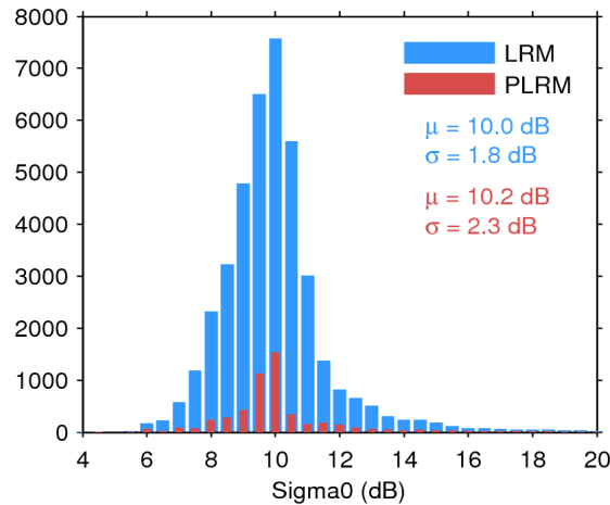
Figure 25. Histogram of flag-valid sigma0 over oceans and lakes for LRM (blue) and PLRM (red) for 16/11/2015. The mean ( \mu ) and standard deviation ( \sigma ) are also shown. Note that values outside [4 20] dB are excluded from the histogram for the sake of readability but not from the computation of \mu and \sigma .
