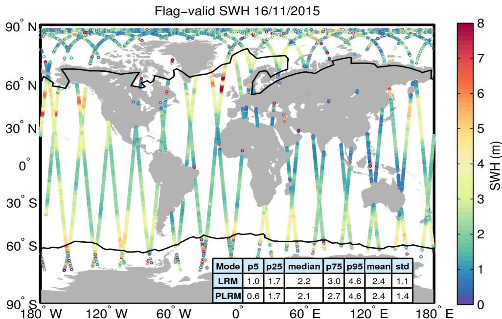
Figure 15. Geographical distribution of flag-valid SWH data over oceans and lakes for 16/11/2015. The statistical values shown in the table refer to the SWH in m and are calculated separately for LRM and PLRM regions. Measurements taken over polar polygons have been excluded from the computation of the statistical values. The black lines mark the outer limit of the Arctic and Antarctic polar polygons.
