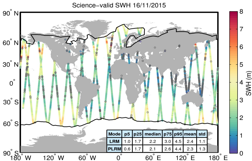
Figure 19. Geographical distribution of science-valid SWH data over oceans and lakes for 16/11/2015. The statistical values shown in the table refer to the SWH in m and are calculated separately for LRM and PLRM regions. The black lines mark the outer limit of the Arctic and Antarctic polar polygons. Gray circles denote records that have been rejected based on the editing criteria described in Table 3.
