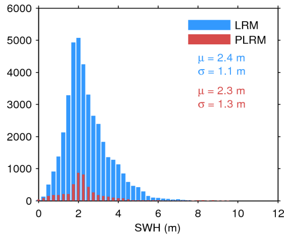
Figure 20. Histogram of science-valid SWH over oceans and lakes for LRM (blue) and PLRM (red) for 16/11/2015. The mean ( \mu ) and standard deviation ( \sigma ) are also shown. Note that values larger than 12 m are excluded from the histogram for the sake of readability but not from the computation of \mu and \sigma .
