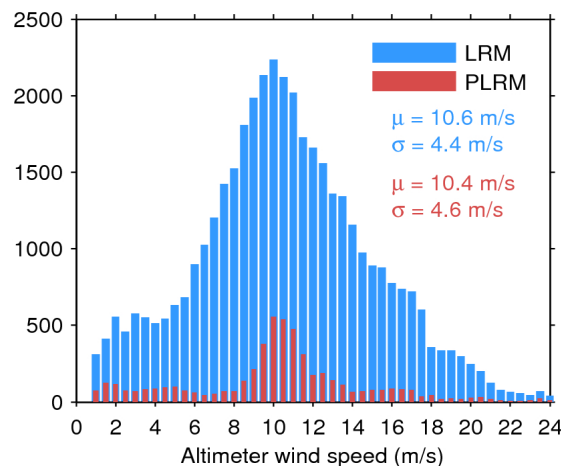
Figure 35. Histogram of science-valid wind over oceans and lakes for LRM (blue) and PLRM (red) for 16/11/2015. The mean ( \mu ) and standard deviation ( \sigma ) are also shown. Note that values larger than 24 m/s are excluded from the histogram for the sake of readability but not from the computation of \mu and \sigma .
