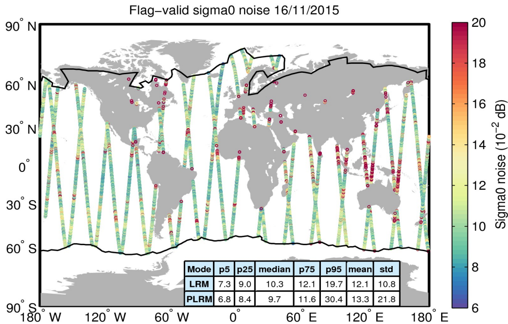
Figure 26. Geographical distribution of flag-valid 20-Hz sigma0 measurement noise over oceans and lakes for 16/11/2015. The statistical values shown in the table refer to the sigma0 noise and are calculated separately for LRM and PLRM regions. Measurements taken over polar polygons have been excluded from the computation of the statistical values. The black lines mark the outer limit of the Arctic and Antarctic polar polygons.
