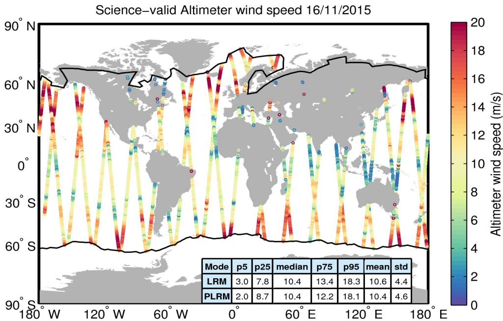
Figure 34. Geographical distribution of science-valid wind data over oceans and lakes for 16/11/2015. The statistical values shown in the table refer to the wind in m/s and are calculated separately for LRM and PLRM regions. The black lines mark the outer limit of the Arctic and Antarctic polar polygons. Gray circles denote records that have been rejected based on the editing criteria described in Table 5.
