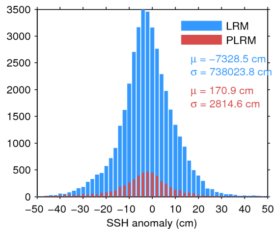
Figure 7. Histogram of flag-valid SSH anomaly over oceans and lakes for LRM (blue) and PLRM (red) for 16/11/2015. The mean ( \mu ) and standard deviation ( \sigma ) are also shown. Note that values outside [-50 \ 50] cm are excluded from the histogram for the sake of readability but not from the computation of \mu and \sigma .
