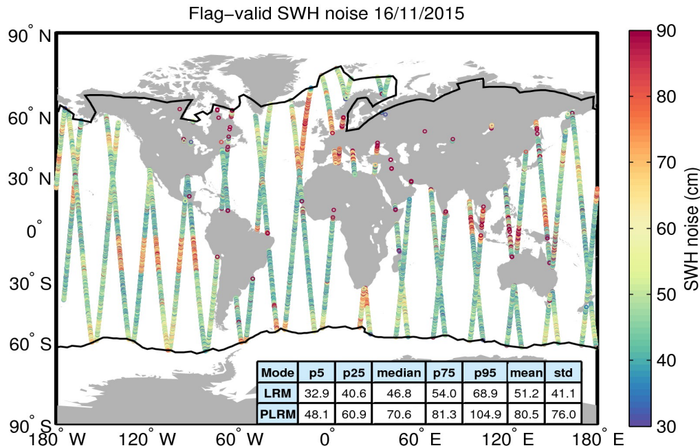
Figure 18. Geographical distribution of flag-valid 20-Hz SWH measurement noise over oceans and lakes for 16/11/2015. The statistical values shown in the table refer to the SWH noise and are calculated separately for LRM and PLRM regions. Measurements taken over polar polygons have been excluded from the computation of the statistical values. The black lines mark the outer limit of the Arctic and Antarctic polar polygons.
