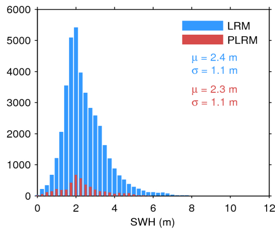
Figure 20. Histogram of science-valid SWH over oceans and lakes for LRM (blue) and PLRM (red) for 15/11/2015. The mean ( \mu ) and standard deviation ( \sigma ) are also shown. Note that values larger than 12 m are excluded from the histogram for the sake of readability but not from the computation of \mu and \sigma .
