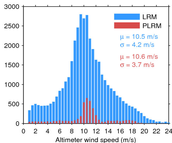
Figure 35. Histogram of science-valid wind over oceans and lakes for LRM (blue) and PLRM (red) for 15/11/2015. The mean ( \mu ) and standard deviation ( \sigma ) are also shown. Note that values larger than 24 m/s are excluded from the histogram for the sake of readability but not from the computation of \mu and \sigma .
