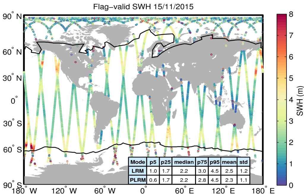
Figure 15. Geographical distribution of flag-valid SWH data over oceans and lakes for 15/11/2015. The statistical values shown in the table refer to the SWH in m and are calculated separately for LRM and PLRM regions. Measurements taken over polar polygons have been excluded from the computation of the statistical values. The black lines mark the outer limit of the Arctic and Antarctic polar polygons.
