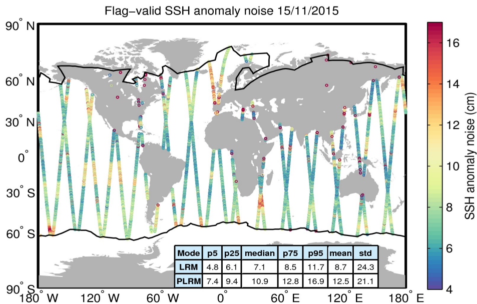
Figure 8. Geographical distribution of flag-valid 20-Hz SSH anomaly measurement noise over oceans and lakes for 15/11/2015. The statistical values shown in the table refer to the SSH anomaly noise and are calculated separately for LRM and PLRM regions. Measurements taken over polar polygons have been excluded from the computation of the statistical values. The black lines mark the outer limit of the Arctic and Antarctic polar polygons.
