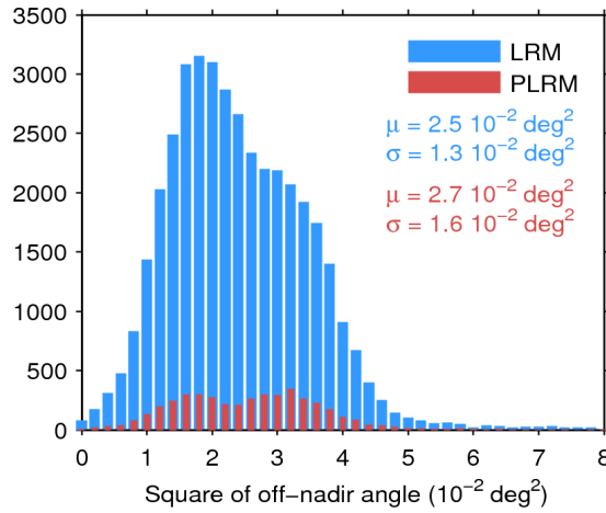
Figure 39. Histogram of flag-valid mispointing over oceans and lakes for LRM (blue) and PLRM (red) for 15/11/2015. Only positive values have been considered. The mean ( \mu ) and standard deviation ( \sigma ) are also shown. Note that values larger than 8 \cdot 10^{-2} \text{ deg}^2 are excluded from the histogram for the sake of readability but not from the computation of \mu and \sigma .
