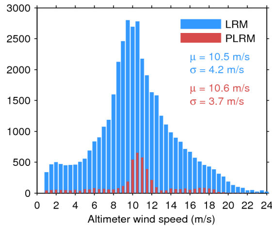
Figure 33. Histogram of flag-valid wind over oceans and lakes for LRM (blue) and PLRM (red) for 15/11/2015. The mean ( \mu ) and standard deviation ( \sigma ) are also shown. Note that values larger than 24 m/s are excluded from the histogram for the sake of readability but not from the computation of \mu and \sigma .
