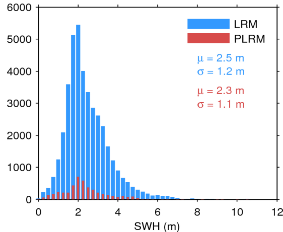
Figure 17. Histogram of flag-valid SWH over oceans and lakes for LRM (blue) and PLRM (red) for 15/11/2015. The mean ( \mu ) and standard deviation ( \sigma ) are also shown. Note that values larger than 12 m are excluded from the histogram for the sake of readability but not from the computation of \mu and \sigma .
