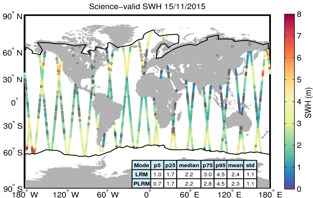
Figure 19. Geographical distribution of science-valid SWH data over oceans and lakes for 15/11/2015. The statistical values shown in the table refer to the SWH in m and are calculated separately for LRM and PLRM regions. The black lines mark the outer limit of the Arctic and Antarctic polar polygons. Gray circles denote records that have been rejected based on the editing criteria described in Table 3.
