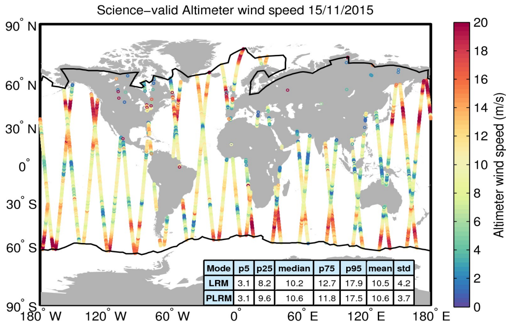
Figure 34. Geographical distribution of science-valid wind data over oceans and lakes for 15/11/2015. The statistical values shown in the table refer to the wind in m/s and are calculated separately for LRM and PLRM regions. The black lines mark the outer limit of the Arctic and Antarctic polar polygons. Gray circles denote records that have been rejected based on the editing criteria described in Table 5.
