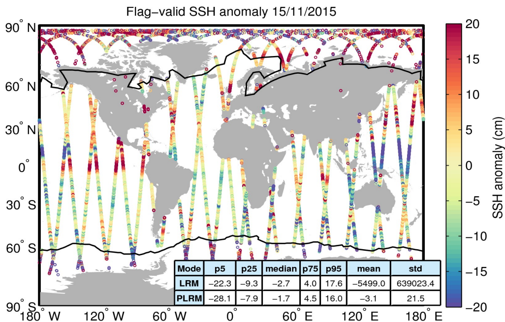
Figure 5. Geographical distribution of flag-valid 1-Hz SSH anomaly data over oceans and lakes for 15/11/2015. The statistical values shown in the table refer to the SSH anomaly in cm and are calculated separately for LRM and PLRM regions. Measurements taken over polar polygons have been excluded from the computation of the statistical values. The black lines mark the outer limit of the Arctic and Antarctic polar polygons.
