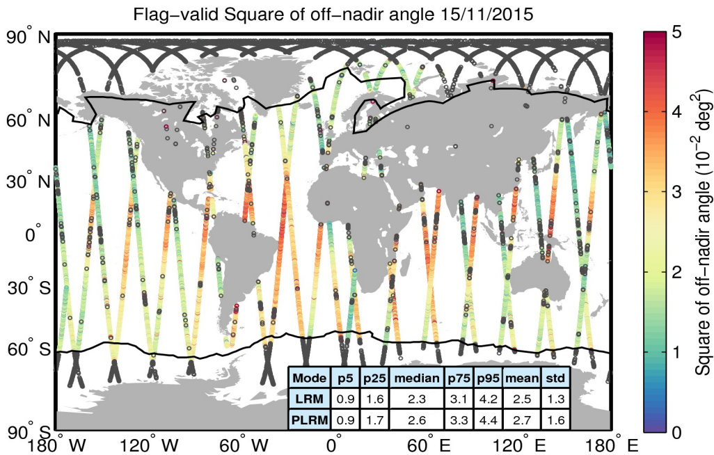
Figure 37. Geographical distribution of flag-valid mispointing data over oceans and lakes for 15/11/2015. The statistical values shown in the table refer to the mispointing in 10^{-2} deg 2 and are calculated separately for LRM and PLRM regions. Measurements taken over polar polygons have been excluded from the computation of the statistical values. The black lines mark the outer limit of the Arctic and Antarctic polar polygons. Gray circles denote negative values.
