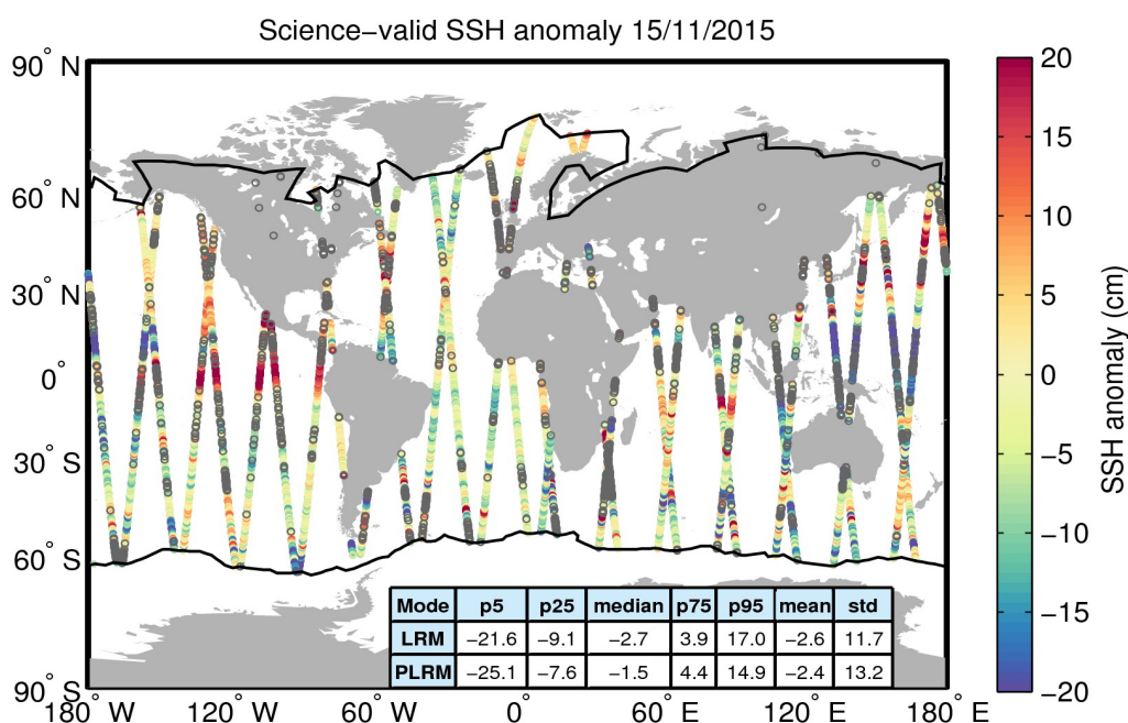
Figure 10. Geographical distribution of science-valid SSH anomaly data over oceans and lakes for 15/11/2015. The statistical values shown in the table refer to the SSH anomaly in cm and are calculated separately for LRM and PLRM regions. The black lines mark the outer limit of the Arctic and Antarctic polar polygons. Gray circles denote records that have been rejected based on the editing criteria described in Table 2.
