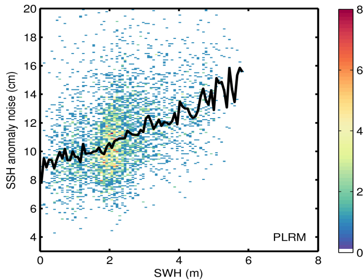
Figure 9. 2D histogram showing flag-valid SSH anomaly noise as a function of SWH for LRM (top) and PLRM (bottom) for 15/11/2015. The black line denotes the median SSH anomaly noise as a function of SWH.
