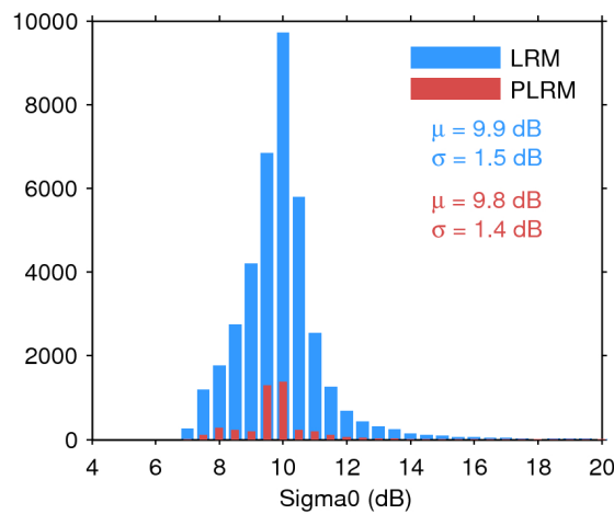
Figure 28. Histogram of science-valid sigma0 over oceans and lakes for LRM (blue) and PLRM (red) for 15/11/2015. The mean ( \mu ) and standard deviation ( \sigma ) are also shown. Note that values outside [4 20] dB are excluded from the histogram for the sake of readability but not from the computation of \mu and \sigma .
