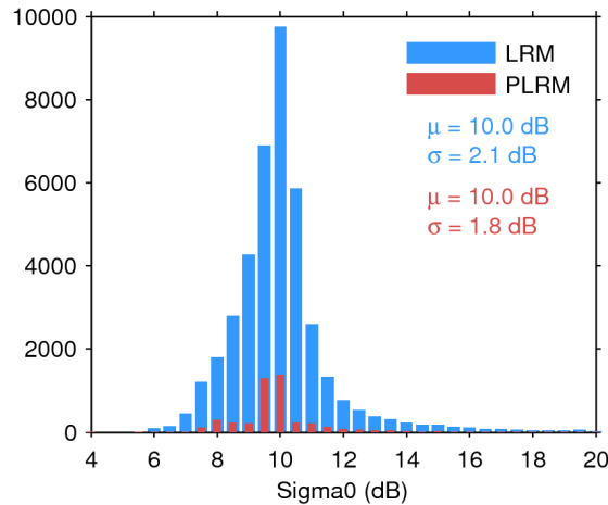
Figure 25. Histogram of flag-valid sigma0 over oceans and lakes for LRM (blue) and PLRM (red) for 15/11/2015. The mean ( \mu ) and standard deviation ( \sigma ) are also shown. Note that values outside [4 20] dB are excluded from the histogram for the sake of readability but not from the computation of \mu and \sigma .
