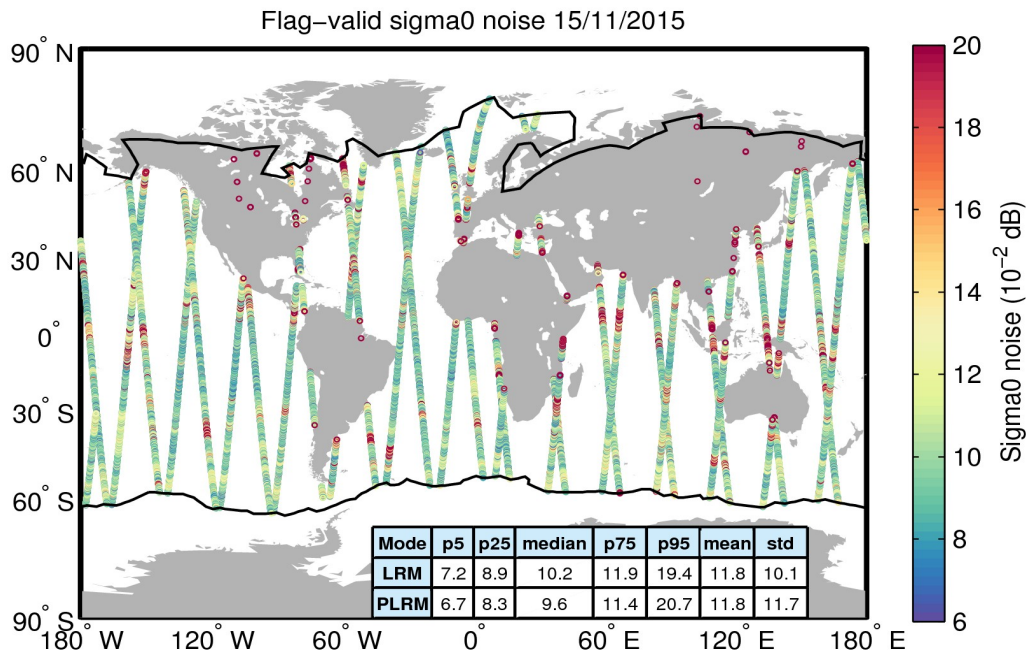
Figure 26. Geographical distribution of flag-valid 20-Hz sigma0 measurement noise over oceans and lakes for 15/11/2015. The statistical values shown in the table refer to the sigma0 noise and are calculated separately for LRM and PLRM regions. Measurements taken over polar polygons have been excluded from the computation of the statistical values. The black lines mark the outer limit of the Arctic and Antarctic polar polygons.
