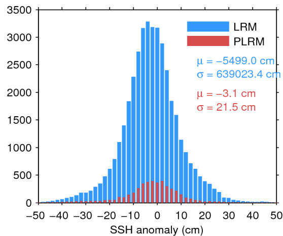
Figure 7. Histogram of flag-valid SSH anomaly over oceans and lakes for LRM (blue) and PLRM (red) for 15/11/2015. The mean ( \mu ) and standard deviation ( \sigma ) are also shown. Note that values outside [-50\ 50] cm are excluded from the histogram for the sake of readability but not from the computation of \mu and \sigma .
