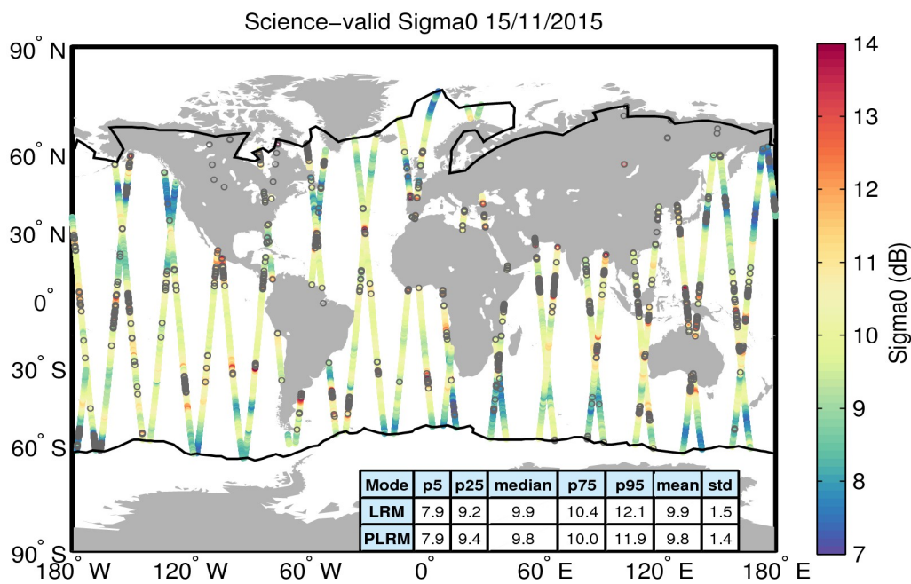
Figure 27. Geographical distribution of science-valid sigma0 data over oceans and lakes for 15/11/2015. The statistical values shown in the table refer to the sigma0 in dB and are calculated separately for LRM and PLRM regions. The black lines mark the outer limit of the Arctic and Antarctic polar polygons. Gray circles denote records that have been rejected based on the editing criteria described in Table 4.
