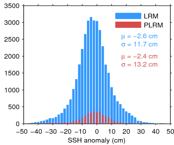
Figure 11. Histogram of science-valid SSH anomaly over oceans and lakes for LRM (blue) and PLRM (red) for 15/11/2015. The mean ( \mu ) and standard deviation ( \sigma ) are also shown. Note that values outside [-50\ 50] cm are excluded from the histogram for the sake of readability but not from the computation of \mu and \sigma .
