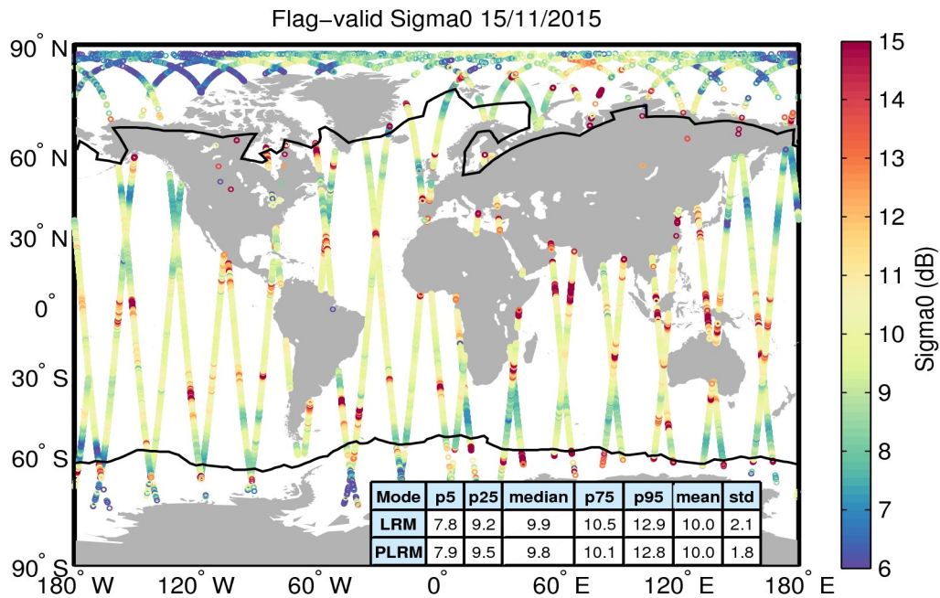
Figure 23. Geographical distribution of flag-valid sigma0 data over oceans and lakes for 15/11/2015. The statistical values shown in the table refer to the sigma0 in dB and are calculated separately for LRM and PLRM regions. Measurements taken over polar polygons have been excluded from the computation of the statistical values. The black lines mark the outer limit of the Arctic and Antarctic polar polygons.
