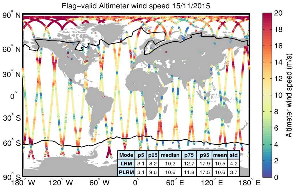
Figure 31. Geographical distribution of flag-valid wind data over oceans and lakes for 15/11/2015. The statistical values shown in the table refer to the wind in m/s and are calculated separately for LRM and PLRM regions. Measurements taken over polar polygons have been excluded from the computation of the statistical values. The black lines mark the outer limit of the Arctic and Antarctic polar polygons.
