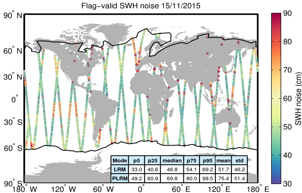
Figure 18. Geographical distribution of flag-valid 20-Hz SWH measurement noise over oceans and lakes for 15/11/2015. The statistical values shown in the table refer to the SWH noise and are calculated separately for LRM and PLRM regions. Measurements taken over polar polygons have been excluded from the computation of the statistical values. The black lines mark the outer limit of the Arctic and Antarctic polar polygons.
