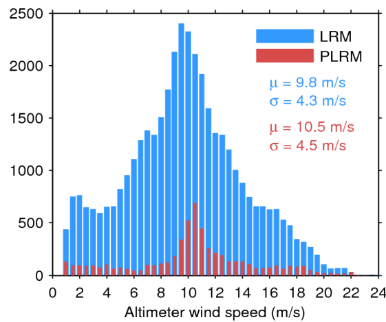
Figure 33. Histogram of flag-valid wind over oceans and lakes for LRM (blue) and PLRM (red) for 14/11/2015. The mean ( \mu ) and standard deviation ( \sigma ) are also shown. Note that values larger than 24 m/s are excluded from the histogram for the sake of readability but not from the computation of \mu and \sigma .
