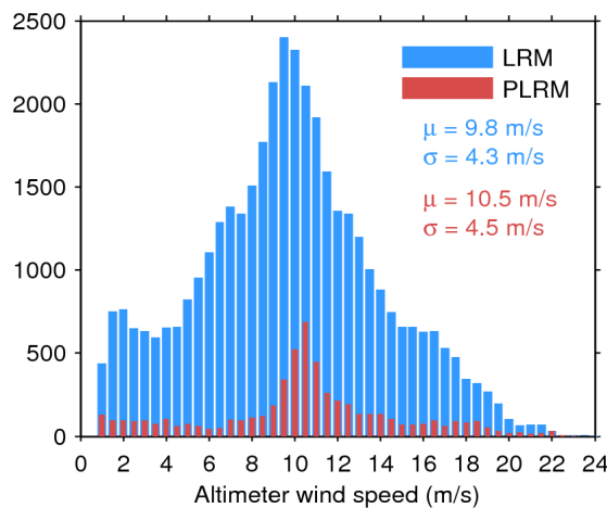
Figure 35. Histogram of science-valid wind over oceans and lakes for LRM (blue) and PLRM (red) for 14/11/2015. The mean ( \mu ) and standard deviation ( \sigma ) are also shown. Note that values larger than 24 m/s are excluded from the histogram for the sake of readability but not from the computation of \mu and \sigma .
