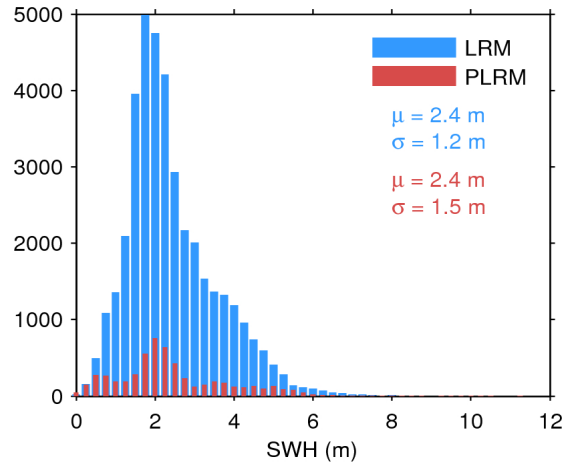
Figure 17. Histogram of flag-valid SWH over oceans and lakes for LRM (blue) and PLRM (red) for 14/11/2015. The mean ( \mu ) and standard deviation ( \sigma ) are also shown. Note that values larger than 12 m are excluded from the histogram for the sake of readability but not from the computation of \mu and \sigma .
