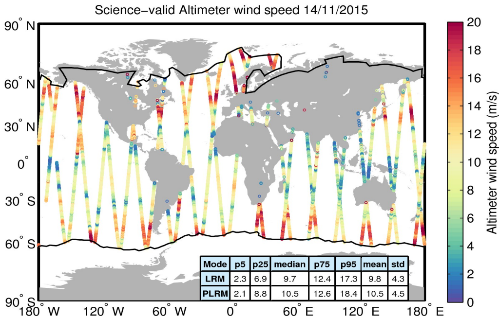
Figure 34. Geographical distribution of science-valid wind data over oceans and lakes for 14/11/2015. The statistical values shown in the table refer to the wind in m/s and are calculated separately for LRM and PLRM regions. The black lines mark the outer limit of the Arctic and Antarctic polar polygons. Gray circles denote records that have been rejected based on the editing criteria described in Table 5.
