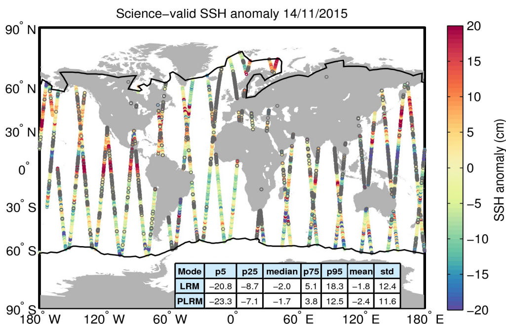
Figure 10. Geographical distribution of science-valid SSH anomaly data over oceans and lakes for 14/11/2015. The statistical values shown in the table refer to the SSH anomaly in cm and are calculated separately for LRM and PLRM regions. The black lines mark the outer limit of the Arctic and Antarctic polar polygons. Gray circles denote records that have been rejected based on the editing criteria described in Table 2.
