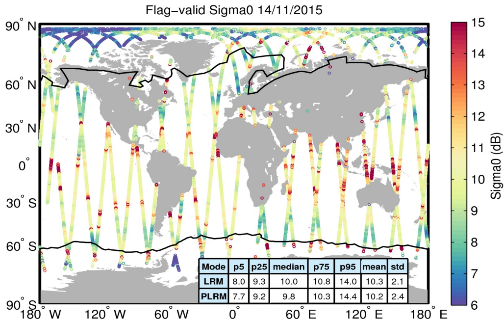
Figure 23. Geographical distribution of flag-valid sigma0 data over oceans and lakes for 14/11/2015. The statistical values shown in the table refer to the sigma0 in dB and are calculated separately for LRM and PLRM regions. Measurements taken over polar polygons have been excluded from the computation of the statistical values. The black lines mark the outer limit of the Arctic and Antarctic polar polygons.
