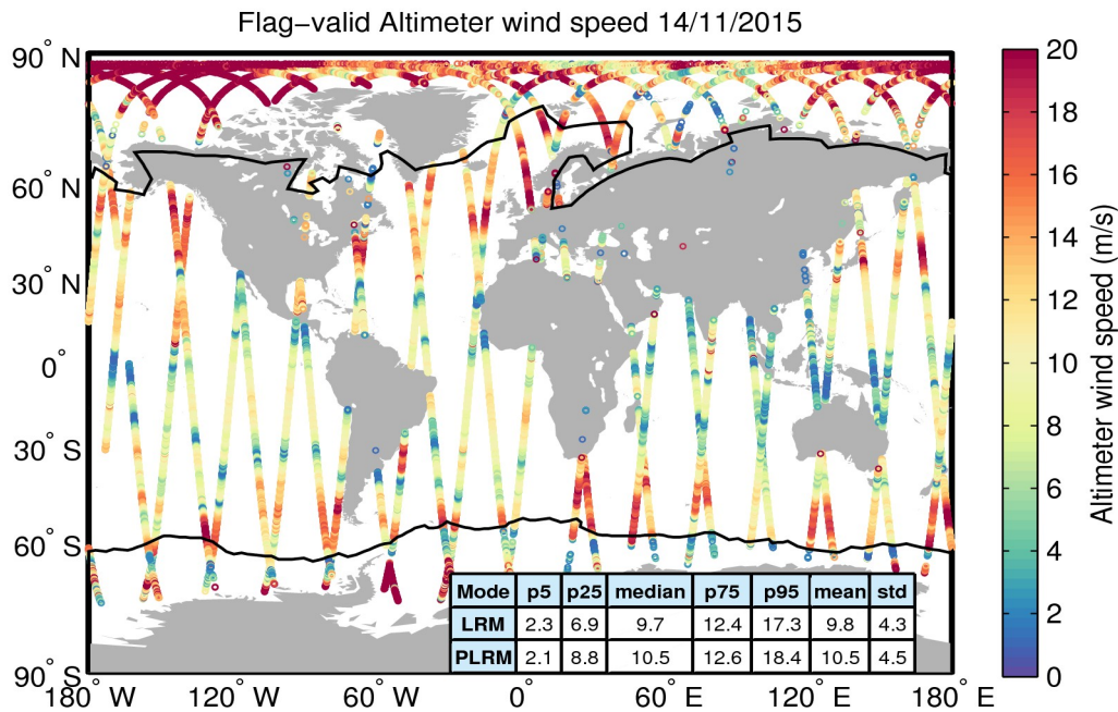
Figure 31. Geographical distribution of flag-valid wind data over oceans and lakes for 14/11/2015. The statistical values shown in the table refer to the wind in m/s and are calculated separately for LRM and PLRM regions. Measurements taken over polar polygons have been excluded from the computation of the statistical values. The black lines mark the outer limit of the Arctic and Antarctic polar polygons.
