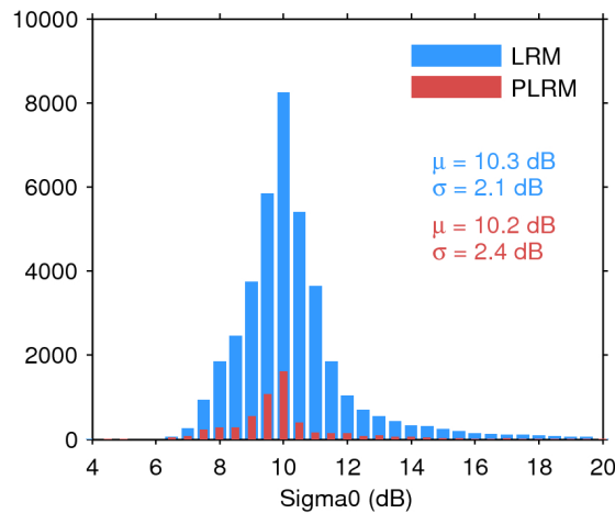
Figure 25. Histogram of flag-valid sigma0 over oceans and lakes for LRM (blue) and PLRM (red) for 14/11/2015. The mean ( \mu ) and standard deviation ( \sigma ) are also shown. Note that values outside [4 20] dB are excluded from the histogram for the sake of readability but not from the computation of \mu and \sigma .
