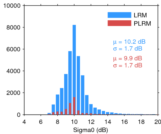
Figure 28. Histogram of science-valid sigma0 over oceans and lakes for LRM (blue) and PLRM (red) for 14/11/2015. The mean ( \mu ) and standard deviation ( \sigma ) are also shown. Note that values outside [4 20] dB are excluded from the histogram for the sake of readability but not from the computation of \mu and \sigma .
