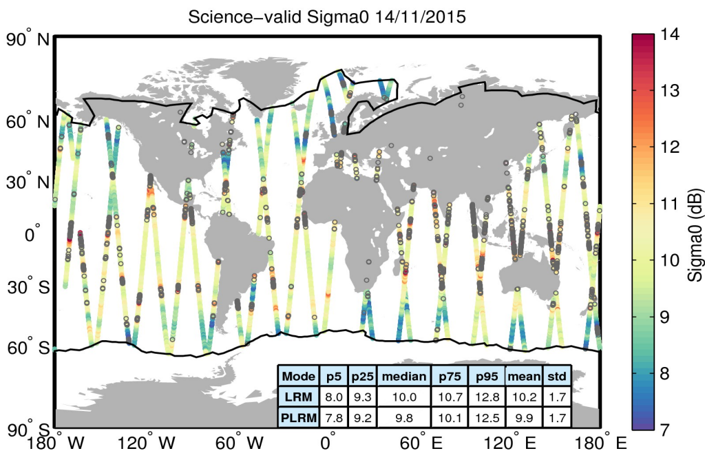
Figure 27. Geographical distribution of science-valid sigma0 data over oceans and lakes for 14/11/2015. The statistical values shown in the table refer to the sigma0 in dB and are calculated separately for LRM and PLRM regions. The black lines mark the outer limit of the Arctic and Antarctic polar polygons. Gray circles denote records that have been rejected based on the editing criteria described in Table 4.
