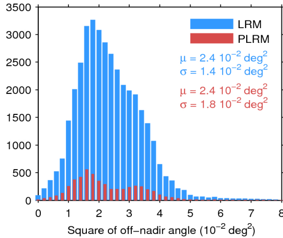
Figure 39. Histogram of flag-valid mispointing over oceans and lakes for LRM (blue) and PLRM (red) for 14/11/2015. Only positive values have been considered. The mean ( \mu ) and standard deviation ( \sigma ) are also shown. Note that values larger than 8 \cdot 10^{-2} \text{ deg}^2 are excluded from the histogram for the sake of readability but not from the computation of \mu and \sigma .
