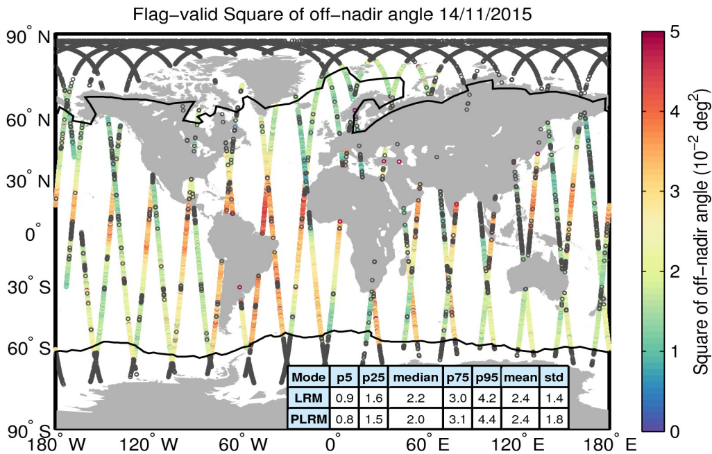
Figure 37. Geographical distribution of flag-valid mispointing data over oceans and lakes for 14/11/2015. The statistical values shown in the table refer to the mispointing in 10^{-2} deg 2 and are calculated separately for LRM and PLRM regions. Measurements taken over polar polygons have been excluded from the computation of the statistical values. The black lines mark the outer limit of the Arctic and Antarctic polar polygons. Gray circles denote negative values.
