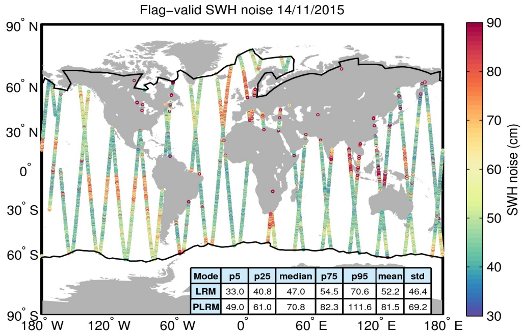
Figure 18. Geographical distribution of flag-valid 20-Hz SWH measurement noise over oceans and lakes for 14/11/2015. The statistical values shown in the table refer to the SWH noise and are calculated separately for LRM and PLRM regions. Measurements taken over polar polygons have been excluded from the computation of the statistical values. The black lines mark the outer limit of the Arctic and Antarctic polar polygons.
