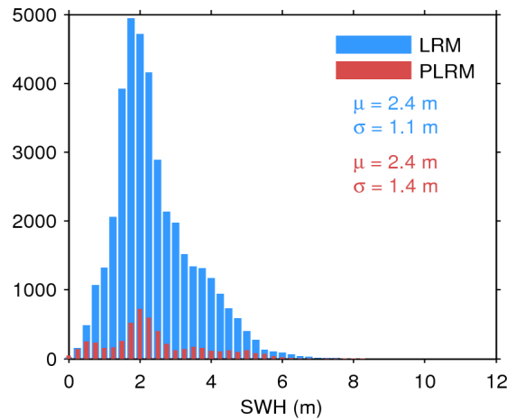
Figure 20. Histogram of science-valid SWH over oceans and lakes for LRM (blue) and PLRM (red) for 14/11/2015. The mean ( \mu ) and standard deviation ( \sigma ) are also shown. Note that values larger than 12 m are excluded from the histogram for the sake of readability but not from the computation of \mu and \sigma .
