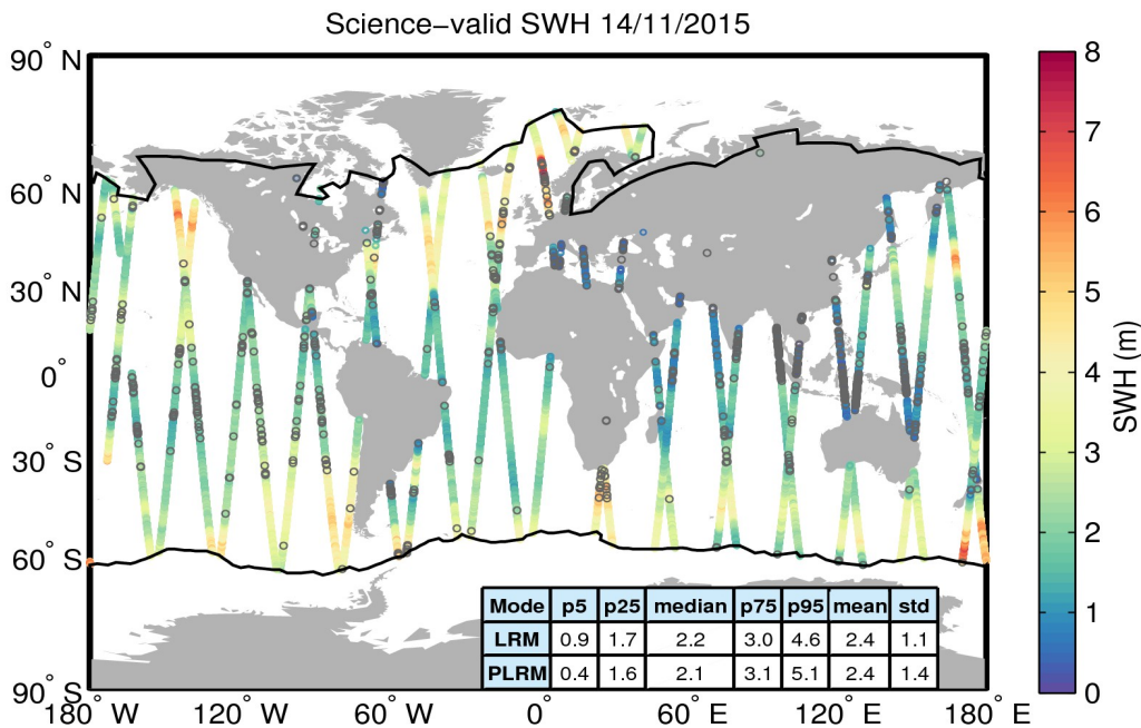
Figure 19. Geographical distribution of science-valid SWH data over oceans and lakes for 14/11/2015. The statistical values shown in the table refer to the SWH in m and are calculated separately for LRM and PLRM regions. The black lines mark the outer limit of the Arctic and Antarctic polar polygons. Gray circles denote records that have been rejected based on the editing criteria described in Table 3.
