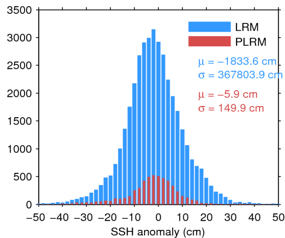
Figure 7. Histogram of flag-valid SSH anomaly over oceans and lakes for LRM (blue) and PLRM (red) for 14/11/2015. The mean ( \mu ) and standard deviation ( \sigma ) are also shown. Note that values outside [-50 \ 50] cm are excluded from the histogram for the sake of readability but not from the computation of \mu and \sigma .
