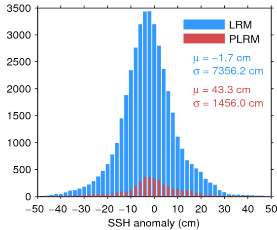
Figure 7. Histogram of flag-valid SSH anomaly over oceans and lakes for LRM (blue) and PLRM (red) for 13/11/2015. The mean ( \mu ) and standard deviation ( \sigma ) are also shown. Note that values outside [-50 50] cm are excluded from the histogram for the sake of readability but not from the computation of \mu and \sigma .
