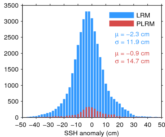
Figure 11. Histogram of science-valid SSH anomaly over oceans and lakes for LRM (blue) and PLRM (red) for 13/11/2015. The mean ( \mu ) and standard deviation ( \sigma ) are also shown. Note that values outside [-50\ 50] cm are excluded from the histogram for the sake of readability but not from the computation of \mu and \sigma .
