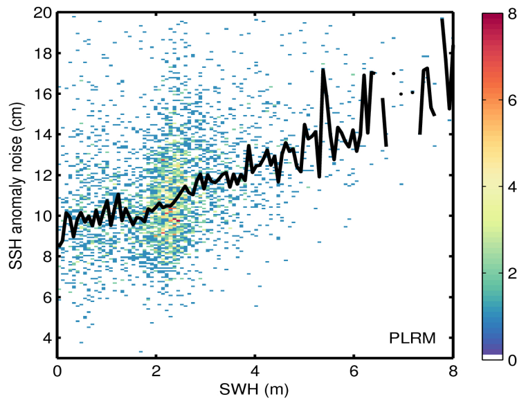
Figure 9. 2D histogram showing flag-valid SSH anomaly noise as a function of SWH for LRM (top) and PLRM (bottom) for 13/11/2015. The black line denotes the median SSH anomaly noise as a function of SWH.
