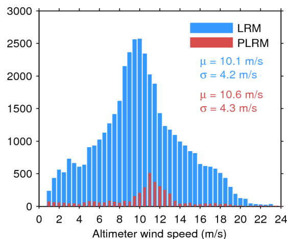
Figure 35. Histogram of science-valid wind over oceans and lakes for LRM (blue) and PLRM (red) for 13/11/2015. The mean ( \mu ) and standard deviation ( \sigma ) are also shown. Note that values larger than 24 m/s are excluded from the histogram for the sake of readability but not from the computation of \mu and \sigma .
