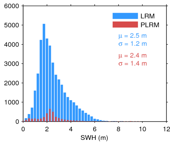
Figure 20. Histogram of science-valid SWH over oceans and lakes for LRM (blue) and PLRM (red) for 13/11/2015. The mean ( \mu ) and standard deviation ( \sigma ) are also shown. Note that values larger than 12 m are excluded from the histogram for the sake of readability but not from the computation of \mu and \sigma .
