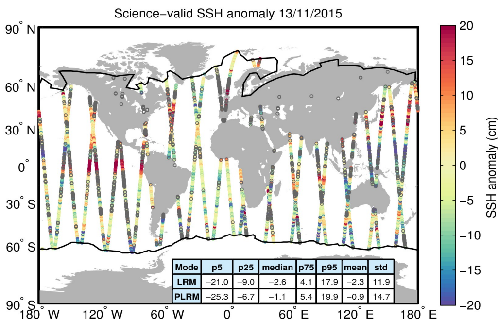
Figure 10. Geographical distribution of science-valid SSH anomaly data over oceans and lakes for 13/11/2015. The statistical values shown in the table refer to the SSH anomaly in cm and are calculated separately for LRM and PLRM regions. The black lines mark the outer limit of the Arctic and Antarctic polar polygons. Gray circles denote records that have been rejected based on the editing criteria described in Table 2.
