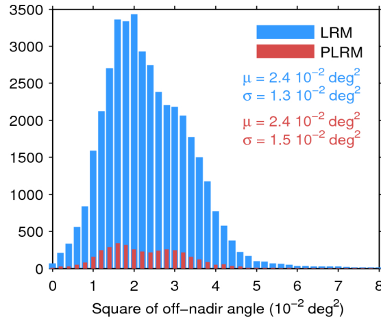
Figure 39. Histogram of flag-valid mispointing over oceans and lakes for LRM (blue) and PLRM (red) for 13/11/2015. Only positive values have been considered. The mean ( \mu ) and standard deviation ( \sigma ) are also shown. Note that values larger than 8 \cdot 10^{-2} \text{ deg}^2 are excluded from the histogram for the sake of readability but not from the computation of \mu and \sigma .
