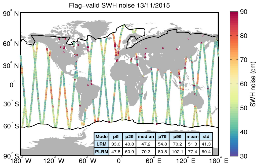
Figure 18. Geographical distribution of flag-valid 20-Hz SWH measurement noise over oceans and lakes for 13/11/2015. The statistical values shown in the table refer to the SWH noise and are calculated separately for LRM and PLRM regions. Measurements taken over polar polygons have been excluded from the computation of the statistical values. The black lines mark the outer limit of the Arctic and Antarctic polar polygons.
