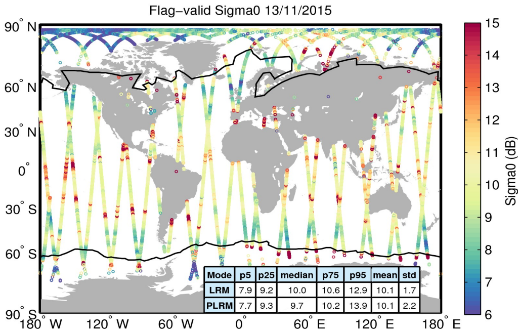
Figure 23. Geographical distribution of flag-valid sigma0 data over oceans and lakes for 13/11/2015. The statistical values shown in the table refer to the sigma0 in dB and are calculated separately for LRM and PLRM regions. Measurements taken over polar polygons have been excluded from the computation of the statistical values. The black lines mark the outer limit of the Arctic and Antarctic polar polygons.
