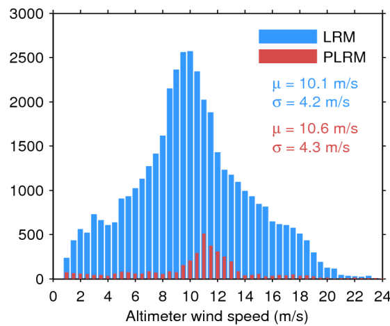
Figure 33. Histogram of flag-valid wind over oceans and lakes for LRM (blue) and PLRM (red) for 13/11/2015. The mean ( \mu ) and standard deviation ( \sigma ) are also shown. Note that values larger than 24 m/s are excluded from the histogram for the sake of readability but not from the computation of \mu and \sigma .
