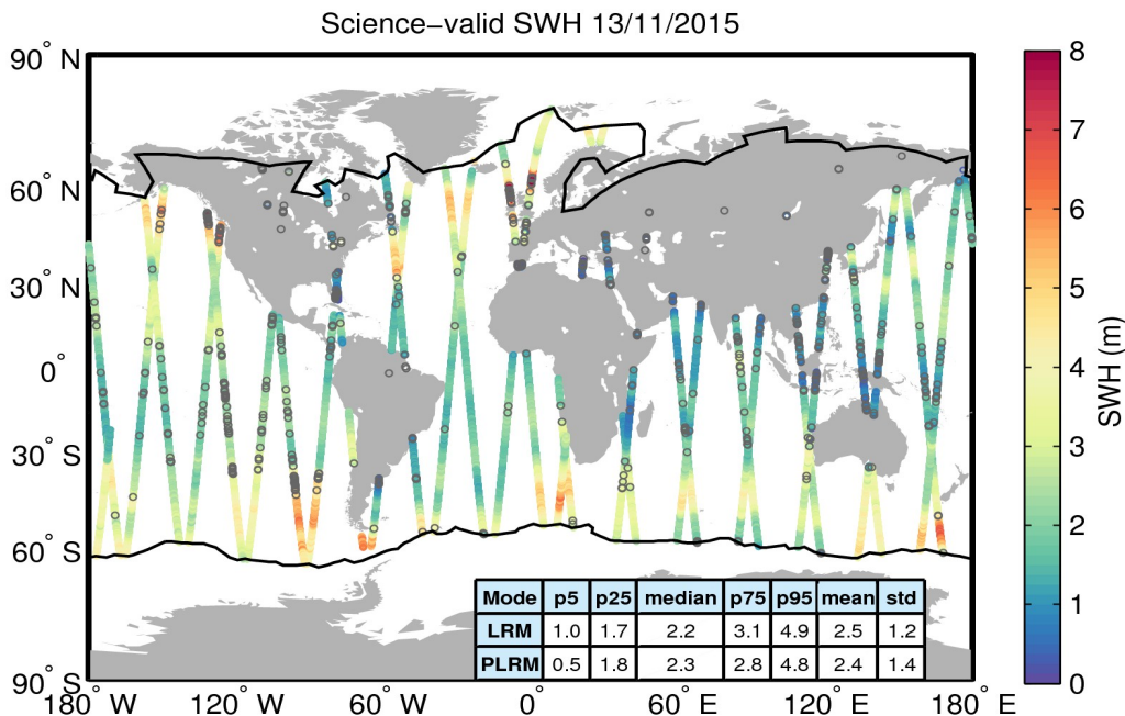
Figure 19. Geographical distribution of science-valid SWH data over oceans and lakes for 13/11/2015. The statistical values shown in the table refer to the SWH in m and are calculated separately for LRM and PLRM regions. The black lines mark the outer limit of the Arctic and Antarctic polar polygons. Gray circles denote records that have been rejected based on the editing criteria described in Table 3.
