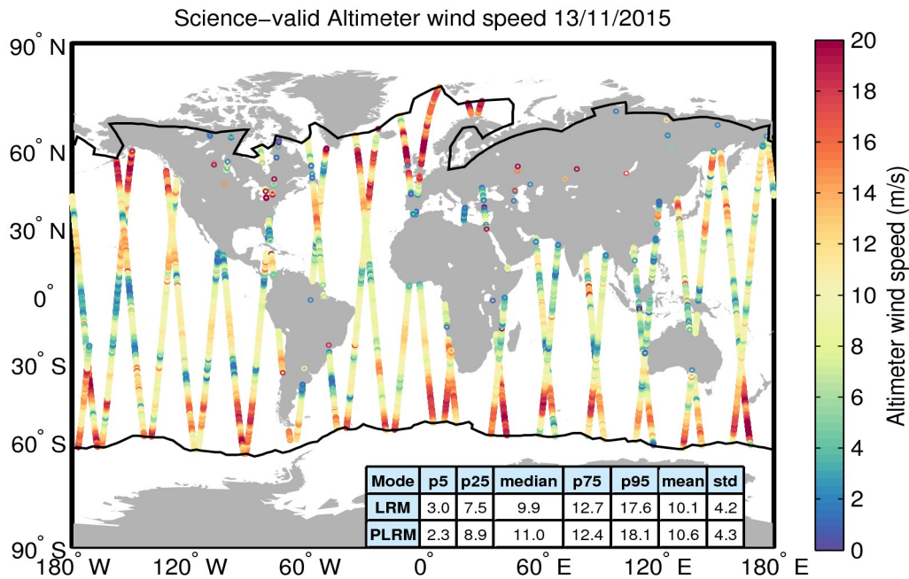
Figure 34. Geographical distribution of science-valid wind data over oceans and lakes for 13/11/2015. The statistical values shown in the table refer to the wind in m/s and are calculated separately for LRM and PLRM regions. The black lines mark the outer limit of the Arctic and Antarctic polar polygons. Gray circles denote records that have been rejected based on the editing criteria described in Table 5.
