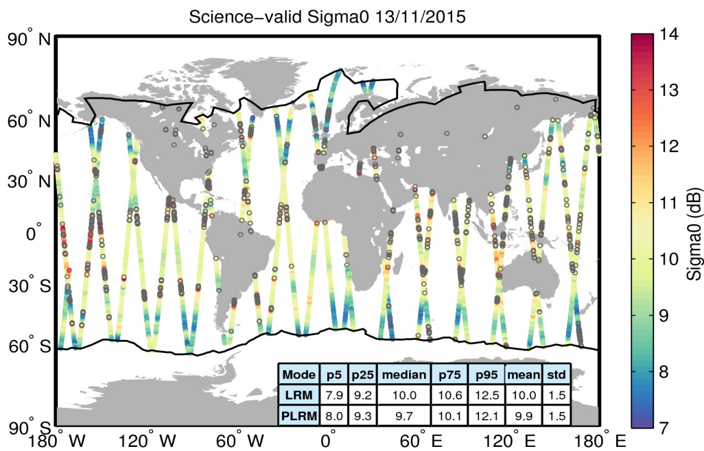
Figure 27. Geographical distribution of science-valid sigma0 data over oceans and lakes for 13/11/2015. The statistical values shown in the table refer to the sigma0 in dB and are calculated separately for LRM and PLRM regions. The black lines mark the outer limit of the Arctic and Antarctic polar polygons. Gray circles denote records that have been rejected based on the editing criteria described in Table 4.
