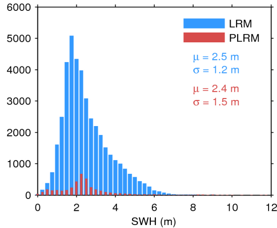
Figure 17. Histogram of flag-valid SWH over oceans and lakes for LRM (blue) and PLRM (red) for 13/11/2015. The mean ( \mu ) and standard deviation ( \sigma ) are also shown. Note that values larger than 12 m are excluded from the histogram for the sake of readability but not from the computation of \mu and \sigma .
