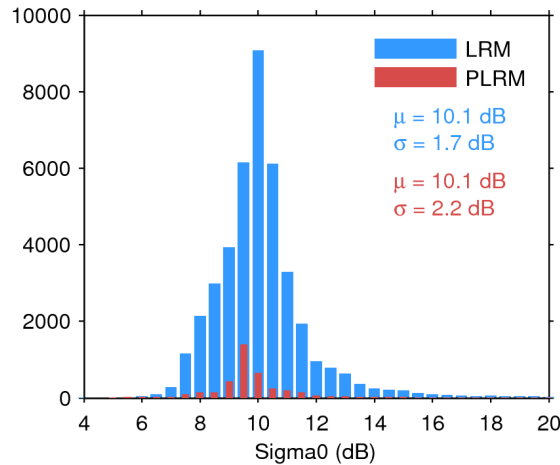
Figure 25. Histogram of flag-valid sigma0 over oceans and lakes for LRM (blue) and PLRM (red) for 13/11/2015. The mean ( \mu ) and standard deviation ( \sigma ) are also shown. Note that values outside [4 20] dB are excluded from the histogram for the sake of readability but not from the computation of \mu and \sigma .
