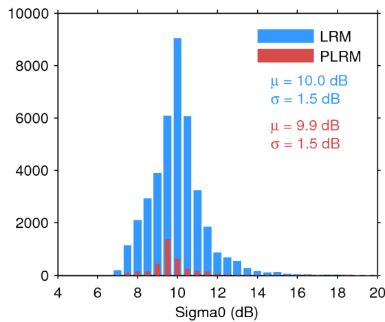
Figure 28. Histogram of science-valid sigma0 over oceans and lakes for LRM (blue) and PLRM (red) for 13/11/2015. The mean ( \mu ) and standard deviation ( \sigma ) are also shown. Note that values outside [4 20] dB are excluded from the histogram for the sake of readability but not from the computation of \mu and \sigma .
