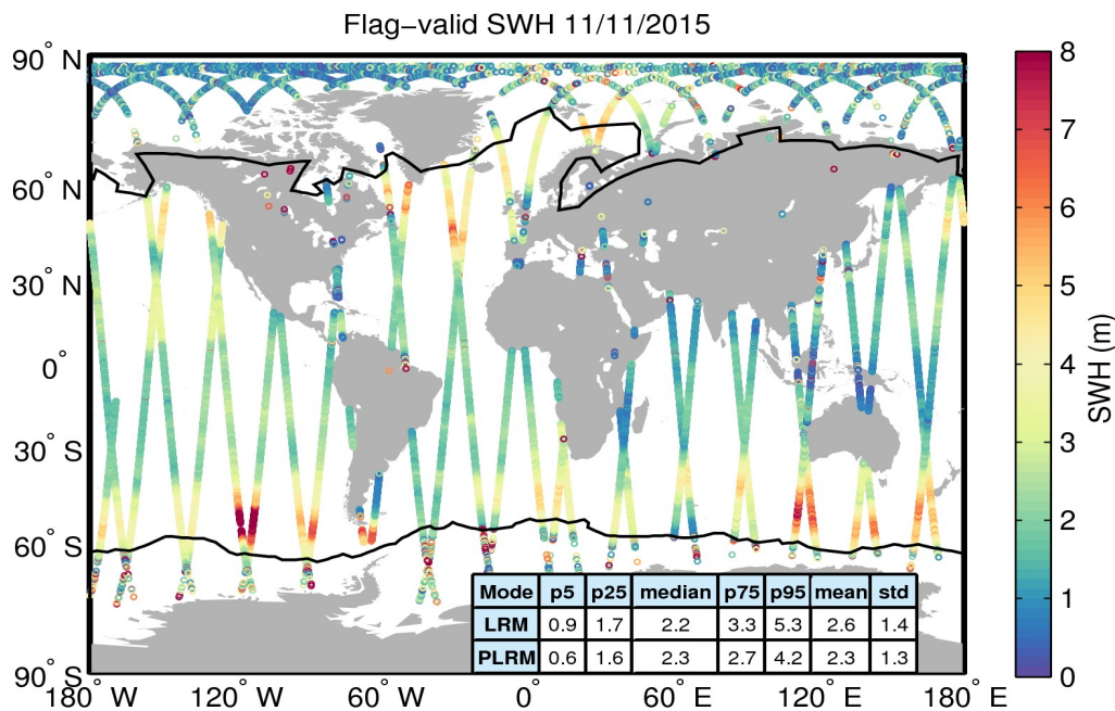
Figure 15. Geographical distribution of flag-valid SWH data over oceans and lakes for 11/11/2015. The statistical values shown in the table refer to the SWH in m and are calculated separately for LRM and PLRM regions. Measurements taken over polar polygons have been excluded from the computation of the statistical values. The black lines mark the outer limit of the Arctic and Antarctic polar polygons.
