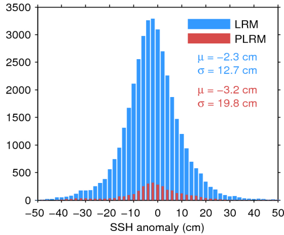
Figure 11. Histogram of science-valid SSH anomaly over oceans and lakes for LRM (blue) and PLRM (red) for 11/11/2015. The mean ( \mu ) and standard deviation ( \sigma ) are also shown. Note that values outside [-50\ 50] cm are excluded from the histogram for the sake of readability but not from the computation of \mu and \sigma .
