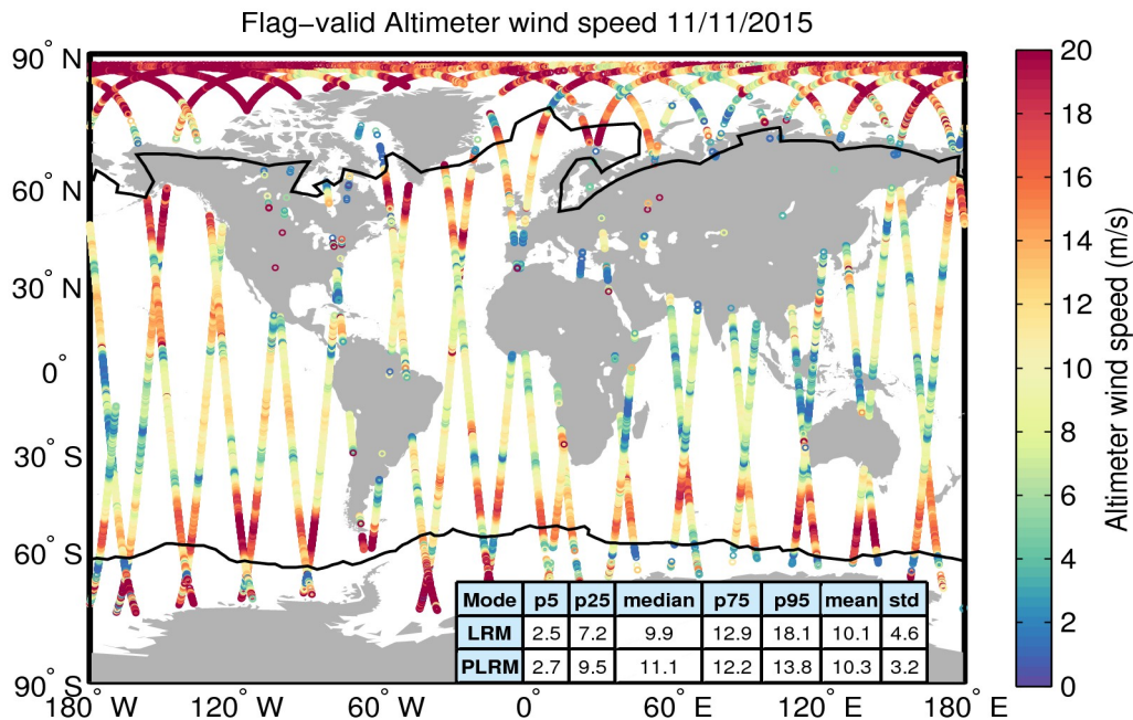
Figure 31. Geographical distribution of flag-valid wind data over oceans and lakes for 11/11/2015. The statistical values shown in the table refer to the wind in m/s and are calculated separately for LRM and PLRM regions. Measurements taken over polar polygons have been excluded from the computation of the statistical values. The black lines mark the outer limit of the Arctic and Antarctic polar polygons.
