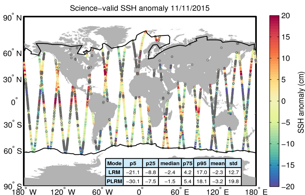
Figure 10. Geographical distribution of science-valid SSH anomaly data over oceans and lakes for 11/11/2015. The statistical values shown in the table refer to the SSH anomaly in cm and are calculated separately for LRM and PLRM regions. The black lines mark the outer limit of the Arctic and Antarctic polar polygons. Gray circles denote records that have been rejected based on the editing criteria described in Table 2.
