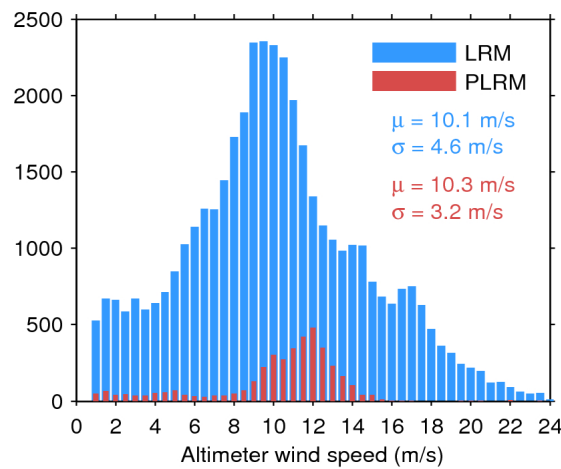
Figure 33. Histogram of flag-valid wind over oceans and lakes for LRM (blue) and PLRM (red) for 11/11/2015. The mean ( \mu ) and standard deviation ( \sigma ) are also shown. Note that values larger than 24 m/s are excluded from the histogram for the sake of readability but not from the computation of \mu and \sigma .
