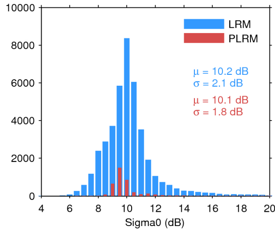
Figure 25. Histogram of flag-valid sigma0 over oceans and lakes for LRM (blue) and PLRM (red) for 11/11/2015. The mean ( \mu ) and standard deviation ( \sigma ) are also shown. Note that values outside [4 20] dB are excluded from the histogram for the sake of readability but not from the computation of \mu and \sigma .
