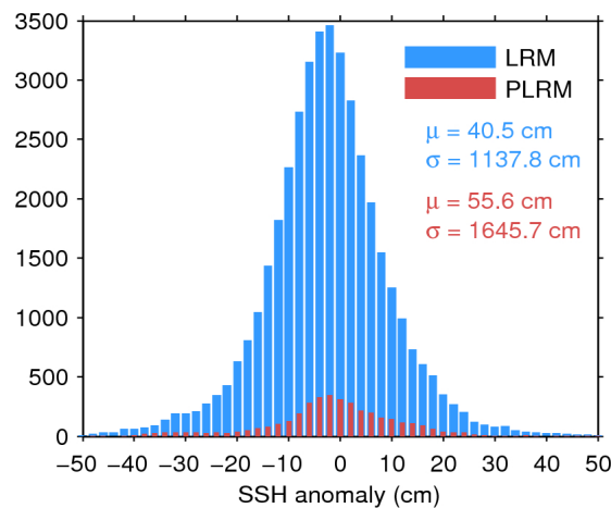
Figure 7. Histogram of flag-valid SSH anomaly over oceans and lakes for LRM (blue) and PLRM (red) for 11/11/2015. The mean ( \mu ) and standard deviation ( \sigma ) are also shown. Note that values outside [-50\ 50] cm are excluded from the histogram for the sake of readability but not from the computation of \mu and \sigma .
