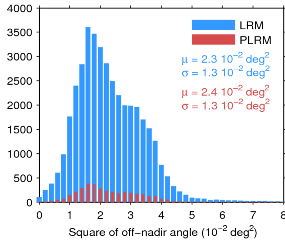
Figure 39. Histogram of flag-valid mispointing over oceans and lakes for LRM (blue) and PLRM (red) for 11/11/2015. Only positive values have been considered. The mean ( \mu ) and standard deviation ( \sigma ) are also shown. Note that values larger than 8 \cdot 10^{-2} \text{ deg}^2 are excluded from the histogram for the sake of readability but not from the computation of \mu and \sigma .
