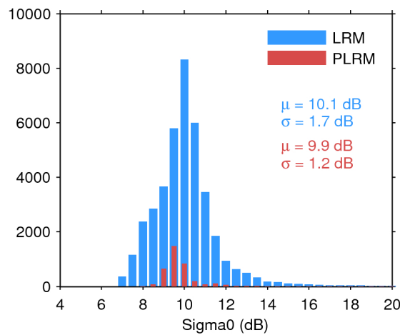
Figure 28. Histogram of science-valid sigma0 over oceans and lakes for LRM (blue) and PLRM (red) for 11/11/2015. The mean ( \mu ) and standard deviation ( \sigma ) are also shown. Note that values outside [4 20] dB are excluded from the histogram for the sake of readability but not from the computation of \mu and \sigma .
