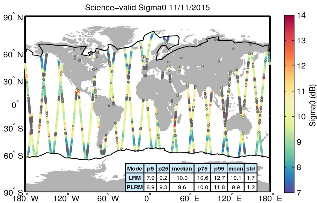
Figure 27. Geographical distribution of science-valid sigma0 data over oceans and lakes for 11/11/2015. The statistical values shown in the table refer to the sigma0 in dB and are calculated separately for LRM and PLRM regions. The black lines mark the outer limit of the Arctic and Antarctic polar polygons. Gray circles denote records that have been rejected based on the editing criteria described in Table 4.
