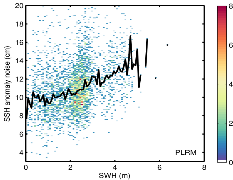
Figure 9. 2D histogram showing flag-valid SSH anomaly noise as a function of SWH for LRM (top) and PLRM (bottom) for 11/11/2015. The black line denotes the median SSH anomaly noise as a function of SWH.
