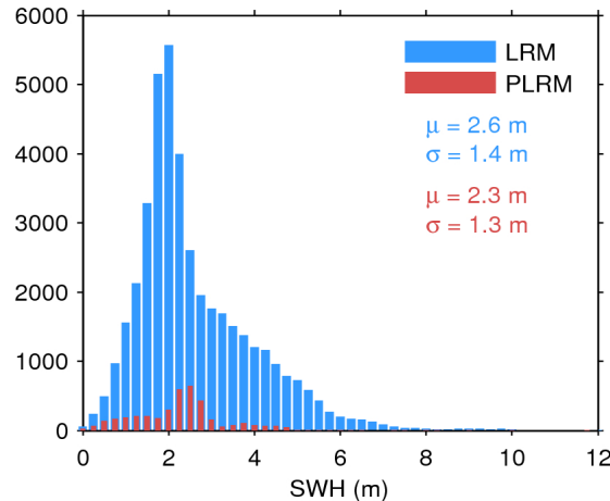
Figure 17. Histogram of flag-valid SWH over oceans and lakes for LRM (blue) and PLRM (red) for 11/11/2015. The mean ( \mu ) and standard deviation ( \sigma ) are also shown. Note that values larger than 12 m are excluded from the histogram for the sake of readability but not from the computation of \mu and \sigma .
