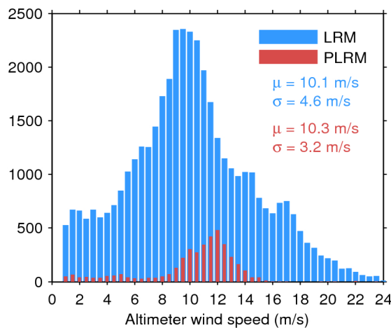
Figure 35. Histogram of science-valid wind over oceans and lakes for LRM (blue) and PLRM (red) for 11/11/2015. The mean ( \mu ) and standard deviation ( \sigma ) are also shown. Note that values larger than 24 m/s are excluded from the histogram for the sake of readability but not from the computation of \mu and \sigma .
