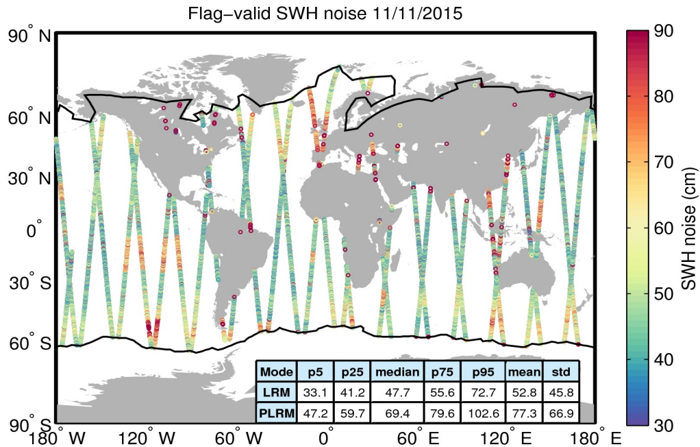
Figure 18. Geographical distribution of flag-valid 20-Hz SWH measurement noise over oceans and lakes for 11/11/2015. The statistical values shown in the table refer to the SWH noise and are calculated separately for LRM and PLRM regions. Measurements taken over polar polygons have been excluded from the computation of the statistical values. The black lines mark the outer limit of the Arctic and Antarctic polar polygons.
