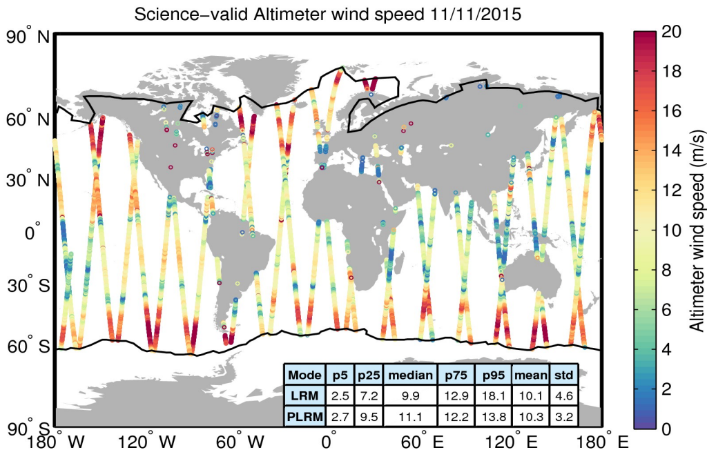
Figure 34. Geographical distribution of science-valid wind data over oceans and lakes for 11/11/2015. The statistical values shown in the table refer to the wind in m/s and are calculated separately for LRM and PLRM regions. The black lines mark the outer limit of the Arctic and Antarctic polar polygons. Gray circles denote records that have been rejected based on the editing criteria described in Table 5.
