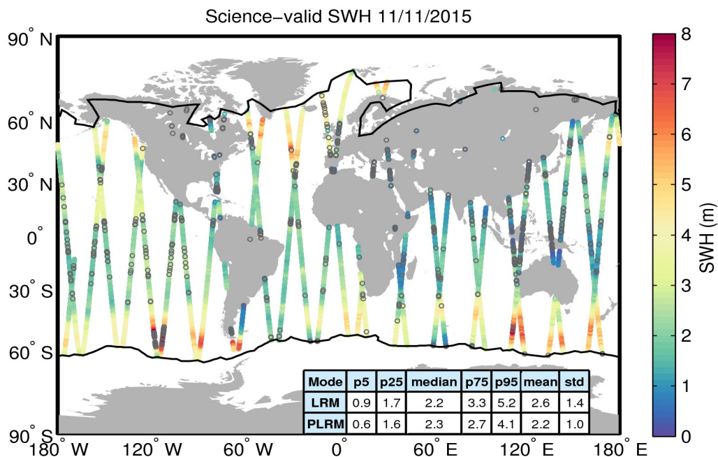
Figure 19. Geographical distribution of science-valid SWH data over oceans and lakes for 11/11/2015. The statistical values shown in the table refer to the SWH in m and are calculated separately for LRM and PLRM regions. The black lines mark the outer limit of the Arctic and Antarctic polar polygons. Gray circles denote records that have been rejected based on the editing criteria described in Table 3.
