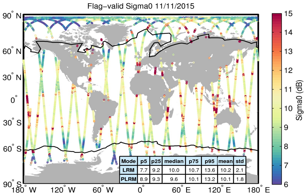
Figure 23. Geographical distribution of flag-valid sigma0 data over oceans and lakes for 11/11/2015. The statistical values shown in the table refer to the sigma0 in dB and are calculated separately for LRM and PLRM regions. Measurements taken over polar polygons have been excluded from the computation of the statistical values. The black lines mark the outer limit of the Arctic and Antarctic polar polygons.
