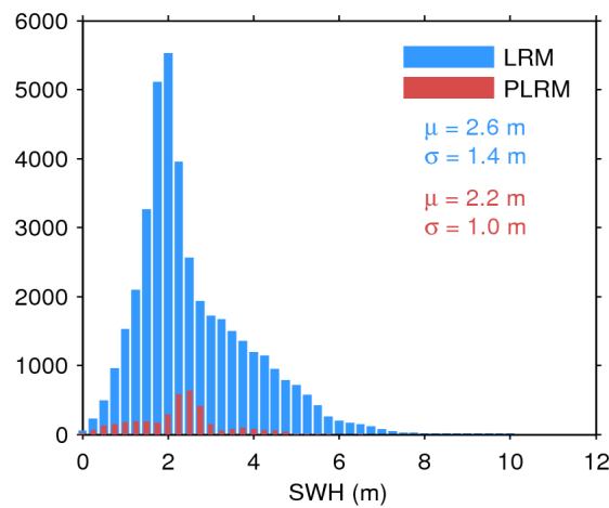
Figure 20. Histogram of science-valid SWH over oceans and lakes for LRM (blue) and PLRM (red) for 11/11/2015. The mean ( \mu ) and standard deviation ( \sigma ) are also shown. Note that values larger than 12 m are excluded from the histogram for the sake of readability but not from the computation of \mu and \sigma .
