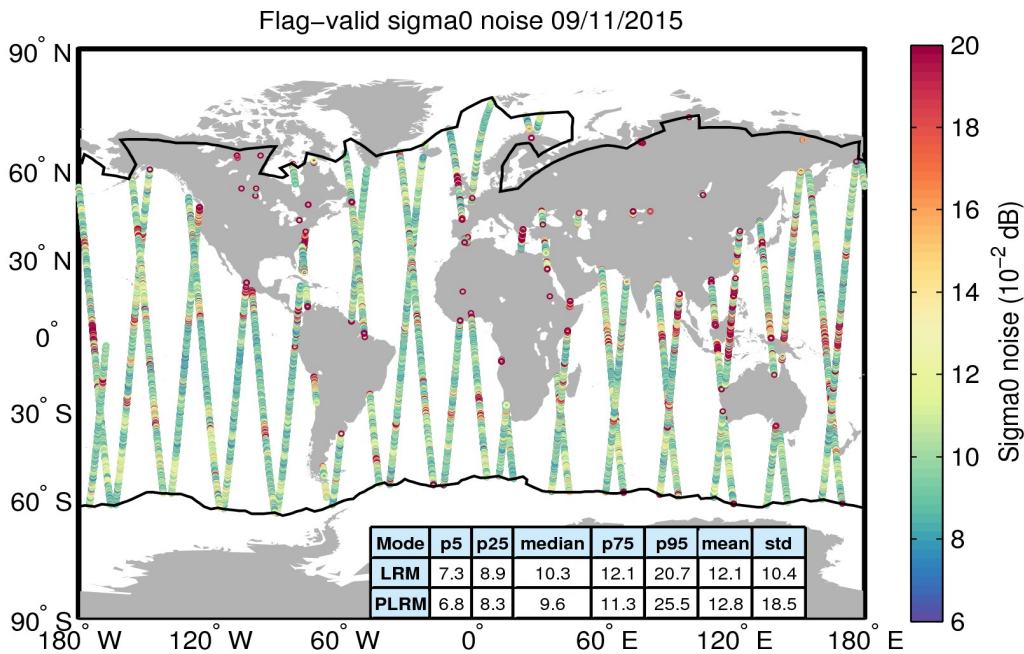
Figure 26. Geographical distribution of flag-valid 20-Hz sigma0 measurement noise over oceans and lakes for 09/11/2015. The statistical values shown in the table refer to the sigma0 noise and are calculated separately for LRM and PLRM regions. Measurements taken over polar polygons have been excluded from the computation of the statistical values. The black lines mark the outer limit of the Arctic and Antarctic polar polygons.
