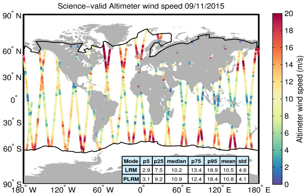
Figure 34. Geographical distribution of science-valid wind data over oceans and lakes for 09/11/2015. The statistical values shown in the table refer to the wind in m/s and are calculated separately for LRM and PLRM regions. The black lines mark the outer limit of the Arctic and Antarctic polar polygons. Gray circles denote records that have been rejected based on the editing criteria described in Table 5.
