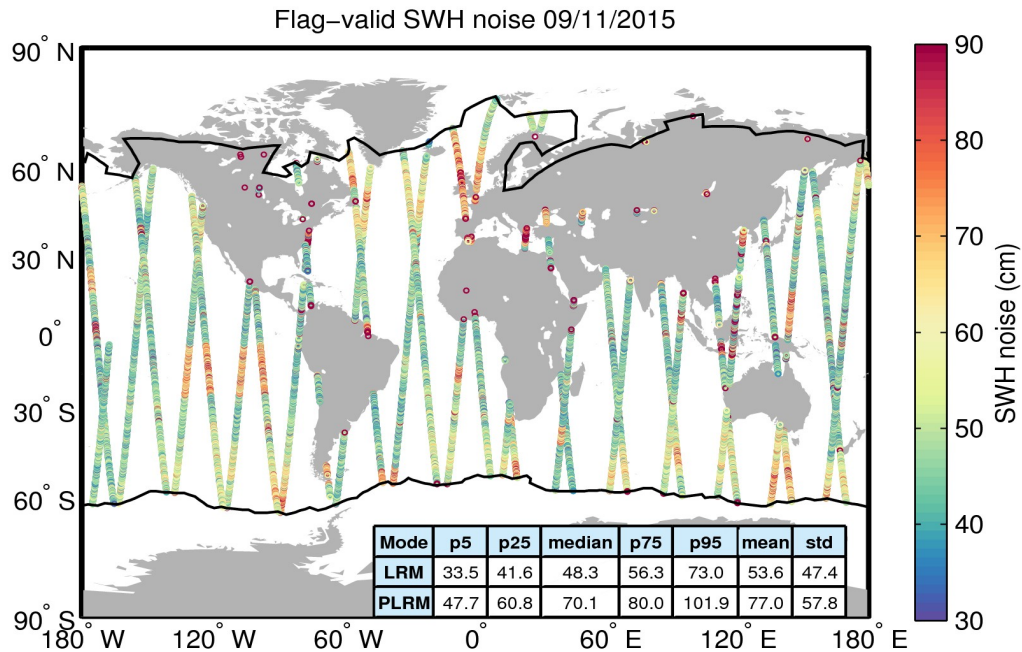
Figure 18. Geographical distribution of flag-valid 20-Hz SWH measurement noise over oceans and lakes for 09/11/2015. The statistical values shown in the table refer to the SWH noise and are calculated separately for LRM and PLRM regions. Measurements taken over polar polygons have been excluded from the computation of the statistical values. The black lines mark the outer limit of the Arctic and Antarctic polar polygons.
