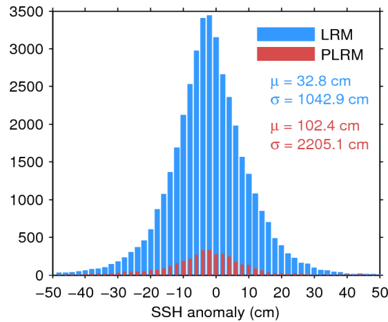
Figure 7. Histogram of flag-valid SSH anomaly over oceans and lakes for LRM (blue) and PLRM (red) for 09/11/2015. The mean ( \mu ) and standard deviation ( \sigma ) are also shown. Note that values outside [-50\ 50] cm are excluded from the histogram for the sake of readability but not from the computation of \mu and \sigma .
