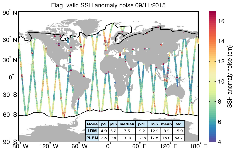
Figure 8. Geographical distribution of flag-valid 20-Hz SSH anomaly measurement noise over oceans and lakes for 09/11/2015. The statistical values shown in the table refer to the SSH anomaly noise and are calculated separately for LRM and PLRM regions. Measurements taken over polar polygons have been excluded from the computation of the statistical values. The black lines mark the outer limit of the Arctic and Antarctic polar polygons.
