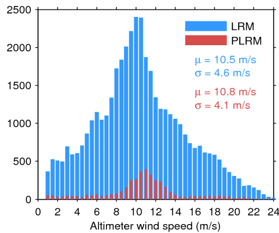
Figure 33. Histogram of flag-valid wind over oceans and lakes for LRM (blue) and PLRM (red) for 09/11/2015. The mean ( \mu ) and standard deviation ( \sigma ) are also shown. Note that values larger than 24 m/s are excluded from the histogram for the sake of readability but not from the computation of \mu and \sigma .
