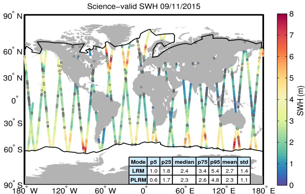
Figure 19. Geographical distribution of science-valid SWH data over oceans and lakes for 09/11/2015. The statistical values shown in the table refer to the SWH in m and are calculated separately for LRM and PLRM regions. The black lines mark the outer limit of the Arctic and Antarctic polar polygons. Gray circles denote records that have been rejected based on the editing criteria described in Table 3.
