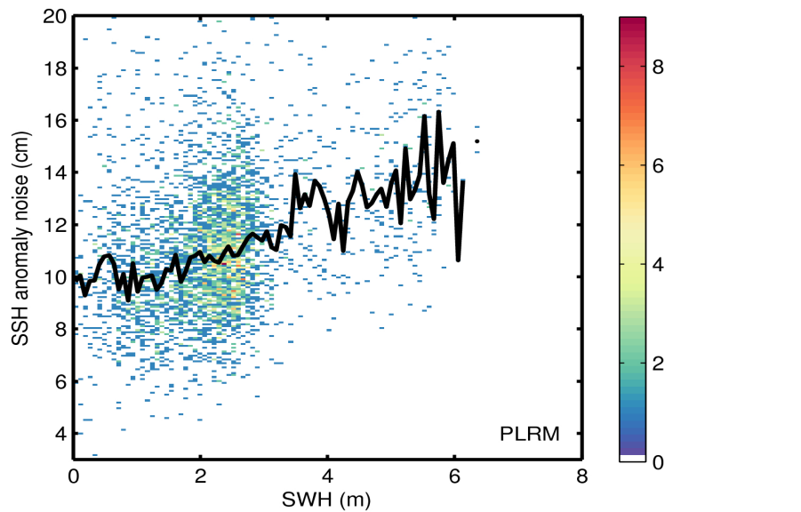
Figure 9. 2D histogram showing flag-valid SSH anomaly noise as a function of SWH for LRM (top) and PLRM (bottom) for 09/11/2015. The black line denotes the median SSH anomaly noise as a function of SWH.
