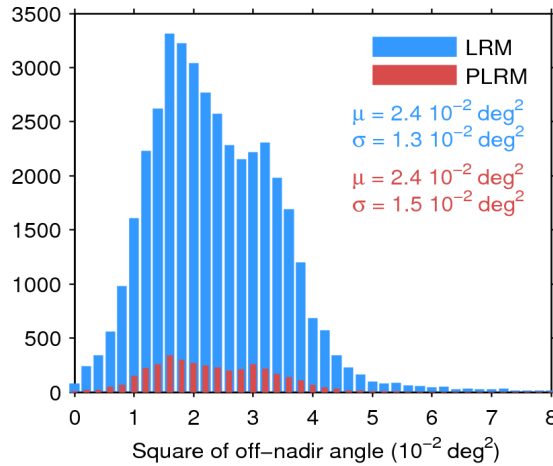
Figure 39. Histogram of flag-valid mispointing over oceans and lakes for LRM (blue) and PLRM (red) for 09/11/2015. Only positive values have been considered. The mean ( \mu ) and standard deviation ( \sigma ) are also shown. Note that values larger than 8 \cdot 10^{-2} \text{ deg}^2 are excluded from the histogram for the sake of readability but not from the computation of \mu and \sigma .
