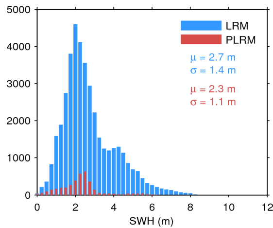
Figure 20. Histogram of science-valid SWH over oceans and lakes for LRM (blue) and PLRM (red) for 09/11/2015. The mean ( \mu ) and standard deviation ( \sigma ) are also shown. Note that values larger than 12 m are excluded from the histogram for the sake of readability but not from the computation of \mu and \sigma .
