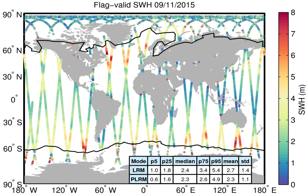
Figure 15. Geographical distribution of flag-valid SWH data over oceans and lakes for 09/11/2015. The statistical values shown in the table refer to the SWH in m and are calculated separately for LRM and PLRM regions. Measurements taken over polar polygons have been excluded from the computation of the statistical values. The black lines mark the outer limit of the Arctic and Antarctic polar polygons.
