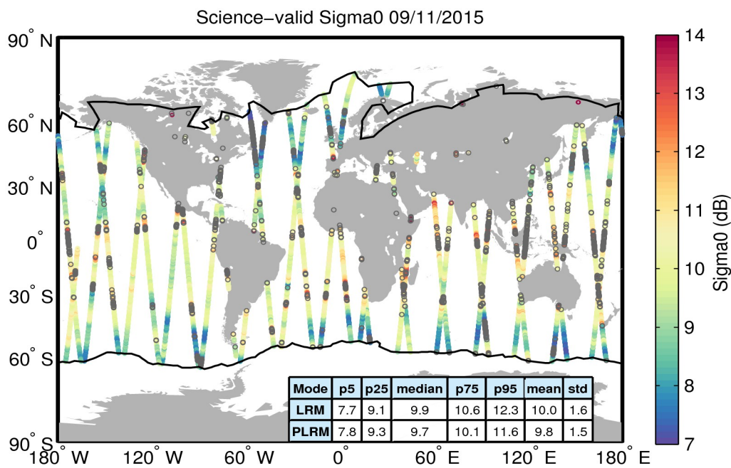
Figure 27. Geographical distribution of science-valid sigma0 data over oceans and lakes for 09/11/2015. The statistical values shown in the table refer to the sigma0 in dB and are calculated separately for LRM and PLRM regions. The black lines mark the outer limit of the Arctic and Antarctic polar polygons. Gray circles denote records that have been rejected based on the editing criteria described in Table 4.
