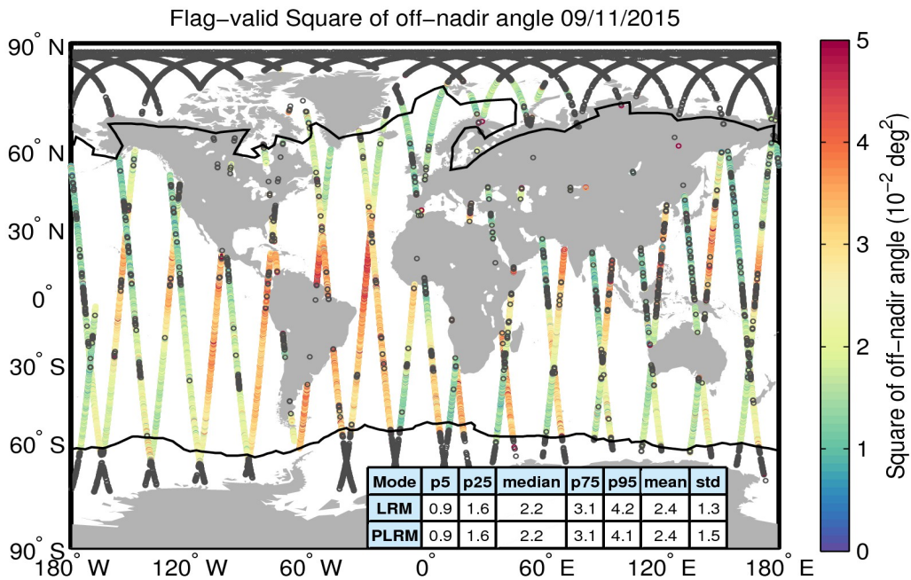
Figure 37. Geographical distribution of flag-valid mispointing data over oceans and lakes for 09/11/2015. The statistical values shown in the table refer to the mispointing in 10^{-2} deg 2 and are calculated separately for LRM and PLRM regions. Measurements taken over polar polygons have been excluded from the computation of the statistical values. The black lines mark the outer limit of the Arctic and Antarctic polar polygons. Gray circles denote negative values.
