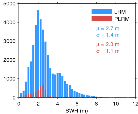
Figure 17. Histogram of flag-valid SWH over oceans and lakes for LRM (blue) and PLRM (red) for 09/11/2015. The mean ( \mu ) and standard deviation ( \sigma ) are also shown. Note that values larger than 12 m are excluded from the histogram for the sake of readability but not from the computation of \mu and \sigma .
