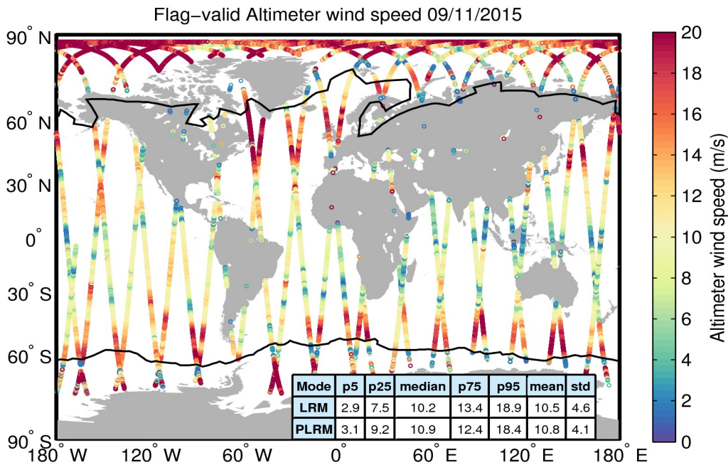
Figure 31. Geographical distribution of flag-valid wind data over oceans and lakes for 09/11/2015. The statistical values shown in the table refer to the wind in m/s and are calculated separately for LRM and PLRM regions. Measurements taken over polar polygons have been excluded from the computation of the statistical values. The black lines mark the outer limit of the Arctic and Antarctic polar polygons.
