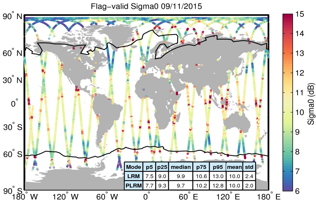
Figure 23. Geographical distribution of flag-valid sigma0 data over oceans and lakes for 09/11/2015. The statistical values shown in the table refer to the sigma0 in dB and are calculated separately for LRM and PLRM regions. Measurements taken over polar polygons have been excluded from the computation of the statistical values. The black lines mark the outer limit of the Arctic and Antarctic polar polygons.
