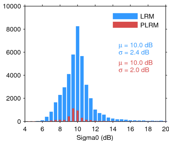
Figure 25. Histogram of flag-valid sigma0 over oceans and lakes for LRM (blue) and PLRM (red) for 09/11/2015. The mean ( \mu ) and standard deviation ( \sigma ) are also shown. Note that values outside [4 20] dB are excluded from the histogram for the sake of readability but not from the computation of \mu and \sigma .
