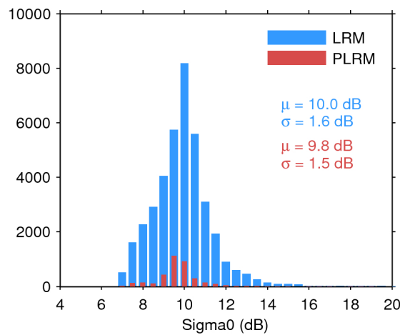
Figure 28. Histogram of science-valid sigma0 over oceans and lakes for LRM (blue) and PLRM (red) for 09/11/2015. The mean ( \mu ) and standard deviation ( \sigma ) are also shown. Note that values outside [4 20] dB are excluded from the histogram for the sake of readability but not from the computation of \mu and \sigma .
