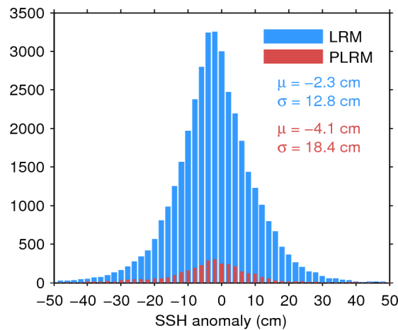
Figure 11. Histogram of science-valid SSH anomaly over oceans and lakes for LRM (blue) and PLRM (red) for 09/11/2015. The mean ( \mu ) and standard deviation ( \sigma ) are also shown. Note that values outside [-50\ 50] cm are excluded from the histogram for the sake of readability but not from the computation of \mu and \sigma .
