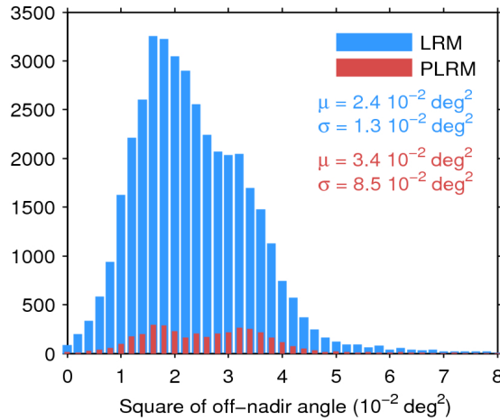
Figure 39. Histogram of flag-valid mispointing over oceans and lakes for LRM (blue) and PLRM (red) for 07/11/2015. Only positive values have been considered. The mean ( \mu ) and standard deviation ( \sigma ) are also shown. Note that values larger than 8 \cdot 10^{-2} \text{ deg}^2 are excluded from the histogram for the sake of readability but not from the computation of \mu and \sigma .
