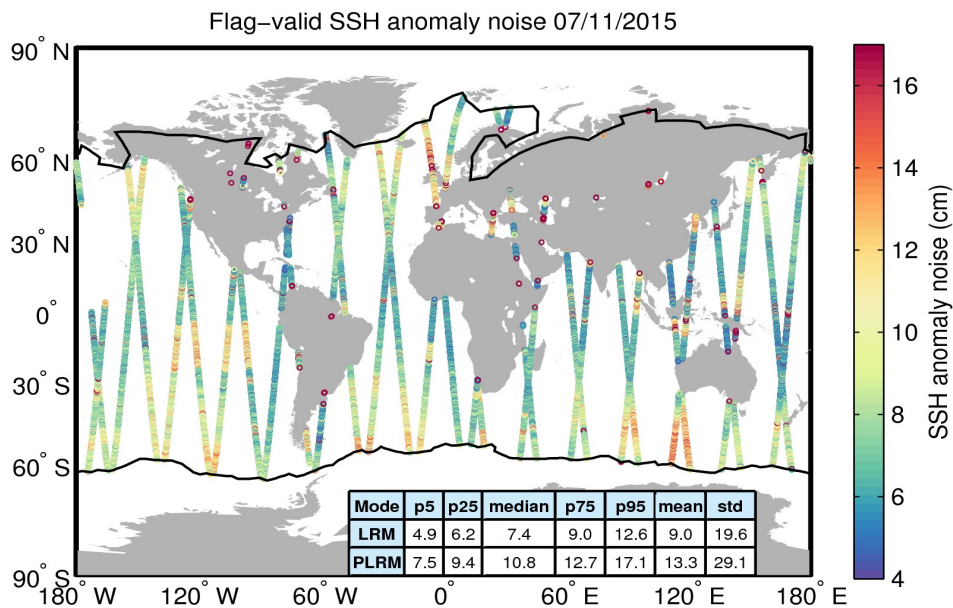
Figure 8. Geographical distribution of flag-valid 20-Hz SSH anomaly measurement noise over oceans and lakes for 07/11/2015. The statistical values shown in the table refer to the SSH anomaly noise and are calculated separately for LRM and PLRM regions. Measurements taken over polar polygons have been excluded from the computation of the statistical values. The black lines mark the outer limit of the Arctic and Antarctic polar polygons.
