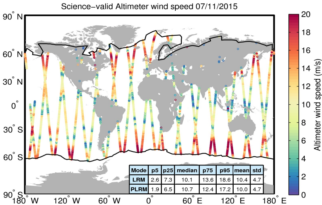
Figure 34. Geographical distribution of science-valid wind data over oceans and lakes for 07/11/2015. The statistical values shown in the table refer to the wind in m/s and are calculated separately for LRM and PLRM regions. The black lines mark the outer limit of the Arctic and Antarctic polar polygons. Gray circles denote records that have been rejected based on the editing criteria described in Table 5.
