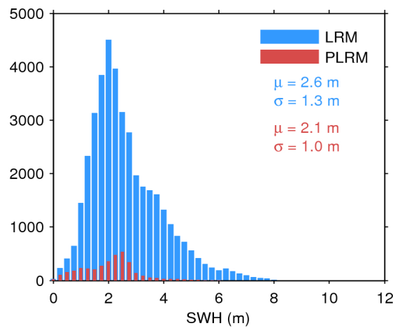
Figure 20. Histogram of science-valid SWH over oceans and lakes for LRM (blue) and PLRM (red) for 07/11/2015. The mean ( \mu ) and standard deviation ( \sigma ) are also shown. Note that values larger than 12 m are excluded from the histogram for the sake of readability but not from the computation of \mu and \sigma .
