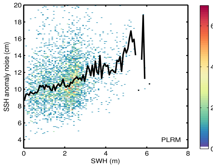
Figure 9. 2D histogram showing flag-valid SSH anomaly noise as a function of SWH for LRM (top) and PLRM (bottom) for 07/11/2015. The black line denotes the median SSH anomaly noise as a function of SWH.
