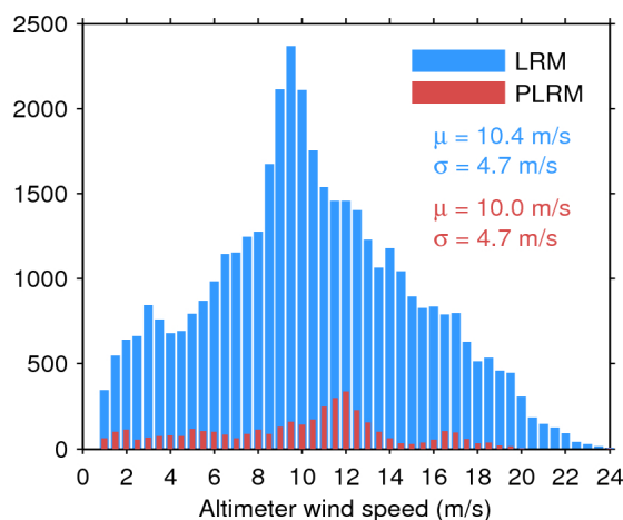
Figure 33. Histogram of flag-valid wind over oceans and lakes for LRM (blue) and PLRM (red) for 07/11/2015. The mean ( \mu ) and standard deviation ( \sigma ) are also shown. Note that values larger than 24 m/s are excluded from the histogram for the sake of readability but not from the computation of \mu and \sigma .
