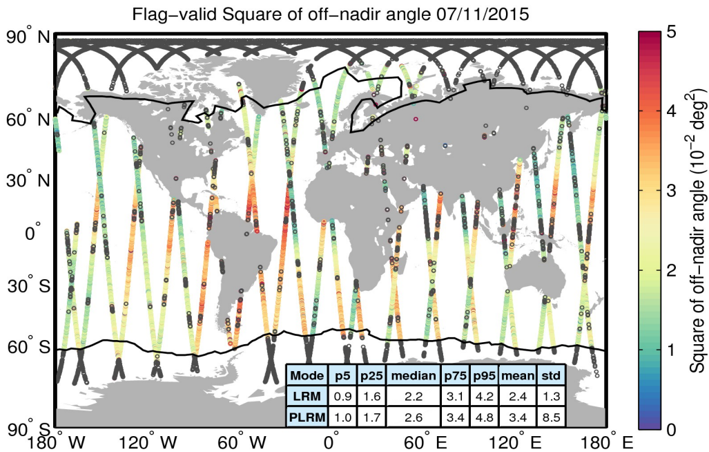
Figure 37. Geographical distribution of flag-valid mispointing data over oceans and lakes for 07/11/2015. The statistical values shown in the table refer to the mispointing in 10^{-2} deg 2 and are calculated separately for LRM and PLRM regions. Measurements taken over polar polygons have been excluded from the computation of the statistical values. The black lines mark the outer limit of the Arctic and Antarctic polar polygons. Gray circles denote negative values.
