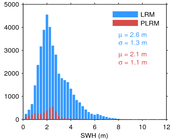
Figure 17. Histogram of flag-valid SWH over oceans and lakes for LRM (blue) and PLRM (red) for 07/11/2015. The mean ( \mu ) and standard deviation ( \sigma ) are also shown. Note that values larger than 12 m are excluded from the histogram for the sake of readability but not from the computation of \mu and \sigma .
