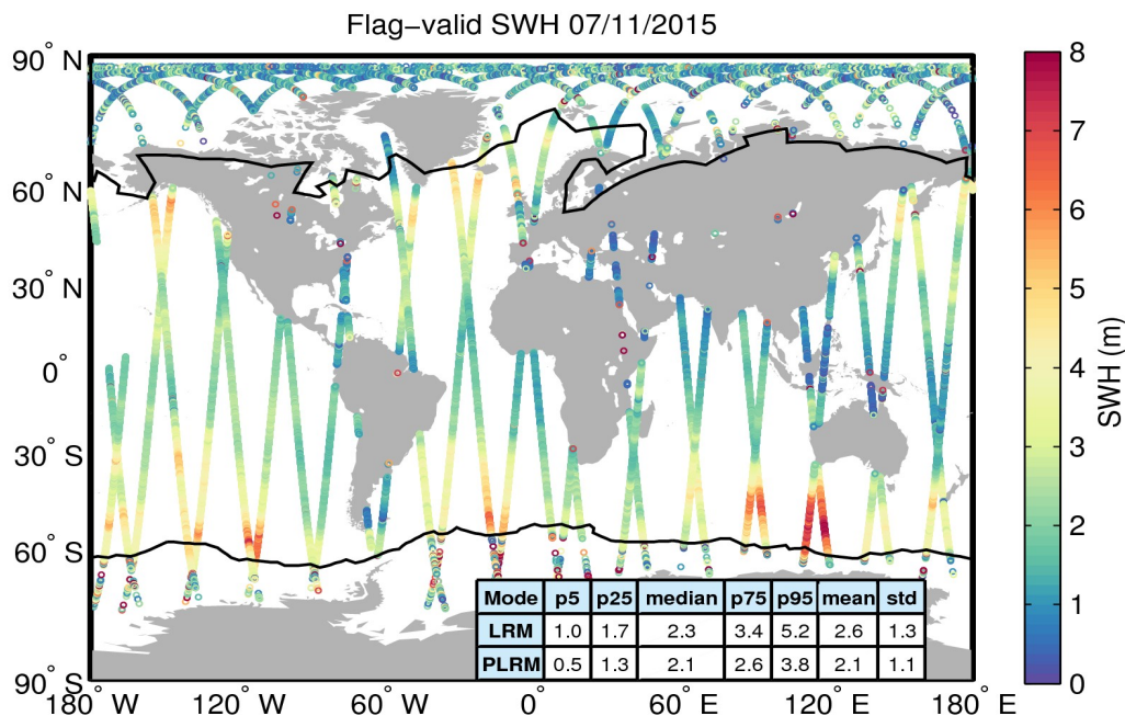
Figure 15. Geographical distribution of flag-valid SWH data over oceans and lakes for 07/11/2015. The statistical values shown in the table refer to the SWH in m and are calculated separately for LRM and PLRM regions. Measurements taken over polar polygons have been excluded from the computation of the statistical values. The black lines mark the outer limit of the Arctic and Antarctic polar polygons.
