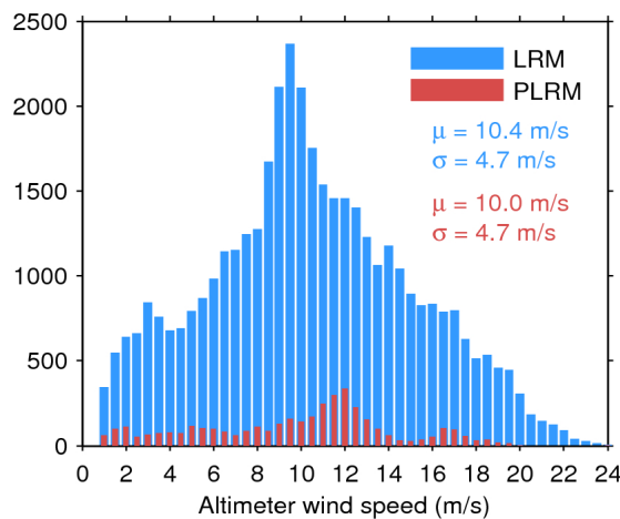
Figure 35. Histogram of science-valid wind over oceans and lakes for LRM (blue) and PLRM (red) for 07/11/2015. The mean ( \mu ) and standard deviation ( \sigma ) are also shown. Note that values larger than 24 m/s are excluded from the histogram for the sake of readability but not from the computation of \mu and \sigma .
