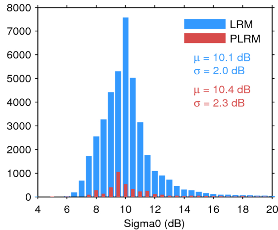
Figure 25. Histogram of flag-valid sigma0 over oceans and lakes for LRM (blue) and PLRM (red) for 07/11/2015. The mean ( \mu ) and standard deviation ( \sigma ) are also shown. Note that values outside [4 20] dB are excluded from the histogram for the sake of readability but not from the computation of \mu and \sigma .
