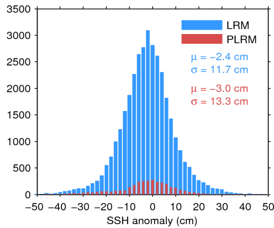
Figure 11. Histogram of science-valid SSH anomaly over oceans and lakes for LRM (blue) and PLRM (red) for 07/11/2015. The mean ( \mu ) and standard deviation ( \sigma ) are also shown. Note that values outside [-50\ 50] cm are excluded from the histogram for the sake of readability but not from the computation of \mu and \sigma .
