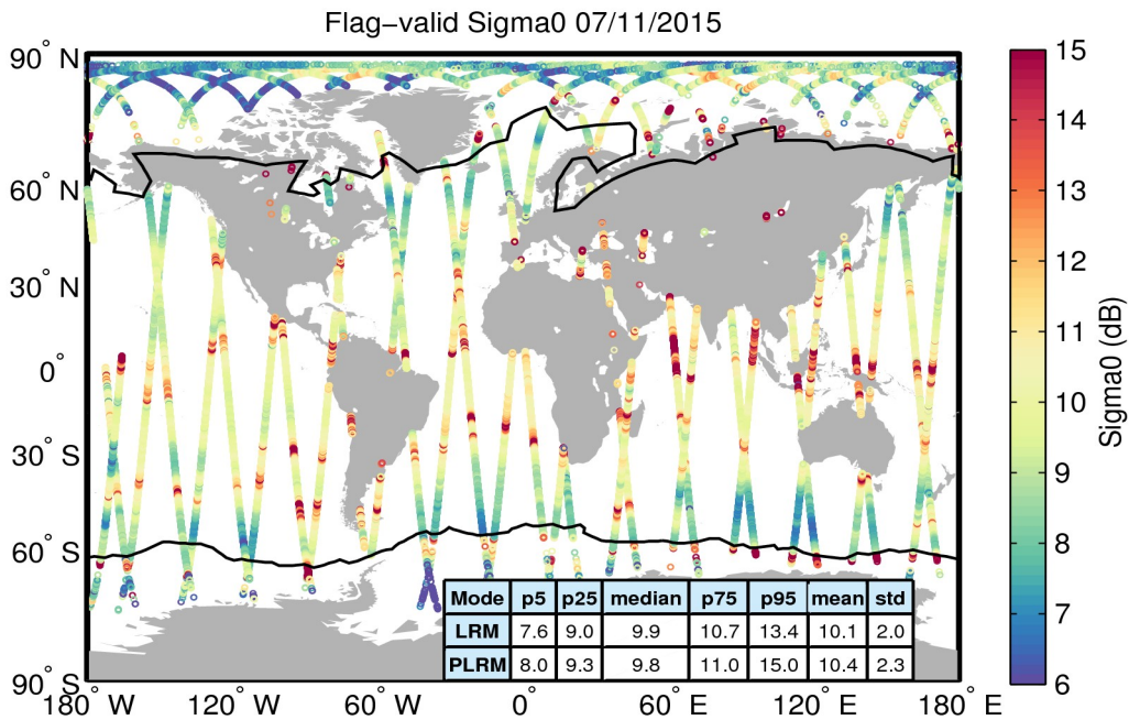
Figure 23. Geographical distribution of flag-valid sigma0 data over oceans and lakes for 07/11/2015. The statistical values shown in the table refer to the sigma0 in dB and are calculated separately for LRM and PLRM regions. Measurements taken over polar polygons have been excluded from the computation of the statistical values. The black lines mark the outer limit of the Arctic and Antarctic polar polygons.
