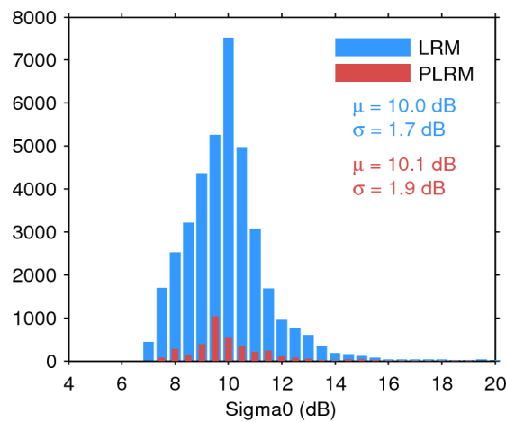
Figure 28. Histogram of science-valid sigma0 over oceans and lakes for LRM (blue) and PLRM (red) for 07/11/2015. The mean ( \mu ) and standard deviation ( \sigma ) are also shown. Note that values outside [4 20] dB are excluded from the histogram for the sake of readability but not from the computation of \mu and \sigma .
