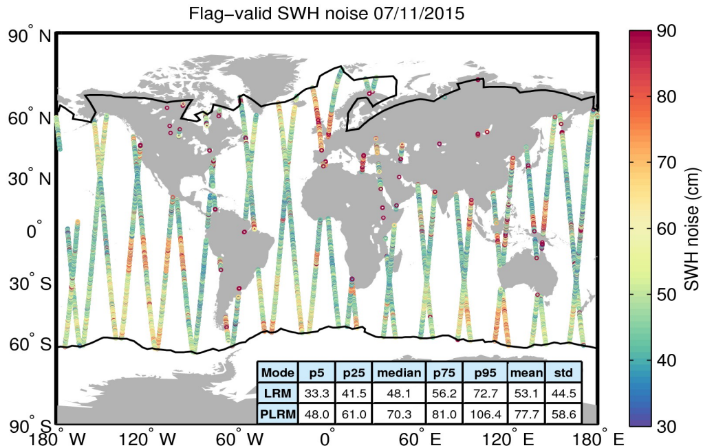
Figure 18. Geographical distribution of flag-valid 20-Hz SWH measurement noise over oceans and lakes for 07/11/2015. The statistical values shown in the table refer to the SWH noise and are calculated separately for LRM and PLRM regions. Measurements taken over polar polygons have been excluded from the computation of the statistical values. The black lines mark the outer limit of the Arctic and Antarctic polar polygons.
