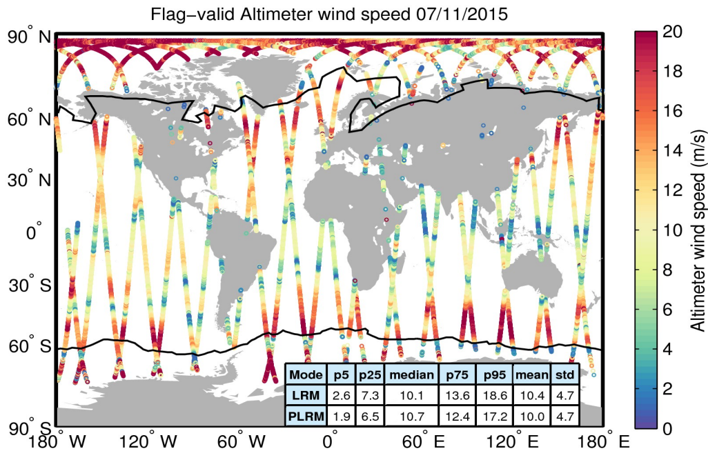
Figure 31. Geographical distribution of flag-valid wind data over oceans and lakes for 07/11/2015. The statistical values shown in the table refer to the wind in m/s and are calculated separately for LRM and PLRM regions. Measurements taken over polar polygons have been excluded from the computation of the statistical values. The black lines mark the outer limit of the Arctic and Antarctic polar polygons.
