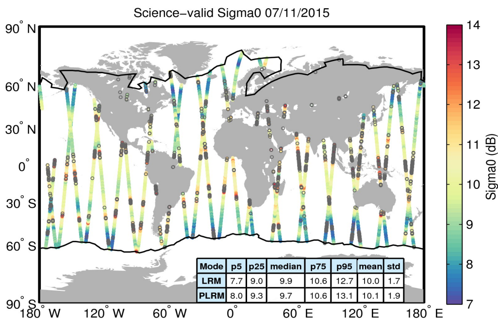
Figure 27. Geographical distribution of science-valid sigma0 data over oceans and lakes for 07/11/2015. The statistical values shown in the table refer to the sigma0 in dB and are calculated separately for LRM and PLRM regions. The black lines mark the outer limit of the Arctic and Antarctic polar polygons. Gray circles denote records that have been rejected based on the editing criteria described in Table 4.
