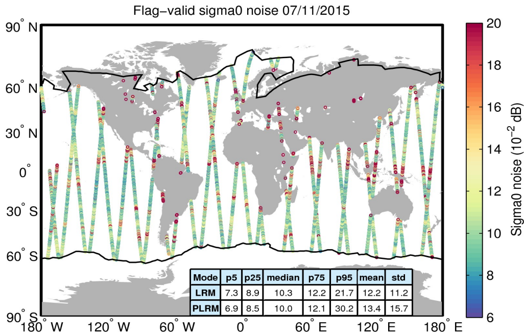
Figure 26. Geographical distribution of flag-valid 20-Hz sigma0 measurement noise over oceans and lakes for 07/11/2015. The statistical values shown in the table refer to the sigma0 noise and are calculated separately for LRM and PLRM regions. Measurements taken over polar polygons have been excluded from the computation of the statistical values. The black lines mark the outer limit of the Arctic and Antarctic polar polygons.
