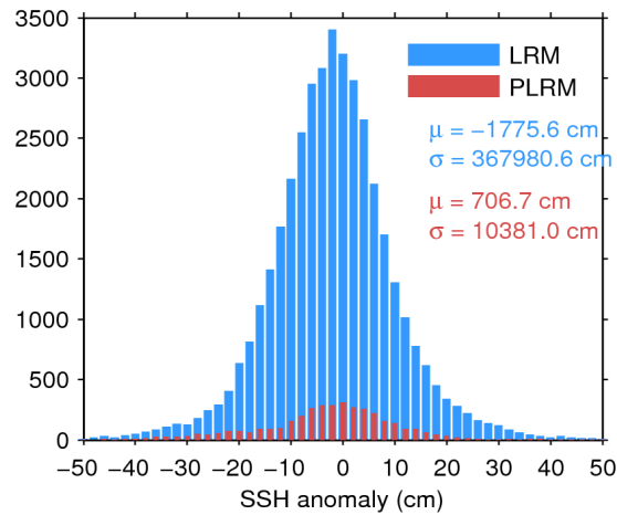
Figure 7. Histogram of flag-valid SSH anomaly over oceans and lakes for LRM (blue) and PLRM (red) for 07/11/2015. The mean ( \mu ) and standard deviation ( \sigma ) are also shown. Note that values outside [-50 \ 50] cm are excluded from the histogram for the sake of readability but not from the computation of \mu and \sigma .
