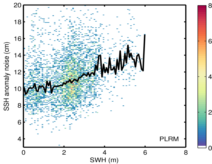
Figure 9. 2D histogram showing flag-valid SSH anomaly noise as a function of SWH for LRM (top) and PLRM (bottom) for 06/11/2015. The black line denotes the median SSH anomaly noise as a function of SWH.
