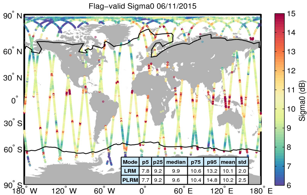
Figure 23. Geographical distribution of flag-valid sigma0 data over oceans and lakes for 06/11/2015. The statistical values shown in the table refer to the sigma0 in dB and are calculated separately for LRM and PLRM regions. Measurements taken over polar polygons have been excluded from the computation of the statistical values. The black lines mark the outer limit of the Arctic and Antarctic polar polygons.
