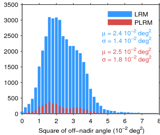
Figure 39. Histogram of flag-valid mispointing over oceans and lakes for LRM (blue) and PLRM (red) for 06/11/2015. Only positive values have been considered. The mean ( \mu ) and standard deviation ( \sigma ) are also shown. Note that values larger than 8 \cdot 10^{-2} \text{ deg}^2 are excluded from the histogram for the sake of readability but not from the computation of \mu and \sigma .
