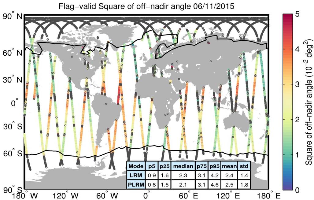
Figure 37. Geographical distribution of flag-valid mispointing data over oceans and lakes for 06/11/2015. The statistical values shown in the table refer to the mispointing in 10^{-2} deg 2 and are calculated separately for LRM and PLRM regions. Measurements taken over polar polygons have been excluded from the computation of the statistical values. The black lines mark the outer limit of the Arctic and Antarctic polar polygons. Gray circles denote negative values.
