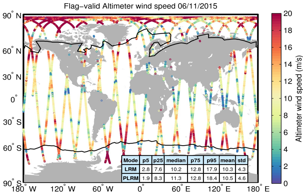
Figure 31. Geographical distribution of flag-valid wind data over oceans and lakes for 06/11/2015. The statistical values shown in the table refer to the wind in m/s and are calculated separately for LRM and PLRM regions. Measurements taken over polar polygons have been excluded from the computation of the statistical values. The black lines mark the outer limit of the Arctic and Antarctic polar polygons.
