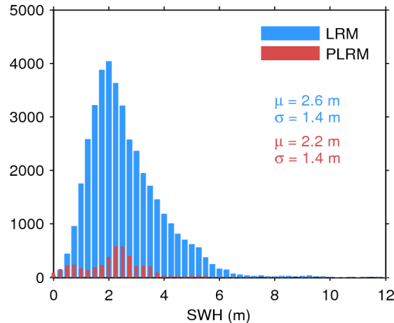
Figure 17. Histogram of flag-valid SWH over oceans and lakes for LRM (blue) and PLRM (red) for 06/11/2015. The mean ( \mu ) and standard deviation ( \sigma ) are also shown. Note that values larger than 12 m are excluded from the histogram for the sake of readability but not from the computation of \mu and \sigma .
