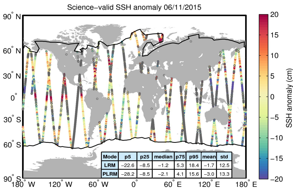
Figure 10. Geographical distribution of science-valid SSH anomaly data over oceans and lakes for 06/11/2015. The statistical values shown in the table refer to the SSH anomaly in cm and are calculated separately for LRM and PLRM regions. The black lines mark the outer limit of the Arctic and Antarctic polar polygons. Gray circles denote records that have been rejected based on the editing criteria described in Table 2.
