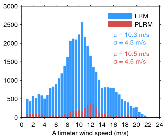
Figure 35. Histogram of science-valid wind over oceans and lakes for LRM (blue) and PLRM (red) for 06/11/2015. The mean ( \mu ) and standard deviation ( \sigma ) are also shown. Note that values larger than 24 m/s are excluded from the histogram for the sake of readability but not from the computation of \mu and \sigma .
