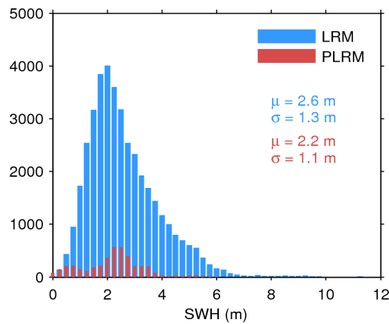
Figure 20. Histogram of science-valid SWH over oceans and lakes for LRM (blue) and PLRM (red) for 06/11/2015. The mean ( \mu ) and standard deviation ( \sigma ) are also shown. Note that values larger than 12 m are excluded from the histogram for the sake of readability but not from the computation of \mu and \sigma .
