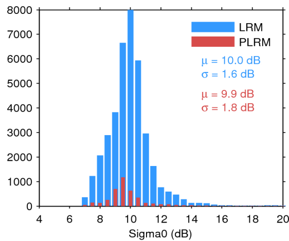
Figure 28. Histogram of science-valid sigma0 over oceans and lakes for LRM (blue) and PLRM (red) for 06/11/2015. The mean ( \mu ) and standard deviation ( \sigma ) are also shown. Note that values outside [4 20] dB are excluded from the histogram for the sake of readability but not from the computation of \mu and \sigma .
