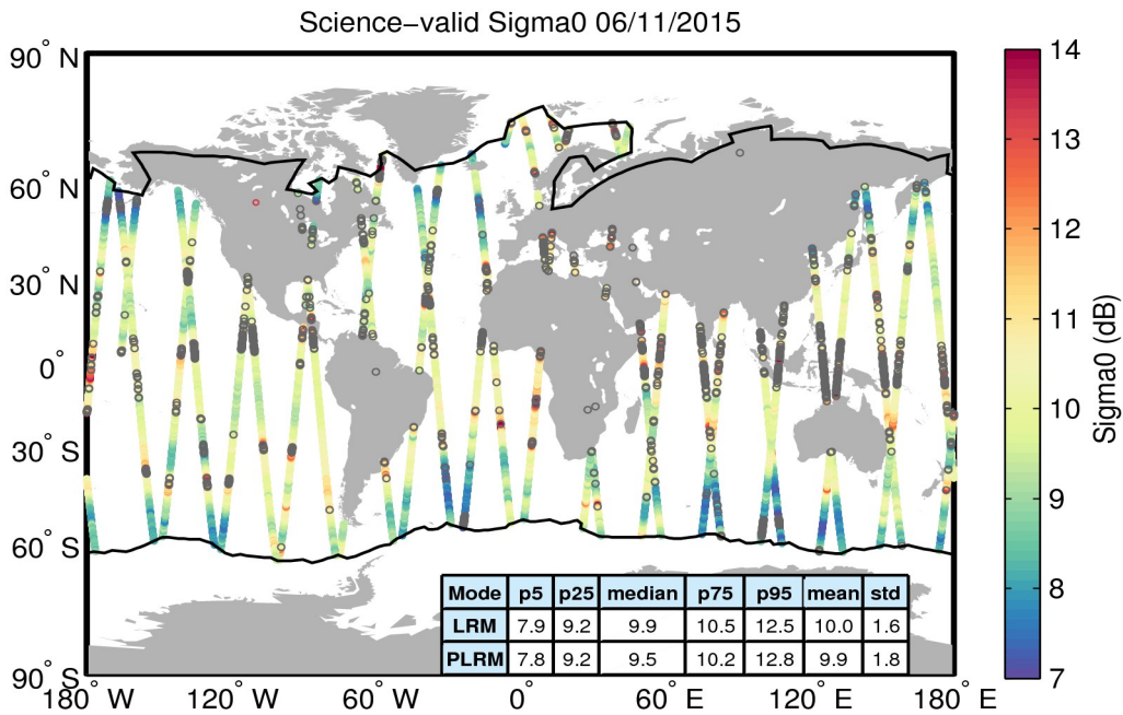
Figure 27. Geographical distribution of science-valid sigma0 data over oceans and lakes for 06/11/2015. The statistical values shown in the table refer to the sigma0 in dB and are calculated separately for LRM and PLRM regions. The black lines mark the outer limit of the Arctic and Antarctic polar polygons. Gray circles denote records that have been rejected based on the editing criteria described in Table 4.
