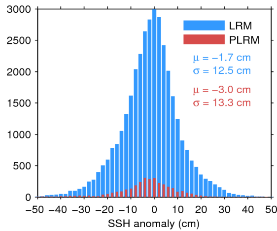
Figure 11. Histogram of science-valid SSH anomaly over oceans and lakes for LRM (blue) and PLRM (red) for 06/11/2015. The mean ( \mu ) and standard deviation ( \sigma ) are also shown. Note that values outside [-50\ 50] cm are excluded from the histogram for the sake of readability but not from the computation of \mu and \sigma .
