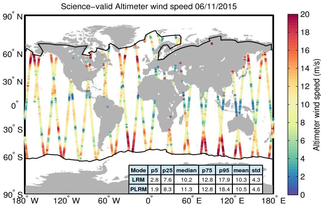
Figure 34. Geographical distribution of science-valid wind data over oceans and lakes for 06/11/2015. The statistical values shown in the table refer to the wind in m/s and are calculated separately for LRM and PLRM regions. The black lines mark the outer limit of the Arctic and Antarctic polar polygons. Gray circles denote records that have been rejected based on the editing criteria described in Table 5.
