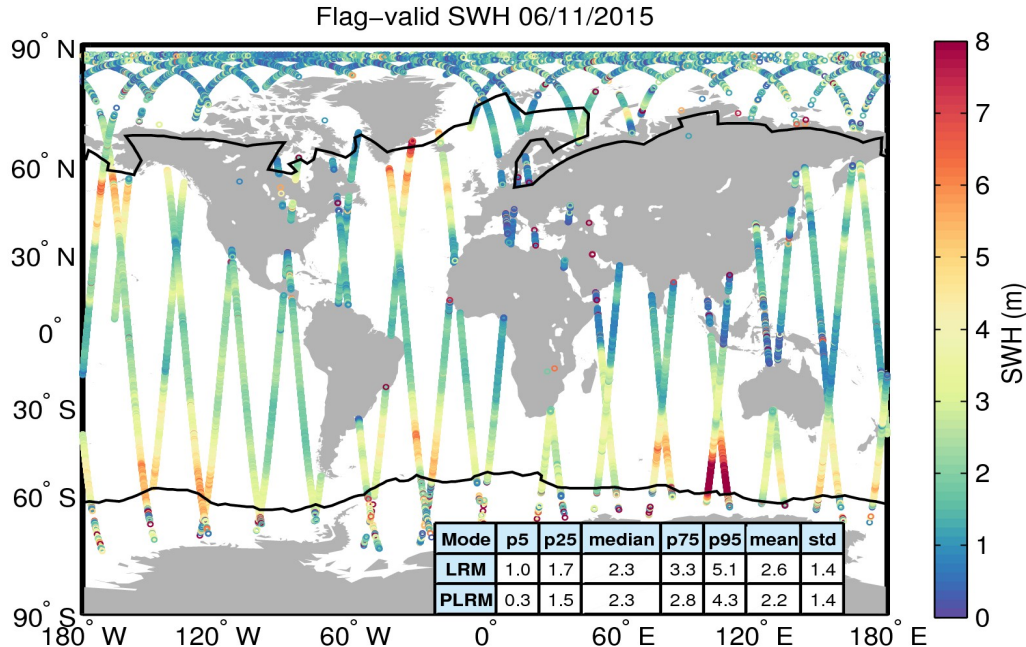
Figure 15. Geographical distribution of flag-valid SWH data over oceans and lakes for 06/11/2015. The statistical values shown in the table refer to the SWH in m and are calculated separately for LRM and PLRM regions. Measurements taken over polar polygons have been excluded from the computation of the statistical values. The black lines mark the outer limit of the Arctic and Antarctic polar polygons.
