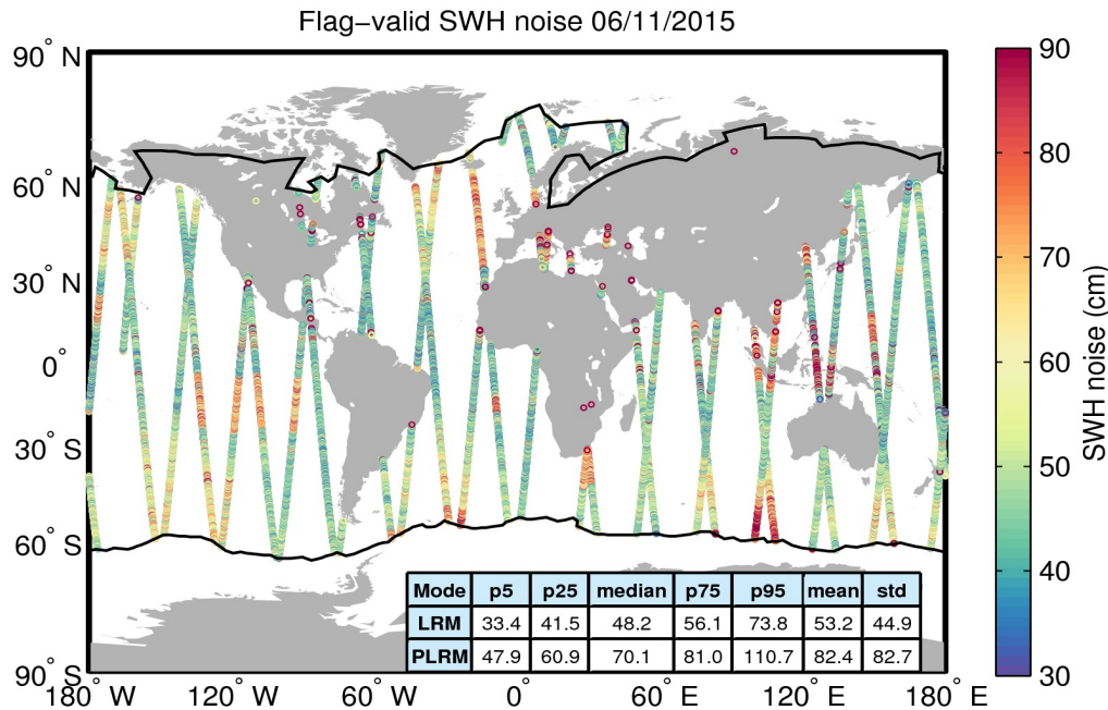
Figure 18. Geographical distribution of flag-valid 20-Hz SWH measurement noise over oceans and lakes for 06/11/2015. The statistical values shown in the table refer to the SWH noise and are calculated separately for LRM and PLRM regions. Measurements taken over polar polygons have been excluded from the computation of the statistical values. The black lines mark the outer limit of the Arctic and Antarctic polar polygons.
