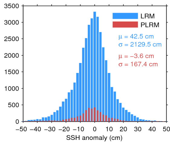
Figure 7. Histogram of flag-valid SSH anomaly over oceans and lakes for LRM (blue) and PLRM (red) for 06/11/2015. The mean ( \mu ) and standard deviation ( \sigma ) are also shown. Note that values outside [-50 50] cm are excluded from the histogram for the sake of readability but not from the computation of \mu and \sigma .
