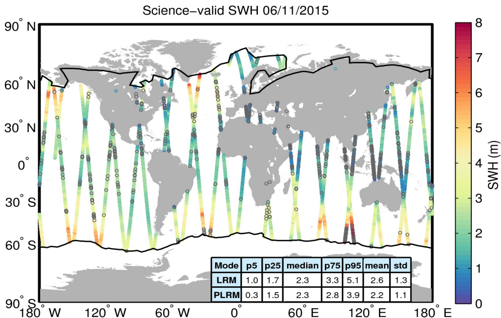
Figure 19. Geographical distribution of science-valid SWH data over oceans and lakes for 06/11/2015. The statistical values shown in the table refer to the SWH in m and are calculated separately for LRM and PLRM regions. The black lines mark the outer limit of the Arctic and Antarctic polar polygons. Gray circles denote records that have been rejected based on the editing criteria described in Table 3.
