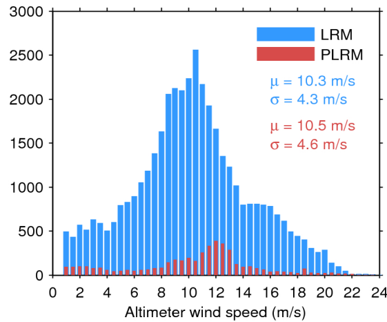
Figure 33. Histogram of flag-valid wind over oceans and lakes for LRM (blue) and PLRM (red) for 06/11/2015. The mean ( \mu ) and standard deviation ( \sigma ) are also shown. Note that values larger than 24 m/s are excluded from the histogram for the sake of readability but not from the computation of \mu and \sigma .
