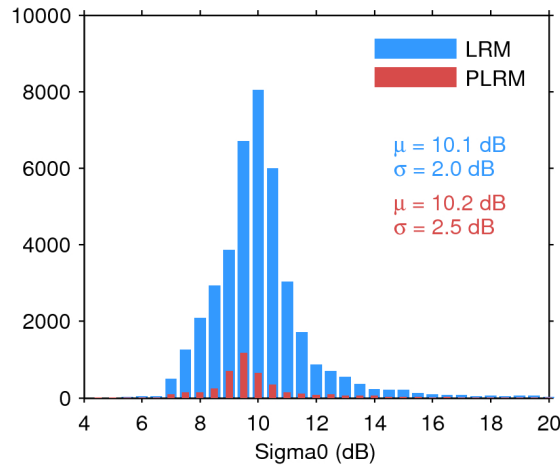
Figure 25. Histogram of flag-valid sigma0 over oceans and lakes for LRM (blue) and PLRM (red) for 06/11/2015. The mean ( \mu ) and standard deviation ( \sigma ) are also shown. Note that values outside [4 20] dB are excluded from the histogram for the sake of readability but not from the computation of \mu and \sigma .
