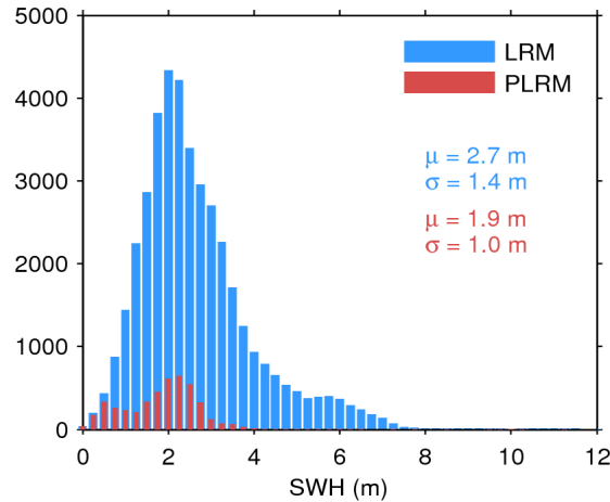
Figure 17. Histogram of flag-valid SWH over oceans and lakes for LRM (blue) and PLRM (red) for 05/11/2015. The mean ( \mu ) and standard deviation ( \sigma ) are also shown. Note that values larger than 12 m are excluded from the histogram for the sake of readability but not from the computation of \mu and \sigma .
