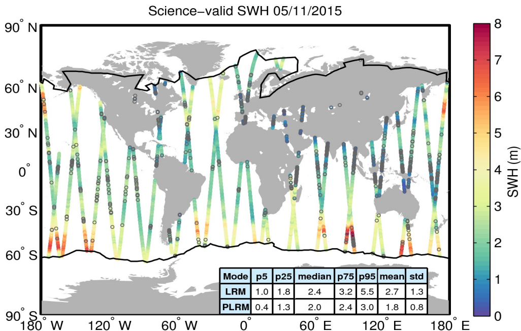
Figure 19. Geographical distribution of science-valid SWH data over oceans and lakes for 05/11/2015. The statistical values shown in the table refer to the SWH in m and are calculated separately for LRM and PLRM regions. The black lines mark the outer limit of the Arctic and Antarctic polar polygons. Gray circles denote records that have been rejected based on the editing criteria described in Table 3.
