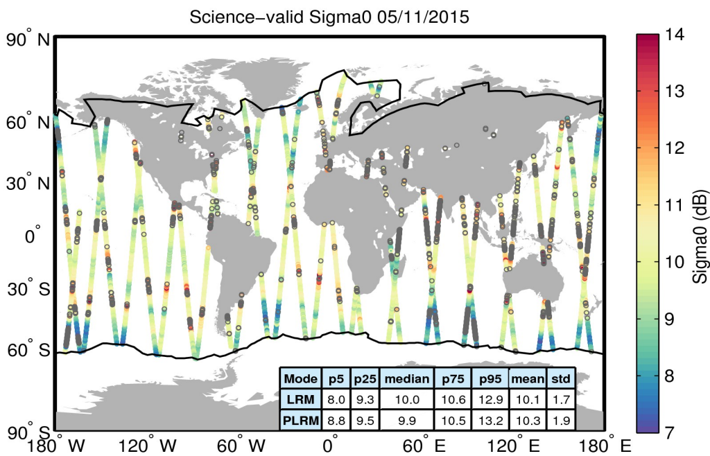
Figure 27. Geographical distribution of science-valid sigma0 data over oceans and lakes for 05/11/2015. The statistical values shown in the table refer to the sigma0 in dB and are calculated separately for LRM and PLRM regions. The black lines mark the outer limit of the Arctic and Antarctic polar polygons. Gray circles denote records that have been rejected based on the editing criteria described in Table 4.
