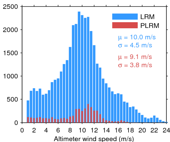
Figure 33. Histogram of flag-valid wind over oceans and lakes for LRM (blue) and PLRM (red) for 05/11/2015. The mean ( \mu ) and standard deviation ( \sigma ) are also shown. Note that values larger than 24 m/s are excluded from the histogram for the sake of readability but not from the computation of \mu and \sigma .
