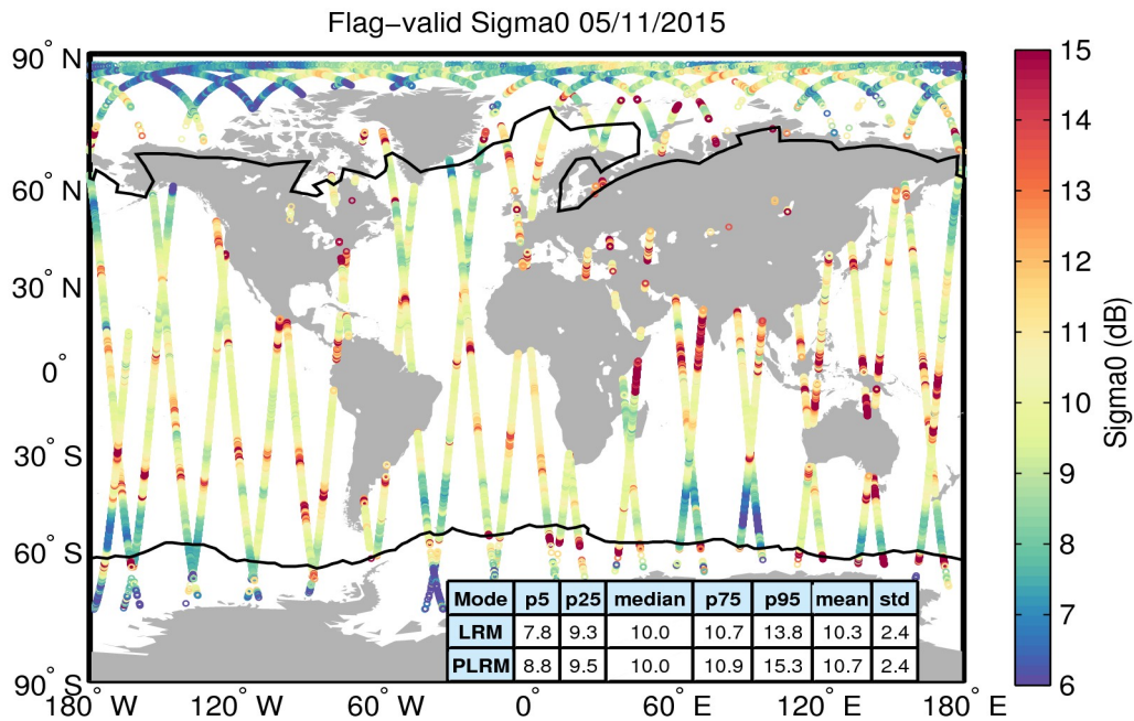
Figure 23. Geographical distribution of flag-valid sigma0 data over oceans and lakes for 05/11/2015. The statistical values shown in the table refer to the sigma0 in dB and are calculated separately for LRM and PLRM regions. Measurements taken over polar polygons have been excluded from the computation of the statistical values. The black lines mark the outer limit of the Arctic and Antarctic polar polygons.
