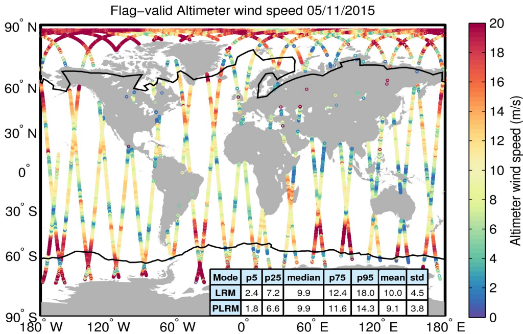
Figure 31. Geographical distribution of flag-valid wind data over oceans and lakes for 05/11/2015. The statistical values shown in the table refer to the wind in m/s and are calculated separately for LRM and PLRM regions. Measurements taken over polar polygons have been excluded from the computation of the statistical values. The black lines mark the outer limit of the Arctic and Antarctic polar polygons.
