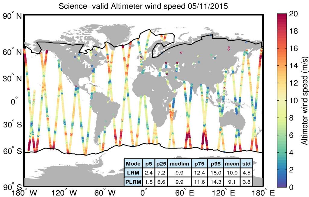
Figure 34. Geographical distribution of science-valid wind data over oceans and lakes for 05/11/2015. The statistical values shown in the table refer to the wind in m/s and are calculated separately for LRM and PLRM regions. The black lines mark the outer limit of the Arctic and Antarctic polar polygons. Gray circles denote records that have been rejected based on the editing criteria described in Table 5.
