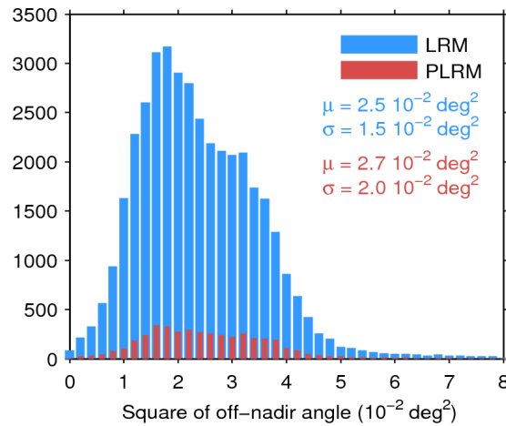
Figure 39. Histogram of flag-valid mispointing over oceans and lakes for LRM (blue) and PLRM (red) for 05/11/2015. Only positive values have been considered. The mean ( \mu ) and standard deviation ( \sigma ) are also shown. Note that values larger than 8 \cdot 10^{-2} \text{ deg}^2 are excluded from the histogram for the sake of readability but not from the computation of \mu and \sigma .
