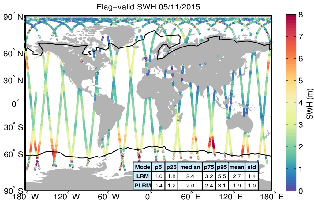
Figure 15. Geographical distribution of flag-valid SWH data over oceans and lakes for 05/11/2015. The statistical values shown in the table refer to the SWH in m and are calculated separately for LRM and PLRM regions. Measurements taken over polar polygons have been excluded from the computation of the statistical values. The black lines mark the outer limit of the Arctic and Antarctic polar polygons.
