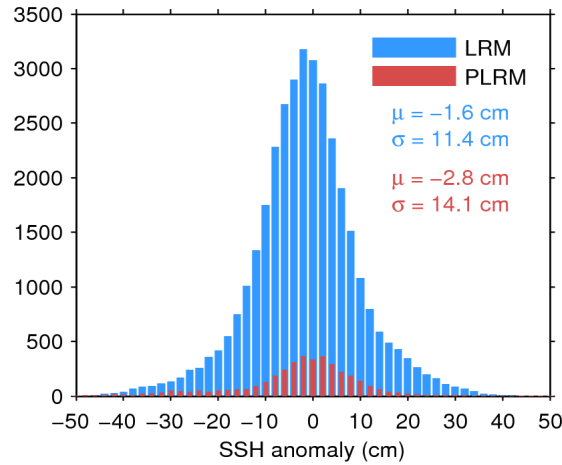
Figure 11. Histogram of science-valid SSH anomaly over oceans and lakes for LRM (blue) and PLRM (red) for 05/11/2015. The mean ( \mu ) and standard deviation ( \sigma ) are also shown. Note that values outside [-50 50] cm are excluded from the histogram for the sake of readability but not from the computation of \mu and \sigma .
