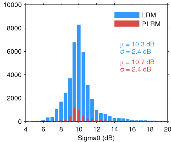
Figure 25. Histogram of flag-valid sigma0 over oceans and lakes for LRM (blue) and PLRM (red) for 05/11/2015. The mean ( \mu ) and standard deviation ( \sigma ) are also shown. Note that values outside [4 20] dB are excluded from the histogram for the sake of readability but not from the computation of \mu and \sigma .
