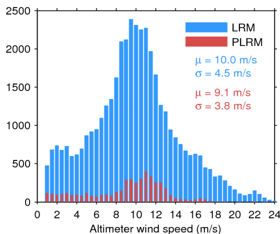
Figure 35. Histogram of science-valid wind over oceans and lakes for LRM (blue) and PLRM (red) for 05/11/2015. The mean ( \mu ) and standard deviation ( \sigma ) are also shown. Note that values larger than 24 m/s are excluded from the histogram for the sake of readability but not from the computation of \mu and \sigma .
