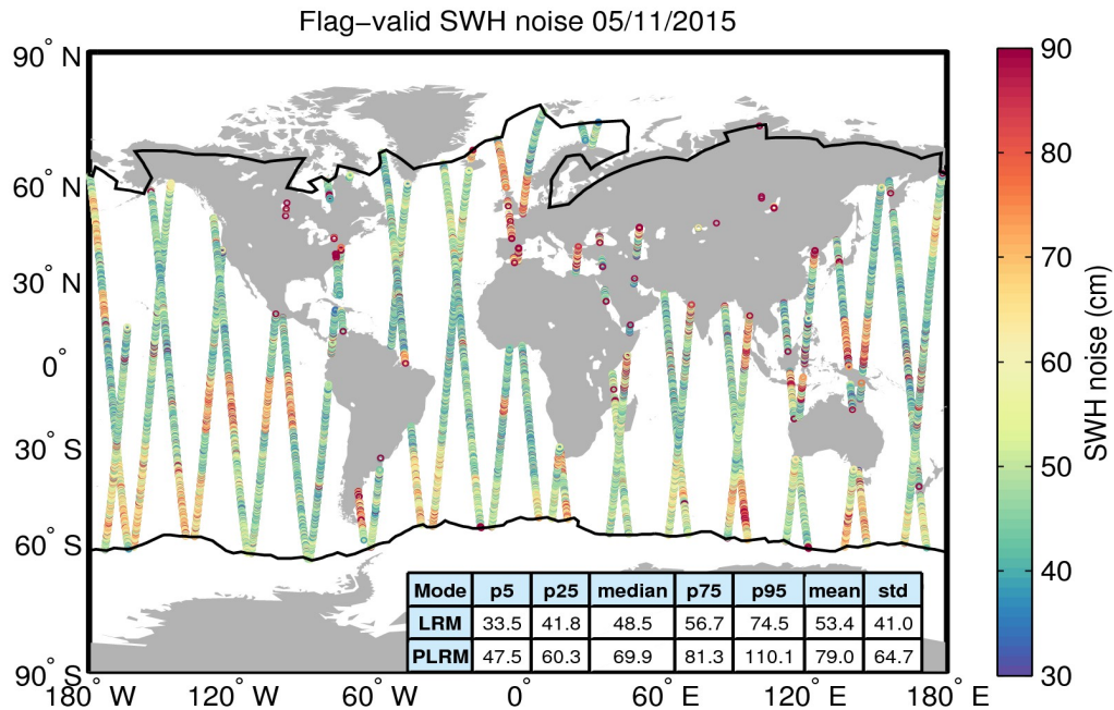
Figure 18. Geographical distribution of flag-valid 20-Hz SWH measurement noise over oceans and lakes for 05/11/2015. The statistical values shown in the table refer to the SWH noise and are calculated separately for LRM and PLRM regions. Measurements taken over polar polygons have been excluded from the computation of the statistical values. The black lines mark the outer limit of the Arctic and Antarctic polar polygons.
