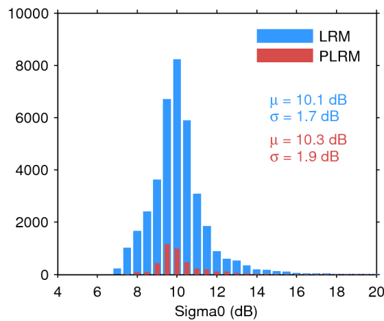
Figure 28. Histogram of science-valid sigma0 over oceans and lakes for LRM (blue) and PLRM (red) for 05/11/2015. The mean ( \mu ) and standard deviation ( \sigma ) are also shown. Note that values outside [4 20] dB are excluded from the histogram for the sake of readability but not from the computation of \mu and \sigma .
