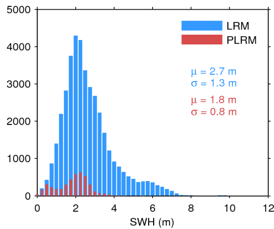
Figure 20. Histogram of science-valid SWH over oceans and lakes for LRM (blue) and PLRM (red) for 05/11/2015. The mean ( \mu ) and standard deviation ( \sigma ) are also shown. Note that values larger than 12 m are excluded from the histogram for the sake of readability but not from the computation of \mu and \sigma .
