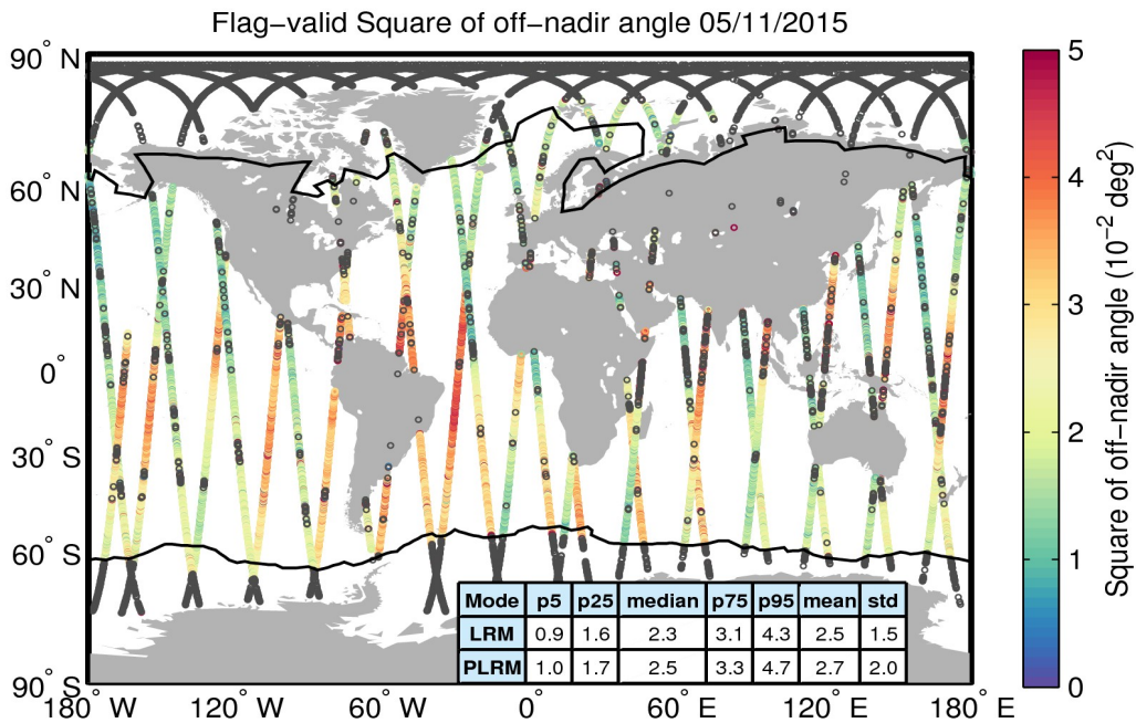
Figure 37. Geographical distribution of flag-valid mispointing data over oceans and lakes for 05/11/2015. The statistical values shown in the table refer to the mispointing in 10^{-2} deg 2 and are calculated separately for LRM and PLRM regions. Measurements taken over polar polygons have been excluded from the computation of the statistical values. The black lines mark the outer limit of the Arctic and Antarctic polar polygons. Gray circles denote negative values.
