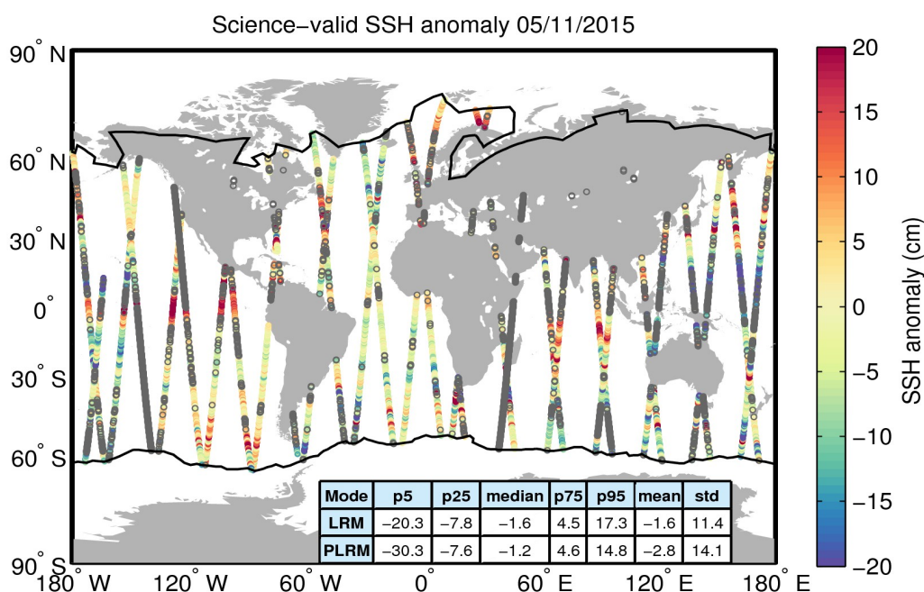
Figure 10. Geographical distribution of science-valid SSH anomaly data over oceans and lakes for 05/11/2015. The statistical values shown in the table refer to the SSH anomaly in cm and are calculated separately for LRM and PLRM regions. The black lines mark the outer limit of the Arctic and Antarctic polar polygons. Gray circles denote records that have been rejected based on the editing criteria described in Table 2.
