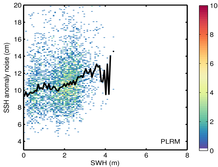
Figure 9. 2D histogram showing flag-valid SSH anomaly noise as a function of SWH for LRM (top) and PLRM (bottom) for 05/11/2015. The black line denotes the median SSH anomaly noise as a function of SWH.
