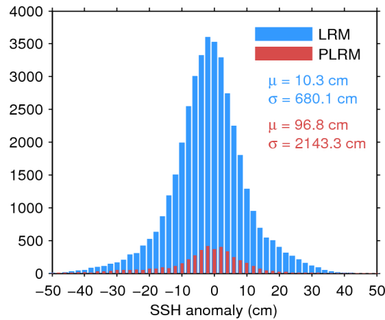
Figure 7. Histogram of flag-valid SSH anomaly over oceans and lakes for LRM (blue) and PLRM (red) for 05/11/2015. The mean ( \mu ) and standard deviation ( \sigma ) are also shown. Note that values outside [-50 50] cm are excluded from the histogram for the sake of readability but not from the computation of \mu and \sigma .
