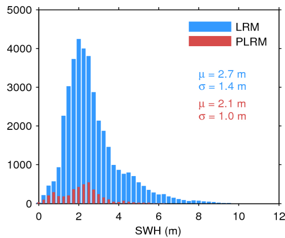
Figure 20. Histogram of science-valid SWH over oceans and lakes for LRM (blue) and PLRM (red) for 03/11/2015. The mean ( \mu ) and standard deviation ( \sigma ) are also shown. Note that values larger than 12 m are excluded from the histogram for the sake of readability but not from the computation of \mu and \sigma .
