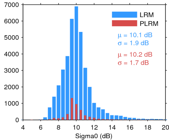
Figure 25. Histogram of flag-valid sigma0 over oceans and lakes for LRM (blue) and PLRM (red) for 03/11/2015. The mean ( \mu ) and standard deviation ( \sigma ) are also shown. Note that values outside [4 20] dB are excluded from the histogram for the sake of readability but not from the computation of \mu and \sigma .
