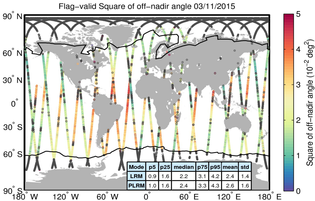
Figure 37. Geographical distribution of flag-valid mispointing data over oceans and lakes for 03/11/2015. The statistical values shown in the table refer to the mispointing in 10^{-2} deg 2 and are calculated separately for LRM and PLRM regions. Measurements taken over polar polygons have been excluded from the computation of the statistical values. The black lines mark the outer limit of the Arctic and Antarctic polar polygons. Gray circles denote negative values.
