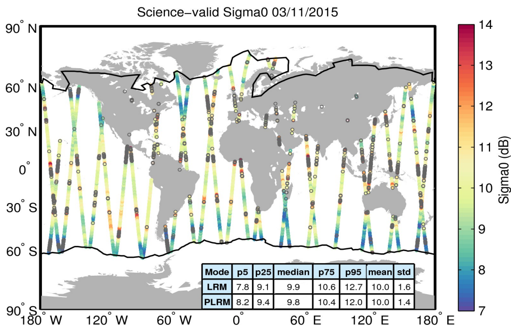
Figure 27. Geographical distribution of science-valid sigma0 data over oceans and lakes for 03/11/2015. The statistical values shown in the table refer to the sigma0 in dB and are calculated separately for LRM and PLRM regions. The black lines mark the outer limit of the Arctic and Antarctic polar polygons. Gray circles denote records that have been rejected based on the editing criteria described in Table 4.
