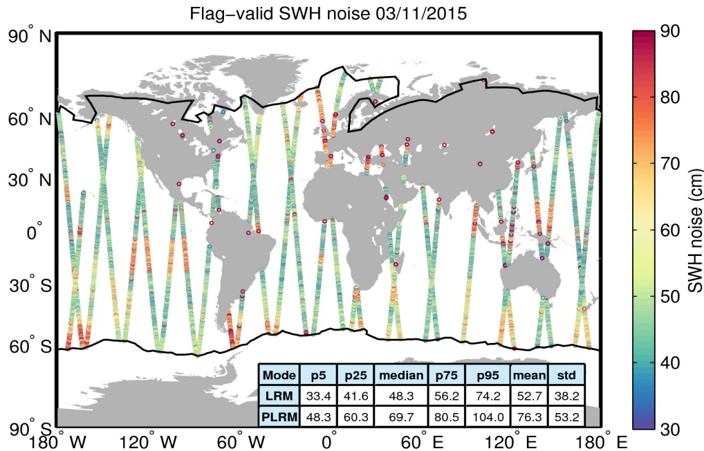
Figure 18. Geographical distribution of flag-valid 20-Hz SWH measurement noise over oceans and lakes for 03/11/2015. The statistical values shown in the table refer to the SWH noise and are calculated separately for LRM and PLRM regions. Measurements taken over polar polygons have been excluded from the computation of the statistical values. The black lines mark the outer limit of the Arctic and Antarctic polar polygons.
