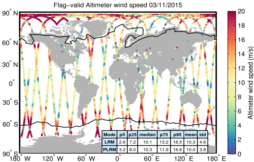
Figure 31. Geographical distribution of flag-valid wind data over oceans and lakes for 03/11/2015. The statistical values shown in the table refer to the wind in m/s and are calculated separately for LRM and PLRM regions. Measurements taken over polar polygons have been excluded from the computation of the statistical values. The black lines mark the outer limit of the Arctic and Antarctic polar polygons.
