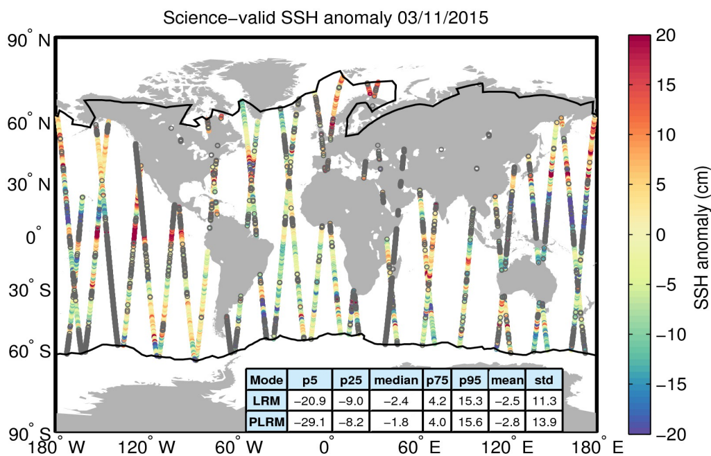
Figure 10. Geographical distribution of science-valid SSH anomaly data over oceans and lakes for 03/11/2015. The statistical values shown in the table refer to the SSH anomaly in cm and are calculated separately for LRM and PLRM regions. The black lines mark the outer limit of the Arctic and Antarctic polar polygons. Gray circles denote records that have been rejected based on the editing criteria described in Table 2.
