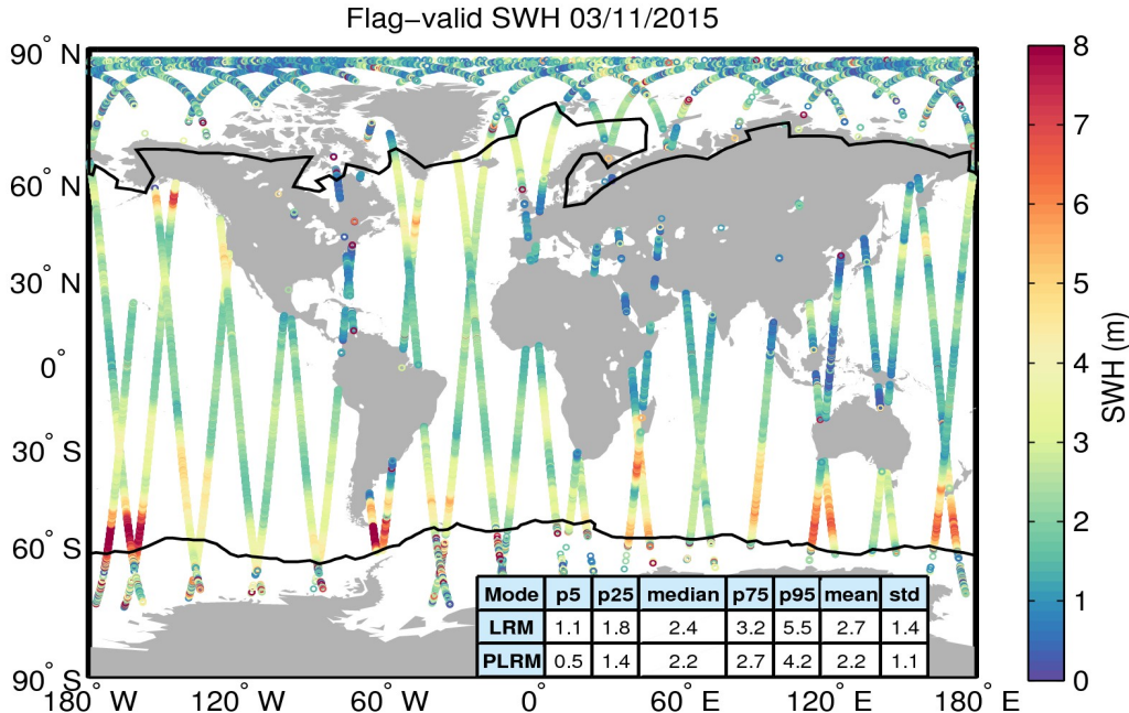
Figure 15. Geographical distribution of flag-valid SWH data over oceans and lakes for 03/11/2015. The statistical values shown in the table refer to the SWH in m and are calculated separately for LRM and PLRM regions. Measurements taken over polar polygons have been excluded from the computation of the statistical values. The black lines mark the outer limit of the Arctic and Antarctic polar polygons.
