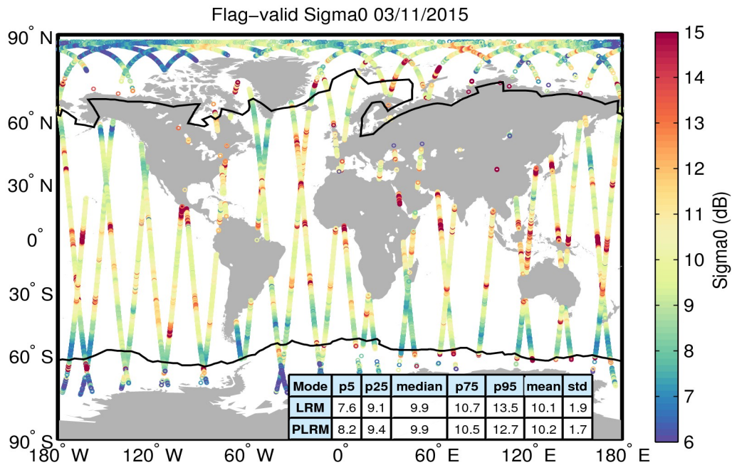
Figure 23. Geographical distribution of flag-valid sigma0 data over oceans and lakes for 03/11/2015. The statistical values shown in the table refer to the sigma0 in dB and are calculated separately for LRM and PLRM regions. Measurements taken over polar polygons have been excluded from the computation of the statistical values. The black lines mark the outer limit of the Arctic and Antarctic polar polygons.
