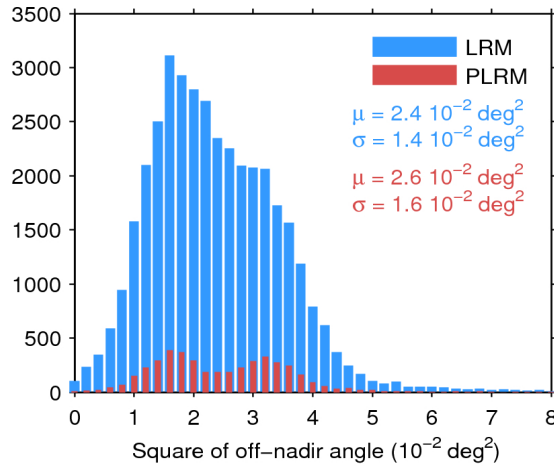
Figure 39. Histogram of flag-valid mispointing over oceans and lakes for LRM (blue) and PLRM (red) for 03/11/2015. Only positive values have been considered. The mean ( \mu ) and standard deviation ( \sigma ) are also shown. Note that values larger than 8 \cdot 10^{-2} \text{ deg}^2 are excluded from the histogram for the sake of readability but not from the computation of \mu and \sigma .
