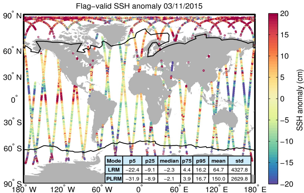
Figure 5. Geographical distribution of flag-valid 1-Hz SSH anomaly data over oceans and lakes for 03/11/2015. The statistical values shown in the table refer to the SSH anomaly in cm and are calculated separately for LRM and PLRM regions. Measurements taken over polar polygons have been excluded from the computation of the statistical values. The black lines mark the outer limit of the Arctic and Antarctic polar polygons.
