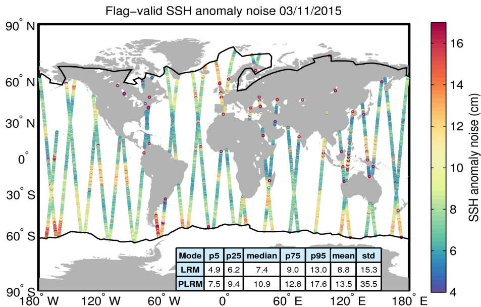
Figure 8. Geographical distribution of flag-valid 20-Hz SSH anomaly measurement noise over oceans and lakes for 03/11/2015. The statistical values shown in the table refer to the SSH anomaly noise and are calculated separately for LRM and PLRM regions. Measurements taken over polar polygons have been excluded from the computation of the statistical values. The black lines mark the outer limit of the Arctic and Antarctic polar polygons.
