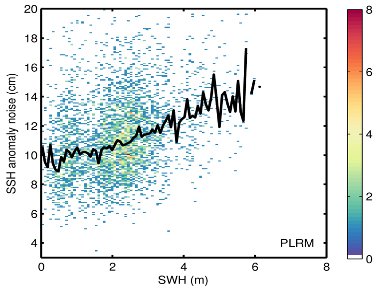
Figure 9. 2D histogram showing flag-valid SSH anomaly noise as a function of SWH for LRM (top) and PLRM (bottom) for 03/11/2015. The black line denotes the median SSH anomaly noise as a function of SWH.
