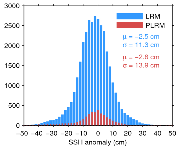
Figure 11. Histogram of science-valid SSH anomaly over oceans and lakes for LRM (blue) and PLRM (red) for 03/11/2015. The mean ( \mu ) and standard deviation ( \sigma ) are also shown. Note that values outside [-50\ 50] cm are excluded from the histogram for the sake of readability but not from the computation of \mu and \sigma .
