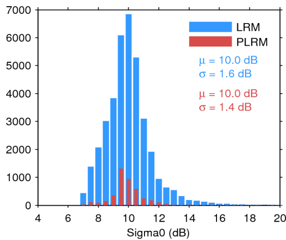
Figure 28. Histogram of science-valid sigma0 over oceans and lakes for LRM (blue) and PLRM (red) for 03/11/2015. The mean ( \mu ) and standard deviation ( \sigma ) are also shown. Note that values outside [4 20] dB are excluded from the histogram for the sake of readability but not from the computation of \mu and \sigma .
