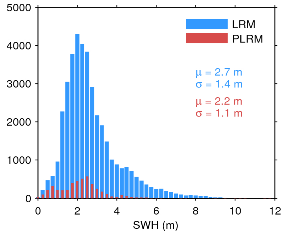
Figure 17. Histogram of flag-valid SWH over oceans and lakes for LRM (blue) and PLRM (red) for 03/11/2015. The mean ( \mu ) and standard deviation ( \sigma ) are also shown. Note that values larger than 12 m are excluded from the histogram for the sake of readability but not from the computation of \mu and \sigma .
