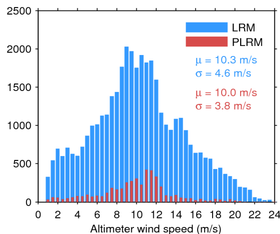
Figure 35. Histogram of science-valid wind over oceans and lakes for LRM (blue) and PLRM (red) for 03/11/2015. The mean ( \mu ) and standard deviation ( \sigma ) are also shown. Note that values larger than 24 m/s are excluded from the histogram for the sake of readability but not from the computation of \mu and \sigma .
