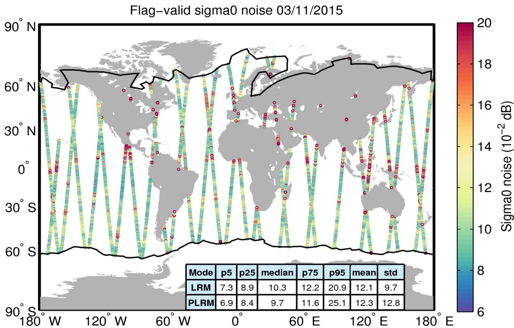
Figure 26. Geographical distribution of flag-valid 20-Hz sigma0 measurement noise over oceans and lakes for 03/11/2015. The statistical values shown in the table refer to the sigma0 noise and are calculated separately for LRM and PLRM regions. Measurements taken over polar polygons have been excluded from the computation of the statistical values. The black lines mark the outer limit of the Arctic and Antarctic polar polygons.
