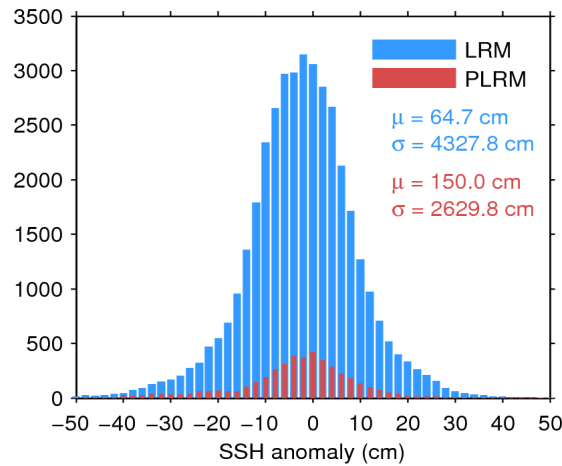
Figure 7. Histogram of flag-valid SSH anomaly over oceans and lakes for LRM (blue) and PLRM (red) for 03/11/2015. The mean ( \mu ) and standard deviation ( \sigma ) are also shown. Note that values outside [-50\ 50] cm are excluded from the histogram for the sake of readability but not from the computation of \mu and \sigma .
