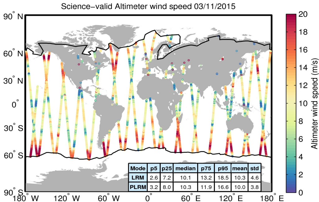
Figure 34. Geographical distribution of science-valid wind data over oceans and lakes for 03/11/2015. The statistical values shown in the table refer to the wind in m/s and are calculated separately for LRM and PLRM regions. The black lines mark the outer limit of the Arctic and Antarctic polar polygons. Gray circles denote records that have been rejected based on the editing criteria described in Table 5.
