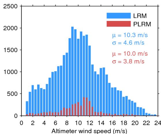
Figure 33. Histogram of flag-valid wind over oceans and lakes for LRM (blue) and PLRM (red) for 03/11/2015. The mean ( \mu ) and standard deviation ( \sigma ) are also shown. Note that values larger than 24 m/s are excluded from the histogram for the sake of readability but not from the computation of \mu and \sigma .
