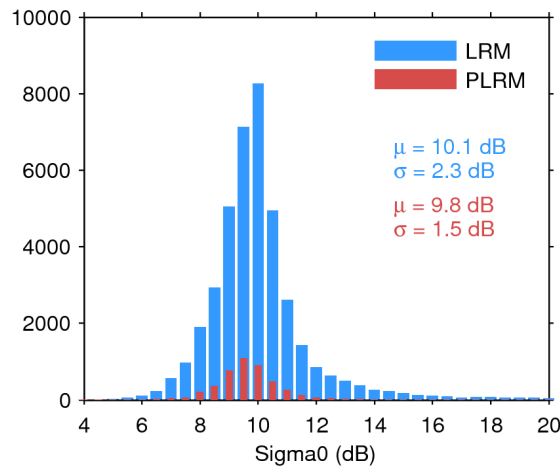
Figure 25. Histogram of flag-valid sigma0 over oceans and lakes for LRM (blue) and PLRM (red) for 02/11/2015. The mean ( \mu ) and standard deviation ( \sigma ) are also shown. Note that values outside [4 20] dB are excluded from the histogram for the sake of readability but not from the computation of \mu and \sigma .
