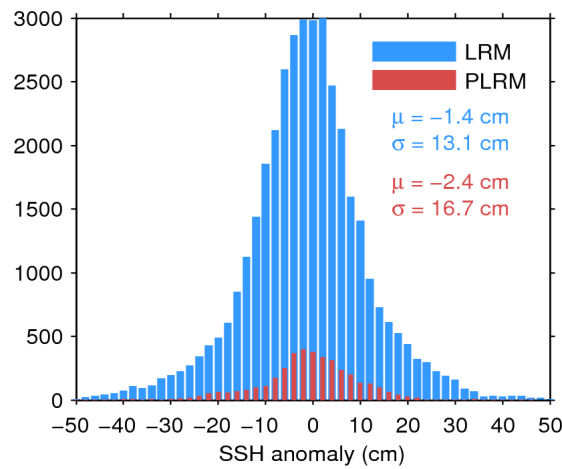
Figure 11. Histogram of science-valid SSH anomaly over oceans and lakes for LRM (blue) and PLRM (red) for 02/11/2015. The mean ( \mu ) and standard deviation ( \sigma ) are also shown. Note that values outside [-50 50] cm are excluded from the histogram for the sake of readability but not from the computation of \mu and \sigma .
