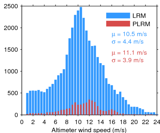
Figure 35. Histogram of science-valid wind over oceans and lakes for LRM (blue) and PLRM (red) for 02/11/2015. The mean ( \mu ) and standard deviation ( \sigma ) are also shown. Note that values larger than 24 m/s are excluded from the histogram for the sake of readability but not from the computation of \mu and \sigma .
