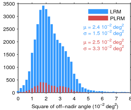
Figure 39. Histogram of flag-valid mispointing over oceans and lakes for LRM (blue) and PLRM (red) for 02/11/2015. Only positive values have been considered. The mean ( \mu ) and standard deviation ( \sigma ) are also shown. Note that values larger than 8 \cdot 10^{-2} \text{ deg}^2 are excluded from the histogram for the sake of readability but not from the computation of \mu and \sigma .
