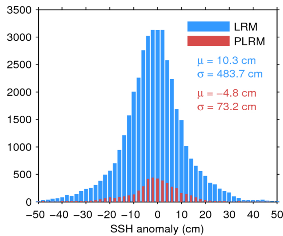
Figure 7. Histogram of flag-valid SSH anomaly over oceans and lakes for LRM (blue) and PLRM (red) for 02/11/2015. The mean ( \mu ) and standard deviation ( \sigma ) are also shown. Note that values outside [-50 50] cm are excluded from the histogram for the sake of readability but not from the computation of \mu and \sigma .
