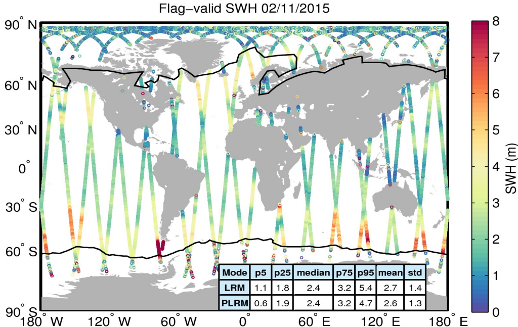
Figure 15. Geographical distribution of flag-valid SWH data over oceans and lakes for 02/11/2015. The statistical values shown in the table refer to the SWH in m and are calculated separately for LRM and PLRM regions. Measurements taken over polar polygons have been excluded from the computation of the statistical values. The black lines mark the outer limit of the Arctic and Antarctic polar polygons.
