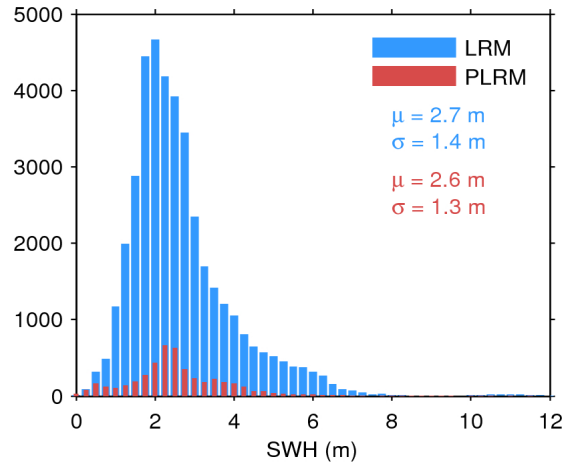
Figure 17. Histogram of flag-valid SWH over oceans and lakes for LRM (blue) and PLRM (red) for 02/11/2015. The mean ( \mu ) and standard deviation ( \sigma ) are also shown. Note that values larger than 12 m are excluded from the histogram for the sake of readability but not from the computation of \mu and \sigma .
