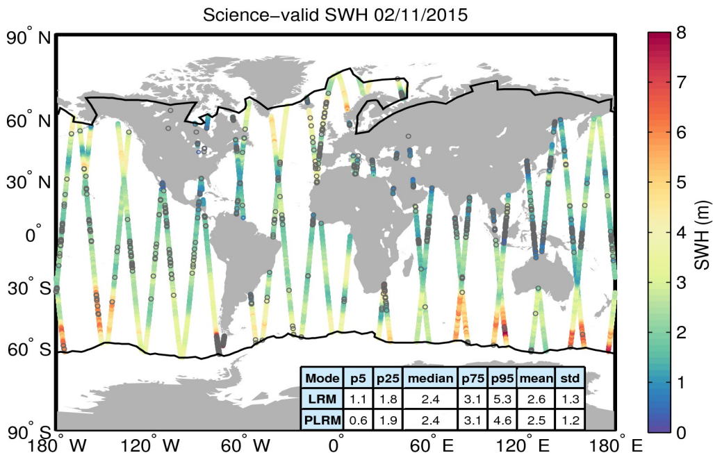
Figure 19. Geographical distribution of science-valid SWH data over oceans and lakes for 02/11/2015. The statistical values shown in the table refer to the SWH in m and are calculated separately for LRM and PLRM regions. The black lines mark the outer limit of the Arctic and Antarctic polar polygons. Gray circles denote records that have been rejected based on the editing criteria described in Table 3.
