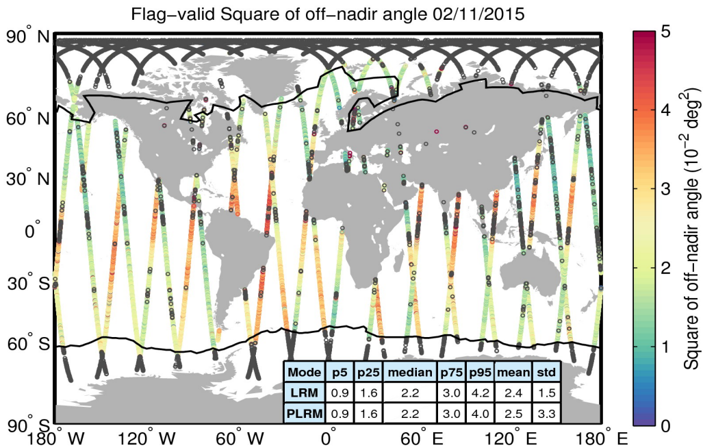
Figure 37. Geographical distribution of flag-valid mispointing data over oceans and lakes for 02/11/2015. The statistical values shown in the table refer to the mispointing in 10^{-2} deg 2 and are calculated separately for LRM and PLRM regions. Measurements taken over polar polygons have been excluded from the computation of the statistical values. The black lines mark the outer limit of the Arctic and Antarctic polar polygons. Gray circles denote negative values.
