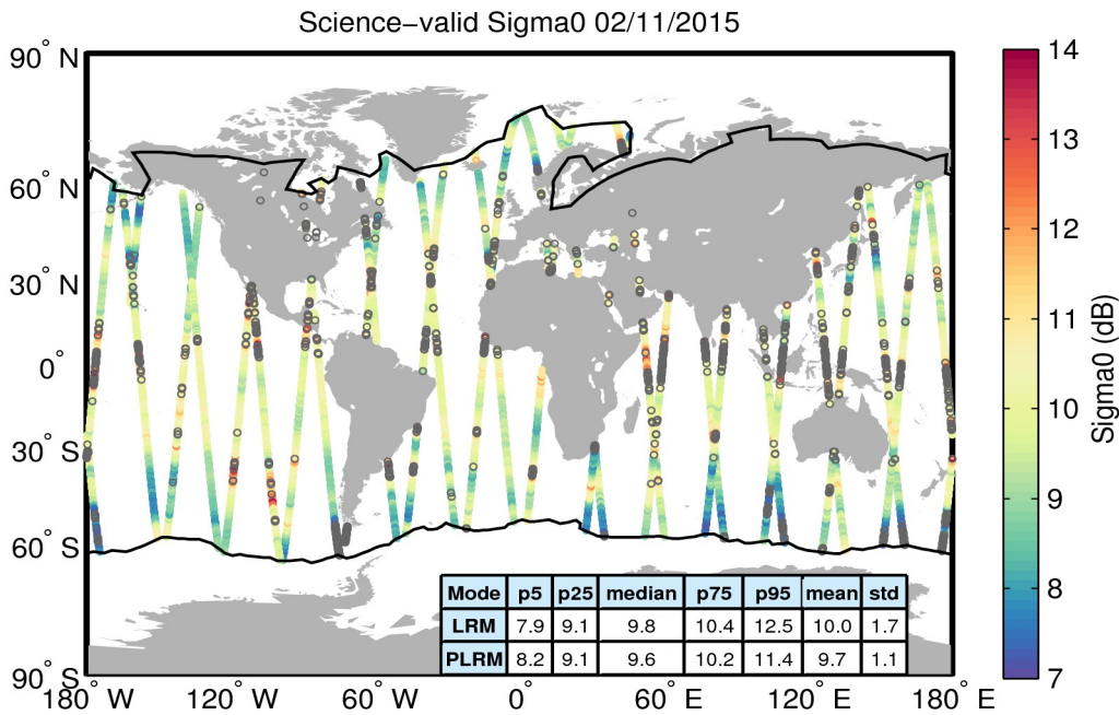
Figure 27. Geographical distribution of science-valid sigma0 data over oceans and lakes for 02/11/2015. The statistical values shown in the table refer to the sigma0 in dB and are calculated separately for LRM and PLRM regions. The black lines mark the outer limit of the Arctic and Antarctic polar polygons. Gray circles denote records that have been rejected based on the editing criteria described in Table 4.
