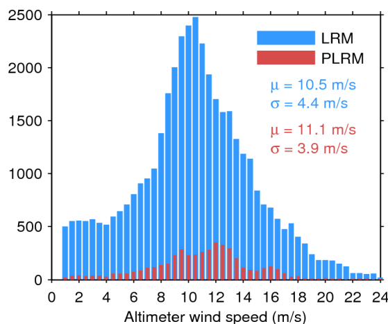
Figure 33. Histogram of flag-valid wind over oceans and lakes for LRM (blue) and PLRM (red) for 02/11/2015. The mean ( \mu ) and standard deviation ( \sigma ) are also shown. Note that values larger than 24 m/s are excluded from the histogram for the sake of readability but not from the computation of \mu and \sigma .
