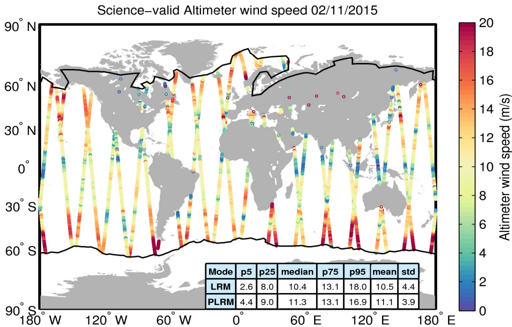
Figure 34. Geographical distribution of science-valid wind data over oceans and lakes for 02/11/2015. The statistical values shown in the table refer to the wind in m/s and are calculated separately for LRM and PLRM regions. The black lines mark the outer limit of the Arctic and Antarctic polar polygons. Gray circles denote records that have been rejected based on the editing criteria described in Table 5.
