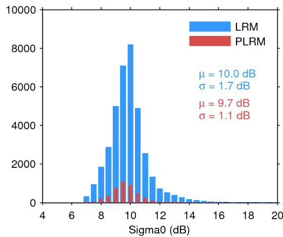
Figure 28. Histogram of science-valid sigma0 over oceans and lakes for LRM (blue) and PLRM (red) for 02/11/2015. The mean ( \mu ) and standard deviation ( \sigma ) are also shown. Note that values outside [4 20] dB are excluded from the histogram for the sake of readability but not from the computation of \mu and \sigma .
