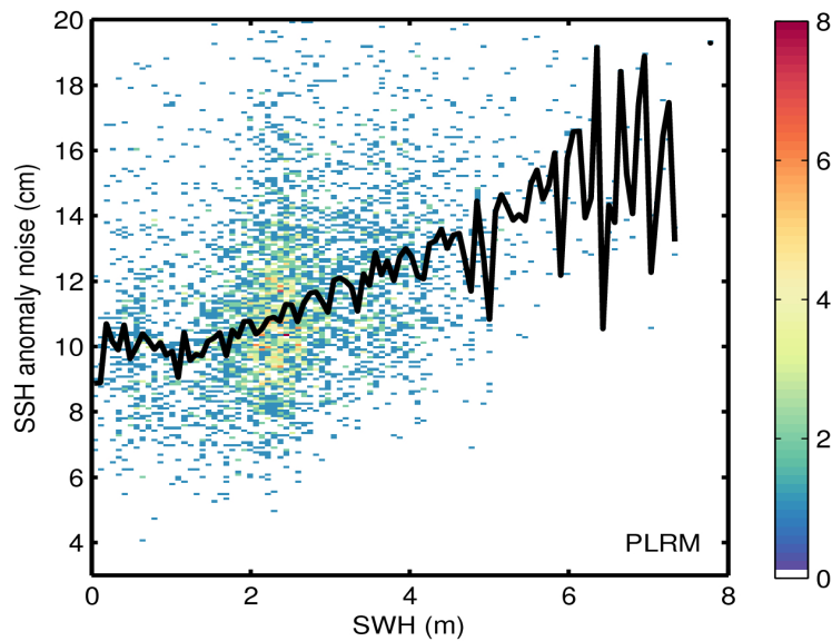
Figure 9. 2D histogram showing flag-valid SSH anomaly noise as a function of SWH for LRM (top) and PLRM (bottom) for 02/11/2015. The black line denotes the median SSH anomaly noise as a function of SWH.
