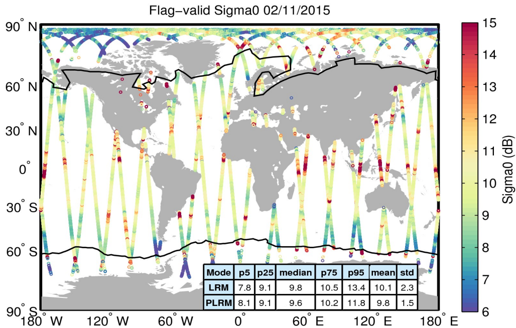
Figure 23. Geographical distribution of flag-valid sigma0 data over oceans and lakes for 02/11/2015. The statistical values shown in the table refer to the sigma0 in dB and are calculated separately for LRM and PLRM regions. Measurements taken over polar polygons have been excluded from the computation of the statistical values. The black lines mark the outer limit of the Arctic and Antarctic polar polygons.
