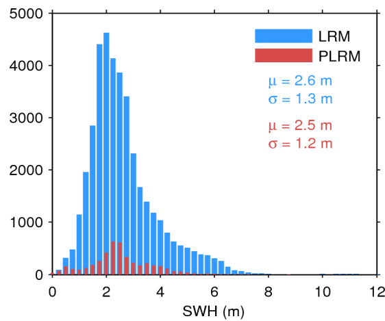
Figure 20. Histogram of science-valid SWH over oceans and lakes for LRM (blue) and PLRM (red) for 02/11/2015. The mean ( \mu ) and standard deviation ( \sigma ) are also shown. Note that values larger than 12 m are excluded from the histogram for the sake of readability but not from the computation of \mu and \sigma .
