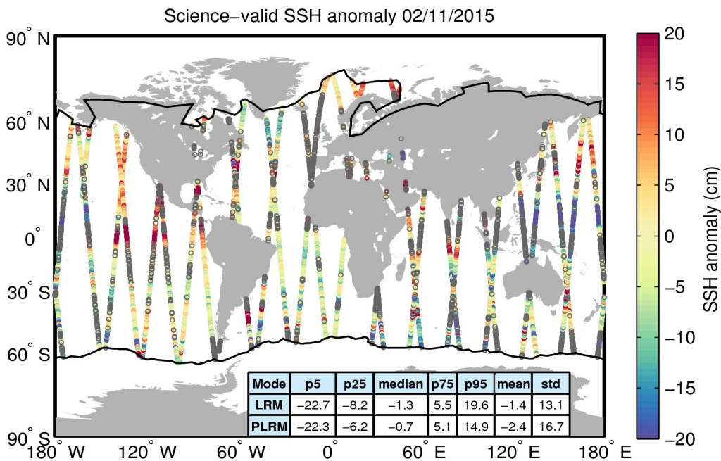
Figure 10. Geographical distribution of science-valid SSH anomaly data over oceans and lakes for 02/11/2015. The statistical values shown in the table refer to the SSH anomaly in cm and are calculated separately for LRM and PLRM regions. The black lines mark the outer limit of the Arctic and Antarctic polar polygons. Gray circles denote records that have been rejected based on the editing criteria described in Table 2.
