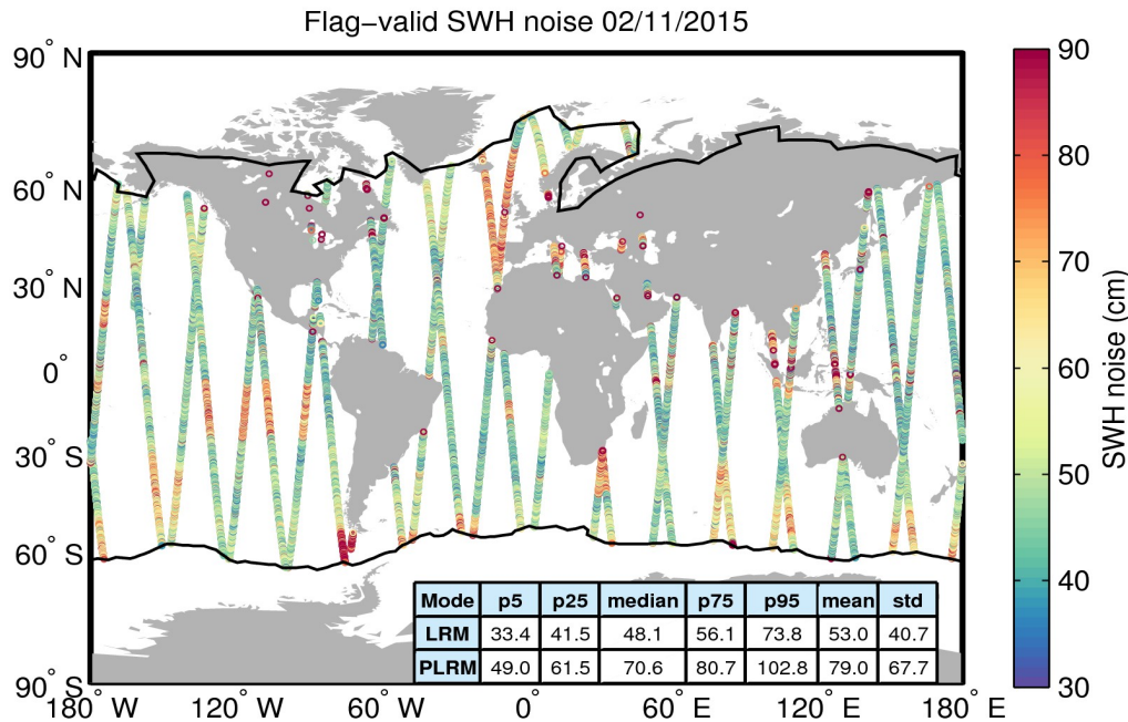
Figure 18. Geographical distribution of flag-valid 20-Hz SWH measurement noise over oceans and lakes for 02/11/2015. The statistical values shown in the table refer to the SWH noise and are calculated separately for LRM and PLRM regions. Measurements taken over polar polygons have been excluded from the computation of the statistical values. The black lines mark the outer limit of the Arctic and Antarctic polar polygons.
