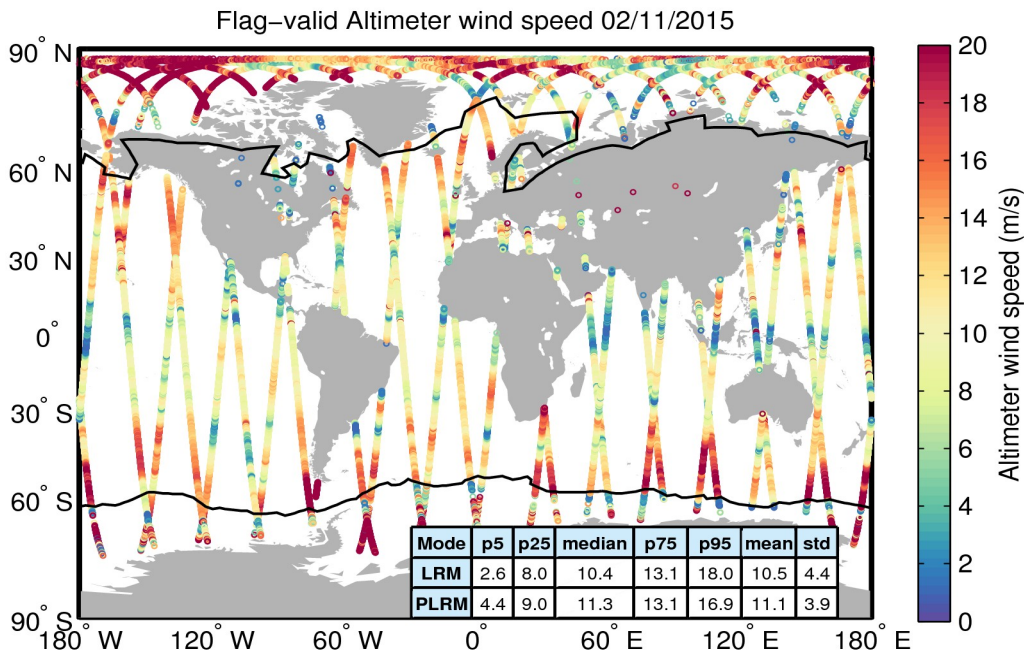
Figure 31. Geographical distribution of flag-valid wind data over oceans and lakes for 02/11/2015. The statistical values shown in the table refer to the wind in m/s and are calculated separately for LRM and PLRM regions. Measurements taken over polar polygons have been excluded from the computation of the statistical values. The black lines mark the outer limit of the Arctic and Antarctic polar polygons.
