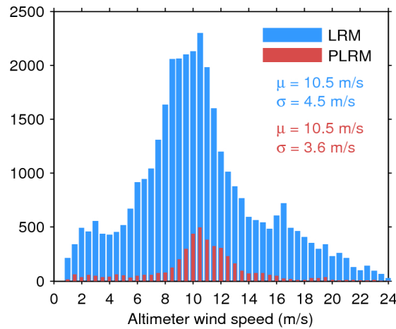
Figure 33. Histogram of flag-valid wind over oceans and lakes for LRM (blue) and PLRM (red) for 31/10/2015. The mean ( \mu ) and standard deviation ( \sigma ) are also shown. Note that values larger than 24 m/s are excluded from the histogram for the sake of readability but not from the computation of \mu and \sigma .
