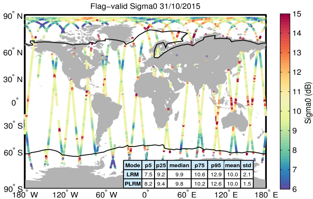
Figure 23. Geographical distribution of flag-valid sigma0 data over oceans and lakes for 31/10/2015. The statistical values shown in the table refer to the sigma0 in dB and are calculated separately for LRM and PLRM regions. Measurements taken over polar polygons have been excluded from the computation of the statistical values. The black lines mark the outer limit of the Arctic and Antarctic polar polygons.
