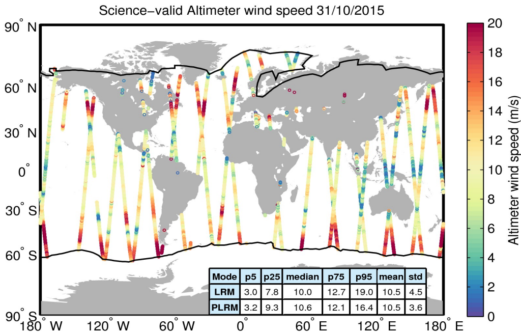
Figure 34. Geographical distribution of science-valid wind data over oceans and lakes for 31/10/2015. The statistical values shown in the table refer to the wind in m/s and are calculated separately for LRM and PLRM regions. The black lines mark the outer limit of the Arctic and Antarctic polar polygons. Gray circles denote records that have been rejected based on the editing criteria described in Table 5.
