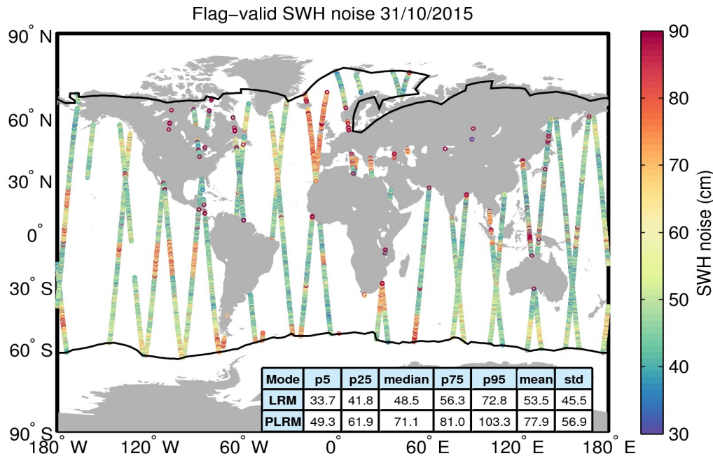
Figure 18. Geographical distribution of flag-valid 20-Hz SWH measurement noise over oceans and lakes for 31/10/2015. The statistical values shown in the table refer to the SWH noise and are calculated separately for LRM and PLRM regions. Measurements taken over polar polygons have been excluded from the computation of the statistical values. The black lines mark the outer limit of the Arctic and Antarctic polar polygons.
