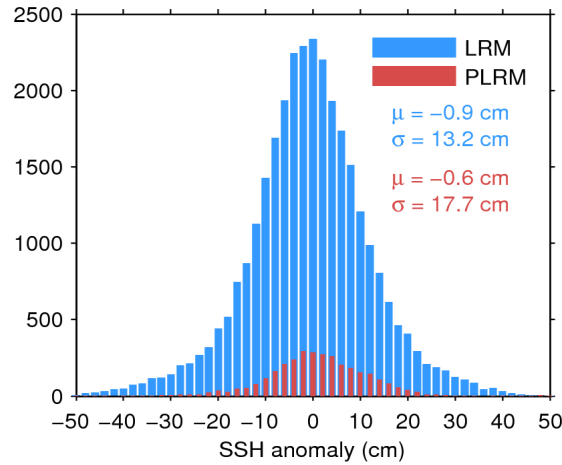
Figure 11. Histogram of science-valid SSH anomaly over oceans and lakes for LRM (blue) and PLRM (red) for 31/10/2015. The mean ( \mu ) and standard deviation ( \sigma ) are also shown. Note that values outside [-50\ 50] cm are excluded from the histogram for the sake of readability but not from the computation of \mu and \sigma .
