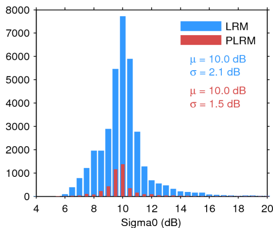
Figure 25. Histogram of flag-valid sigma0 over oceans and lakes for LRM (blue) and PLRM (red) for 31/10/2015. The mean ( \mu ) and standard deviation ( \sigma ) are also shown. Note that values outside [4 20] dB are excluded from the histogram for the sake of readability but not from the computation of \mu and \sigma .
