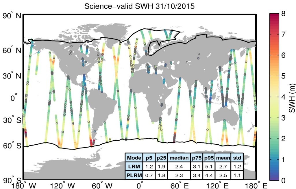
Figure 19. Geographical distribution of science-valid SWH data over oceans and lakes for 31/10/2015. The statistical values shown in the table refer to the SWH in m and are calculated separately for LRM and PLRM regions. The black lines mark the outer limit of the Arctic and Antarctic polar polygons. Gray circles denote records that have been rejected based on the editing criteria described in Table 3.
