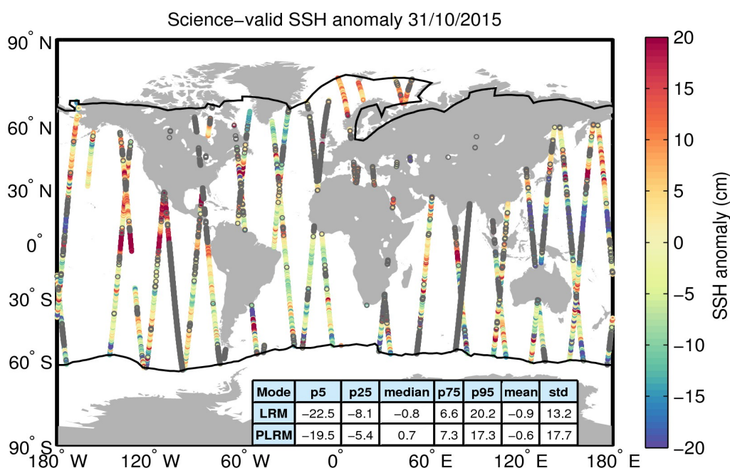
Figure 10. Geographical distribution of science-valid SSH anomaly data over oceans and lakes for 31/10/2015. The statistical values shown in the table refer to the SSH anomaly in cm and are calculated separately for LRM and PLRM regions. The black lines mark the outer limit of the Arctic and Antarctic polar polygons. Gray circles denote records that have been rejected based on the editing criteria described in Table 2.
