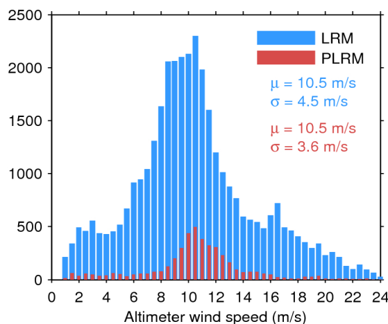
Figure 35. Histogram of science-valid wind over oceans and lakes for LRM (blue) and PLRM (red) for 31/10/2015. The mean ( \mu ) and standard deviation ( \sigma ) are also shown. Note that values larger than 24 m/s are excluded from the histogram for the sake of readability but not from the computation of \mu and \sigma .
