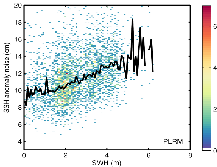
Figure 9. 2D histogram showing flag-valid SSH anomaly noise as a function of SWH for LRM (top) and PLRM (bottom) for 31/10/2015. The black line denotes the median SSH anomaly noise as a function of SWH.
