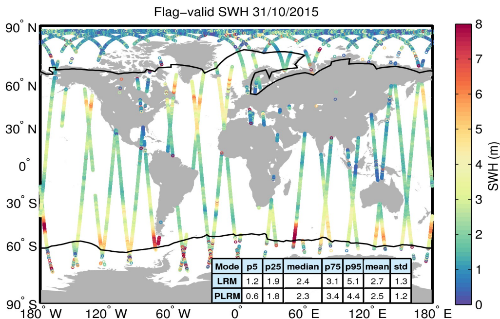
Figure 15. Geographical distribution of flag-valid SWH data over oceans and lakes for 31/10/2015. The statistical values shown in the table refer to the SWH in m and are calculated separately for LRM and PLRM regions. Measurements taken over polar polygons have been excluded from the computation of the statistical values. The black lines mark the outer limit of the Arctic and Antarctic polar polygons.
