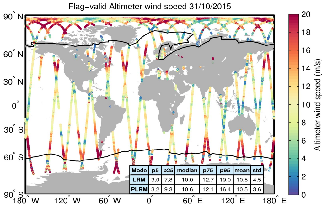
Figure 31. Geographical distribution of flag-valid wind data over oceans and lakes for 31/10/2015. The statistical values shown in the table refer to the wind in m/s and are calculated separately for LRM and PLRM regions. Measurements taken over polar polygons have been excluded from the computation of the statistical values. The black lines mark the outer limit of the Arctic and Antarctic polar polygons.
