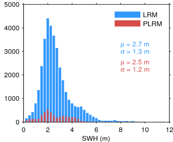
Figure 17. Histogram of flag-valid SWH over oceans and lakes for LRM (blue) and PLRM (red) for 31/10/2015. The mean ( \mu ) and standard deviation ( \sigma ) are also shown. Note that values larger than 12 m are excluded from the histogram for the sake of readability but not from the computation of \mu and \sigma .
