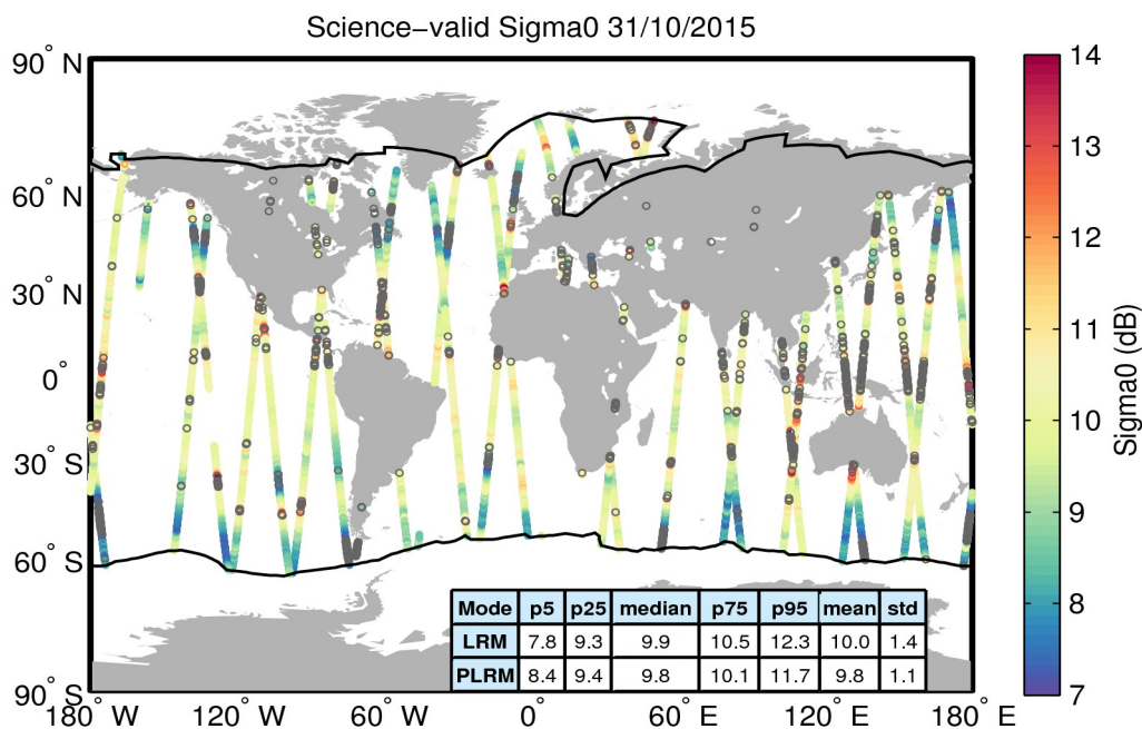
Figure 27. Geographical distribution of science-valid sigma0 data over oceans and lakes for 31/10/2015. The statistical values shown in the table refer to the sigma0 in dB and are calculated separately for LRM and PLRM regions. The black lines mark the outer limit of the Arctic and Antarctic polar polygons. Gray circles denote records that have been rejected based on the editing criteria described in Table 4.
