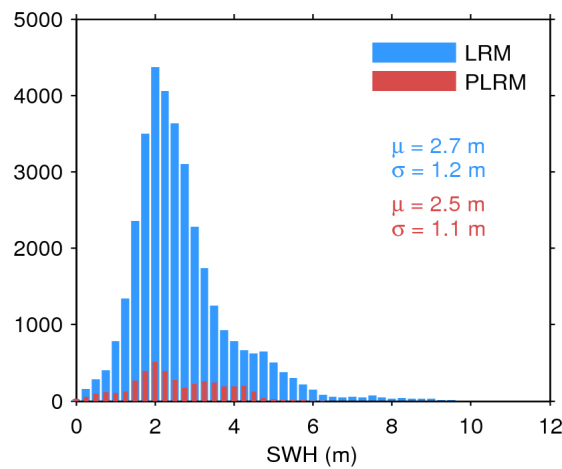
Figure 20. Histogram of science-valid SWH over oceans and lakes for LRM (blue) and PLRM (red) for 31/10/2015. The mean ( \mu ) and standard deviation ( \sigma ) are also shown. Note that values larger than 12 m are excluded from the histogram for the sake of readability but not from the computation of \mu and \sigma .
