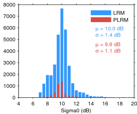
Figure 28. Histogram of science-valid sigma0 over oceans and lakes for LRM (blue) and PLRM (red) for 31/10/2015. The mean ( \mu ) and standard deviation ( \sigma ) are also shown. Note that values outside [4 20] dB are excluded from the histogram for the sake of readability but not from the computation of \mu and \sigma .
