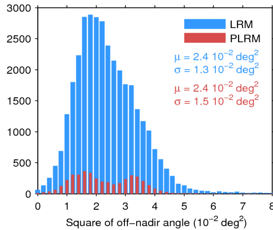
Figure 39. Histogram of flag-valid mispointing over oceans and lakes for LRM (blue) and PLRM (red) for 31/10/2015. Only positive values have been considered. The mean ( \mu ) and standard deviation ( \sigma ) are also shown. Note that values larger than 8 \cdot 10^{-2} \text{ deg}^2 are excluded from the histogram for the sake of readability but not from the computation of \mu and \sigma .
