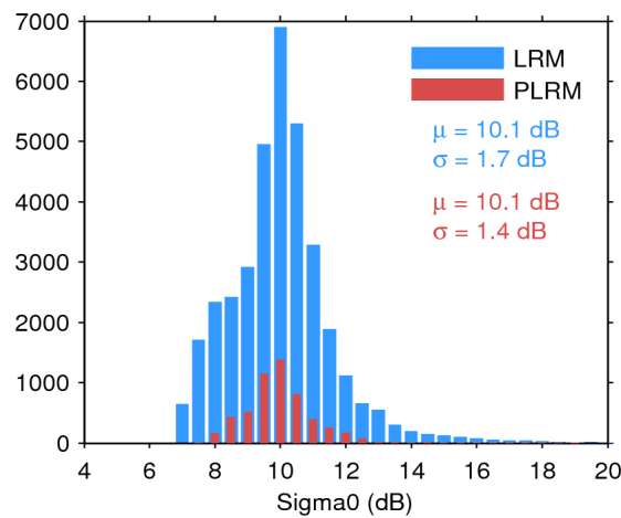
Figure 28. Histogram of science-valid sigma0 over oceans and lakes for LRM (blue) and PLRM (red) for 25/10/2015. The mean ( \mu ) and standard deviation ( \sigma ) are also shown. Note that values outside [4 20] dB are excluded from the histogram for the sake of readability but not from the computation of \mu and \sigma .
