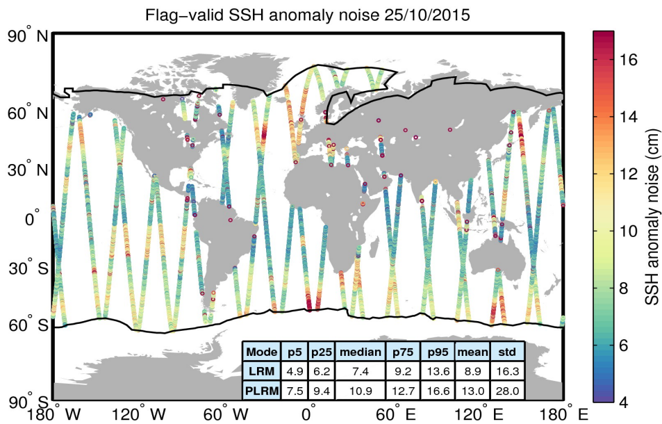
Figure 8. Geographical distribution of flag-valid 20-Hz SSH anomaly measurement noise over oceans and lakes for 25/10/2015. The statistical values shown in the table refer to the SSH anomaly noise and are calculated separately for LRM and PLRM regions. Measurements taken over polar polygons have been excluded from the computation of the statistical values. The black lines mark the outer limit of the Arctic and Antarctic polar polygons.
