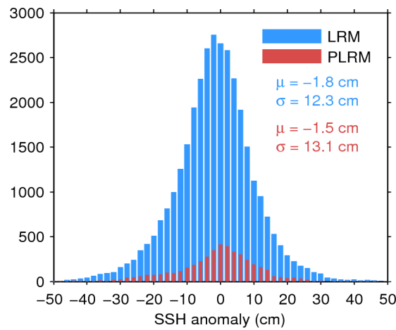
Figure 11. Histogram of science-valid SSH anomaly over oceans and lakes for LRM (blue) and PLRM (red) for 25/10/2015. The mean ( \mu ) and standard deviation ( \sigma ) are also shown. Note that values outside [-50 50] cm are excluded from the histogram for the sake of readability but not from the computation of \mu and \sigma .
