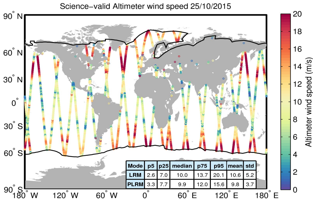
Figure 34. Geographical distribution of science-valid wind data over oceans and lakes for 25/10/2015. The statistical values shown in the table refer to the wind in m/s and are calculated separately for LRM and PLRM regions. The black lines mark the outer limit of the Arctic and Antarctic polar polygons. Gray circles denote records that have been rejected based on the editing criteria described in Table 5.
