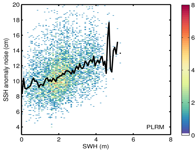
Figure 9. 2D histogram showing flag-valid SSH anomaly noise as a function of SWH for LRM (top) and PLRM (bottom) for 25/10/2015. The black line denotes the median SSH anomaly noise as a function of SWH.
