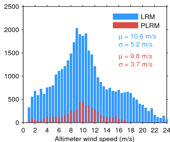
Figure 35. Histogram of science-valid wind over oceans and lakes for LRM (blue) and PLRM (red) for 25/10/2015. The mean ( \mu ) and standard deviation ( \sigma ) are also shown. Note that values larger than 24 m/s are excluded from the histogram for the sake of readability but not from the computation of \mu and \sigma .
