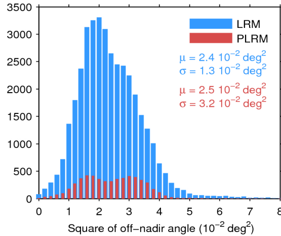
Figure 39. Histogram of flag-valid mispointing over oceans and lakes for LRM (blue) and PLRM (red) for 25/10/2015. Only positive values have been considered. The mean ( \mu ) and standard deviation ( \sigma ) are also shown. Note that values larger than 8 \cdot 10^{-2} \text{ deg}^2 are excluded from the histogram for the sake of readability but not from the computation of \mu and \sigma .
