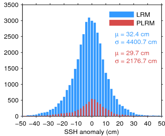
Figure 7. Histogram of flag-valid SSH anomaly over oceans and lakes for LRM (blue) and PLRM (red) for 25/10/2015. The mean ( \mu ) and standard deviation ( \sigma ) are also shown. Note that values outside [-50\ 50] cm are excluded from the histogram for the sake of readability but not from the computation of \mu and \sigma .
