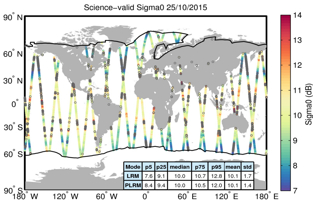
Figure 27. Geographical distribution of science-valid sigma0 data over oceans and lakes for 25/10/2015. The statistical values shown in the table refer to the sigma0 in dB and are calculated separately for LRM and PLRM regions. The black lines mark the outer limit of the Arctic and Antarctic polar polygons. Gray circles denote records that have been rejected based on the editing criteria described in Table 4.
