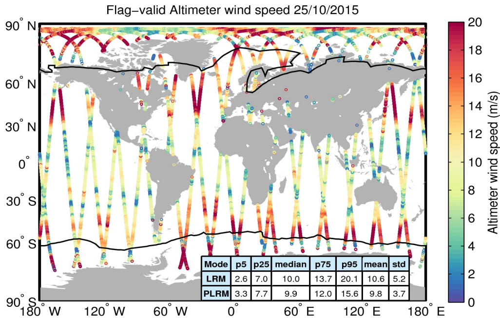
Figure 31. Geographical distribution of flag-valid wind data over oceans and lakes for 25/10/2015. The statistical values shown in the table refer to the wind in m/s and are calculated separately for LRM and PLRM regions. Measurements taken over polar polygons have been excluded from the computation of the statistical values. The black lines mark the outer limit of the Arctic and Antarctic polar polygons.
