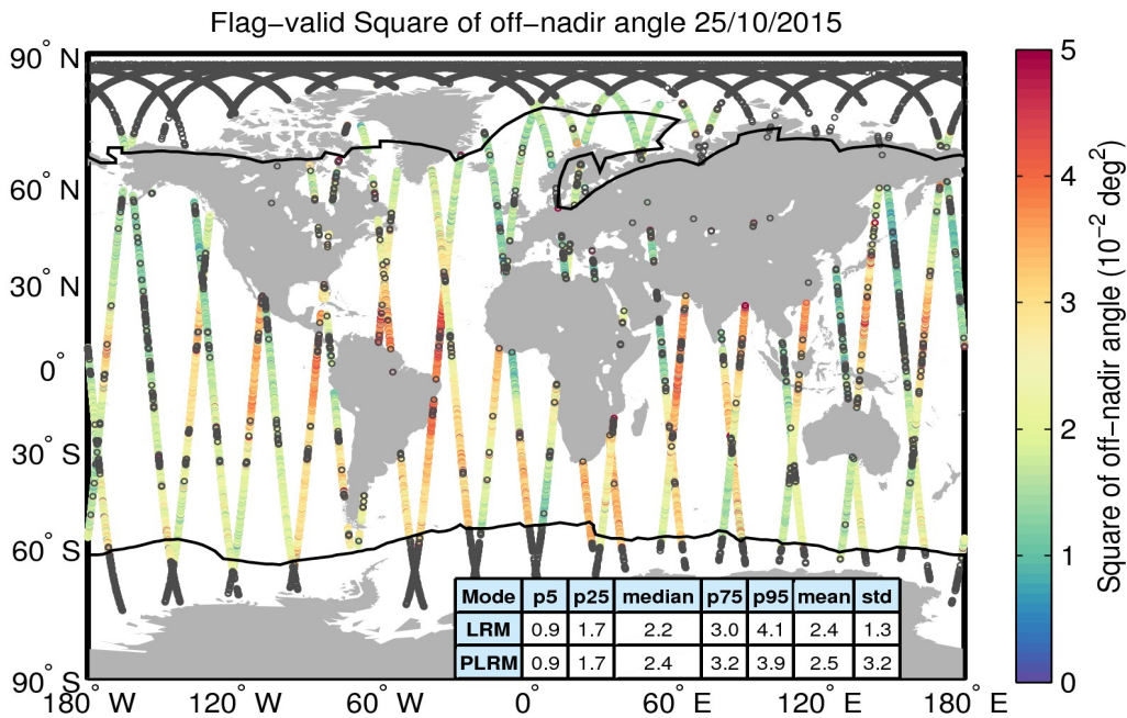
Figure 37. Geographical distribution of flag-valid mispointing data over oceans and lakes for 25/10/2015. The statistical values shown in the table refer to the mispointing in 10^{-2} deg 2 and are calculated separately for LRM and PLRM regions. Measurements taken over polar polygons have been excluded from the computation of the statistical values. The black lines mark the outer limit of the Arctic and Antarctic polar polygons. Gray circles denote negative values.
