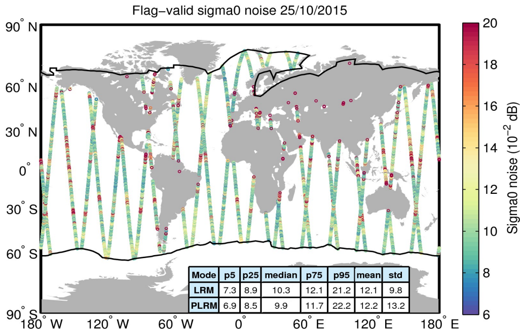
Figure 26. Geographical distribution of flag-valid 20-Hz sigma0 measurement noise over oceans and lakes for 25/10/2015. The statistical values shown in the table refer to the sigma0 noise and are calculated separately for LRM and PLRM regions. Measurements taken over polar polygons have been excluded from the computation of the statistical values. The black lines mark the outer limit of the Arctic and Antarctic polar polygons.
