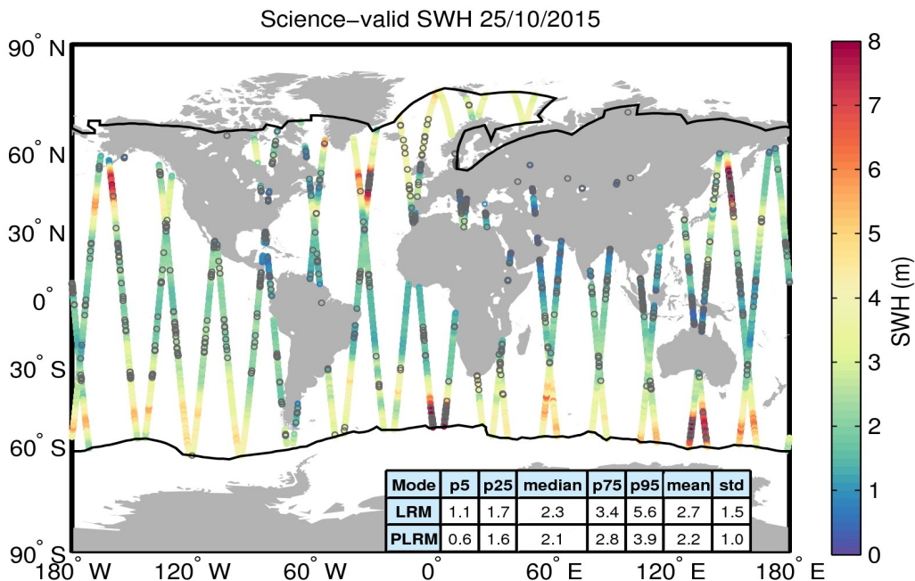
Figure 19. Geographical distribution of science-valid SWH data over oceans and lakes for 25/10/2015. The statistical values shown in the table refer to the SWH in m and are calculated separately for LRM and PLRM regions. The black lines mark the outer limit of the Arctic and Antarctic polar polygons. Gray circles denote records that have been rejected based on the editing criteria described in Table 3.
