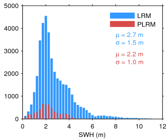
Figure 20. Histogram of science-valid SWH over oceans and lakes for LRM (blue) and PLRM (red) for 25/10/2015. The mean ( \mu ) and standard deviation ( \sigma ) are also shown. Note that values larger than 12 m are excluded from the histogram for the sake of readability but not from the computation of \mu and \sigma .
