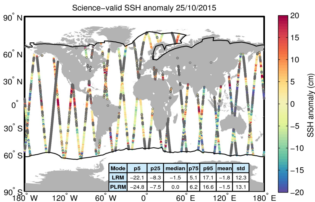
Figure 10. Geographical distribution of science-valid SSH anomaly data over oceans and lakes for 25/10/2015. The statistical values shown in the table refer to the SSH anomaly in cm and are calculated separately for LRM and PLRM regions. The black lines mark the outer limit of the Arctic and Antarctic polar polygons. Gray circles denote records that have been rejected based on the editing criteria described in Table 2.
