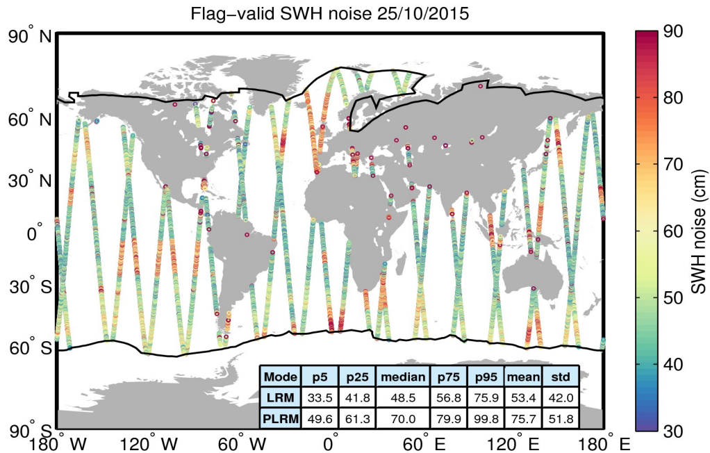
Figure 18. Geographical distribution of flag-valid 20-Hz SWH measurement noise over oceans and lakes for 25/10/2015. The statistical values shown in the table refer to the SWH noise and are calculated separately for LRM and PLRM regions. Measurements taken over polar polygons have been excluded from the computation of the statistical values. The black lines mark the outer limit of the Arctic and Antarctic polar polygons.
