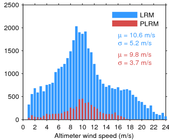
Figure 33. Histogram of flag-valid wind over oceans and lakes for LRM (blue) and PLRM (red) for 25/10/2015. The mean ( \mu ) and standard deviation ( \sigma ) are also shown. Note that values larger than 24 m/s are excluded from the histogram for the sake of readability but not from the computation of \mu and \sigma .
