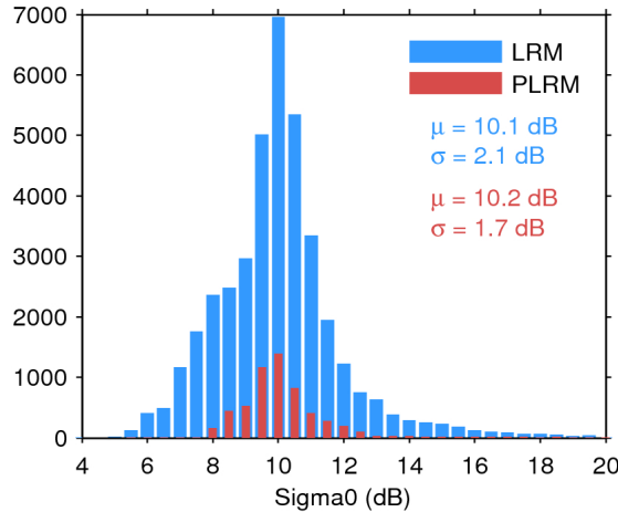
Figure 25. Histogram of flag-valid sigma0 over oceans and lakes for LRM (blue) and PLRM (red) for 25/10/2015. The mean ( \mu ) and standard deviation ( \sigma ) are also shown. Note that values outside [4 20] dB are excluded from the histogram for the sake of readability but not from the computation of \mu and \sigma .
