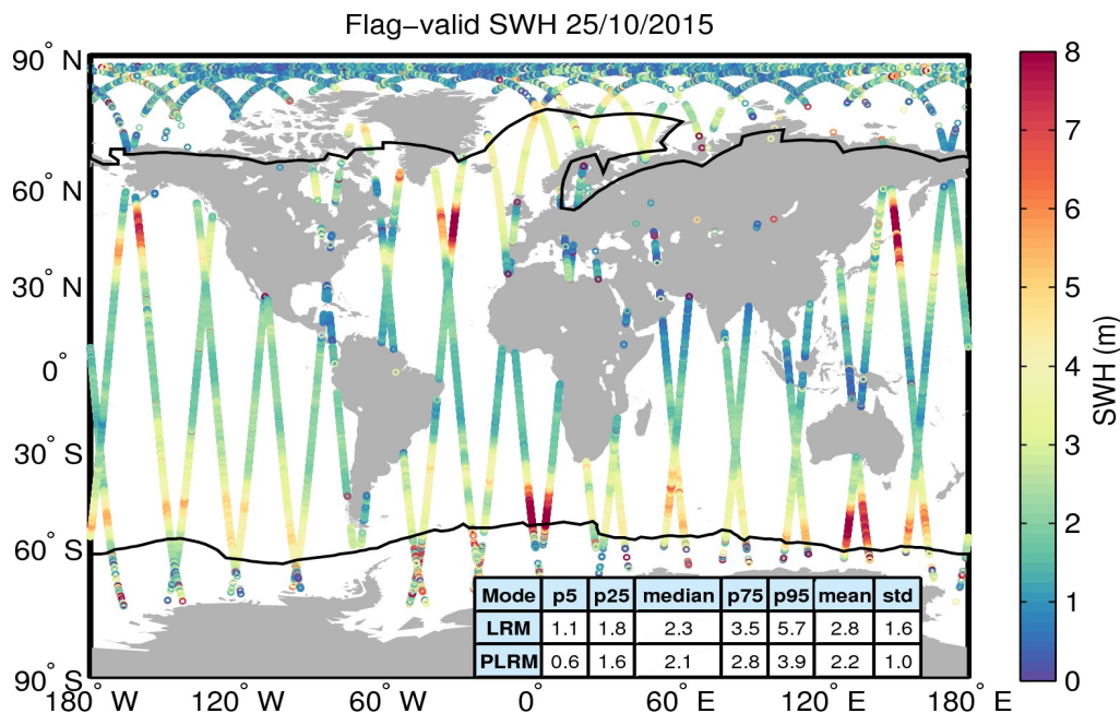
Figure 15. Geographical distribution of flag-valid SWH data over oceans and lakes for 25/10/2015. The statistical values shown in the table refer to the SWH in m and are calculated separately for LRM and PLRM regions. Measurements taken over polar polygons have been excluded from the computation of the statistical values. The black lines mark the outer limit of the Arctic and Antarctic polar polygons.
