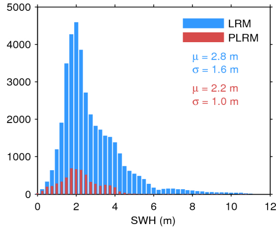
Figure 17. Histogram of flag-valid SWH over oceans and lakes for LRM (blue) and PLRM (red) for 25/10/2015. The mean ( \mu ) and standard deviation ( \sigma ) are also shown. Note that values larger than 12 m are excluded from the histogram for the sake of readability but not from the computation of \mu and \sigma .
