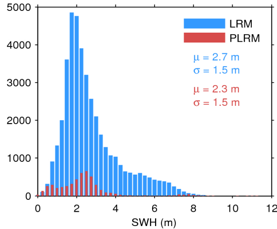
Figure 17. Histogram of flag-valid SWH over oceans and lakes for LRM (blue) and PLRM (red) for 18/10/2015. The mean ( \mu ) and standard deviation ( \sigma ) are also shown. Note that values larger than 12 m are excluded from the histogram for the sake of readability but not from the computation of \mu and \sigma .
