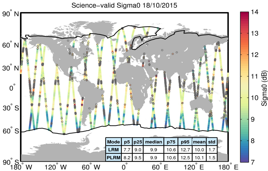
Figure 27. Geographical distribution of science-valid sigma0 data over oceans and lakes for 18/10/2015. The statistical values shown in the table refer to the sigma0 in dB and are calculated separately for LRM and PLRM regions. The black lines mark the outer limit of the Arctic and Antarctic polar polygons. Gray circles denote records that have been rejected based on the editing criteria described in Table 4.
