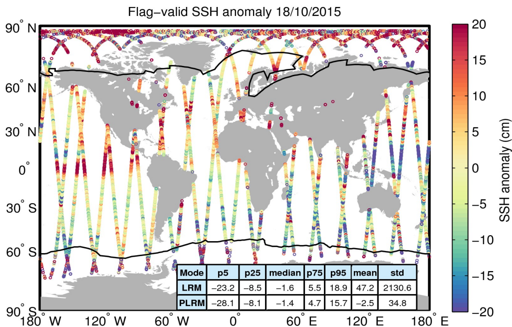
Figure 5. Geographical distribution of flag-valid 1-Hz SSH anomaly data over oceans and lakes for 18/10/2015. The statistical values shown in the table refer to the SSH anomaly in cm and are calculated separately for LRM and PLRM regions. Measurements taken over polar polygons have been excluded from the computation of the statistical values. The black lines mark the outer limit of the Arctic and Antarctic polar polygons.
