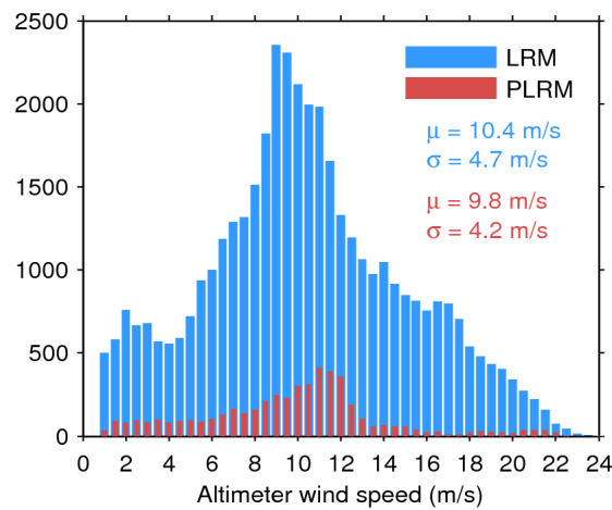
Figure 33. Histogram of flag-valid wind over oceans and lakes for LRM (blue) and PLRM (red) for 18/10/2015. The mean ( \mu ) and standard deviation ( \sigma ) are also shown. Note that values larger than 24 m/s are excluded from the histogram for the sake of readability but not from the computation of \mu and \sigma .
