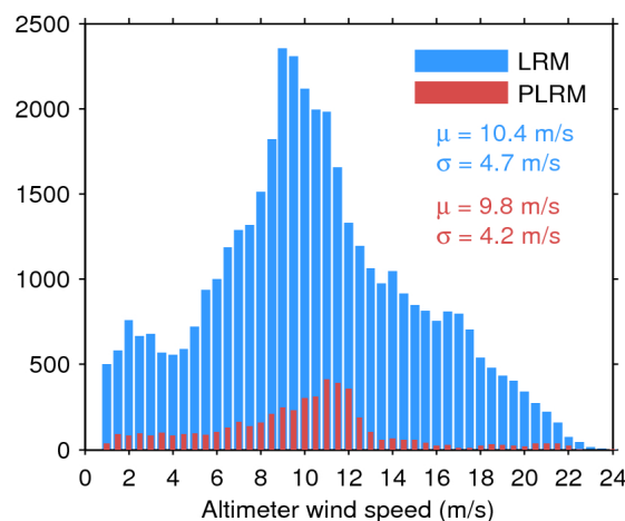
Figure 35. Histogram of science-valid wind over oceans and lakes for LRM (blue) and PLRM (red) for 18/10/2015. The mean ( \mu ) and standard deviation ( \sigma ) are also shown. Note that values larger than 24 m/s are excluded from the histogram for the sake of readability but not from the computation of \mu and \sigma .
