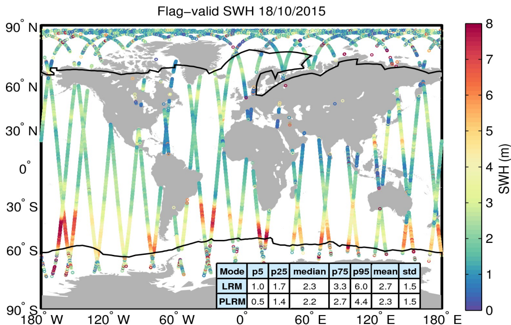
Figure 15. Geographical distribution of flag-valid SWH data over oceans and lakes for 18/10/2015. The statistical values shown in the table refer to the SWH in m and are calculated separately for LRM and PLRM regions. Measurements taken over polar polygons have been excluded from the computation of the statistical values. The black lines mark the outer limit of the Arctic and Antarctic polar polygons.
