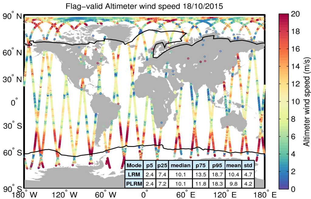
Figure 31. Geographical distribution of flag-valid wind data over oceans and lakes for 18/10/2015. The statistical values shown in the table refer to the wind in m/s and are calculated separately for LRM and PLRM regions. Measurements taken over polar polygons have been excluded from the computation of the statistical values. The black lines mark the outer limit of the Arctic and Antarctic polar polygons.
