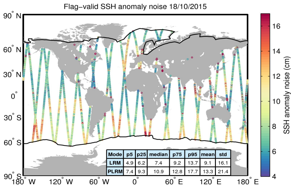
Figure 8. Geographical distribution of flag-valid 20-Hz SSH anomaly measurement noise over oceans and lakes for 18/10/2015. The statistical values shown in the table refer to the SSH anomaly noise and are calculated separately for LRM and PLRM regions. Measurements taken over polar polygons have been excluded from the computation of the statistical values. The black lines mark the outer limit of the Arctic and Antarctic polar polygons.
