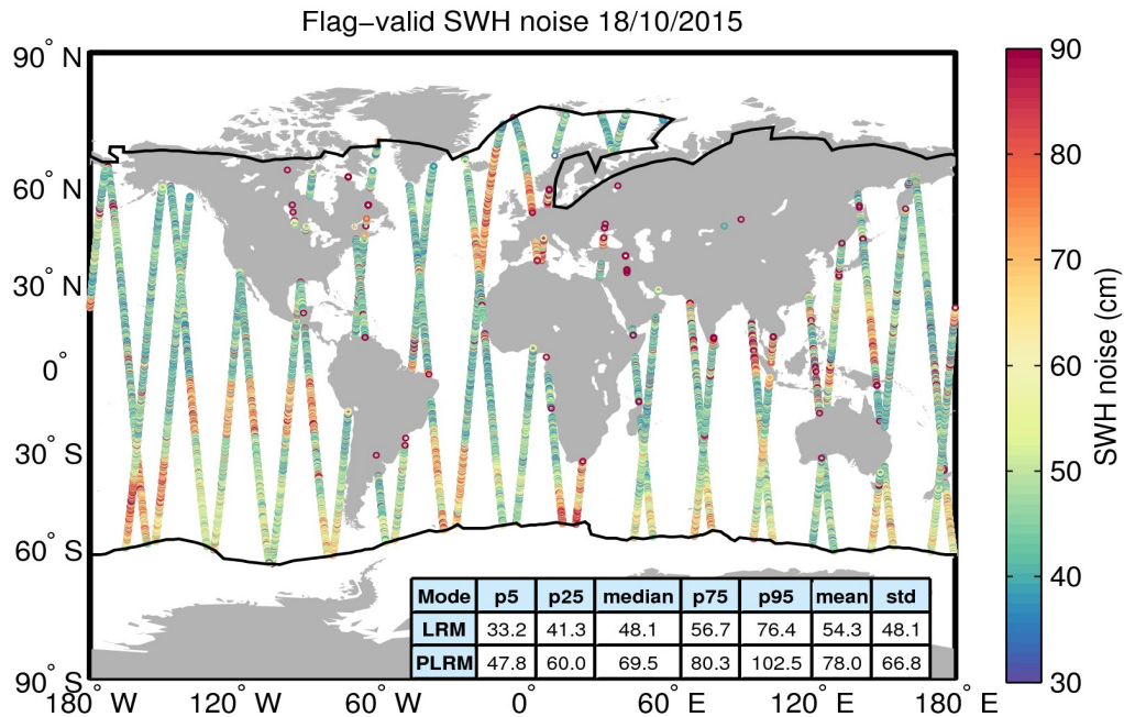
Figure 18. Geographical distribution of flag-valid 20-Hz SWH measurement noise over oceans and lakes for 18/10/2015. The statistical values shown in the table refer to the SWH noise and are calculated separately for LRM and PLRM regions. Measurements taken over polar polygons have been excluded from the computation of the statistical values. The black lines mark the outer limit of the Arctic and Antarctic polar polygons.
