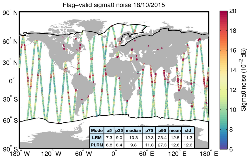
Figure 26. Geographical distribution of flag-valid 20-Hz sigma0 measurement noise over oceans and lakes for 18/10/2015. The statistical values shown in the table refer to the sigma0 noise and are calculated separately for LRM and PLRM regions. Measurements taken over polar polygons have been excluded from the computation of the statistical values. The black lines mark the outer limit of the Arctic and Antarctic polar polygons.
