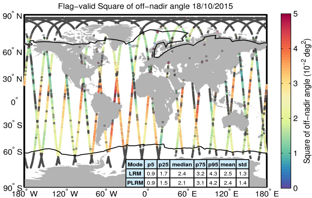
Figure 37. Geographical distribution of flag-valid mispointing data over oceans and lakes for 18/10/2015. The statistical values shown in the table refer to the mispointing in 10^{-2} deg 2 and are calculated separately for LRM and PLRM regions. Measurements taken over polar polygons have been excluded from the computation of the statistical values. The black lines mark the outer limit of the Arctic and Antarctic polar polygons. Gray circles denote negative values.
