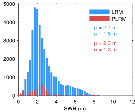
Figure 20. Histogram of science-valid SWH over oceans and lakes for LRM (blue) and PLRM (red) for 18/10/2015. The mean ( \mu ) and standard deviation ( \sigma ) are also shown. Note that values larger than 12 m are excluded from the histogram for the sake of readability but not from the computation of \mu and \sigma .
