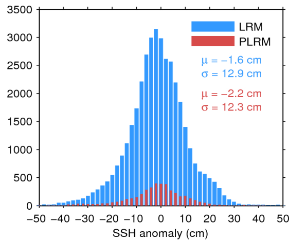
Figure 11. Histogram of science-valid SSH anomaly over oceans and lakes for LRM (blue) and PLRM (red) for 18/10/2015. The mean ( \mu ) and standard deviation ( \sigma ) are also shown. Note that values outside [-50\ 50] cm are excluded from the histogram for the sake of readability but not from the computation of \mu and \sigma .
