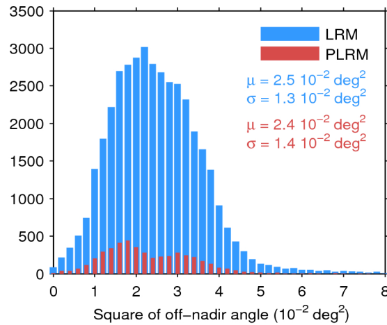
Figure 39. Histogram of flag-valid mispointing over oceans and lakes for LRM (blue) and PLRM (red) for 18/10/2015. Only positive values have been considered. The mean ( \mu ) and standard deviation ( \sigma ) are also shown. Note that values larger than 8 \times 10^{-2} \text{ deg}^2 are excluded from the histogram for the sake of readability but not from the computation of \mu and \sigma .
