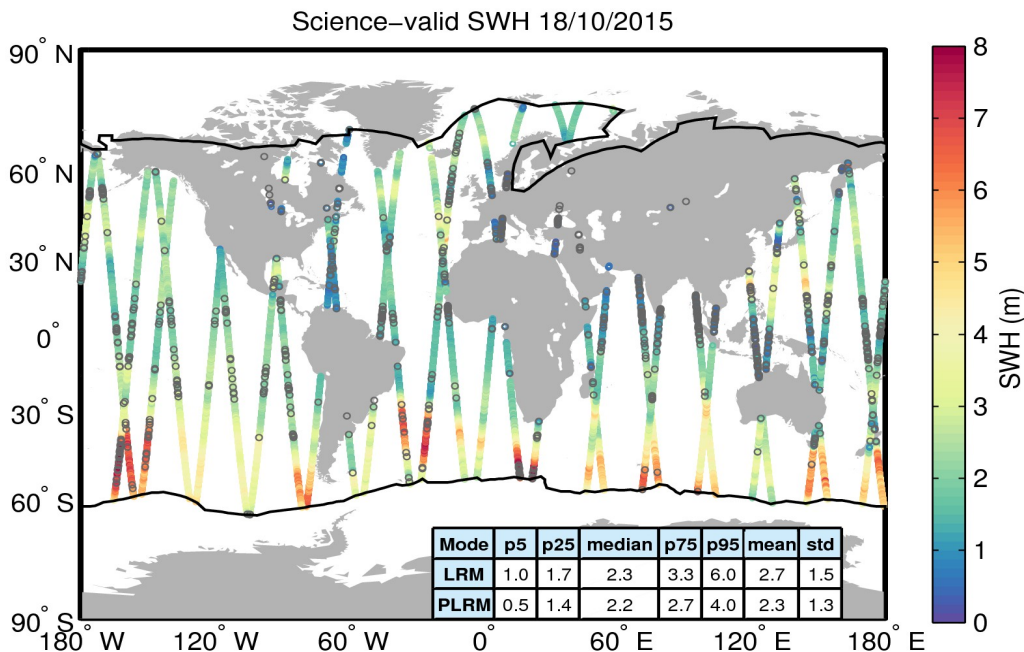
Figure 19. Geographical distribution of science-valid SWH data over oceans and lakes for 18/10/2015. The statistical values shown in the table refer to the SWH in m and are calculated separately for LRM and PLRM regions. The black lines mark the outer limit of the Arctic and Antarctic polar polygons. Gray circles denote records that have been rejected based on the editing criteria described in Table 3.
