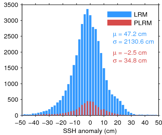
Figure 7. Histogram of flag-valid SSH anomaly over oceans and lakes for LRM (blue) and PLRM (red) for 18/10/2015. The mean ( \mu ) and standard deviation ( \sigma ) are also shown. Note that values outside [-50 50] cm are excluded from the histogram for the sake of readability but not from the computation of \mu and \sigma .
