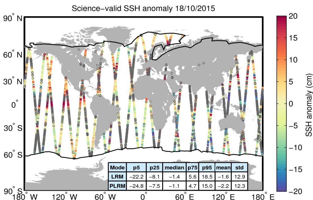
Figure 10. Geographical distribution of science-valid SSH anomaly data over oceans and lakes for 18/10/2015. The statistical values shown in the table refer to the SSH anomaly in cm and are calculated separately for LRM and PLRM regions. The black lines mark the outer limit of the Arctic and Antarctic polar polygons. Gray circles denote records that have been rejected based on the editing criteria described in Table 2.
