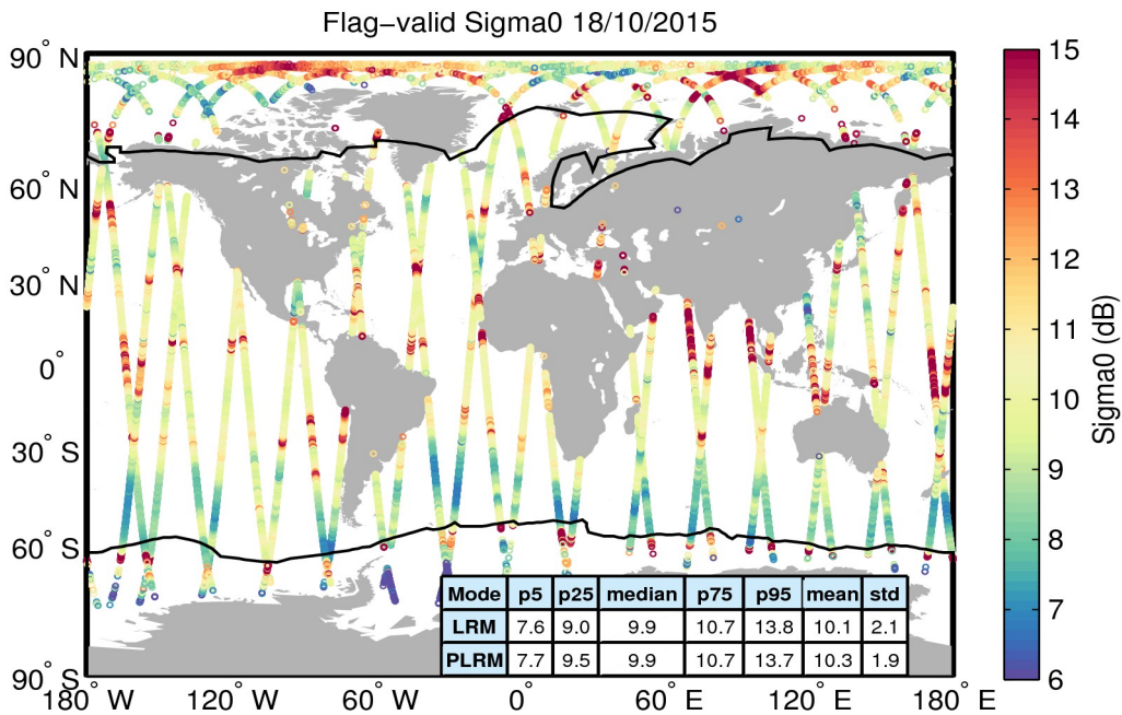
Figure 23. Geographical distribution of flag-valid sigma0 data over oceans and lakes for 18/10/2015. The statistical values shown in the table refer to the sigma0 in dB and are calculated separately for LRM and PLRM regions. Measurements taken over polar polygons have been excluded from the computation of the statistical values. The black lines mark the outer limit of the Arctic and Antarctic polar polygons.
