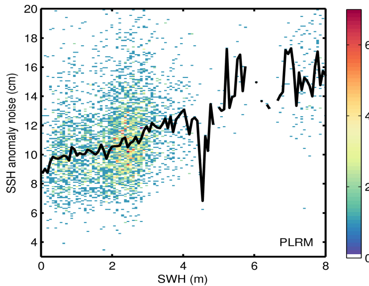
Figure 9. 2D histogram showing flag-valid SSH anomaly noise as a function of SWH for LRM (top) and PLRM (bottom) for 18/10/2015. The black line denotes the median SSH anomaly noise as a function of SWH.
