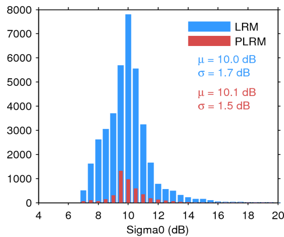
Figure 28. Histogram of science-valid sigma0 over oceans and lakes for LRM (blue) and PLRM (red) for 18/10/2015. The mean ( \mu ) and standard deviation ( \sigma ) are also shown. Note that values outside [4 20] dB are excluded from the histogram for the sake of readability but not from the computation of \mu and \sigma .
