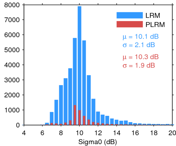
Figure 25. Histogram of flag-valid sigma0 over oceans and lakes for LRM (blue) and PLRM (red) for 18/10/2015. The mean ( \mu ) and standard deviation ( \sigma ) are also shown. Note that values outside [4 20] dB are excluded from the histogram for the sake of readability but not from the computation of \mu and \sigma .
