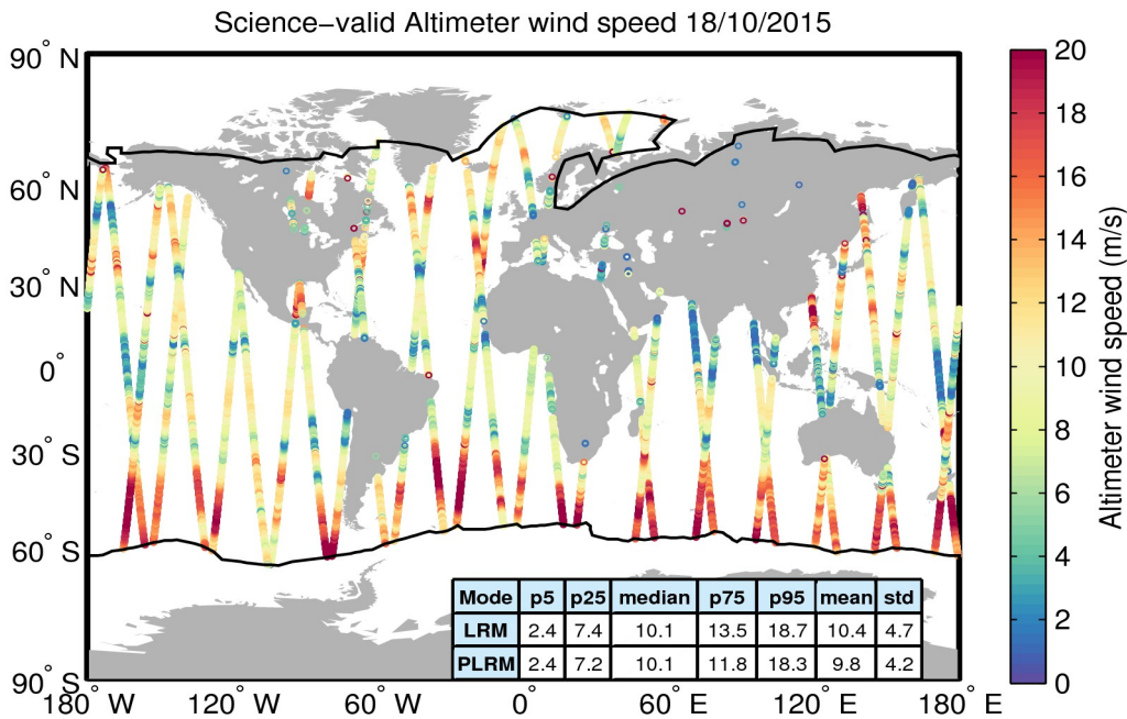
Figure 34. Geographical distribution of science-valid wind data over oceans and lakes for 18/10/2015. The statistical values shown in the table refer to the wind in m/s and are calculated separately for LRM and PLRM regions. The black lines mark the outer limit of the Arctic and Antarctic polar polygons. Gray circles denote records that have been rejected based on the editing criteria described in Table 5.
