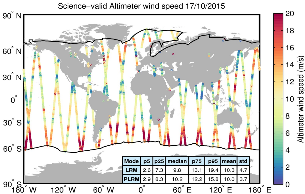
Figure 34. Geographical distribution of science-valid wind data over oceans and lakes for 17/10/2015. The statistical values shown in the table refer to the wind in m/s and are calculated separately for LRM and PLRM regions. The black lines mark the outer limit of the Arctic and Antarctic polar polygons. Gray circles denote records that have been rejected based on the editing criteria described in Table 5.
