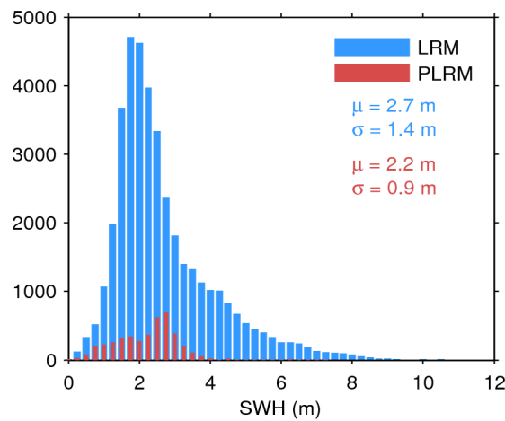
Figure 20. Histogram of science-valid SWH over oceans and lakes for LRM (blue) and PLRM (red) for 17/10/2015. The mean ( \mu ) and standard deviation ( \sigma ) are also shown. Note that values larger than 12 m are excluded from the histogram for the sake of readability but not from the computation of \mu and \sigma .
