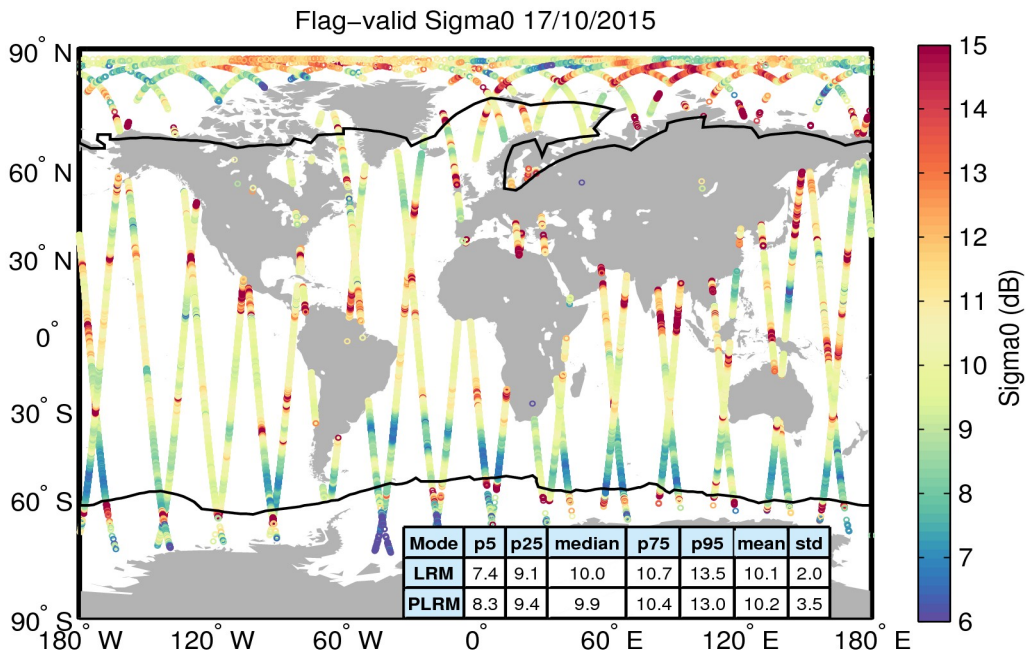
Figure 23. Geographical distribution of flag-valid sigma0 data over oceans and lakes for 17/10/2015. The statistical values shown in the table refer to the sigma0 in dB and are calculated separately for LRM and PLRM regions. Measurements taken over polar polygons have been excluded from the computation of the statistical values. The black lines mark the outer limit of the Arctic and Antarctic polar polygons.
