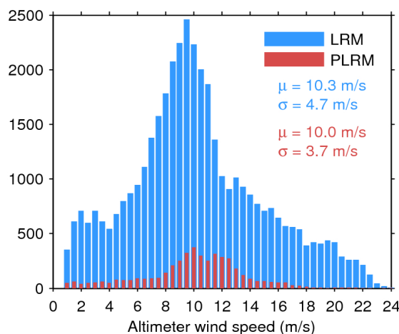
Figure 35. Histogram of science-valid wind over oceans and lakes for LRM (blue) and PLRM (red) for 17/10/2015. The mean ( \mu ) and standard deviation ( \sigma ) are also shown. Note that values larger than 24 m/s are excluded from the histogram for the sake of readability but not from the computation of \mu and \sigma .
