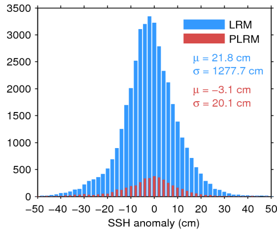
Figure 7. Histogram of flag-valid SSH anomaly over oceans and lakes for LRM (blue) and PLRM (red) for 17/10/2015. The mean ( \mu ) and standard deviation ( \sigma ) are also shown. Note that values outside [-50 50] cm are excluded from the histogram for the sake of readability but not from the computation of \mu and \sigma .
