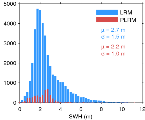
Figure 17. Histogram of flag-valid SWH over oceans and lakes for LRM (blue) and PLRM (red) for 17/10/2015. The mean ( \mu ) and standard deviation ( \sigma ) are also shown. Note that values larger than 12 m are excluded from the histogram for the sake of readability but not from the computation of \mu and \sigma .
