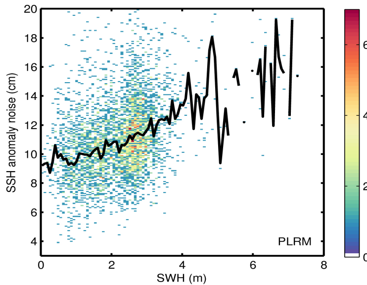
Figure 9. 2D histogram showing flag-valid SSH anomaly noise as a function of SWH for LRM (top) and PLRM (bottom) for 17/10/2015. The black line denotes the median SSH anomaly noise as a function of SWH.
