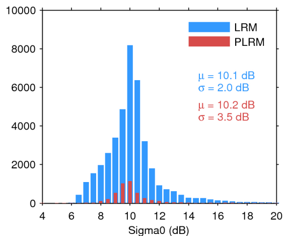
Figure 25. Histogram of flag-valid sigma0 over oceans and lakes for LRM (blue) and PLRM (red) for 17/10/2015. The mean ( \mu ) and standard deviation ( \sigma ) are also shown. Note that values outside [4 20] dB are excluded from the histogram for the sake of readability but not from the computation of \mu and \sigma .
