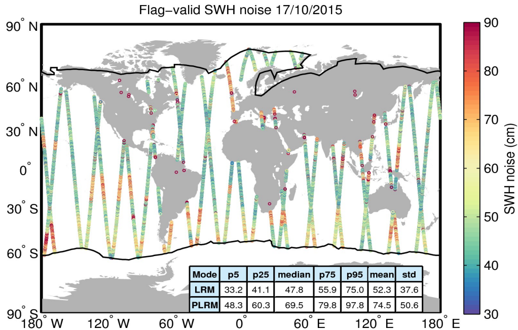
Figure 18. Geographical distribution of flag-valid 20-Hz SWH measurement noise over oceans and lakes for 17/10/2015. The statistical values shown in the table refer to the SWH noise and are calculated separately for LRM and PLRM regions. Measurements taken over polar polygons have been excluded from the computation of the statistical values. The black lines mark the outer limit of the Arctic and Antarctic polar polygons.
