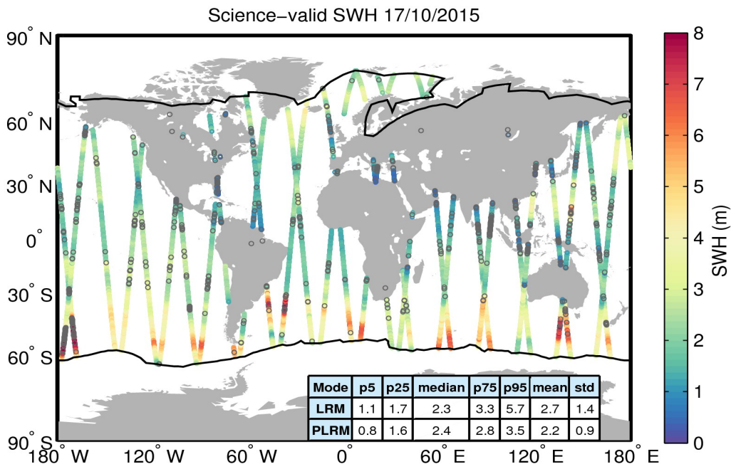
Figure 19. Geographical distribution of science-valid SWH data over oceans and lakes for 17/10/2015. The statistical values shown in the table refer to the SWH in m and are calculated separately for LRM and PLRM regions. The black lines mark the outer limit of the Arctic and Antarctic polar polygons. Gray circles denote records that have been rejected based on the editing criteria described in Table 3.
