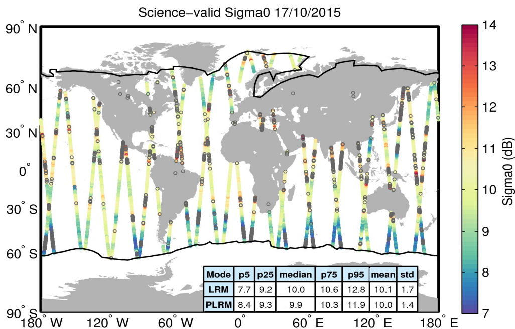
Figure 27. Geographical distribution of science-valid sigma0 data over oceans and lakes for 17/10/2015. The statistical values shown in the table refer to the sigma0 in dB and are calculated separately for LRM and PLRM regions. The black lines mark the outer limit of the Arctic and Antarctic polar polygons. Gray circles denote records that have been rejected based on the editing criteria described in Table 4.
