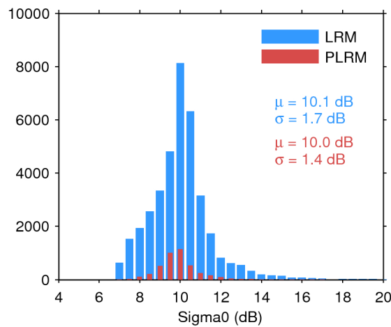
Figure 28. Histogram of science-valid sigma0 over oceans and lakes for LRM (blue) and PLRM (red) for 17/10/2015. The mean ( \mu ) and standard deviation ( \sigma ) are also shown. Note that values outside [4 20] dB are excluded from the histogram for the sake of readability but not from the computation of \mu and \sigma .
