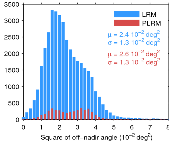
Figure 39. Histogram of flag-valid mispointing over oceans and lakes for LRM (blue) and PLRM (red) for 17/10/2015. Only positive values have been considered. The mean ( \mu ) and standard deviation ( \sigma ) are also shown. Note that values larger than 8 \cdot 10^{-2} \text{ deg}^2 are excluded from the histogram for the sake of readability but not from the computation of \mu and \sigma .
