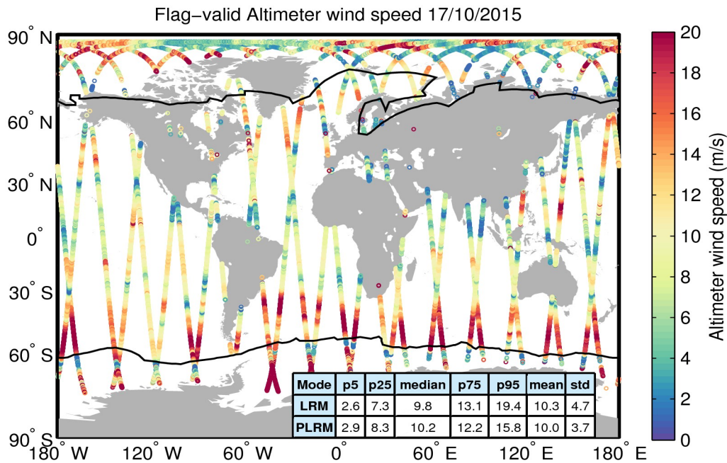
Figure 31. Geographical distribution of flag-valid wind data over oceans and lakes for 17/10/2015. The statistical values shown in the table refer to the wind in m/s and are calculated separately for LRM and PLRM regions. Measurements taken over polar polygons have been excluded from the computation of the statistical values. The black lines mark the outer limit of the Arctic and Antarctic polar polygons.
