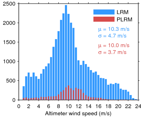
Figure 33. Histogram of flag-valid wind over oceans and lakes for LRM (blue) and PLRM (red) for 17/10/2015. The mean ( \mu ) and standard deviation ( \sigma ) are also shown. Note that values larger than 24 m/s are excluded from the histogram for the sake of readability but not from the computation of \mu and \sigma .
