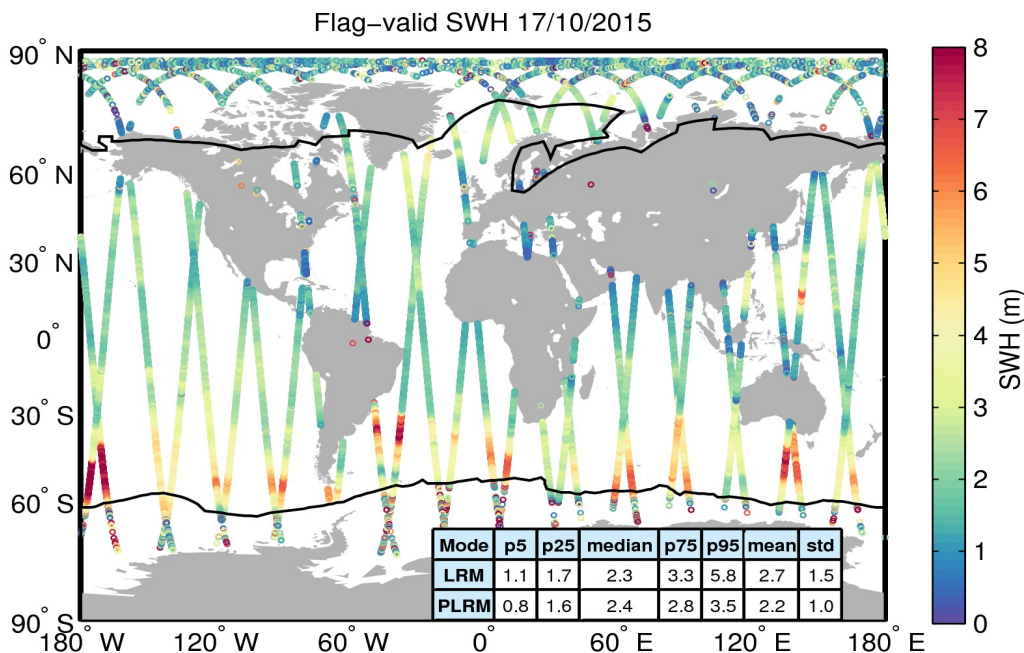
Figure 15. Geographical distribution of flag-valid SWH data over oceans and lakes for 17/10/2015. The statistical values shown in the table refer to the SWH in m and are calculated separately for LRM and PLRM regions. Measurements taken over polar polygons have been excluded from the computation of the statistical values. The black lines mark the outer limit of the Arctic and Antarctic polar polygons.
