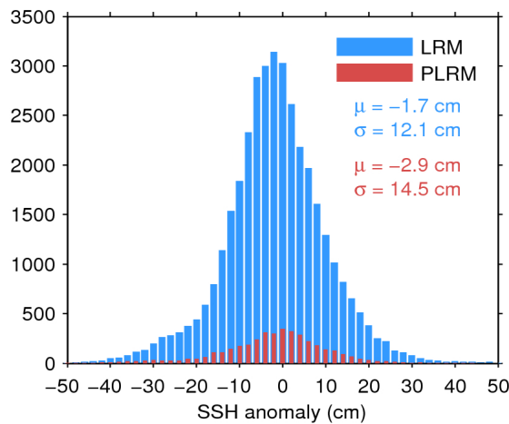
Figure 11. Histogram of science-valid SSH anomaly over oceans and lakes for LRM (blue) and PLRM (red) for 17/10/2015. The mean ( \mu ) and standard deviation ( \sigma ) are also shown. Note that values outside [-50 50] cm are excluded from the histogram for the sake of readability but not from the computation of \mu and \sigma .
