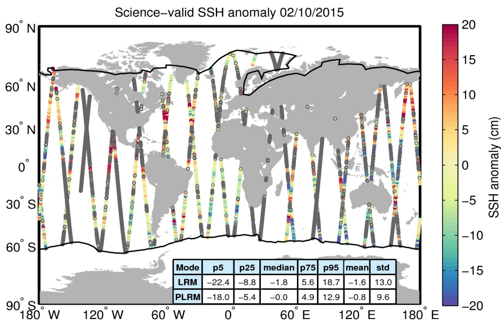
Figure 10. Geographical distribution of science-valid SSH anomaly data over oceans and lakes for 02/10/2015. The statistical values shown in the table refer to the SSH anomaly in cm and are calculated separately for LRM and PLRM regions. The black lines mark the outer limit of the Arctic and Antarctic polar polygons. Gray circles denote records that have been rejected based on the editing criteria described in Table 2.
