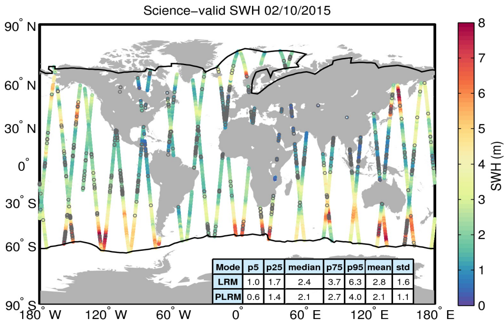
Figure 19. Geographical distribution of science-valid SWH data over oceans and lakes for 02/10/2015. The statistical values shown in the table refer to the SWH in m and are calculated separately for LRM and PLRM regions. The black lines mark the outer limit of the Arctic and Antarctic polar polygons. Gray circles denote records that have been rejected based on the editing criteria described in Table 3.
