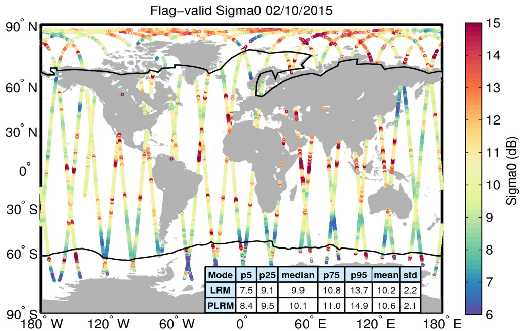
Figure 23. Geographical distribution of flag-valid sigma0 data over oceans and lakes for 02/10/2015. The statistical values shown in the table refer to the sigma0 in dB and are calculated separately for LRM and PLRM regions. Measurements taken over polar polygons have been excluded from the computation of the statistical values. The black lines mark the outer limit of the Arctic and Antarctic polar polygons.
