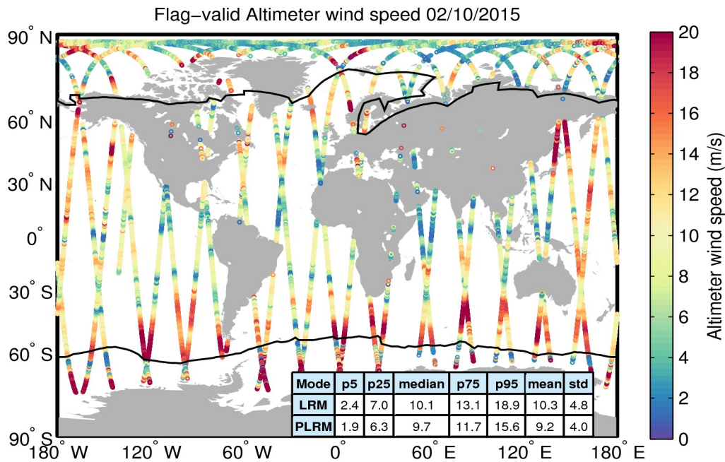
Figure 31. Geographical distribution of flag-valid wind data over oceans and lakes for 02/10/2015. The statistical values shown in the table refer to the wind in m/s and are calculated separately for LRM and PLRM regions. Measurements taken over polar polygons have been excluded from the computation of the statistical values. The black lines mark the outer limit of the Arctic and Antarctic polar polygons.
