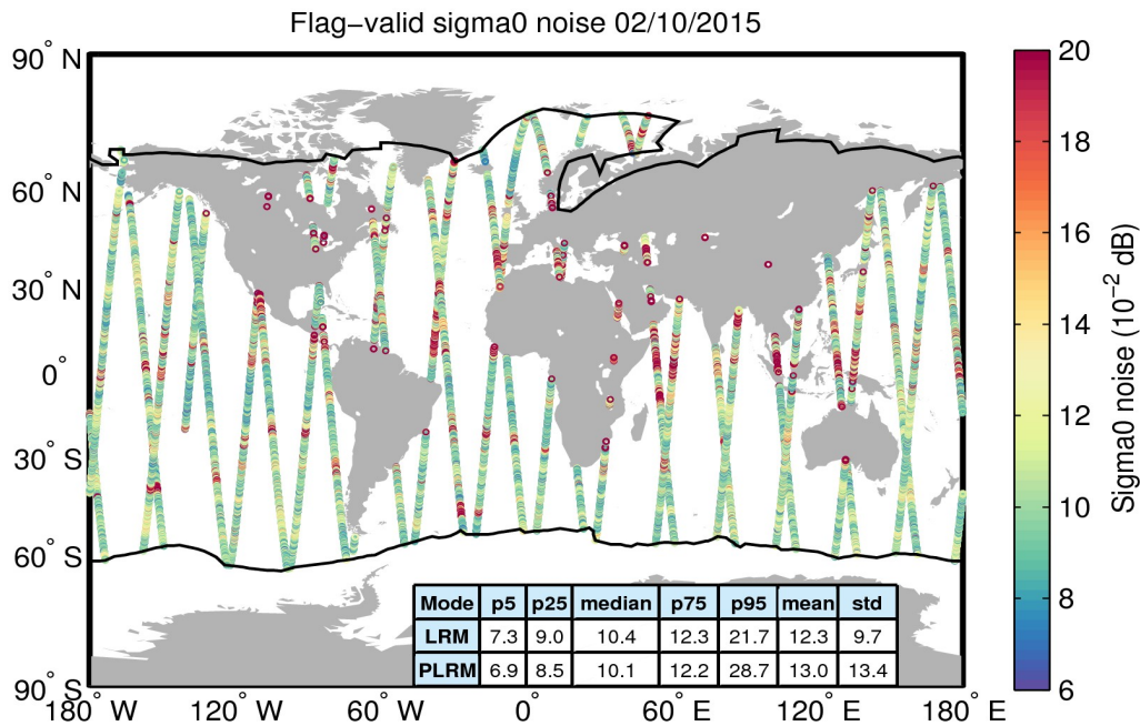
Figure 26. Geographical distribution of flag-valid 20-Hz sigma0 measurement noise over oceans and lakes for 02/10/2015. The statistical values shown in the table refer to the sigma0 noise and are calculated separately for LRM and PLRM regions. Measurements taken over polar polygons have been excluded from the computation of the statistical values. The black lines mark the outer limit of the Arctic and Antarctic polar polygons.
