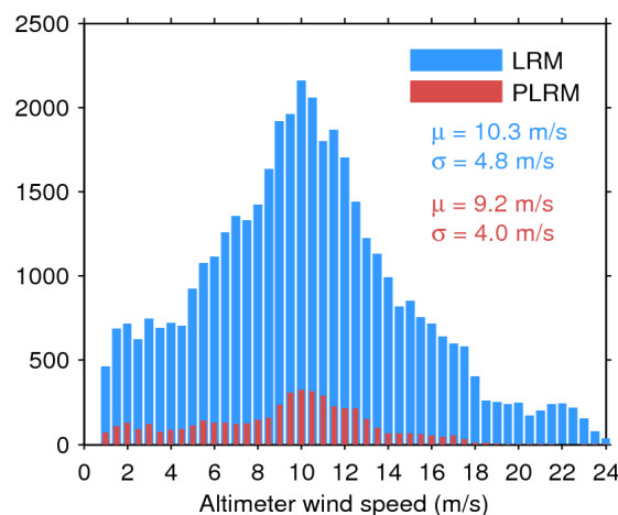
Figure 35. Histogram of science-valid wind over oceans and lakes for LRM (blue) and PLRM (red) for 02/10/2015. The mean ( \mu ) and standard deviation ( \sigma ) are also shown. Note that values larger than 24 m/s are excluded from the histogram for the sake of readability but not from the computation of \mu and \sigma .
