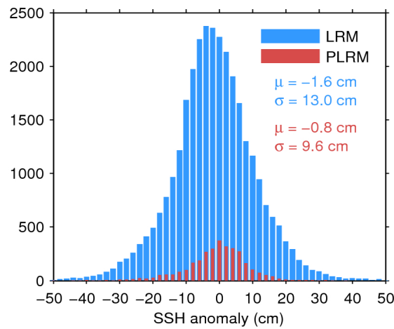
Figure 11. Histogram of science-valid SSH anomaly over oceans and lakes for LRM (blue) and PLRM (red) for 02/10/2015. The mean ( \mu ) and standard deviation ( \sigma ) are also shown. Note that values outside [-50 50] cm are excluded from the histogram for the sake of readability but not from the computation of \mu and \sigma .
