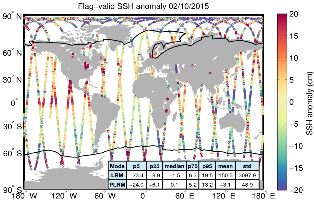
Figure 5. Geographical distribution of flag-valid 1-Hz SSH anomaly data over oceans and lakes for 02/10/2015. The statistical values shown in the table refer to the SSH anomaly in cm and are calculated separately for LRM and PLRM regions. Measurements taken over polar polygons have been excluded from the computation of the statistical values. The black lines mark the outer limit of the Arctic and Antarctic polar polygons.
