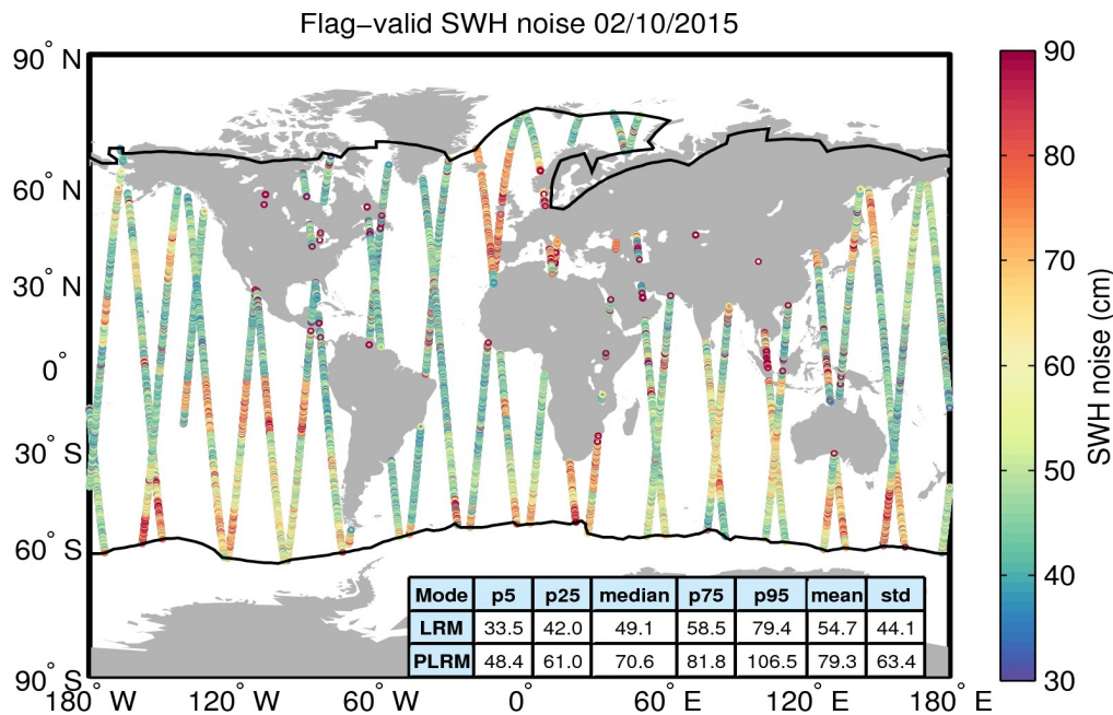
Figure 18. Geographical distribution of flag-valid 20-Hz SWH measurement noise over oceans and lakes for 02/10/2015. The statistical values shown in the table refer to the SWH noise and are calculated separately for LRM and PLRM regions. Measurements taken over polar polygons have been excluded from the computation of the statistical values. The black lines mark the outer limit of the Arctic and Antarctic polar polygons.
