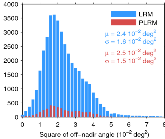
Figure 39. Histogram of flag-valid mispointing over oceans and lakes for LRM (blue) and PLRM (red) for 02/10/2015. Only positive values have been considered. The mean ( \mu ) and standard deviation ( \sigma ) are also shown. Note that values larger than 8 \cdot 10^{-2} \text{ deg}^2 are excluded from the histogram for the sake of readability but not from the computation of \mu and \sigma .
