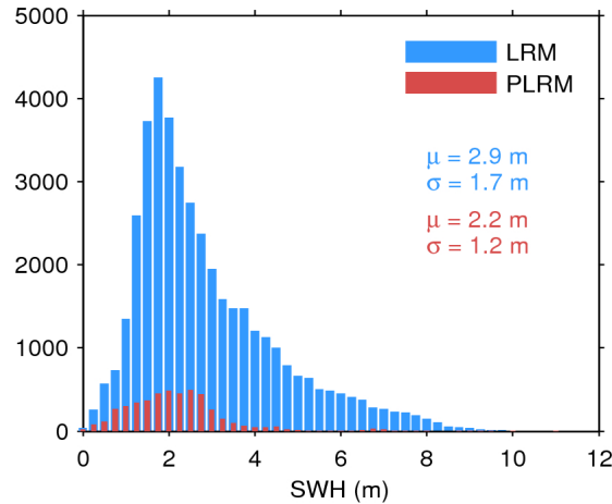
Figure 17. Histogram of flag-valid SWH over oceans and lakes for LRM (blue) and PLRM (red) for 02/10/2015. The mean ( \mu ) and standard deviation ( \sigma ) are also shown. Note that values larger than 12 m are excluded from the histogram for the sake of readability but not from the computation of \mu and \sigma .
