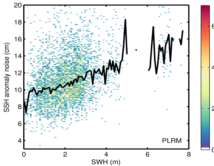
Figure 9. 2D histogram showing flag-valid SSH anomaly noise as a function of SWH for LRM (top) and PLRM (bottom) for 02/10/2015. The black line denotes the median SSH anomaly noise as a function of SWH.
