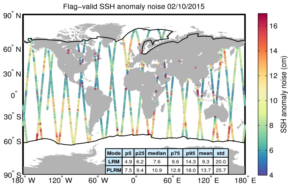
Figure 8. Geographical distribution of flag-valid 20-Hz SSH anomaly measurement noise over oceans and lakes for 02/10/2015. The statistical values shown in the table refer to the SSH anomaly noise and are calculated separately for LRM and PLRM regions. Measurements taken over polar polygons have been excluded from the computation of the statistical values. The black lines mark the outer limit of the Arctic and Antarctic polar polygons.
