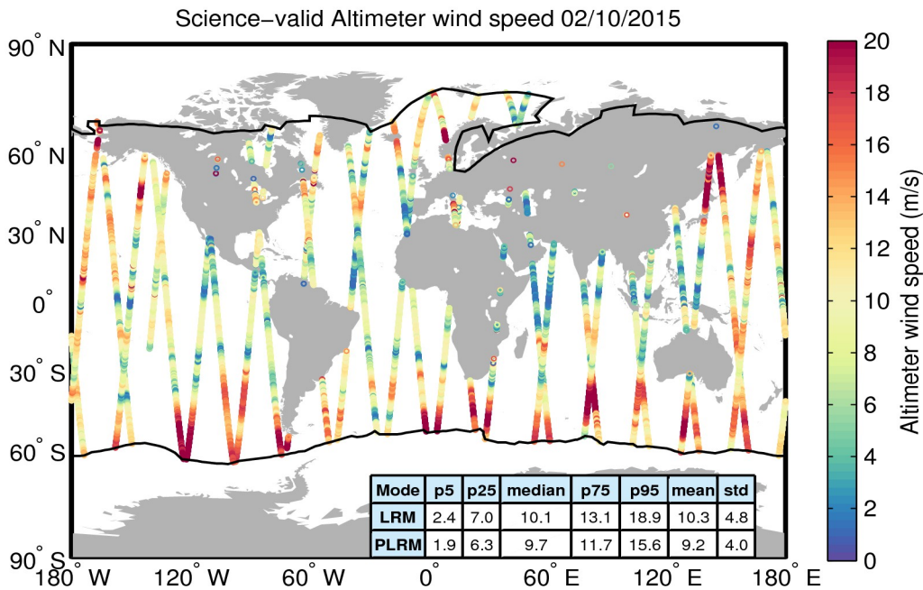
Figure 34. Geographical distribution of science-valid wind data over oceans and lakes for 02/10/2015. The statistical values shown in the table refer to the wind in m/s and are calculated separately for LRM and PLRM regions. The black lines mark the outer limit of the Arctic and Antarctic polar polygons. Gray circles denote records that have been rejected based on the editing criteria described in Table 5.
