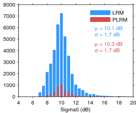
Figure 28. Histogram of science-valid sigma0 over oceans and lakes for LRM (blue) and PLRM (red) for 02/10/2015. The mean ( \mu ) and standard deviation ( \sigma ) are also shown. Note that values outside [4 20] dB are excluded from the histogram for the sake of readability but not from the computation of \mu and \sigma .
