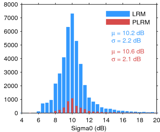
Figure 25. Histogram of flag-valid sigma0 over oceans and lakes for LRM (blue) and PLRM (red) for 02/10/2015. The mean ( \mu ) and standard deviation ( \sigma ) are also shown. Note that values outside [4 20] dB are excluded from the histogram for the sake of readability but not from the computation of \mu and \sigma .
