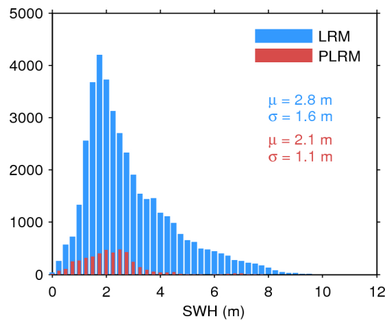
Figure 20. Histogram of science-valid SWH over oceans and lakes for LRM (blue) and PLRM (red) for 02/10/2015. The mean ( \mu ) and standard deviation ( \sigma ) are also shown. Note that values larger than 12 m are excluded from the histogram for the sake of readability but not from the computation of \mu and \sigma .
