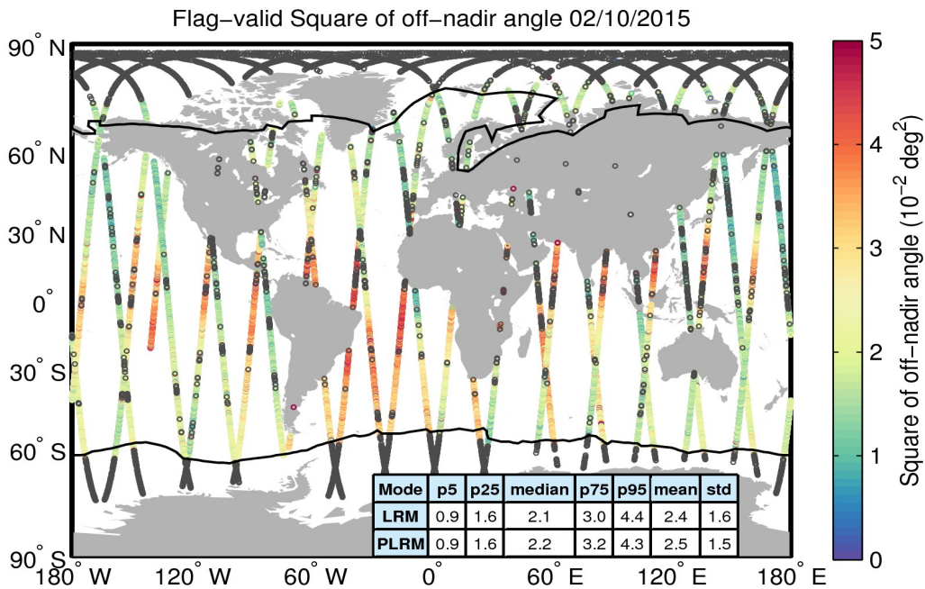
Figure 37. Geographical distribution of flag-valid mispointing data over oceans and lakes for 02/10/2015. The statistical values shown in the table refer to the mispointing in 10^{-2} deg 2 and are calculated separately for LRM and PLRM regions. Measurements taken over polar polygons have been excluded from the computation of the statistical values. The black lines mark the outer limit of the Arctic and Antarctic polar polygons. Gray circles denote negative values.
