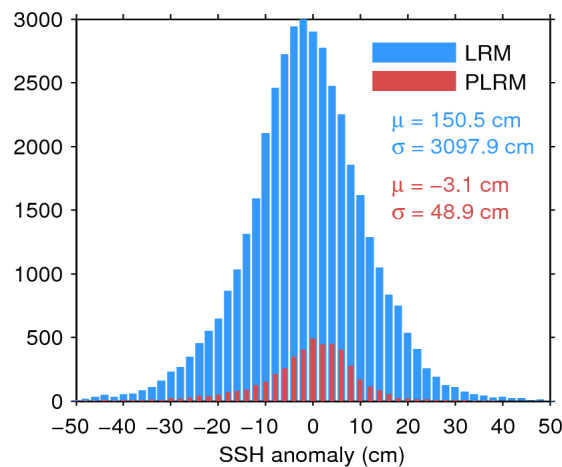
Figure 7. Histogram of flag-valid SSH anomaly over oceans and lakes for LRM (blue) and PLRM (red) for 02/10/2015. The mean ( \mu ) and standard deviation ( \sigma ) are also shown. Note that values outside [-50 50] cm are excluded from the histogram for the sake of readability but not from the computation of \mu and \sigma .
