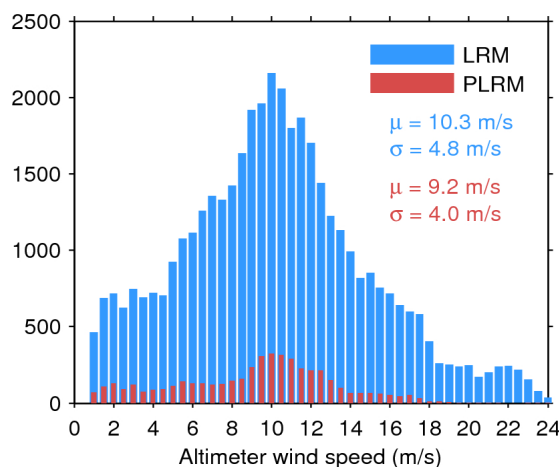
Figure 33. Histogram of flag-valid wind over oceans and lakes for LRM (blue) and PLRM (red) for 02/10/2015. The mean ( \mu ) and standard deviation ( \sigma ) are also shown. Note that values larger than 24 m/s are excluded from the histogram for the sake of readability but not from the computation of \mu and \sigma .
