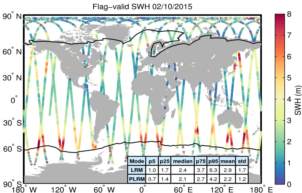
Figure 15. Geographical distribution of flag-valid SWH data over oceans and lakes for 02/10/2015. The statistical values shown in the table refer to the SWH in m and are calculated separately for LRM and PLRM regions. Measurements taken over polar polygons have been excluded from the computation of the statistical values. The black lines mark the outer limit of the Arctic and Antarctic polar polygons.
