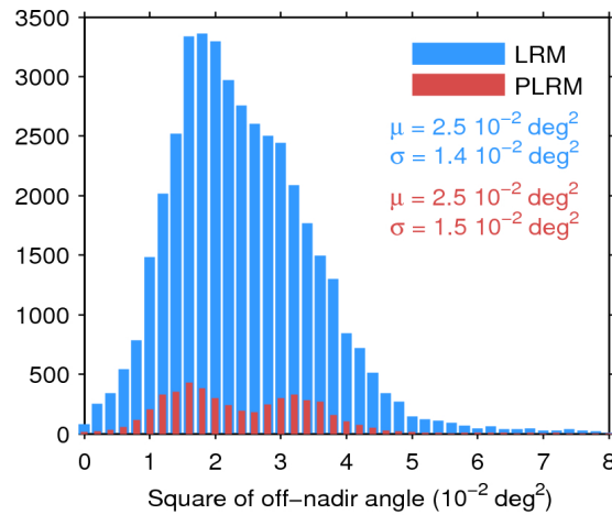
Figure 39. Histogram of flag-valid mispointing over oceans and lakes for LRM (blue) and PLRM (red) for 28/09/2015. Only positive values have been considered. The mean ( \mu ) and standard deviation ( \sigma ) are also shown. Note that values larger than 8 \cdot 10^{-2} \text{ deg}^2 are excluded from the histogram for the sake of readability but not from the computation of \mu and \sigma .
