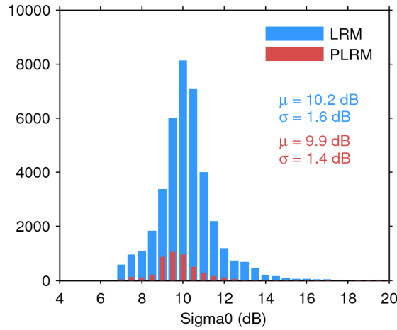
Figure 28. Histogram of science-valid sigma0 over oceans and lakes for LRM (blue) and PLRM (red) for 28/09/2015. The mean ( \mu ) and standard deviation ( \sigma ) are also shown. Note that values outside [4 20] dB are excluded from the histogram for the sake of readability but not from the computation of \mu and \sigma .
