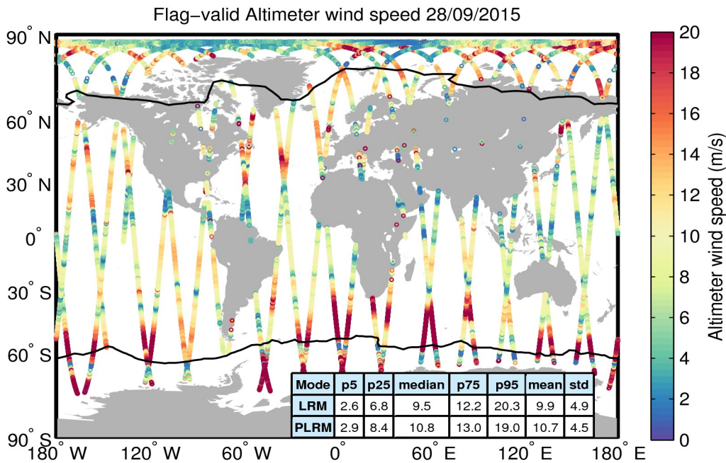
Figure 31. Geographical distribution of flag-valid wind data over oceans and lakes for 28/09/2015. The statistical values shown in the table refer to the wind in m/s and are calculated separately for LRM and PLRM regions. Measurements taken over polar polygons have been excluded from the computation of the statistical values. The black lines mark the outer limit of the Arctic and Antarctic polar polygons.
