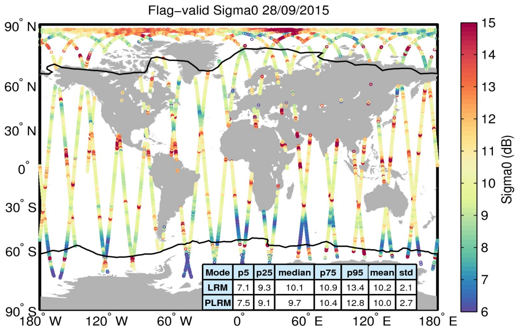
Figure 23. Geographical distribution of flag-valid sigma0 data over oceans and lakes for 28/09/2015. The statistical values shown in the table refer to the sigma0 in dB and are calculated separately for LRM and PLRM regions. Measurements taken over polar polygons have been excluded from the computation of the statistical values. The black lines mark the outer limit of the Arctic and Antarctic polar polygons.
