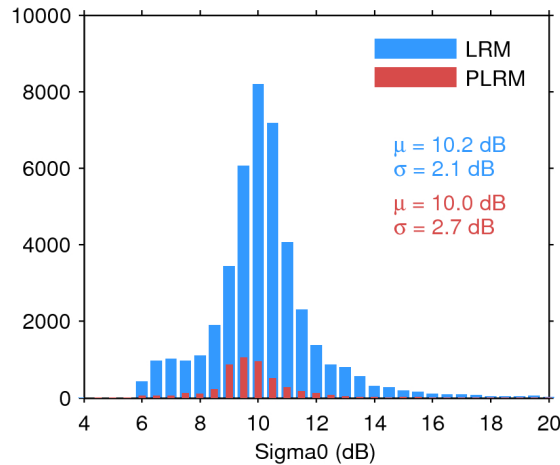
Figure 25. Histogram of flag-valid sigma0 over oceans and lakes for LRM (blue) and PLRM (red) for 28/09/2015. The mean ( \mu ) and standard deviation ( \sigma ) are also shown. Note that values outside [4 20] dB are excluded from the histogram for the sake of readability but not from the computation of \mu and \sigma .
