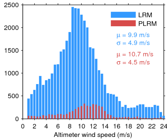
Figure 33. Histogram of flag-valid wind over oceans and lakes for LRM (blue) and PLRM (red) for 28/09/2015. The mean ( \mu ) and standard deviation ( \sigma ) are also shown. Note that values larger than 24 m/s are excluded from the histogram for the sake of readability but not from the computation of \mu and \sigma .
