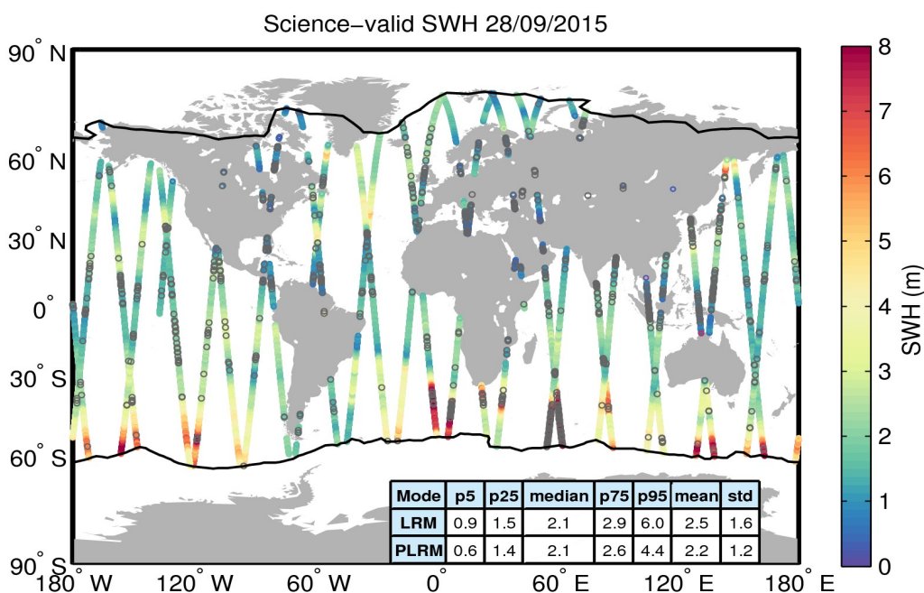
Figure 19. Geographical distribution of science-valid SWH data over oceans and lakes for 28/09/2015. The statistical values shown in the table refer to the SWH in m and are calculated separately for LRM and PLRM regions. The black lines mark the outer limit of the Arctic and Antarctic polar polygons. Gray circles denote records that have been rejected based on the editing criteria described in Table 3.
