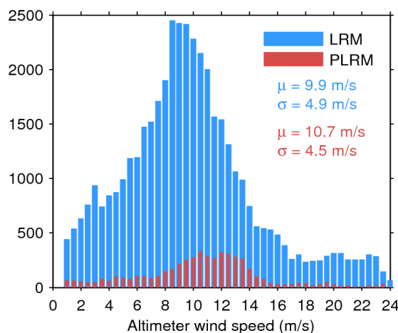
Figure 35. Histogram of science-valid wind over oceans and lakes for LRM (blue) and PLRM (red) for 28/09/2015. The mean ( \mu ) and standard deviation ( \sigma ) are also shown. Note that values larger than 24 m/s are excluded from the histogram for the sake of readability but not from the computation of \mu and \sigma .
