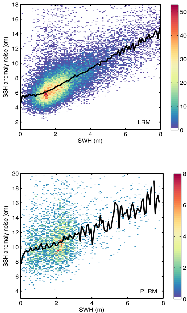
Figure 9. 2D histogram showing flag-valid SSH anomaly noise as a function of SWH for LRM (top) and PLRM (bottom) for 28/09/2015. The black line denotes the median SSH anomaly noise as a function of SWH.
