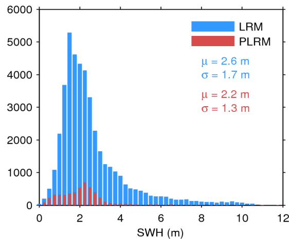
Figure 17. Histogram of flag-valid SWH over oceans and lakes for LRM (blue) and PLRM (red) for 28/09/2015. The mean ( \mu ) and standard deviation ( \sigma ) are also shown. Note that values larger than 12 m are excluded from the histogram for the sake of readability but not from the computation of \mu and \sigma .
