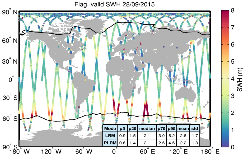
Figure 15. Geographical distribution of flag-valid SWH data over oceans and lakes for 28/09/2015. The statistical values shown in the table refer to the SWH in m and are calculated separately for LRM and PLRM regions. Measurements taken over polar polygons have been excluded from the computation of the statistical values. The black lines mark the outer limit of the Arctic and Antarctic polar polygons.
