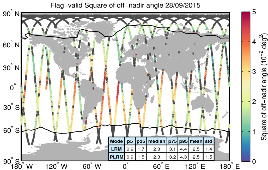
Figure 37. Geographical distribution of flag-valid mispointing data over oceans and lakes for 28/09/2015. The statistical values shown in the table refer to the mispointing in 10^{-2} \text{ deg}^2 and are calculated separately for LRM and PLRM regions. Measurements taken over polar polygons have been excluded from the computation of the statistical values. The black lines mark the outer limit of the Arctic and Antarctic polar polygons. Gray circles denote negative values.
