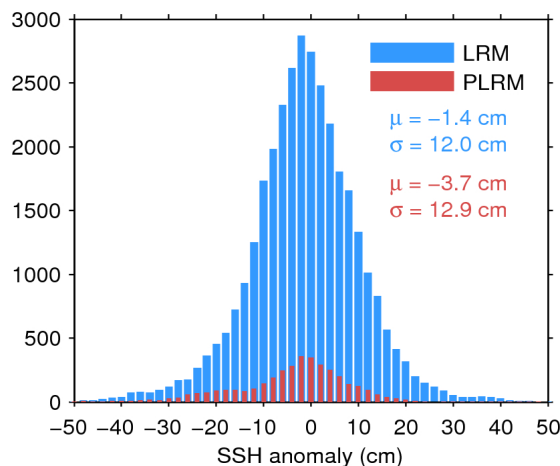
Figure 11. Histogram of science-valid SSH anomaly over oceans and lakes for LRM (blue) and PLRM (red) for 28/09/2015. The mean ( \mu ) and standard deviation ( \sigma ) are also shown. Note that values outside [-50 50] cm are excluded from the histogram for the sake of readability but not from the computation of \mu and \sigma .
