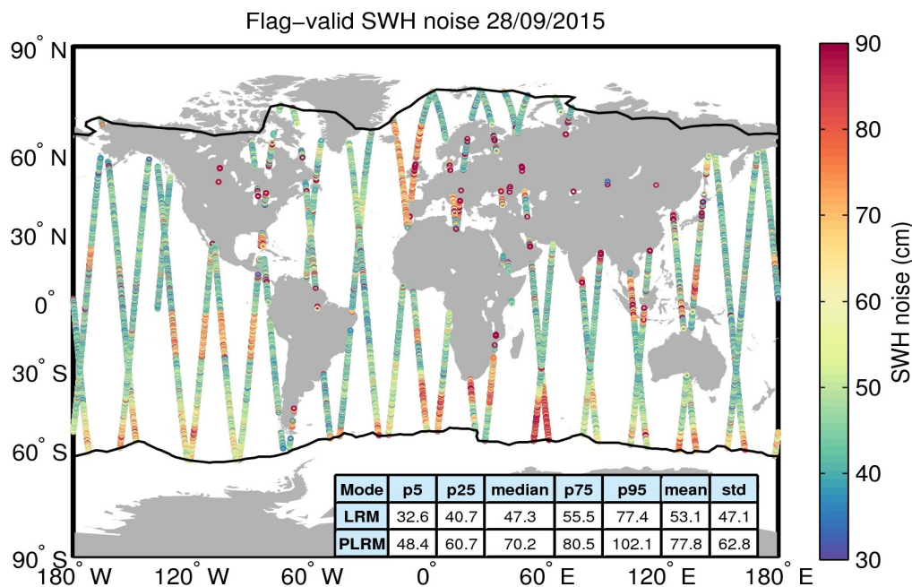
Figure 18. Geographical distribution of flag-valid 20-Hz SWH measurement noise over oceans and lakes for 28/09/2015. The statistical values shown in the table refer to the SWH noise and are calculated separately for LRM and PLRM regions. Measurements taken over polar polygons have been excluded from the computation of the statistical values. The black lines mark the outer limit of the Arctic and Antarctic polar polygons.
