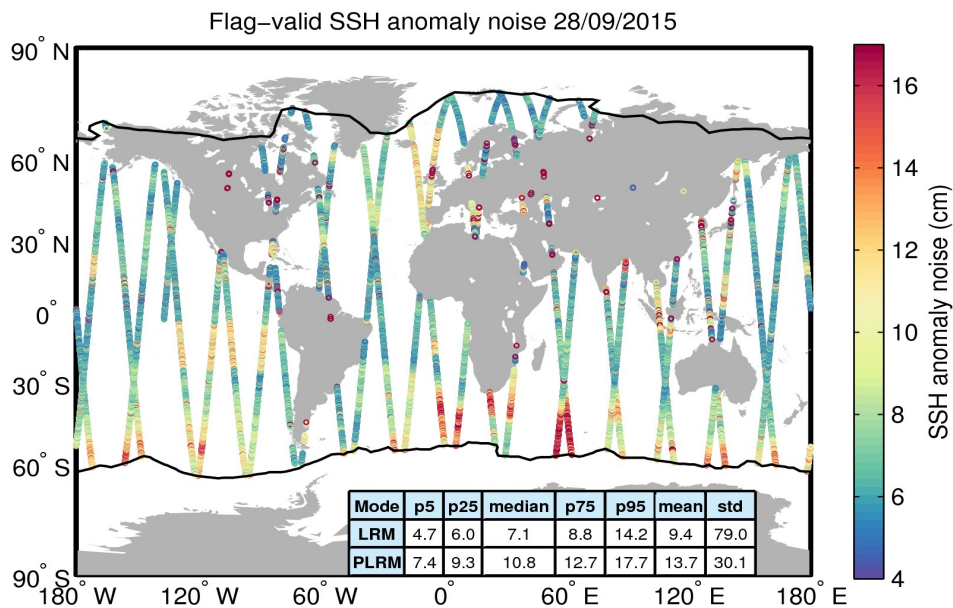
Figure 8. Geographical distribution of flag-valid 20-Hz SSH anomaly measurement noise over oceans and lakes for 28/09/2015. The statistical values shown in the table refer to the SSH anomaly noise and are calculated separately for LRM and PLRM regions. Measurements taken over polar polygons have been excluded from the computation of the statistical values. The black lines mark the outer limit of the Arctic and Antarctic polar polygons.
