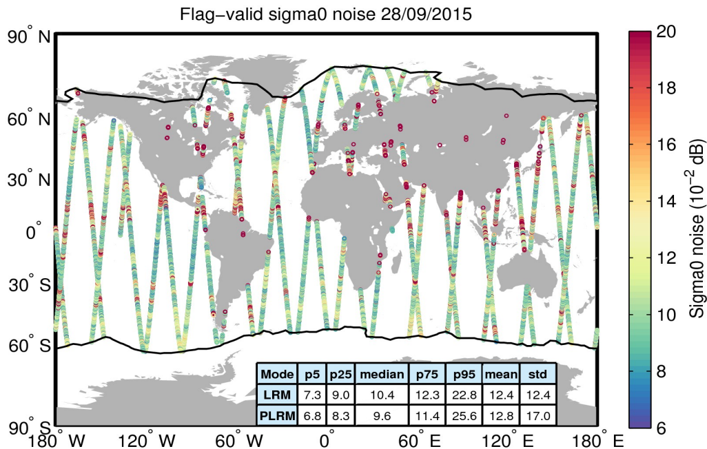
Figure 26. Geographical distribution of flag-valid 20-Hz sigma0 measurement noise over oceans and lakes for 28/09/2015. The statistical values shown in the table refer to the sigma0 noise and are calculated separately for LRM and PLRM regions. Measurements taken over polar polygons have been excluded from the computation of the statistical values. The black lines mark the outer limit of the Arctic and Antarctic polar polygons.
