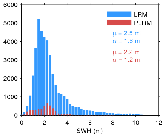
Figure 20. Histogram of science-valid SWH over oceans and lakes for LRM (blue) and PLRM (red) for 28/09/2015. The mean ( \mu ) and standard deviation ( \sigma ) are also shown. Note that values larger than 12 m are excluded from the histogram for the sake of readability but not from the computation of \mu and \sigma .
