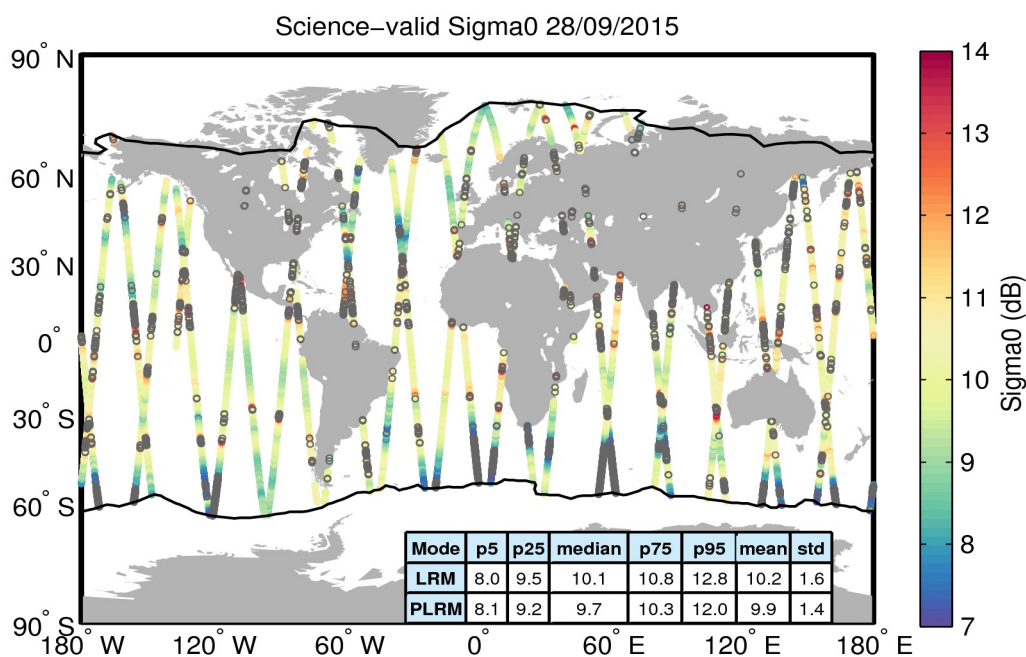
Figure 27. Geographical distribution of science-valid sigma0 data over oceans and lakes for 28/09/2015. The statistical values shown in the table refer to the sigma0 in dB and are calculated separately for LRM and PLRM regions. The black lines mark the outer limit of the Arctic and Antarctic polar polygons. Gray circles denote records that have been rejected based on the editing criteria described in Table 4.
