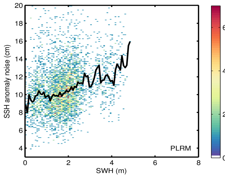
Figure 9. 2D histogram showing flag-valid SSH anomaly noise as a function of SWH for LRM (top) and PLRM (bottom) for 20/09/2015. The black line denotes the median SSH anomaly noise as a function of SWH.
