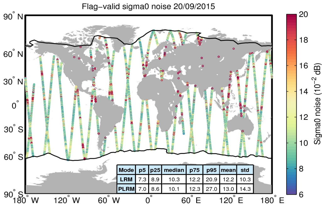
Figure 26. Geographical distribution of flag-valid 20-Hz sigma0 measurement noise over oceans and lakes for 20/09/2015. The statistical values shown in the table refer to the sigma0 noise and are calculated separately for LRM and PLRM regions. Measurements taken over polar polygons have been excluded from the computation of the statistical values. The black lines mark the outer limit of the Arctic and Antarctic polar polygons.
