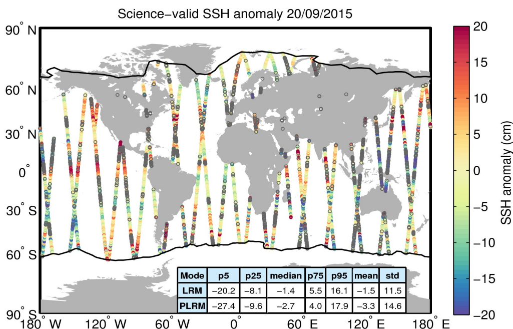
Figure 10. Geographical distribution of science-valid SSH anomaly data over oceans and lakes for 20/09/2015. The statistical values shown in the table refer to the SSH anomaly in cm and are calculated separately for LRM and PLRM regions. The black lines mark the outer limit of the Arctic and Antarctic polar polygons. Gray circles denote records that have been rejected based on the editing criteria described in Table 2.
