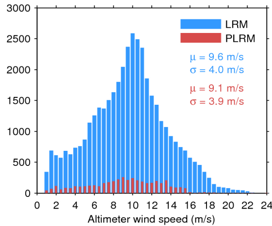
Figure 33. Histogram of flag-valid wind over oceans and lakes for LRM (blue) and PLRM (red) for 20/09/2015. The mean ( \mu ) and standard deviation ( \sigma ) are also shown. Note that values larger than 24 m/s are excluded from the histogram for the sake of readability but not from the computation of \mu and \sigma .
