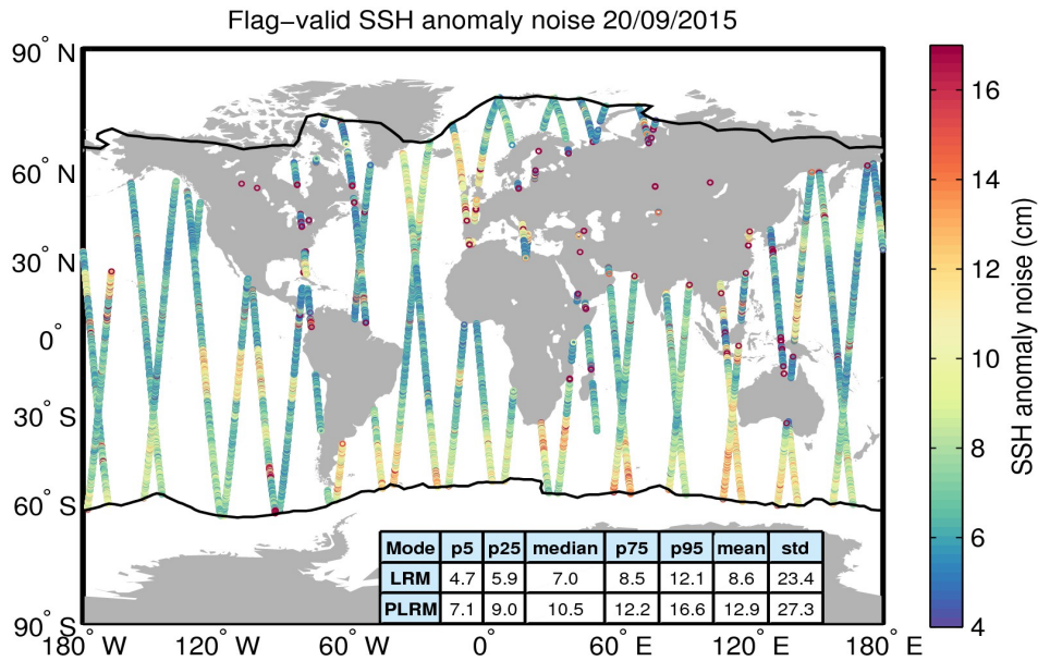
Figure 8. Geographical distribution of flag-valid 20-Hz SSH anomaly measurement noise over oceans and lakes for 20/09/2015. The statistical values shown in the table refer to the SSH anomaly noise and are calculated separately for LRM and PLRM regions. Measurements taken over polar polygons have been excluded from the computation of the statistical values. The black lines mark the outer limit of the Arctic and Antarctic polar polygons.
