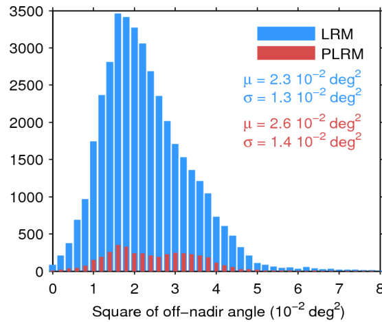
Figure 39. Histogram of flag-valid mispointing over oceans and lakes for LRM (blue) and PLRM (red) for 20/09/2015. Only positive values have been considered. The mean ( \mu ) and standard deviation ( \sigma ) are also shown. Note that values larger than 8 \cdot 10^{-2} \text{ deg}^2 are excluded from the histogram for the sake of readability but not from the computation of \mu and \sigma .
