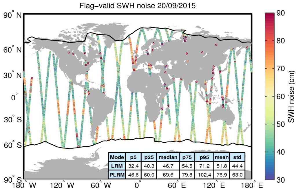
Figure 18. Geographical distribution of flag-valid 20-Hz SWH measurement noise over oceans and lakes for 20/09/2015. The statistical values shown in the table refer to the SWH noise and are calculated separately for LRM and PLRM regions. Measurements taken over polar polygons have been excluded from the computation of the statistical values. The black lines mark the outer limit of the Arctic and Antarctic polar polygons.
