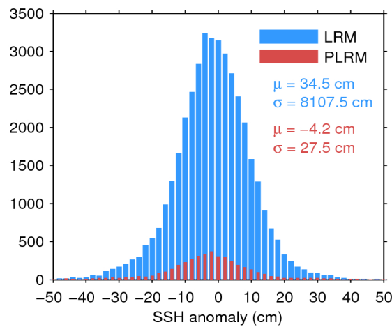
Figure 7. Histogram of flag-valid SSH anomaly over oceans and lakes for LRM (blue) and PLRM (red) for 20/09/2015. The mean ( \mu ) and standard deviation ( \sigma ) are also shown. Note that values outside [-50 50] cm are excluded from the histogram for the sake of readability but not from the computation of \mu and \sigma .
