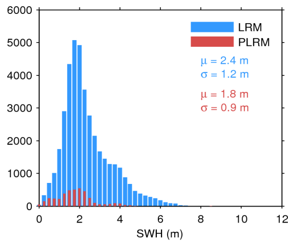
Figure 20. Histogram of science-valid SWH over oceans and lakes for LRM (blue) and PLRM (red) for 20/09/2015. The mean ( \mu ) and standard deviation ( \sigma ) are also shown. Note that values larger than 12 m are excluded from the histogram for the sake of readability but not from the computation of \mu and \sigma .
