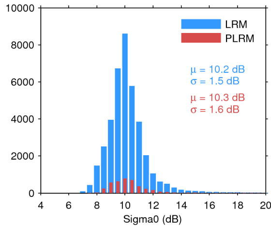
Figure 28. Histogram of science-valid sigma0 over oceans and lakes for LRM (blue) and PLRM (red) for 20/09/2015. The mean ( \mu ) and standard deviation ( \sigma ) are also shown. Note that values outside [4 20] dB are excluded from the histogram for the sake of readability but not from the computation of \mu and \sigma .
