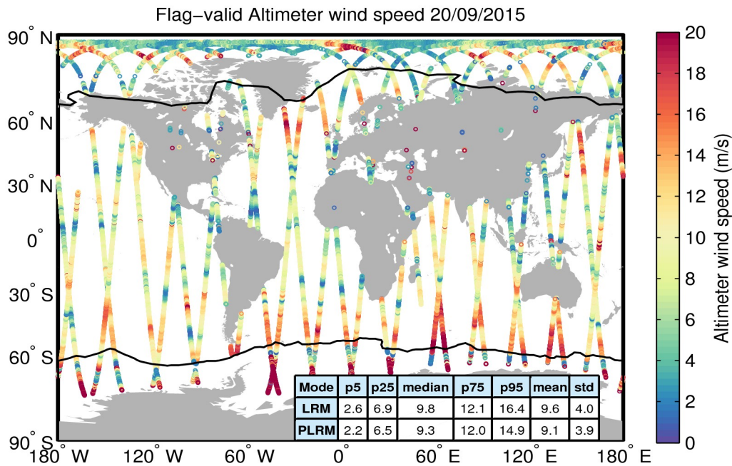
Figure 31. Geographical distribution of flag-valid wind data over oceans and lakes for 20/09/2015. The statistical values shown in the table refer to the wind in m/s and are calculated separately for LRM and PLRM regions. Measurements taken over polar polygons have been excluded from the computation of the statistical values. The black lines mark the outer limit of the Arctic and Antarctic polar polygons.
