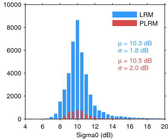
Figure 25. Histogram of flag-valid sigma0 over oceans and lakes for LRM (blue) and PLRM (red) for 20/09/2015. The mean ( \mu ) and standard deviation ( \sigma ) are also shown. Note that values outside [4 20] dB are excluded from the histogram for the sake of readability but not from the computation of \mu and \sigma .
