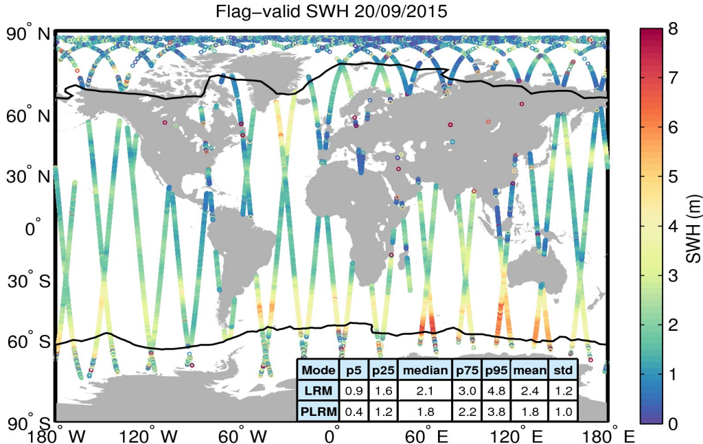
Figure 15. Geographical distribution of flag-valid SWH data over oceans and lakes for 20/09/2015. The statistical values shown in the table refer to the SWH in m and are calculated separately for LRM and PLRM regions. Measurements taken over polar polygons have been excluded from the computation of the statistical values. The black lines mark the outer limit of the Arctic and Antarctic polar polygons.
