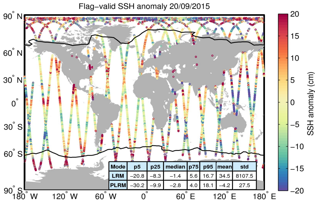
Figure 5. Geographical distribution of flag-valid 1-Hz SSH anomaly data over oceans and lakes for 20/09/2015. The statistical values shown in the table refer to the SSH anomaly in cm and are calculated separately for LRM and PLRM regions. Measurements taken over polar polygons have been excluded from the computation of the statistical values. The black lines mark the outer limit of the Arctic and Antarctic polar polygons.
