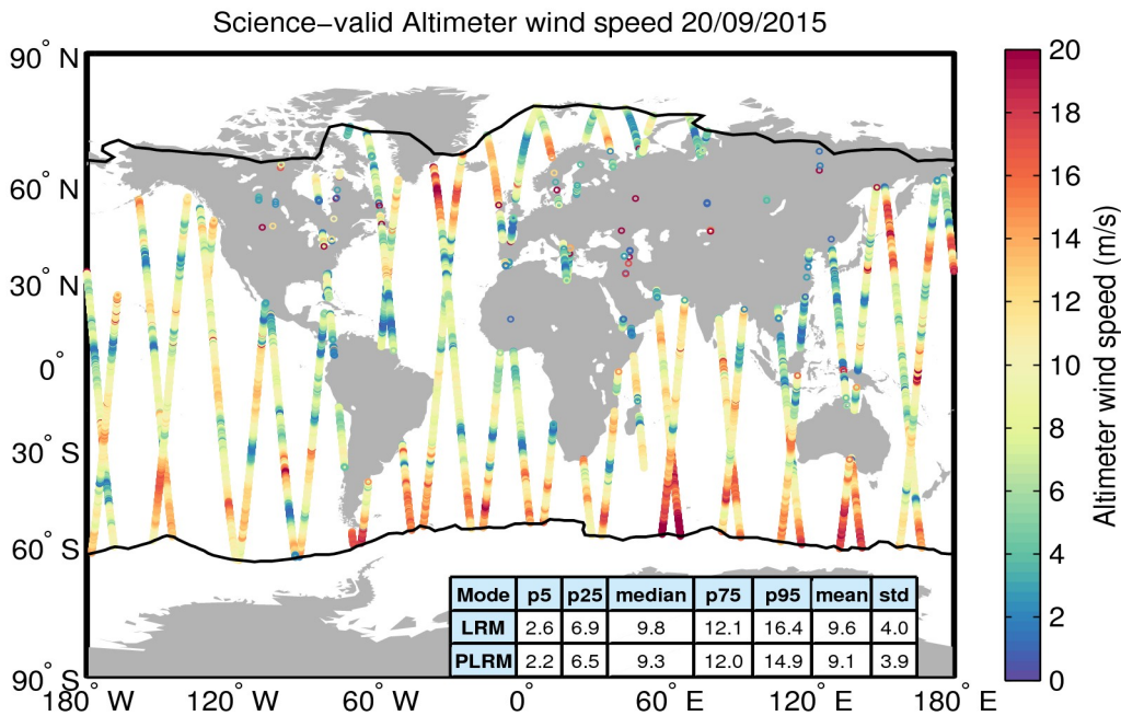
Figure 34. Geographical distribution of science-valid wind data over oceans and lakes for 20/09/2015. The statistical values shown in the table refer to the wind in m/s and are calculated separately for LRM and PLRM regions. The black lines mark the outer limit of the Arctic and Antarctic polar polygons. Gray circles denote records that have been rejected based on the editing criteria described in Table 5.
