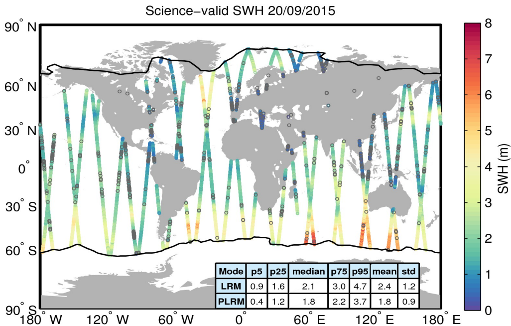
Figure 19. Geographical distribution of science-valid SWH data over oceans and lakes for 20/09/2015. The statistical values shown in the table refer to the SWH in m and are calculated separately for LRM and PLRM regions. The black lines mark the outer limit of the Arctic and Antarctic polar polygons. Gray circles denote records that have been rejected based on the editing criteria described in Table 3.
