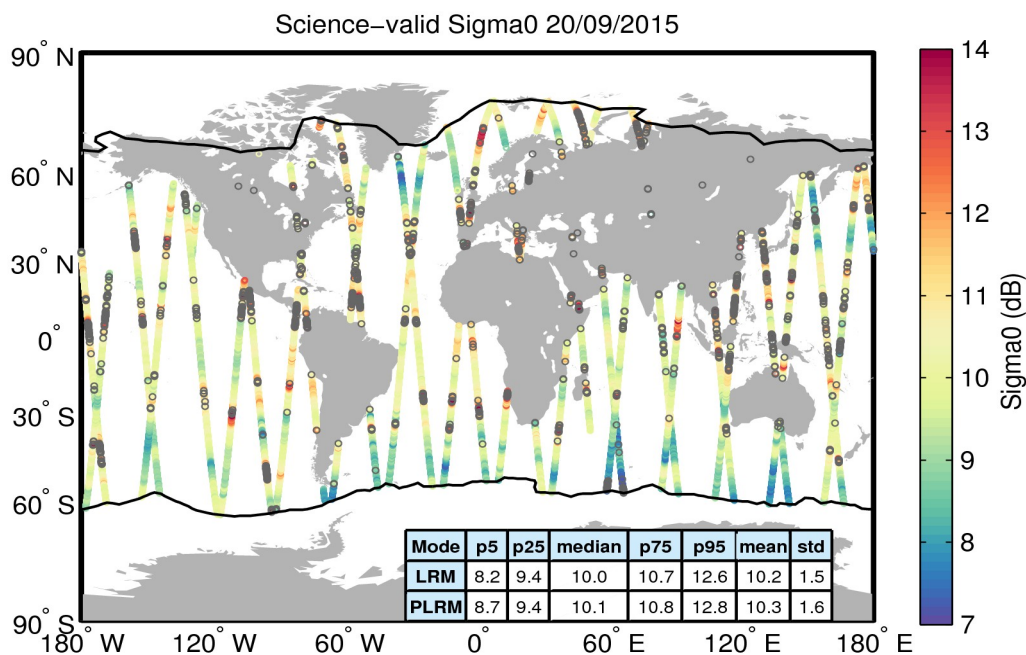
Figure 27. Geographical distribution of science-valid sigma0 data over oceans and lakes for 20/09/2015. The statistical values shown in the table refer to the sigma0 in dB and are calculated separately for LRM and PLRM regions. The black lines mark the outer limit of the Arctic and Antarctic polar polygons. Gray circles denote records that have been rejected based on the editing criteria described in Table 4.
