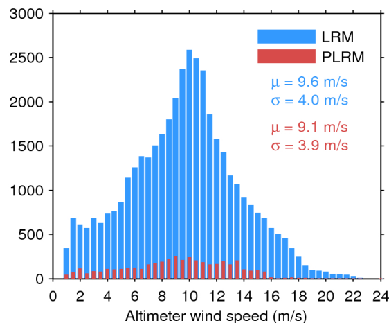
Figure 35. Histogram of science-valid wind over oceans and lakes for LRM (blue) and PLRM (red) for 20/09/2015. The mean ( \mu ) and standard deviation ( \sigma ) are also shown. Note that values larger than 24 m/s are excluded from the histogram for the sake of readability but not from the computation of \mu and \sigma .
