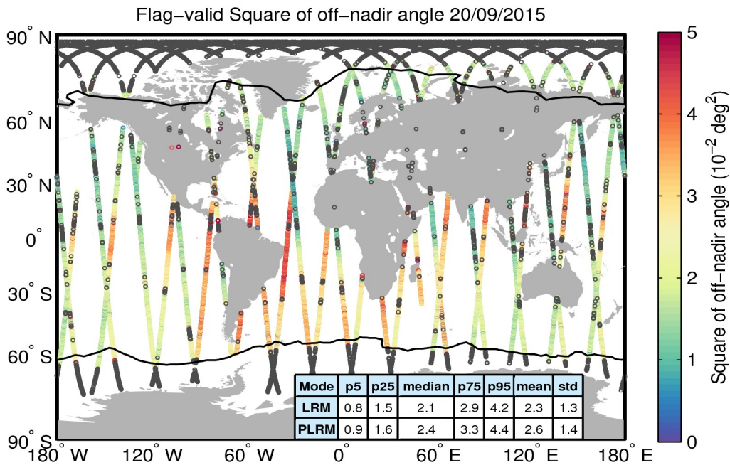
Figure 37. Geographical distribution of flag-valid mispointing data over oceans and lakes for 20/09/2015. The statistical values shown in the table refer to the mispointing in 10^{-2} deg 2 and are calculated separately for LRM and PLRM regions. Measurements taken over polar polygons have been excluded from the computation of the statistical values. The black lines mark the outer limit of the Arctic and Antarctic polar polygons. Gray circles denote negative values.
