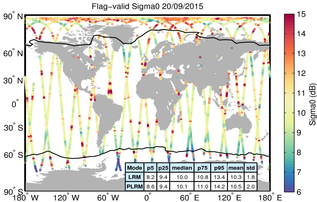
Figure 23. Geographical distribution of flag-valid sigma0 data over oceans and lakes for 20/09/2015. The statistical values shown in the table refer to the sigma0 in dB and are calculated separately for LRM and PLRM regions. Measurements taken over polar polygons have been excluded from the computation of the statistical values. The black lines mark the outer limit of the Arctic and Antarctic polar polygons.
