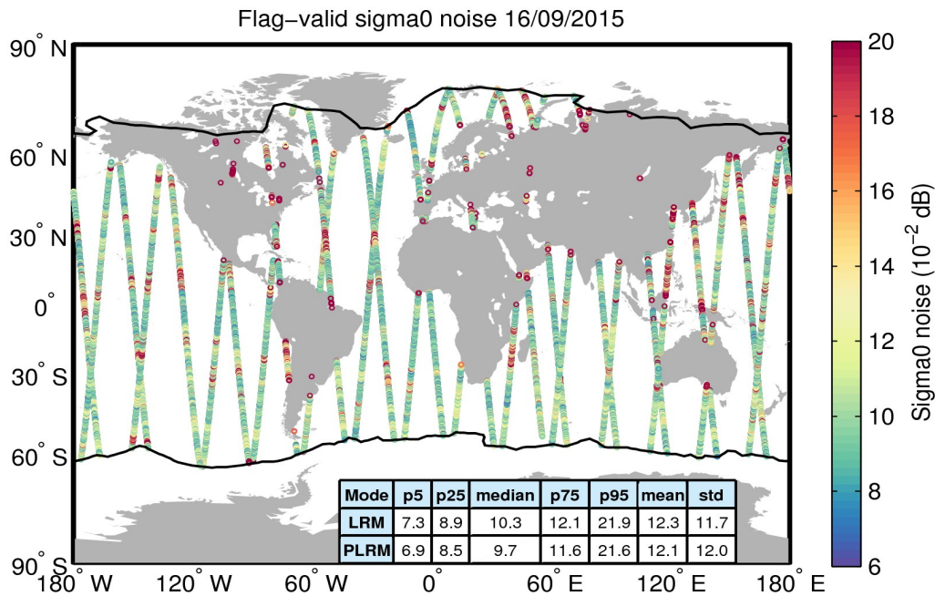
Figure 26. Geographical distribution of flag-valid 20-Hz sigma0 measurement noise over oceans and lakes for 16/09/2015. The statistical values shown in the table refer to the sigma0 noise and are calculated separately for LRM and PLRM regions. Measurements taken over polar polygons have been excluded from the computation of the statistical values. The black lines mark the outer limit of the Arctic and Antarctic polar polygons.
