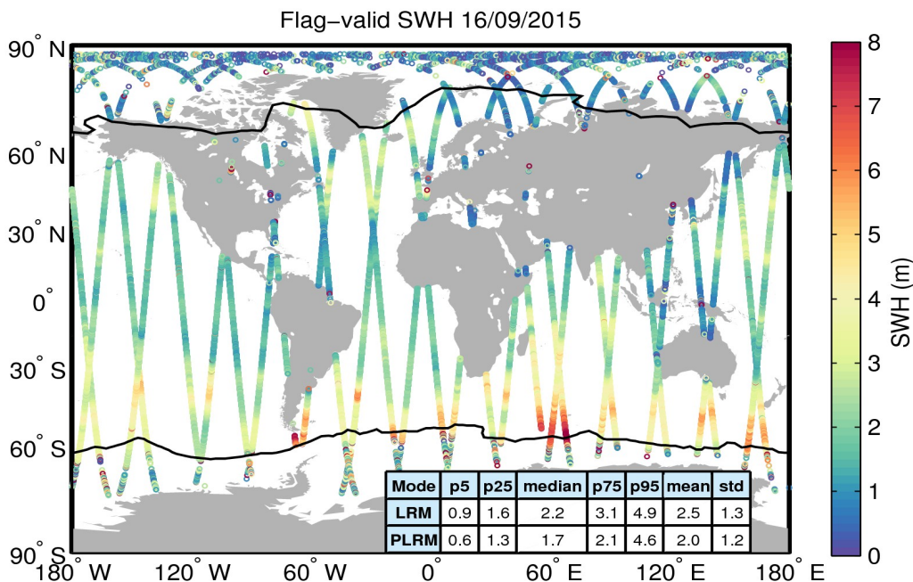
Figure 15. Geographical distribution of flag-valid SWH data over oceans and lakes for 16/09/2015. The statistical values shown in the table refer to the SWH in m and are calculated separately for LRM and PLRM regions. Measurements taken over polar polygons have been excluded from the computation of the statistical values. The black lines mark the outer limit of the Arctic and Antarctic polar polygons.
