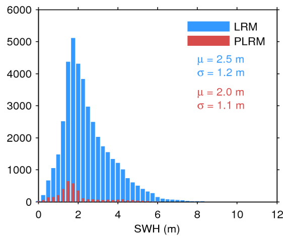
Figure 20. Histogram of science-valid SWH over oceans and lakes for LRM (blue) and PLRM (red) for 16/09/2015. The mean ( \mu ) and standard deviation ( \sigma ) are also shown. Note that values larger than 12 m are excluded from the histogram for the sake of readability but not from the computation of \mu and \sigma .
