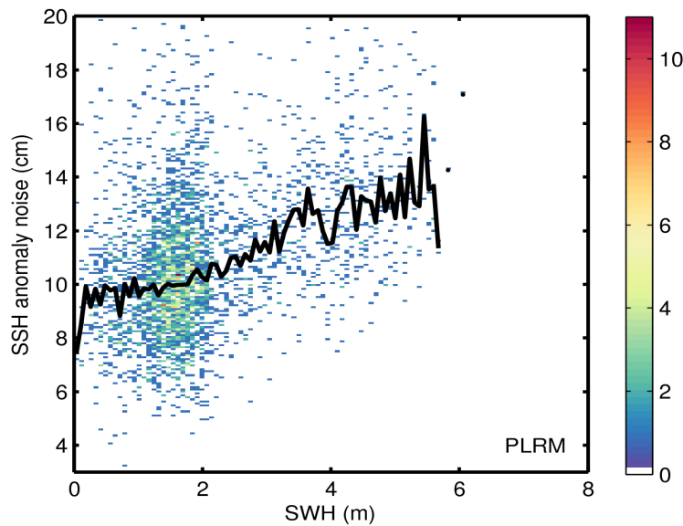
Figure 9. 2D histogram showing flag-valid SSH anomaly noise as a function of SWH for LRM (top) and PLRM (bottom) for 16/09/2015. The black line denotes the median SSH anomaly noise as a function of SWH.
