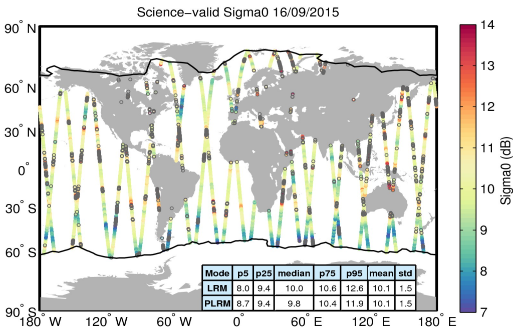
Figure 27. Geographical distribution of science-valid sigma0 data over oceans and lakes for 16/09/2015. The statistical values shown in the table refer to the sigma0 in dB and are calculated separately for LRM and PLRM regions. The black lines mark the outer limit of the Arctic and Antarctic polar polygons. Gray circles denote records that have been rejected based on the editing criteria described in Table 4.
