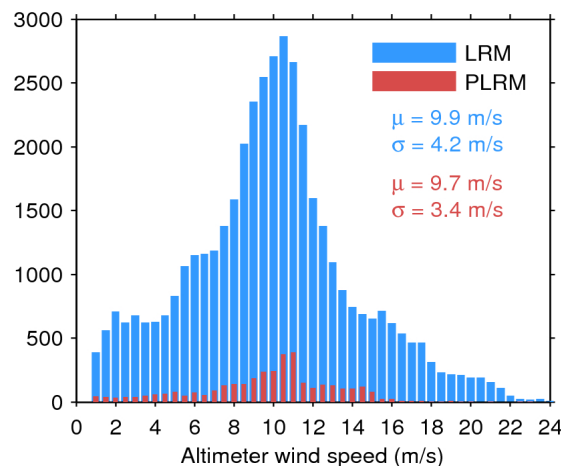
Figure 35. Histogram of science-valid wind over oceans and lakes for LRM (blue) and PLRM (red) for 16/09/2015. The mean ( \mu ) and standard deviation ( \sigma ) are also shown. Note that values larger than 24 m/s are excluded from the histogram for the sake of readability but not from the computation of \mu and \sigma .
