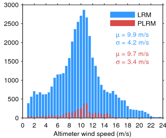
Figure 33. Histogram of flag-valid wind over oceans and lakes for LRM (blue) and PLRM (red) for 16/09/2015. The mean ( \mu ) and standard deviation ( \sigma ) are also shown. Note that values larger than 24 m/s are excluded from the histogram for the sake of readability but not from the computation of \mu and \sigma .
