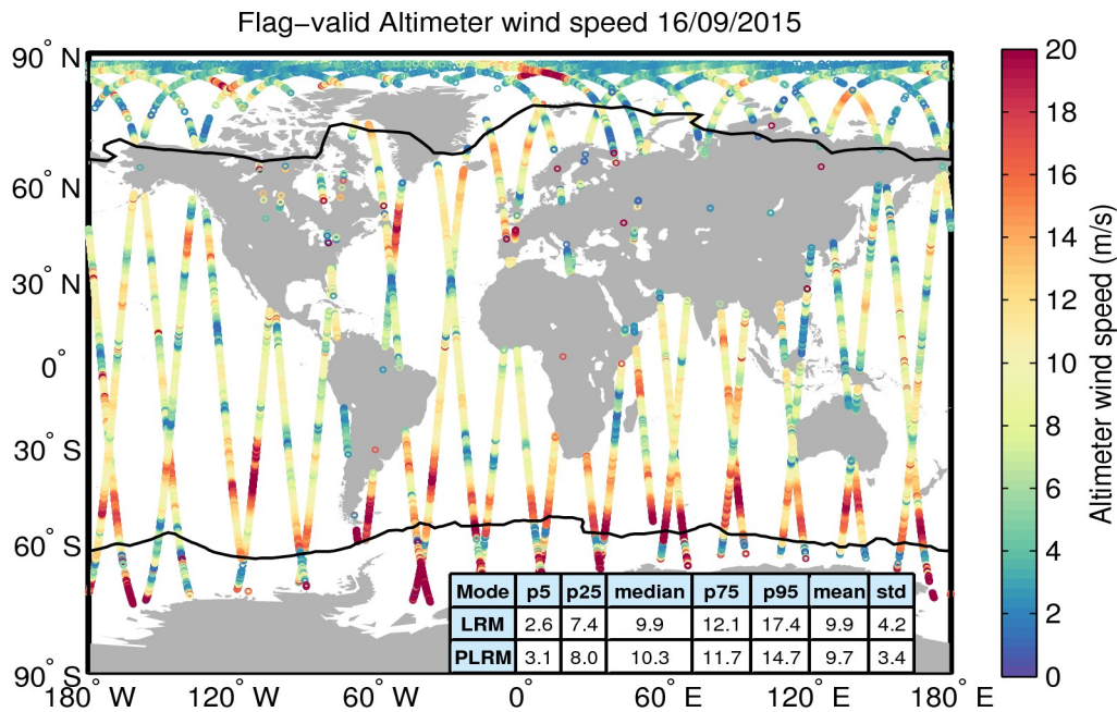
Figure 31. Geographical distribution of flag-valid wind data over oceans and lakes for 16/09/2015. The statistical values shown in the table refer to the wind in m/s and are calculated separately for LRM and PLRM regions. Measurements taken over polar polygons have been excluded from the computation of the statistical values. The black lines mark the outer limit of the Arctic and Antarctic polar polygons.
