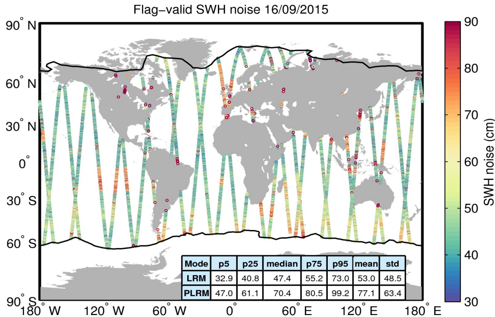
Figure 18. Geographical distribution of flag-valid 20-Hz SWH measurement noise over oceans and lakes for 16/09/2015. The statistical values shown in the table refer to the SWH noise and are calculated separately for LRM and PLRM regions. Measurements taken over polar polygons have been excluded from the computation of the statistical values. The black lines mark the outer limit of the Arctic and Antarctic polar polygons.
