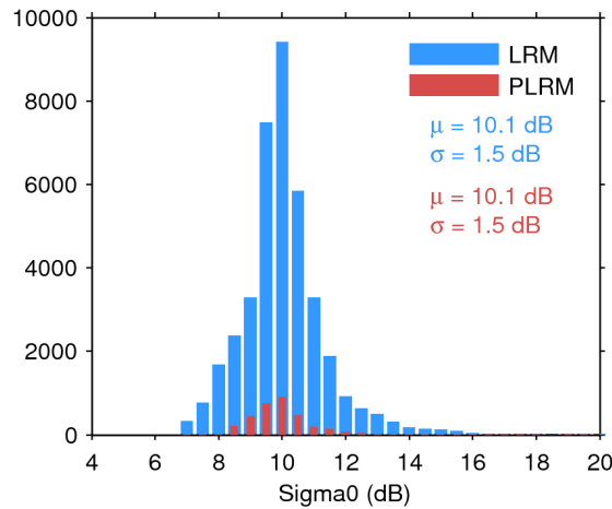
Figure 28. Histogram of science-valid sigma0 over oceans and lakes for LRM (blue) and PLRM (red) for 16/09/2015. The mean ( \mu ) and standard deviation ( \sigma ) are also shown. Note that values outside [4 20] dB are excluded from the histogram for the sake of readability but not from the computation of \mu and \sigma .
