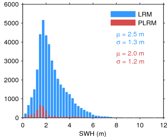
Figure 17. Histogram of flag-valid SWH over oceans and lakes for LRM (blue) and PLRM (red) for 16/09/2015. The mean ( \mu ) and standard deviation ( \sigma ) are also shown. Note that values larger than 12 m are excluded from the histogram for the sake of readability but not from the computation of \mu and \sigma .
