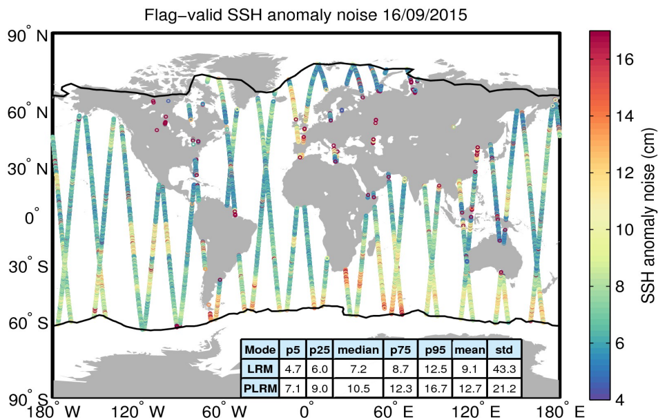
Figure 8. Geographical distribution of flag-valid 20-Hz SSH anomaly measurement noise over oceans and lakes for 16/09/2015. The statistical values shown in the table refer to the SSH anomaly noise and are calculated separately for LRM and PLRM regions. Measurements taken over polar polygons have been excluded from the computation of the statistical values. The black lines mark the outer limit of the Arctic and Antarctic polar polygons.
