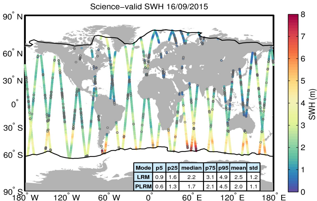
Figure 19. Geographical distribution of science-valid SWH data over oceans and lakes for 16/09/2015. The statistical values shown in the table refer to the SWH in m and are calculated separately for LRM and PLRM regions. The black lines mark the outer limit of the Arctic and Antarctic polar polygons. Gray circles denote records that have been rejected based on the editing criteria described in Table 3.
