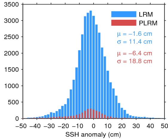
Figure 11. Histogram of science-valid SSH anomaly over oceans and lakes for LRM (blue) and PLRM (red) for 16/09/2015. The mean ( \mu ) and standard deviation ( \sigma ) are also shown. Note that values outside [-50 50] cm are excluded from the histogram for the sake of readability but not from the computation of \mu and \sigma .
