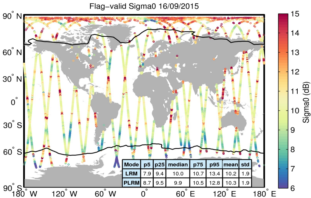
Figure 23. Geographical distribution of flag-valid sigma0 data over oceans and lakes for 16/09/2015. The statistical values shown in the table refer to the sigma0 in dB and are calculated separately for LRM and PLRM regions. Measurements taken over polar polygons have been excluded from the computation of the statistical values. The black lines mark the outer limit of the Arctic and Antarctic polar polygons.
