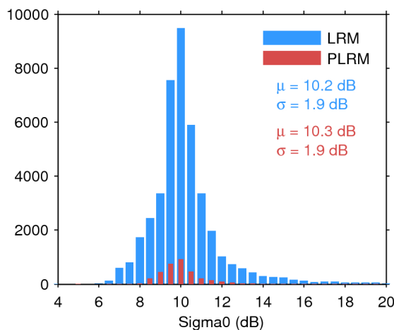
Figure 25. Histogram of flag-valid sigma0 over oceans and lakes for LRM (blue) and PLRM (red) for 16/09/2015. The mean ( \mu ) and standard deviation ( \sigma ) are also shown. Note that values outside [4 20] dB are excluded from the histogram for the sake of readability but not from the computation of \mu and \sigma .
