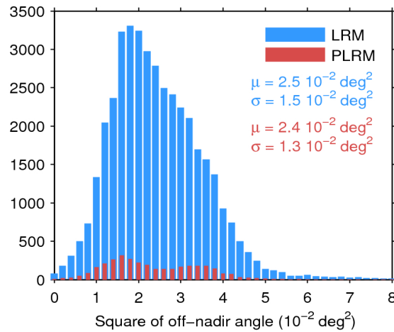
Figure 39. Histogram of flag-valid mispointing over oceans and lakes for LRM (blue) and PLRM (red) for 16/09/2015. Only positive values have been considered. The mean ( \mu ) and standard deviation ( \sigma ) are also shown. Note that values larger than 8 \cdot 10^{-2} \text{ deg}^2 are excluded from the histogram for the sake of readability but not from the computation of \mu and \sigma .
