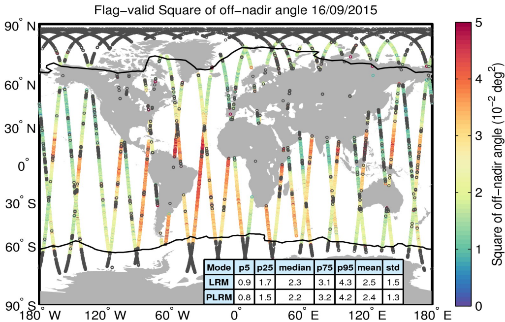
Figure 37. Geographical distribution of flag-valid mispointing data over oceans and lakes for 16/09/2015. The statistical values shown in the table refer to the mispointing in 10^{-2} deg 2 and are calculated separately for LRM and PLRM regions. Measurements taken over polar polygons have been excluded from the computation of the statistical values. The black lines mark the outer limit of the Arctic and Antarctic polar polygons. Gray circles denote negative values.
