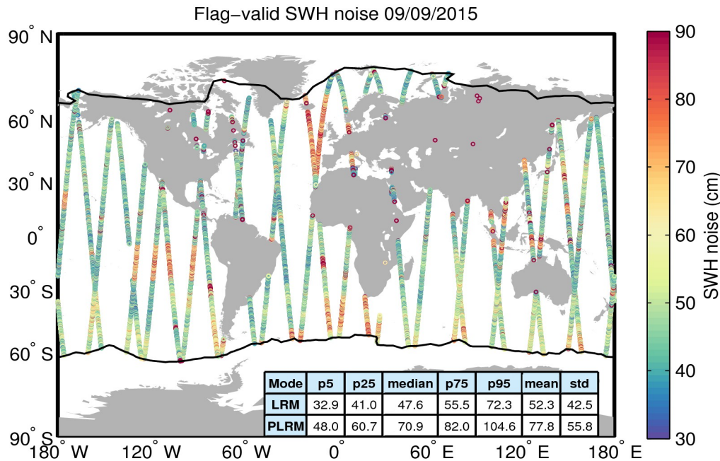
Figure 18. Geographical distribution of flag-valid 20-Hz SWH measurement noise over oceans and lakes for 09/09/2015. The statistical values shown in the table refer to the SWH noise and are calculated separately for LRM and PLRM regions. Measurements taken over polar polygons have been excluded from the computation of the statistical values. The black lines mark the outer limit of the Arctic and Antarctic polar polygons.
