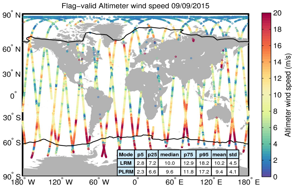
Figure 31. Geographical distribution of flag-valid wind data over oceans and lakes for 09/09/2015. The statistical values shown in the table refer to the wind in m/s and are calculated separately for LRM and PLRM regions. Measurements taken over polar polygons have been excluded from the computation of the statistical values. The black lines mark the outer limit of the Arctic and Antarctic polar polygons.
