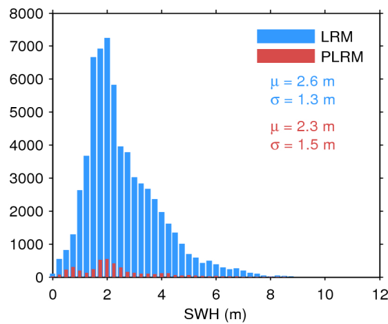
Figure 20. Histogram of science-valid SWH over oceans and lakes for LRM (blue) and PLRM (red) for 09/09/2015. The mean ( \mu ) and standard deviation ( \sigma ) are also shown. Note that values larger than 12 m are excluded from the histogram for the sake of readability but not from the computation of \mu and \sigma .
