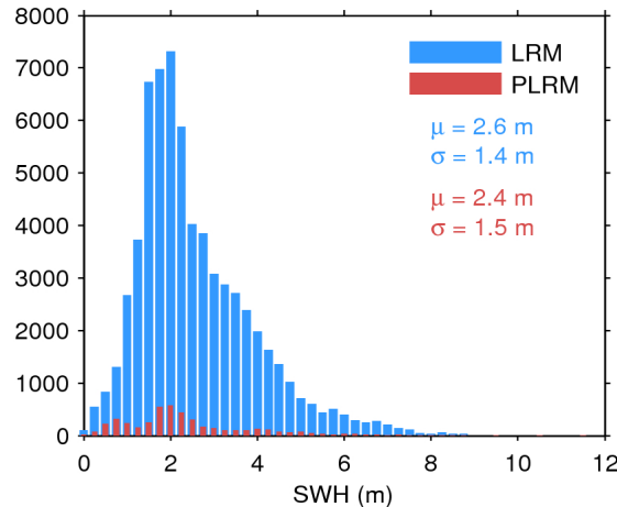
Figure 17. Histogram of flag-valid SWH over oceans and lakes for LRM (blue) and PLRM (red) for 09/09/2015. The mean ( \mu ) and standard deviation ( \sigma ) are also shown. Note that values larger than 12 m are excluded from the histogram for the sake of readability but not from the computation of \mu and \sigma .
