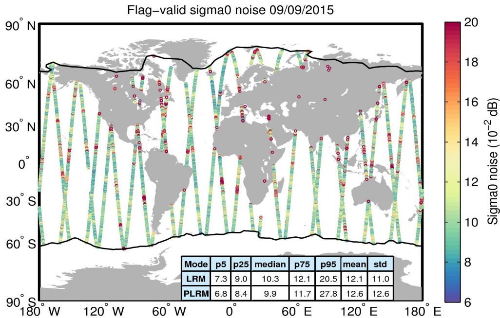
Figure 26. Geographical distribution of flag-valid 20-Hz sigma0 measurement noise over oceans and lakes for 09/09/2015. The statistical values shown in the table refer to the sigma0 noise and are calculated separately for LRM and PLRM regions. Measurements taken over polar polygons have been excluded from the computation of the statistical values. The black lines mark the outer limit of the Arctic and Antarctic polar polygons.
