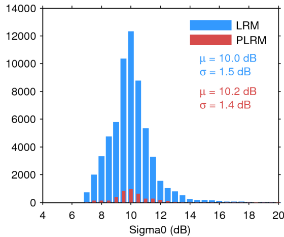
Figure 28. Histogram of science-valid sigma0 over oceans and lakes for LRM (blue) and PLRM (red) for 09/09/2015. The mean ( \mu ) and standard deviation ( \sigma ) are also shown. Note that values outside [4 20] dB are excluded from the histogram for the sake of readability but not from the computation of \mu and \sigma .
