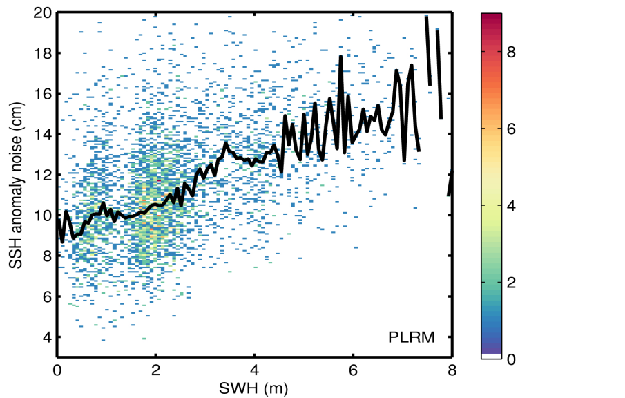
Figure 9. 2D histogram showing flag-valid SSH anomaly noise as a function of SWH for LRM (top) and PLRM (bottom) for 09/09/2015. The black line denotes the median SSH anomaly noise as a function of SWH.
