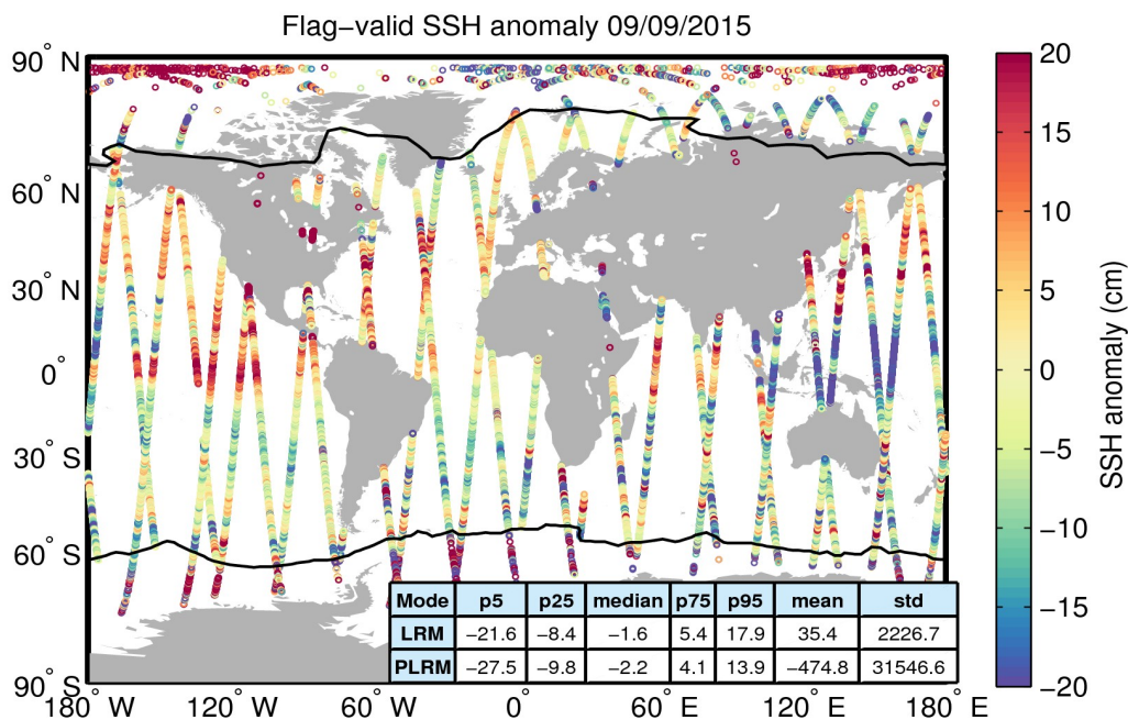
Figure 5. Geographical distribution of flag-valid 1-Hz SSH anomaly data over oceans and lakes for 09/09/2015. The statistical values shown in the table refer to the SSH anomaly in cm and are calculated separately for LRM and PLRM regions. Measurements taken over polar polygons have been excluded from the computation of the statistical values. The black lines mark the outer limit of the Arctic and Antarctic polar polygons.
