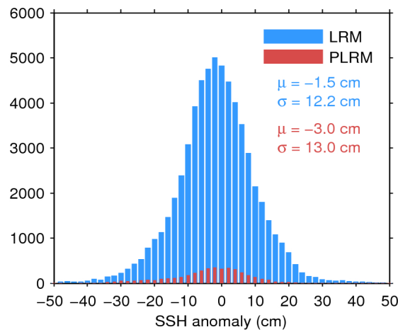
Figure 11. Histogram of science-valid SSH anomaly over oceans and lakes for LRM (blue) and PLRM (red) for 09/09/2015. The mean ( \mu ) and standard deviation ( \sigma ) are also shown. Note that values outside [-50 50] cm are excluded from the histogram for the sake of readability but not from the computation of \mu and \sigma .
