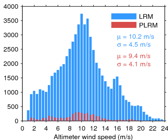
Figure 33. Histogram of flag-valid wind over oceans and lakes for LRM (blue) and PLRM (red) for 09/09/2015. The mean ( \mu ) and standard deviation ( \sigma ) are also shown. Note that values larger than 24 m/s are excluded from the histogram for the sake of readability but not from the computation of \mu and \sigma .
