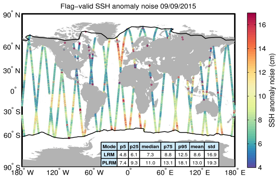
Figure 8. Geographical distribution of flag-valid 20-Hz SSH anomaly measurement noise over oceans and lakes for 09/09/2015. The statistical values shown in the table refer to the SSH anomaly noise and are calculated separately for LRM and PLRM regions. Measurements taken over polar polygons have been excluded from the computation of the statistical values. The black lines mark the outer limit of the Arctic and Antarctic polar polygons.
