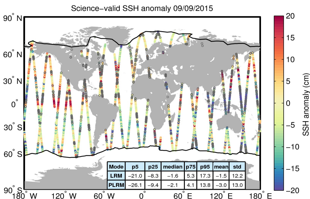
Figure 10. Geographical distribution of science-valid SSH anomaly data over oceans and lakes for 09/09/2015. The statistical values shown in the table refer to the SSH anomaly in cm and are calculated separately for LRM and PLRM regions. The black lines mark the outer limit of the Arctic and Antarctic polar polygons. Gray circles denote records that have been rejected based on the editing criteria described in Table 2.
