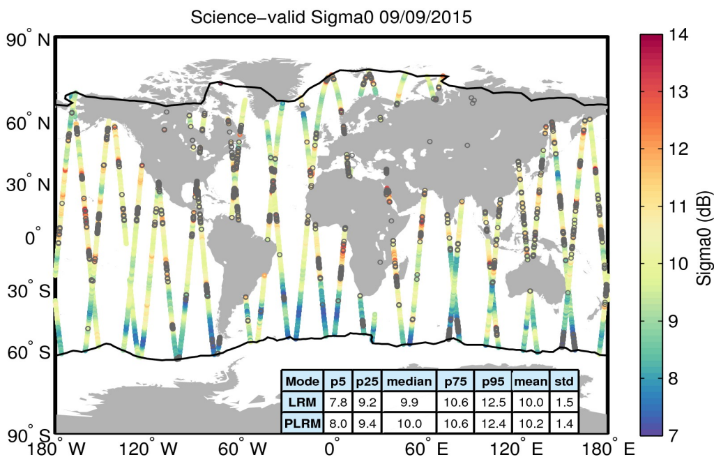
Figure 27. Geographical distribution of science-valid sigma0 data over oceans and lakes for 09/09/2015. The statistical values shown in the table refer to the sigma0 in dB and are calculated separately for LRM and PLRM regions. The black lines mark the outer limit of the Arctic and Antarctic polar polygons. Gray circles denote records that have been rejected based on the editing criteria described in Table 4.
