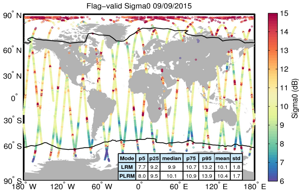
Figure 23. Geographical distribution of flag-valid sigma0 data over oceans and lakes for 09/09/2015. The statistical values shown in the table refer to the sigma0 in dB and are calculated separately for LRM and PLRM regions. Measurements taken over polar polygons have been excluded from the computation of the statistical values. The black lines mark the outer limit of the Arctic and Antarctic polar polygons.
