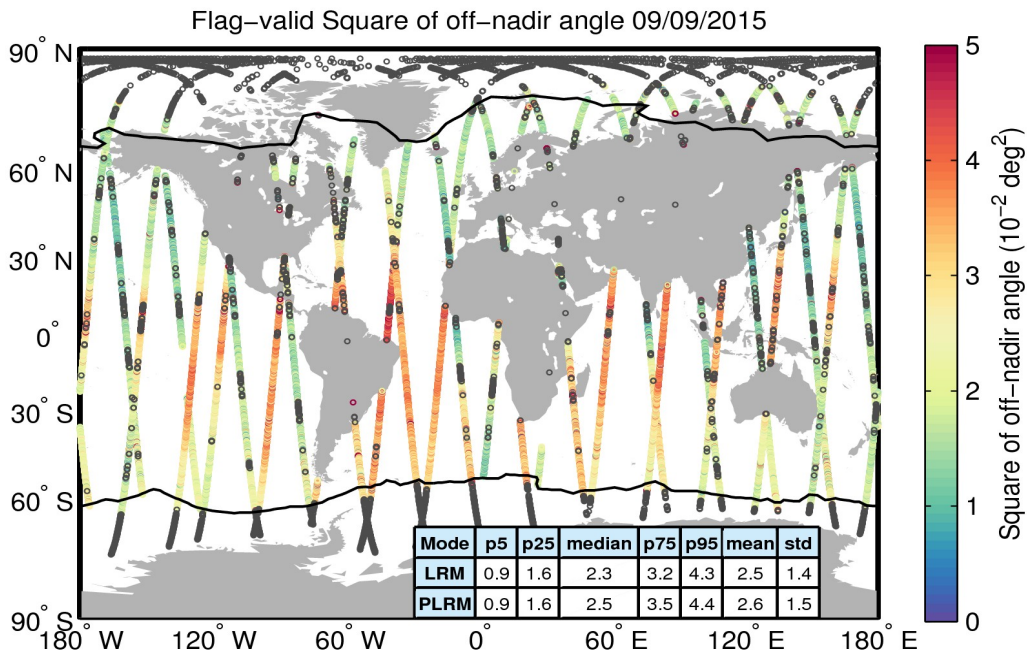
Figure 37. Geographical distribution of flag-valid mispointing data over oceans and lakes for 09/09/2015. The statistical values shown in the table refer to the mispointing in 10^{-2} deg 2 and are calculated separately for LRM and PLRM regions. Measurements taken over polar polygons have been excluded from the computation of the statistical values. The black lines mark the outer limit of the Arctic and Antarctic polar polygons. Gray circles denote negative values.
