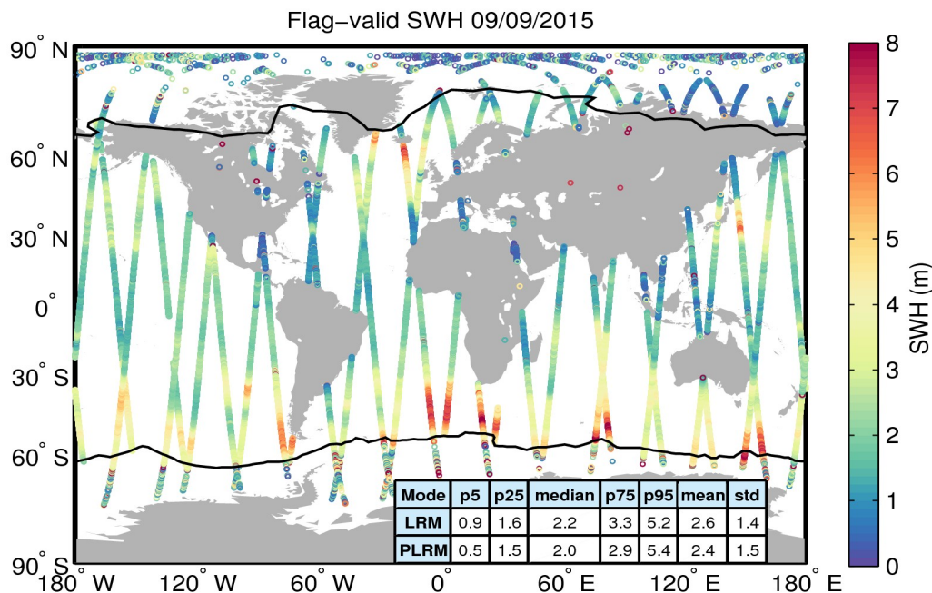
Figure 15. Geographical distribution of flag-valid SWH data over oceans and lakes for 09/09/2015. The statistical values shown in the table refer to the SWH in m and are calculated separately for LRM and PLRM regions. Measurements taken over polar polygons have been excluded from the computation of the statistical values. The black lines mark the outer limit of the Arctic and Antarctic polar polygons.
