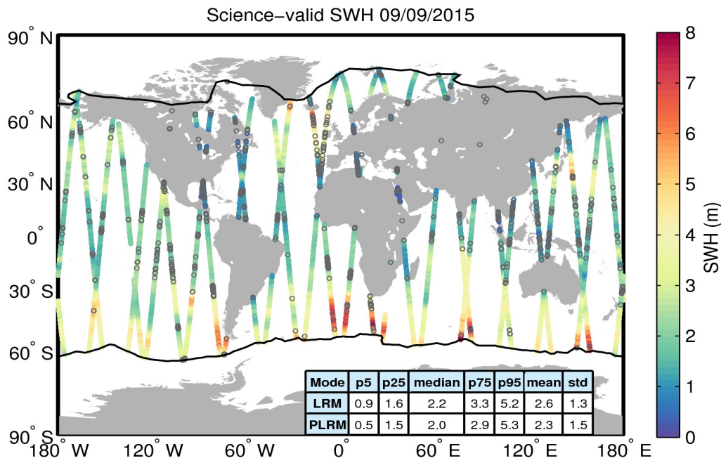
Figure 19. Geographical distribution of science-valid SWH data over oceans and lakes for 09/09/2015. The statistical values shown in the table refer to the SWH in m and are calculated separately for LRM and PLRM regions. The black lines mark the outer limit of the Arctic and Antarctic polar polygons. Gray circles denote records that have been rejected based on the editing criteria described in Table 3.
