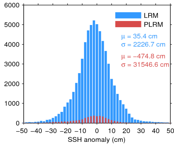
Figure 7. Histogram of flag-valid SSH anomaly over oceans and lakes for LRM (blue) and PLRM (red) for 09/09/2015. The mean ( \mu ) and standard deviation ( \sigma ) are also shown. Note that values outside [-50 50] cm are excluded from the histogram for the sake of readability but not from the computation of \mu and \sigma .
