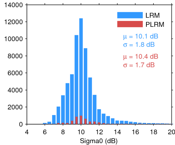
Figure 25. Histogram of flag-valid sigma0 over oceans and lakes for LRM (blue) and PLRM (red) for 09/09/2015. The mean ( \mu ) and standard deviation ( \sigma ) are also shown. Note that values outside [4 20] dB are excluded from the histogram for the sake of readability but not from the computation of \mu and \sigma .
