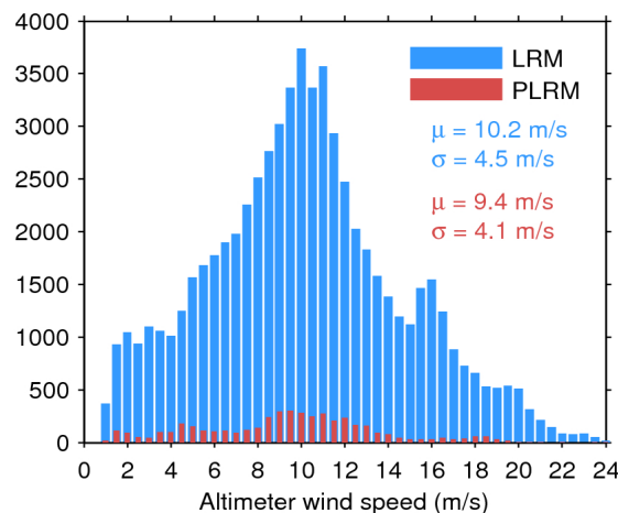
Figure 35. Histogram of science-valid wind over oceans and lakes for LRM (blue) and PLRM (red) for 09/09/2015. The mean ( \mu ) and standard deviation ( \sigma ) are also shown. Note that values larger than 24 m/s are excluded from the histogram for the sake of readability but not from the computation of \mu and \sigma .
