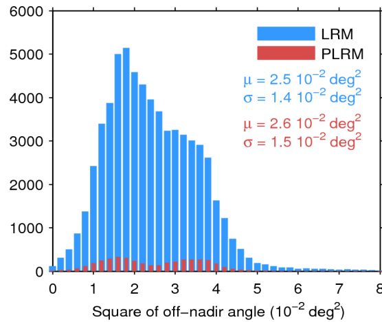
Figure 39. Histogram of flag-valid mispointing over oceans and lakes for LRM (blue) and PLRM (red) for 09/09/2015. Only positive values have been considered. The mean ( \mu ) and standard deviation ( \sigma ) are also shown. Note that values larger than 8 \cdot 10^{-2} \text{ deg}^2 are excluded from the histogram for the sake of readability but not from the computation of \mu and \sigma .
