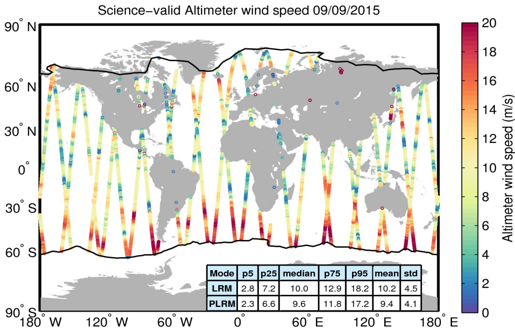
Figure 34. Geographical distribution of science-valid wind data over oceans and lakes for 09/09/2015. The statistical values shown in the table refer to the wind in m/s and are calculated separately for LRM and PLRM regions. The black lines mark the outer limit of the Arctic and Antarctic polar polygons. Gray circles denote records that have been rejected based on the editing criteria described in Table 5.
