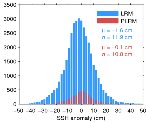
Figure 11. Histogram of science-valid SSH anomaly over oceans and lakes for LRM (blue) and PLRM (red) for 05/09/2015. The mean ( \mu ) and standard deviation ( \sigma ) are also shown. Note that values outside [-50 50] cm are excluded from the histogram for the sake of readability but not from the computation of \mu and \sigma .
