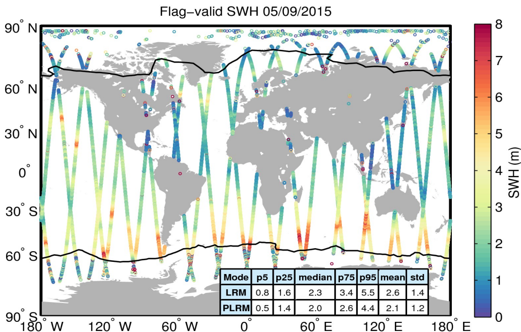
Figure 15. Geographical distribution of flag-valid SWH data over oceans and lakes for 05/09/2015. The statistical values shown in the table refer to the SWH in m and are calculated separately for LRM and PLRM regions. Measurements taken over polar polygons have been excluded from the computation of the statistical values. The black lines mark the outer limit of the Arctic and Antarctic polar polygons.
