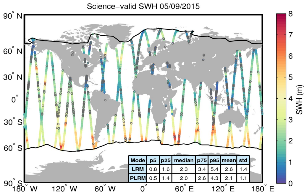
Figure 19. Geographical distribution of science-valid SWH data over oceans and lakes for 05/09/2015. The statistical values shown in the table refer to the SWH in m and are calculated separately for LRM and PLRM regions. The black lines mark the outer limit of the Arctic and Antarctic polar polygons. Gray circles denote records that have been rejected based on the editing criteria described in Table 3.
