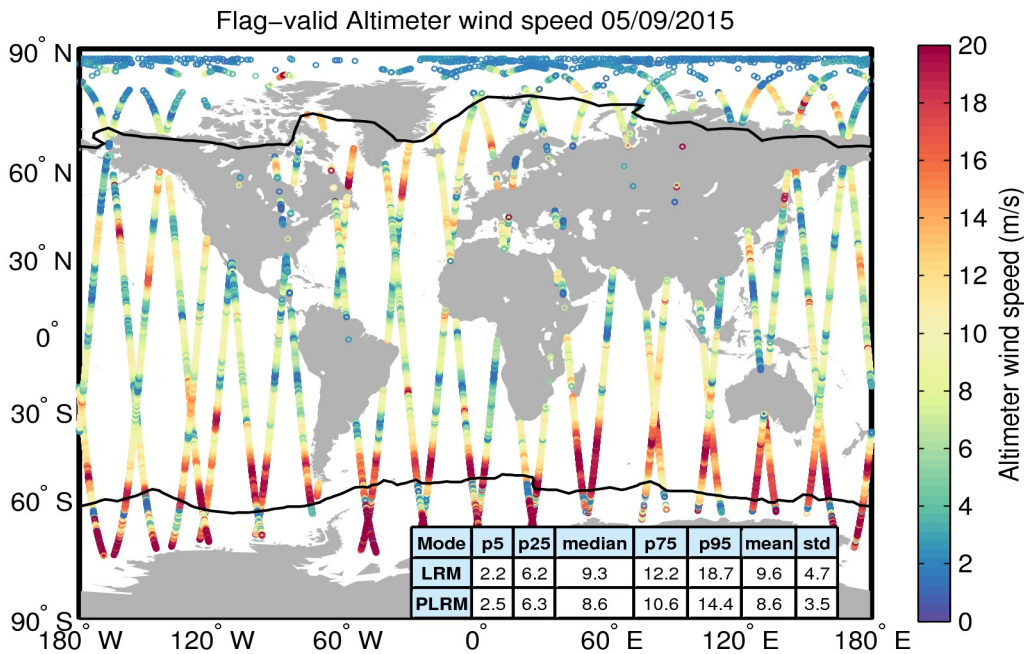
Figure 31. Geographical distribution of flag-valid wind data over oceans and lakes for 05/09/2015. The statistical values shown in the table refer to the wind in m/s and are calculated separately for LRM and PLRM regions. Measurements taken over polar polygons have been excluded from the computation of the statistical values. The black lines mark the outer limit of the Arctic and Antarctic polar polygons.
