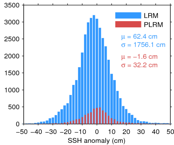
Figure 7. Histogram of flag-valid SSH anomaly over oceans and lakes for LRM (blue) and PLRM (red) for 05/09/2015. The mean ( \mu ) and standard deviation ( \sigma ) are also shown. Note that values outside [-50\ 50] cm are excluded from the histogram for the sake of readability but not from the computation of \mu and \sigma .
