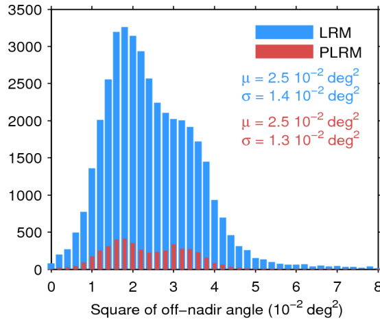
Figure 39. Histogram of flag-valid mispointing over oceans and lakes for LRM (blue) and PLRM (red) for 05/09/2015. Only positive values have been considered. The mean ( \mu ) and standard deviation ( \sigma ) are also shown. Note that values larger than 8 \cdot 10^{-2} \text{ deg}^2 are excluded from the histogram for the sake of readability but not from the computation of \mu and \sigma .
