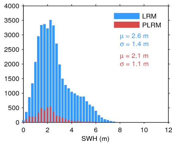
Figure 20. Histogram of science-valid SWH over oceans and lakes for LRM (blue) and PLRM (red) for 05/09/2015. The mean ( \mu ) and standard deviation ( \sigma ) are also shown. Note that values larger than 12 m are excluded from the histogram for the sake of readability but not from the computation of \mu and \sigma .
