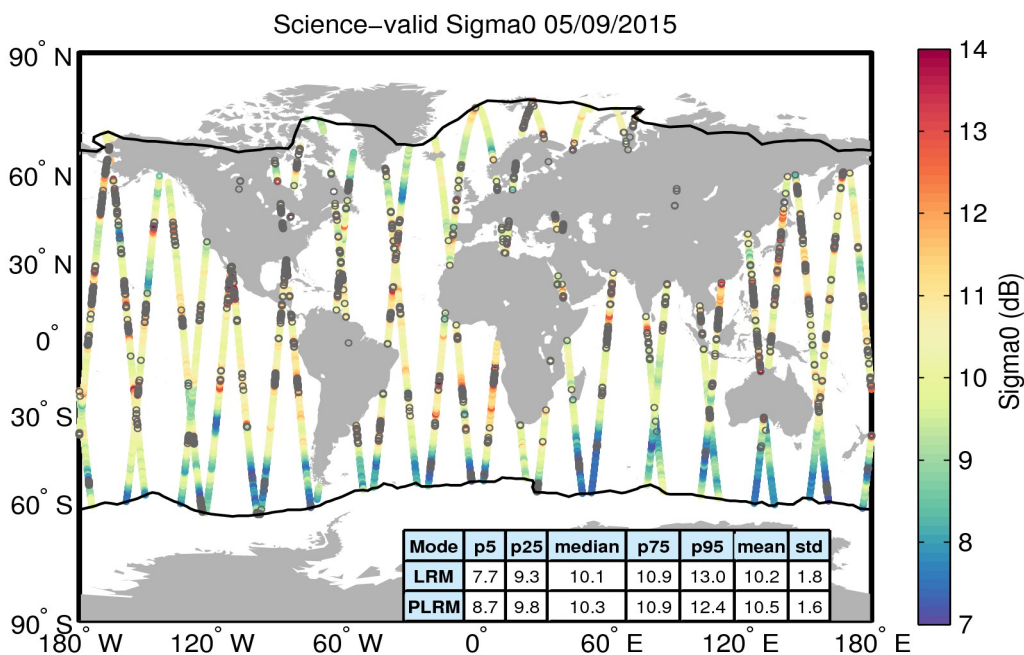
Figure 27. Geographical distribution of science-valid sigma0 data over oceans and lakes for 05/09/2015. The statistical values shown in the table refer to the sigma0 in dB and are calculated separately for LRM and PLRM regions. The black lines mark the outer limit of the Arctic and Antarctic polar polygons. Gray circles denote records that have been rejected based on the editing criteria described in Table 4.
