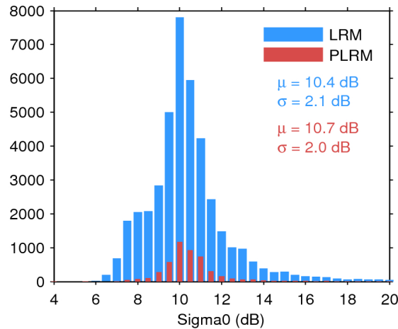
Figure 25. Histogram of flag-valid sigma0 over oceans and lakes for LRM (blue) and PLRM (red) for 05/09/2015. The mean ( \mu ) and standard deviation ( \sigma ) are also shown. Note that values outside [4 20] dB are excluded from the histogram for the sake of readability but not from the computation of \mu and \sigma .
