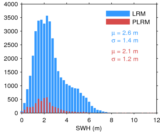
Figure 17. Histogram of flag-valid SWH over oceans and lakes for LRM (blue) and PLRM (red) for 05/09/2015. The mean ( \mu ) and standard deviation ( \sigma ) are also shown. Note that values larger than 12 m are excluded from the histogram for the sake of readability but not from the computation of \mu and \sigma .
