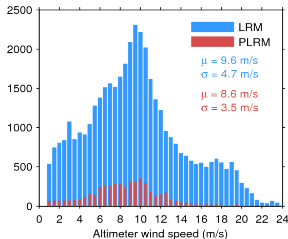
Figure 35. Histogram of science-valid wind over oceans and lakes for LRM (blue) and PLRM (red) for 05/09/2015. The mean ( \mu ) and standard deviation ( \sigma ) are also shown. Note that values larger than 24 m/s are excluded from the histogram for the sake of readability but not from the computation of \mu and \sigma .
