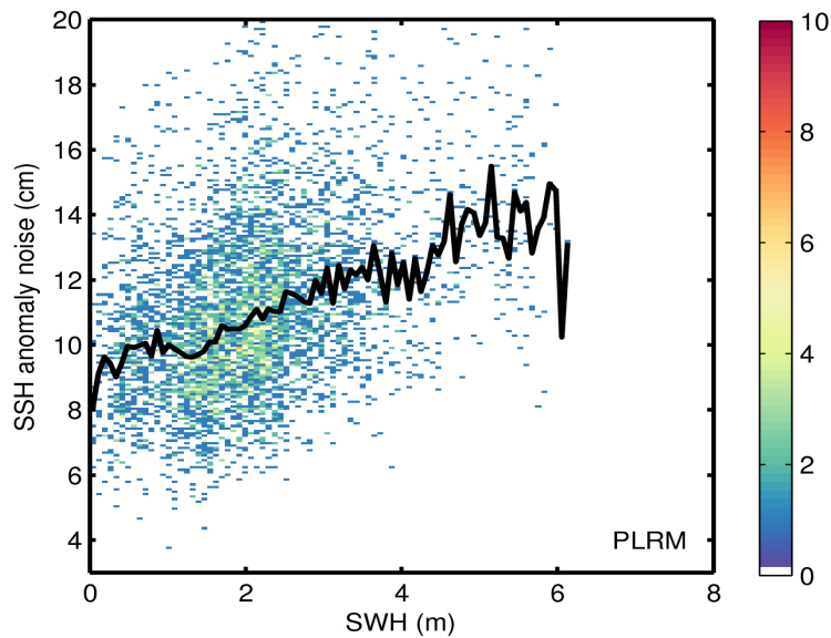
Figure 9. 2D histogram showing flag-valid SSH anomaly noise as a function of SWH for LRM (top) and PLRM (bottom) for 05/09/2015. The black line denotes the median SSH anomaly as a function of SWH.
