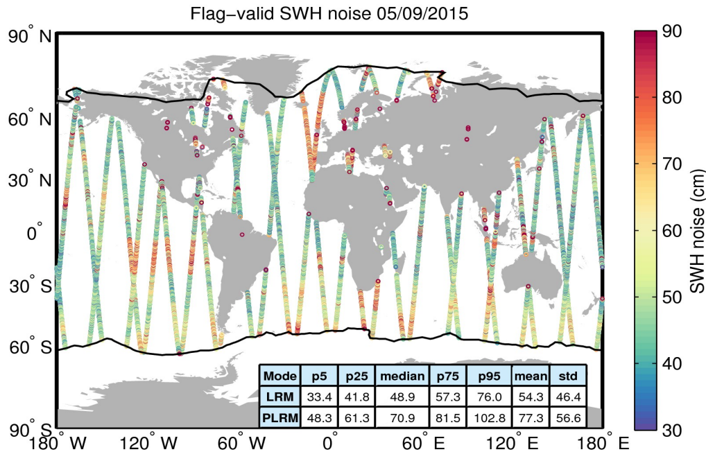
Figure 18. Geographical distribution of flag-valid 20-Hz SWH measurement noise over oceans and lakes for 05/09/2015. The statistical values shown in the table refer to the SWH noise and are calculated separately for LRM and PLRM regions. Measurements taken over polar polygons have been excluded from the computation of the statistical values. The black lines mark the outer limit of the Arctic and Antarctic polar polygons.
