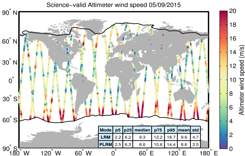
Figure 34. Geographical distribution of science-valid wind data over oceans and lakes for 05/09/2015. The statistical values shown in the table refer to the wind in m/s and are calculated separately for LRM and PLRM regions. The black lines mark the outer limit of the Arctic and Antarctic polar polygons. Gray circles denote records that have been rejected based on the editing criteria described in Table 5.
