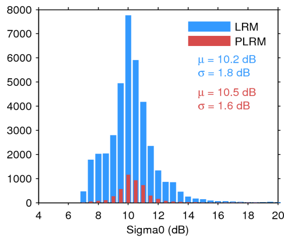
Figure 28. Histogram of science-valid sigma0 over oceans and lakes for LRM (blue) and PLRM (red) for 05/09/2015. The mean ( \mu ) and standard deviation ( \sigma ) are also shown. Note that values outside [4 20] dB are excluded from the histogram for the sake of readability but not from the computation of \mu and \sigma .
