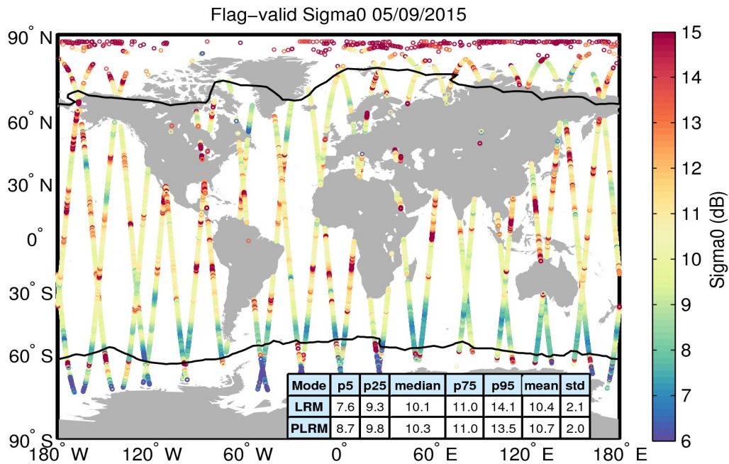
Figure 23. Geographical distribution of flag-valid sigma0 data over oceans and lakes for 05/09/2015. The statistical values shown in the table refer to the sigma0 in dB and are calculated separately for LRM and PLRM regions. Measurements taken over polar polygons have been excluded from the computation of the statistical values. The black lines mark the outer limit of the Arctic and Antarctic polar polygons.
