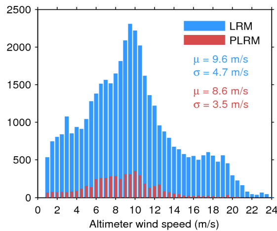
Figure 33. Histogram of flag-valid wind over oceans and lakes for LRM (blue) and PLRM (red) for 05/09/2015. The mean ( \mu ) and standard deviation ( \sigma ) are also shown. Note that values larger than 24 m/s are excluded from the histogram for the sake of readability but not from the computation of \mu and \sigma .
