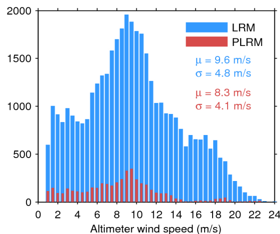
Figure 35. Histogram of science-valid wind over oceans and lakes for LRM (blue) and PLRM (red) for 04/09/2015. The mean ( \mu ) and standard deviation ( \sigma ) are also shown. Note that values larger than 24 m/s are excluded from the histogram for the sake of readability but not from the computation of \mu and \sigma .
