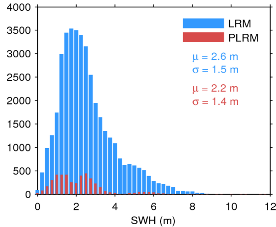
Figure 17. Histogram of flag-valid SWH over oceans and lakes for LRM (blue) and PLRM (red) for 04/09/2015. The mean ( \mu ) and standard deviation ( \sigma ) are also shown. Note that values larger than 12 m are excluded from the histogram for the sake of readability but not from the computation of \mu and \sigma .
