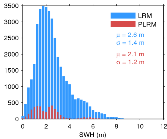
Figure 20. Histogram of science-valid SWH over oceans and lakes for LRM (blue) and PLRM (red) for 04/09/2015. The mean ( \mu ) and standard deviation ( \sigma ) are also shown. Note that values larger than 12 m are excluded from the histogram for the sake of readability but not from the computation of \mu and \sigma .
