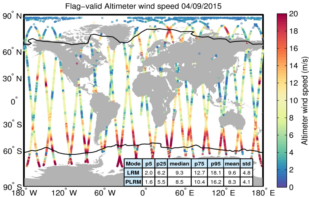
Figure 31. Geographical distribution of flag-valid wind data over oceans and lakes for 04/09/2015. The statistical values shown in the table refer to the wind in m/s and are calculated separately for LRM and PLRM regions. Measurements taken over polar polygons have been excluded from the computation of the statistical values. The black lines mark the outer limit of the Arctic and Antarctic polar polygons.
