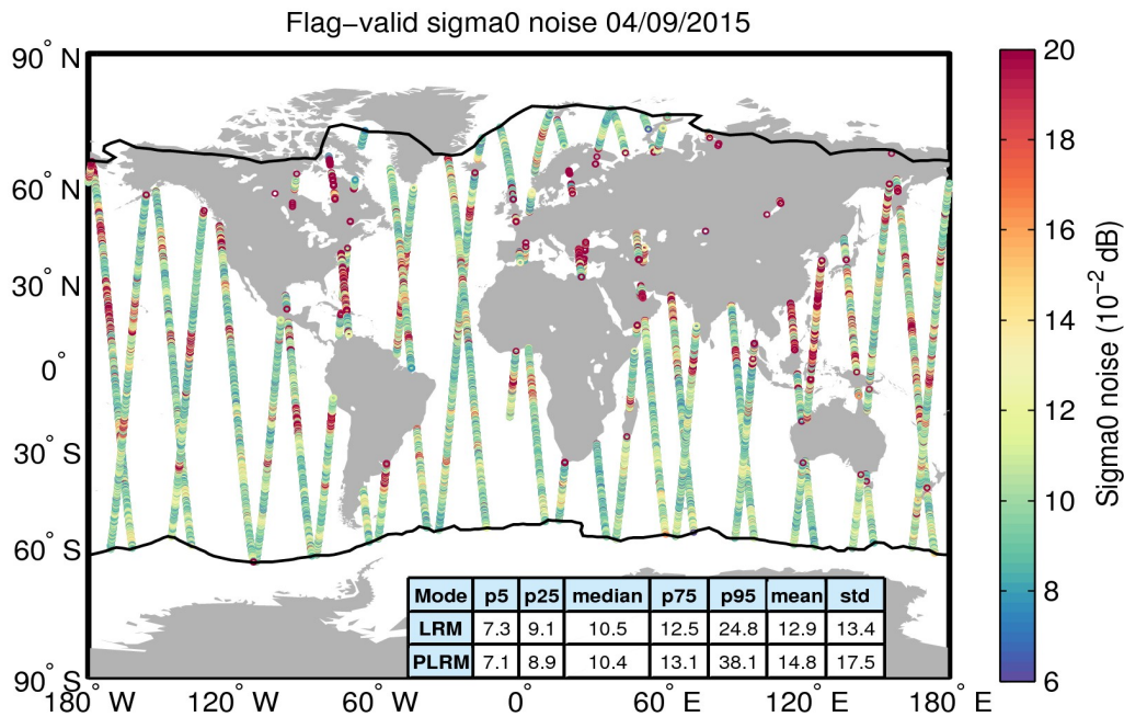
Figure 26. Geographical distribution of flag-valid 20-Hz sigma0 measurement noise over oceans and lakes for 04/09/2015. The statistical values shown in the table refer to the sigma0 noise and are calculated separately for LRM and PLRM regions. Measurements taken over polar polygons have been excluded from the computation of the statistical values. The black lines mark the outer limit of the Arctic and Antarctic polar polygons.
