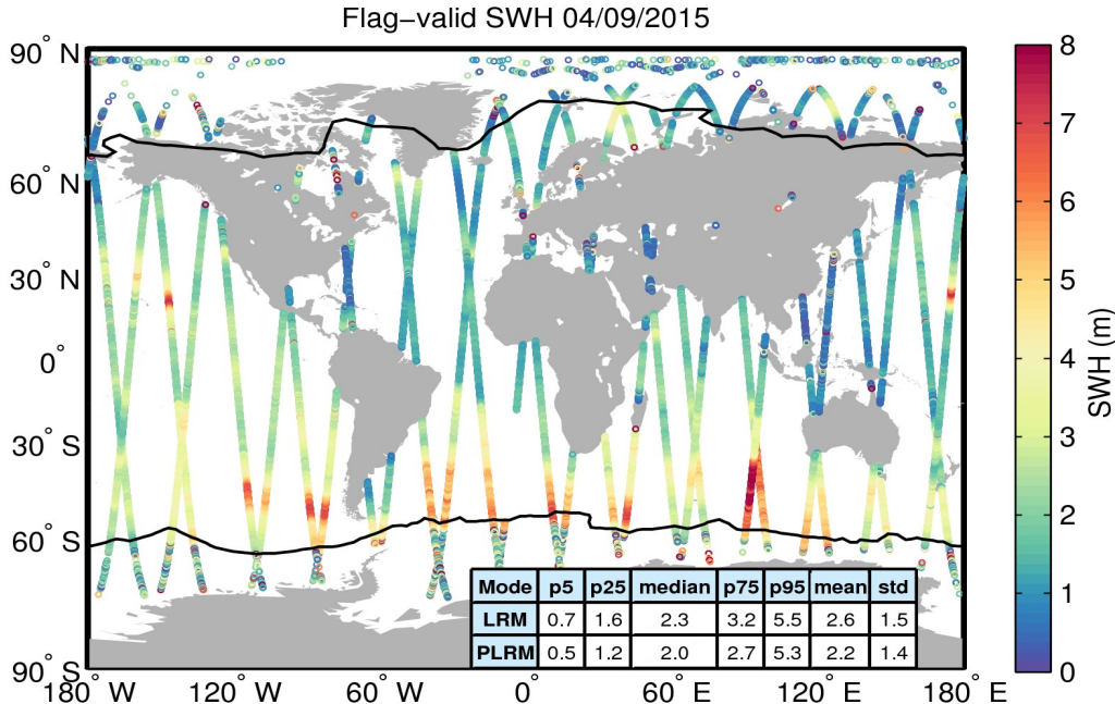
Figure 15. Geographical distribution of flag-valid SWH data over oceans and lakes for 04/09/2015. The statistical values shown in the table refer to the SWH in m and are calculated separately for LRM and PLRM regions. Measurements taken over polar polygons have been excluded from the computation of the statistical values. The black lines mark the outer limit of the Arctic and Antarctic polar polygons.
