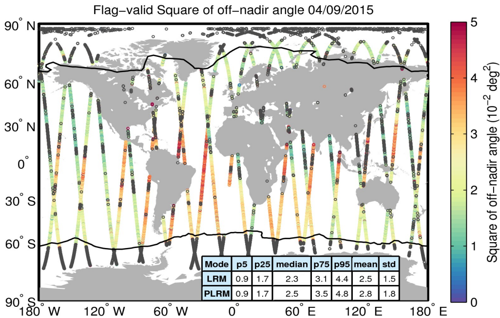
Figure 37. Geographical distribution of flag-valid mispointing data over oceans and lakes for 04/09/2015. The statistical values shown in the table refer to the mispointing in 10^{-2} deg 2 and are calculated separately for LRM and PLRM regions. Measurements taken over polar polygons have been excluded from the computation of the statistical values. The black lines mark the outer limit of the Arctic and Antarctic polar polygons. Gray circles denote negative values.
