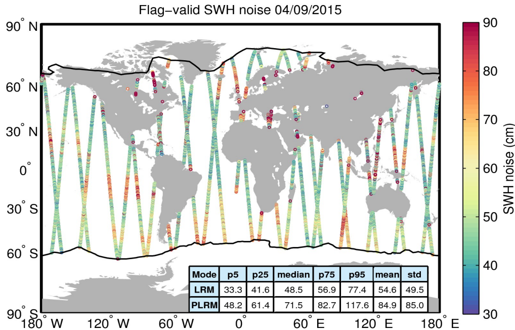
Figure 18. Geographical distribution of flag-valid 20-Hz SWH measurement noise over oceans and lakes for 04/09/2015. The statistical values shown in the table refer to the SWH noise and are calculated separately for LRM and PLRM regions. Measurements taken over polar polygons have been excluded from the computation of the statistical values. The black lines mark the outer limit of the Arctic and Antarctic polar polygons.
