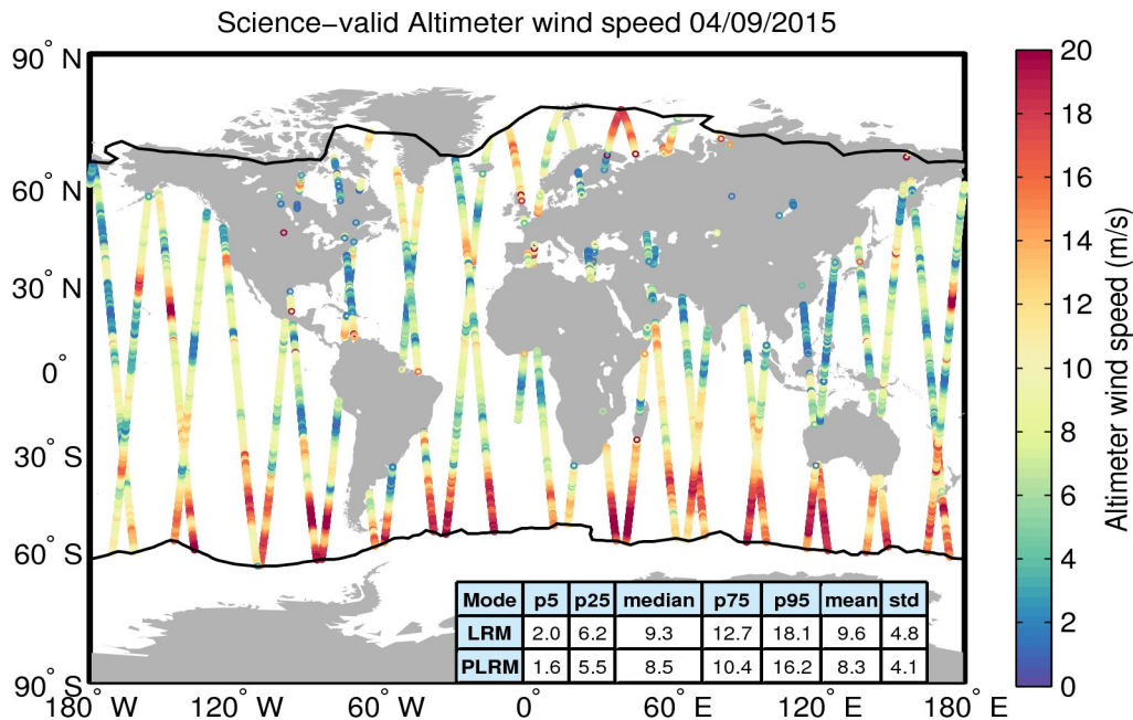
Figure 34. Geographical distribution of science-valid wind data over oceans and lakes for 04/09/2015. The statistical values shown in the table refer to the wind in m/s and are calculated separately for LRM and PLRM regions. The black lines mark the outer limit of the Arctic and Antarctic polar polygons. Gray circles denote records that have been rejected based on the editing criteria described in Table 5.
