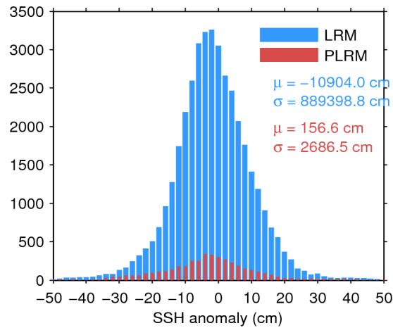
Figure 7. Histogram of flag-valid SSH anomaly over oceans and lakes for LRM (blue) and PLRM (red) for 04/09/2015. The mean ( \mu ) and standard deviation ( \sigma ) are also shown. Note that values outside [-50 \ 50] cm are excluded from the histogram for the sake of readability but not from the computation of \mu and \sigma .
