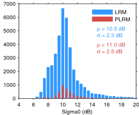
Figure 25. Histogram of flag-valid sigma0 over oceans and lakes for LRM (blue) and PLRM (red) for 04/09/2015. The mean ( \mu ) and standard deviation ( \sigma ) are also shown. Note that values outside [4 20] dB are excluded from the histogram for the sake of readability but not from the computation of \mu and \sigma .
