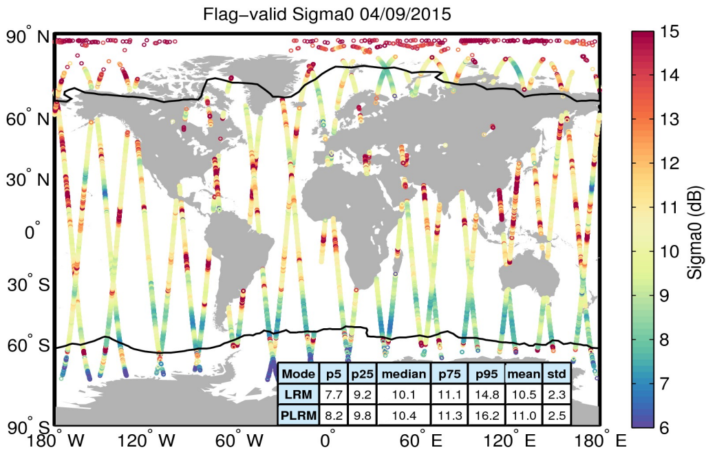
Figure 23. Geographical distribution of flag-valid sigma0 data over oceans and lakes for 04/09/2015. The statistical values shown in the table refer to the sigma0 in dB and are calculated separately for LRM and PLRM regions. Measurements taken over polar polygons have been excluded from the computation of the statistical values. The black lines mark the outer limit of the Arctic and Antarctic polar polygons.
