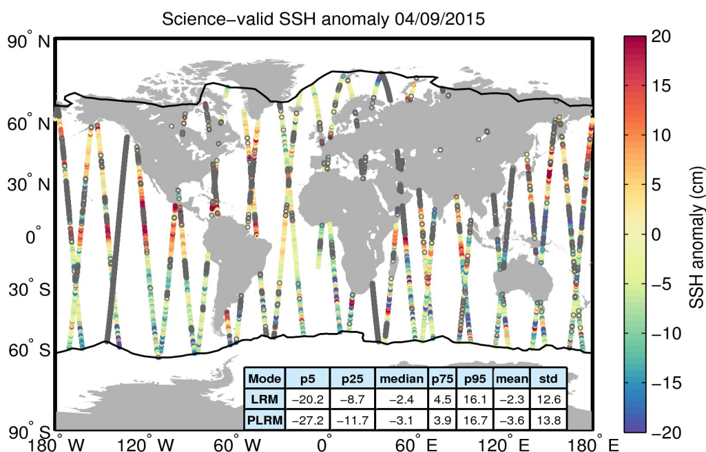
Figure 10. Geographical distribution of science-valid SSH anomaly data over oceans and lakes for 04/09/2015. The statistical values shown in the table refer to the SSH anomaly in cm and are calculated separately for LRM and PLRM regions. The black lines mark the outer limit of the Arctic and Antarctic polar polygons. Gray circles denote records that have been rejected based on the editing criteria described in Table 2.
