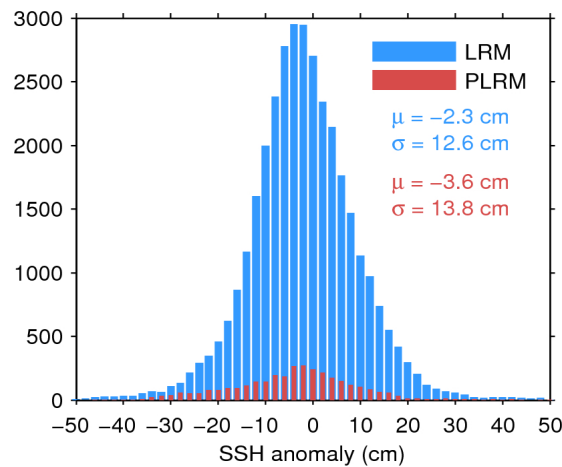
Figure 11. Histogram of science-valid SSH anomaly over oceans and lakes for LRM (blue) and PLRM (red) for 04/09/2015. The mean ( \mu ) and standard deviation ( \sigma ) are also shown. Note that values outside [-50 50] cm are excluded from the histogram for the sake of readability but not from the computation of \mu and \sigma .
