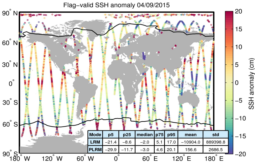
Figure 5. Geographical distribution of flag-valid 1-Hz SSH anomaly data over oceans and lakes for 04/09/2015. The statistical values shown in the table refer to the SSH anomaly in cm and are calculated separately for LRM and PLRM regions. Measurements taken over polar polygons have been excluded from the computation of the statistical values. The black lines mark the outer limit of the Arctic and Antarctic polar polygons.
