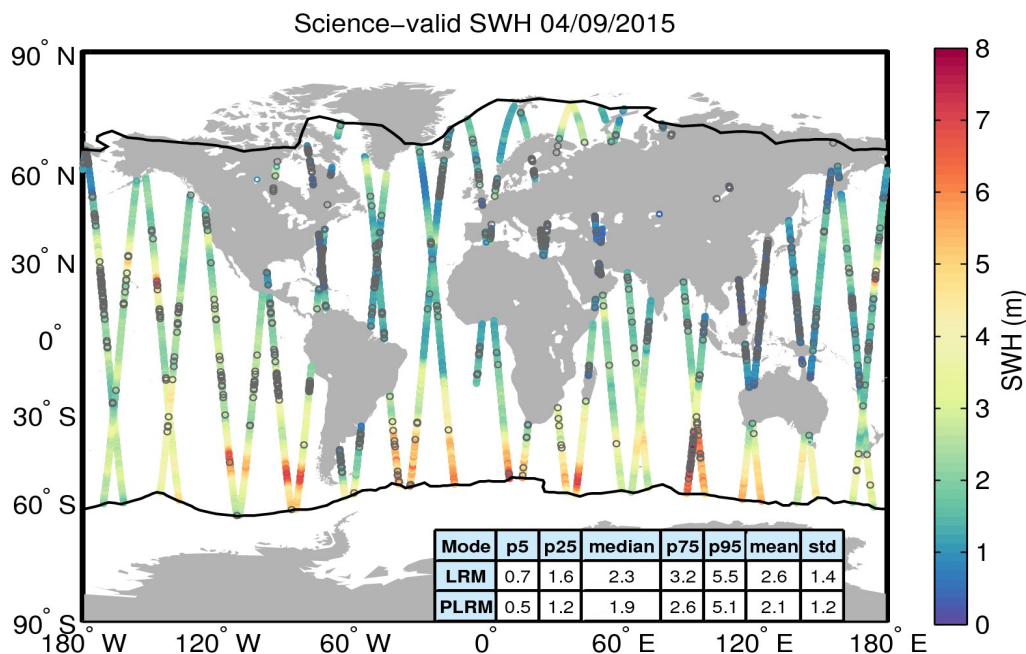
Figure 19. Geographical distribution of science-valid SWH data over oceans and lakes for 04/09/2015. The statistical values shown in the table refer to the SWH in m and are calculated separately for LRM and PLRM regions. The black lines mark the outer limit of the Arctic and Antarctic polar polygons. Gray circles denote records that have been rejected based on the editing criteria described in Table 3.
