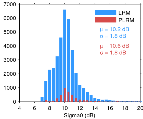
Figure 28. Histogram of science-valid sigma0 over oceans and lakes for LRM (blue) and PLRM (red) for 04/09/2015. The mean ( \mu ) and standard deviation ( \sigma ) are also shown. Note that values outside [4 20] dB are excluded from the histogram for the sake of readability but not from the computation of \mu and \sigma .
