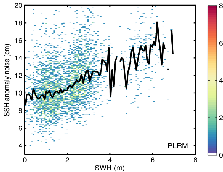
Figure 9. 2D histogram showing flag-valid SSH anomaly noise as a function of SWH for LRM (top) and PLRM (bottom) for 04/09/2015. The black line denotes the median SSH anomaly as a function of SWH.
