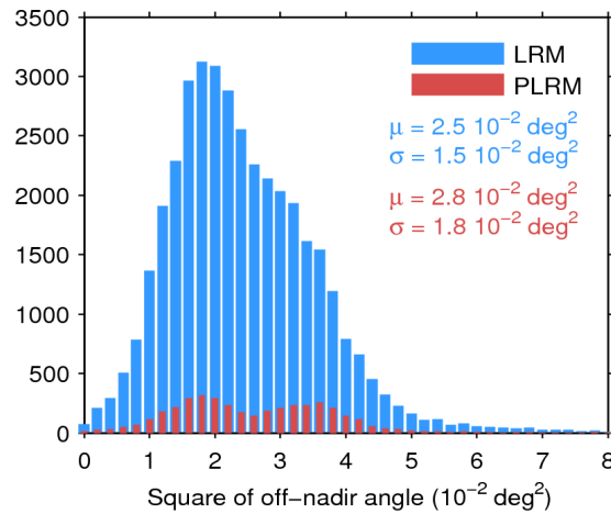
Figure 39. Histogram of flag-valid mispointing over oceans and lakes for LRM (blue) and PLRM (red) for 04/09/2015. Only positive values have been considered. The mean ( \mu ) and standard deviation ( \sigma ) are also shown. Note that values larger than 8 \cdot 10^{-2} \text{ deg}^2 are excluded from the histogram for the sake of readability but not from the computation of \mu and \sigma .
