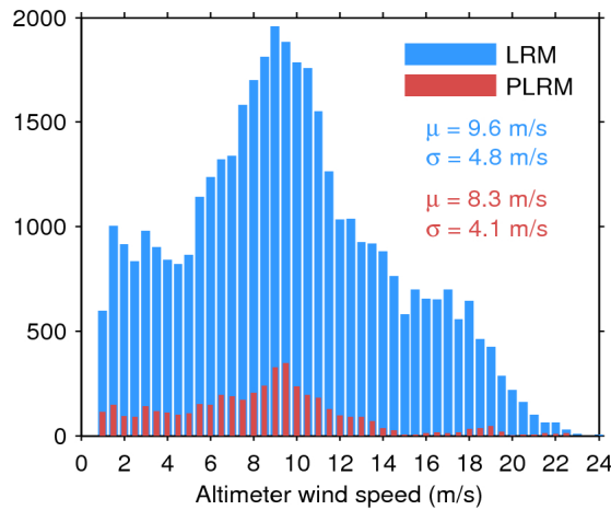
Figure 33. Histogram of flag-valid wind over oceans and lakes for LRM (blue) and PLRM (red) for 04/09/2015. The mean ( \mu ) and standard deviation ( \sigma ) are also shown. Note that values larger than 24 m/s are excluded from the histogram for the sake of readability but not from the computation of \mu and \sigma .
