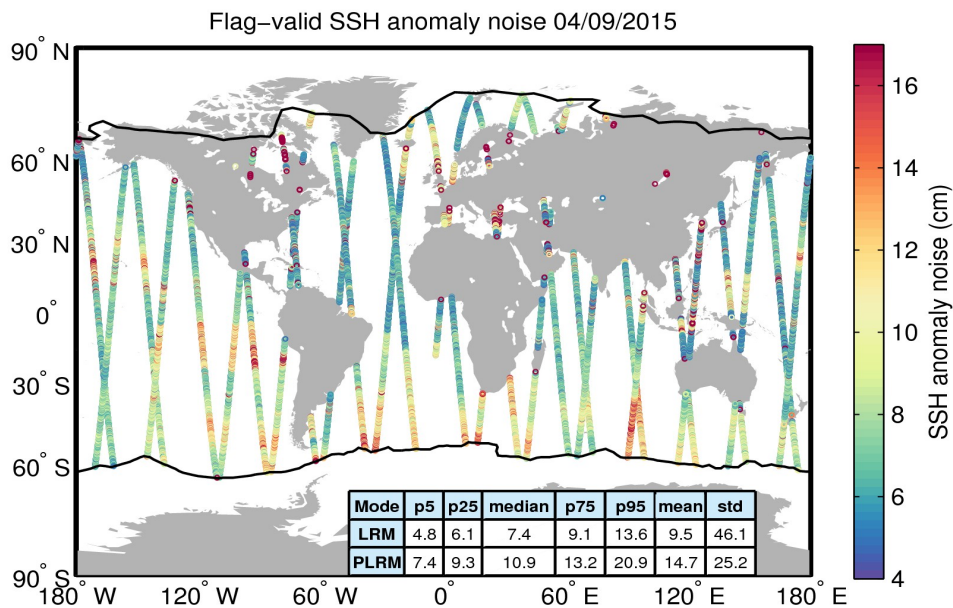
Figure 8. Geographical distribution of flag-valid 20-Hz SSH anomaly measurement noise over oceans and lakes for 04/09/2015. The statistical values shown in the table refer to the SSH anomaly noise and are calculated separately for LRM and PLRM regions. Measurements taken over polar polygons have been excluded from the computation of the statistical values. The black lines mark the outer limit of the Arctic and Antarctic polar polygons.
