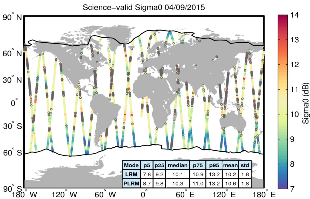
Figure 27. Geographical distribution of science-valid sigma0 data over oceans and lakes for 04/09/2015. The statistical values shown in the table refer to the sigma0 in dB and are calculated separately for LRM and PLRM regions. The black lines mark the outer limit of the Arctic and Antarctic polar polygons. Gray circles denote records that have been rejected based on the editing criteria described in Table 4.
