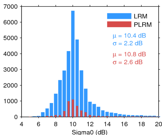
Figure 25. Histogram of flag-valid sigma0 over oceans and lakes for LRM (blue) and PLRM (red) for 03/09/2015. The mean ( \mu ) and standard deviation ( \sigma ) are also shown. Note that values outside [4 20] dB are excluded from the histogram for the sake of readability but not from the computation of \mu and \sigma .
