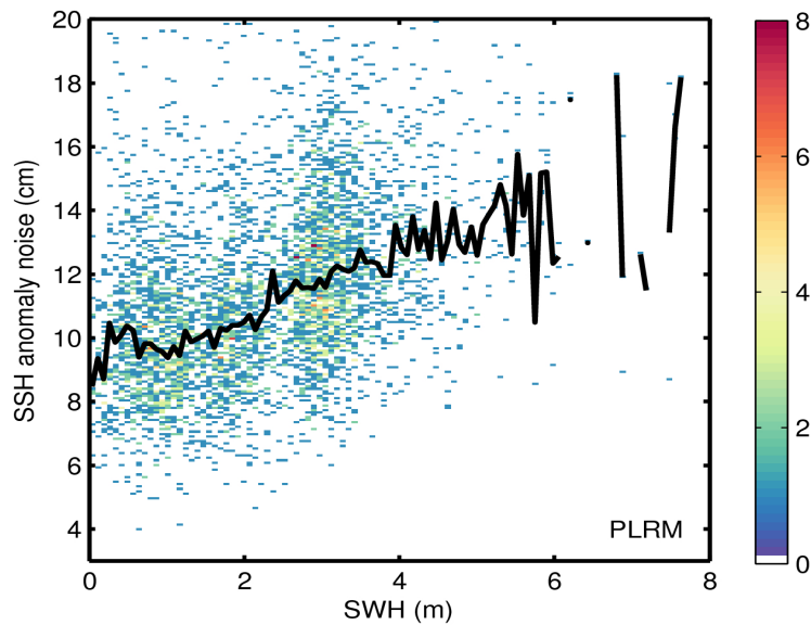
Figure 9. 2D histogram showing flag-valid SSH anomaly noise as a function of SWH for LRM (top) and PLRM (bottom) for 03/09/2015. The black line denotes the median SSH anomaly as a function of SWH.
