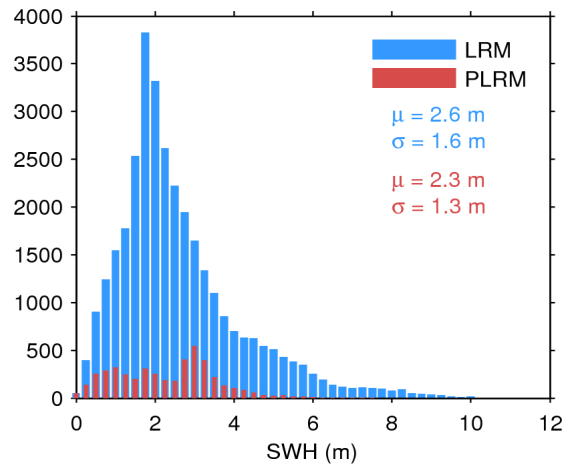
Figure 20. Histogram of science-valid SWH over oceans and lakes for LRM (blue) and PLRM (red) for 03/09/2015. The mean ( \mu ) and standard deviation ( \sigma ) are also shown. Note that values larger than 12 m are excluded from the histogram for the sake of readability but not from the computation of \mu and \sigma .
