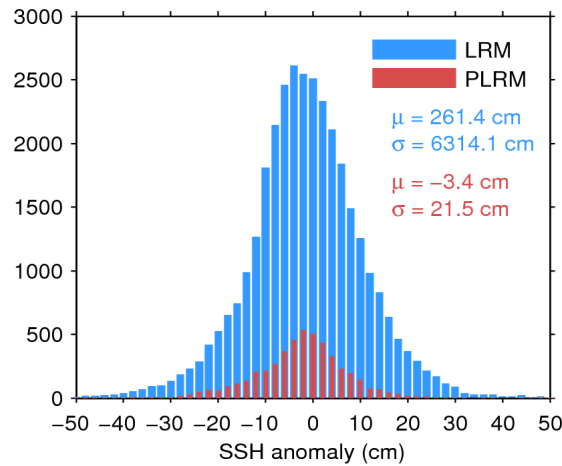
Figure 7. Histogram of flag-valid SSH anomaly over oceans and lakes for LRM (blue) and PLRM (red) for 03/09/2015. The mean ( \mu ) and standard deviation ( \sigma ) are also shown. Note that values outside [-50 50] cm are excluded from the histogram for the sake of readability but not from the computation of \mu and \sigma .
