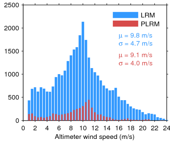
Figure 33. Histogram of flag-valid wind over oceans and lakes for LRM (blue) and PLRM (red) for 03/09/2015. The mean ( \mu ) and standard deviation ( \sigma ) are also shown. Note that values larger than 24 m/s are excluded from the histogram for the sake of readability but not from the computation of \mu and \sigma .
