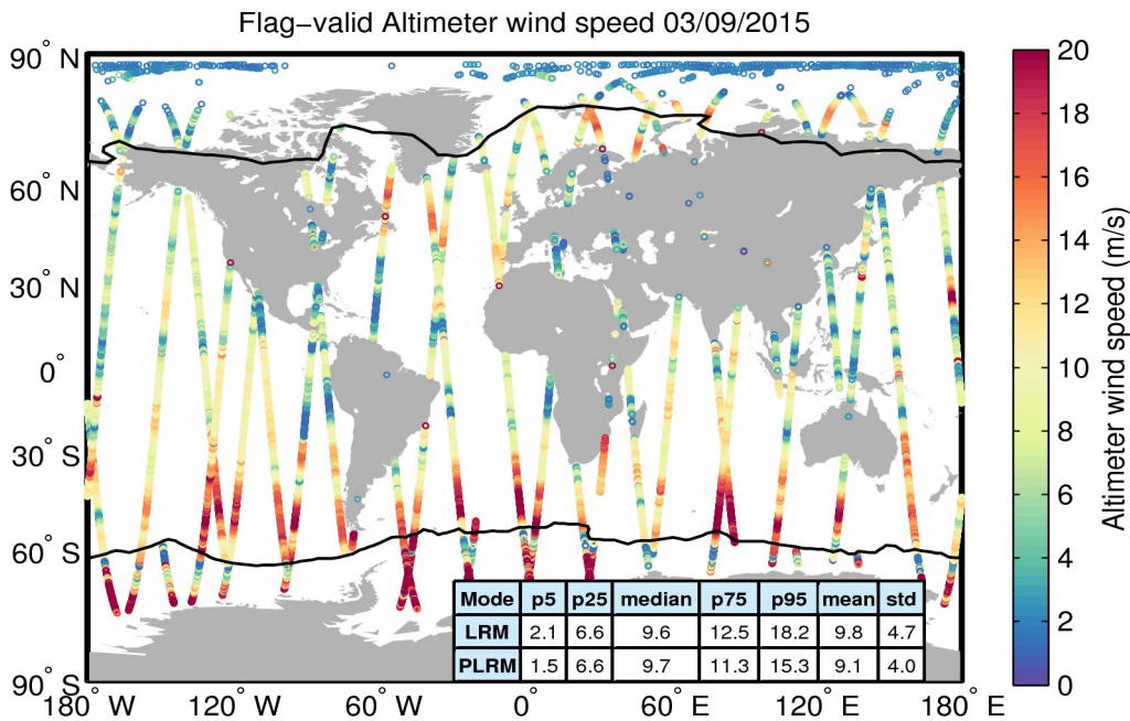
Figure 31. Geographical distribution of flag-valid wind data over oceans and lakes for 03/09/2015. The statistical values shown in the table refer to the wind in m/s and are calculated separately for LRM and PLRM regions. Measurements taken over polar polygons have been excluded from the computation of the statistical values. The black lines mark the outer limit of the Arctic and Antarctic polar polygons.
