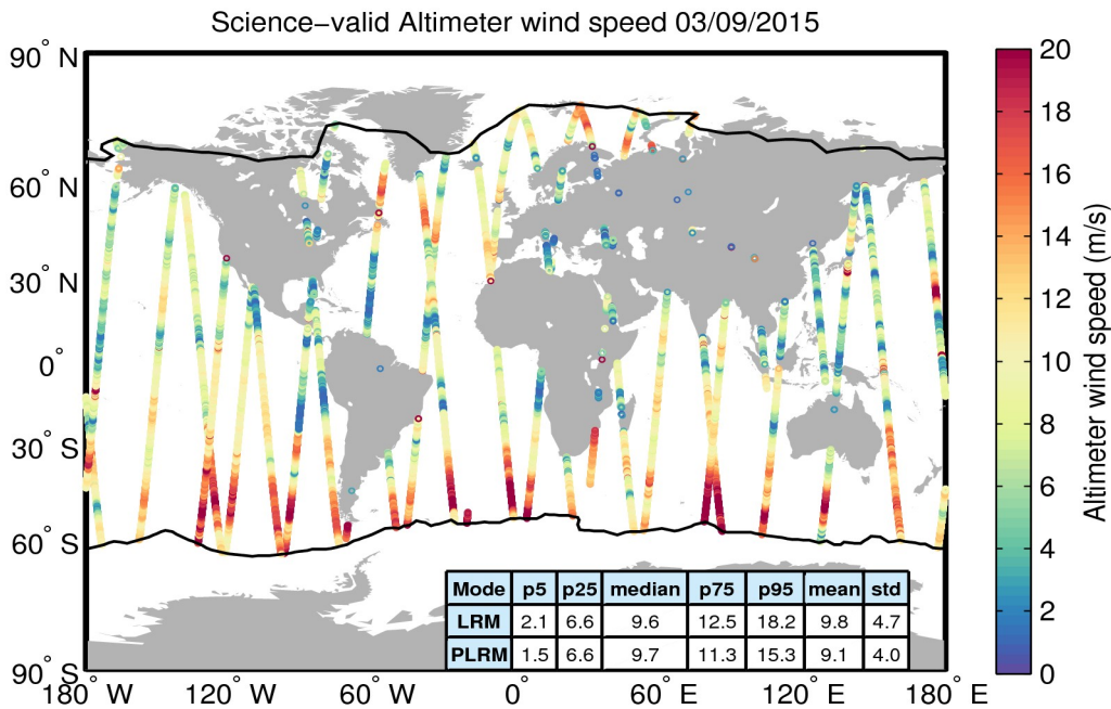
Figure 34. Geographical distribution of science-valid wind data over oceans and lakes for 03/09/2015. The statistical values shown in the table refer to the wind in m/s and are calculated separately for LRM and PLRM regions. The black lines mark the outer limit of the Arctic and Antarctic polar polygons. Gray circles denote records that have been rejected based on the editing criteria described in Table 5.
