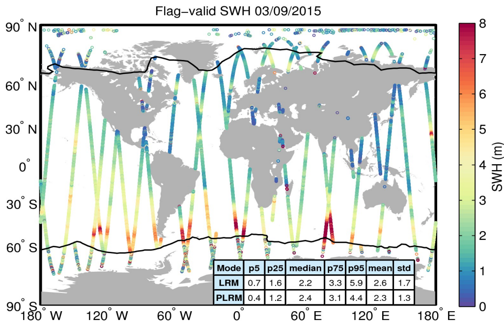
Figure 15. Geographical distribution of flag-valid SWH data over oceans and lakes for 03/09/2015. The statistical values shown in the table refer to the SWH in m and are calculated separately for LRM and PLRM regions. Measurements taken over polar polygons have been excluded from the computation of the statistical values. The black lines mark the outer limit of the Arctic and Antarctic polar polygons.
