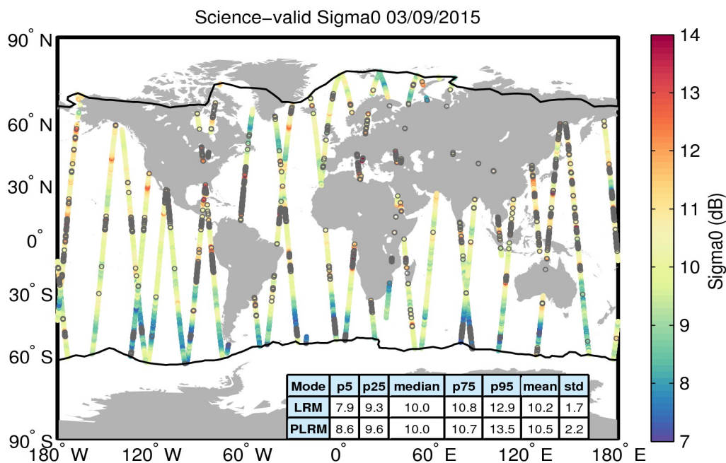
Figure 27. Geographical distribution of science-valid sigma0 data over oceans and lakes for 03/09/2015. The statistical values shown in the table refer to the sigma0 in dB and are calculated separately for LRM and PLRM regions. The black lines mark the outer limit of the Arctic and Antarctic polar polygons. Gray circles denote records that have been rejected based on the editing criteria described in Table 4.
