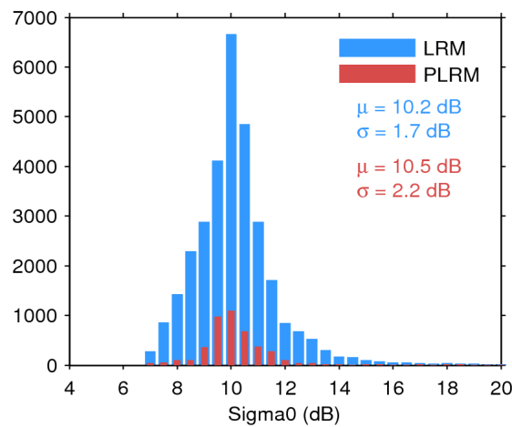
Figure 28. Histogram of science-valid sigma0 over oceans and lakes for LRM (blue) and PLRM (red) for 03/09/2015. The mean ( \mu ) and standard deviation ( \sigma ) are also shown. Note that values outside [4 20] dB are excluded from the histogram for the sake of readability but not from the computation of \mu and \sigma .
