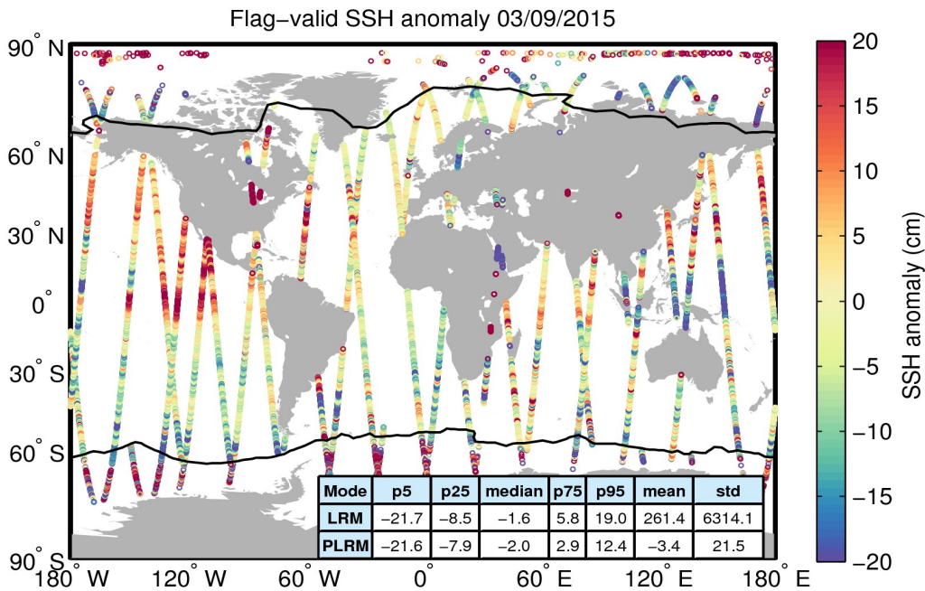
Figure 5. Geographical distribution of flag-valid 1-Hz SSH anomaly data over oceans and lakes for 03/09/2015. The statistical values shown in the table refer to the SSH anomaly in cm and are calculated separately for LRM and PLRM regions. Measurements taken over polar polygons have been excluded from the computation of the statistical values. The black lines mark the outer limit of the Arctic and Antarctic polar polygons.
