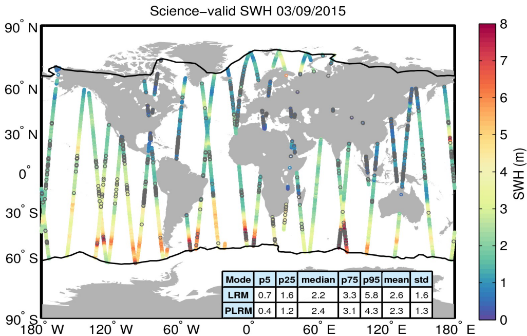
Figure 19. Geographical distribution of science-valid SWH data over oceans and lakes for 03/09/2015. The statistical values shown in the table refer to the SWH in m and are calculated separately for LRM and PLRM regions. The black lines mark the outer limit of the Arctic and Antarctic polar polygons. Gray circles denote records that have been rejected based on the editing criteria described in Table 3.
