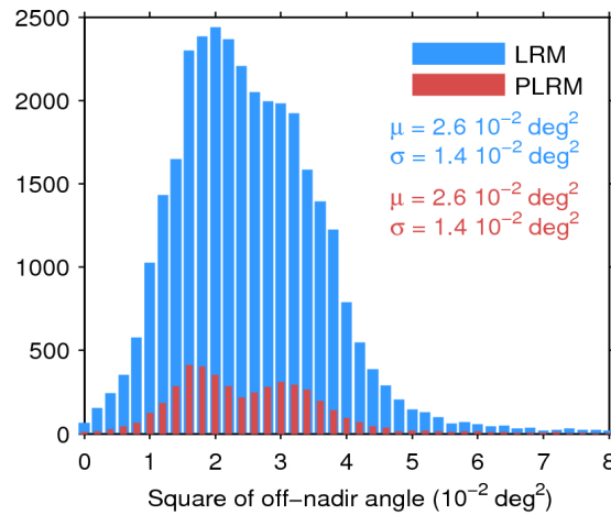
Figure 39. Histogram of flag-valid mispointing over oceans and lakes for LRM (blue) and PLRM (red) for 03/09/2015. Only positive values have been considered. The mean ( \mu ) and standard deviation ( \sigma ) are also shown. Note that values larger than 8 \cdot 10^{-2} \text{ deg}^2 are excluded from the histogram for the sake of readability but not from the computation of \mu and \sigma .
