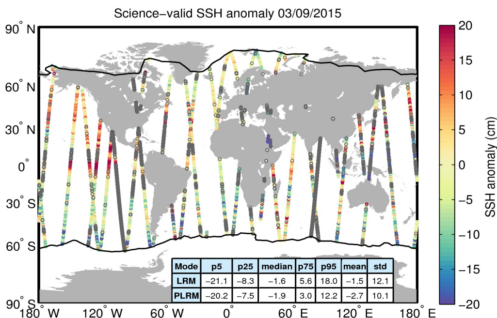
Figure 10. Geographical distribution of science-valid SSH anomaly data over oceans and lakes for 03/09/2015. The statistical values shown in the table refer to the SSH anomaly in cm and are calculated separately for LRM and PLRM regions. The black lines mark the outer limit of the Arctic and Antarctic polar polygons. Gray circles denote records that have been rejected based on the editing criteria described in Table 2.
