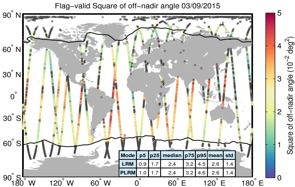
Figure 37. Geographical distribution of flag-valid mispointing data over oceans and lakes for 03/09/2015. The statistical values shown in the table refer to the mispointing in 10^{-2} deg 2 and are calculated separately for LRM and PLRM regions. Measurements taken over polar polygons have been excluded from the computation of the statistical values. The black lines mark the outer limit of the Arctic and Antarctic polar polygons. Gray circles denote negative values.
