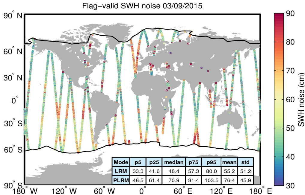
Figure 18. Geographical distribution of flag-valid 20-Hz SWH measurement noise over oceans and lakes for 03/09/2015. The statistical values shown in the table refer to the SWH noise and are calculated separately for LRM and PLRM regions. Measurements taken over polar polygons have been excluded from the computation of the statistical values. The black lines mark the outer limit of the Arctic and Antarctic polar polygons.
