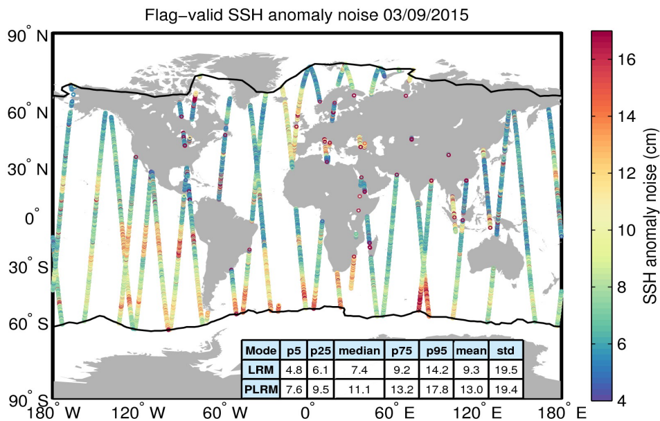
Figure 8. Geographical distribution of flag-valid 20-Hz SSH anomaly measurement noise over oceans and lakes for 03/09/2015. The statistical values shown in the table refer to the SSH anomaly noise and are calculated separately for LRM and PLRM regions. Measurements taken over polar polygons have been excluded from the computation of the statistical values. The black lines mark the outer limit of the Arctic and Antarctic polar polygons.
