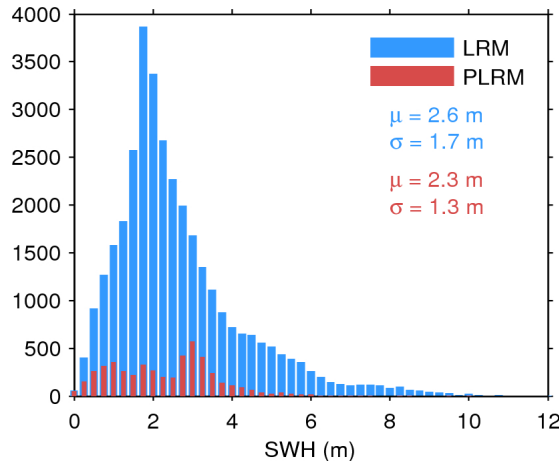
Figure 17. Histogram of flag-valid SWH over oceans and lakes for LRM (blue) and PLRM (red) for 03/09/2015. The mean ( \mu ) and standard deviation ( \sigma ) are also shown. Note that values larger than 12 m are excluded from the histogram for the sake of readability but not from the computation of \mu and \sigma .
