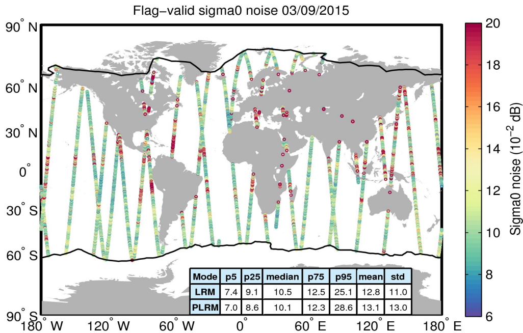
Figure 26. Geographical distribution of flag-valid 20-Hz sigma0 measurement noise over oceans and lakes for 03/09/2015. The statistical values shown in the table refer to the sigma0 noise and are calculated separately for LRM and PLRM regions. Measurements taken over polar polygons have been excluded from the computation of the statistical values. The black lines mark the outer limit of the Arctic and Antarctic polar polygons.
