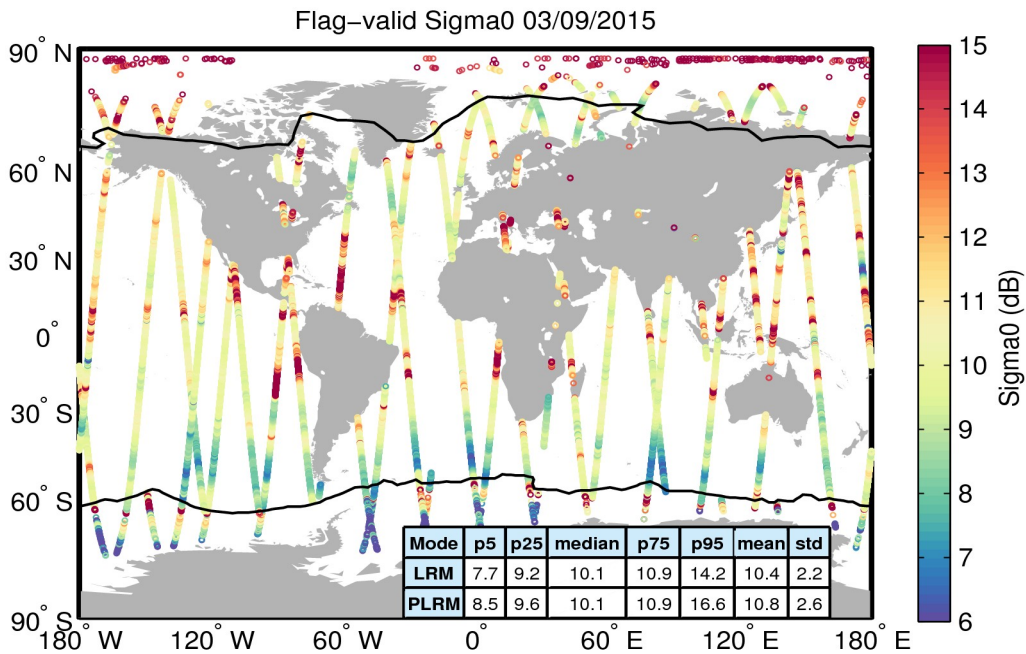
Figure 23. Geographical distribution of flag-valid sigma0 data over oceans and lakes for 03/09/2015. The statistical values shown in the table refer to the sigma0 in dB and are calculated separately for LRM and PLRM regions. Measurements taken over polar polygons have been excluded from the computation of the statistical values. The black lines mark the outer limit of the Arctic and Antarctic polar polygons.
