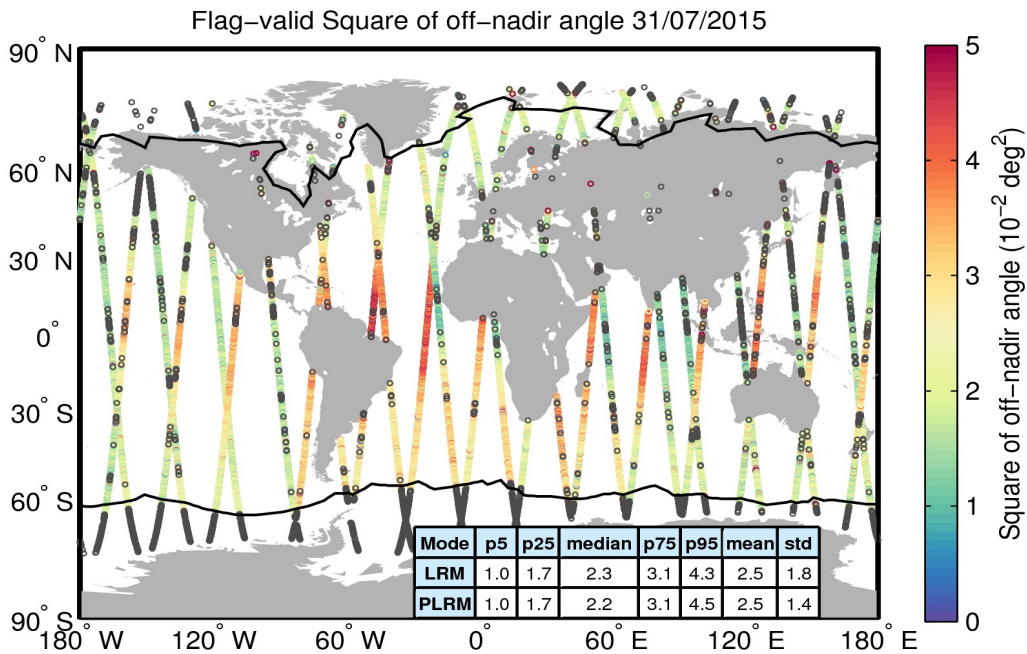
Figure 37. Geographical distribution of flag-valid mispointing data over oceans and lakes for 31/07/2015. The statistical values shown in the table refer to the mispointing in 10^{-2} \text{ deg}^2 and are calculated separately for LRM and PLRM regions. Measurements taken over polar polygons have been excluded from the computation of the statistical values. The black lines mark the outer limit of the Arctic and Antarctic polar polygons. Gray circles denote negative values.
