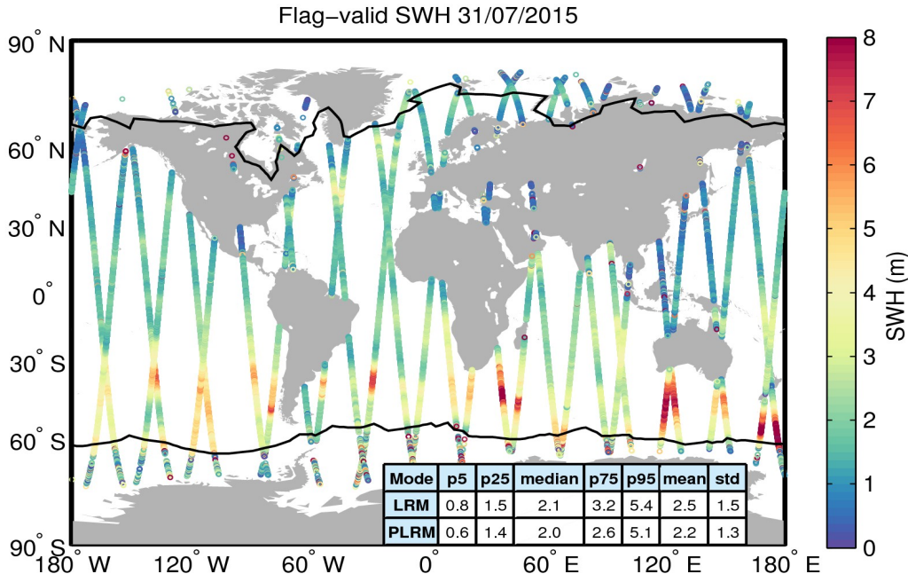
Figure 15. Geographical distribution of flag-valid SWH data over oceans and lakes for 31/07/2015. The statistical values shown in the table refer to the SWH in m and are calculated separately for LRM and PLRM regions. Measurements taken over polar polygons have been excluded from the computation of the statistical values. The black lines mark the outer limit of the Arctic and Antarctic polar polygons.
