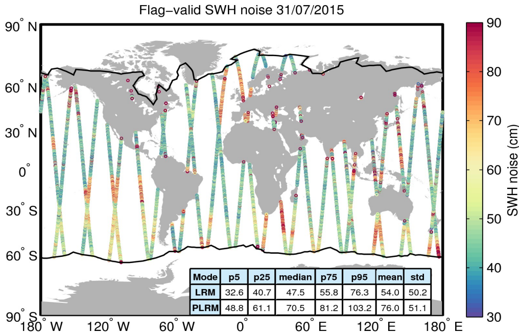
Figure 18. Geographical distribution of flag-valid 20-Hz SWH measurement noise over oceans and lakes for 31/07/2015. The statistical values shown in the table refer to the SWH noise and are calculated separately for LRM and PLRM regions. Measurements taken over polar polygons have been excluded from the computation of the statistical values. The black lines mark the outer limit of the Arctic and Antarctic polar polygons.
