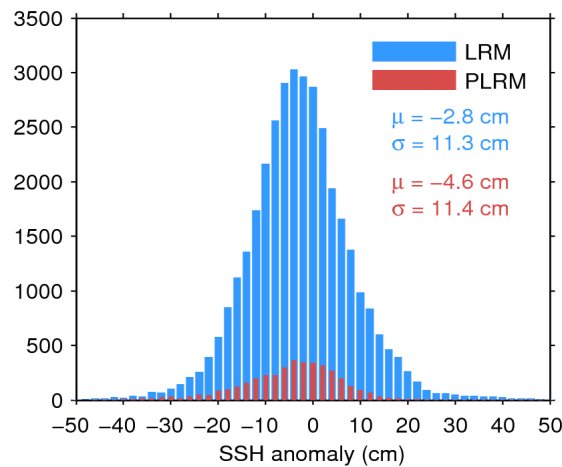
Figure 11. Histogram of science-valid SSH anomaly over oceans and lakes for LRM (blue) and PLRM (red) for 31/07/2015. The mean ( \mu ) and standard deviation ( \sigma ) are also shown. Note that values outside [-50 50] cm are excluded from the histogram for the sake of readability but not from the computation of \mu and \sigma .
