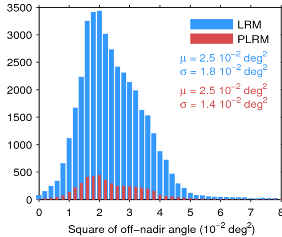
Figure 39. Histogram of flag-valid mispointing over oceans and lakes for LRM (blue) and PLRM (red) for 31/07/2015. Only positive values have been considered. The mean ( \mu ) and standard deviation ( \sigma ) are also shown. Note that values larger than 8 \cdot 10^{-2} \text{ deg}^2 are excluded from the histogram for the sake of readability but not from the computation of \mu and \sigma .
