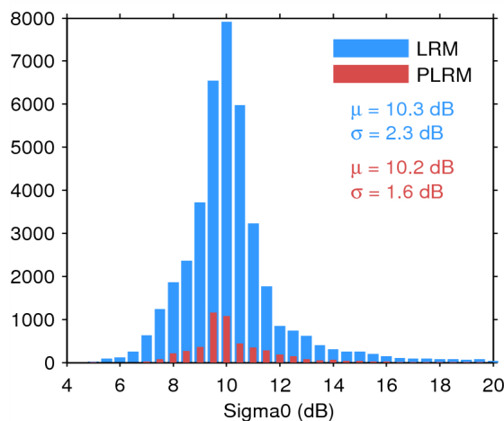
Figure 25. Histogram of flag-valid sigma0 over oceans and lakes for LRM (blue) and PLRM (red) for 31/07/2015. The mean ( \mu ) and standard deviation ( \sigma ) are also shown. Note that values outside [4 20] dB are excluded from the histogram for the sake of readability but not from the computation of \mu and \sigma .
