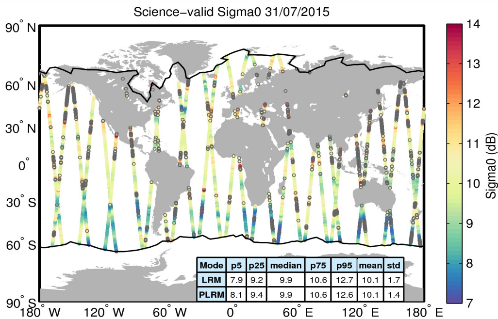
Figure 27. Geographical distribution of science-valid sigma0 data over oceans and lakes for 31/07/2015. The statistical values shown in the table refer to the sigma0 in dB and are calculated separately for LRM and PLRM regions. The black lines mark the outer limit of the Arctic and Antarctic polar polygons. Gray circles denote records that have been rejected based on the editing criteria described in Table 4.
