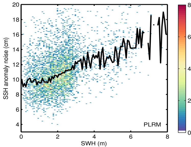
Figure 9. 2D histogram showing flag-valid SSH anomaly noise as a function of SWH for LRM (top) and PLRM (bottom) for 31/07/2015. The black line denotes the median SSH anomaly as a function of SWH.
