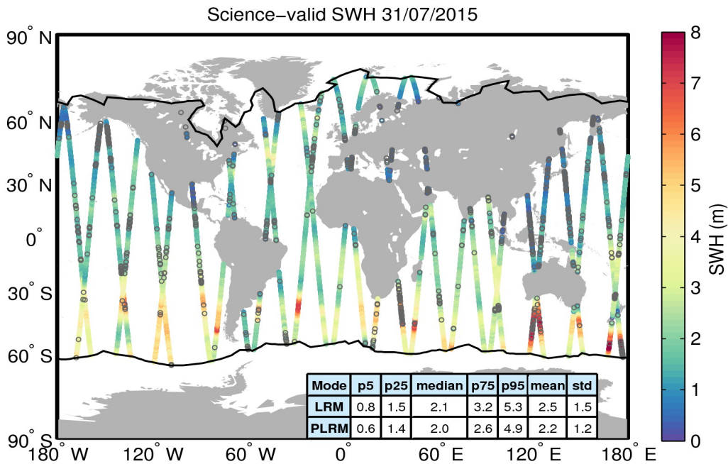
Figure 19. Geographical distribution of science-valid SWH data over oceans and lakes for 31/07/2015. The statistical values shown in the table refer to the SWH in m and are calculated separately for LRM and PLRM regions. The black lines mark the outer limit of the Arctic and Antarctic polar polygons. Gray circles denote records that have been rejected based on the editing criteria described in Table 3.
