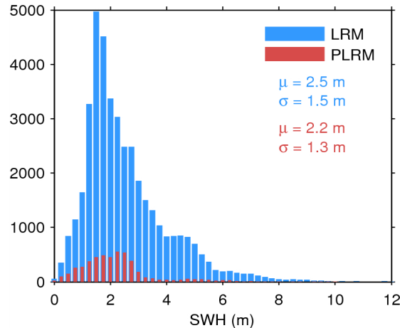
Figure 17. Histogram of flag-valid SWH over oceans and lakes for LRM (blue) and PLRM (red) for 31/07/2015. The mean ( \mu ) and standard deviation ( \sigma ) are also shown. Note that values larger than 12 m are excluded from the histogram for the sake of readability but not from the computation of \mu and \sigma .
