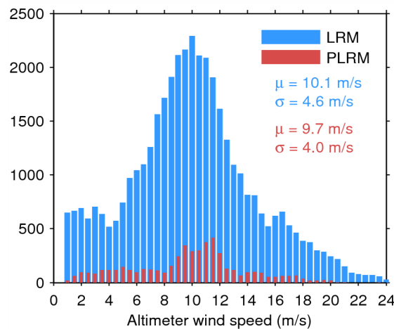
Figure 35. Histogram of science-valid wind over oceans and lakes for LRM (blue) and PLRM (red) for 31/07/2015. The mean ( \mu ) and standard deviation ( \sigma ) are also shown. Note that values larger than 24 m/s are excluded from the histogram for the sake of readability but not from the computation of \mu and \sigma .
