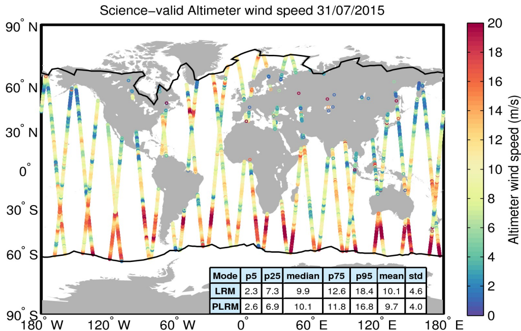
Figure 34. Geographical distribution of science-valid wind data over oceans and lakes for 31/07/2015. The statistical values shown in the table refer to the wind in m/s and are calculated separately for LRM and PLRM regions. The black lines mark the outer limit of the Arctic and Antarctic polar polygons. Gray circles denote records that have been rejected based on the editing criteria described in Table 5.
