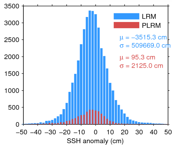
Figure 7. Histogram of flag-valid SSH anomaly over oceans and lakes for LRM (blue) and PLRM (red) for 31/07/2015. The mean ( \mu ) and standard deviation ( \sigma ) are also shown. Note that values outside [-50\ 50] cm are excluded from the histogram for the sake of readability but not from the computation of \mu and \sigma .
