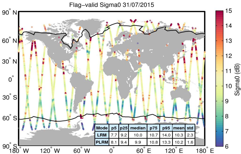
Figure 23. Geographical distribution of flag-valid sigma0 data over oceans and lakes for 31/07/2015. The statistical values shown in the table refer to the sigma0 in dB and are calculated separately for LRM and PLRM regions. Measurements taken over polar polygons have been excluded from the computation of the statistical values. The black lines mark the outer limit of the Arctic and Antarctic polar polygons.
