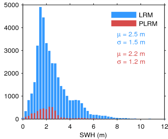
Figure 20. Histogram of science-valid SWH over oceans and lakes for LRM (blue) and PLRM (red) for 31/07/2015. The mean ( \mu ) and standard deviation ( \sigma ) are also shown. Note that values larger than 12 m are excluded from the histogram for the sake of readability but not from the computation of \mu and \sigma .
