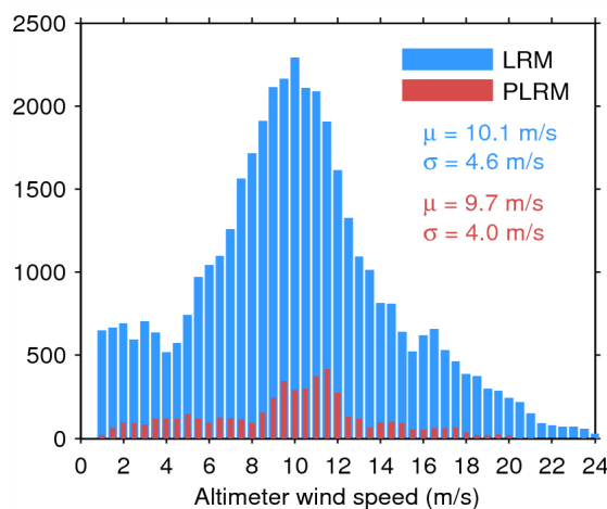
Figure 33. Histogram of flag-valid wind over oceans and lakes for LRM (blue) and PLRM (red) for 31/07/2015. The mean ( \mu ) and standard deviation ( \sigma ) are also shown. Note that values larger than 24 m/s are excluded from the histogram for the sake of readability but not from the computation of \mu and \sigma .
