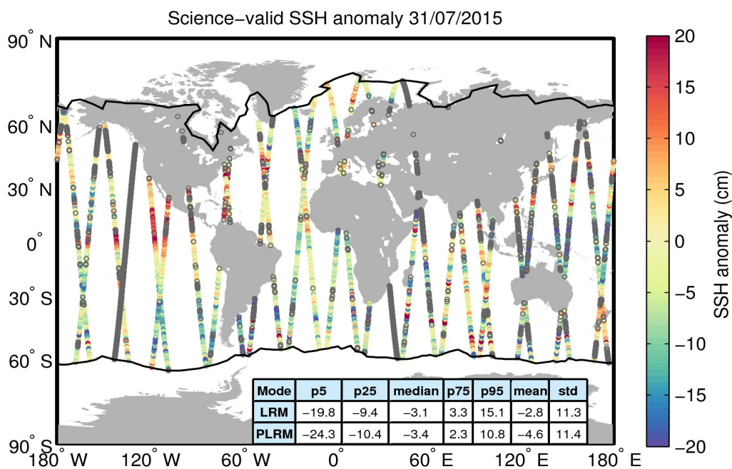
Figure 10. Geographical distribution of science-valid SSH anomaly data over oceans and lakes for 31/07/2015. The statistical values shown in the table refer to the SSH anomaly in cm and are calculated separately for LRM and PLRM regions. The black lines mark the outer limit of the Arctic and Antarctic polar polygons. Gray circles denote records that have been rejected based on the editing criteria described in Table 2.
