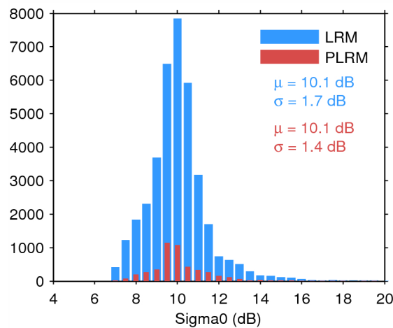
Figure 28. Histogram of science-valid sigma0 over oceans and lakes for LRM (blue) and PLRM (red) for 31/07/2015. The mean ( \mu ) and standard deviation ( \sigma ) are also shown. Note that values outside [4 20] dB are excluded from the histogram for the sake of readability but not from the computation of \mu and \sigma .
