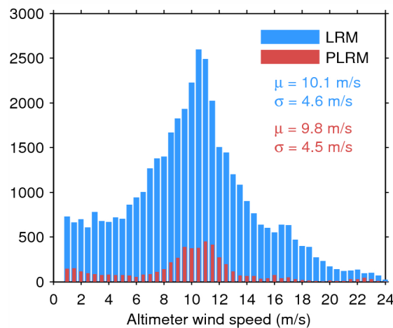
Figure 35. Histogram of science-valid wind over oceans and lakes for LRM (blue) and PLRM (red) for 30/07/2015. The mean ( \mu ) and standard deviation ( \sigma ) are also shown. Note that values larger than 24 m/s are excluded from the histogram for the sake of readability but not from the computation of \mu and \sigma .
