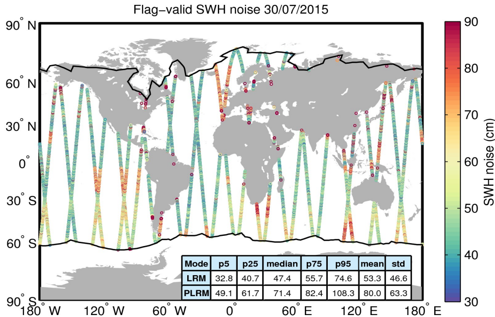
Figure 18. Geographical distribution of flag-valid 20-Hz SWH measurement noise over oceans and lakes for 30/07/2015. The statistical values shown in the table refer to the SWH noise and are calculated separately for LRM and PLRM regions. Measurements taken over polar polygons have been excluded from the computation of the statistical values. The black lines mark the outer limit of the Arctic and Antarctic polar polygons.
