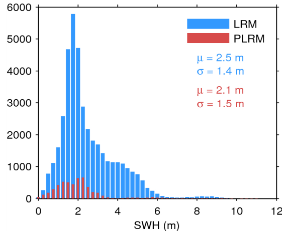
Figure 17. Histogram of flag-valid SWH over oceans and lakes for LRM (blue) and PLRM (red) for 30/07/2015. The mean ( \mu ) and standard deviation ( \sigma ) are also shown. Note that values larger than 12 m are excluded from the histogram for the sake of readability but not from the computation of \mu and \sigma .
