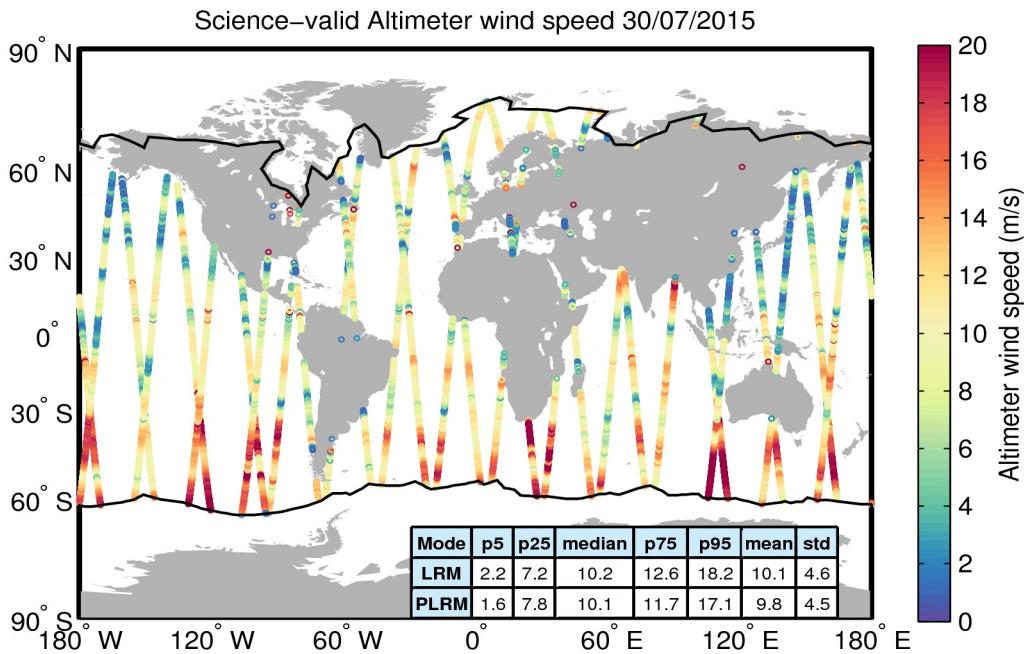
Figure 34. Geographical distribution of science-valid wind data over oceans and lakes for 30/07/2015. The statistical values shown in the table refer to the wind in m/s and are calculated separately for LRM and PLRM regions. The black lines mark the outer limit of the Arctic and Antarctic polar polygons. Gray circles denote records that have been rejected based on the editing criteria described in Table 5.
