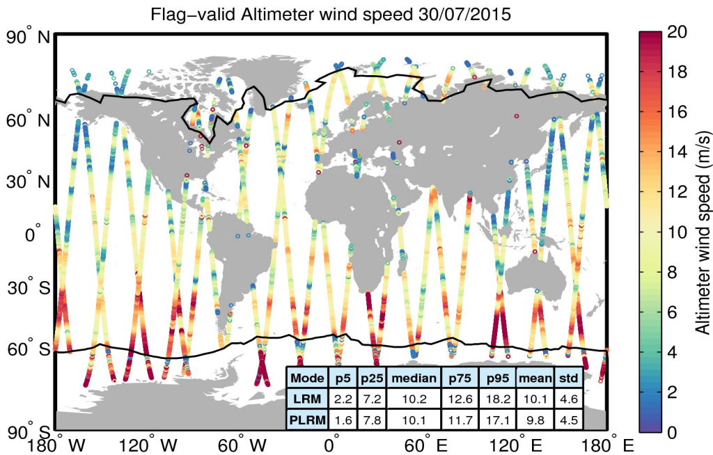
Figure 31. Geographical distribution of flag-valid wind data over oceans and lakes for 30/07/2015. The statistical values shown in the table refer to the wind in m/s and are calculated separately for LRM and PLRM regions. Measurements taken over polar polygons have been excluded from the computation of the statistical values. The black lines mark the outer limit of the Arctic and Antarctic polar polygons.
