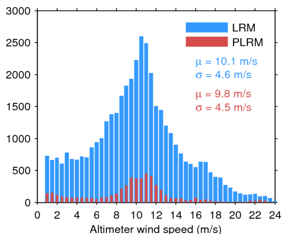
Figure 33. Histogram of flag-valid wind over oceans and lakes for LRM (blue) and PLRM (red) for 30/07/2015. The mean ( \mu ) and standard deviation ( \sigma ) are also shown. Note that values larger than 24 m/s are excluded from the histogram for the sake of readability but not from the computation of \mu and \sigma .
