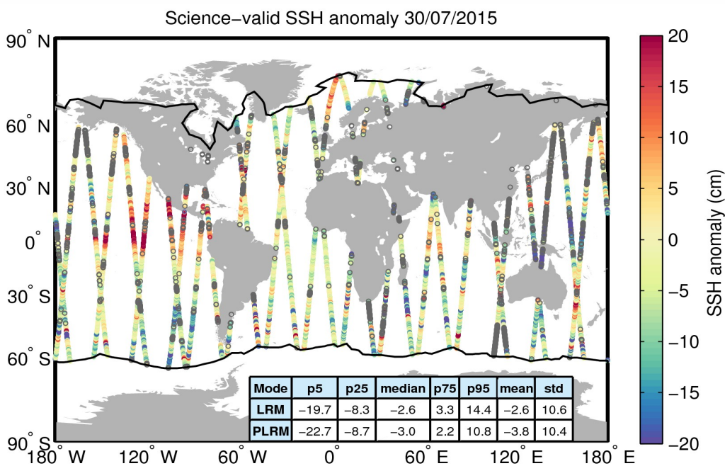
Figure 10. Geographical distribution of science-valid SSH anomaly data over oceans and lakes for 30/07/2015. The statistical values shown in the table refer to the SSH anomaly in cm and are calculated separately for LRM and PLRM regions. The black lines mark the outer limit of the Arctic and Antarctic polar polygons. Gray circles denote records that have been rejected based on the editing criteria described in Table 2.
