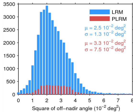
Figure 39. Histogram of flag-valid mispointing over oceans and lakes for LRM (blue) and PLRM (red) for 30/07/2015. Only positive values have been considered. The mean ( \mu ) and standard deviation ( \sigma ) are also shown. Note that values larger than 8 \cdot 10^{-2} \text{ deg}^2 are excluded from the histogram for the sake of readability but not from the computation of \mu and \sigma .
