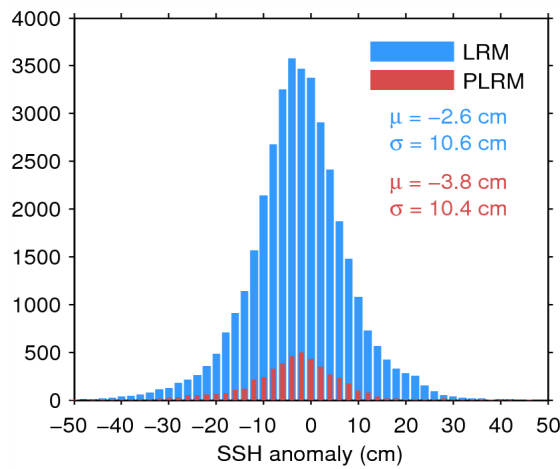
Figure 11. Histogram of science-valid SSH anomaly over oceans and lakes for LRM (blue) and PLRM (red) for 30/07/2015. The mean ( \mu ) and standard deviation ( \sigma ) are also shown. Note that values outside [-50\ 50] cm are excluded from the histogram for the sake of readability but not from the computation of \mu and \sigma .
