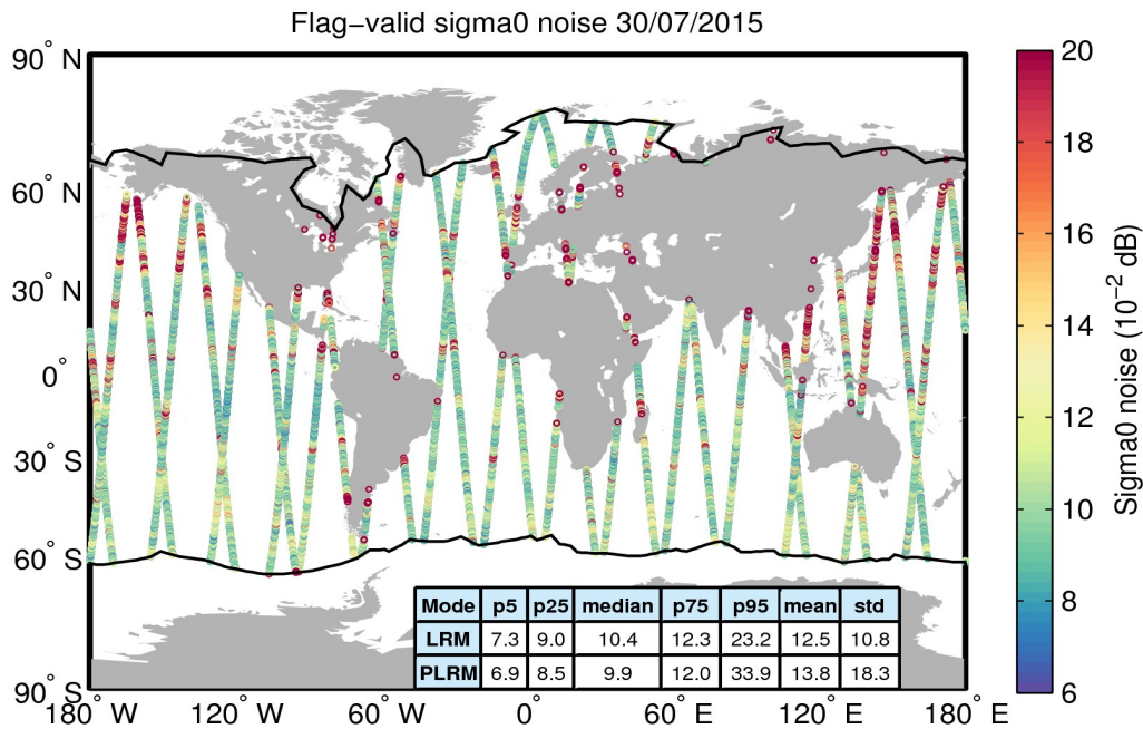
Figure 26. Geographical distribution of flag-valid 20-Hz sigma0 measurement noise over oceans and lakes for 30/07/2015. The statistical values shown in the table refer to the sigma0 noise and are calculated separately for LRM and PLRM regions. Measurements taken over polar polygons have been excluded from the computation of the statistical values. The black lines mark the outer limit of the Arctic and Antarctic polar polygons.
