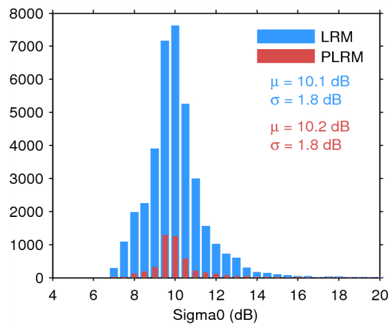
Figure 28. Histogram of science-valid sigma0 over oceans and lakes for LRM (blue) and PLRM (red) for 30/07/2015. The mean ( \mu ) and standard deviation ( \sigma ) are also shown. Note that values outside [4 20] dB are excluded from the histogram for the sake of readability but not from the computation of \mu and \sigma .
