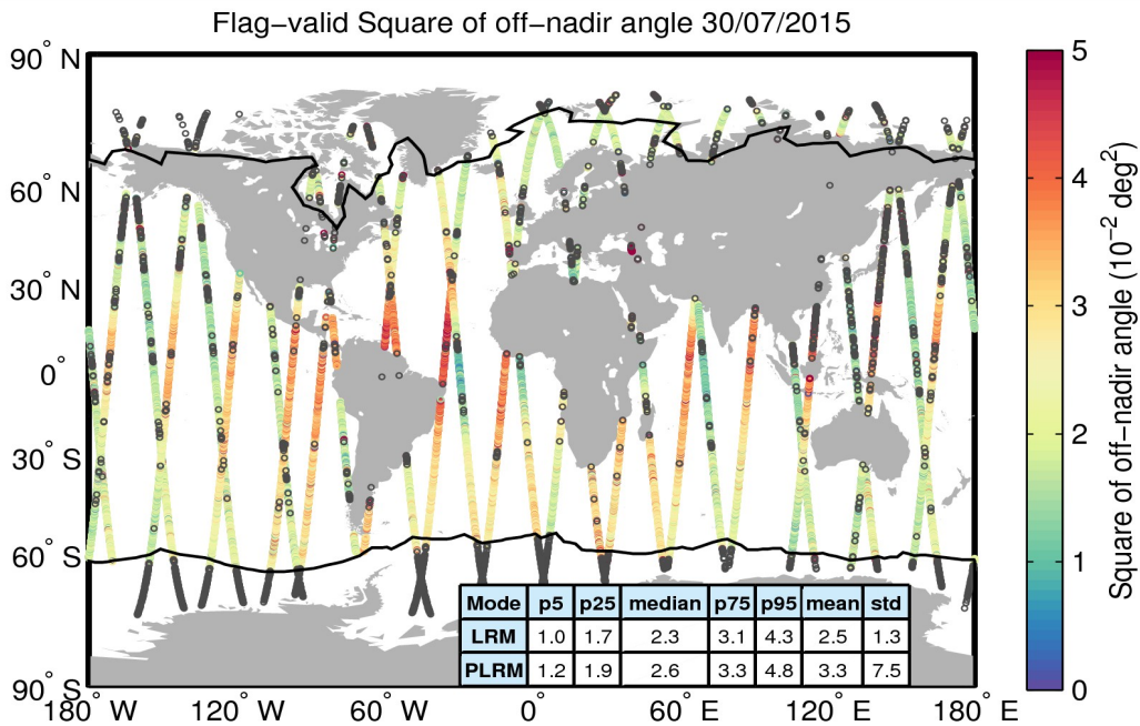
Figure 37. Geographical distribution of flag-valid mispointing data over oceans and lakes for 30/07/2015. The statistical values shown in the table refer to the mispointing in 10^{-2} deg 2 and are calculated separately for LRM and PLRM regions. Measurements taken over polar polygons have been excluded from the computation of the statistical values. The black lines mark the outer limit of the Arctic and Antarctic polar polygons. Gray circles denote negative values.
