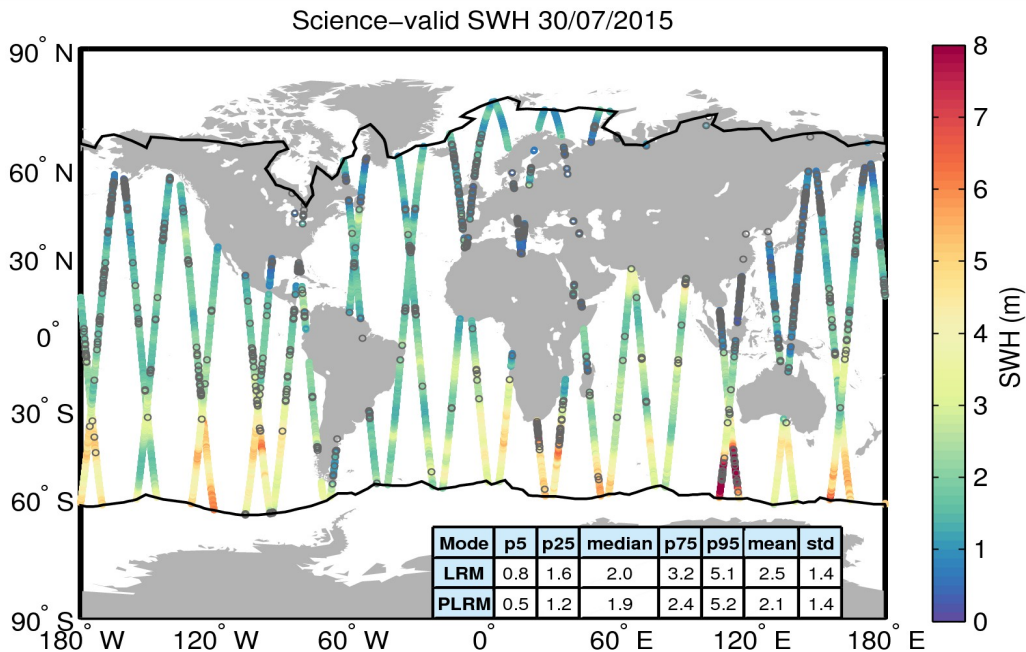
Figure 19. Geographical distribution of science-valid SWH data over oceans and lakes for 30/07/2015. The statistical values shown in the table refer to the SWH in m and are calculated separately for LRM and PLRM regions. The black lines mark the outer limit of the Arctic and Antarctic polar polygons. Gray circles denote records that have been rejected based on the editing criteria described in Table 3.
