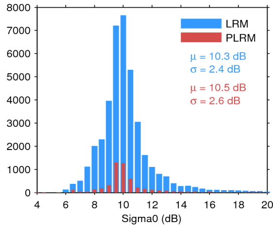
Figure 25. Histogram of flag-valid sigma0 over oceans and lakes for LRM (blue) and PLRM (red) for 30/07/2015. The mean ( \mu ) and standard deviation ( \sigma ) are also shown. Note that values outside [4 20] dB are excluded from the histogram for the sake of readability but not from the computation of \mu and \sigma .
