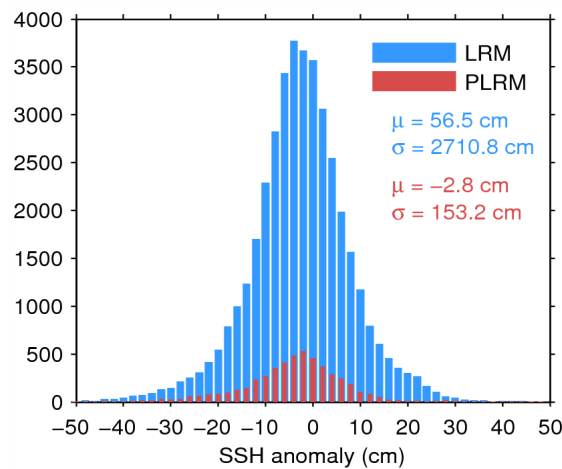
Figure 7. Histogram of flag-valid SSH anomaly over oceans and lakes for LRM (blue) and PLRM (red) for 30/07/2015. The mean ( \mu ) and standard deviation ( \sigma ) are also shown. Note that values outside [-50 \ 50] cm are excluded from the histogram for the sake of readability but not from the computation of \mu and \sigma .
