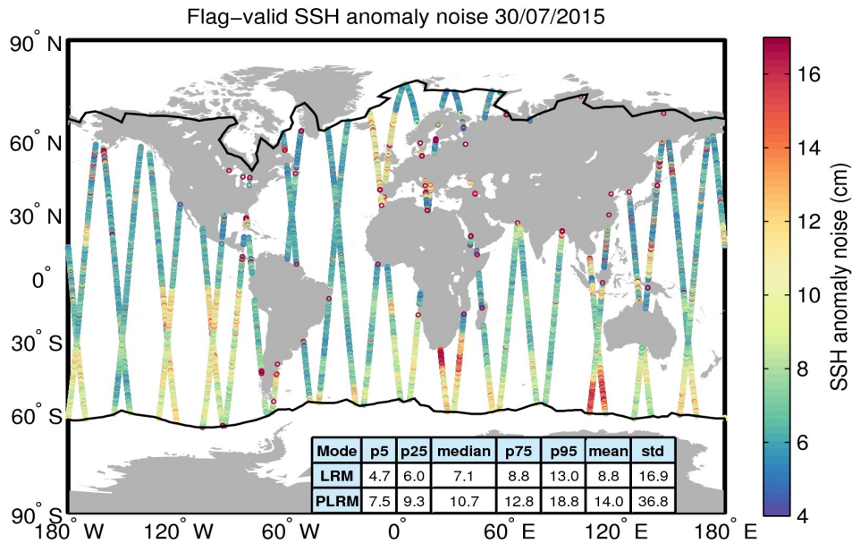
Figure 8. Geographical distribution of flag-valid 20-Hz SSH anomaly measurement noise over oceans and lakes for 30/07/2015. The statistical values shown in the table refer to the SSH anomaly noise and are calculated separately for LRM and PLRM regions. Measurements taken over polar polygons have been excluded from the computation of the statistical values. The black lines mark the outer limit of the Arctic and Antarctic polar polygons.
