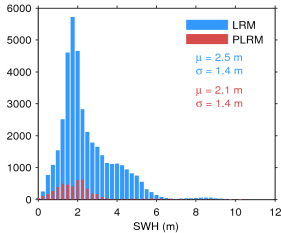
Figure 20. Histogram of science-valid SWH over oceans and lakes for LRM (blue) and PLRM (red) for 30/07/2015. The mean ( \mu ) and standard deviation ( \sigma ) are also shown. Note that values larger than 12 m are excluded from the histogram for the sake of readability but not from the computation of \mu and \sigma .
