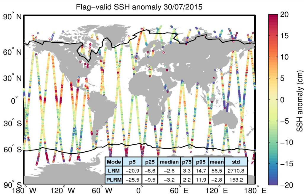
Figure 5. Geographical distribution of flag-valid 1-Hz SSH anomaly data over oceans and lakes for 30/07/2015. The statistical values shown in the table refer to the SSH anomaly in cm and are calculated separately for LRM and PLRM regions. Measurements taken over polar polygons have been excluded from the computation of the statistical values. The black lines mark the outer limit of the Arctic and Antarctic polar polygons.
