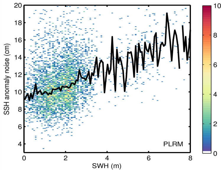
Figure 9. 2D histogram showing flag-valid SSH anomaly noise as a function of SWH for LRM (top) and PLRM (bottom) for 30/07/2015. The black line denotes the median SSH anomaly as a function of SWH.
