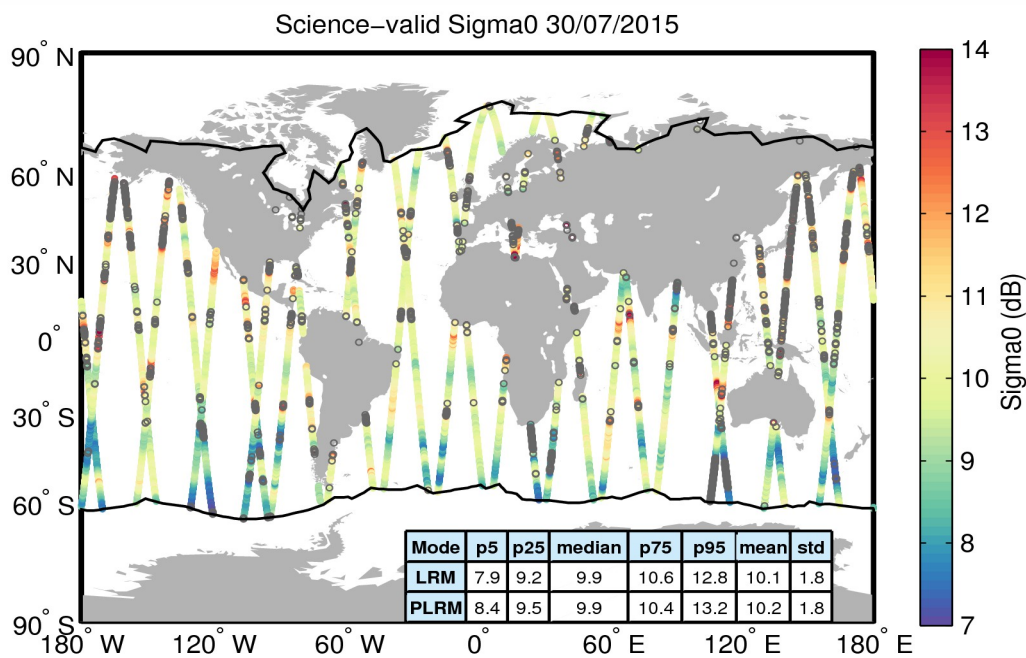
Figure 27. Geographical distribution of science-valid sigma0 data over oceans and lakes for 30/07/2015. The statistical values shown in the table refer to the sigma0 in dB and are calculated separately for LRM and PLRM regions. The black lines mark the outer limit of the Arctic and Antarctic polar polygons. Gray circles denote records that have been rejected based on the editing criteria described in Table 4.
