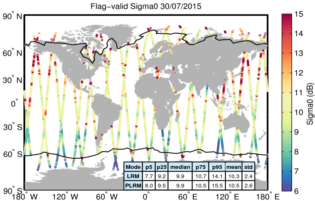
Figure 23. Geographical distribution of flag-valid sigma0 data over oceans and lakes for 30/07/2015. The statistical values shown in the table refer to the sigma0 in dB and are calculated separately for LRM and PLRM regions. Measurements taken over polar polygons have been excluded from the computation of the statistical values. The black lines mark the outer limit of the Arctic and Antarctic polar polygons.
