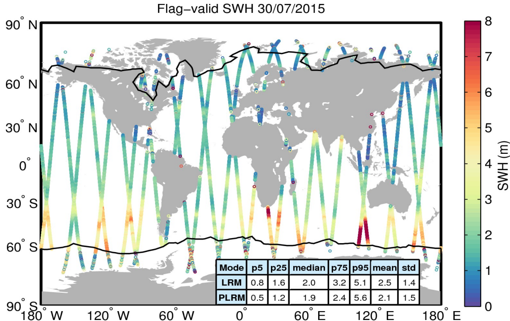
Figure 15. Geographical distribution of flag-valid SWH data over oceans and lakes for 30/07/2015. The statistical values shown in the table refer to the SWH in m and are calculated separately for LRM and PLRM regions. Measurements taken over polar polygons have been excluded from the computation of the statistical values. The black lines mark the outer limit of the Arctic and Antarctic polar polygons.
