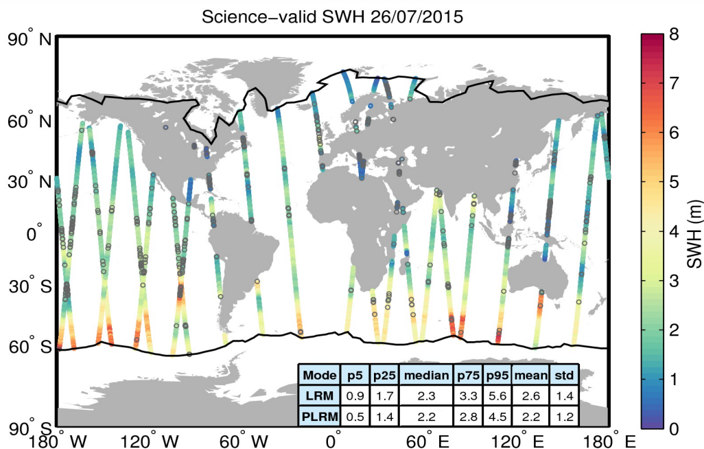
Figure 19. Geographical distribution of science-valid SWH data over oceans and lakes for 26/07/2015. The statistical values shown in the table refer to the SWH in m and are calculated separately for LRM and PLRM regions. The black lines mark the outer limit of the Arctic and Antarctic polar polygons. Gray circles denote records that have been rejected based on the editing criteria described in Table 3.
