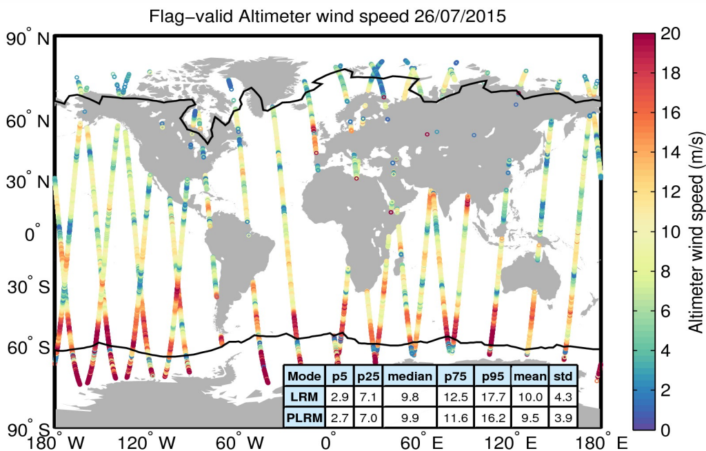
Figure 31. Geographical distribution of flag-valid wind data over oceans and lakes for 26/07/2015. The statistical values shown in the table refer to the wind in m/s and are calculated separately for LRM and PLRM regions. Measurements taken over polar polygons have been excluded from the computation of the statistical values. The black lines mark the outer limit of the Arctic and Antarctic polar polygons.
