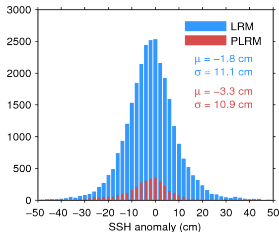
Figure 11. Histogram of science-valid SSH anomaly over oceans and lakes for LRM (blue) and PLRM (red) for 26/07/2015. The mean ( \mu ) and standard deviation ( \sigma ) are also shown. Note that values outside [-50 50] cm are excluded from the histogram for the sake of readability but not from the computation of \mu and \sigma .
