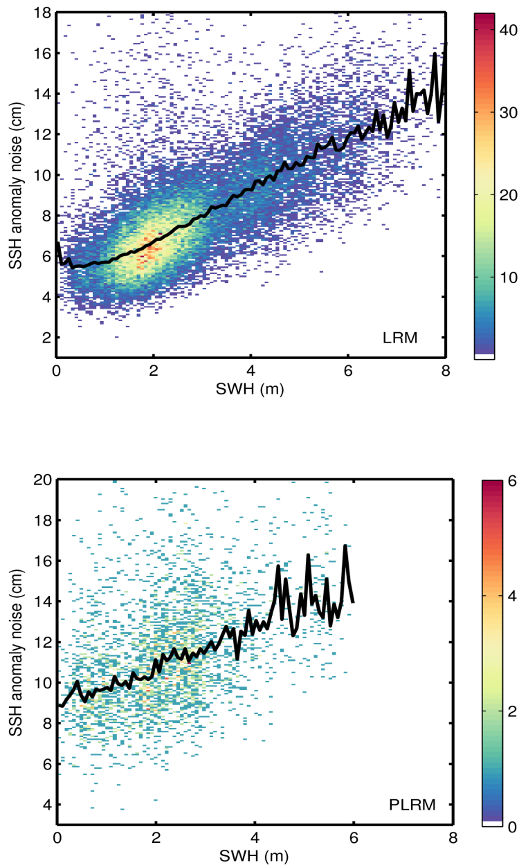
Figure 9. 2D histogram showing flag-valid SSH anomaly noise as a function of SWH for LRM (top) and PLRM (bottom) for 26/07/2015. The black line denotes the median SSH anomaly as a function of SWH.
