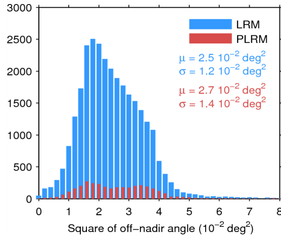
Figure 39. Histogram of flag-valid mispointing over oceans and lakes for LRM (blue) and PLRM (red) for 26/07/2015. Only positive values have been considered. The mean ( \mu ) and standard deviation ( \sigma ) are also shown. Note that values larger than 8 \cdot 10^{-2} \text{ deg}^2 are excluded from the histogram for the sake of readability but not from the computation of \mu and \sigma .
