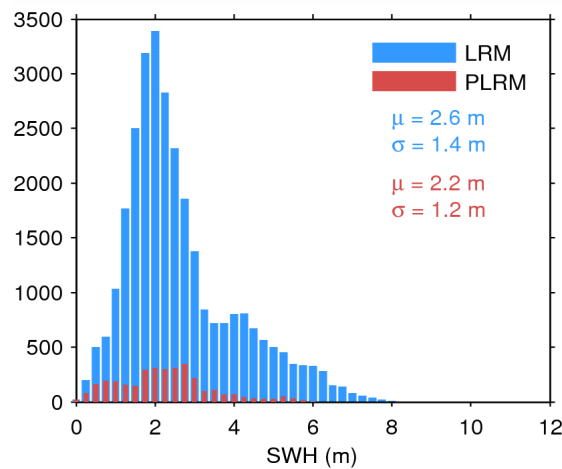
Figure 20. Histogram of science-valid SWH over oceans and lakes for LRM (blue) and PLRM (red) for 26/07/2015. The mean ( \mu ) and standard deviation ( \sigma ) are also shown. Note that values larger than 12 m are excluded from the histogram for the sake of readability but not from the computation of \mu and \sigma .
