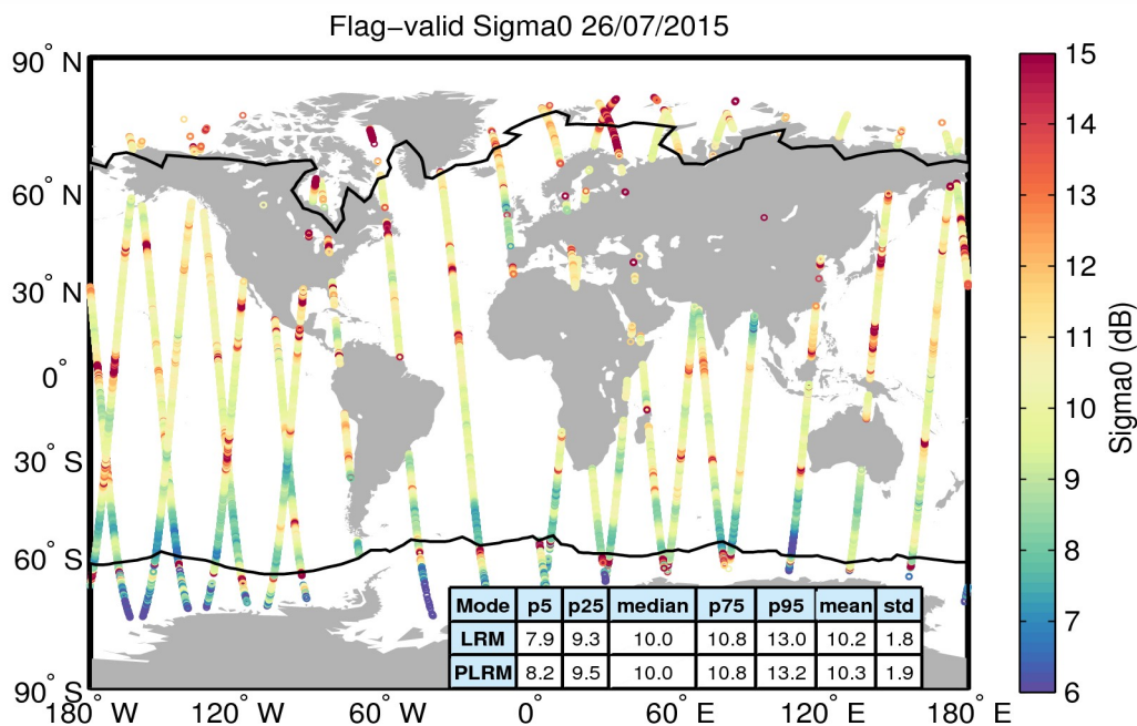
Figure 23. Geographical distribution of flag-valid sigma0 data over oceans and lakes for 26/07/2015. The statistical values shown in the table refer to the sigma0 in dB and are calculated separately for LRM and PLRM regions. Measurements taken over polar polygons have been excluded from the computation of the statistical values. The black lines mark the outer limit of the Arctic and Antarctic polar polygons.
