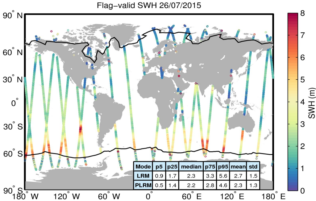
Figure 15. Geographical distribution of flag-valid SWH data over oceans and lakes for 26/07/2015. The statistical values shown in the table refer to the SWH in m and are calculated separately for LRM and PLRM regions. Measurements taken over polar polygons have been excluded from the computation of the statistical values. The black lines mark the outer limit of the Arctic and Antarctic polar polygons.
