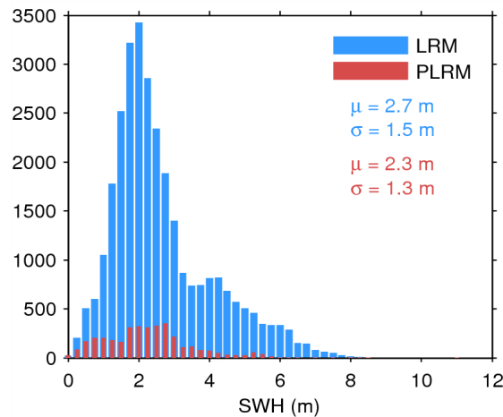
Figure 17. Histogram of flag-valid SWH over oceans and lakes for LRM (blue) and PLRM (red) for 26/07/2015. The mean ( \mu ) and standard deviation ( \sigma ) are also shown. Note that values larger than 12 m are excluded from the histogram for the sake of readability but not from the computation of \mu and \sigma .
