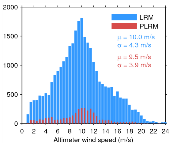
Figure 35. Histogram of science-valid wind over oceans and lakes for LRM (blue) and PLRM (red) for 26/07/2015. The mean ( \mu ) and standard deviation ( \sigma ) are also shown. Note that values larger than 24 m/s are excluded from the histogram for the sake of readability but not from the computation of \mu and \sigma .
