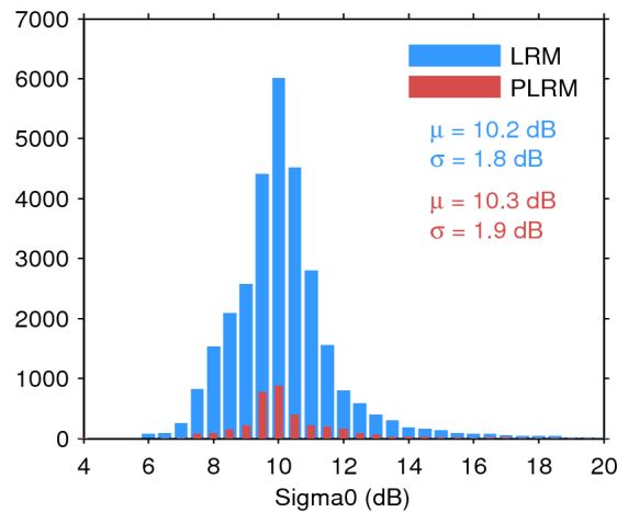
Figure 25. Histogram of flag-valid sigma0 over oceans and lakes for LRM (blue) and PLRM (red) for 26/07/2015. The mean ( \mu ) and standard deviation ( \sigma ) are also shown. Note that values outside [4 20] dB are excluded from the histogram for the sake of readability but not from the computation of \mu and \sigma .
