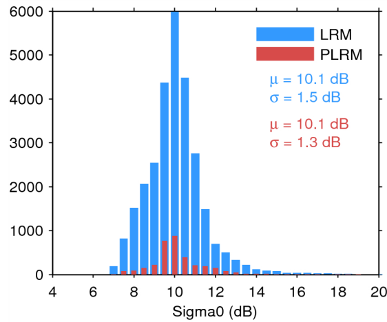
Figure 28. Histogram of science-valid sigma0 over oceans and lakes for LRM (blue) and PLRM (red) for 26/07/2015. The mean ( \mu ) and standard deviation ( \sigma ) are also shown. Note that values outside [4 20] dB are excluded from the histogram for the sake of readability but not from the computation of \mu and \sigma .
