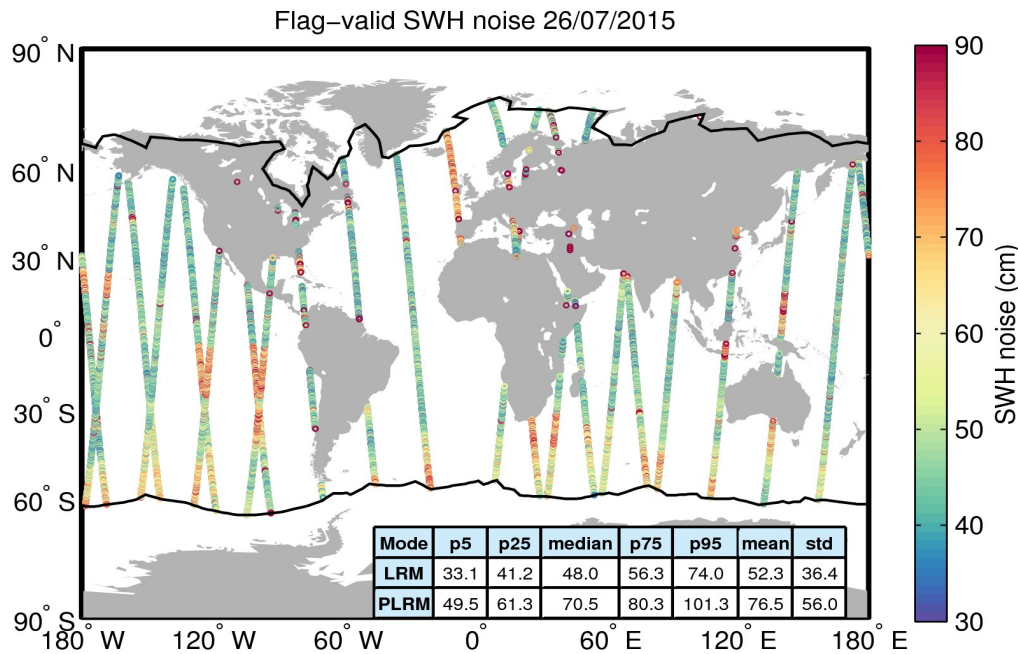
Figure 18. Geographical distribution of flag-valid 20-Hz SWH measurement noise over oceans and lakes for 26/07/2015. The statistical values shown in the table refer to the SWH noise and are calculated separately for LRM and PLRM regions. Measurements taken over polar polygons have been excluded from the computation of the statistical values. The black lines mark the outer limit of the Arctic and Antarctic polar polygons.
