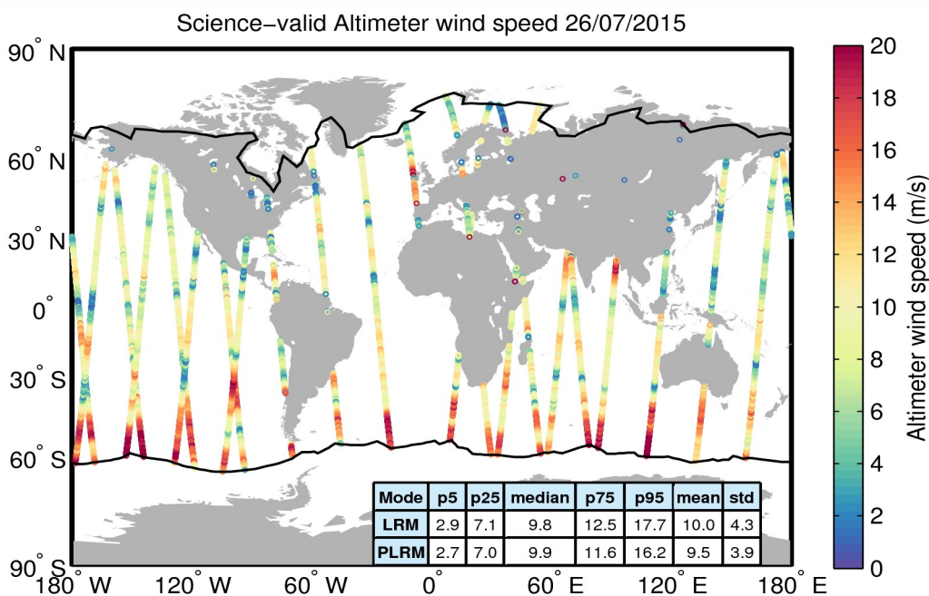
Figure 34. Geographical distribution of science-valid wind data over oceans and lakes for 26/07/2015. The statistical values shown in the table refer to the wind in m/s and are calculated separately for LRM and PLRM regions. The black lines mark the outer limit of the Arctic and Antarctic polar polygons. Gray circles denote records that have been rejected based on the editing criteria described in Table 5.
