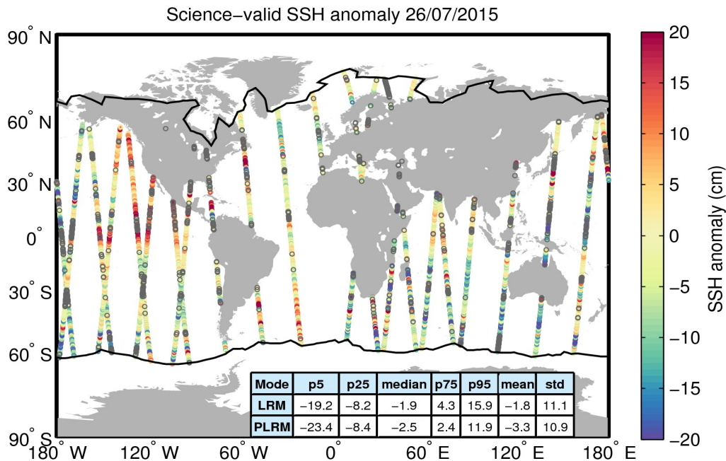
Figure 10. Geographical distribution of science-valid SSH anomaly data over oceans and lakes for 26/07/2015. The statistical values shown in the table refer to the SSH anomaly in cm and are calculated separately for LRM and PLRM regions. The black lines mark the outer limit of the Arctic and Antarctic polar polygons. Gray circles denote records that have been rejected based on the editing criteria described in Table 2.
