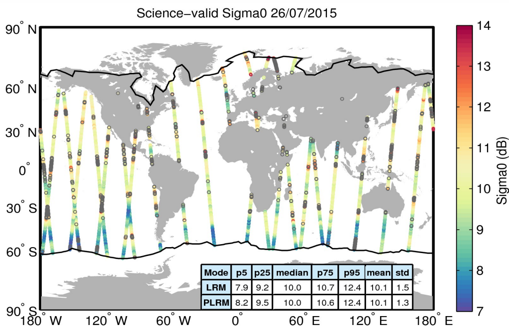
Figure 27. Geographical distribution of science-valid sigma0 data over oceans and lakes for 26/07/2015. The statistical values shown in the table refer to the sigma0 in dB and are calculated separately for LRM and PLRM regions. The black lines mark the outer limit of the Arctic and Antarctic polar polygons. Gray circles denote records that have been rejected based on the editing criteria described in Table 4.
