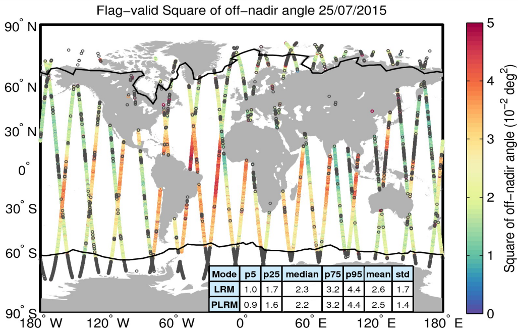
Figure 37. Geographical distribution of flag-valid mispointing data over oceans and lakes for 25/07/2015. The statistical values shown in the table refer to the mispointing in 10^{-2} \text{ deg}^2 and are calculated separately for LRM and PLRM regions. Measurements taken over polar polygons have been excluded from the computation of the statistical values. The black lines mark the outer limit of the Arctic and Antarctic polar polygons. Gray circles denote negative values.
