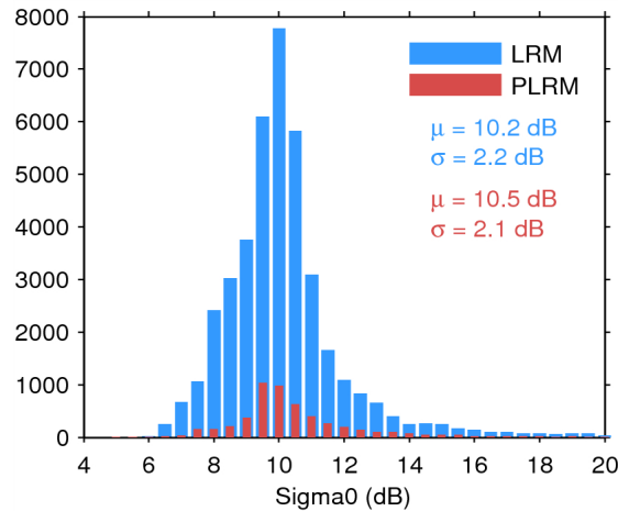
Figure 25. Histogram of flag-valid sigma0 over oceans and lakes for LRM (blue) and PLRM (red) for 25/07/2015. The mean ( \mu ) and standard deviation ( \sigma ) are also shown. Note that values outside [4 20] dB are excluded from the histogram for the sake of readability but not from the computation of \mu and \sigma .
