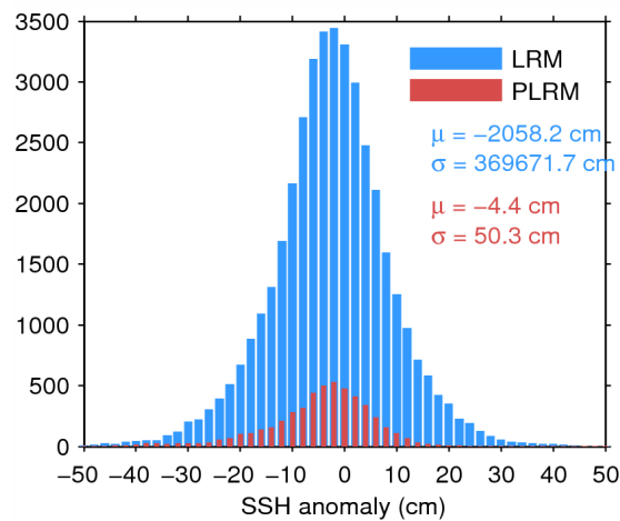
Figure 7. Histogram of flag-valid SSH anomaly over oceans and lakes for LRM (blue) and PLRM (red) for 25/07/2015. The mean ( \mu ) and standard deviation ( \sigma ) are also shown. Note that values outside [-50 \ 50] cm are excluded from the histogram for the sake of readability but not from the computation of \mu and \sigma .
