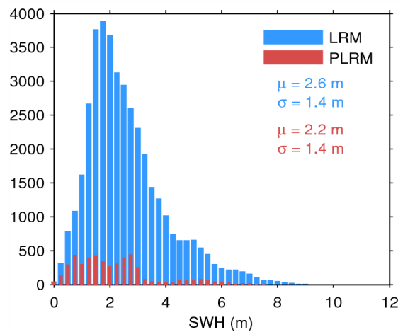
Figure 20. Histogram of science-valid SWH over oceans and lakes for LRM (blue) and PLRM (red) for 25/07/2015. The mean ( \mu ) and standard deviation ( \sigma ) are also shown. Note that values larger than 12 m are excluded from the histogram for the sake of readability but not from the computation of \mu and \sigma .
