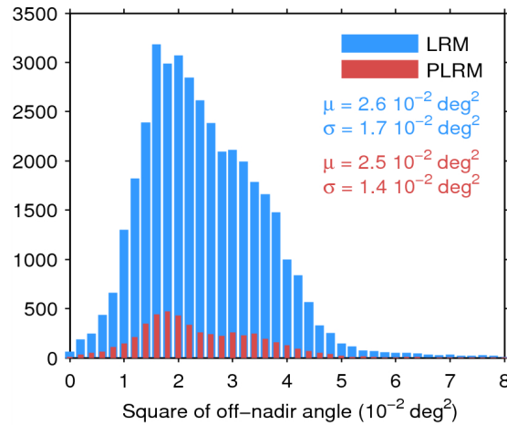
Figure 39. Histogram of flag-valid mispointing over oceans and lakes for LRM (blue) and PLRM (red) for 25/07/2015. Only positive values have been considered. The mean ( \mu ) and standard deviation ( \sigma ) are also shown. Note that values larger than 8 \cdot 10^{-2} \text{ deg}^2 are excluded from the histogram for the sake of readability but not from the computation of \mu and \sigma .
