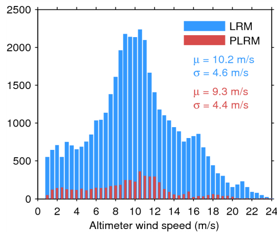
Figure 33. Histogram of flag-valid wind over oceans and lakes for LRM (blue) and PLRM (red) for 25/07/2015. The mean ( \mu ) and standard deviation ( \sigma ) are also shown. Note that values larger than 24 m/s are excluded from the histogram for the sake of readability but not from the computation of \mu and \sigma .
