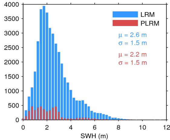
Figure 17. Histogram of flag-valid SWH over oceans and lakes for LRM (blue) and PLRM (red) for 25/07/2015. The mean ( \mu ) and standard deviation ( \sigma ) are also shown. Note that values larger than 12 m are excluded from the histogram for the sake of readability but not from the computation of \mu and \sigma .
