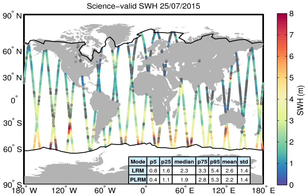
Figure 19. Geographical distribution of science-valid SWH data over oceans and lakes for 25/07/2015. The statistical values shown in the table refer to the SWH in m and are calculated separately for LRM and PLRM regions. The black lines mark the outer limit of the Arctic and Antarctic polar polygons. Gray circles denote records that have been rejected based on the editing criteria described in Table 3.
