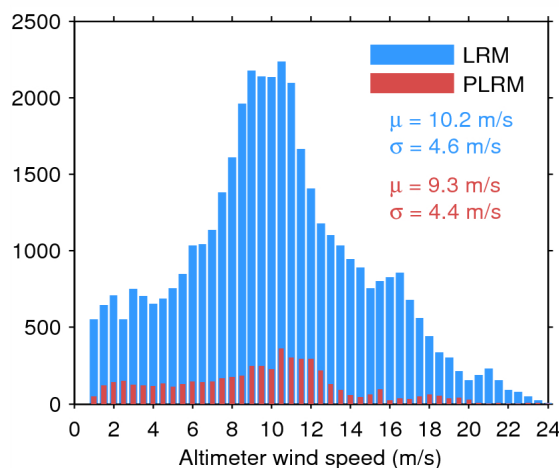
Figure 35. Histogram of science-valid wind over oceans and lakes for LRM (blue) and PLRM (red) for 25/07/2015. The mean ( \mu ) and standard deviation ( \sigma ) are also shown. Note that values larger than 24 m/s are excluded from the histogram for the sake of readability but not from the computation of \mu and \sigma .
