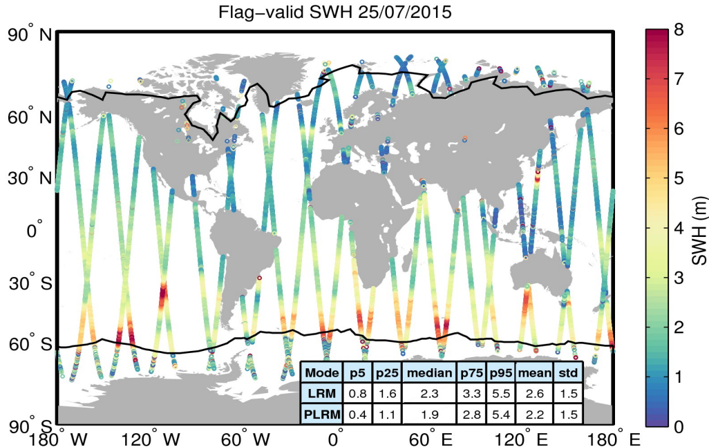
Figure 15. Geographical distribution of flag-valid SWH data over oceans and lakes for 25/07/2015. The statistical values shown in the table refer to the SWH in m and are calculated separately for LRM and PLRM regions. Measurements taken over polar polygons have been excluded from the computation of the statistical values. The black lines mark the outer limit of the Arctic and Antarctic polar polygons.
