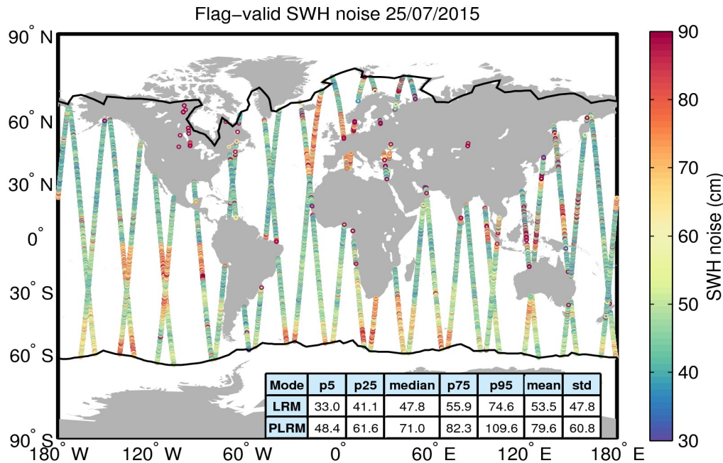
Figure 18. Geographical distribution of flag-valid 20-Hz SWH measurement noise over oceans and lakes for 25/07/2015. The statistical values shown in the table refer to the SWH noise and are calculated separately for LRM and PLRM regions. Measurements taken over polar polygons have been excluded from the computation of the statistical values. The black lines mark the outer limit of the Arctic and Antarctic polar polygons.
