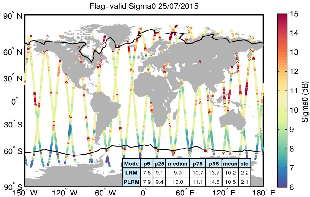
Figure 23. Geographical distribution of flag-valid sigma0 data over oceans and lakes for 25/07/2015. The statistical values shown in the table refer to the sigma0 in dB and are calculated separately for LRM and PLRM regions. Measurements taken over polar polygons have been excluded from the computation of the statistical values. The black lines mark the outer limit of the Arctic and Antarctic polar polygons.
