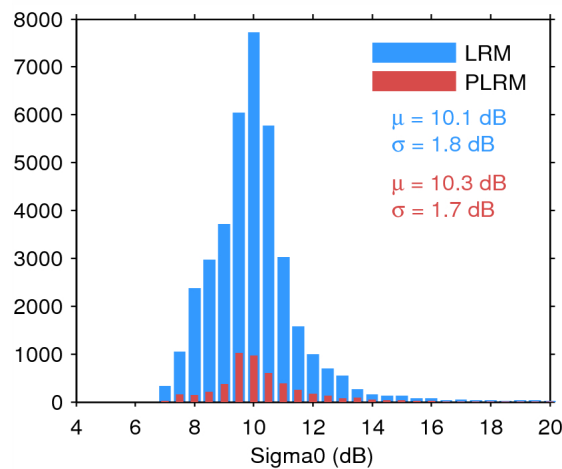
Figure 28. Histogram of science-valid sigma0 over oceans and lakes for LRM (blue) and PLRM (red) for 25/07/2015. The mean ( \mu ) and standard deviation ( \sigma ) are also shown. Note that values outside [4 20] dB are excluded from the histogram for the sake of readability but not from the computation of \mu and \sigma .
