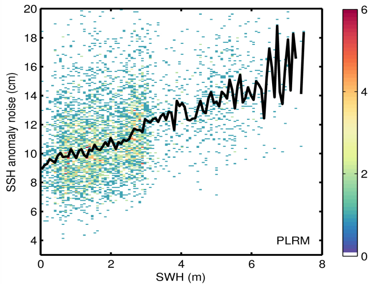
Figure 9. 2D histogram showing flag-valid SSH anomaly noise as a function of SWH for LRM (top) and PLRM (bottom) for 25/07/2015. The black line denotes the median SSH anomaly as a function of SWH.
