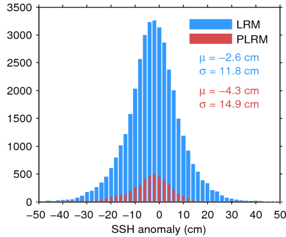
Figure 11. Histogram of science-valid SSH anomaly over oceans and lakes for LRM (blue) and PLRM (red) for 25/07/2015. The mean ( \mu ) and standard deviation ( \sigma ) are also shown. Note that values outside [-50\ 50] cm are excluded from the histogram for the sake of readability but not from the computation of \mu and \sigma .
