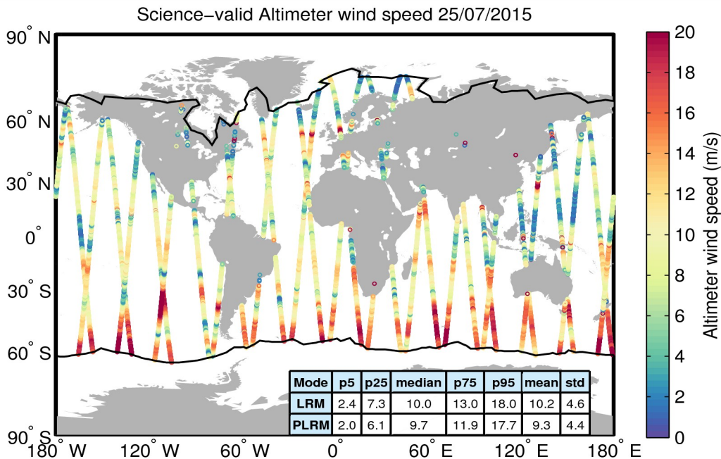
Figure 34. Geographical distribution of science-valid wind data over oceans and lakes for 25/07/2015. The statistical values shown in the table refer to the wind in m/s and are calculated separately for LRM and PLRM regions. The black lines mark the outer limit of the Arctic and Antarctic polar polygons. Gray circles denote records that have been rejected based on the editing criteria described in Table 5.
