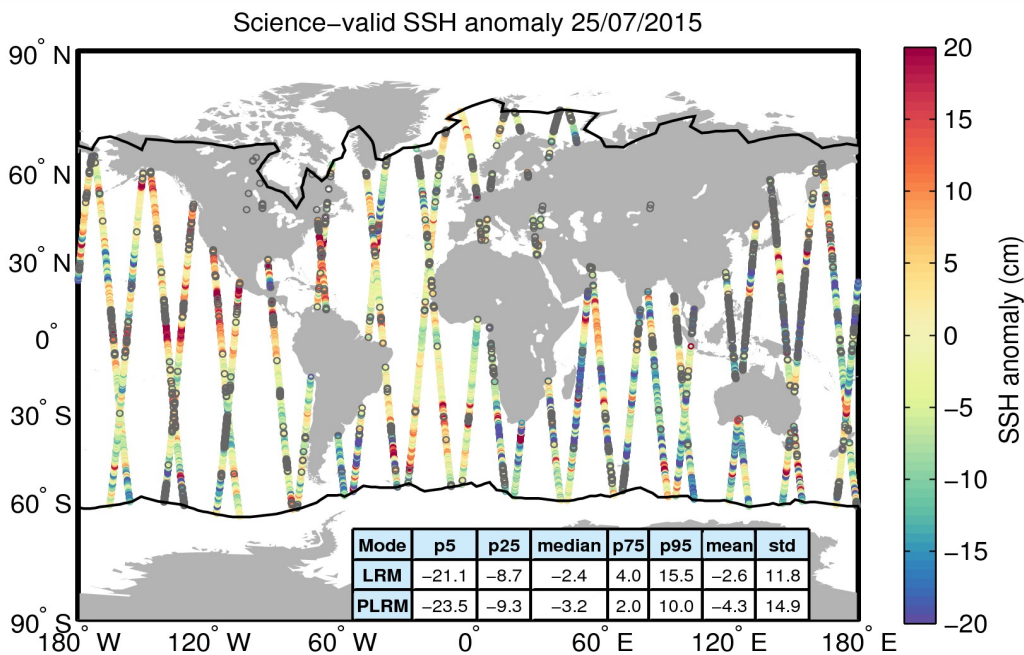
Figure 10. Geographical distribution of science-valid SSH anomaly data over oceans and lakes for 25/07/2015. The statistical values shown in the table refer to the SSH anomaly in cm and are calculated separately for LRM and PLRM regions. The black lines mark the outer limit of the Arctic and Antarctic polar polygons. Gray circles denote records that have been rejected based on the editing criteria described in Table 2.
