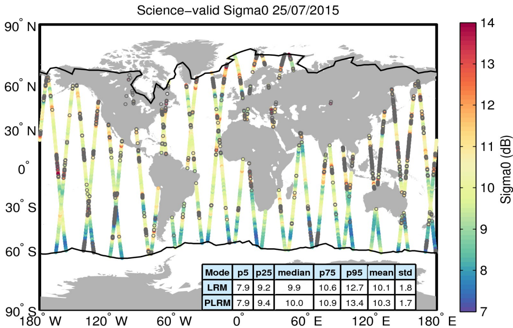
Figure 27. Geographical distribution of science-valid sigma0 data over oceans and lakes for 25/07/2015. The statistical values shown in the table refer to the sigma0 in dB and are calculated separately for LRM and PLRM regions. The black lines mark the outer limit of the Arctic and Antarctic polar polygons. Gray circles denote records that have been rejected based on the editing criteria described in Table 4.
