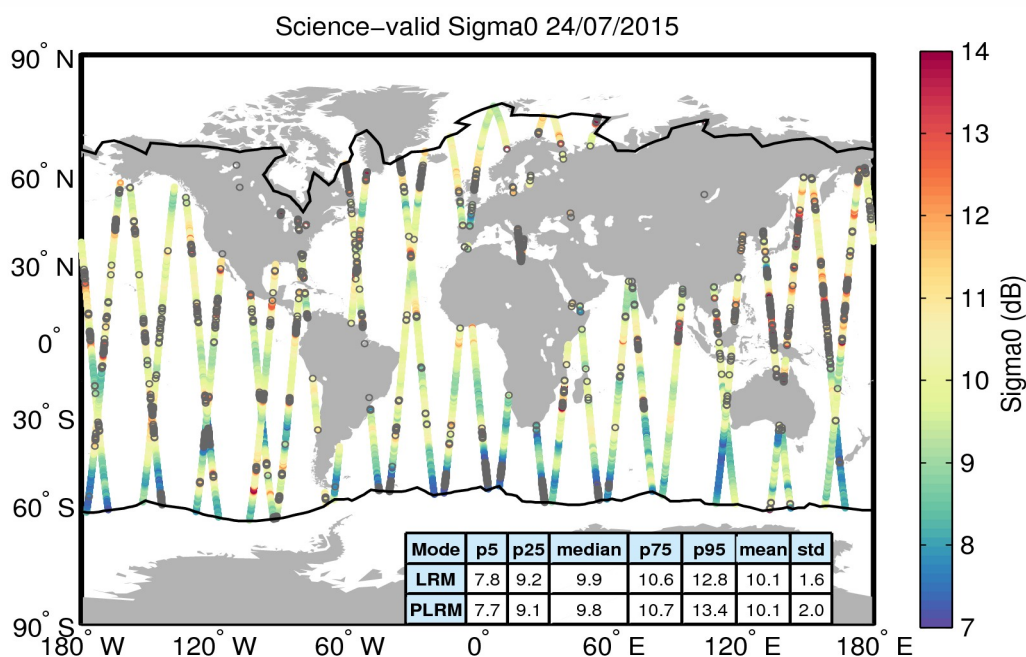
Figure 27. Geographical distribution of science-valid sigma0 data over oceans and lakes for 24/07/2015. The statistical values shown in the table refer to the sigma0 in dB and are calculated separately for LRM and PLRM regions. The black lines mark the outer limit of the Arctic and Antarctic polar polygons. Gray circles denote records that have been rejected based on the editing criteria described in Table 4.
