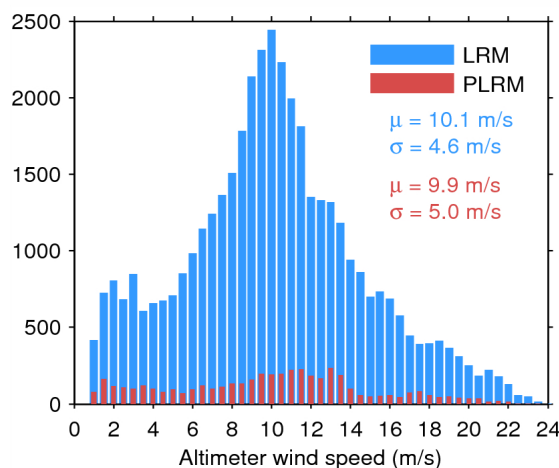
Figure 35. Histogram of science-valid wind over oceans and lakes for LRM (blue) and PLRM (red) for 24/07/2015. The mean ( \mu ) and standard deviation ( \sigma ) are also shown. Note that values larger than 24 m/s are excluded from the histogram for the sake of readability but not from the computation of \mu and \sigma .
