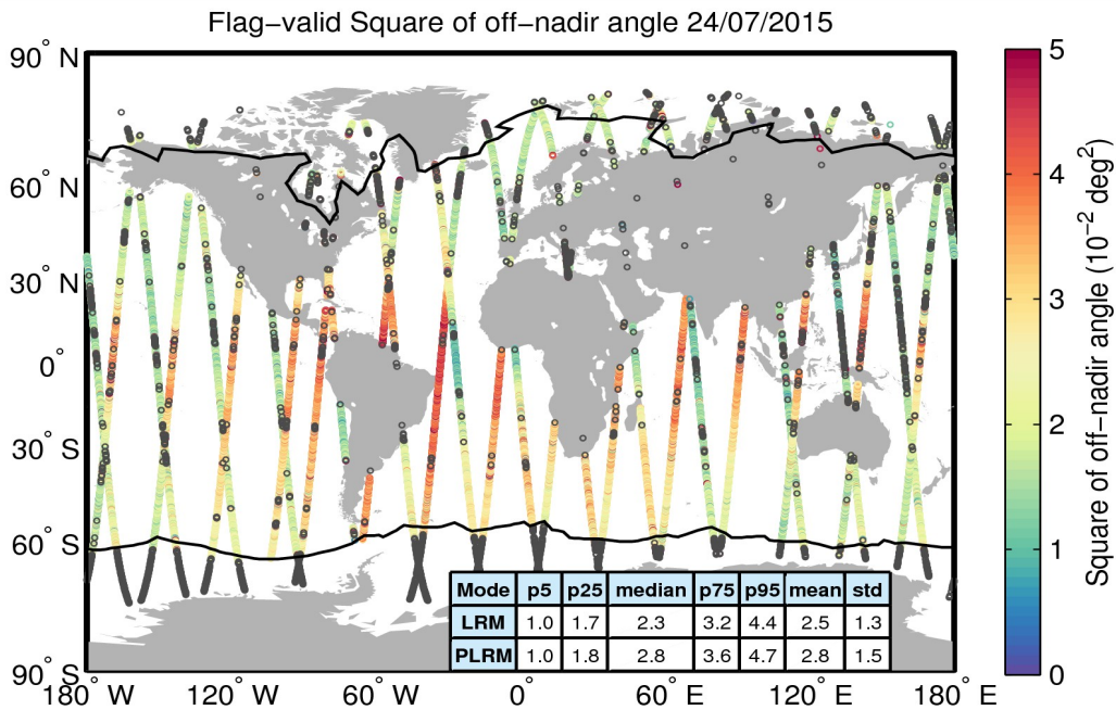
Figure 37. Geographical distribution of flag-valid mispointing data over oceans and lakes for 24/07/2015. The statistical values shown in the table refer to the mispointing in 10^{-2} deg 2 and are calculated separately for LRM and PLRM regions. Measurements taken over polar polygons have been excluded from the computation of the statistical values. The black lines mark the outer limit of the Arctic and Antarctic polar polygons. Gray circles denote negative values.
