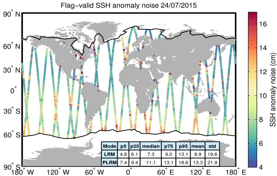
Figure 8. Geographical distribution of flag-valid 20-Hz SSH anomaly measurement noise over oceans and lakes for 24/07/2015. The statistical values shown in the table refer to the SSH anomaly noise and are calculated separately for LRM and PLRM regions. Measurements taken over polar polygons have been excluded from the computation of the statistical values. The black lines mark the outer limit of the Arctic and Antarctic polar polygons.
