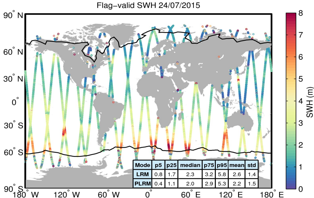
Figure 15. Geographical distribution of flag-valid SWH data over oceans and lakes for 24/07/2015. The statistical values shown in the table refer to the SWH in m and are calculated separately for LRM and PLRM regions. Measurements taken over polar polygons have been excluded from the computation of the statistical values. The black lines mark the outer limit of the Arctic and Antarctic polar polygons.
