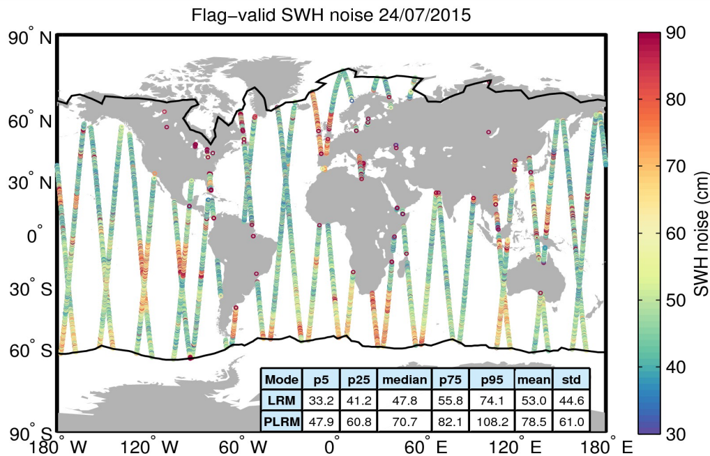
Figure 18. Geographical distribution of flag-valid 20-Hz SWH measurement noise over oceans and lakes for 24/07/2015. The statistical values shown in the table refer to the SWH noise and are calculated separately for LRM and PLRM regions. Measurements taken over polar polygons have been excluded from the computation of the statistical values. The black lines mark the outer limit of the Arctic and Antarctic polar polygons.
