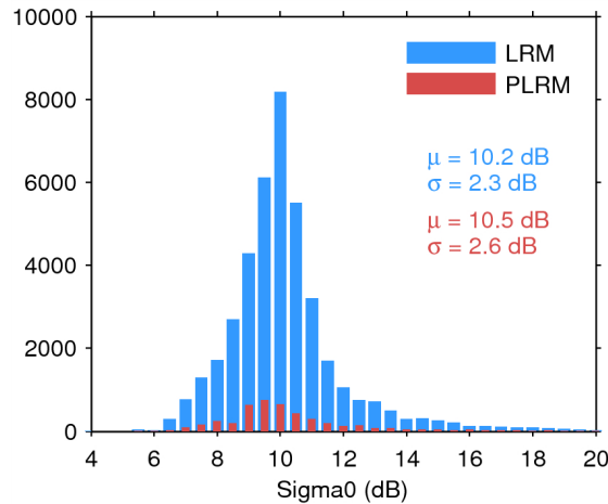
Figure 25. Histogram of flag-valid sigma0 over oceans and lakes for LRM (blue) and PLRM (red) for 24/07/2015. The mean ( \mu ) and standard deviation ( \sigma ) are also shown. Note that values outside [4 20] dB are excluded from the histogram for the sake of readability but not from the computation of \mu and \sigma .
