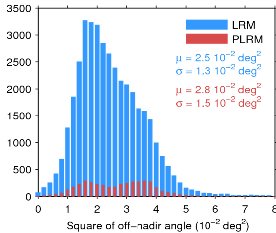
Figure 39. Histogram of flag-valid mispointing over oceans and lakes for LRM (blue) and PLRM (red) for 24/07/2015. Only positive values have been considered. The mean ( \mu ) and standard deviation ( \sigma ) are also shown. Note that values larger than 8 \cdot 10^{-2} \text{ deg}^2 are excluded from the histogram for the sake of readability but not from the computation of \mu and \sigma .
