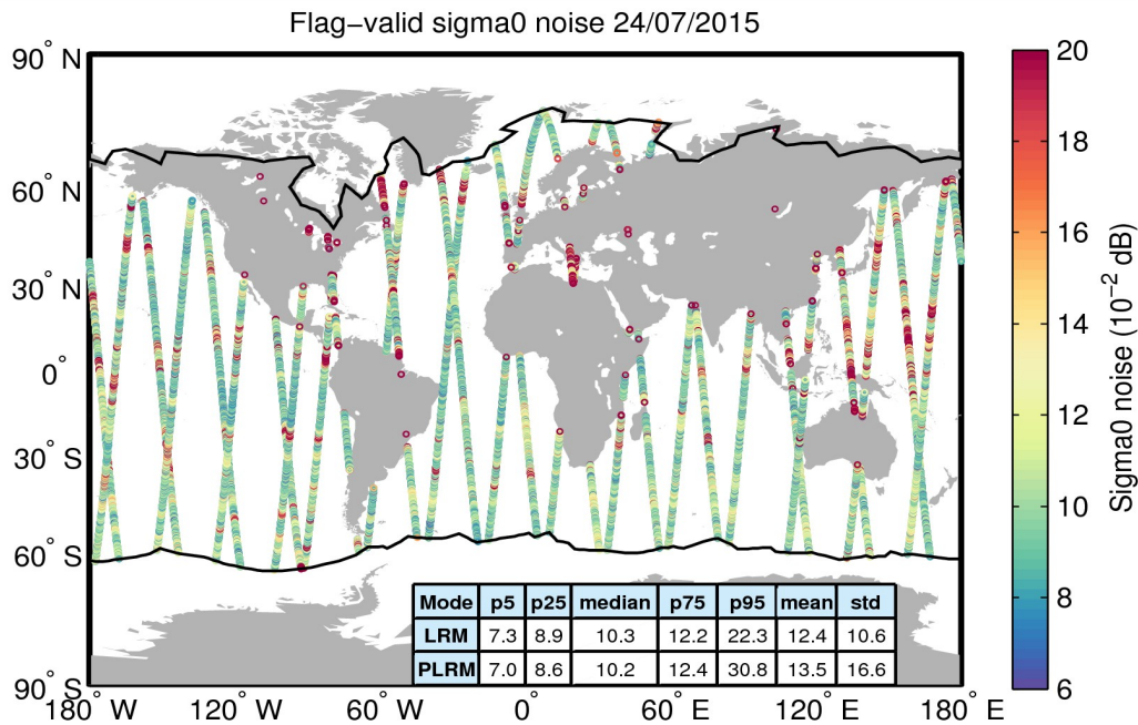
Figure 26. Geographical distribution of flag-valid 20-Hz sigma0 measurement noise over oceans and lakes for 24/07/2015. The statistical values shown in the table refer to the sigma0 noise and are calculated separately for LRM and PLRM regions. Measurements taken over polar polygons have been excluded from the computation of the statistical values. The black lines mark the outer limit of the Arctic and Antarctic polar polygons.
