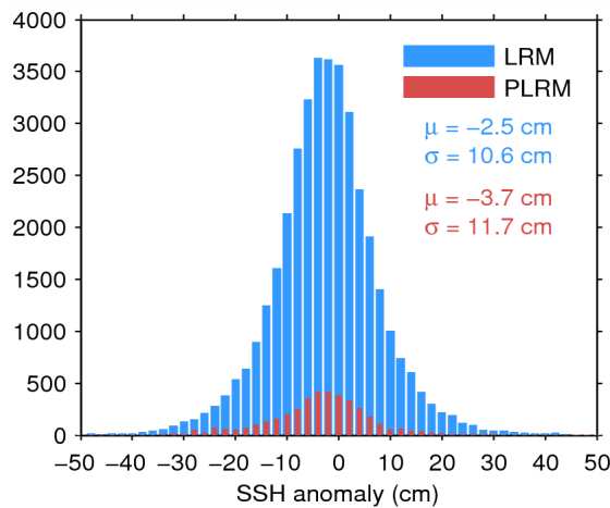
Figure 11. Histogram of science-valid SSH anomaly over oceans and lakes for LRM (blue) and PLRM (red) for 24/07/2015. The mean ( \mu ) and standard deviation ( \sigma ) are also shown. Note that values outside [-50 50] cm are excluded from the histogram for the sake of readability but not from the computation of \mu and \sigma .
