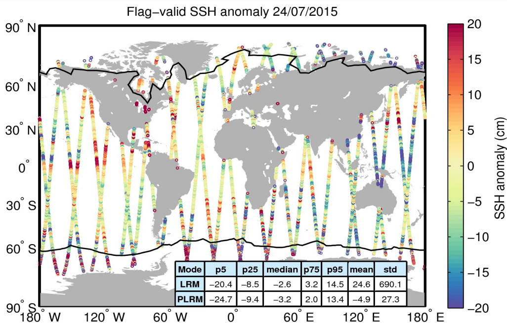
Figure 5. Geographical distribution of flag-valid 1-Hz SSH anomaly data over oceans and lakes for 24/07/2015. The statistical values shown in the table refer to the SSH anomaly in cm and are calculated separately for LRM and PLRM regions. Measurements taken over polar polygons have been excluded from the computation of the statistical values. The black lines mark the outer limit of the Arctic and Antarctic polar polygons.
