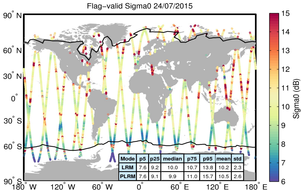
Figure 23. Geographical distribution of flag-valid sigma0 data over oceans and lakes for 24/07/2015. The statistical values shown in the table refer to the sigma0 in dB and are calculated separately for LRM and PLRM regions. Measurements taken over polar polygons have been excluded from the computation of the statistical values. The black lines mark the outer limit of the Arctic and Antarctic polar polygons.
