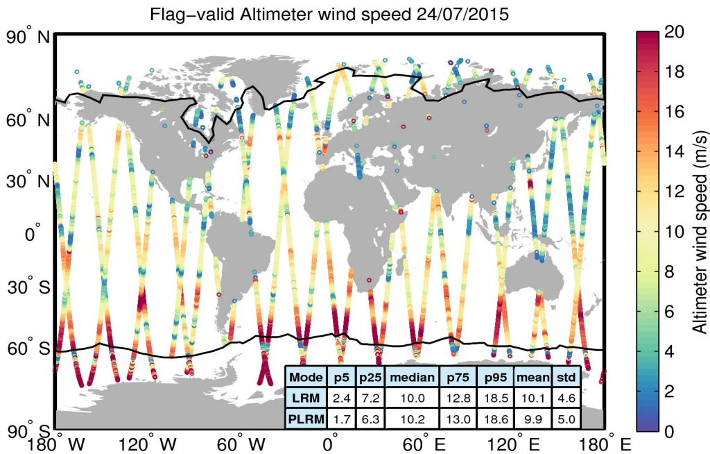
Figure 31. Geographical distribution of flag-valid wind data over oceans and lakes for 24/07/2015. The statistical values shown in the table refer to the wind in m/s and are calculated separately for LRM and PLRM regions. Measurements taken over polar polygons have been excluded from the computation of the statistical values. The black lines mark the outer limit of the Arctic and Antarctic polar polygons.
