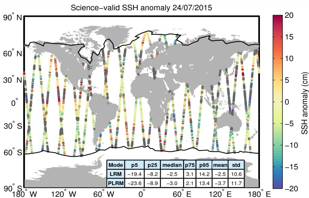
Figure 10. Geographical distribution of science-valid SSH anomaly data over oceans and lakes for 24/07/2015. The statistical values shown in the table refer to the SSH anomaly in cm and are calculated separately for LRM and PLRM regions. The black lines mark the outer limit of the Arctic and Antarctic polar polygons. Gray circles denote records that have been rejected based on the editing criteria described in Table 2.
