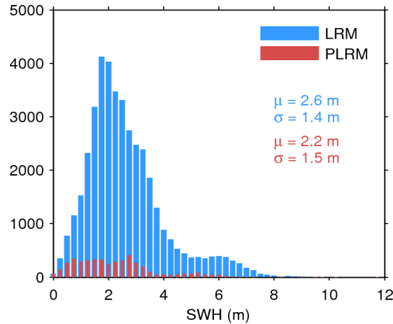
Figure 17. Histogram of flag-valid SWH over oceans and lakes for LRM (blue) and PLRM (red) for 24/07/2015. The mean ( \mu ) and standard deviation ( \sigma ) are also shown. Note that values larger than 12 m are excluded from the histogram for the sake of readability but not from the computation of \mu and \sigma .
