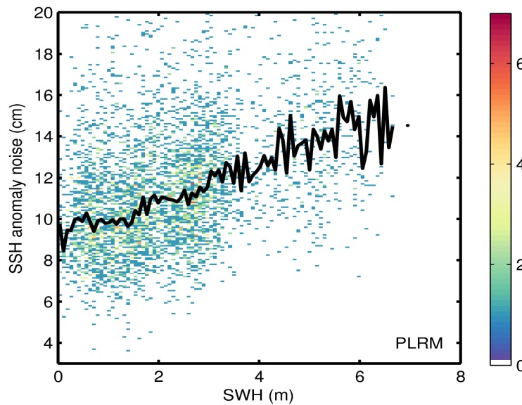
Figure 9. 2D histogram showing flag-valid SSH anomaly noise as a function of SWH for LRM (top) and PLRM (bottom) for 24/07/2015. The black line denotes the median SSH anomaly as a function of SWH.
