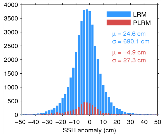
Figure 7. Histogram of flag-valid SSH anomaly over oceans and lakes for LRM (blue) and PLRM (red) for 24/07/2015. The mean ( \mu ) and standard deviation ( \sigma ) are also shown. Note that values outside [-50\ 50] cm are excluded from the histogram for the sake of readability but not from the computation of \mu and \sigma .
