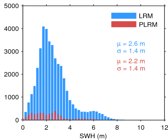
Figure 20. Histogram of science-valid SWH over oceans and lakes for LRM (blue) and PLRM (red) for 24/07/2015. The mean ( \mu ) and standard deviation ( \sigma ) are also shown. Note that values larger than 12 m are excluded from the histogram for the sake of readability but not from the computation of \mu and \sigma .
