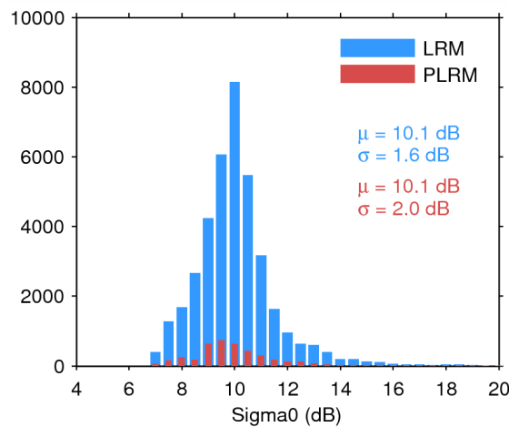
Figure 28. Histogram of science-valid sigma0 over oceans and lakes for LRM (blue) and PLRM (red) for 24/07/2015. The mean ( \mu ) and standard deviation ( \sigma ) are also shown. Note that values outside [4 20] dB are excluded from the histogram for the sake of readability but not from the computation of \mu and \sigma .
