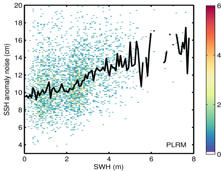
Figure 9. 2D histogram showing flag-valid SSH anomaly noise as a function of SWH for LRM (top) and PLRM (bottom) for 20/07/2015. The black line denotes the median SSH anomaly as a function of SWH.
