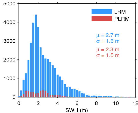
Figure 17. Histogram of flag-valid SWH over oceans and lakes for LRM (blue) and PLRM (red) for 20/07/2015. The mean ( \mu ) and standard deviation ( \sigma ) are also shown. Note that values larger than 12 m are excluded from the histogram for the sake of readability but not from the computation of \mu and \sigma .
