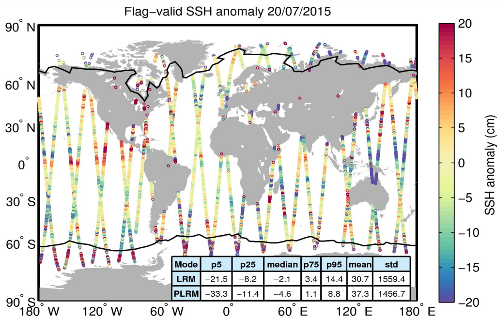
Figure 5. Geographical distribution of flag-valid 1-Hz SSH anomaly data over oceans and lakes for 20/07/2015. The statistical values shown in the table refer to the SSH anomaly in cm and are calculated separately for LRM and PLRM regions. Measurements taken over polar polygons have been excluded from the computation of the statistical values. The black lines mark the outer limit of the Arctic and Antarctic polar polygons.
