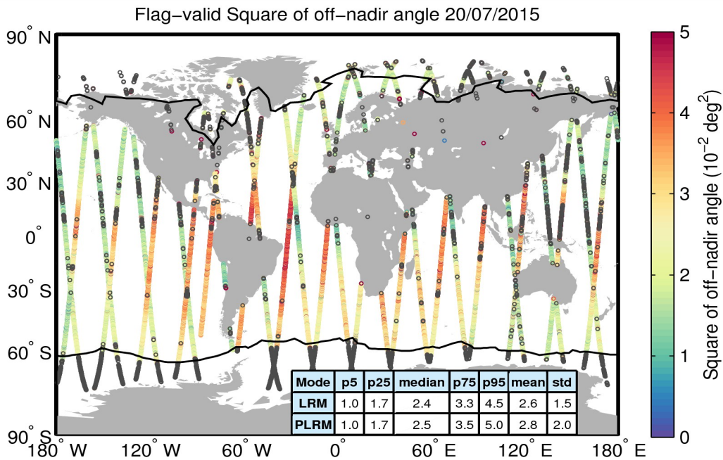
Figure 37. Geographical distribution of flag-valid mispointing data over oceans and lakes for 20/07/2015. The statistical values shown in the table refer to the mispointing in 10^{-2} deg 2 and are calculated separately for LRM and PLRM regions. Measurements taken over polar polygons have been excluded from the computation of the statistical values. The black lines mark the outer limit of the Arctic and Antarctic polar polygons. Gray circles denote negative values.
