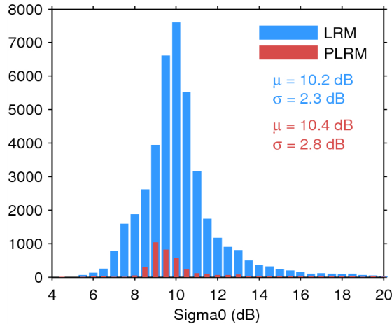
Figure 25. Histogram of flag-valid sigma0 over oceans and lakes for LRM (blue) and PLRM (red) for 20/07/2015. The mean ( \mu ) and standard deviation ( \sigma ) are also shown. Note that values outside [4 20] dB are excluded from the histogram for the sake of readability but not from the computation of \mu and \sigma .
