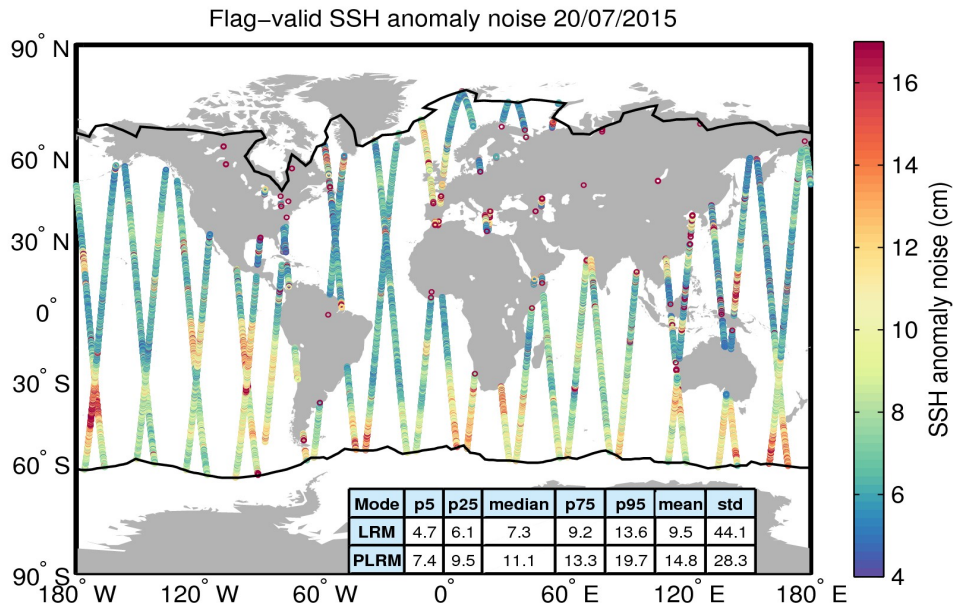
Figure 8. Geographical distribution of flag-valid 20-Hz SSH anomaly measurement noise over oceans and lakes for 20/07/2015. The statistical values shown in the table refer to the SSH anomaly noise and are calculated separately for LRM and PLRM regions. Measurements taken over polar polygons have been excluded from the computation of the statistical values. The black lines mark the outer limit of the Arctic and Antarctic polar polygons.
