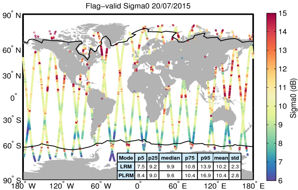
Figure 23. Geographical distribution of flag-valid sigma0 data over oceans and lakes for 20/07/2015. The statistical values shown in the table refer to the sigma0 in dB and are calculated separately for LRM and PLRM regions. Measurements taken over polar polygons have been excluded from the computation of the statistical values. The black lines mark the outer limit of the Arctic and Antarctic polar polygons.
