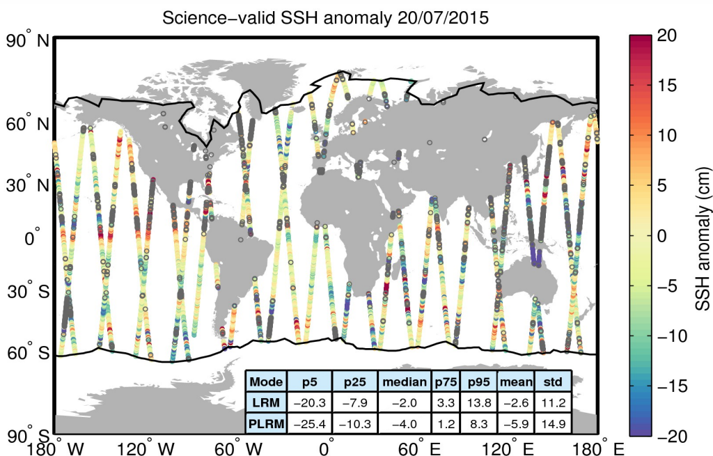
Figure 10. Geographical distribution of science-valid SSH anomaly data over oceans and lakes for 20/07/2015. The statistical values shown in the table refer to the SSH anomaly in cm and are calculated separately for LRM and PLRM regions. The black lines mark the outer limit of the Arctic and Antarctic polar polygons. Gray circles denote records that have been rejected based on the editing criteria described in Table 2.
