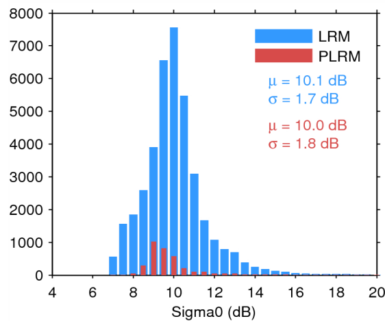
Figure 28. Histogram of science-valid sigma0 over oceans and lakes for LRM (blue) and PLRM (red) for 20/07/2015. The mean ( \mu ) and standard deviation ( \sigma ) are also shown. Note that values outside [4 20] dB are excluded from the histogram for the sake of readability but not from the computation of \mu and \sigma .
