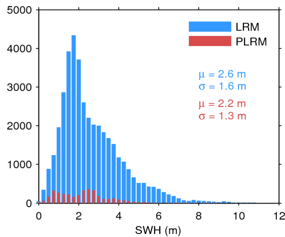
Figure 20. Histogram of science-valid SWH over oceans and lakes for LRM (blue) and PLRM (red) for 20/07/2015. The mean ( \mu ) and standard deviation ( \sigma ) are also shown. Note that values larger than 12 m are excluded from the histogram for the sake of readability but not from the computation of \mu and \sigma .
