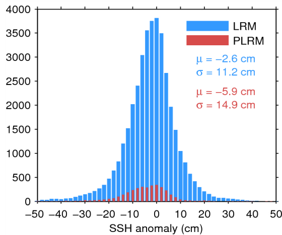
Figure 11. Histogram of science-valid SSH anomaly over oceans and lakes for LRM (blue) and PLRM (red) for 20/07/2015. The mean ( \mu ) and standard deviation ( \sigma ) are also shown. Note that values outside [-50 50] cm are excluded from the histogram for the sake of readability but not from the computation of \mu and \sigma .
