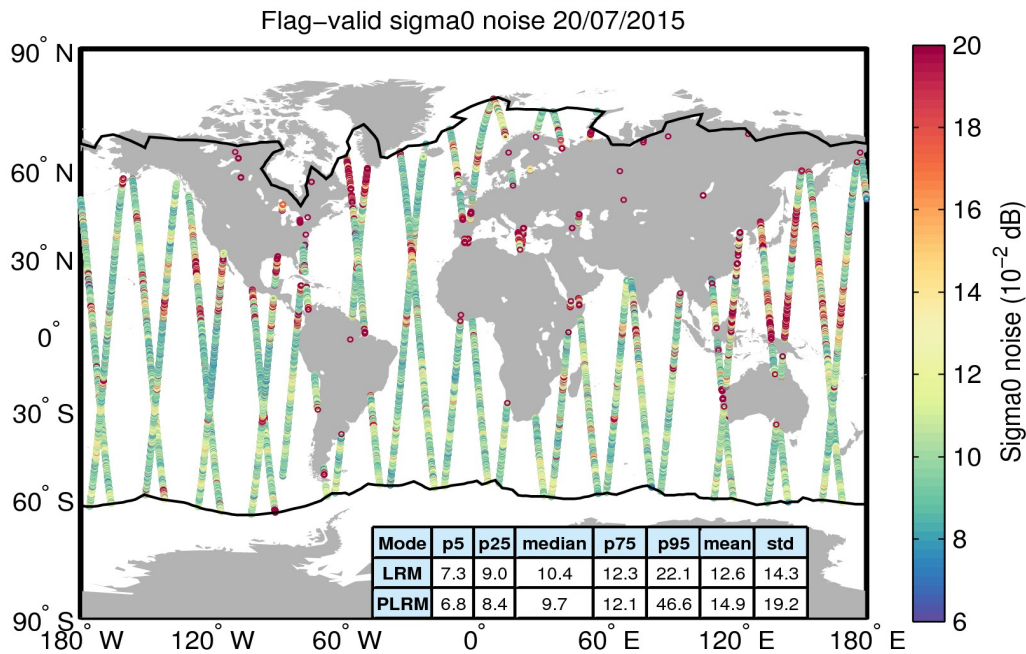
Figure 26. Geographical distribution of flag-valid 20-Hz sigma0 measurement noise over oceans and lakes for 20/07/2015. The statistical values shown in the table refer to the sigma0 noise and are calculated separately for LRM and PLRM regions. Measurements taken over polar polygons have been excluded from the computation of the statistical values. The black lines mark the outer limit of the Arctic and Antarctic polar polygons.
