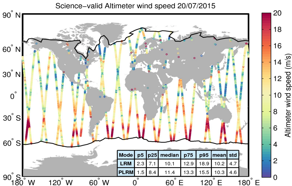
Figure 34. Geographical distribution of science-valid wind data over oceans and lakes for 20/07/2015. The statistical values shown in the table refer to the wind in m/s and are calculated separately for LRM and PLRM regions. The black lines mark the outer limit of the Arctic and Antarctic polar polygons. Gray circles denote records that have been rejected based on the editing criteria described in Table 5.
