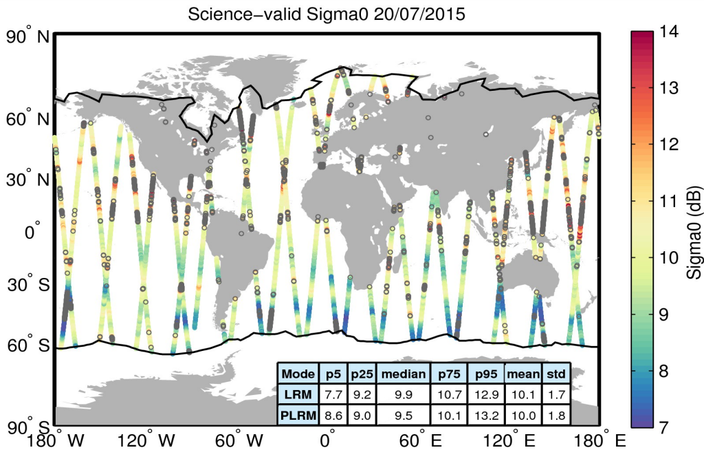
Figure 27. Geographical distribution of science-valid sigma0 data over oceans and lakes for 20/07/2015. The statistical values shown in the table refer to the sigma0 in dB and are calculated separately for LRM and PLRM regions. The black lines mark the outer limit of the Arctic and Antarctic polar polygons. Gray circles denote records that have been rejected based on the editing criteria described in Table 4.
