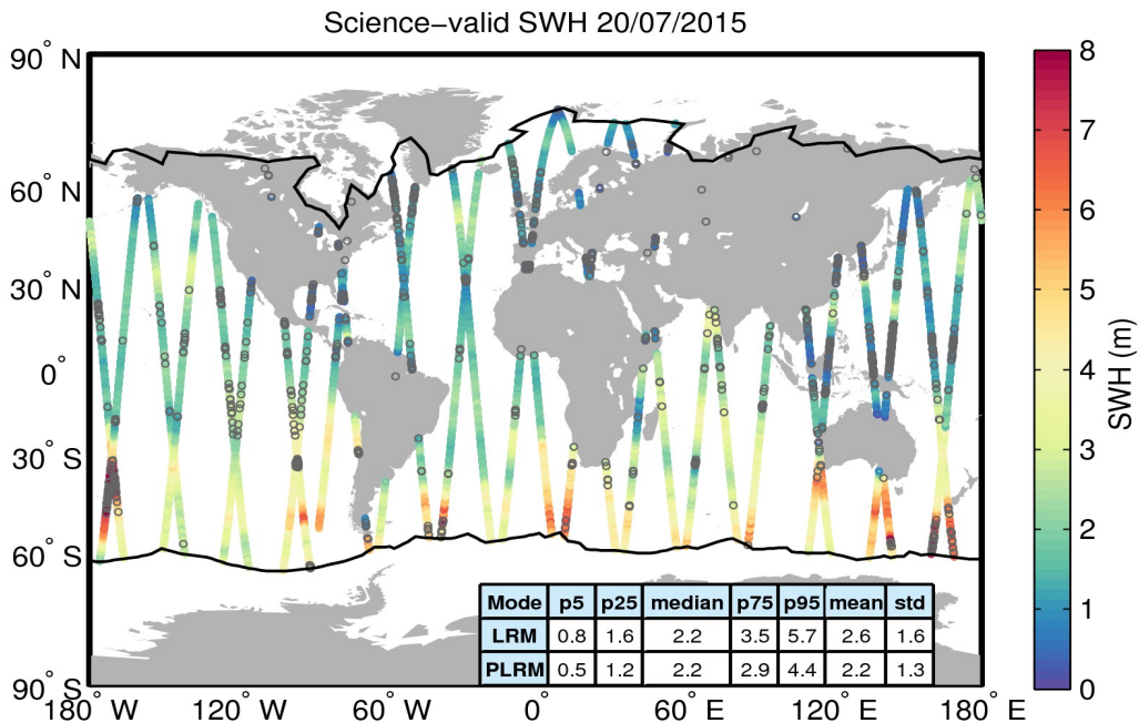
Figure 19. Geographical distribution of science-valid SWH data over oceans and lakes for 20/07/2015. The statistical values shown in the table refer to the SWH in m and are calculated separately for LRM and PLRM regions. The black lines mark the outer limit of the Arctic and Antarctic polar polygons. Gray circles denote records that have been rejected based on the editing criteria described in Table 3.
