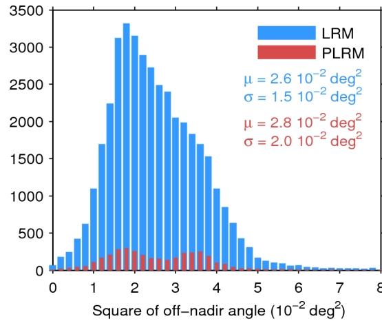
Figure 39. Histogram of flag-valid mispointing over oceans and lakes for LRM (blue) and PLRM (red) for 20/07/2015. Only positive values have been considered. The mean ( \mu ) and standard deviation ( \sigma ) are also shown. Note that values larger than 8 \cdot 10^{-2} \text{ deg}^2 are excluded from the histogram for the sake of readability but not from the computation of \mu and \sigma .
