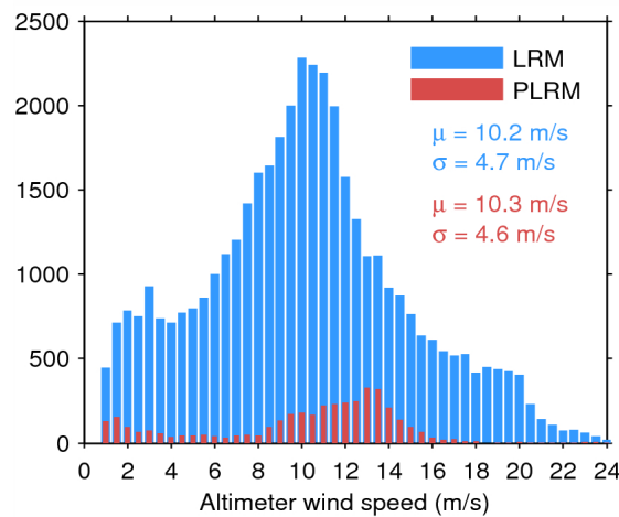
Figure 33. Histogram of flag-valid wind over oceans and lakes for LRM (blue) and PLRM (red) for 20/07/2015. The mean ( \mu ) and standard deviation ( \sigma ) are also shown. Note that values larger than 24 m/s are excluded from the histogram for the sake of readability but not from the computation of \mu and \sigma .
