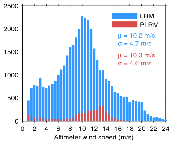
Figure 35. Histogram of science-valid wind over oceans and lakes for LRM (blue) and PLRM (red) for 20/07/2015. The mean ( \mu ) and standard deviation ( \sigma ) are also shown. Note that values larger than 24 m/s are excluded from the histogram for the sake of readability but not from the computation of \mu and \sigma .
