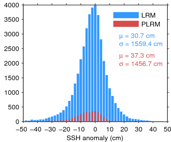
Figure 7. Histogram of flag-valid SSH anomaly over oceans and lakes for LRM (blue) and PLRM (red) for 20/07/2015. The mean ( \mu ) and standard deviation ( \sigma ) are also shown. Note that values outside [-50\ 50] cm are excluded from the histogram for the sake of readability but not from the computation of \mu and \sigma .
