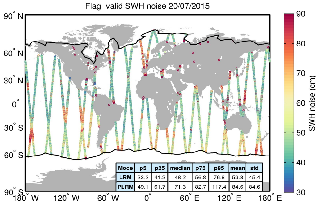
Figure 18. Geographical distribution of flag-valid 20-Hz SWH measurement noise over oceans and lakes for 20/07/2015. The statistical values shown in the table refer to the SWH noise and are calculated separately for LRM and PLRM regions. Measurements taken over polar polygons have been excluded from the computation of the statistical values. The black lines mark the outer limit of the Arctic and Antarctic polar polygons.
