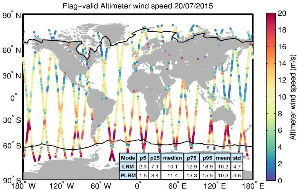
Figure 31. Geographical distribution of flag-valid wind data over oceans and lakes for 20/07/2015. The statistical values shown in the table refer to the wind in m/s and are calculated separately for LRM and PLRM regions. Measurements taken over polar polygons have been excluded from the computation of the statistical values. The black lines mark the outer limit of the Arctic and Antarctic polar polygons.
