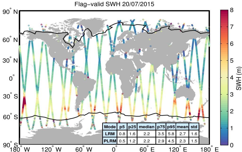
Figure 15. Geographical distribution of flag-valid SWH data over oceans and lakes for 20/07/2015. The statistical values shown in the table refer to the SWH in m and are calculated separately for LRM and PLRM regions. Measurements taken over polar polygons have been excluded from the computation of the statistical values. The black lines mark the outer limit of the Arctic and Antarctic polar polygons.
