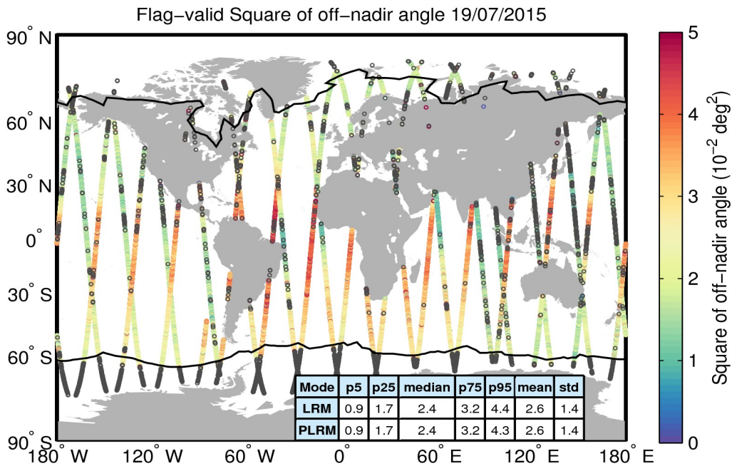
Figure 37. Geographical distribution of flag-valid mispointing data over oceans and lakes for 19/07/2015. The statistical values shown in the table refer to the mispointing in 10^{-2} deg 2 and are calculated separately for LRM and PLRM regions. Measurements taken over polar polygons have been excluded from the computation of the statistical values. The black lines mark the outer limit of the Arctic and Antarctic polar polygons. Gray circles denote negative values.
