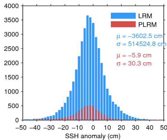
Figure 7. Histogram of flag-valid SSH anomaly over oceans and lakes for LRM (blue) and PLRM (red) for 19/07/2015. The mean ( \mu ) and standard deviation ( \sigma ) are also shown. Note that values outside [-50\ 50] cm are excluded from the histogram for the sake of readability but not from the computation of \mu and \sigma .
