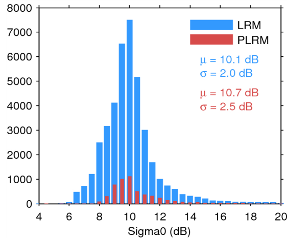
Figure 25. Histogram of flag-valid sigma0 over oceans and lakes for LRM (blue) and PLRM (red) for 19/07/2015. The mean ( \mu ) and standard deviation ( \sigma ) are also shown. Note that values outside [4 20] dB are excluded from the histogram for the sake of readability but not from the computation of \mu and \sigma .
