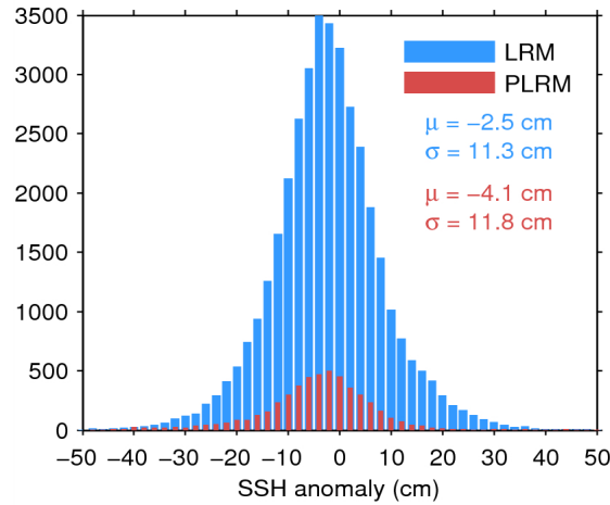
Figure 11. Histogram of science-valid SSH anomaly over oceans and lakes for LRM (blue) and PLRM (red) for 19/07/2015. The mean ( \mu ) and standard deviation ( \sigma ) are also shown. Note that values outside [-50\ 50] cm are excluded from the histogram for the sake of readability but not from the computation of \mu and \sigma .
