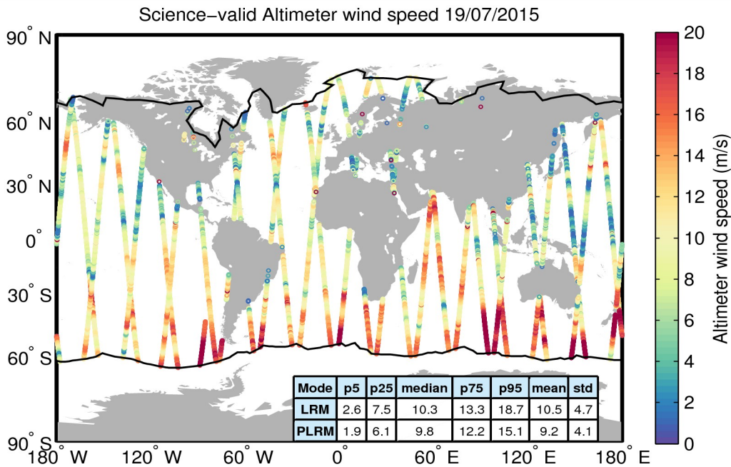
Figure 34. Geographical distribution of science-valid wind data over oceans and lakes for 19/07/2015. The statistical values shown in the table refer to the wind in m/s and are calculated separately for LRM and PLRM regions. The black lines mark the outer limit of the Arctic and Antarctic polar polygons. Gray circles denote records that have been rejected based on the editing criteria described in Table 5.
