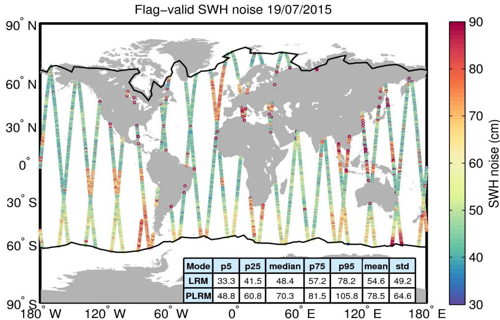
Figure 18. Geographical distribution of flag-valid 20-Hz SWH measurement noise over oceans and lakes for 19/07/2015. The statistical values shown in the table refer to the SWH noise and are calculated separately for LRM and PLRM regions. Measurements taken over polar polygons have been excluded from the computation of the statistical values. The black lines mark the outer limit of the Arctic and Antarctic polar polygons.
