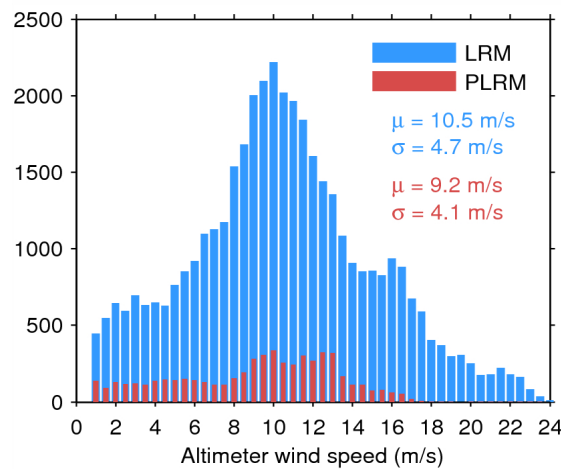
Figure 33. Histogram of flag-valid wind over oceans and lakes for LRM (blue) and PLRM (red) for 19/07/2015. The mean ( \mu ) and standard deviation ( \sigma ) are also shown. Note that values larger than 24 m/s are excluded from the histogram for the sake of readability but not from the computation of \mu and \sigma .
