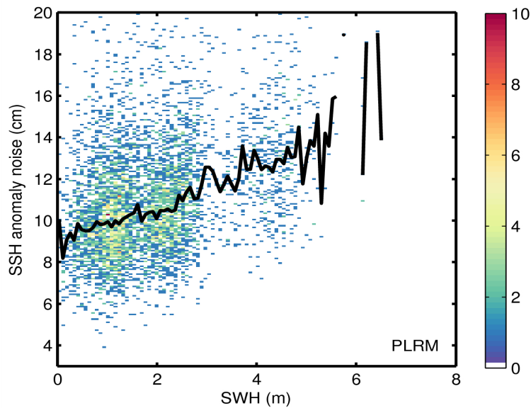
Figure 9. 2D histogram showing flag-valid SSH anomaly noise as a function of SWH for LRM (top) and PLRM (bottom) for 19/07/2015. The black line denotes the median SSH anomaly as a function of SWH.
