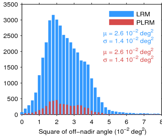
Figure 39. Histogram of flag-valid mispointing over oceans and lakes for LRM (blue) and PLRM (red) for 19/07/2015. Only positive values have been considered. The mean ( \mu ) and standard deviation ( \sigma ) are also shown. Note that values larger than 8 \cdot 10^{-2} \text{ deg}^2 are excluded from the histogram for the sake of readability but not from the computation of \mu and \sigma .
