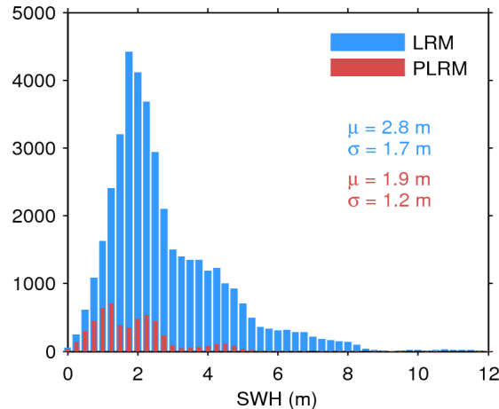
Figure 17. Histogram of flag-valid SWH over oceans and lakes for LRM (blue) and PLRM (red) for 19/07/2015. The mean ( \mu ) and standard deviation ( \sigma ) are also shown. Note that values larger than 12 m are excluded from the histogram for the sake of readability but not from the computation of \mu and \sigma .
