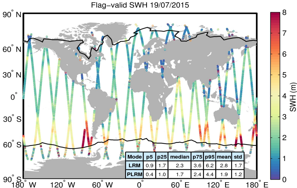
Figure 15. Geographical distribution of flag-valid SWH data over oceans and lakes for 19/07/2015. The statistical values shown in the table refer to the SWH in m and are calculated separately for LRM and PLRM regions. Measurements taken over polar polygons have been excluded from the computation of the statistical values. The black lines mark the outer limit of the Arctic and Antarctic polar polygons.
