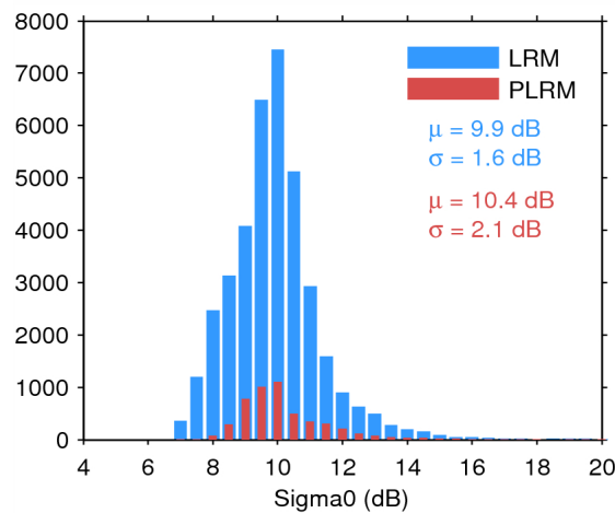
Figure 28. Histogram of science-valid sigma0 over oceans and lakes for LRM (blue) and PLRM (red) for 19/07/2015. The mean ( \mu ) and standard deviation ( \sigma ) are also shown. Note that values outside [4 20] dB are excluded from the histogram for the sake of readability but not from the computation of \mu and \sigma .
