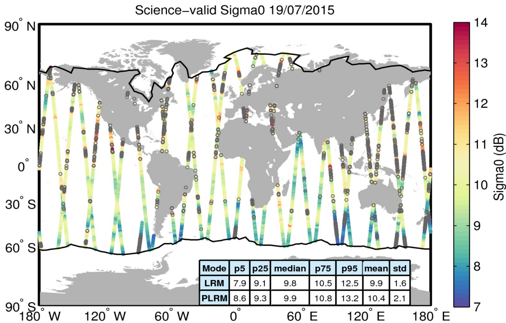
Figure 27. Geographical distribution of science-valid sigma0 data over oceans and lakes for 19/07/2015. The statistical values shown in the table refer to the sigma0 in dB and are calculated separately for LRM and PLRM regions. The black lines mark the outer limit of the Arctic and Antarctic polar polygons. Gray circles denote records that have been rejected based on the editing criteria described in Table 4.
