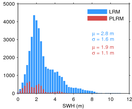
Figure 20. Histogram of science-valid SWH over oceans and lakes for LRM (blue) and PLRM (red) for 19/07/2015. The mean ( \mu ) and standard deviation ( \sigma ) are also shown. Note that values larger than 12 m are excluded from the histogram for the sake of readability but not from the computation of \mu and \sigma .
