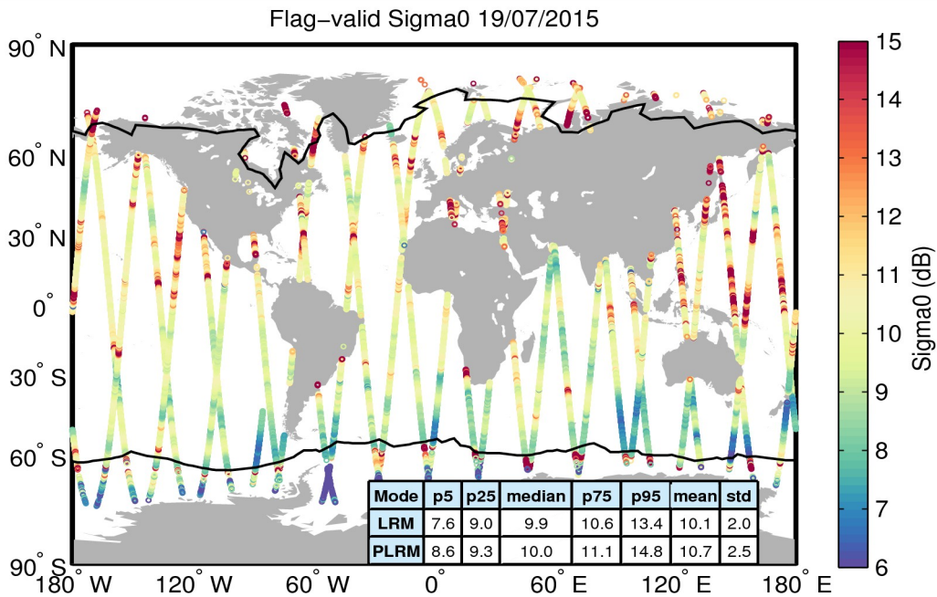
Figure 23. Geographical distribution of flag-valid sigma0 data over oceans and lakes for 19/07/2015. The statistical values shown in the table refer to the sigma0 in dB and are calculated separately for LRM and PLRM regions. Measurements taken over polar polygons have been excluded from the computation of the statistical values. The black lines mark the outer limit of the Arctic and Antarctic polar polygons.
