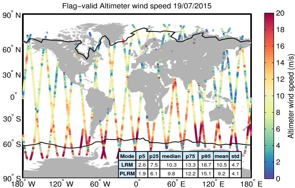
Figure 31. Geographical distribution of flag-valid wind data over oceans and lakes for 19/07/2015. The statistical values shown in the table refer to the wind in m/s and are calculated separately for LRM and PLRM regions. Measurements taken over polar polygons have been excluded from the computation of the statistical values. The black lines mark the outer limit of the Arctic and Antarctic polar polygons.
