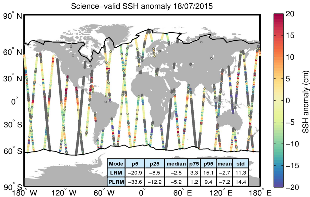
Figure 10. Geographical distribution of science-valid SSH anomaly data over oceans and lakes for 18/07/2015. The statistical values shown in the table refer to the SSH anomaly in cm and are calculated separately for LRM and PLRM regions. The black lines mark the outer limit of the Arctic and Antarctic polar polygons. Gray circles denote records that have been rejected based on the editing criteria described in Table 2.
