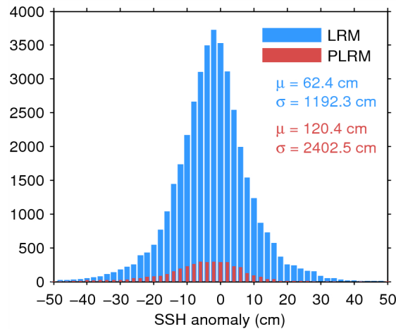
Figure 7. Histogram of flag-valid SSH anomaly over oceans and lakes for LRM (blue) and PLRM (red) for 18/07/2015. The mean ( \mu ) and standard deviation ( \sigma ) are also shown. Note that values outside [-50\ 50] cm are excluded from the histogram for the sake of readability but not from the computation of \mu and \sigma .
