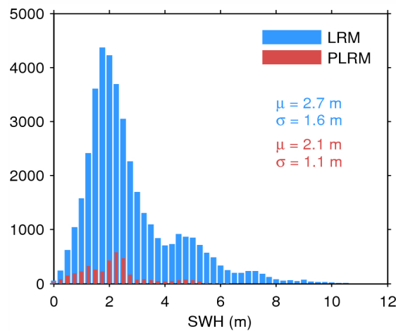
Figure 20. Histogram of science-valid SWH over oceans and lakes for LRM (blue) and PLRM (red) for 18/07/2015. The mean ( \mu ) and standard deviation ( \sigma ) are also shown. Note that values larger than 12 m are excluded from the histogram for the sake of readability but not from the computation of \mu and \sigma .
