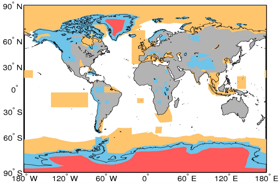
Figure A1. Extent of the regions defining the geographical mode mask for 18/07/2015. The regions where SAR, and SARIn are operated are denoted by the orange and blue polygons, respectively. LRM is operated over areas of the continental ice sheets (red polygons) and over oceans and land not covered by other modes.
