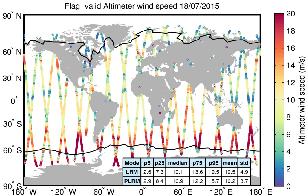
Figure 31. Geographical distribution of flag-valid wind data over oceans and lakes for 18/07/2015. The statistical values shown in the table refer to the wind in m/s and are calculated separately for LRM and PLRM regions. Measurements taken over polar polygons have been excluded from the computation of the statistical values. The black lines mark the outer limit of the Arctic and Antarctic polar polygons.
