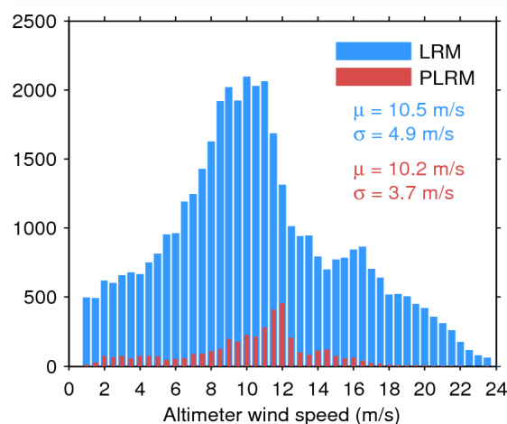
Figure 35. Histogram of science-valid wind over oceans and lakes for LRM (blue) and PLRM (red) for 18/07/2015. The mean ( \mu ) and standard deviation ( \sigma ) are also shown. Note that values larger than 24 m/s are excluded from the histogram for the sake of readability but not from the computation of \mu and \sigma .
