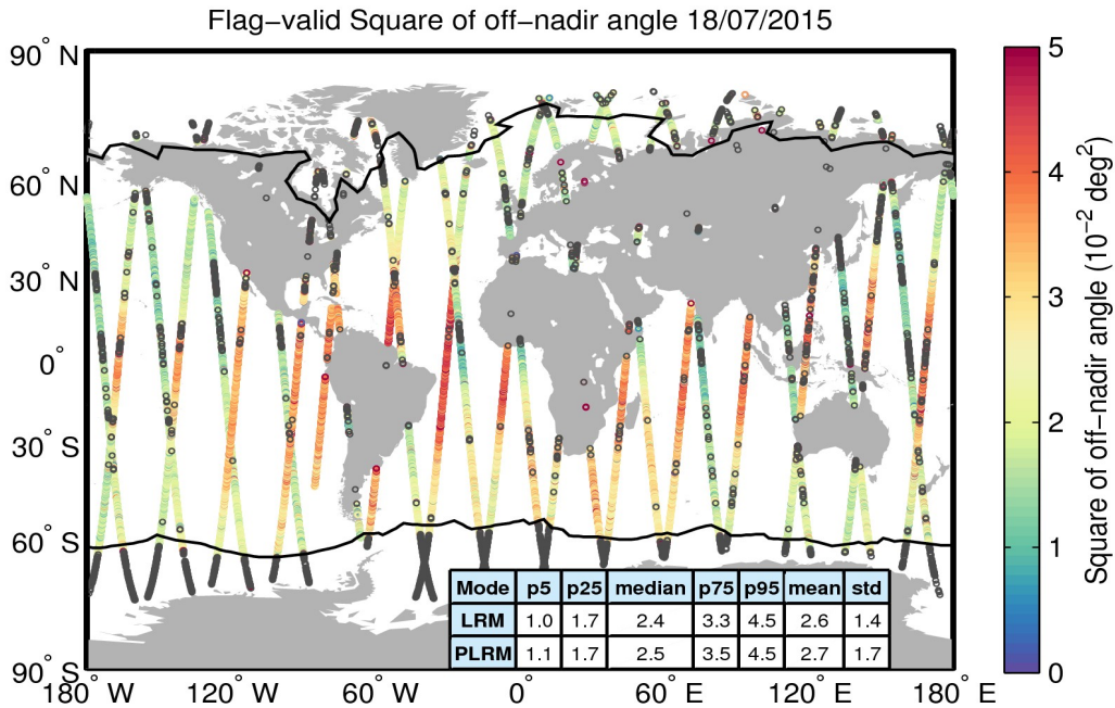
Figure 37. Geographical distribution of flag-valid mispointing data over oceans and lakes for 18/07/2015. The statistical values shown in the table refer to the mispointing in 10^{-2} deg 2 and are calculated separately for LRM and PLRM regions. Measurements taken over polar polygons have been excluded from the computation of the statistical values. The black lines mark the outer limit of the Arctic and Antarctic polar polygons. Gray circles denote negative values.
