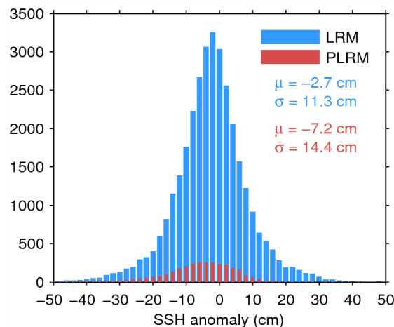
Figure 11. Histogram of science-valid SSH anomaly over oceans and lakes for LRM (blue) and PLRM (red) for 18/07/2015. The mean ( \mu ) and standard deviation ( \sigma ) are also shown. Note that values outside [-50 50] cm are excluded from the histogram for the sake of readability but not from the computation of \mu and \sigma .
