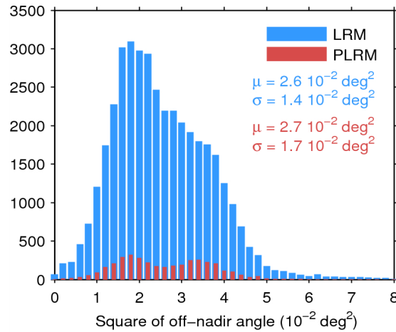
Figure 39. Histogram of flag-valid mispointing over oceans and lakes for LRM (blue) and PLRM (red) for 18/07/2015. Only positive values have been considered. The mean ( \mu ) and standard deviation ( \sigma ) are also shown. Note that values larger than 8 \cdot 10^{-2} \text{ deg}^2 are excluded from the histogram for the sake of readability but not from the computation of \mu and \sigma .
