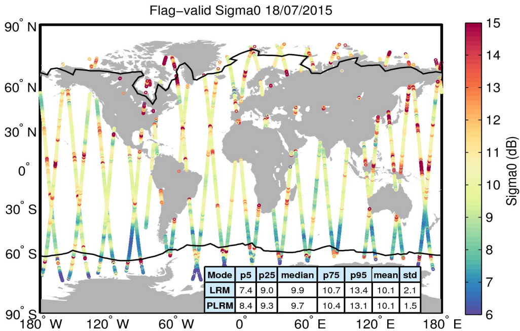
Figure 23. Geographical distribution of flag-valid sigma0 data over oceans and lakes for 18/07/2015. The statistical values shown in the table refer to the sigma0 in dB and are calculated separately for LRM and PLRM regions. Measurements taken over polar polygons have been excluded from the computation of the statistical values. The black lines mark the outer limit of the Arctic and Antarctic polar polygons.
