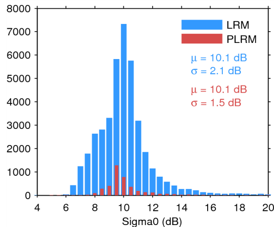
Figure 25. Histogram of flag-valid sigma0 over oceans and lakes for LRM (blue) and PLRM (red) for 18/07/2015. The mean ( \mu ) and standard deviation ( \sigma ) are also shown. Note that values outside [4 20] dB are excluded from the histogram for the sake of readability but not from the computation of \mu and \sigma .
