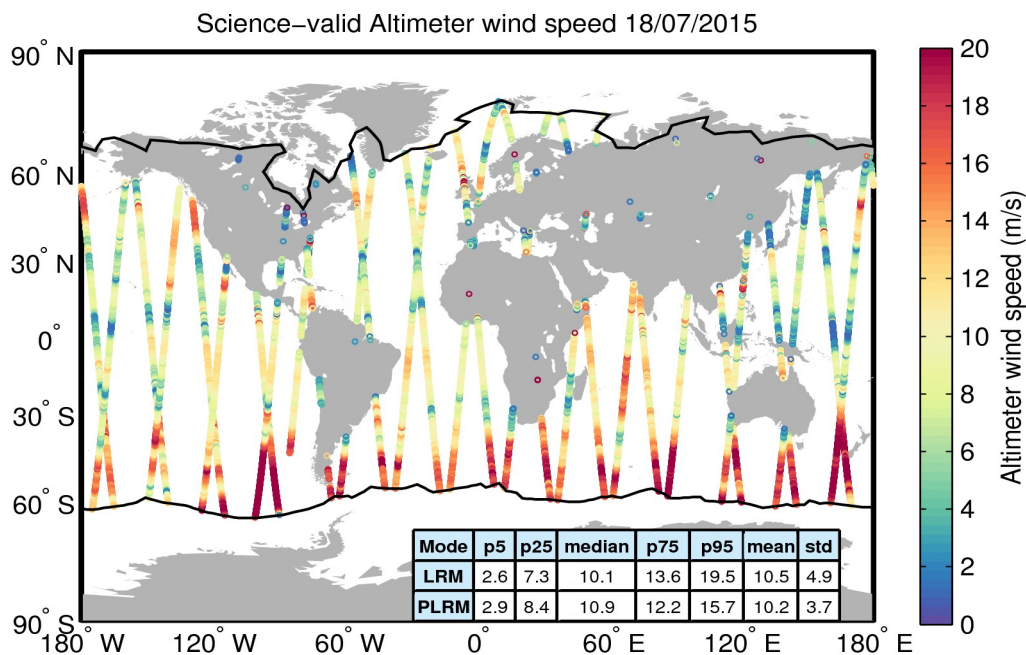
Figure 34. Geographical distribution of science-valid wind data over oceans and lakes for 18/07/2015. The statistical values shown in the table refer to the wind in m/s and are calculated separately for LRM and PLRM regions. The black lines mark the outer limit of the Arctic and Antarctic polar polygons. Gray circles denote records that have been rejected based on the editing criteria described in Table 5.
