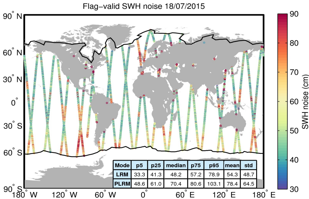
Figure 18. Geographical distribution of flag-valid 20-Hz SWH measurement noise over oceans and lakes for 18/07/2015. The statistical values shown in the table refer to the SWH noise and are calculated separately for LRM and PLRM regions. Measurements taken over polar polygons have been excluded from the computation of the statistical values. The black lines mark the outer limit of the Arctic and Antarctic polar polygons.
