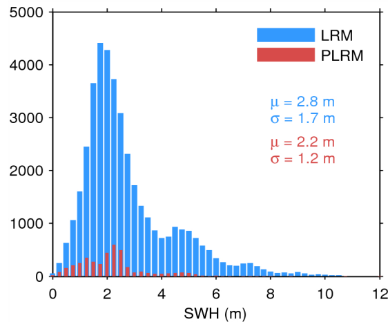
Figure 17. Histogram of flag-valid SWH over oceans and lakes for LRM (blue) and PLRM (red) for 18/07/2015. The mean ( \mu ) and standard deviation ( \sigma ) are also shown. Note that values larger than 12 m are excluded from the histogram for the sake of readability but not from the computation of \mu and \sigma .
