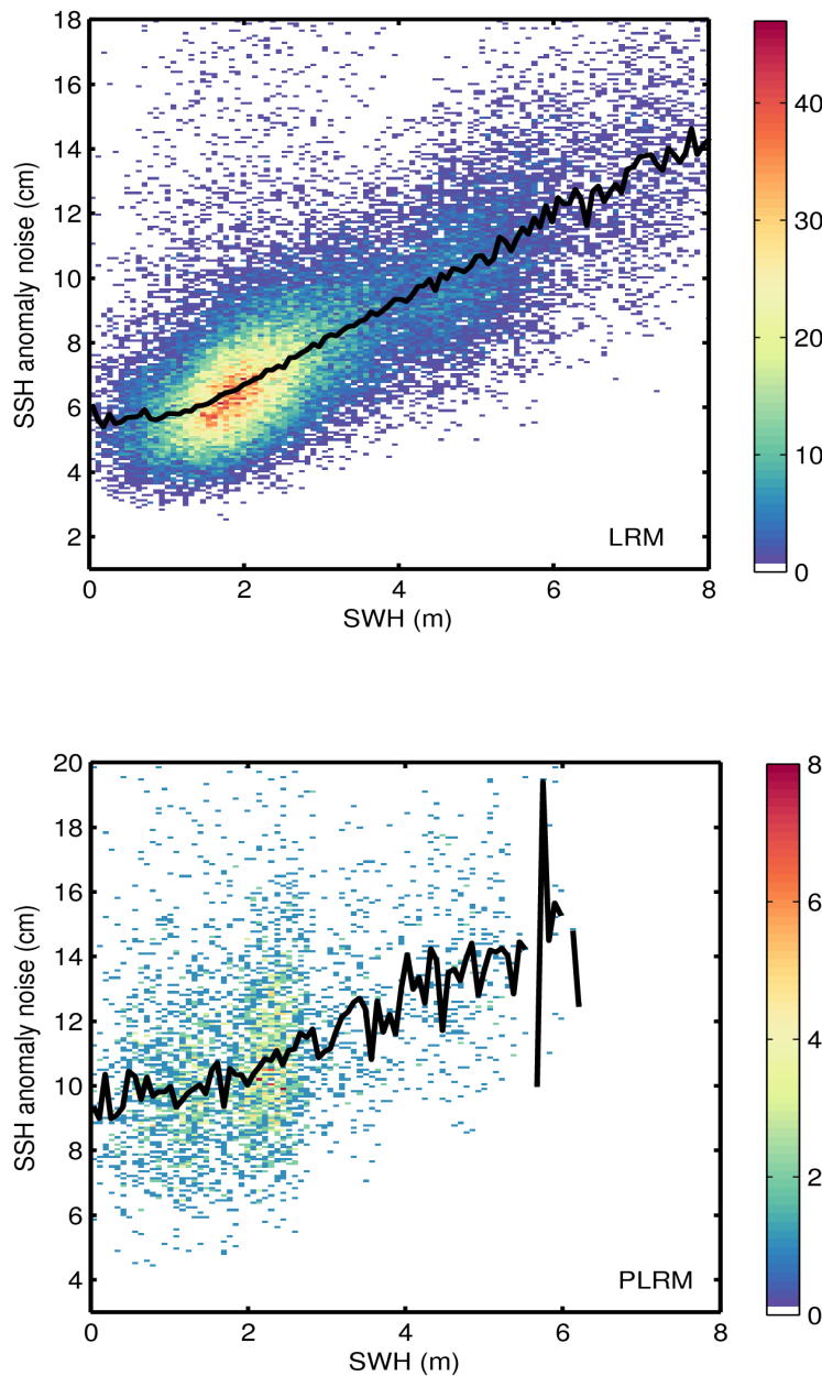
Figure 9. 2D histogram showing flag-valid SSH anomaly noise as a function of SWH for LRM (top) and PLRM (bottom) for 18/07/2015. The black line denotes the median SSH anomaly as a function of SWH.
