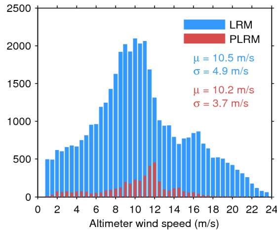
Figure 33. Histogram of flag-valid wind over oceans and lakes for LRM (blue) and PLRM (red) for 18/07/2015. The mean ( \mu ) and standard deviation ( \sigma ) are also shown. Note that values larger than 24 m/s are excluded from the histogram for the sake of readability but not from the computation of \mu and \sigma .
