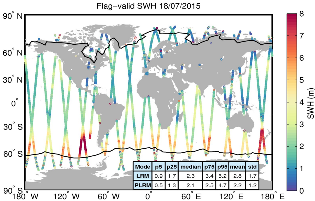
Figure 15. Geographical distribution of flag-valid SWH data over oceans and lakes for 18/07/2015. The statistical values shown in the table refer to the SWH in m and are calculated separately for LRM and PLRM regions. Measurements taken over polar polygons have been excluded from the computation of the statistical values. The black lines mark the outer limit of the Arctic and Antarctic polar polygons.
