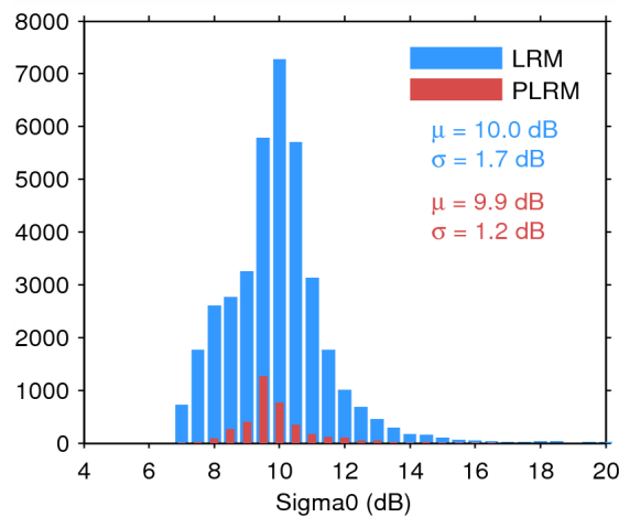
Figure 28. Histogram of science-valid sigma0 over oceans and lakes for LRM (blue) and PLRM (red) for 18/07/2015. The mean ( \mu ) and standard deviation ( \sigma ) are also shown. Note that values outside [4 20] dB are excluded from the histogram for the sake of readability but not from the computation of \mu and \sigma .
