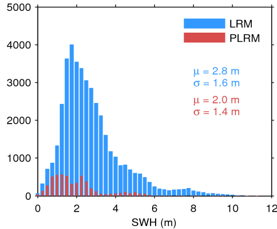
Figure 17. Histogram of flag-valid SWH over oceans and lakes for LRM (blue) and PLRM (red) for 17/07/2015. The mean ( \mu ) and standard deviation ( \sigma ) are also shown. Note that values larger than 12 m are excluded from the histogram for the sake of readability but not from the computation of \mu and \sigma .
