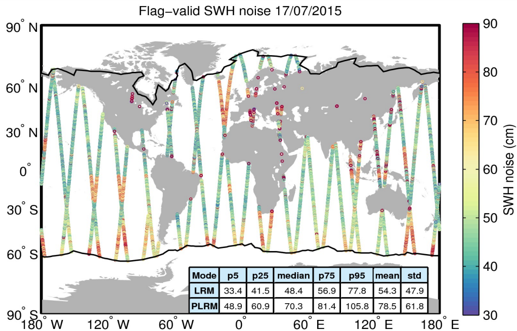
Figure 18. Geographical distribution of flag-valid 20-Hz SWH measurement noise over oceans and lakes for 17/07/2015. The statistical values shown in the table refer to the SWH noise and are calculated separately for LRM and PLRM regions. Measurements taken over polar polygons have been excluded from the computation of the statistical values. The black lines mark the outer limit of the Arctic and Antarctic polar polygons.
