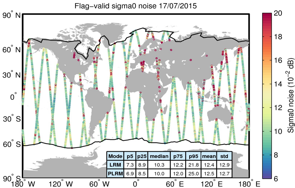
Figure 26. Geographical distribution of flag-valid 20-Hz sigma0 measurement noise over oceans and lakes for 17/07/2015. The statistical values shown in the table refer to the sigma0 noise and are calculated separately for LRM and PLRM regions. Measurements taken over polar polygons have been excluded from the computation of the statistical values. The black lines mark the outer limit of the Arctic and Antarctic polar polygons.
