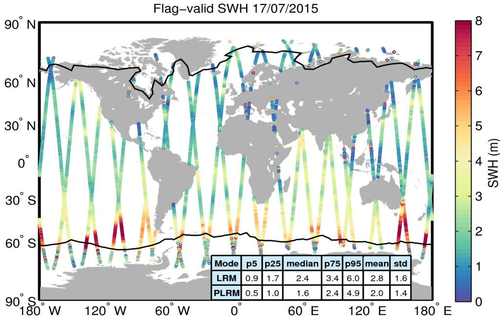
Figure 15. Geographical distribution of flag-valid SWH data over oceans and lakes for 17/07/2015. The statistical values shown in the table refer to the SWH in m and are calculated separately for LRM and PLRM regions. Measurements taken over polar polygons have been excluded from the computation of the statistical values. The black lines mark the outer limit of the Arctic and Antarctic polar polygons.
