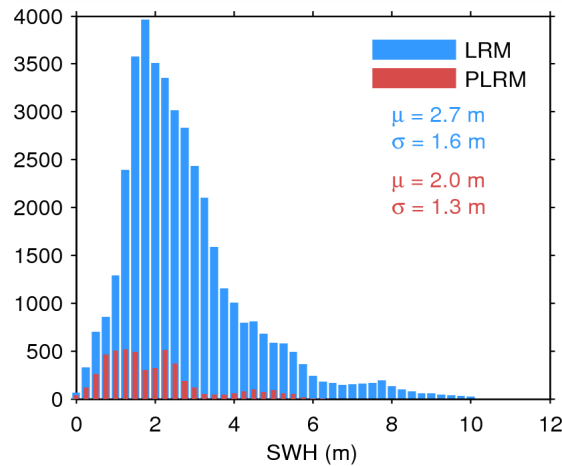
Figure 20. Histogram of science-valid SWH over oceans and lakes for LRM (blue) and PLRM (red) for 17/07/2015. The mean ( \mu ) and standard deviation ( \sigma ) are also shown. Note that values larger than 12 m are excluded from the histogram for the sake of readability but not from the computation of \mu and \sigma .
