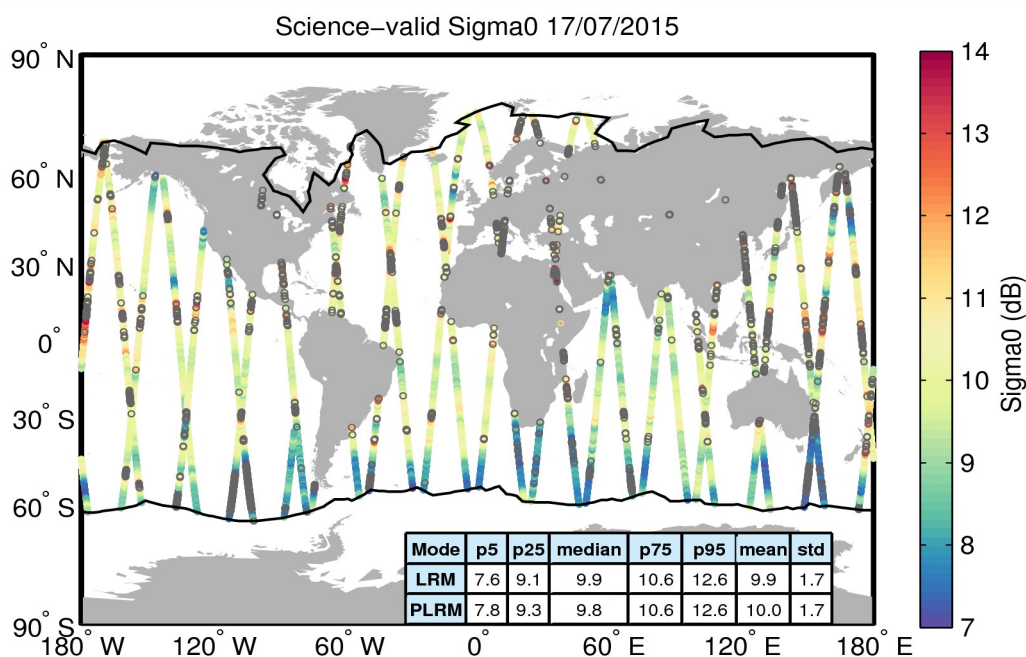
Figure 27. Geographical distribution of science-valid sigma0 data over oceans and lakes for 17/07/2015. The statistical values shown in the table refer to the sigma0 in dB and are calculated separately for LRM and PLRM regions. The black lines mark the outer limit of the Arctic and Antarctic polar polygons. Gray circles denote records that have been rejected based on the editing criteria described in Table 4.
