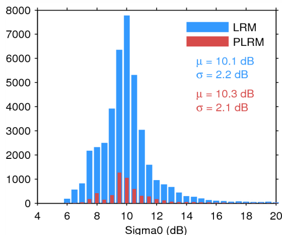
Figure 25. Histogram of flag-valid sigma0 over oceans and lakes for LRM (blue) and PLRM (red) for 17/07/2015. The mean ( \mu ) and standard deviation ( \sigma ) are also shown. Note that values outside [4 20] dB are excluded from the histogram for the sake of readability but not from the computation of \mu and \sigma .
