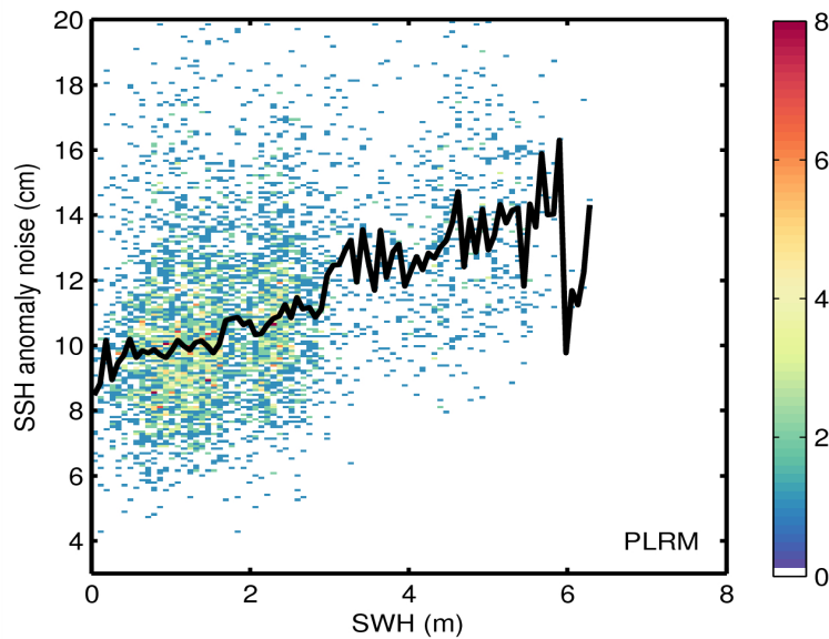
Figure 9. 2D histogram showing flag-valid SSH anomaly noise as a function of SWH for LRM (top) and PLRM (bottom) for 17/07/2015. The black line denotes the median SSH anomaly as a function of SWH.
