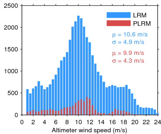
Figure 33. Histogram of flag-valid wind over oceans and lakes for LRM (blue) and PLRM (red) for 17/07/2015. The mean ( \mu ) and standard deviation ( \sigma ) are also shown. Note that values larger than 24 m/s are excluded from the histogram for the sake of readability but not from the computation of \mu and \sigma .
