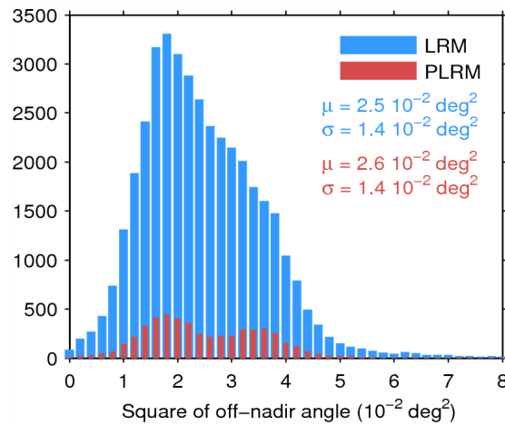
Figure 39. Histogram of flag-valid mispointing over oceans and lakes for LRM (blue) and PLRM (red) for 17/07/2015. Only positive values have been considered. The mean ( \mu ) and standard deviation ( \sigma ) are also shown. Note that values larger than 8 \cdot 10^{-2} \text{ deg}^2 are excluded from the histogram for the sake of readability but not from the computation of \mu and \sigma .
