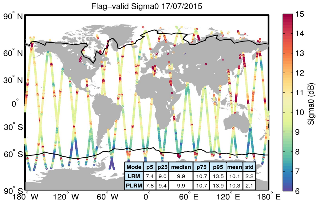
Figure 23. Geographical distribution of flag-valid sigma0 data over oceans and lakes for 17/07/2015. The statistical values shown in the table refer to the sigma0 in dB and are calculated separately for LRM and PLRM regions. Measurements taken over polar polygons have been excluded from the computation of the statistical values. The black lines mark the outer limit of the Arctic and Antarctic polar polygons.
