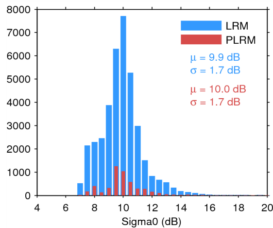
Figure 28. Histogram of science-valid sigma0 over oceans and lakes for LRM (blue) and PLRM (red) for 17/07/2015. The mean ( \mu ) and standard deviation ( \sigma ) are also shown. Note that values outside [4 20] dB are excluded from the histogram for the sake of readability but not from the computation of \mu and \sigma .
