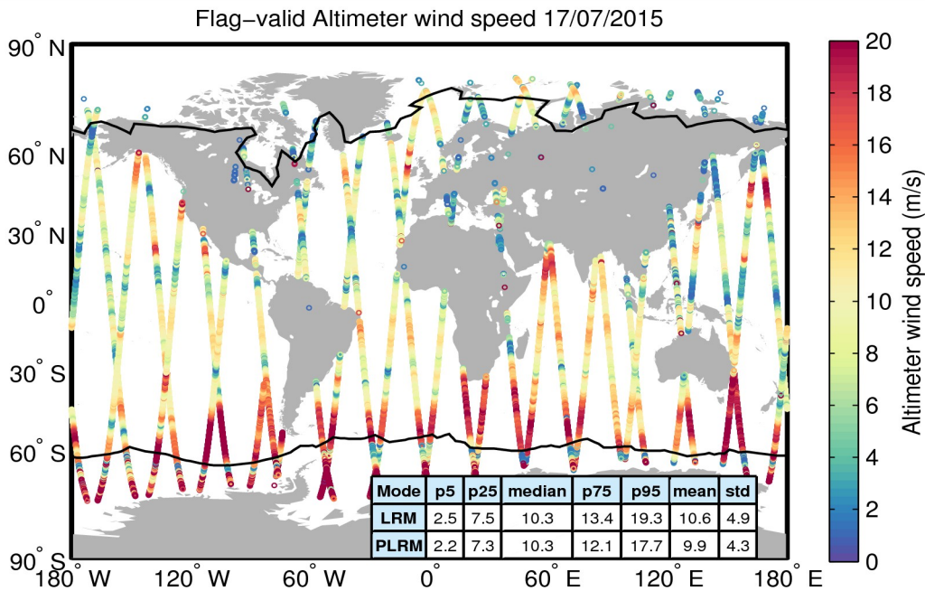
Figure 31. Geographical distribution of flag-valid wind data over oceans and lakes for 17/07/2015. The statistical values shown in the table refer to the wind in m/s and are calculated separately for LRM and PLRM regions. Measurements taken over polar polygons have been excluded from the computation of the statistical values. The black lines mark the outer limit of the Arctic and Antarctic polar polygons.
