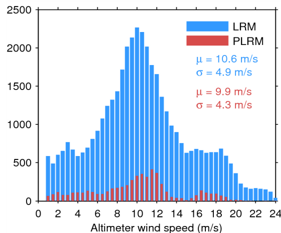
Figure 35. Histogram of science-valid wind over oceans and lakes for LRM (blue) and PLRM (red) for 17/07/2015. The mean ( \mu ) and standard deviation ( \sigma ) are also shown. Note that values larger than 24 m/s are excluded from the histogram for the sake of readability but not from the computation of \mu and \sigma .
