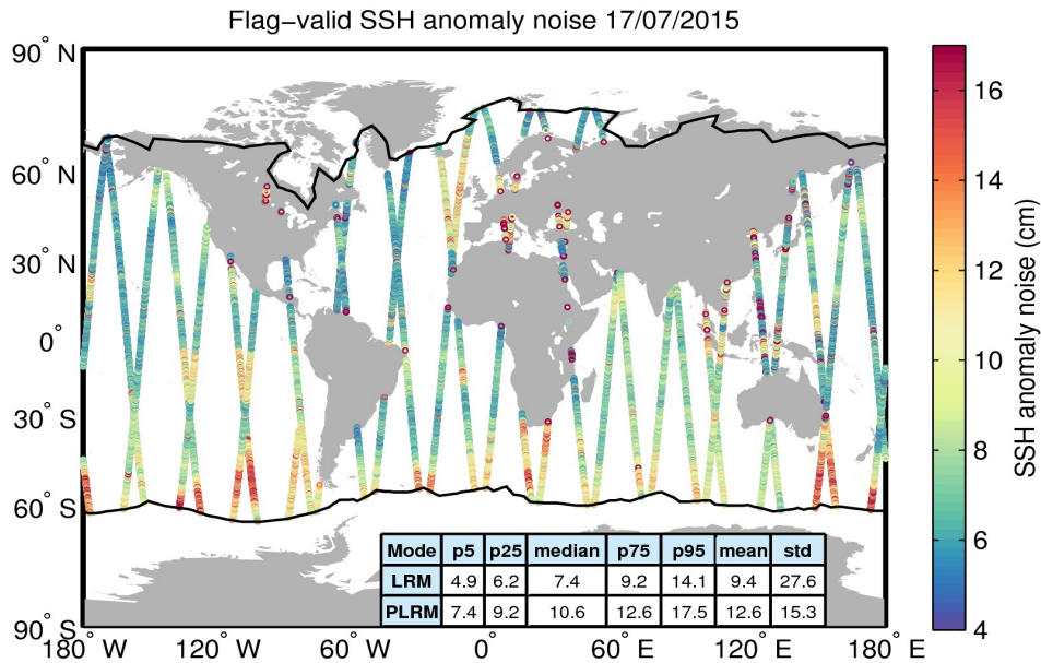
Figure 8. Geographical distribution of flag-valid 20-Hz SSH anomaly measurement noise over oceans and lakes for 17/07/2015. The statistical values shown in the table refer to the SSH anomaly noise and are calculated separately for LRM and PLRM regions. Measurements taken over polar polygons have been excluded from the computation of the statistical values. The black lines mark the outer limit of the Arctic and Antarctic polar polygons.
