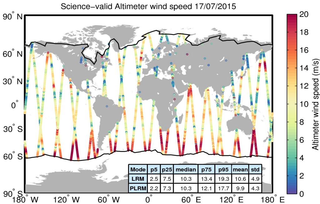
Figure 34. Geographical distribution of science-valid wind data over oceans and lakes for 17/07/2015. The statistical values shown in the table refer to the wind in m/s and are calculated separately for LRM and PLRM regions. The black lines mark the outer limit of the Arctic and Antarctic polar polygons. Gray circles denote records that have been rejected based on the editing criteria described in Table 5.
