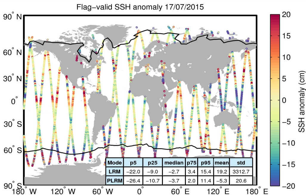
Figure 5. Geographical distribution of flag-valid 1-Hz SSH anomaly data over oceans and lakes for 17/07/2015. The statistical values shown in the table refer to the SSH anomaly in cm and are calculated separately for LRM and PLRM regions. Measurements taken over polar polygons have been excluded from the computation of the statistical values. The black lines mark the outer limit of the Arctic and Antarctic polar polygons.
