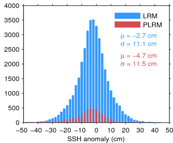
Figure 11. Histogram of science-valid SSH anomaly over oceans and lakes for LRM (blue) and PLRM (red) for 17/07/2015. The mean ( \mu ) and standard deviation ( \sigma ) are also shown. Note that values outside [-50\ 50] cm are excluded from the histogram for the sake of readability but not from the computation of \mu and \sigma .
