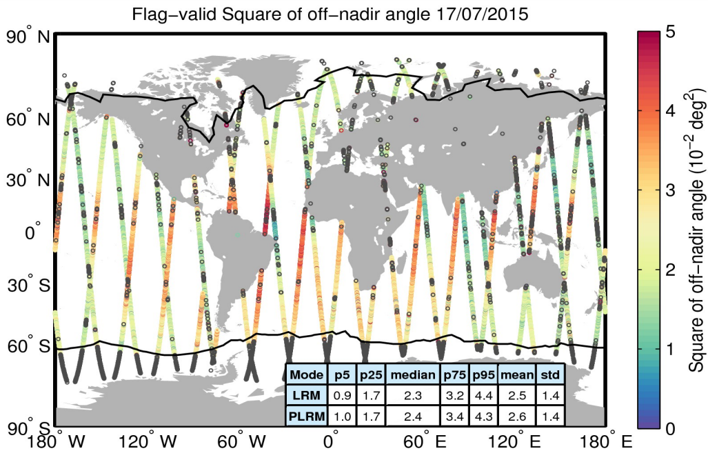
Figure 37. Geographical distribution of flag-valid mispointing data over oceans and lakes for 17/07/2015. The statistical values shown in the table refer to the mispointing in 10^{-2} deg 2 and are calculated separately for LRM and PLRM regions. Measurements taken over polar polygons have been excluded from the computation of the statistical values. The black lines mark the outer limit of the Arctic and Antarctic polar polygons. Gray circles denote negative values.
