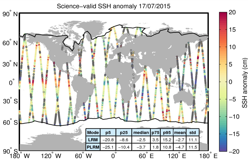
Figure 10. Geographical distribution of science-valid SSH anomaly data over oceans and lakes for 17/07/2015. The statistical values shown in the table refer to the SSH anomaly in cm and are calculated separately for LRM and PLRM regions. The black lines mark the outer limit of the Arctic and Antarctic polar polygons. Gray circles denote records that have been rejected based on the editing criteria described in Table 2.
