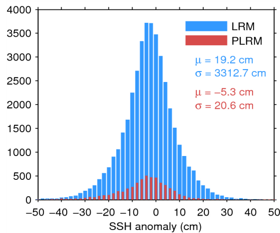
Figure 7. Histogram of flag-valid SSH anomaly over oceans and lakes for LRM (blue) and PLRM (red) for 17/07/2015. The mean ( \mu ) and standard deviation ( \sigma ) are also shown. Note that values outside [-50\ 50] cm are excluded from the histogram for the sake of readability but not from the computation of \mu and \sigma .
