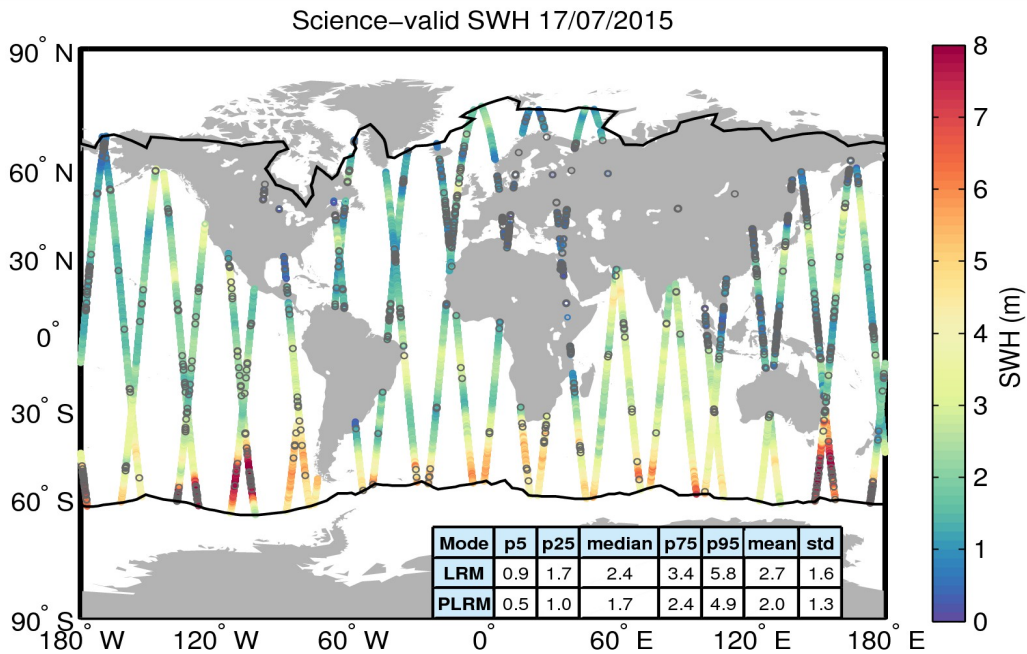
Figure 19. Geographical distribution of science-valid SWH data over oceans and lakes for 17/07/2015. The statistical values shown in the table refer to the SWH in m and are calculated separately for LRM and PLRM regions. The black lines mark the outer limit of the Arctic and Antarctic polar polygons. Gray circles denote records that have been rejected based on the editing criteria described in Table 3.
