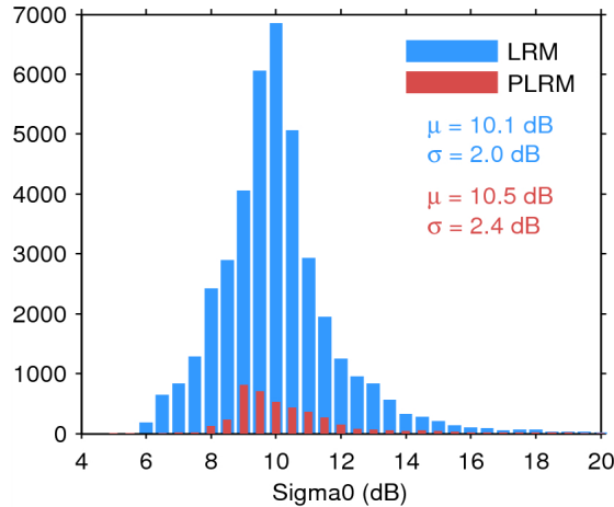
Figure 25. Histogram of flag-valid sigma0 over oceans and lakes for LRM (blue) and PLRM (red) for 16/07/2015. The mean ( \mu ) and standard deviation ( \sigma ) are also shown. Note that values outside [4 20] dB are excluded from the histogram for the sake of readability but not from the computation of \mu and \sigma .
