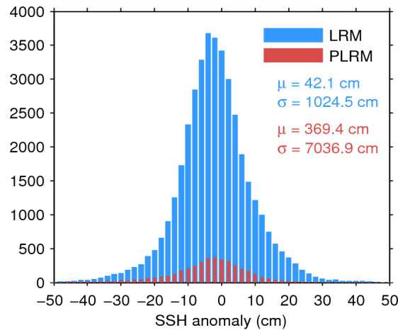
Figure 7. Histogram of flag-valid SSH anomaly over oceans and lakes for LRM (blue) and PLRM (red) for 16/07/2015. The mean ( \mu ) and standard deviation ( \sigma ) are also shown. Note that values outside [-50\ 50] cm are excluded from the histogram for the sake of readability but not from the computation of \mu and \sigma .
