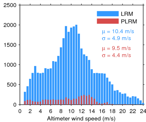
Figure 33. Histogram of flag-valid wind over oceans and lakes for LRM (blue) and PLRM (red) for 16/07/2015. The mean ( \mu ) and standard deviation ( \sigma ) are also shown. Note that values larger than 24 m/s are excluded from the histogram for the sake of readability but not from the computation of \mu and \sigma .
