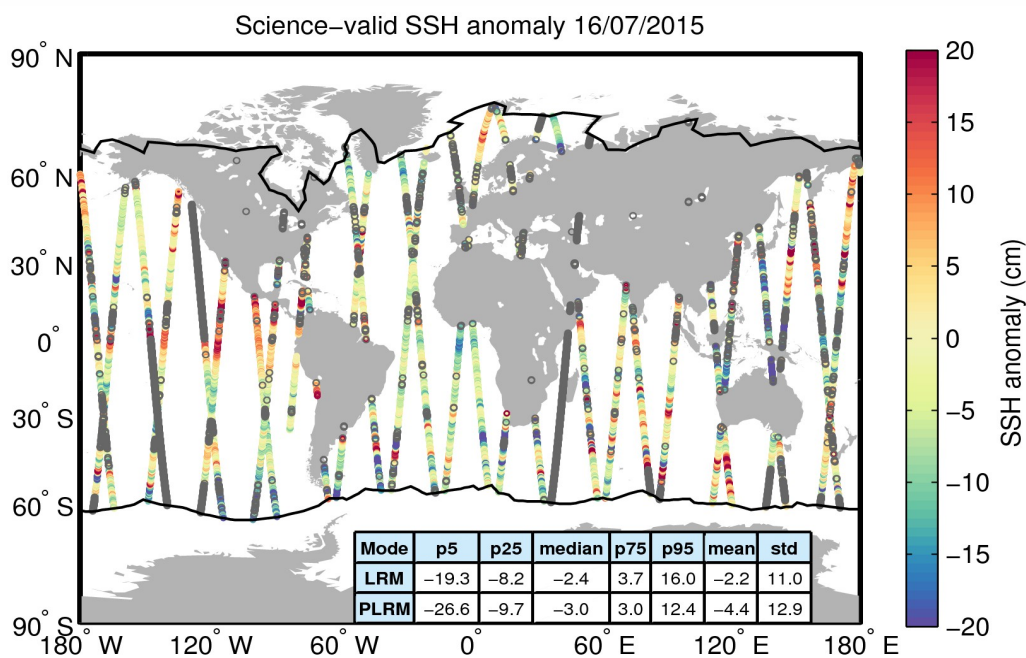
Figure 10. Geographical distribution of science-valid SSH anomaly data over oceans and lakes for 16/07/2015. The statistical values shown in the table refer to the SSH anomaly in cm and are calculated separately for LRM and PLRM regions. The black lines mark the outer limit of the Arctic and Antarctic polar polygons. Gray circles denote records that have been rejected based on the editing criteria described in Table 2.
