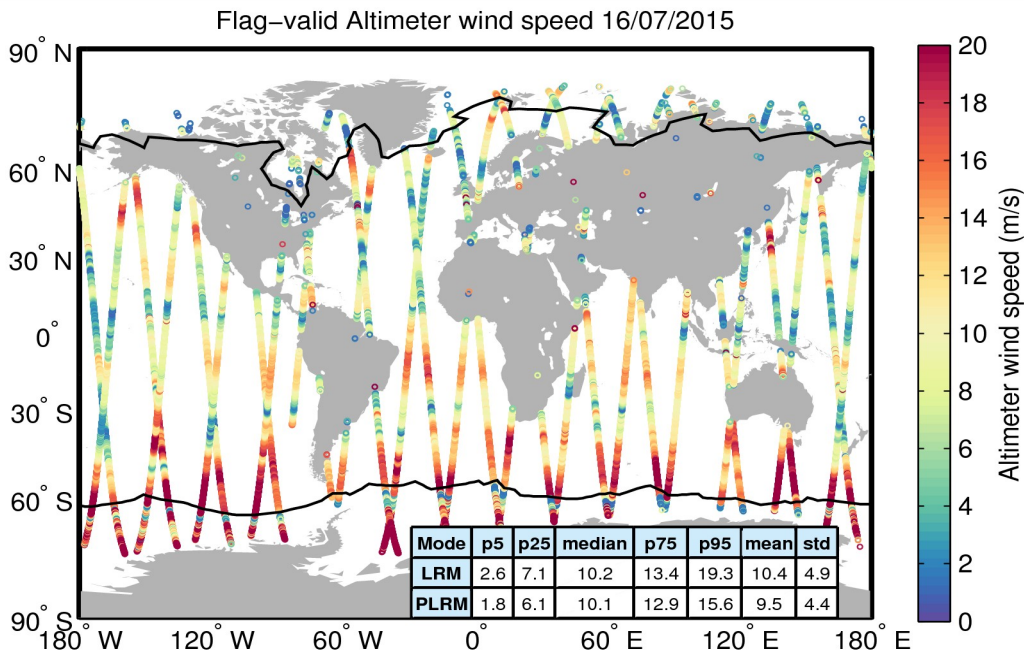
Figure 31. Geographical distribution of flag-valid wind data over oceans and lakes for 16/07/2015. The statistical values shown in the table refer to the wind in m/s and are calculated separately for LRM and PLRM regions. Measurements taken over polar polygons have been excluded from the computation of the statistical values. The black lines mark the outer limit of the Arctic and Antarctic polar polygons.
