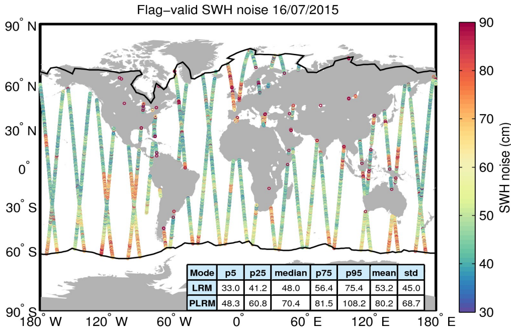
Figure 18. Geographical distribution of flag-valid 20-Hz SWH measurement noise over oceans and lakes for 16/07/2015. The statistical values shown in the table refer to the SWH noise and are calculated separately for LRM and PLRM regions. Measurements taken over polar polygons have been excluded from the computation of the statistical values. The black lines mark the outer limit of the Arctic and Antarctic polar polygons.
