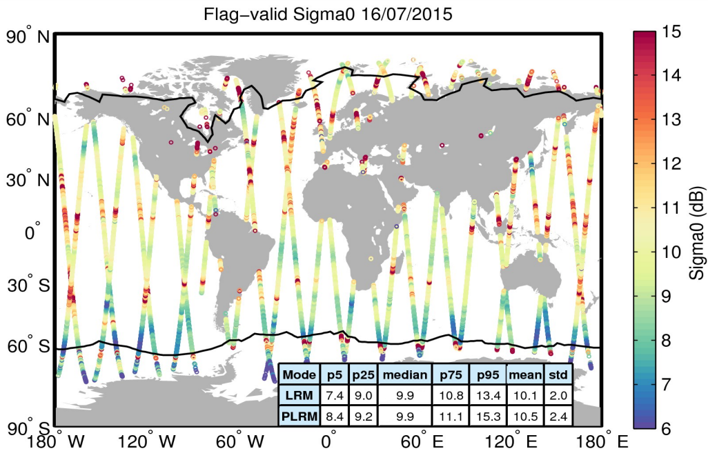
Figure 23. Geographical distribution of flag-valid sigma0 data over oceans and lakes for 16/07/2015. The statistical values shown in the table refer to the sigma0 in dB and are calculated separately for LRM and PLRM regions. Measurements taken over polar polygons have been excluded from the computation of the statistical values. The black lines mark the outer limit of the Arctic and Antarctic polar polygons.
