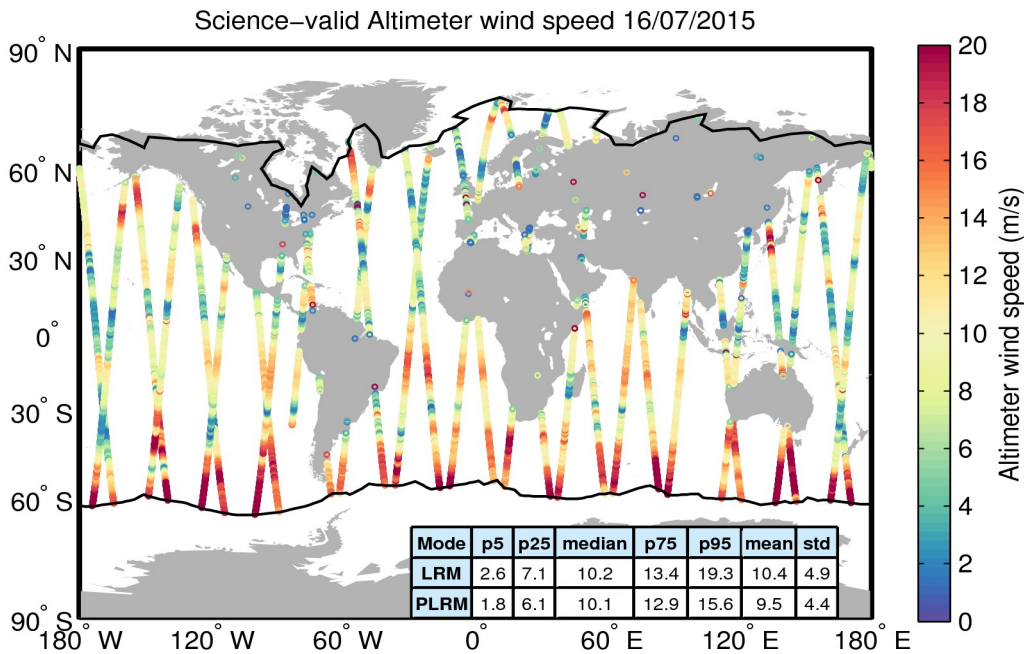
Figure 34. Geographical distribution of science-valid wind data over oceans and lakes for 16/07/2015. The statistical values shown in the table refer to the wind in m/s and are calculated separately for LRM and PLRM regions. The black lines mark the outer limit of the Arctic and Antarctic polar polygons. Gray circles denote records that have been rejected based on the editing criteria described in Table 5.
