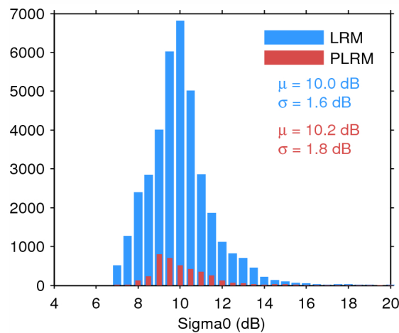
Figure 28. Histogram of science-valid sigma0 over oceans and lakes for LRM (blue) and PLRM (red) for 16/07/2015. The mean ( \mu ) and standard deviation ( \sigma ) are also shown. Note that values outside [4 20] dB are excluded from the histogram for the sake of readability but not from the computation of \mu and \sigma .
