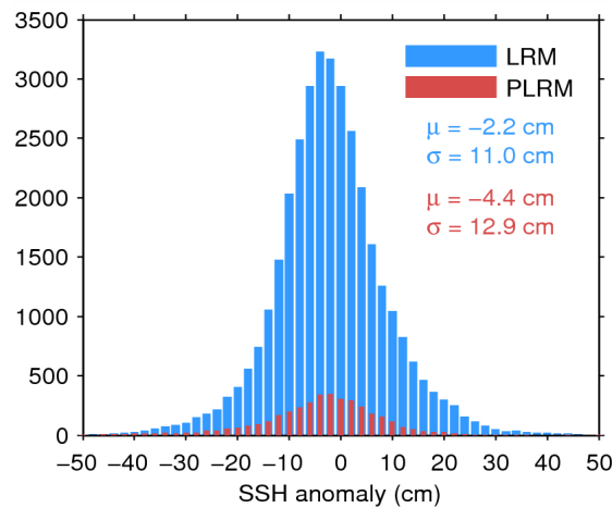
Figure 11. Histogram of science-valid SSH anomaly over oceans and lakes for LRM (blue) and PLRM (red) for 16/07/2015. The mean ( \mu ) and standard deviation ( \sigma ) are also shown. Note that values outside [-50 50] cm are excluded from the histogram for the sake of readability but not from the computation of \mu and \sigma .
