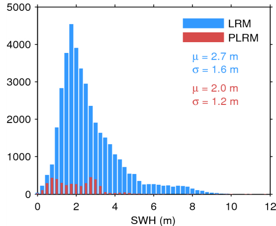
Figure 17. Histogram of flag-valid SWH over oceans and lakes for LRM (blue) and PLRM (red) for 16/07/2015. The mean ( \mu ) and standard deviation ( \sigma ) are also shown. Note that values larger than 12 m are excluded from the histogram for the sake of readability but not from the computation of \mu and \sigma .
