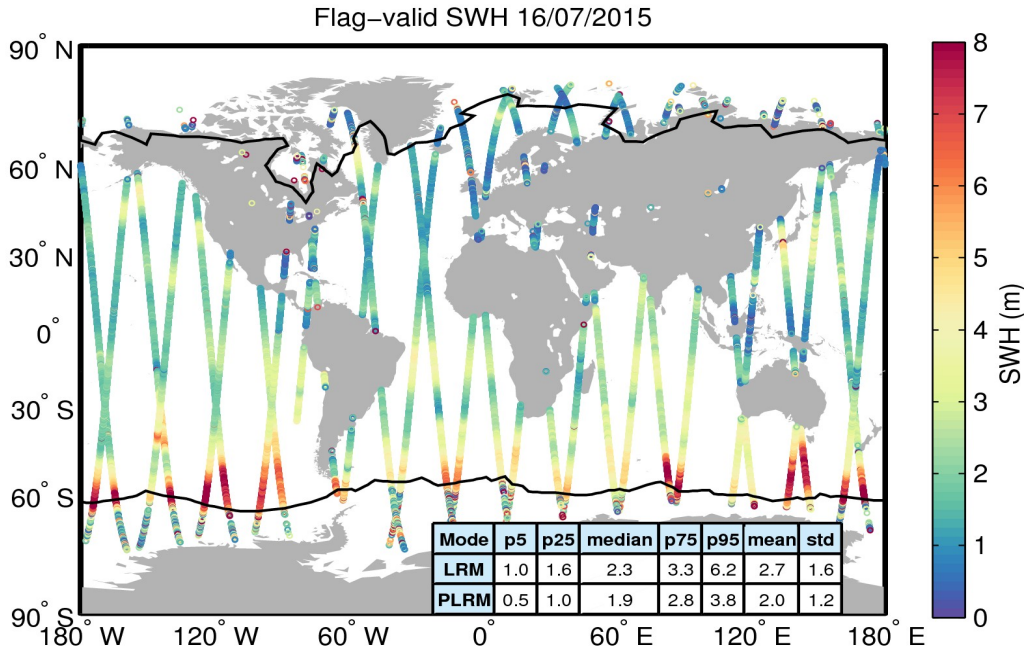
Figure 15. Geographical distribution of flag-valid SWH data over oceans and lakes for 16/07/2015. The statistical values shown in the table refer to the SWH in m and are calculated separately for LRM and PLRM regions. Measurements taken over polar polygons have been excluded from the computation of the statistical values. The black lines mark the outer limit of the Arctic and Antarctic polar polygons.
