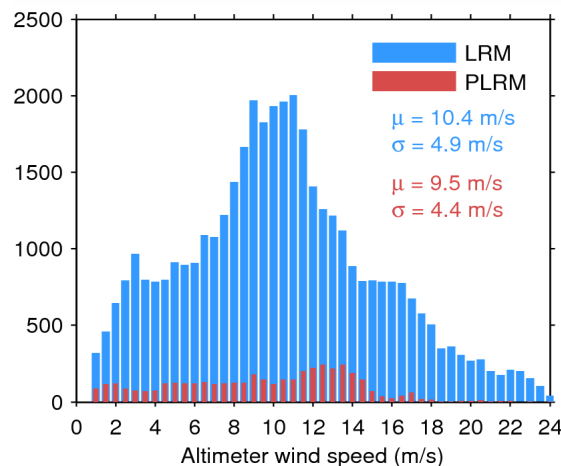
Figure 35. Histogram of science-valid wind over oceans and lakes for LRM (blue) and PLRM (red) for 16/07/2015. The mean ( \mu ) and standard deviation ( \sigma ) are also shown. Note that values larger than 24 m/s are excluded from the histogram for the sake of readability but not from the computation of \mu and \sigma .
