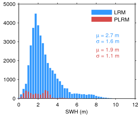
Figure 20. Histogram of science-valid SWH over oceans and lakes for LRM (blue) and PLRM (red) for 16/07/2015. The mean ( \mu ) and standard deviation ( \sigma ) are also shown. Note that values larger than 12 m are excluded from the histogram for the sake of readability but not from the computation of \mu and \sigma .
