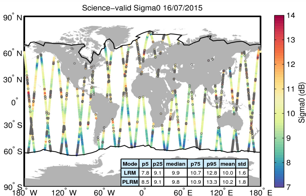
Figure 27. Geographical distribution of science-valid sigma0 data over oceans and lakes for 16/07/2015. The statistical values shown in the table refer to the sigma0 in dB and are calculated separately for LRM and PLRM regions. The black lines mark the outer limit of the Arctic and Antarctic polar polygons. Gray circles denote records that have been rejected based on the editing criteria described in Table 4.
