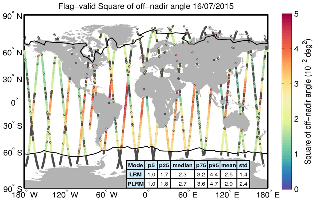
Figure 37. Geographical distribution of flag-valid mispointing data over oceans and lakes for 16/07/2015. The statistical values shown in the table refer to the mispointing in 10^{-2} \text{ deg}^2 and are calculated separately for LRM and PLRM regions. Measurements taken over polar polygons have been excluded from the computation of the statistical values. The black lines mark the outer limit of the Arctic and Antarctic polar polygons. Gray circles denote negative values.
