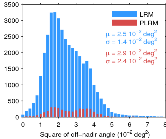
Figure 39. Histogram of flag-valid mispointing over oceans and lakes for LRM (blue) and PLRM (red) for 16/07/2015. Only positive values have been considered. The mean ( \mu ) and standard deviation ( \sigma ) are also shown. Note that values larger than 8 \cdot 10^{-2} \text{ deg}^2 are excluded from the histogram for the sake of readability but not from the computation of \mu and \sigma .
