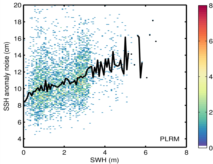
Figure 9. 2D histogram showing flag-valid SSH anomaly noise as a function of SWH for LRM (top) and PLRM (bottom) for 16/07/2015. The black line denotes the median SSH anomaly as a function of SWH.
