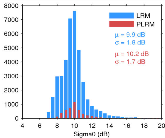
Figure 28. Histogram of science-valid sigma0 over oceans and lakes for LRM (blue) and PLRM (red) for 15/07/2015. The mean ( \mu ) and standard deviation ( \sigma ) are also shown. Note that values outside [4 20] dB are excluded from the histogram for the sake of readability but not from the computation of \mu and \sigma .
