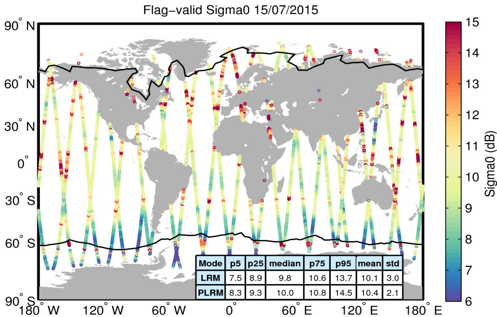
Figure 23. Geographical distribution of flag-valid sigma0 data over oceans and lakes for 15/07/2015. The statistical values shown in the table refer to the sigma0 in dB and are calculated separately for LRM and PLRM regions. Measurements taken over polar polygons have been excluded from the computation of the statistical values. The black lines mark the outer limit of the Arctic and Antarctic polar polygons.
