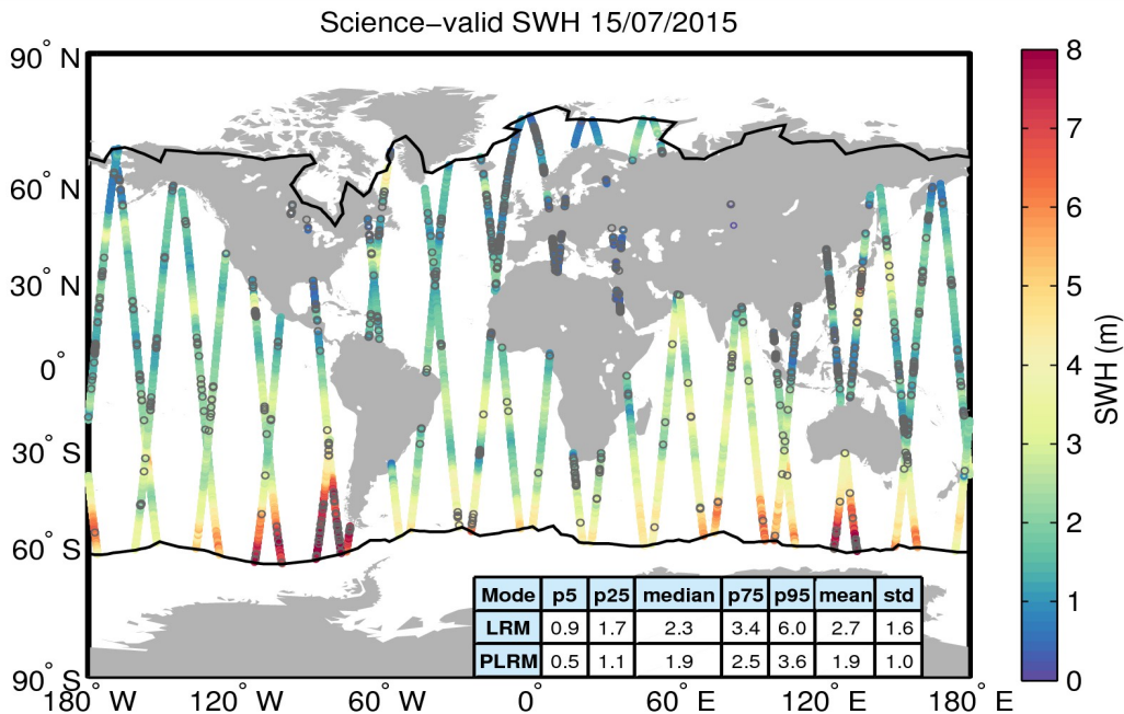
Figure 19. Geographical distribution of science-valid SWH data over oceans and lakes for 15/07/2015. The statistical values shown in the table refer to the SWH in m and are calculated separately for LRM and PLRM regions. The black lines mark the outer limit of the Arctic and Antarctic polar polygons. Gray circles denote records that have been rejected based on the editing criteria described in Table 3.
