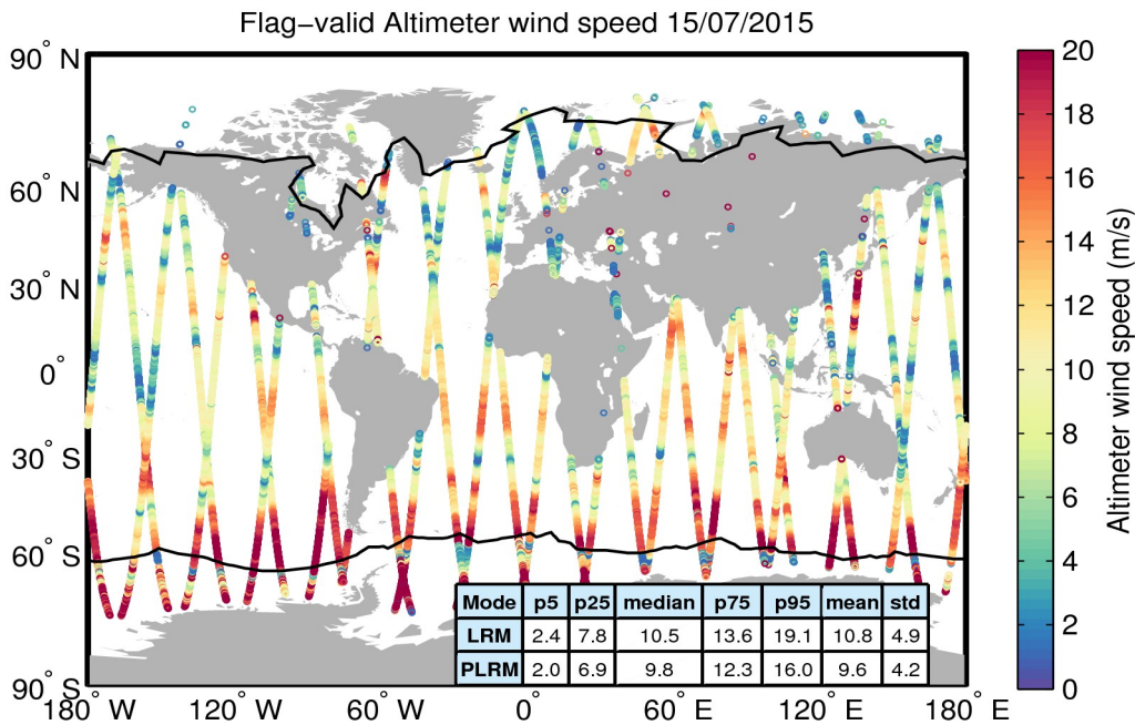
Figure 31. Geographical distribution of flag-valid wind data over oceans and lakes for 15/07/2015. The statistical values shown in the table refer to the wind in m/s and are calculated separately for LRM and PLRM regions. Measurements taken over polar polygons have been excluded from the computation of the statistical values. The black lines mark the outer limit of the Arctic and Antarctic polar polygons.
