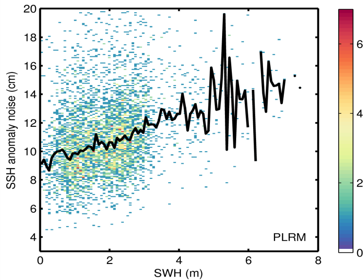
Figure 9. 2D histogram showing flag-valid SSH anomaly noise as a function of SWH for LRM (top) and PLRM (bottom) for 15/07/2015. The black line denotes the median SSH anomaly as a function of SWH.
