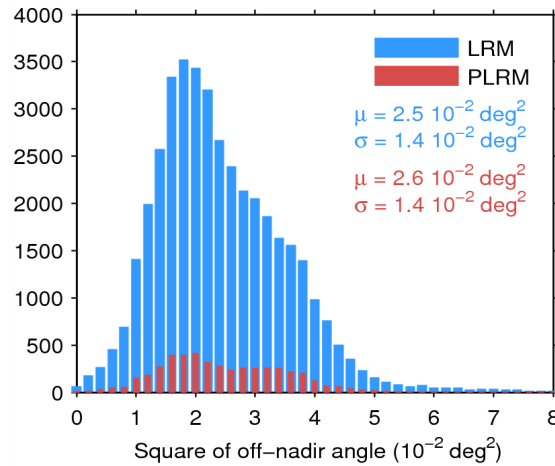
Figure 39. Histogram of flag-valid mispointing over oceans and lakes for LRM (blue) and PLRM (red) for 15/07/2015. Only positive values have been considered. The mean ( \mu ) and standard deviation ( \sigma ) are also shown. Note that values larger than 8 \cdot 10^{-2} \text{ deg}^2 are excluded from the histogram for the sake of readability but not from the computation of \mu and \sigma .
