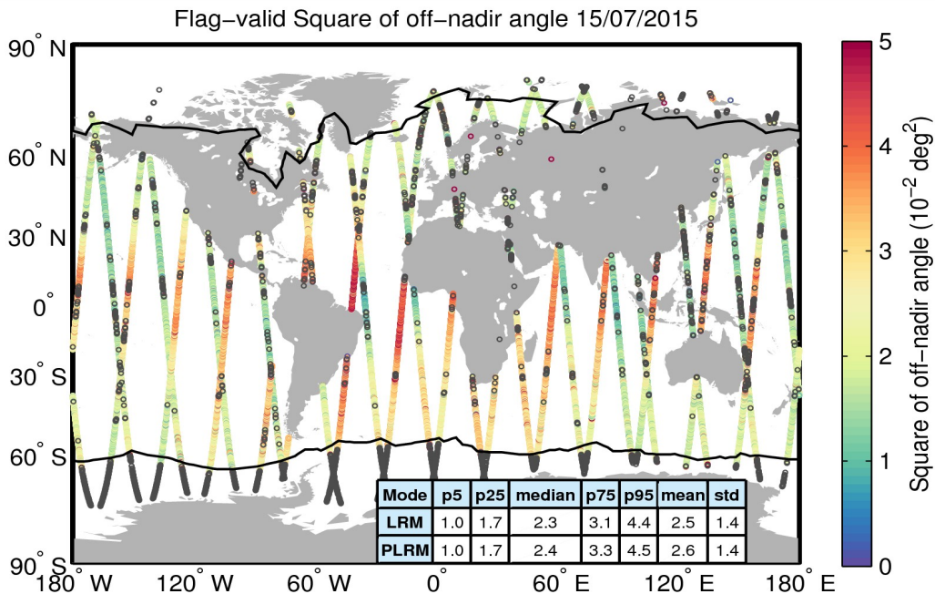
Figure 37. Geographical distribution of flag-valid mispointing data over oceans and lakes for 15/07/2015. The statistical values shown in the table refer to the mispointing in 10^{-2} deg 2 and are calculated separately for LRM and PLRM regions. Measurements taken over polar polygons have been excluded from the computation of the statistical values. The black lines mark the outer limit of the Arctic and Antarctic polar polygons. Gray circles denote negative values.
