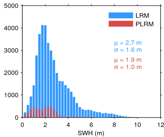
Figure 20. Histogram of science-valid SWH over oceans and lakes for LRM (blue) and PLRM (red) for 15/07/2015. The mean ( \mu ) and standard deviation ( \sigma ) are also shown. Note that values larger than 12 m are excluded from the histogram for the sake of readability but not from the computation of \mu and \sigma .
