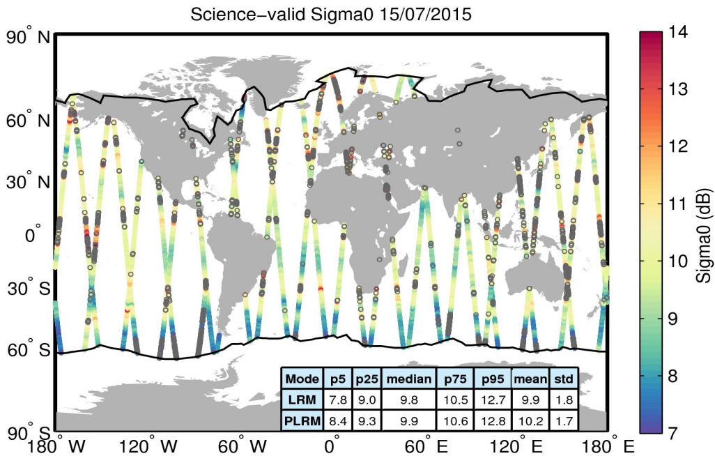
Figure 27. Geographical distribution of science-valid sigma0 data over oceans and lakes for 15/07/2015. The statistical values shown in the table refer to the sigma0 in dB and are calculated separately for LRM and PLRM regions. The black lines mark the outer limit of the Arctic and Antarctic polar polygons. Gray circles denote records that have been rejected based on the editing criteria described in Table 4.
