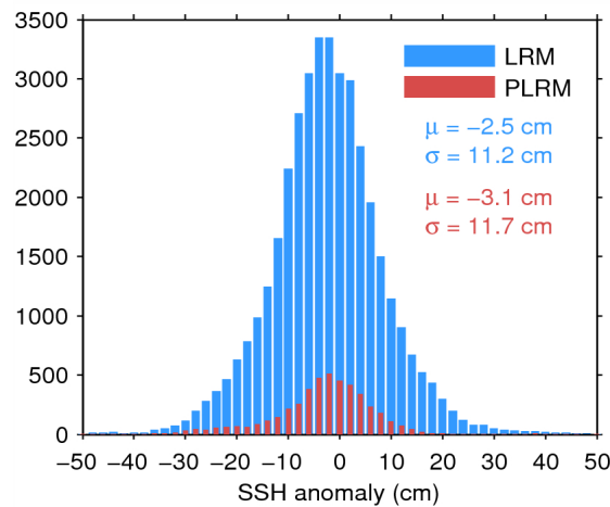
Figure 11. Histogram of science-valid SSH anomaly over oceans and lakes for LRM (blue) and PLRM (red) for 15/07/2015. The mean ( \mu ) and standard deviation ( \sigma ) are also shown. Note that values outside [-50\ 50] cm are excluded from the histogram for the sake of readability but not from the computation of \mu and \sigma .
