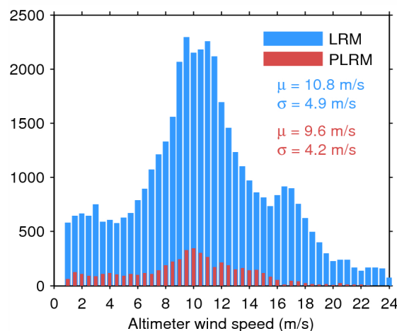
Figure 35. Histogram of science-valid wind over oceans and lakes for LRM (blue) and PLRM (red) for 15/07/2015. The mean ( \mu ) and standard deviation ( \sigma ) are also shown. Note that values larger than 24 m/s are excluded from the histogram for the sake of readability but not from the computation of \mu and \sigma .
