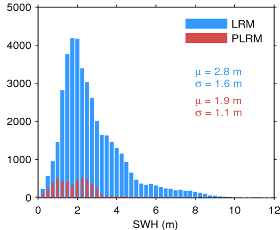
Figure 17. Histogram of flag-valid SWH over oceans and lakes for LRM (blue) and PLRM (red) for 15/07/2015. The mean ( \mu ) and standard deviation ( \sigma ) are also shown. Note that values larger than 12 m are excluded from the histogram for the sake of readability but not from the computation of \mu and \sigma .
