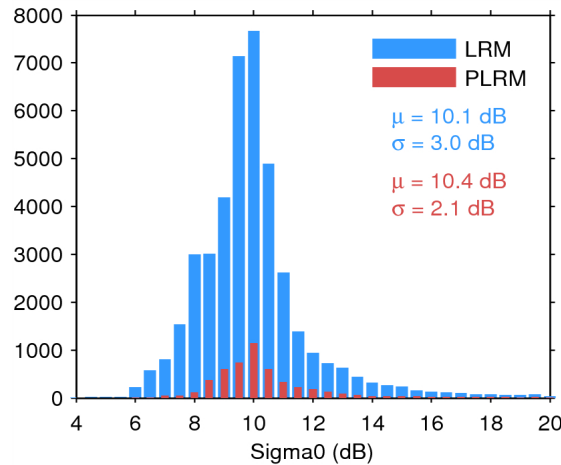
Figure 25. Histogram of flag-valid sigma0 over oceans and lakes for LRM (blue) and PLRM (red) for 15/07/2015. The mean ( \mu ) and standard deviation ( \sigma ) are also shown. Note that values outside [4 20] dB are excluded from the histogram for the sake of readability but not from the computation of \mu and \sigma .
