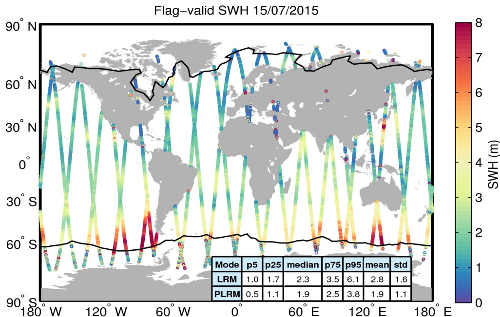
Figure 15. Geographical distribution of flag-valid SWH data over oceans and lakes for 15/07/2015. The statistical values shown in the table refer to the SWH in m and are calculated separately for LRM and PLRM regions. Measurements taken over polar polygons have been excluded from the computation of the statistical values. The black lines mark the outer limit of the Arctic and Antarctic polar polygons.
