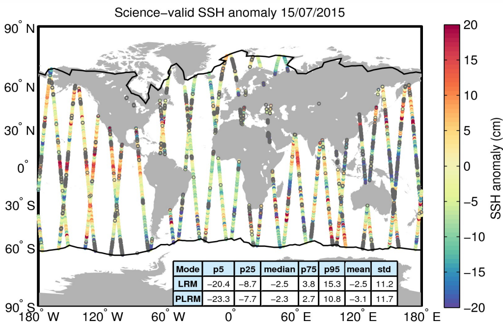
Figure 10. Geographical distribution of science-valid SSH anomaly data over oceans and lakes for 15/07/2015. The statistical values shown in the table refer to the SSH anomaly in cm and are calculated separately for LRM and PLRM regions. The black lines mark the outer limit of the Arctic and Antarctic polar polygons. Gray circles denote records that have been rejected based on the editing criteria described in Table 2.
