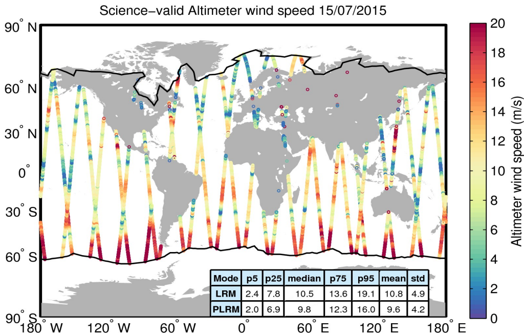
Figure 34. Geographical distribution of science-valid wind data over oceans and lakes for 15/07/2015. The statistical values shown in the table refer to the wind in m/s and are calculated separately for LRM and PLRM regions. The black lines mark the outer limit of the Arctic and Antarctic polar polygons. Gray circles denote records that have been rejected based on the editing criteria described in Table 5.
