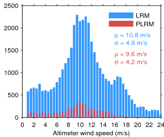
Figure 33. Histogram of flag-valid wind over oceans and lakes for LRM (blue) and PLRM (red) for 15/07/2015. The mean ( \mu ) and standard deviation ( \sigma ) are also shown. Note that values larger than 24 m/s are excluded from the histogram for the sake of readability but not from the computation of \mu and \sigma .
