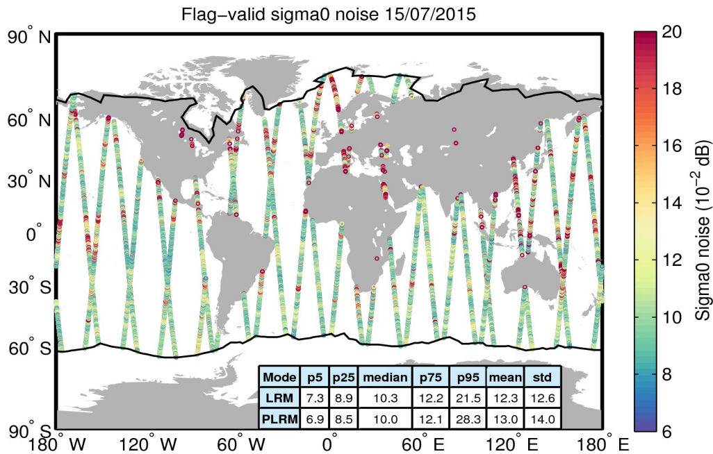
Figure 26. Geographical distribution of flag-valid 20-Hz sigma0 measurement noise over oceans and lakes for 15/07/2015. The statistical values shown in the table refer to the sigma0 noise and are calculated separately for LRM and PLRM regions. Measurements taken over polar polygons have been excluded from the computation of the statistical values. The black lines mark the outer limit of the Arctic and Antarctic polar polygons.
