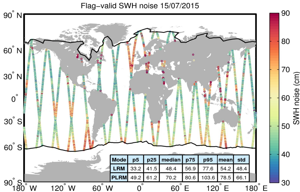
Figure 18. Geographical distribution of flag-valid 20-Hz SWH measurement noise over oceans and lakes for 15/07/2015. The statistical values shown in the table refer to the SWH noise and are calculated separately for LRM and PLRM regions. Measurements taken over polar polygons have been excluded from the computation of the statistical values. The black lines mark the outer limit of the Arctic and Antarctic polar polygons.
