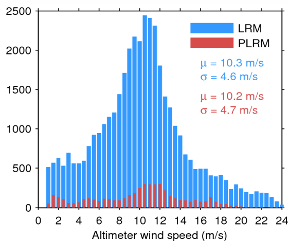
Figure 33. Histogram of flag-valid wind over oceans and lakes for LRM (blue) and PLRM (red) for 12/07/2015. The mean ( \mu ) and standard deviation ( \sigma ) are also shown. Note that values larger than 24 m/s are excluded from the histogram for the sake of readability but not from the computation of \mu and \sigma .
