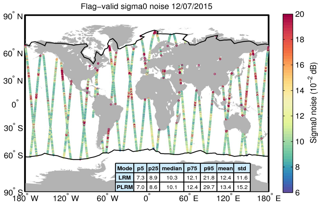
Figure 26. Geographical distribution of flag-valid 20-Hz sigma0 measurement noise over oceans and lakes for 12/07/2015. The statistical values shown in the table refer to the sigma0 noise and are calculated separately for LRM and PLRM regions. Measurements taken over polar polygons have been excluded from the computation of the statistical values. The black lines mark the outer limit of the Arctic and Antarctic polar polygons.
