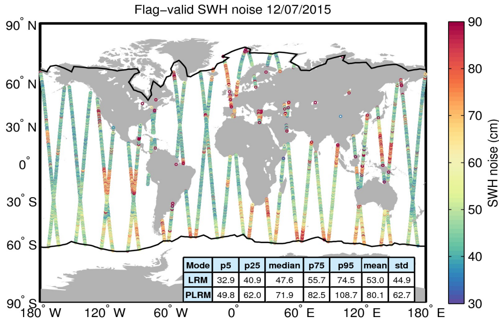
Figure 18. Geographical distribution of flag-valid 20-Hz SWH measurement noise over oceans and lakes for 12/07/2015. The statistical values shown in the table refer to the SWH noise and are calculated separately for LRM and PLRM regions. Measurements taken over polar polygons have been excluded from the computation of the statistical values. The black lines mark the outer limit of the Arctic and Antarctic polar polygons.
