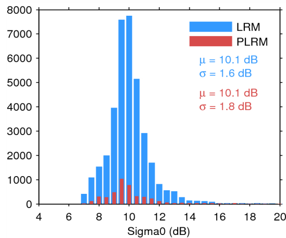
Figure 28. Histogram of science-valid sigma0 over oceans and lakes for LRM (blue) and PLRM (red) for 12/07/2015. The mean ( \mu ) and standard deviation ( \sigma ) are also shown. Note that values outside [4 20] dB are excluded from the histogram for the sake of readability but not from the computation of \mu and \sigma .
