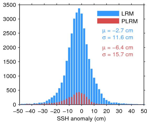
Figure 11. Histogram of science-valid SSH anomaly over oceans and lakes for LRM (blue) and PLRM (red) for 12/07/2015. The mean ( \mu ) and standard deviation ( \sigma ) are also shown. Note that values outside [-50 50] cm are excluded from the histogram for the sake of readability but not from the computation of \mu and \sigma .
