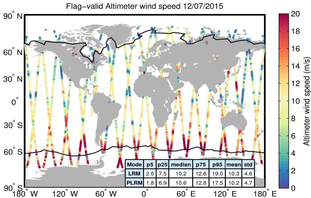
Figure 31. Geographical distribution of flag-valid wind data over oceans and lakes for 12/07/2015. The statistical values shown in the table refer to the wind in m/s and are calculated separately for LRM and PLRM regions. Measurements taken over polar polygons have been excluded from the computation of the statistical values. The black lines mark the outer limit of the Arctic and Antarctic polar polygons.
