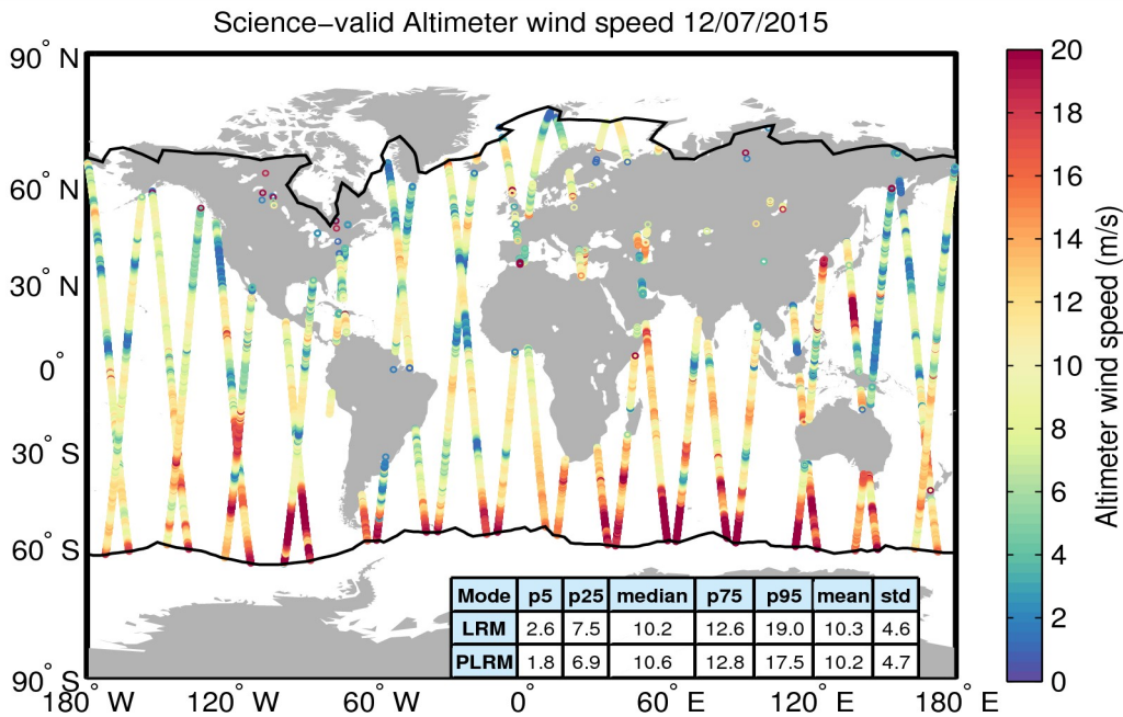
Figure 34. Geographical distribution of science-valid wind data over oceans and lakes for 12/07/2015. The statistical values shown in the table refer to the wind in m/s and are calculated separately for LRM and PLRM regions. The black lines mark the outer limit of the Arctic and Antarctic polar polygons. Gray circles denote records that have been rejected based on the editing criteria described in Table 5.
