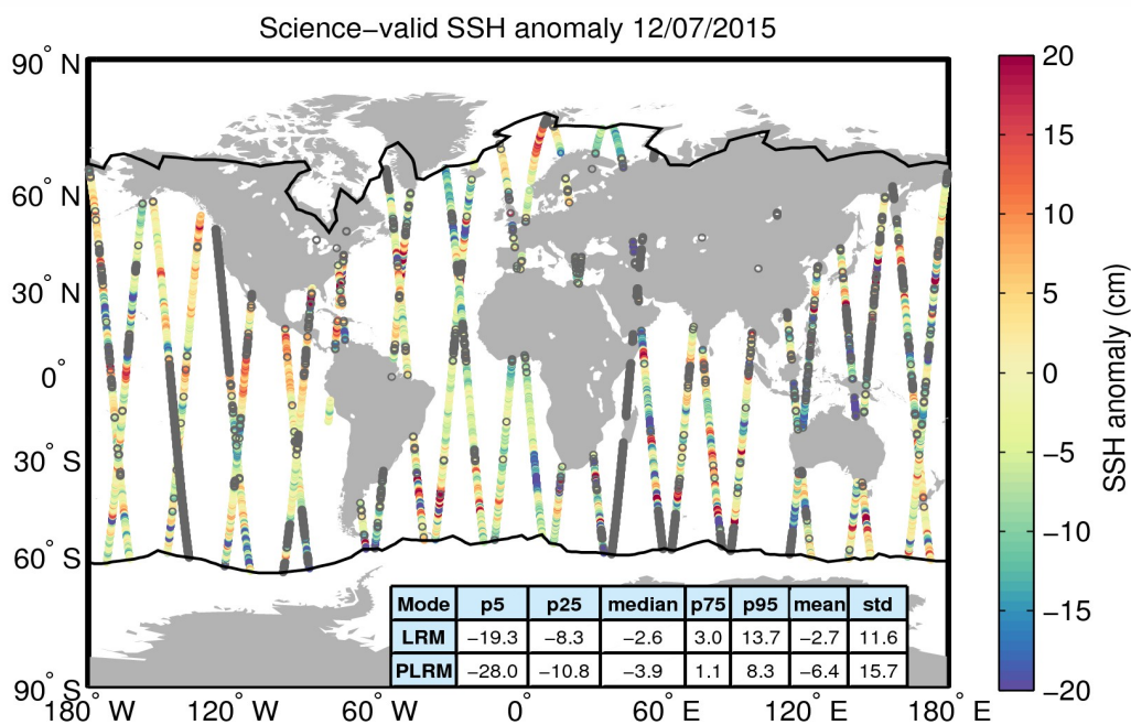
Figure 10. Geographical distribution of science-valid SSH anomaly data over oceans and lakes for 12/07/2015. The statistical values shown in the table refer to the SSH anomaly in cm and are calculated separately for LRM and PLRM regions. The black lines mark the outer limit of the Arctic and Antarctic polar polygons. Gray circles denote records that have been rejected based on the editing criteria described in Table 2.
