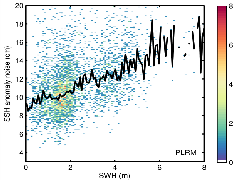
Figure 9. 2D histogram showing flag-valid SSH anomaly noise as a function of SWH for LRM (top) and PLRM (bottom) for 12/07/2015. The black line denotes the median SSH anomaly as a function of SWH.
