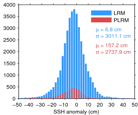
Figure 7. Histogram of flag-valid SSH anomaly over oceans and lakes for LRM (blue) and PLRM (red) for 12/07/2015. The mean ( \mu ) and standard deviation ( \sigma ) are also shown. Note that values outside [-50\ 50] cm are excluded from the histogram for the sake of readability but not from the computation of \mu and \sigma .
