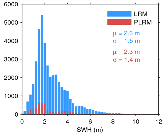
Figure 17. Histogram of flag-valid SWH over oceans and lakes for LRM (blue) and PLRM (red) for 12/07/2015. The mean ( \mu ) and standard deviation ( \sigma ) are also shown. Note that values larger than 12 m are excluded from the histogram for the sake of readability but not from the computation of \mu and \sigma .
