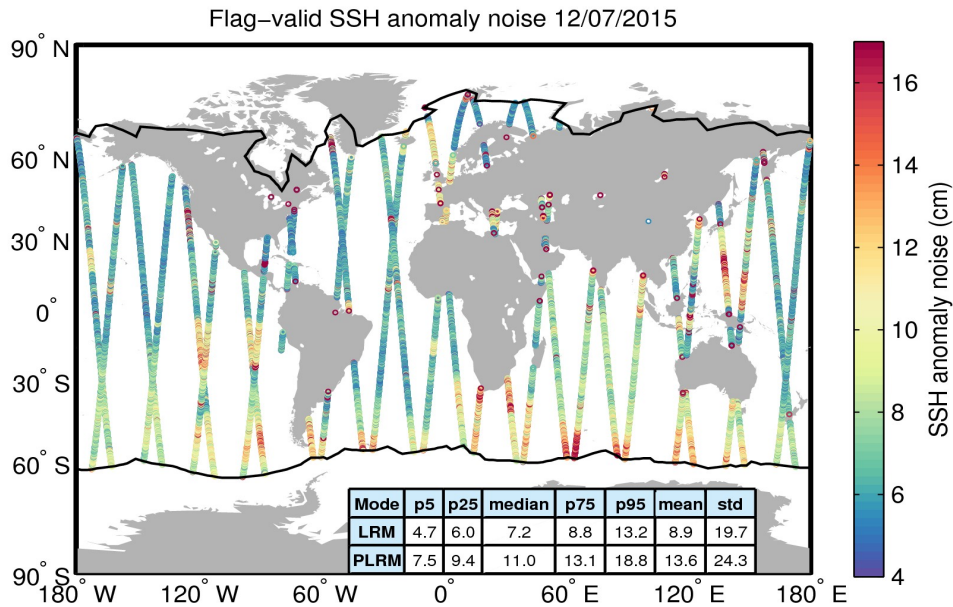
Figure 8. Geographical distribution of flag-valid 20-Hz SSH anomaly measurement noise over oceans and lakes for 12/07/2015. The statistical values shown in the table refer to the SSH anomaly noise and are calculated separately for LRM and PLRM regions. Measurements taken over polar polygons have been excluded from the computation of the statistical values. The black lines mark the outer limit of the Arctic and Antarctic polar polygons.
