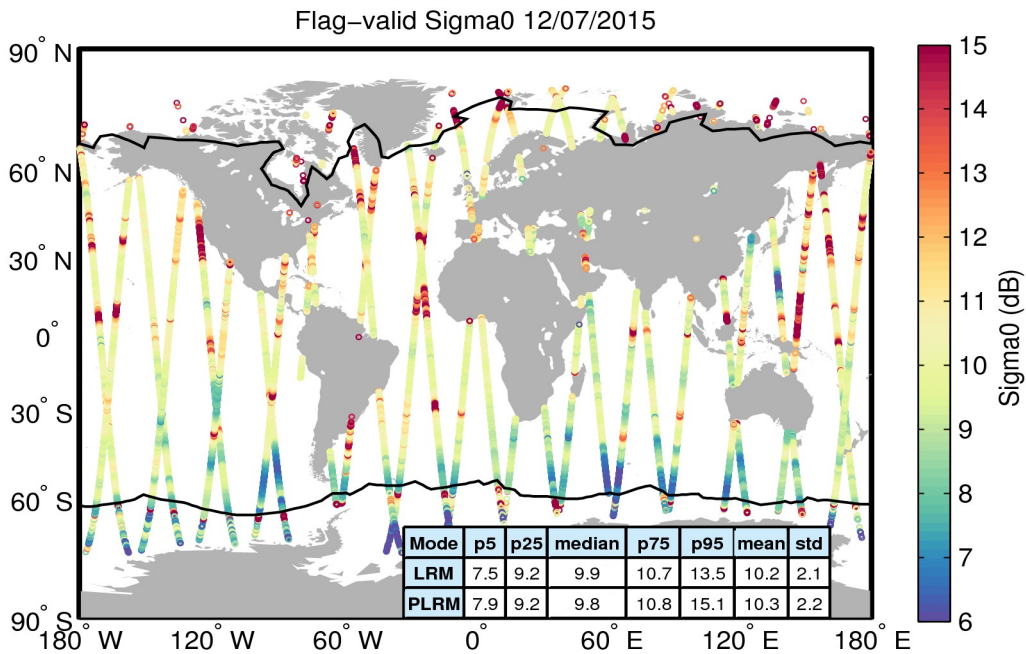
Figure 23. Geographical distribution of flag-valid sigma0 data over oceans and lakes for 12/07/2015. The statistical values shown in the table refer to the sigma0 in dB and are calculated separately for LRM and PLRM regions. Measurements taken over polar polygons have been excluded from the computation of the statistical values. The black lines mark the outer limit of the Arctic and Antarctic polar polygons.
