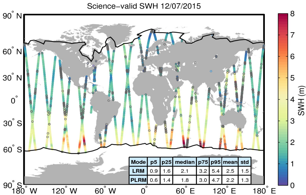
Figure 19. Geographical distribution of science-valid SWH data over oceans and lakes for 12/07/2015. The statistical values shown in the table refer to the SWH in m and are calculated separately for LRM and PLRM regions. The black lines mark the outer limit of the Arctic and Antarctic polar polygons. Gray circles denote records that have been rejected based on the editing criteria described in Table 3.
