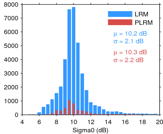
Figure 25. Histogram of flag-valid sigma0 over oceans and lakes for LRM (blue) and PLRM (red) for 12/07/2015. The mean ( \mu ) and standard deviation ( \sigma ) are also shown. Note that values outside [4 20] dB are excluded from the histogram for the sake of readability but not from the computation of \mu and \sigma .
