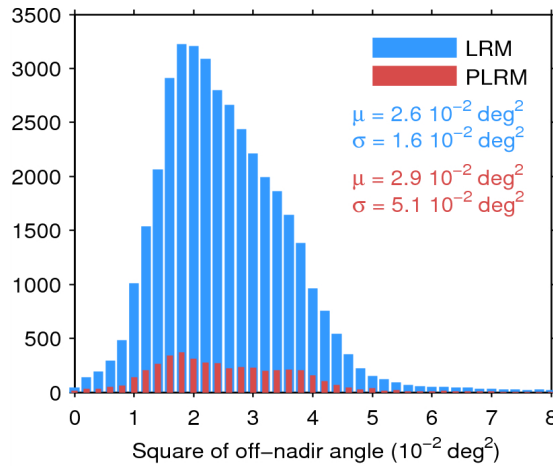
Figure 39. Histogram of flag-valid mispointing over oceans and lakes for LRM (blue) and PLRM (red) for 12/07/2015. Only positive values have been considered. The mean ( \mu ) and standard deviation ( \sigma ) are also shown. Note that values larger than 8 \cdot 10^{-2} \text{ deg}^2 are excluded from the histogram for the sake of readability but not from the computation of \mu and \sigma .
