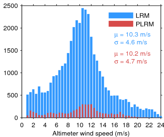
Figure 35. Histogram of science-valid wind over oceans and lakes for LRM (blue) and PLRM (red) for 12/07/2015. The mean ( \mu ) and standard deviation ( \sigma ) are also shown. Note that values larger than 24 m/s are excluded from the histogram for the sake of readability but not from the computation of \mu and \sigma .
