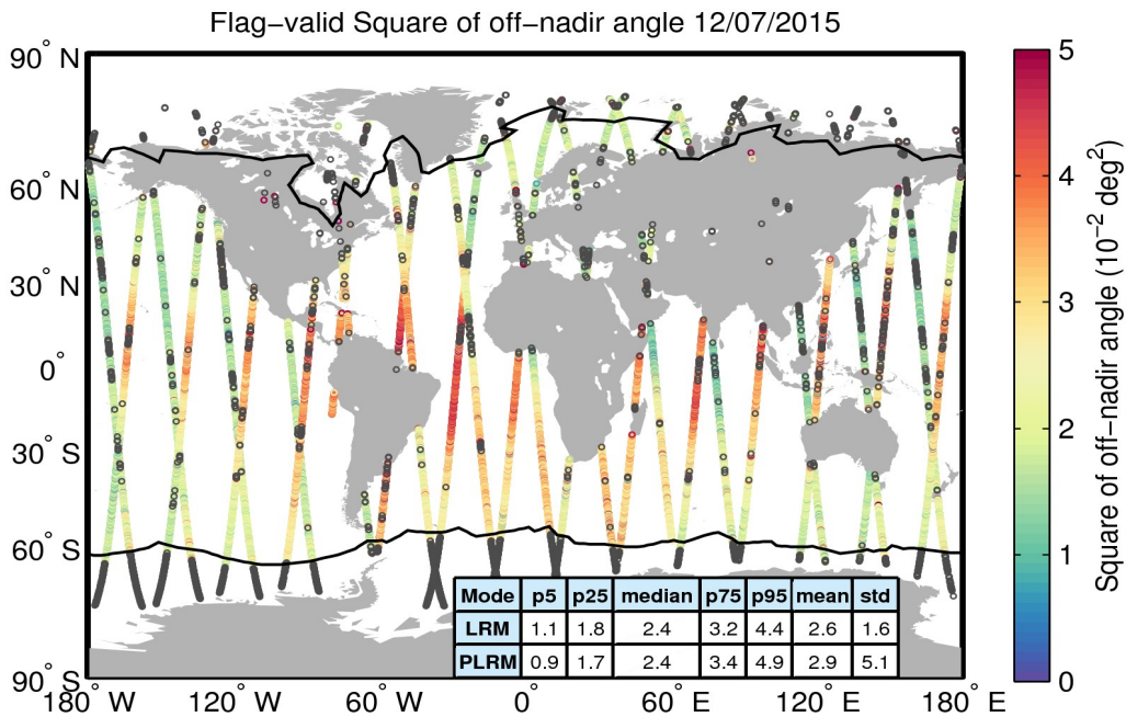
Figure 37. Geographical distribution of flag-valid mispointing data over oceans and lakes for 12/07/2015. The statistical values shown in the table refer to the mispointing in 10^{-2} deg 2 and are calculated separately for LRM and PLRM regions. Measurements taken over polar polygons have been excluded from the computation of the statistical values. The black lines mark the outer limit of the Arctic and Antarctic polar polygons. Gray circles denote negative values.
