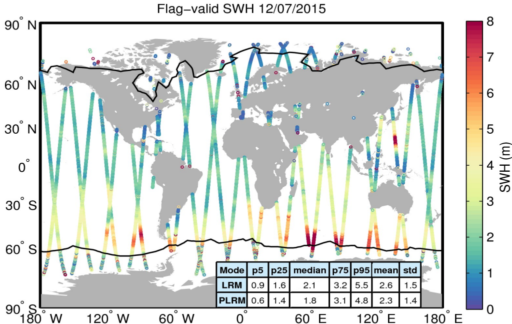
Figure 15. Geographical distribution of flag-valid SWH data over oceans and lakes for 12/07/2015. The statistical values shown in the table refer to the SWH in m and are calculated separately for LRM and PLRM regions. Measurements taken over polar polygons have been excluded from the computation of the statistical values. The black lines mark the outer limit of the Arctic and Antarctic polar polygons.
