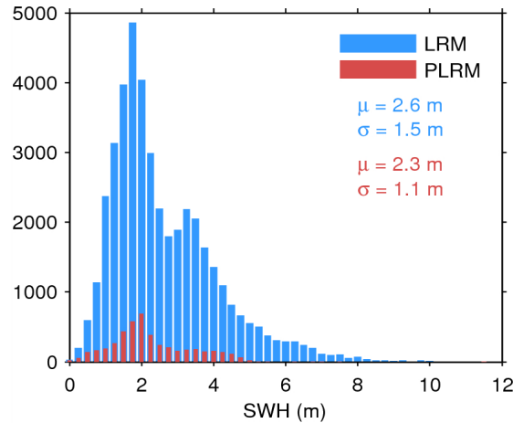
Figure 17. Histogram of flag-valid SWH over oceans and lakes for LRM (blue) and PLRM (red) for 11/07/2015. The mean ( \mu ) and standard deviation ( \sigma ) are also shown. Note that values larger than 12 m are excluded from the histogram for the sake of readability but not from the computation of \mu and \sigma .
