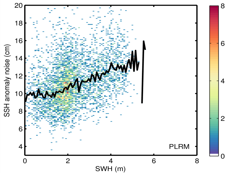
Figure 9. 2D histogram showing flag-valid SSH anomaly noise as a function of SWH for LRM (top) and PLRM (bottom) for 11/07/2015. The black line denotes the median SSH anomaly as a function of SWH.
