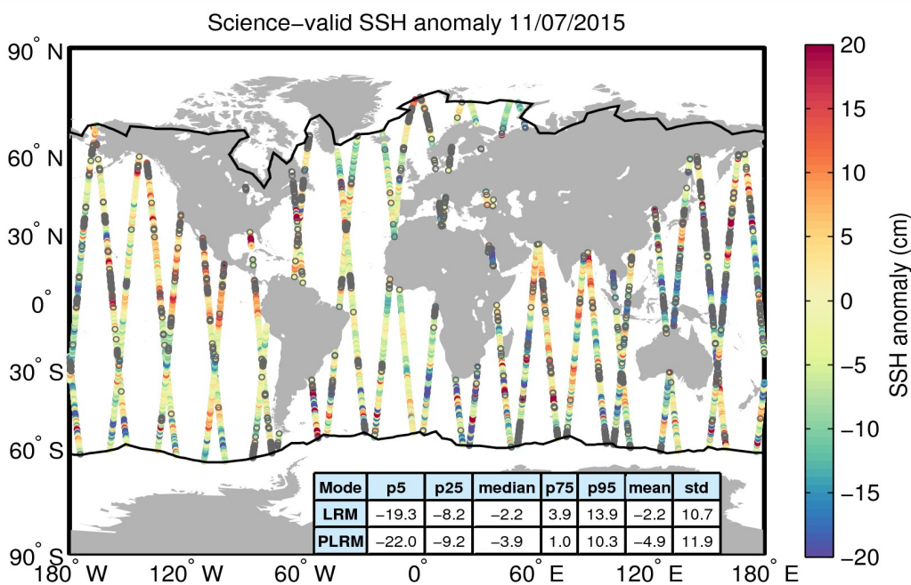
Figure 10. Geographical distribution of science-valid SSH anomaly data over oceans and lakes for 11/07/2015. The statistical values shown in the table refer to the SSH anomaly in cm and are calculated separately for LRM and PLRM regions. The black lines mark the outer limit of the Arctic and Antarctic polar polygons. Gray circles denote records that have been rejected based on the editing criteria described in Table 2.
