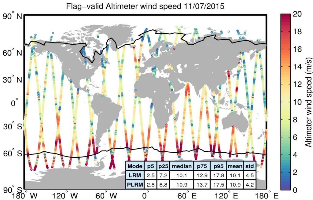
Figure 31. Geographical distribution of flag-valid wind data over oceans and lakes for 11/07/2015. The statistical values shown in the table refer to the wind in m/s and are calculated separately for LRM and PLRM regions. Measurements taken over polar polygons have been excluded from the computation of the statistical values. The black lines mark the outer limit of the Arctic and Antarctic polar polygons.
