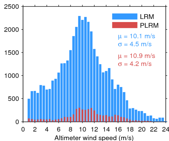
Figure 35. Histogram of science-valid wind over oceans and lakes for LRM (blue) and PLRM (red) for 11/07/2015. The mean ( \mu ) and standard deviation ( \sigma ) are also shown. Note that values larger than 24 m/s are excluded from the histogram for the sake of readability but not from the computation of \mu and \sigma .
