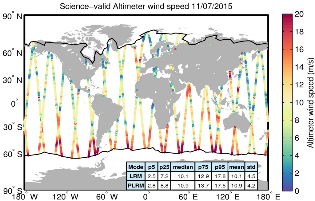
Figure 34. Geographical distribution of science-valid wind data over oceans and lakes for 11/07/2015. The statistical values shown in the table refer to the wind in m/s and are calculated separately for LRM and PLRM regions. The black lines mark the outer limit of the Arctic and Antarctic polar polygons. Gray circles denote records that have been rejected based on the editing criteria described in Table 5.
