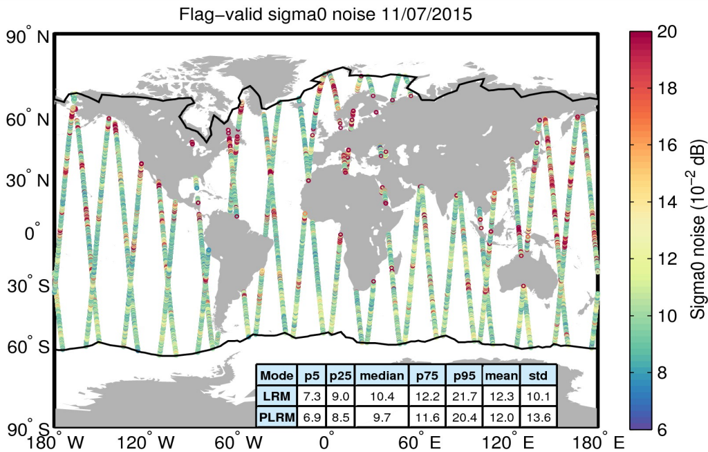
Figure 26. Geographical distribution of flag-valid 20-Hz sigma0 measurement noise over oceans and lakes for 11/07/2015. The statistical values shown in the table refer to the sigma0 noise and are calculated separately for LRM and PLRM regions. Measurements taken over polar polygons have been excluded from the computation of the statistical values. The black lines mark the outer limit of the Arctic and Antarctic polar polygons.
