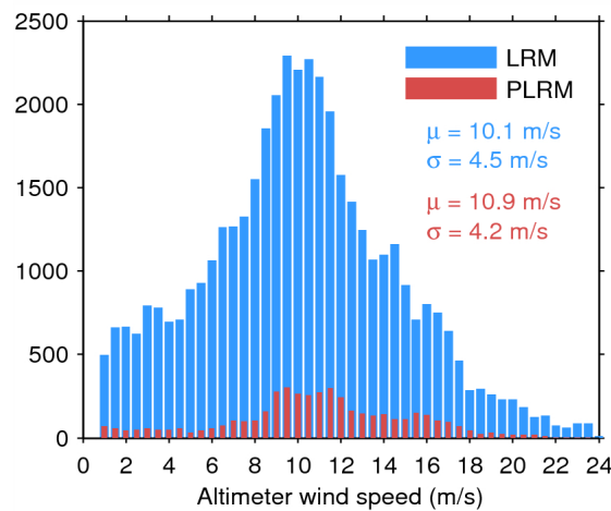
Figure 33. Histogram of flag-valid wind over oceans and lakes for LRM (blue) and PLRM (red) for 11/07/2015. The mean ( \mu ) and standard deviation ( \sigma ) are also shown. Note that values larger than 24 m/s are excluded from the histogram for the sake of readability but not from the computation of \mu and \sigma .
