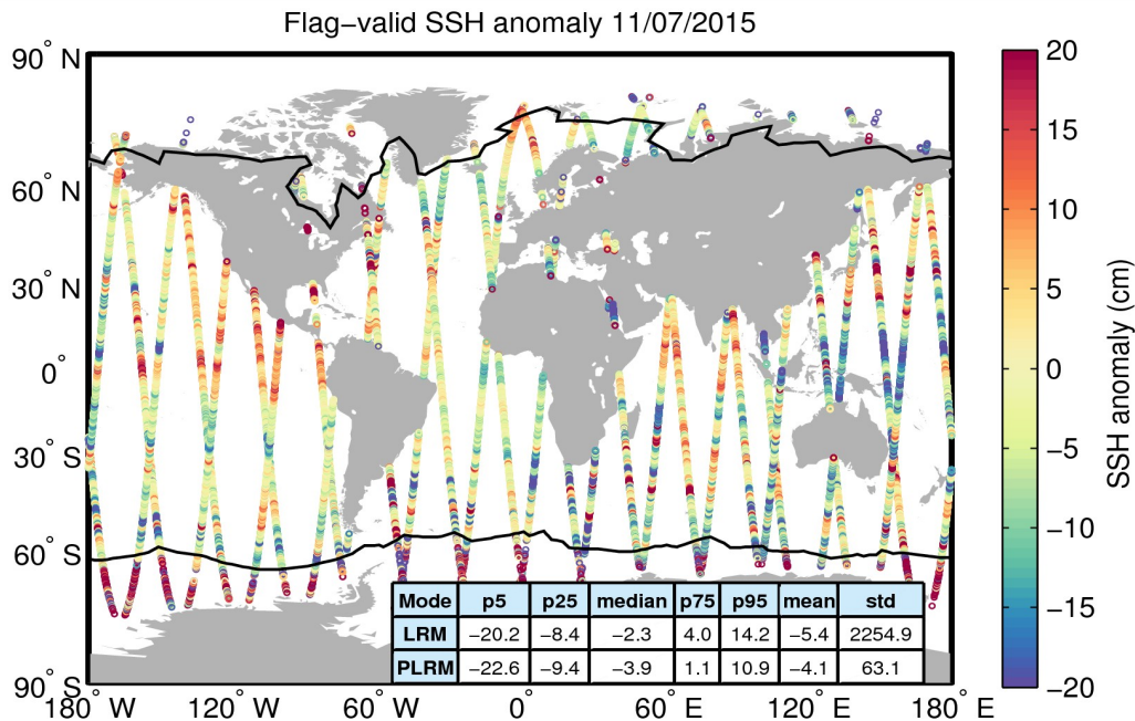
Figure 5. Geographical distribution of flag-valid 1-Hz SSH anomaly data over oceans and lakes for 11/07/2015. The statistical values shown in the table refer to the SSH anomaly in cm and are calculated separately for LRM and PLRM regions. Measurements taken over polar polygons have been excluded from the computation of the statistical values. The black lines mark the outer limit of the Arctic and Antarctic polar polygons.
