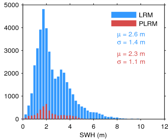
Figure 20. Histogram of science-valid SWH over oceans and lakes for LRM (blue) and PLRM (red) for 11/07/2015. The mean ( \mu ) and standard deviation ( \sigma ) are also shown. Note that values larger than 12 m are excluded from the histogram for the sake of readability but not from the computation of \mu and \sigma .
