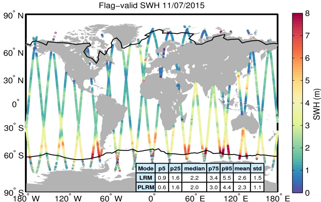
Figure 15. Geographical distribution of flag-valid SWH data over oceans and lakes for 11/07/2015. The statistical values shown in the table refer to the SWH in m and are calculated separately for LRM and PLRM regions. Measurements taken over polar polygons have been excluded from the computation of the statistical values. The black lines mark the outer limit of the Arctic and Antarctic polar polygons.
