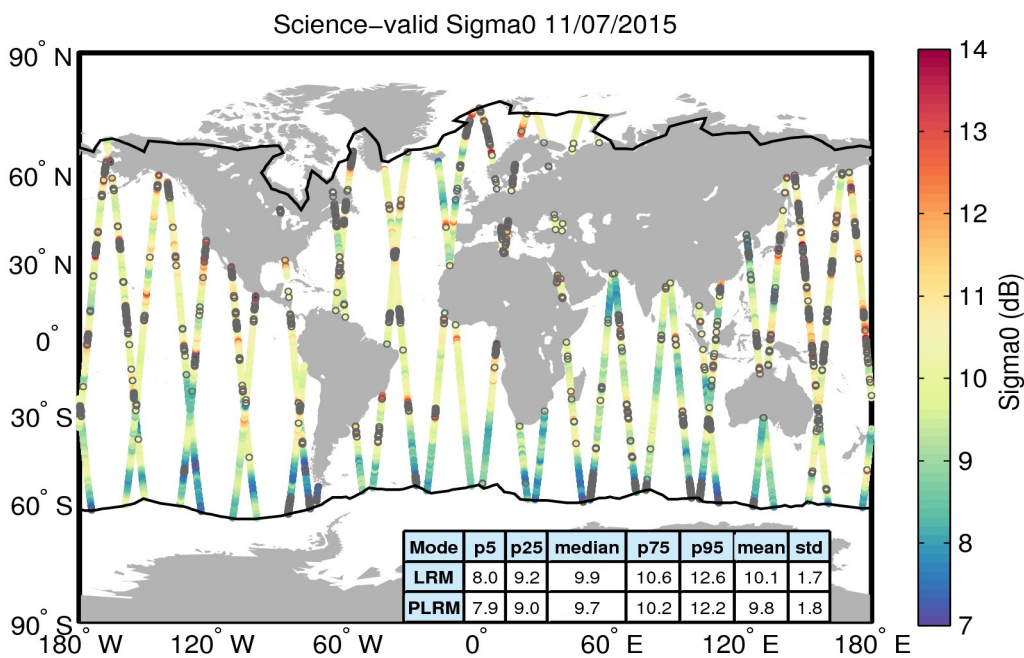
Figure 27. Geographical distribution of science-valid sigma0 data over oceans and lakes for 11/07/2015. The statistical values shown in the table refer to the sigma0 in dB and are calculated separately for LRM and PLRM regions. The black lines mark the outer limit of the Arctic and Antarctic polar polygons. Gray circles denote records that have been rejected based on the editing criteria described in Table 4.
