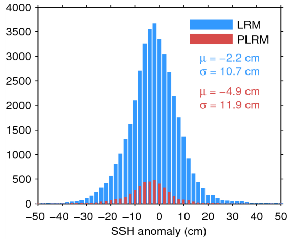
Figure 11. Histogram of science-valid SSH anomaly over oceans and lakes for LRM (blue) and PLRM (red) for 11/07/2015. The mean ( \mu ) and standard deviation ( \sigma ) are also shown. Note that values outside [-50\ 50] cm are excluded from the histogram for the sake of readability but not from the computation of \mu and \sigma .
