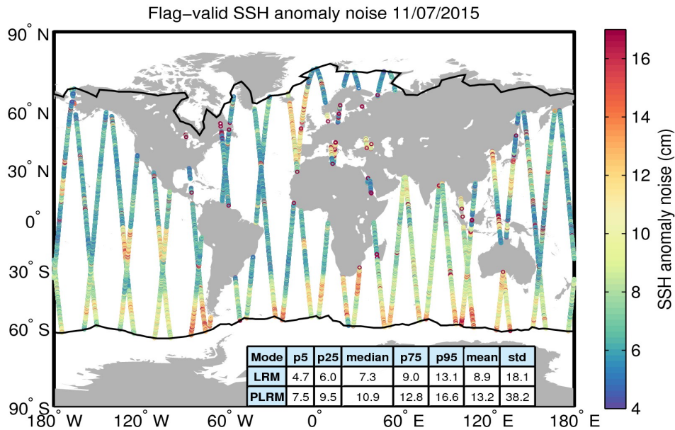
Figure 8. Geographical distribution of flag-valid 20-Hz SSH anomaly measurement noise over oceans and lakes for 11/07/2015. The statistical values shown in the table refer to the SSH anomaly noise and are calculated separately for LRM and PLRM regions. Measurements taken over polar polygons have been excluded from the computation of the statistical values. The black lines mark the outer limit of the Arctic and Antarctic polar polygons.
