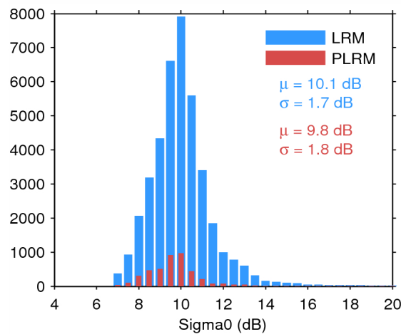
Figure 28. Histogram of science-valid sigma0 over oceans and lakes for LRM (blue) and PLRM (red) for 11/07/2015. The mean ( \mu ) and standard deviation ( \sigma ) are also shown. Note that values outside [4 20] dB are excluded from the histogram for the sake of readability but not from the computation of \mu and \sigma .
