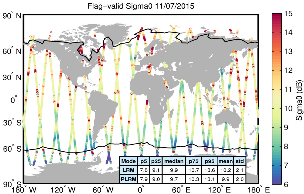
Figure 23. Geographical distribution of flag-valid sigma0 data over oceans and lakes for 11/07/2015. The statistical values shown in the table refer to the sigma0 in dB and are calculated separately for LRM and PLRM regions. Measurements taken over polar polygons have been excluded from the computation of the statistical values. The black lines mark the outer limit of the Arctic and Antarctic polar polygons.
