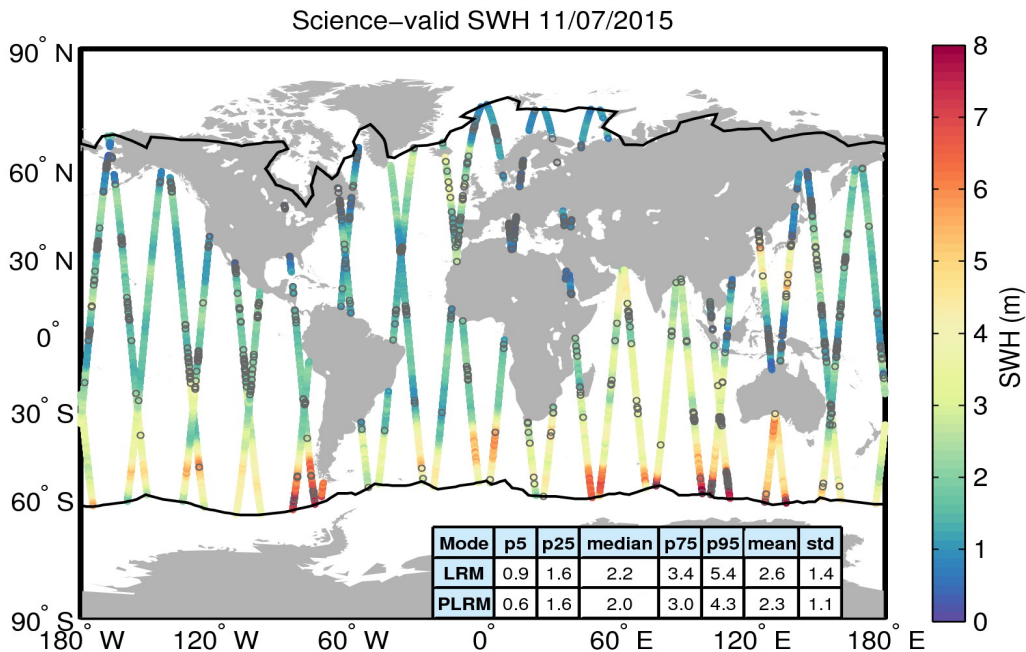
Figure 19. Geographical distribution of science-valid SWH data over oceans and lakes for 11/07/2015. The statistical values shown in the table refer to the SWH in m and are calculated separately for LRM and PLRM regions. The black lines mark the outer limit of the Arctic and Antarctic polar polygons. Gray circles denote records that have been rejected based on the editing criteria described in Table 3.
