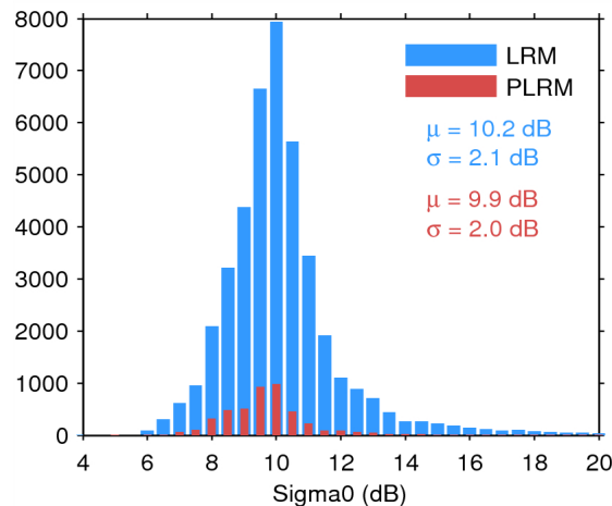
Figure 25. Histogram of flag-valid sigma0 over oceans and lakes for LRM (blue) and PLRM (red) for 11/07/2015. The mean ( \mu ) and standard deviation ( \sigma ) are also shown. Note that values outside [4 20] dB are excluded from the histogram for the sake of readability but not from the computation of \mu and \sigma .
