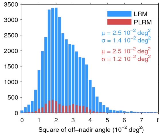
Figure 39. Histogram of flag-valid mispointing over oceans and lakes for LRM (blue) and PLRM (red) for 11/07/2015. Only positive values have been considered. The mean ( \mu ) and standard deviation ( \sigma ) are also shown. Note that values larger than 8 \cdot 10^{-2} \text{ deg}^2 are excluded from the histogram for the sake of readability but not from the computation of \mu and \sigma .
