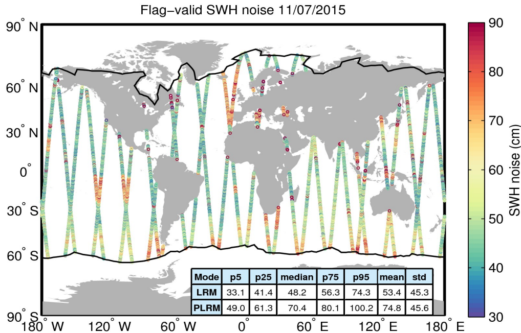
Figure 18. Geographical distribution of flag-valid 20-Hz SWH measurement noise over oceans and lakes for 11/07/2015. The statistical values shown in the table refer to the SWH noise and are calculated separately for LRM and PLRM regions. Measurements taken over polar polygons have been excluded from the computation of the statistical values. The black lines mark the outer limit of the Arctic and Antarctic polar polygons.
