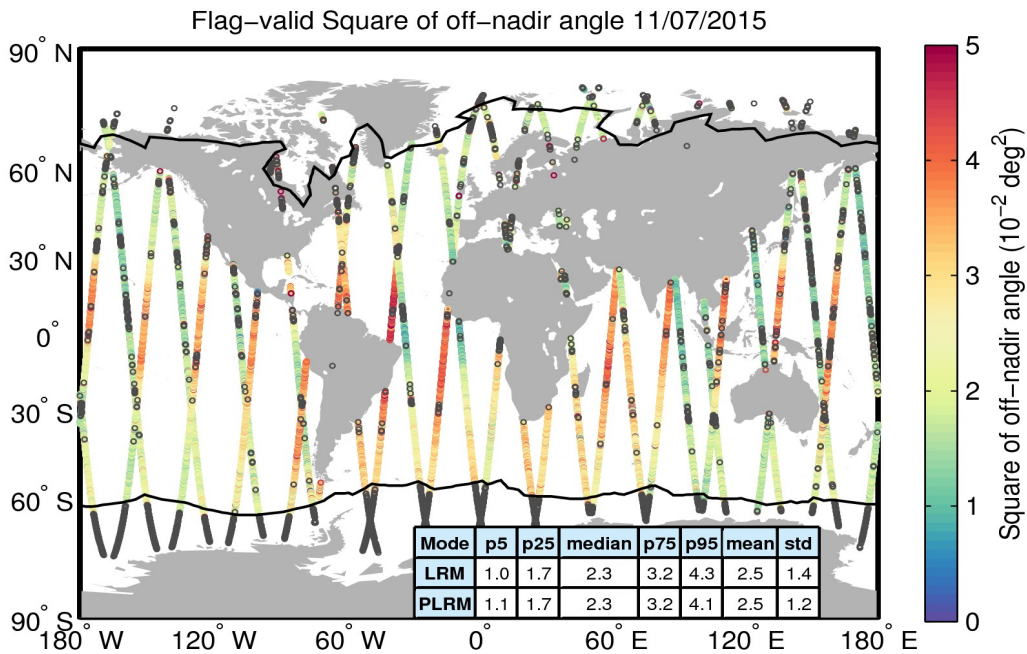
Figure 37. Geographical distribution of flag-valid mispointing data over oceans and lakes for 11/07/2015. The statistical values shown in the table refer to the mispointing in 10^{-2} \text{ deg}^2 and are calculated separately for LRM and PLRM regions. Measurements taken over polar polygons have been excluded from the computation of the statistical values. The black lines mark the outer limit of the Arctic and Antarctic polar polygons. Gray circles denote negative values.
