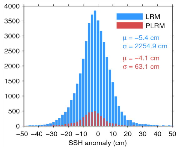
Figure 7. Histogram of flag-valid SSH anomaly over oceans and lakes for LRM (blue) and PLRM (red) for 11/07/2015. The mean ( \mu ) and standard deviation ( \sigma ) are also shown. Note that values outside [-50\ 50] cm are excluded from the histogram for the sake of readability but not from the computation of \mu and \sigma .
