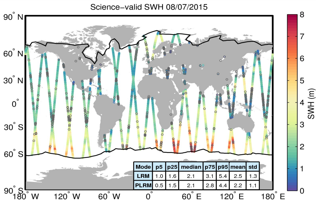
Figure 19. Geographical distribution of science-valid SWH data over oceans and lakes for 08/07/2015. The statistical values shown in the table refer to the SWH in m and are calculated separately for LRM and PLRM regions. The black lines mark the outer limit of the Arctic and Antarctic polar polygons. Gray circles denote records that have been rejected based on the editing criteria described in Table 3.
