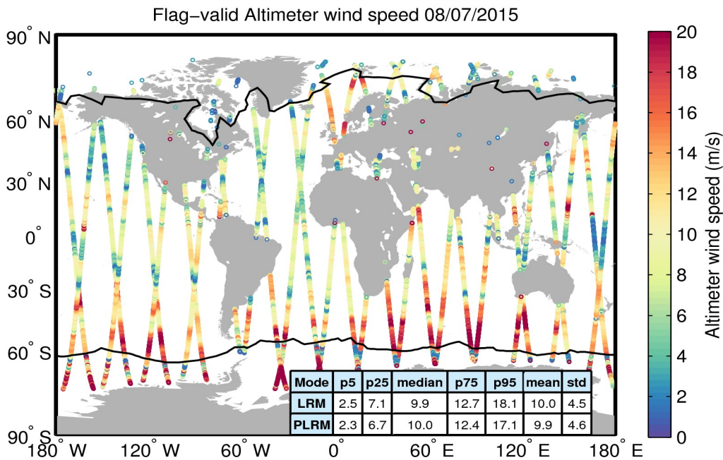
Figure 31. Geographical distribution of flag-valid wind data over oceans and lakes for 08/07/2015. The statistical values shown in the table refer to the wind in m/s and are calculated separately for LRM and PLRM regions. Measurements taken over polar polygons have been excluded from the computation of the statistical values. The black lines mark the outer limit of the Arctic and Antarctic polar polygons.
