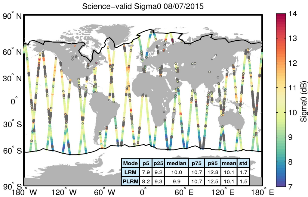
Figure 27. Geographical distribution of science-valid sigma0 data over oceans and lakes for 08/07/2015. The statistical values shown in the table refer to the sigma0 in dB and are calculated separately for LRM and PLRM regions. The black lines mark the outer limit of the Arctic and Antarctic polar polygons. Gray circles denote records that have been rejected based on the editing criteria described in Table 4.
