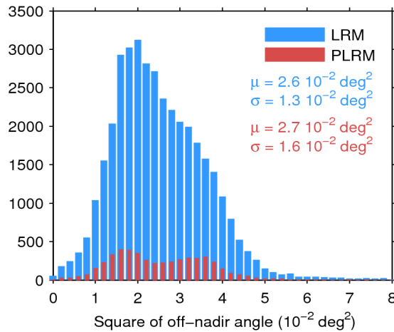
Figure 39. Histogram of flag-valid mispointing over oceans and lakes for LRM (blue) and PLRM (red) for 08/07/2015. Only positive values have been considered. The mean ( \mu ) and standard deviation ( \sigma ) are also shown. Note that values larger than 8 \cdot 10^{-2} \text{ deg}^2 are excluded from the histogram for the sake of readability but not from the computation of \mu and \sigma .
