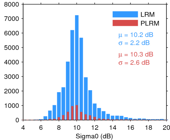
Figure 25. Histogram of flag-valid sigma0 over oceans and lakes for LRM (blue) and PLRM (red) for 08/07/2015. The mean ( \mu ) and standard deviation ( \sigma ) are also shown. Note that values outside [4 20] dB are excluded from the histogram for the sake of readability but not from the computation of \mu and \sigma .
