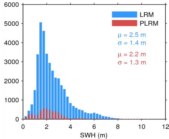
Figure 17. Histogram of flag-valid SWH over oceans and lakes for LRM (blue) and PLRM (red) for 08/07/2015. The mean ( \mu ) and standard deviation ( \sigma ) are also shown. Note that values larger than 12 m are excluded from the histogram for the sake of readability but not from the computation of \mu and \sigma .
