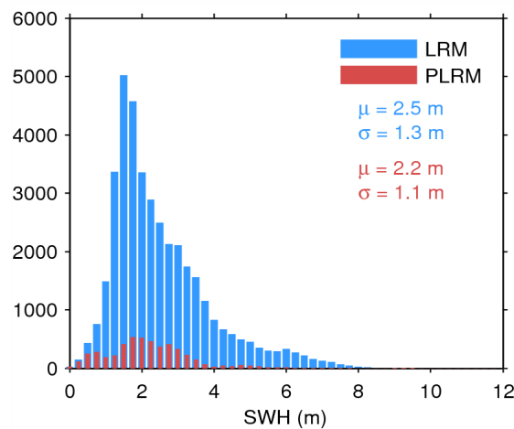
Figure 20. Histogram of science-valid SWH over oceans and lakes for LRM (blue) and PLRM (red) for 08/07/2015. The mean ( \mu ) and standard deviation ( \sigma ) are also shown. Note that values larger than 12 m are excluded from the histogram for the sake of readability but not from the computation of \mu and \sigma .
