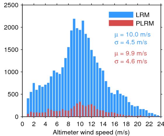
Figure 33. Histogram of flag-valid wind over oceans and lakes for LRM (blue) and PLRM (red) for 08/07/2015. The mean ( \mu ) and standard deviation ( \sigma ) are also shown. Note that values larger than 24 m/s are excluded from the histogram for the sake of readability but not from the computation of \mu and \sigma .
