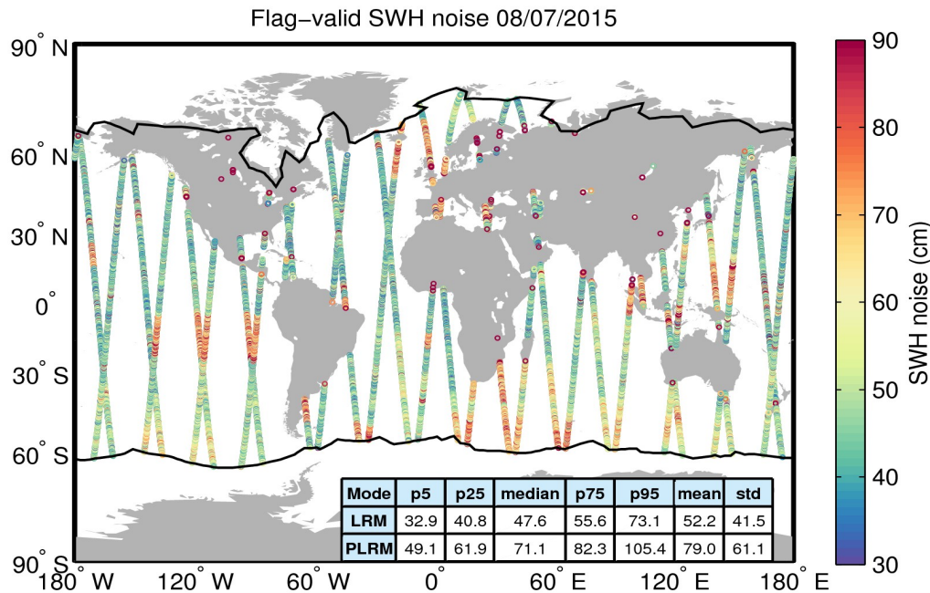
Figure 18. Geographical distribution of flag-valid 20-Hz SWH measurement noise over oceans and lakes for 08/07/2015. The statistical values shown in the table refer to the SWH noise and are calculated separately for LRM and PLRM regions. Measurements taken over polar polygons have been excluded from the computation of the statistical values. The black lines mark the outer limit of the Arctic and Antarctic polar polygons.
