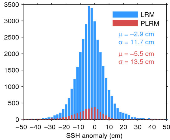
Figure 11. Histogram of science-valid SSH anomaly over oceans and lakes for LRM (blue) and PLRM (red) for 08/07/2015. The mean ( \mu ) and standard deviation ( \sigma ) are also shown. Note that values outside [-50 50] cm are excluded from the histogram for the sake of readability but not from the computation of \mu and \sigma .
