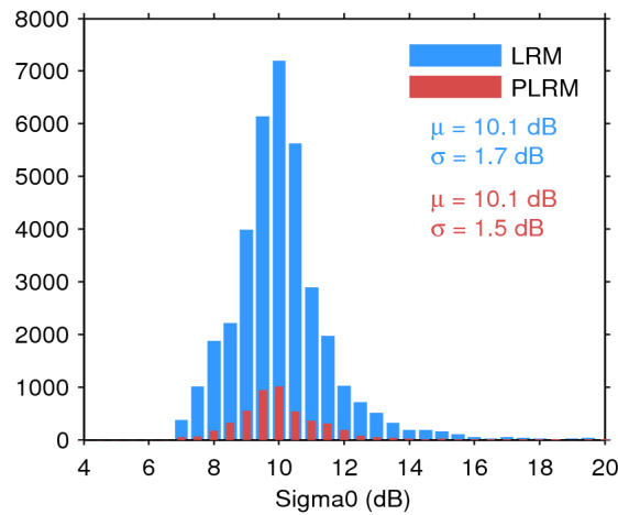
Figure 28. Histogram of science-valid sigma0 over oceans and lakes for LRM (blue) and PLRM (red) for 08/07/2015. The mean ( \mu ) and standard deviation ( \sigma ) are also shown. Note that values outside [4 20] dB are excluded from the histogram for the sake of readability but not from the computation of \mu and \sigma .
