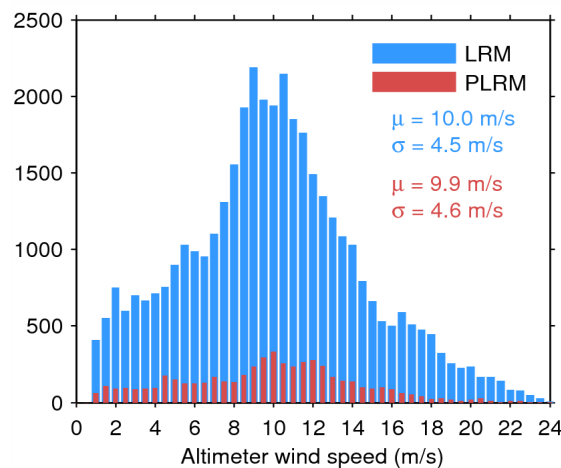
Figure 35. Histogram of science-valid wind over oceans and lakes for LRM (blue) and PLRM (red) for 08/07/2015. The mean ( \mu ) and standard deviation ( \sigma ) are also shown. Note that values larger than 24 m/s are excluded from the histogram for the sake of readability but not from the computation of \mu and \sigma .
