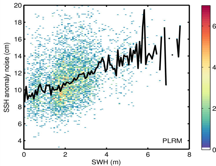
Figure 9. 2D histogram showing flag-valid SSH anomaly noise as a function of SWH for LRM (top) and PLRM (bottom) for 08/07/2015. The black line denotes the median SSH anomaly as a function of SWH.
