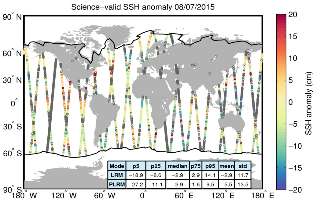
Figure 10. Geographical distribution of science-valid SSH anomaly data over oceans and lakes for 08/07/2015. The statistical values shown in the table refer to the SSH anomaly in cm and are calculated separately for LRM and PLRM regions. The black lines mark the outer limit of the Arctic and Antarctic polar polygons. Gray circles denote records that have been rejected based on the editing criteria described in Table 2.
