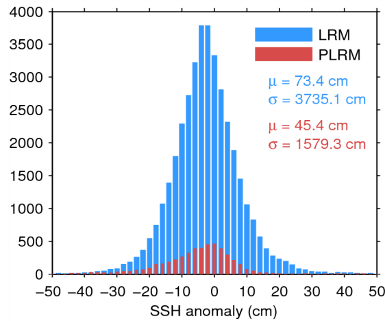
Figure 7. Histogram of flag-valid SSH anomaly over oceans and lakes for LRM (blue) and PLRM (red) for 08/07/2015. The mean ( \mu ) and standard deviation ( \sigma ) are also shown. Note that values outside [-50\ 50] cm are excluded from the histogram for the sake of readability but not from the computation of \mu and \sigma .
