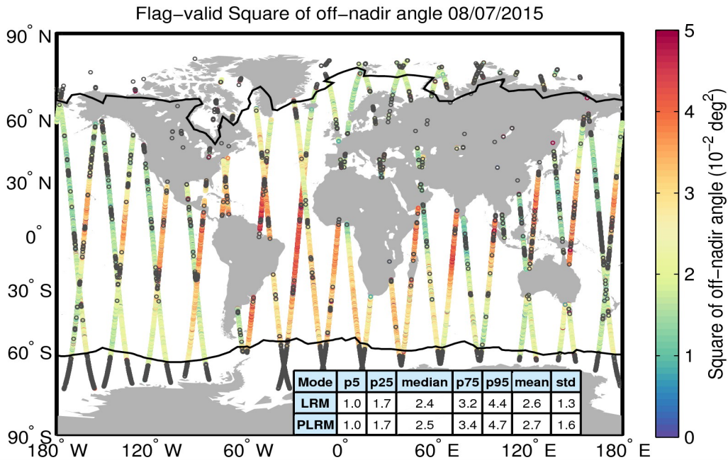
Figure 37. Geographical distribution of flag-valid mispointing data over oceans and lakes for 08/07/2015. The statistical values shown in the table refer to the mispointing in 10^{-2} \text{ deg}^2 and are calculated separately for LRM and PLRM regions. Measurements taken over polar polygons have been excluded from the computation of the statistical values. The black lines mark the outer limit of the Arctic and Antarctic polar polygons. Gray circles denote negative values.
