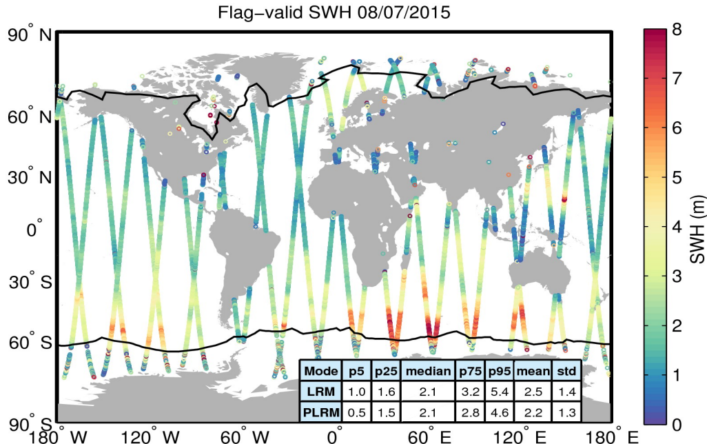
Figure 15. Geographical distribution of flag-valid SWH data over oceans and lakes for 08/07/2015. The statistical values shown in the table refer to the SWH in m and are calculated separately for LRM and PLRM regions. Measurements taken over polar polygons have been excluded from the computation of the statistical values. The black lines mark the outer limit of the Arctic and Antarctic polar polygons.
