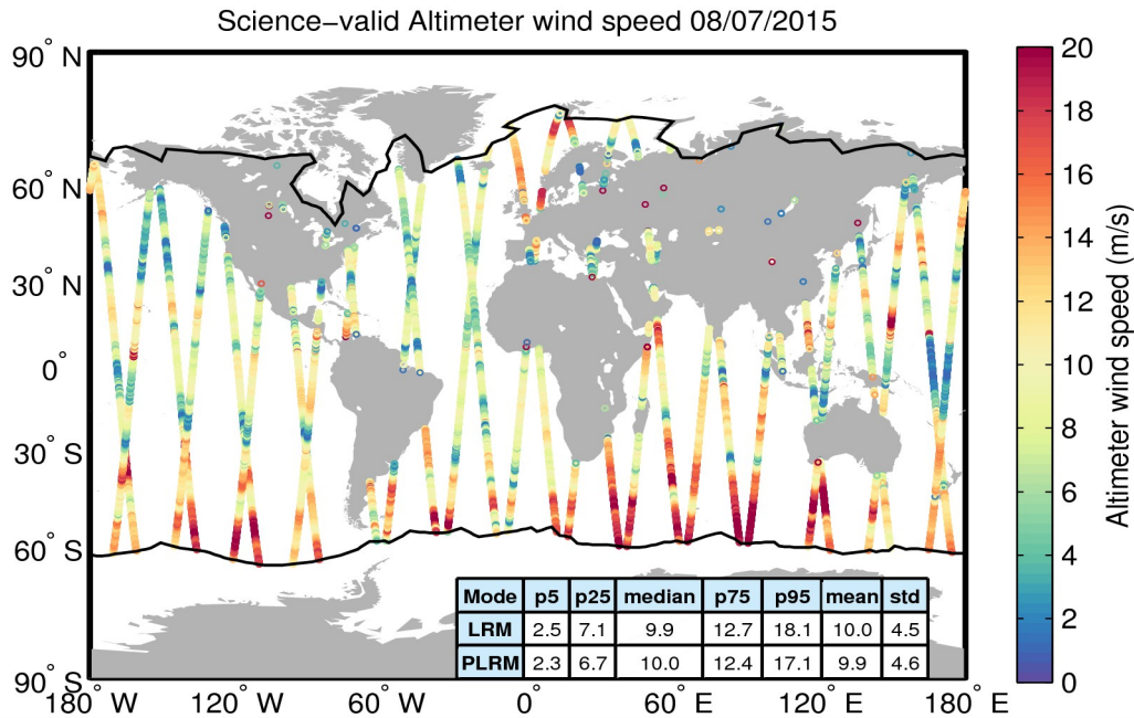
Figure 34. Geographical distribution of science-valid wind data over oceans and lakes for 08/07/2015. The statistical values shown in the table refer to the wind in m/s and are calculated separately for LRM and PLRM regions. The black lines mark the outer limit of the Arctic and Antarctic polar polygons. Gray circles denote records that have been rejected based on the editing criteria described in Table 5.
