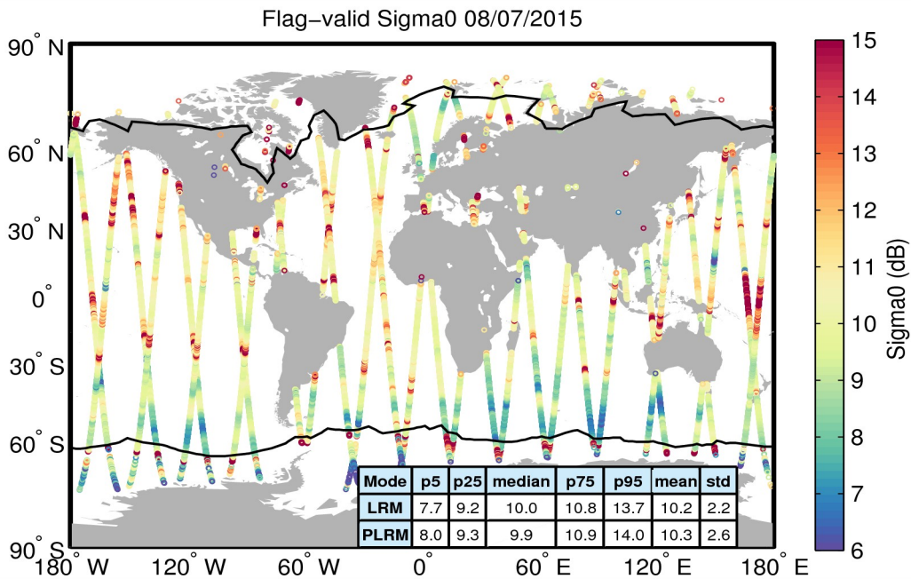
Figure 23. Geographical distribution of flag-valid sigma0 data over oceans and lakes for 08/07/2015. The statistical values shown in the table refer to the sigma0 in dB and are calculated separately for LRM and PLRM regions. Measurements taken over polar polygons have been excluded from the computation of the statistical values. The black lines mark the outer limit of the Arctic and Antarctic polar polygons.
